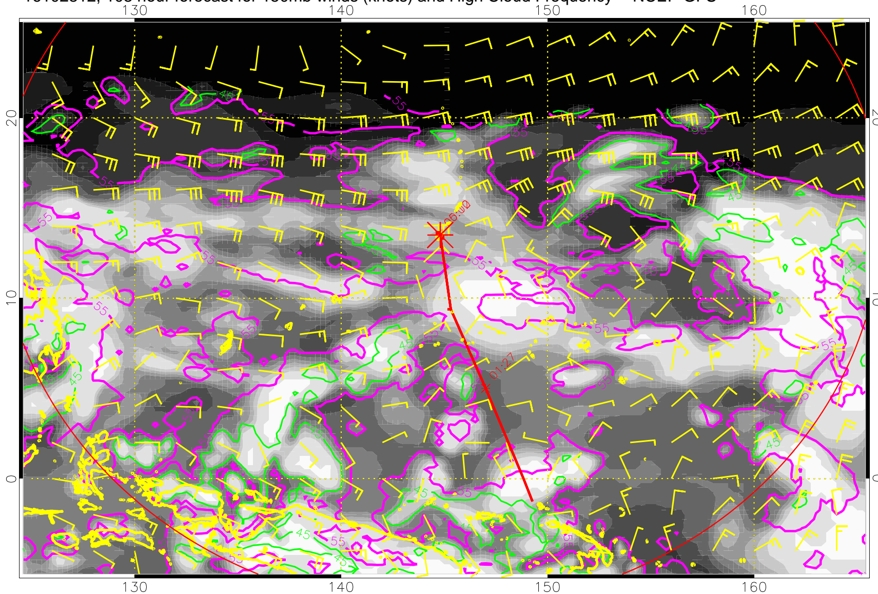
16102812, 108 hour forecast for 150mb winds (knots) and High Cloud Frequency -- NCEP GFS
