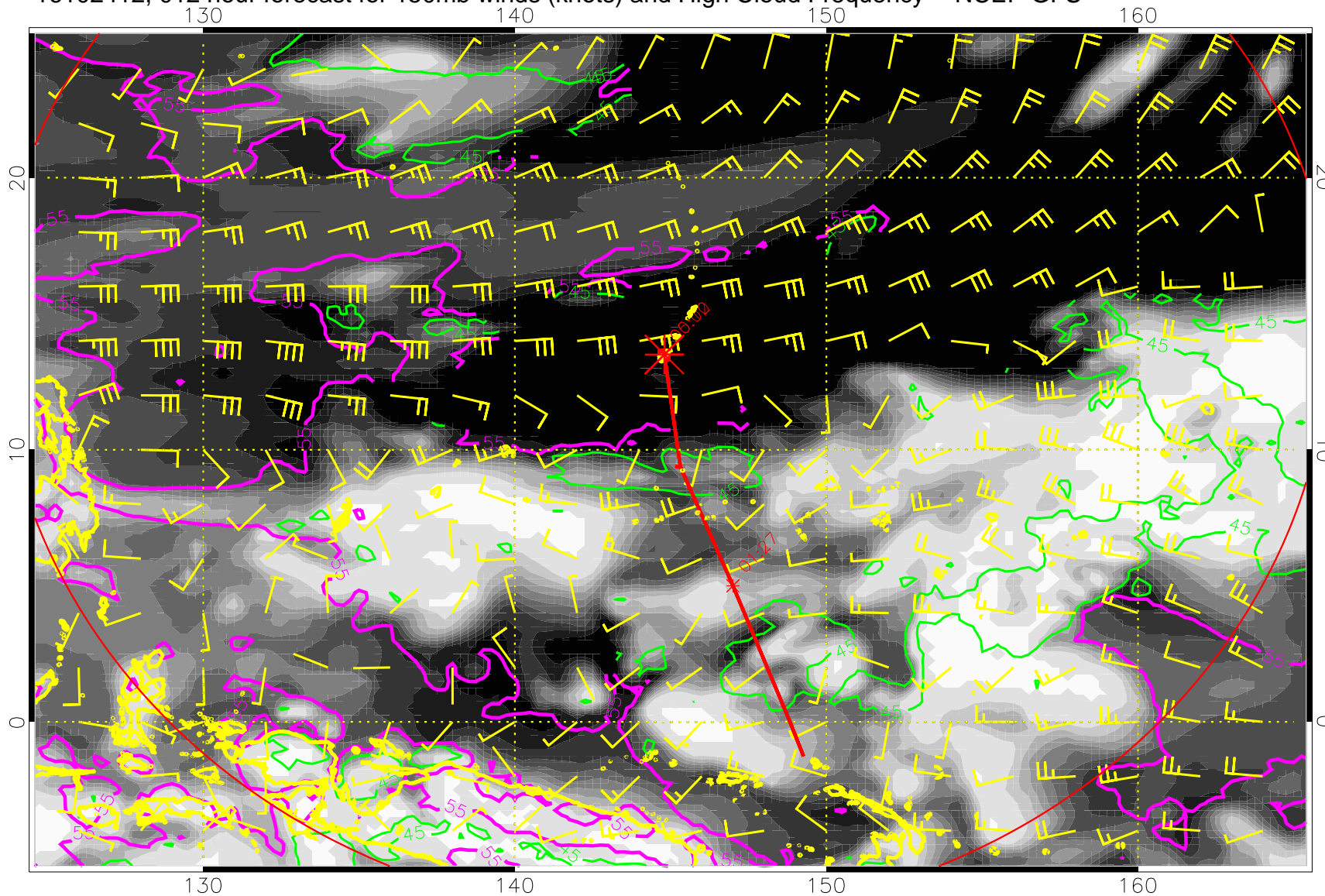
16102412, 012 hour forecast for 150mb winds (knots) and High Cloud Frequency -- NCEP GFS
