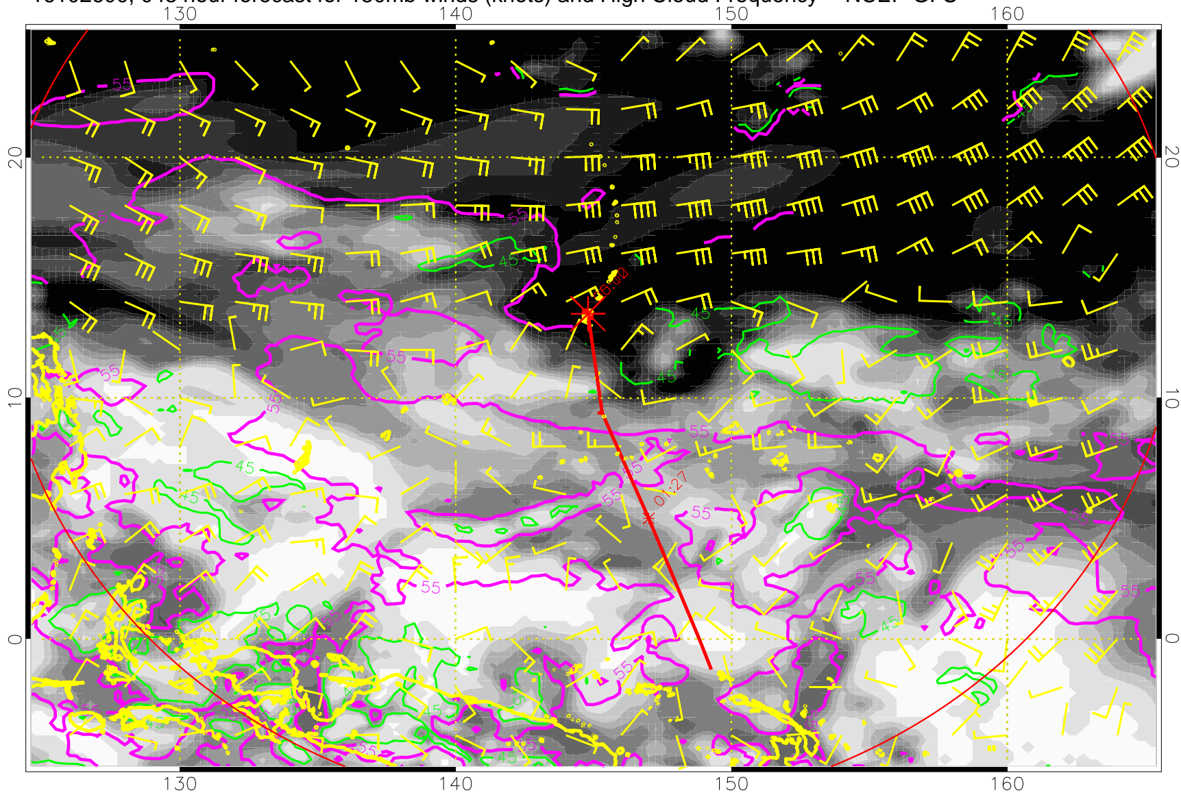
16102600, 048 hour forecast for 150mb winds (knots) and High Cloud Frequency -- NCEP GFS
