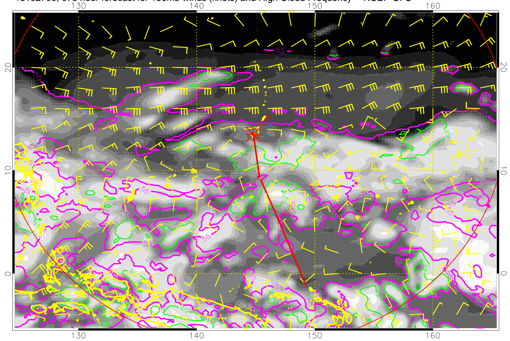
16102706, 078 hour forecast for 150mb winds (knots) and High Cloud Frequency -- NCEP GFS
