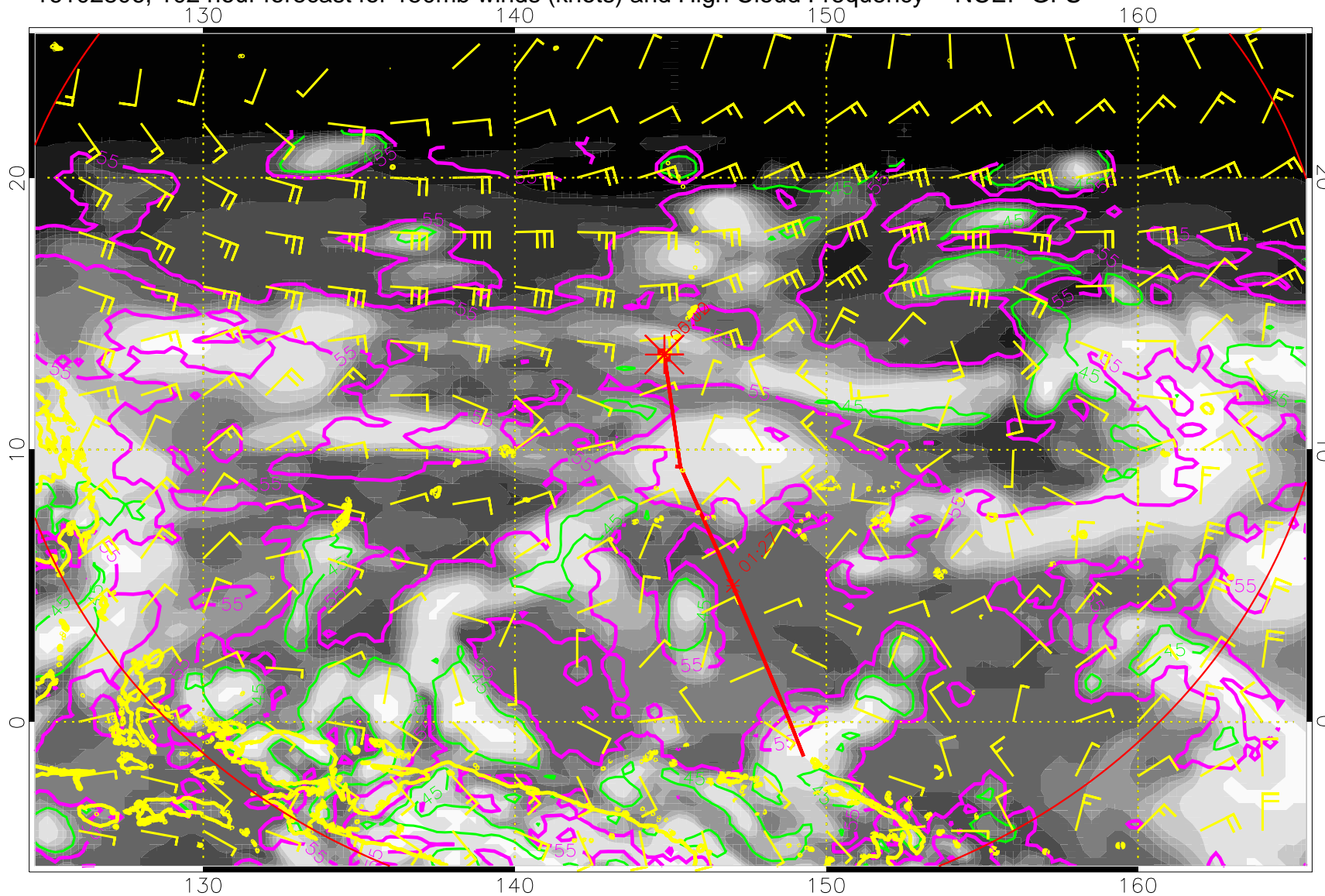
16102806, 102 hour forecast for 150mb winds (knots) and High Cloud Frequency -- NCEP GFS
