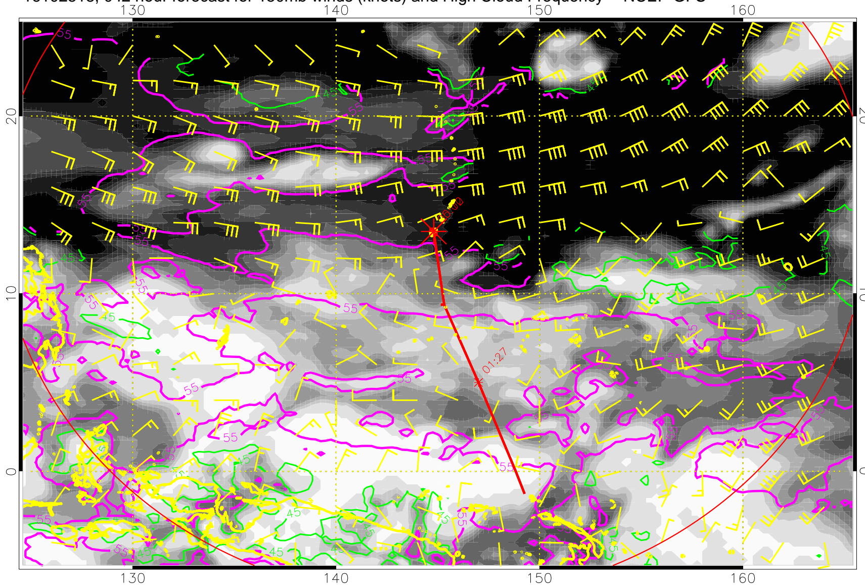
16102518, 042 hour forecast for 150mb winds (knots) and High Cloud Frequency -- NCEP GFS
