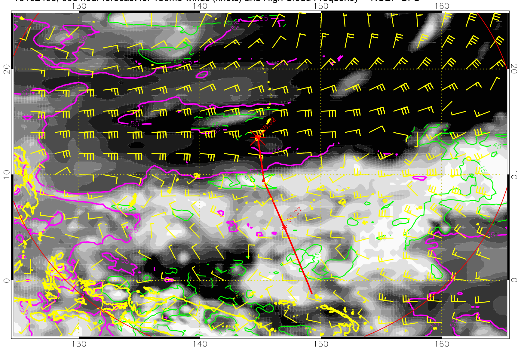
16102406, 006 hour forecast for 150mb winds (knots) and High Cloud Frequency -- NCEP GFS
