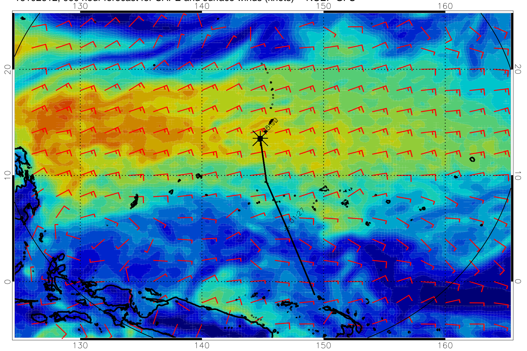
16102612, 060 hour forecast for CAPE and surface winds (knots) -- NCEP GFS
