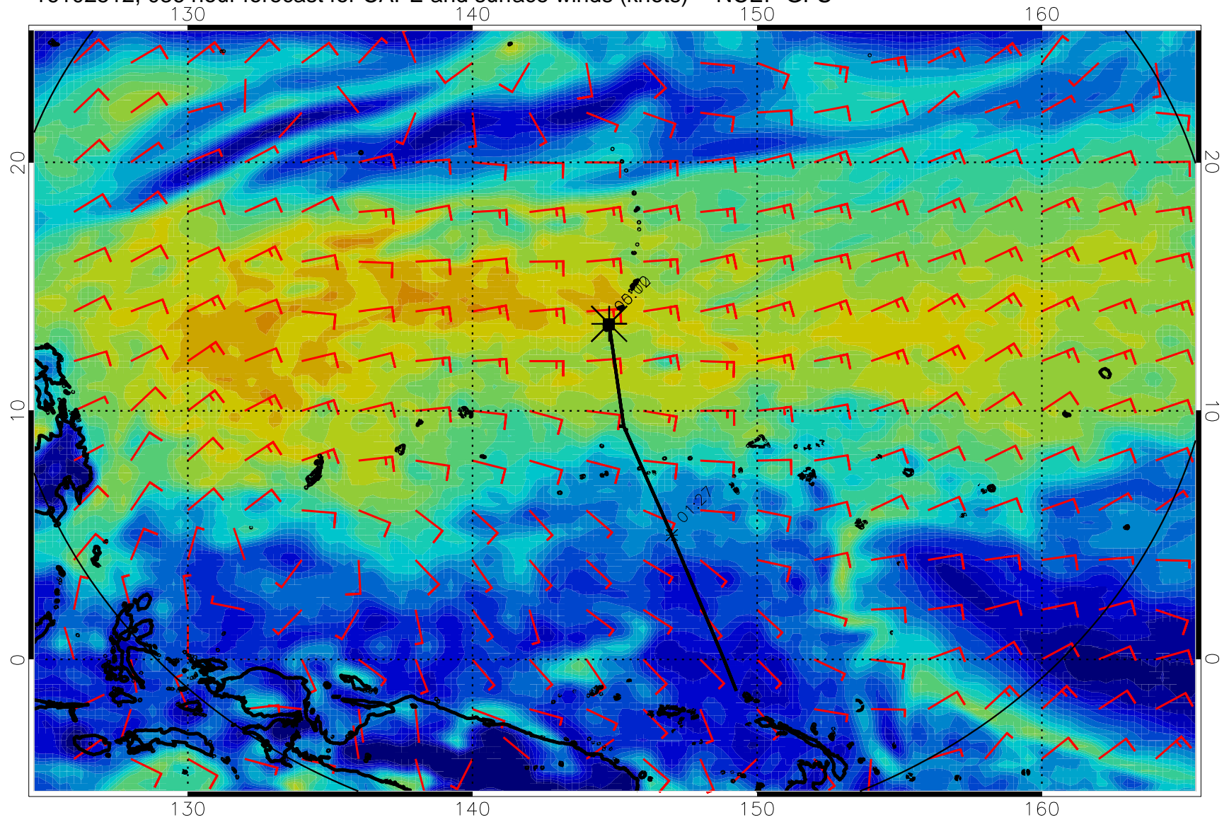
16102512, 036 hour forecast for CAPE and surface winds (knots) -- NCEP GFS
