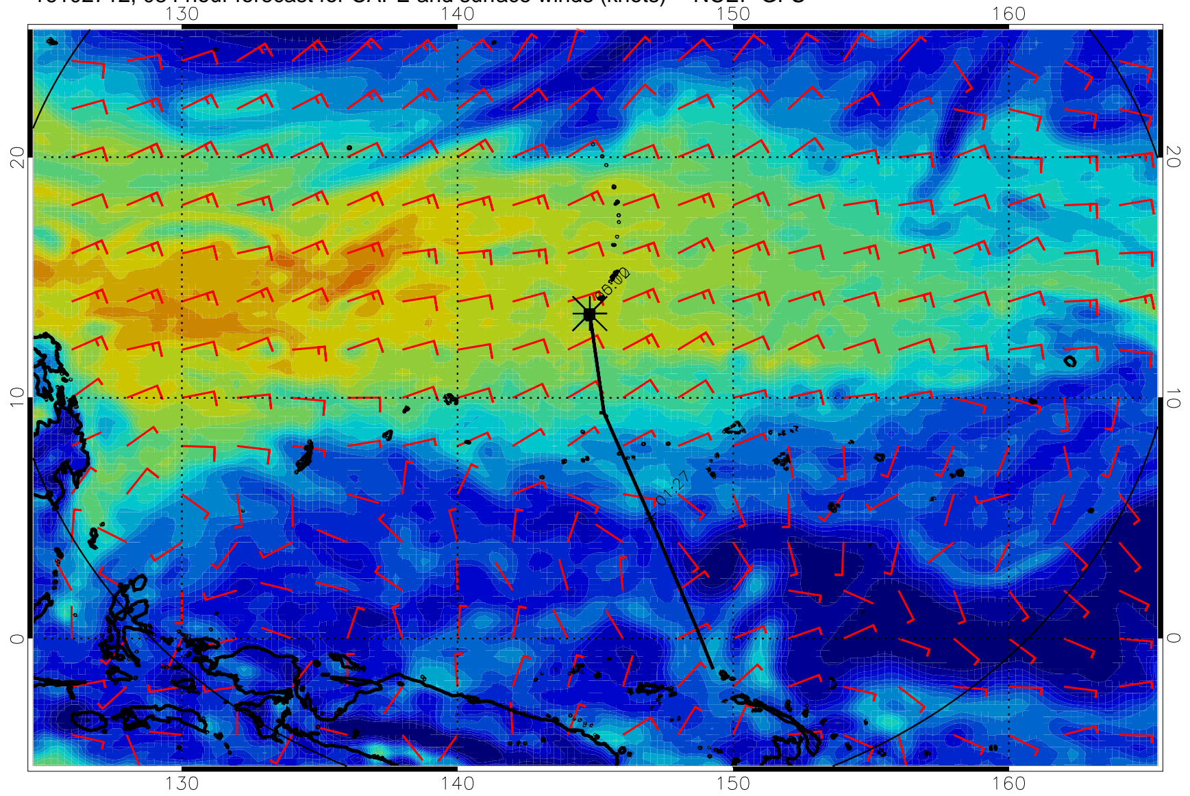
16102712, 084 hour forecast for CAPE and surface winds (knots) -- NCEP GFS
