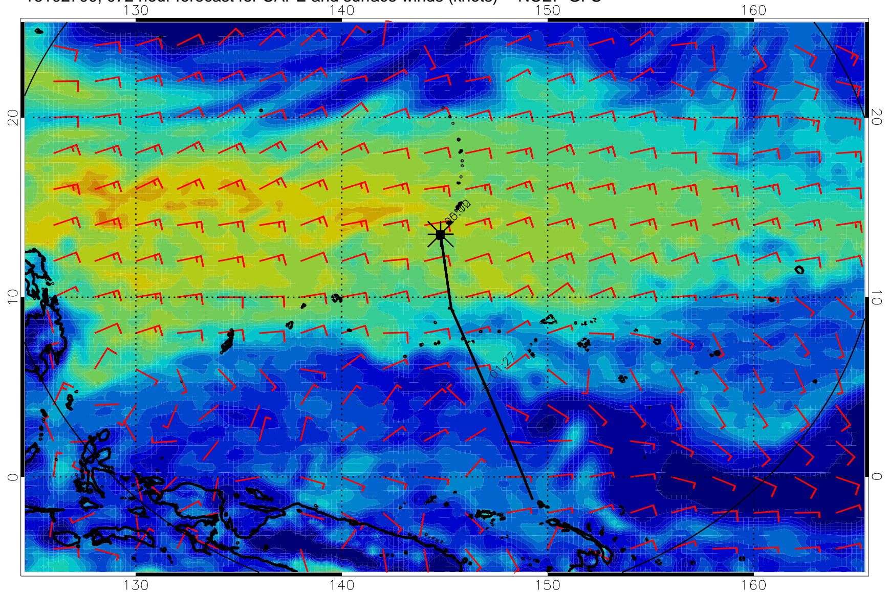
16102700, 072 hour forecast for CAPE and surface winds (knots) -- NCEP GFS
