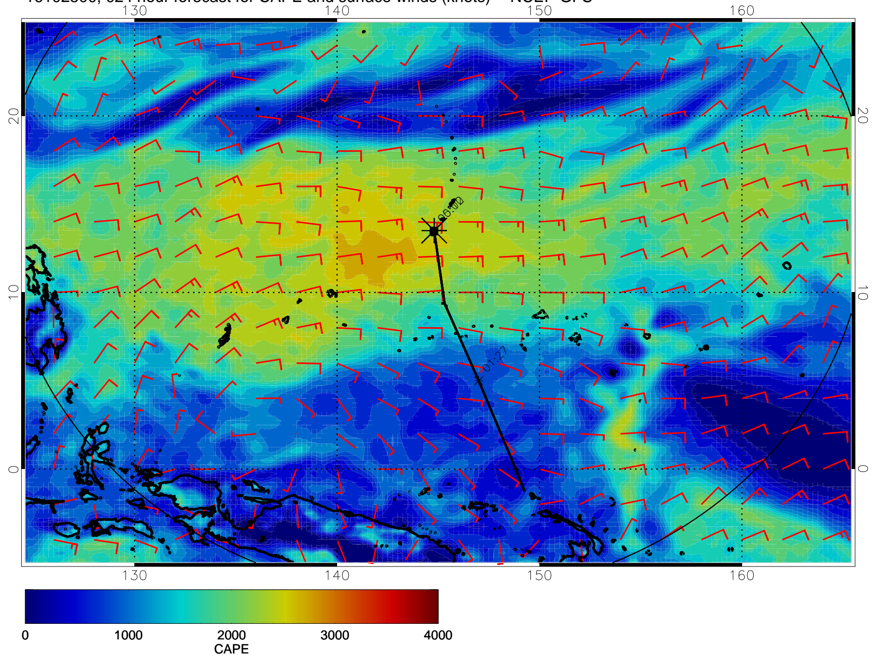
16102500, 024 hour forecast for CAPE and surface winds (knots) -- NCEP GFS
