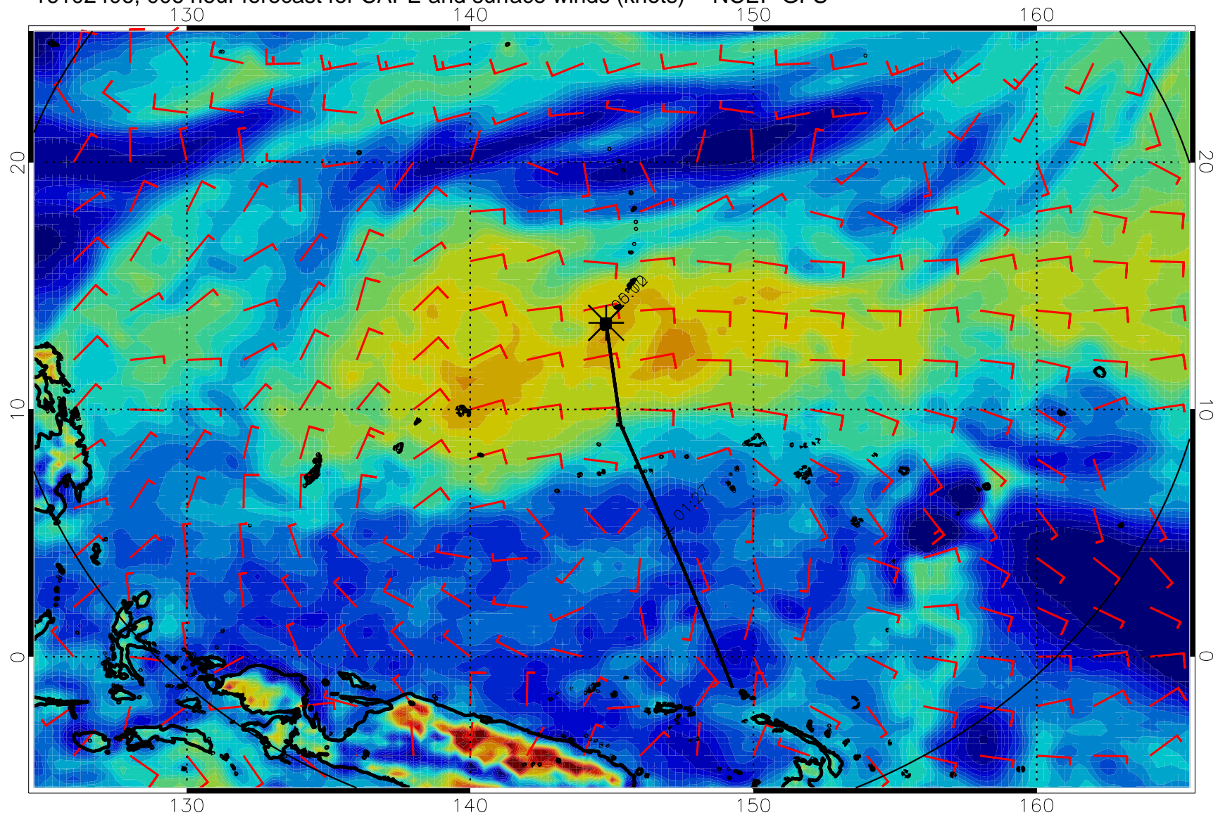
16102406, 006 hour forecast for CAPE and surface winds (knots) -- NCEP GFS
