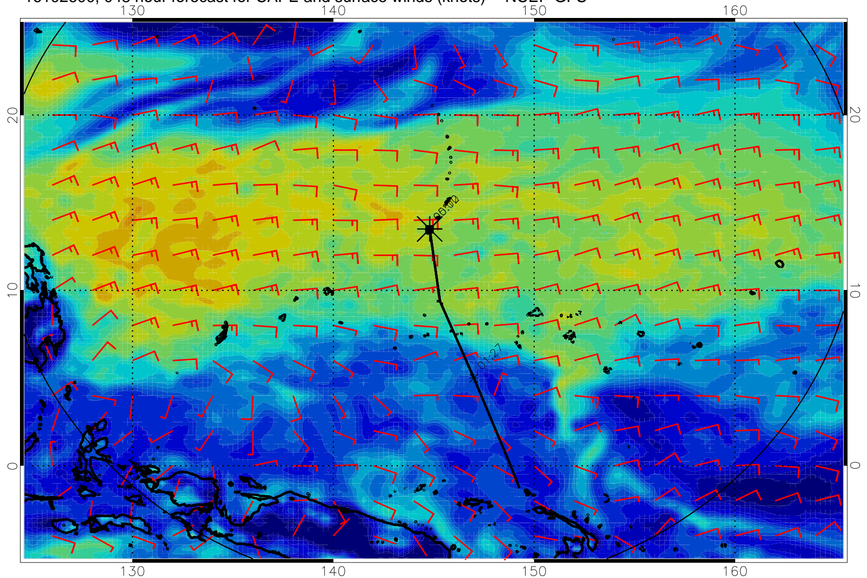
16102600, 048 hour forecast for CAPE and surface winds (knots) -- NCEP GFS
