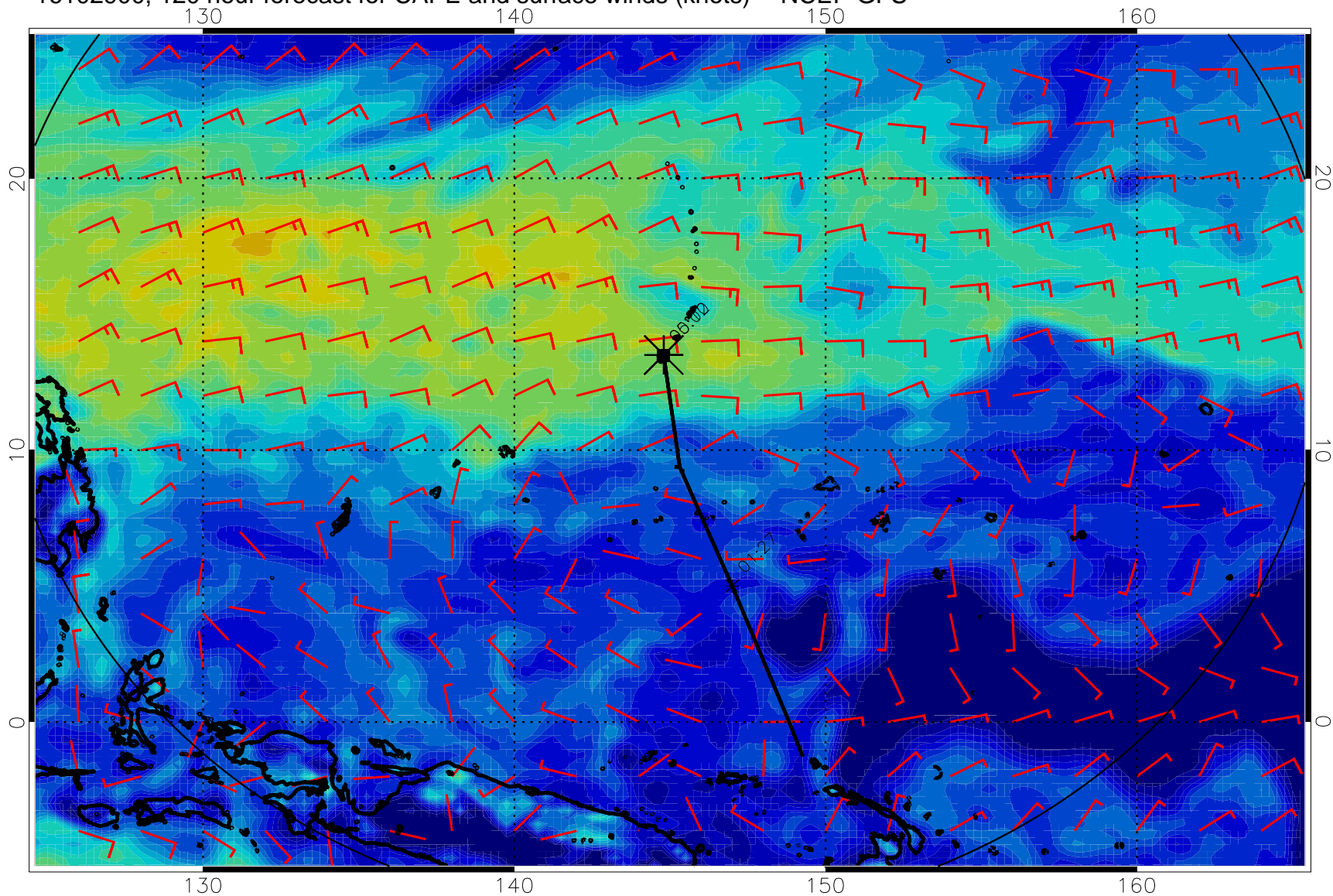
16102900, 120 hour forecast for CAPE and surface winds (knots) -- NCEP GFS
