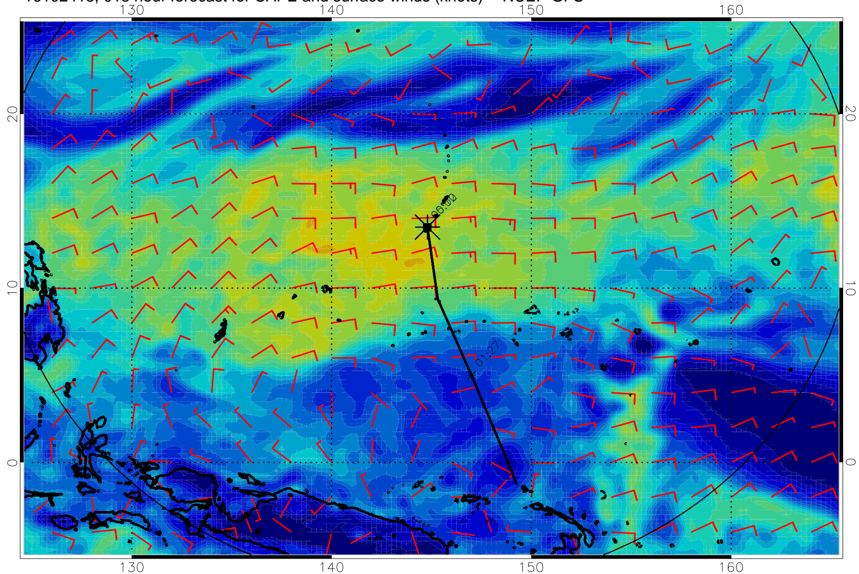
16102418, 018 hour forecast for CAPE and surface winds (knots) -- NCEP GFS
