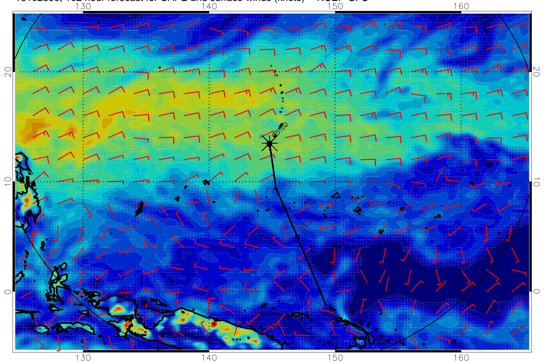
16102806, 102 hour forecast for CAPE and surface winds (knots) -- NCEP GFS
