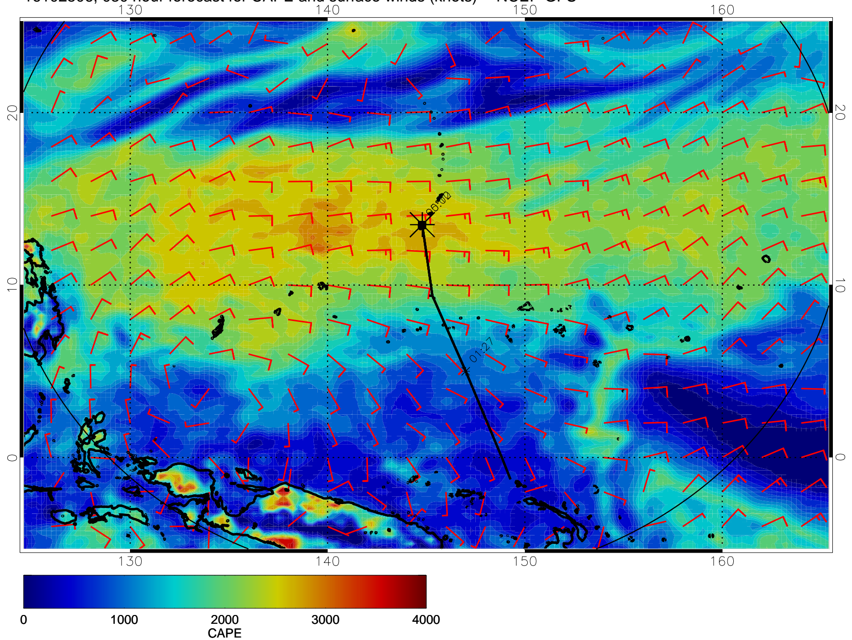
16102506, 030 hour forecast for CAPE and surface winds (knots) -- NCEP GFS
