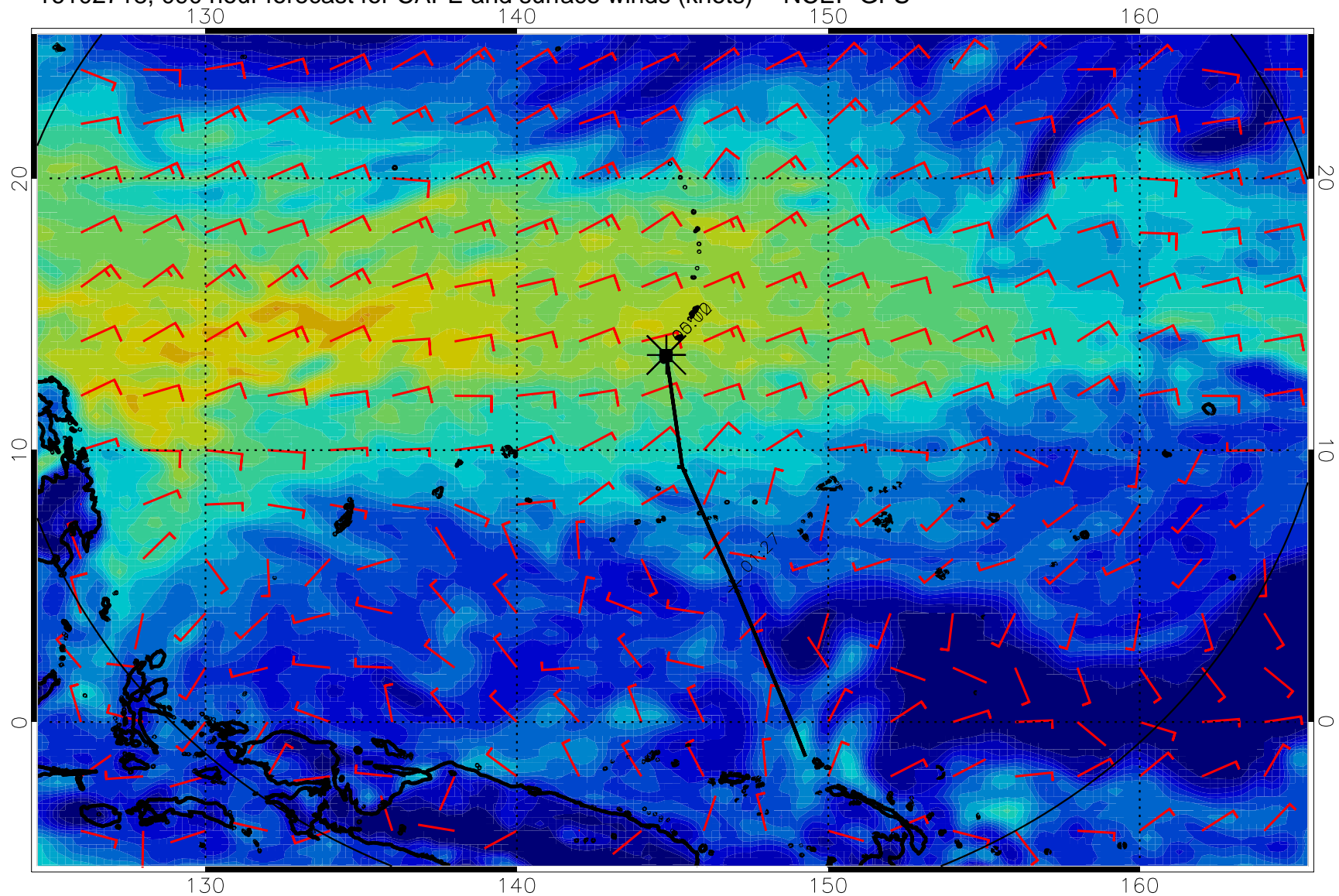
16102718, 090 hour forecast for CAPE and surface winds (knots) -- NCEP GFS
