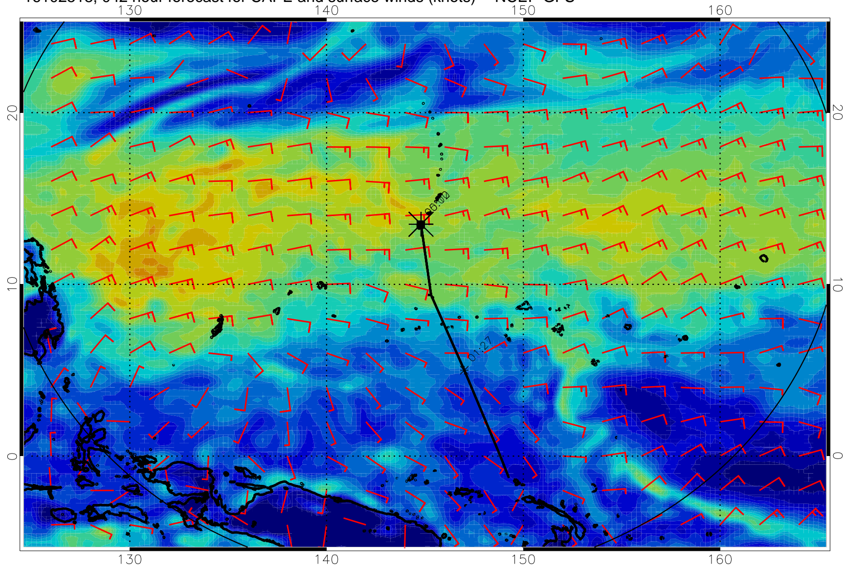
16102518, 042 hour forecast for CAPE and surface winds (knots) -- NCEP GFS
