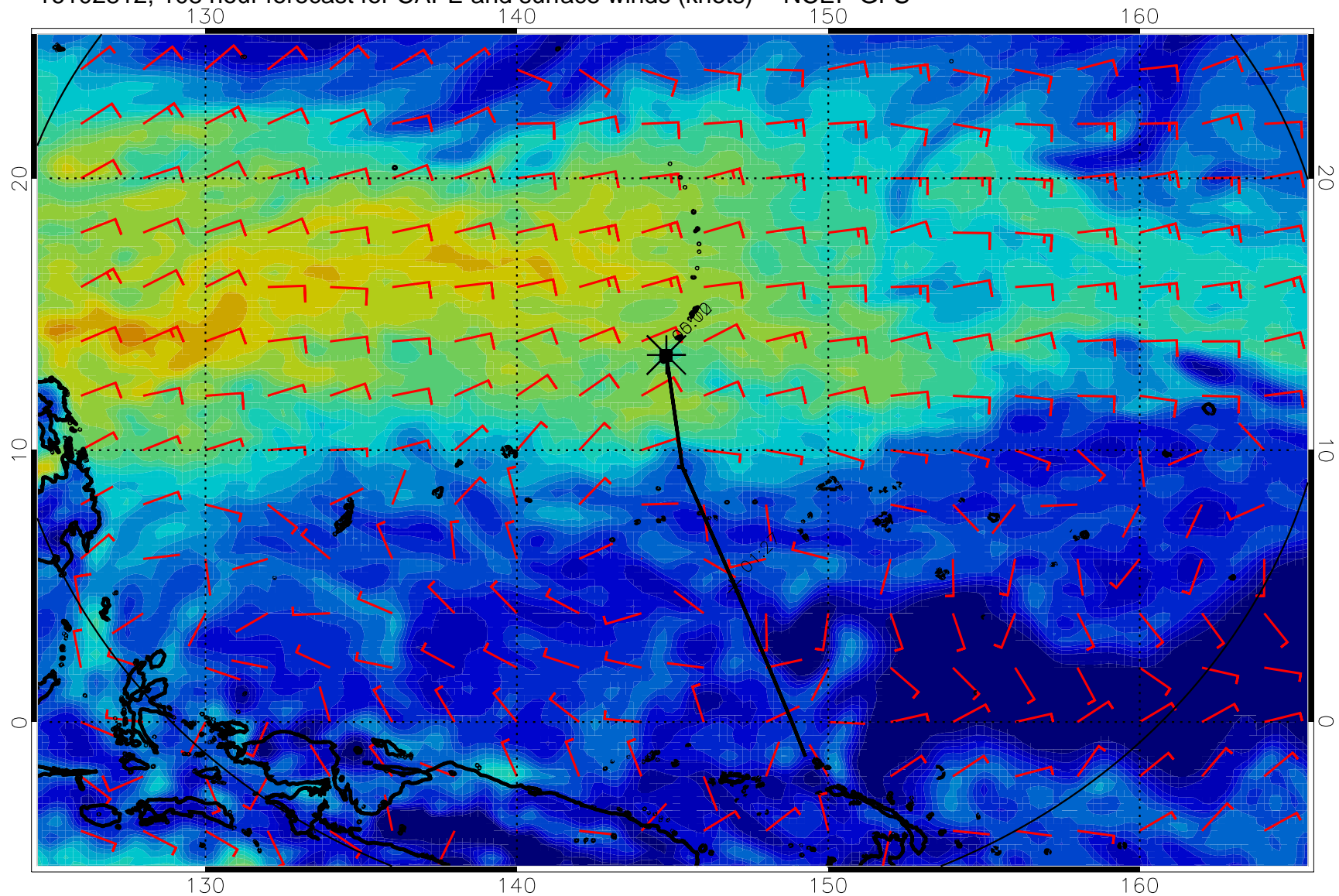
16102812, 108 hour forecast for CAPE and surface winds (knots) -- NCEP GFS
