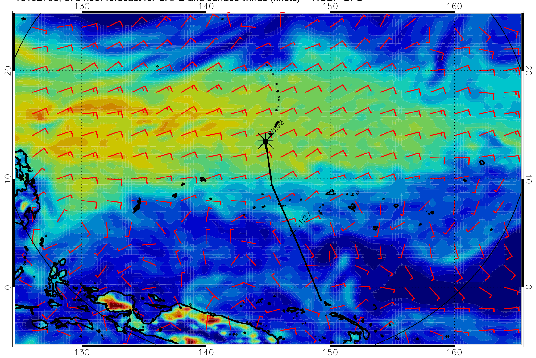
16102706, 078 hour forecast for CAPE and surface winds (knots) -- NCEP GFS
