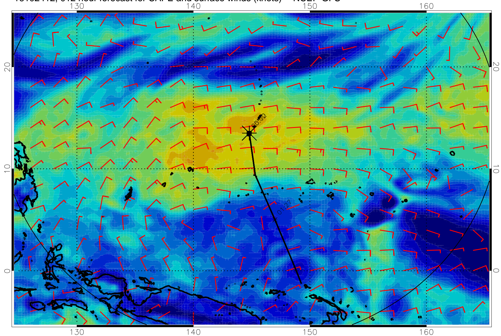
16102412, 012 hour forecast for CAPE and surface winds (knots) -- NCEP GFS
