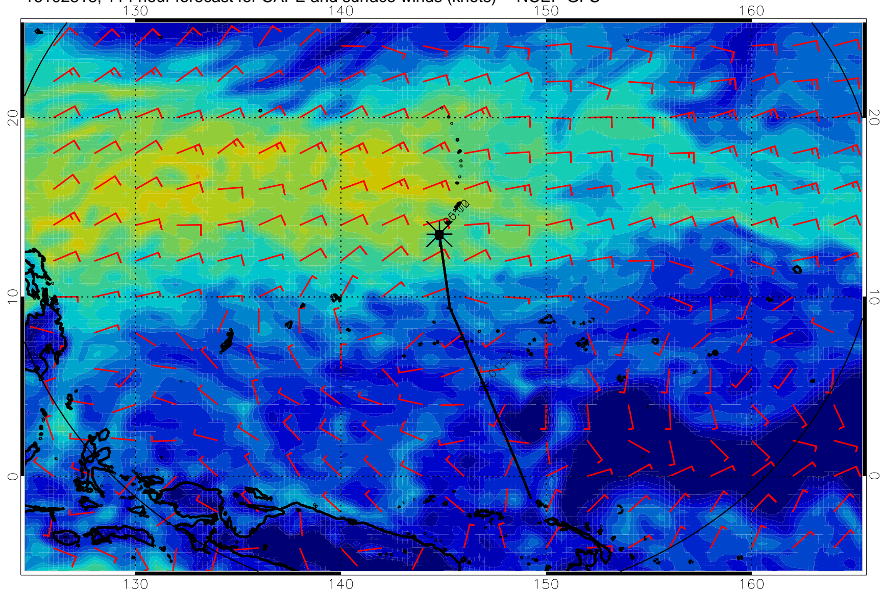
16102818, 114 hour forecast for CAPE and surface winds (knots) -- NCEP GFS
