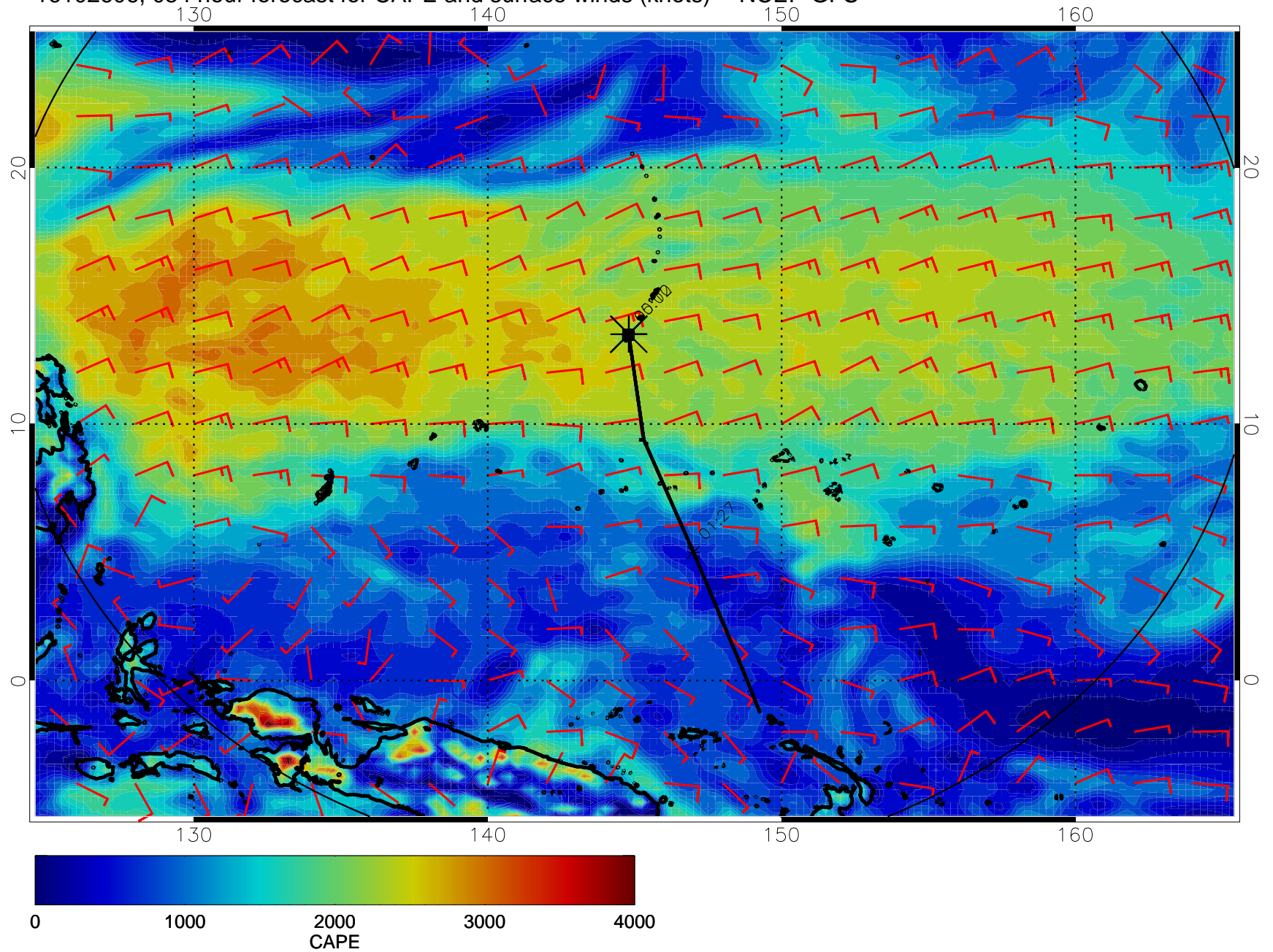
16102606, 054 hour forecast for CAPE and surface winds (knots) -- NCEP GFS
