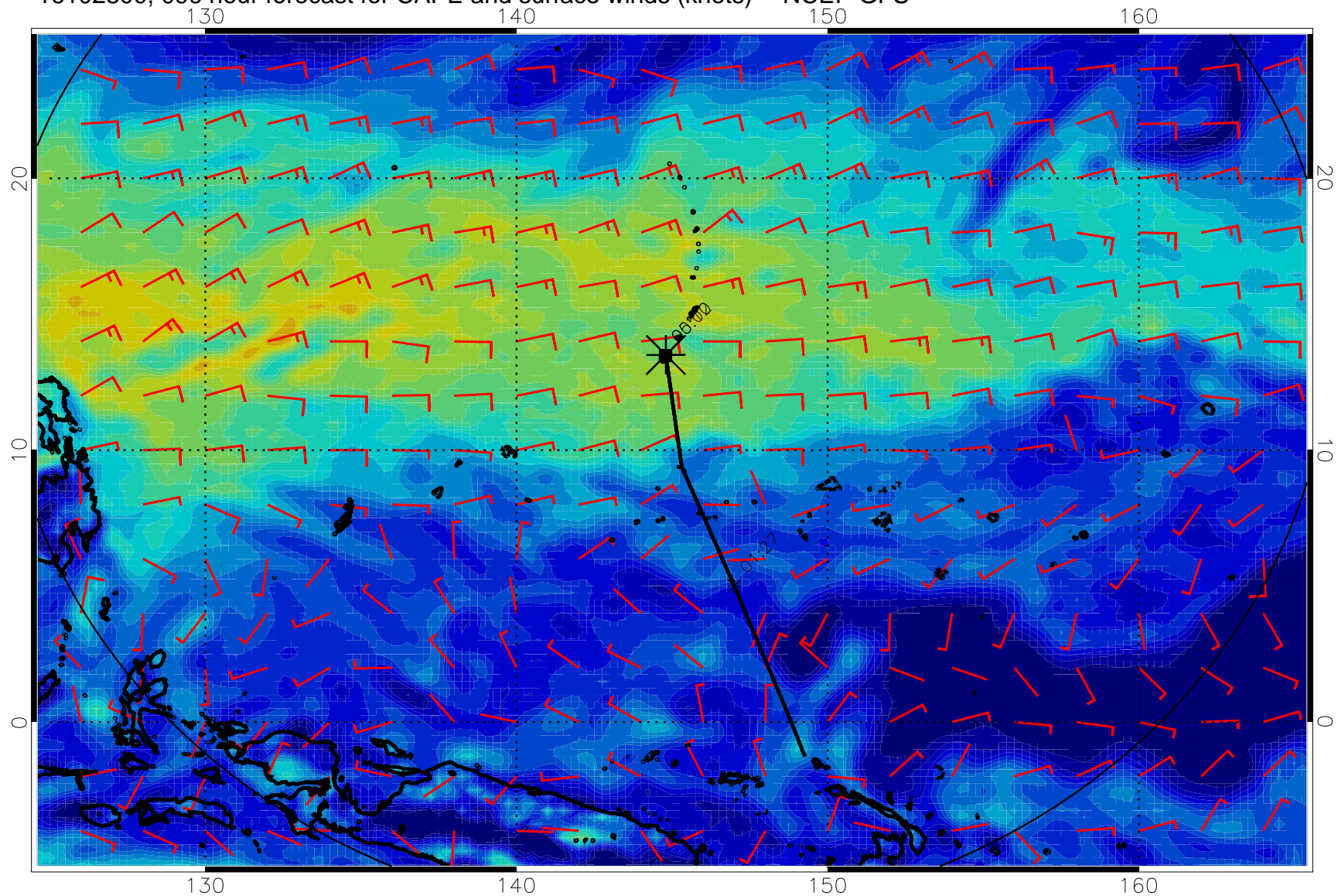
16102800, 096 hour forecast for CAPE and surface winds (knots) -- NCEP GFS
