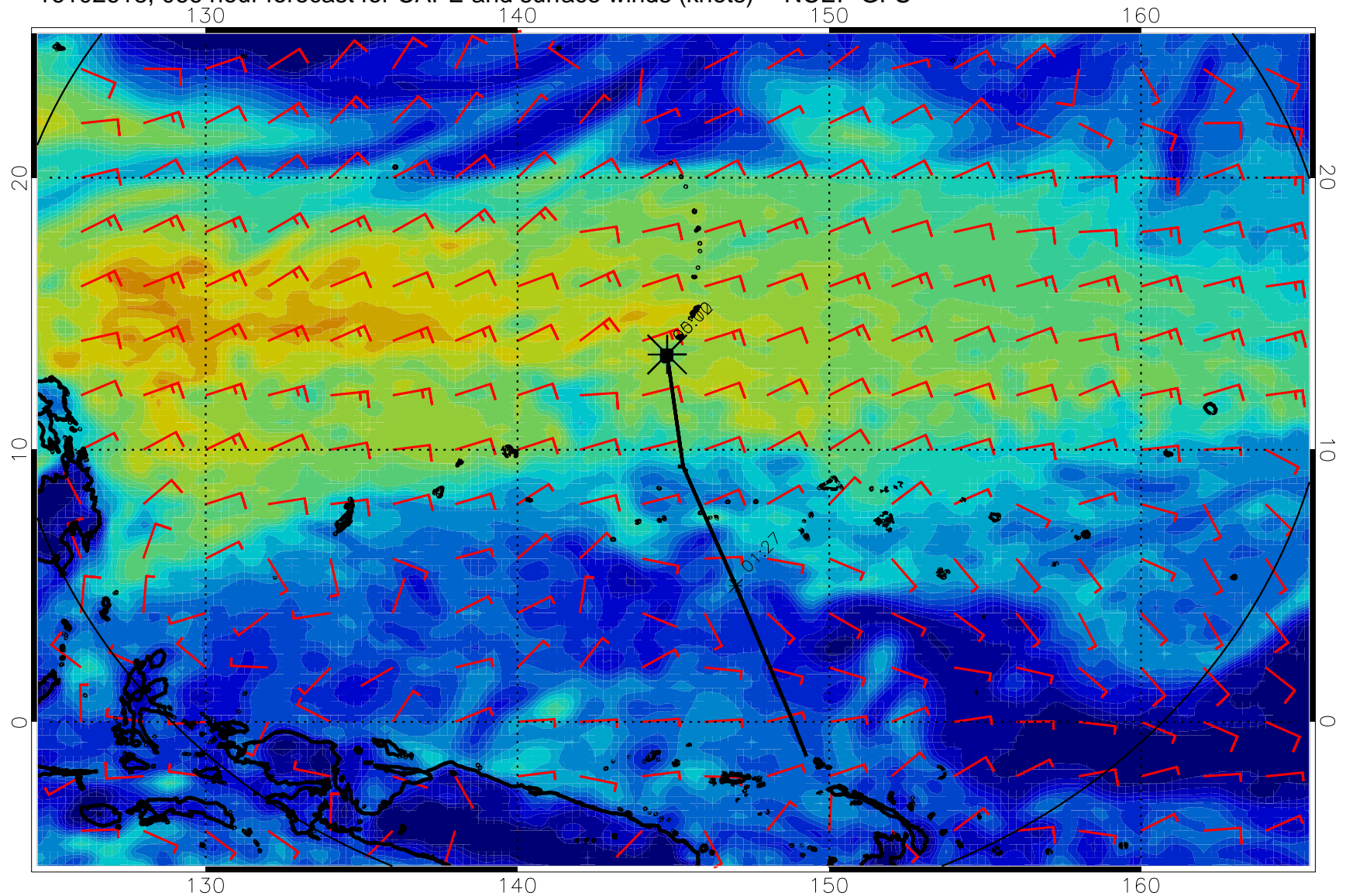
16102618, 066 hour forecast for CAPE and surface winds (knots) -- NCEP GFS
