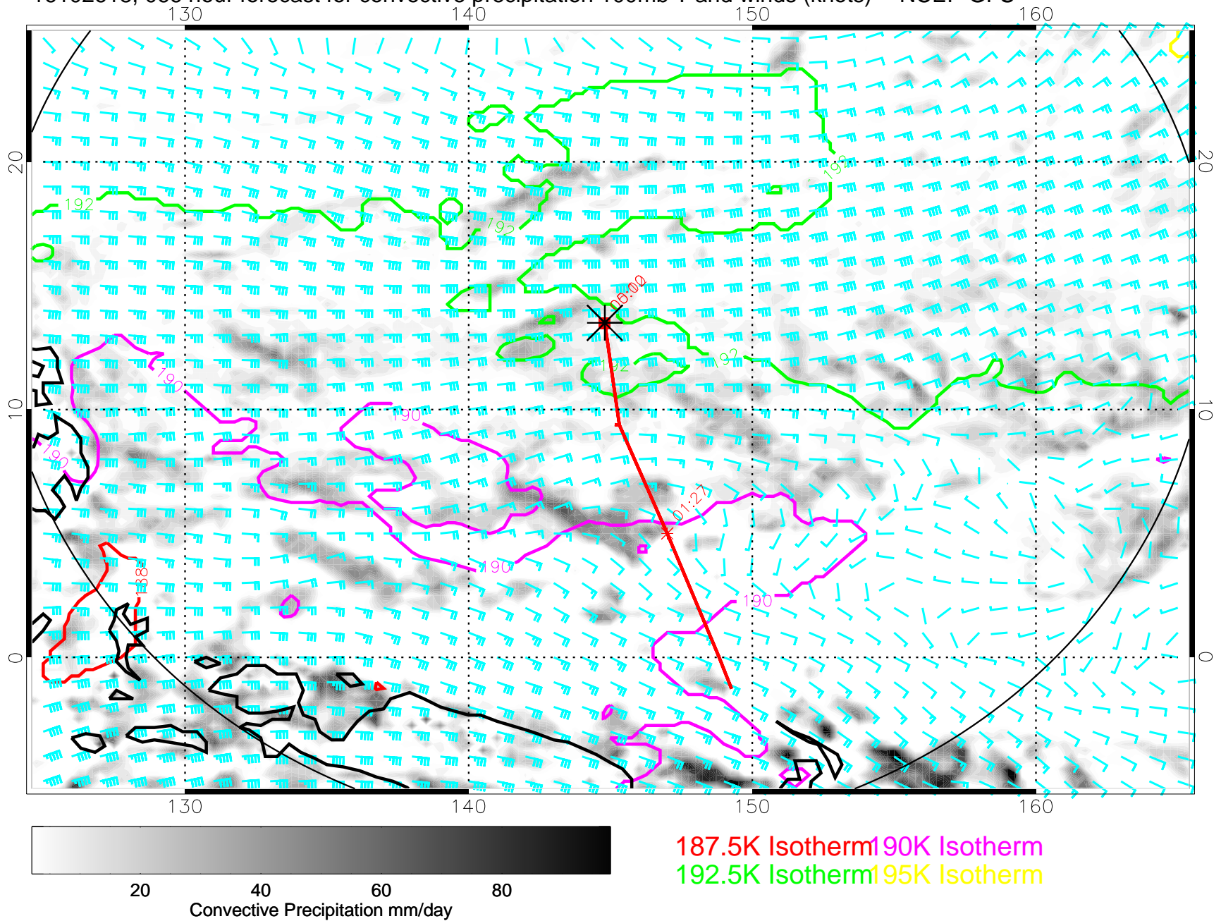
16102618, 066 hour forecast for convective precipitation 100mb T and winds (knots) -- NCEP GFS
