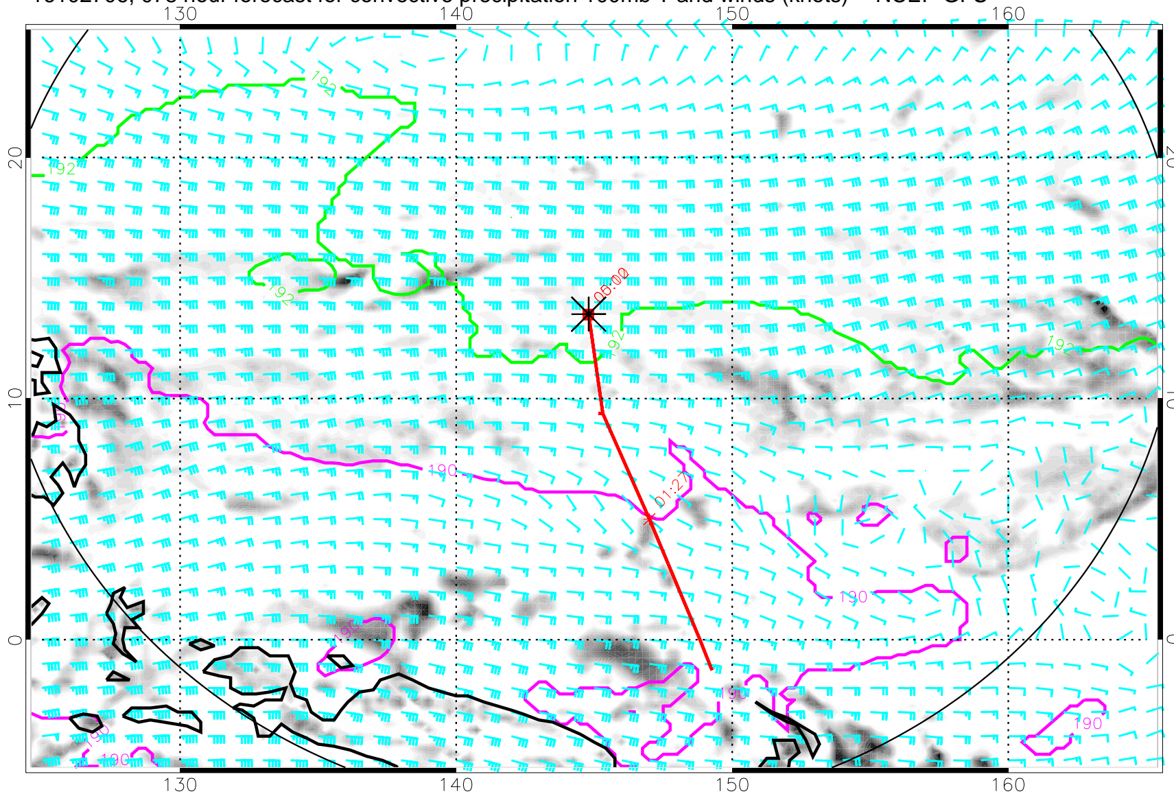
16102706, 078 hour forecast for convective precipitation 100mb T and winds (knots) -- NCEP GFS
