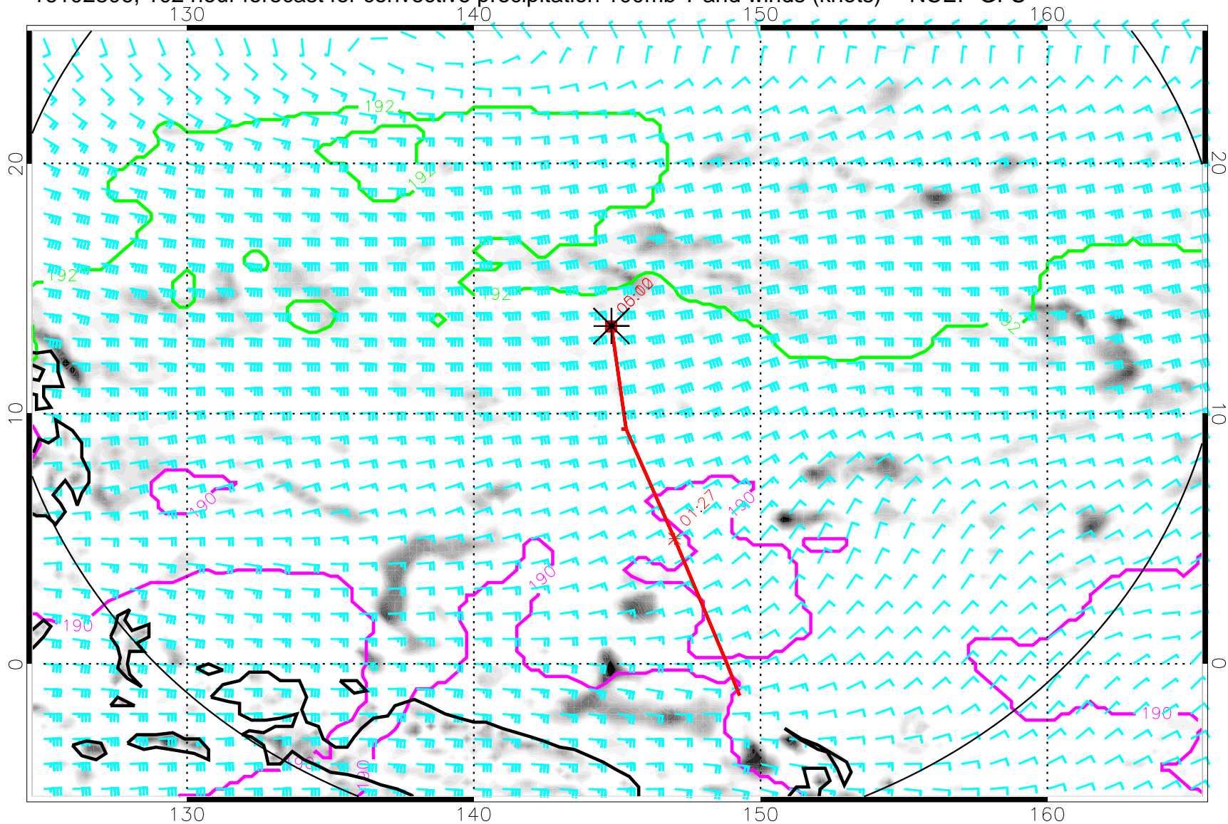
16102806, 102 hour forecast for convective precipitation 100mb T and winds (knots) -- NCEP GFS
