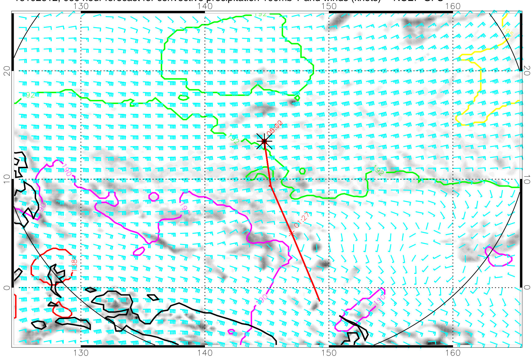
16102612, 060 hour forecast for convective precipitation 100mb T and winds (knots) -- NCEP GFS
