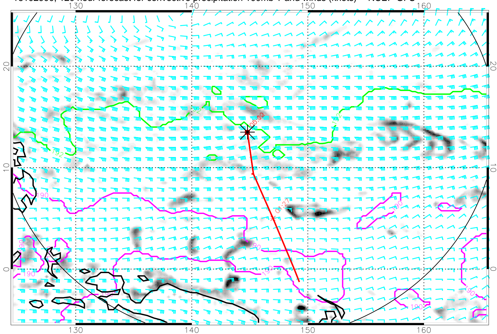
16102900, 120 hour forecast for convective precipitation 100mb T and winds (knots) -- NCEP GFS
