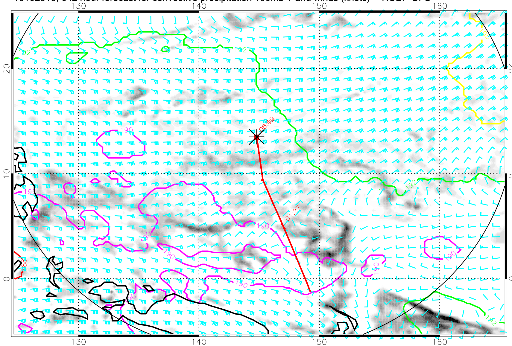
16102518, 04Z hour forecast for convective precipitation 100mb T and winds (knots) -- NCEP GFS
