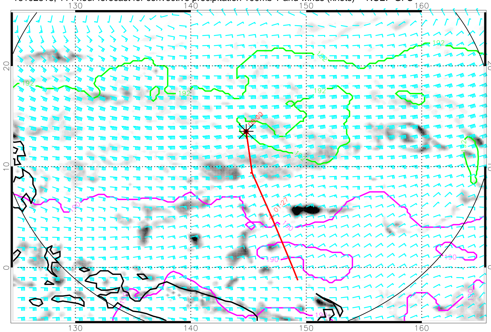
16102818, 114 hour forecast for convective precipitation 100mb T and winds (knots) -- NCEP GFS
