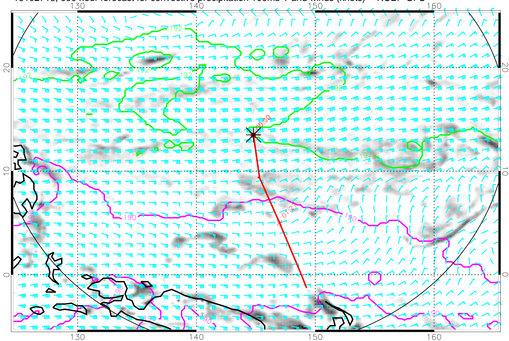
16102718, 090 hour forecast for convective precipitation 100mb T and winds (knots) -- NCEP GFS
