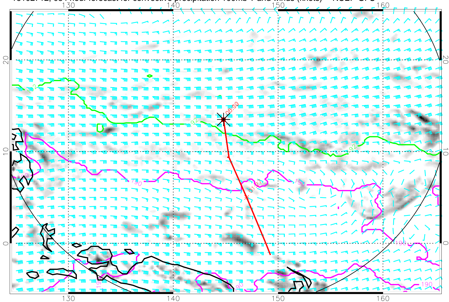
16102712, 084 hour forecast for convective precipitation 100mb T and winds (knots) -- NCEP GFS
