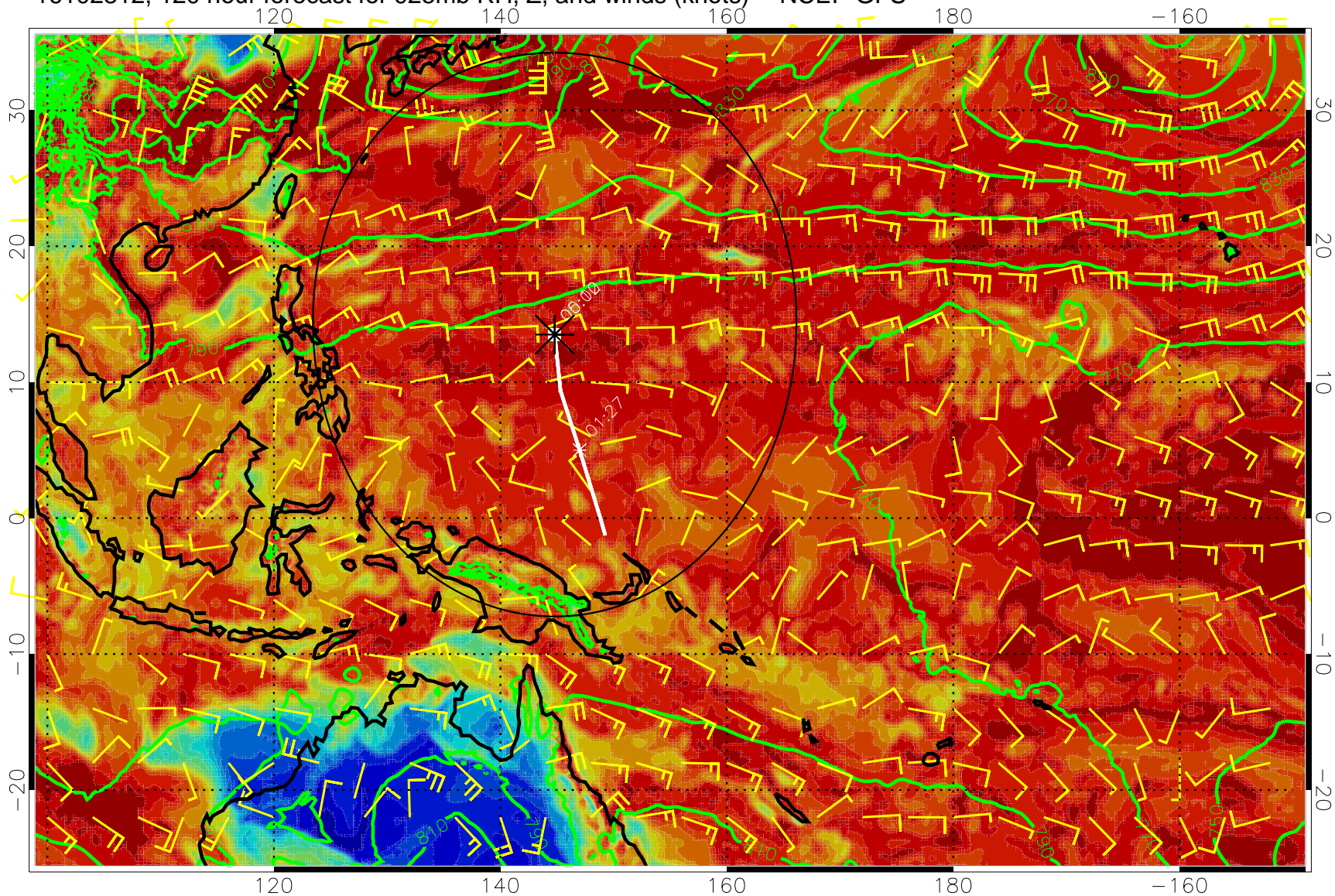
16102812, 120 hour forecast for 925mb RH, Z, and winds (knots) -- NCEP GFS
