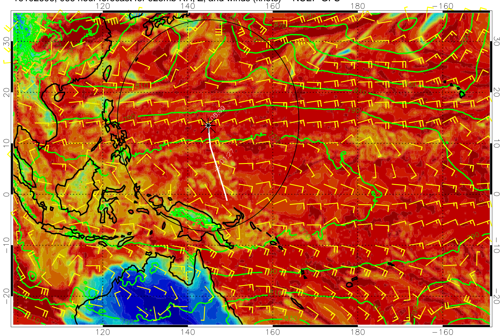
16102606, 066 hour forecast for 925mb RH, Z, and winds (knots) -- NCEP GFS
