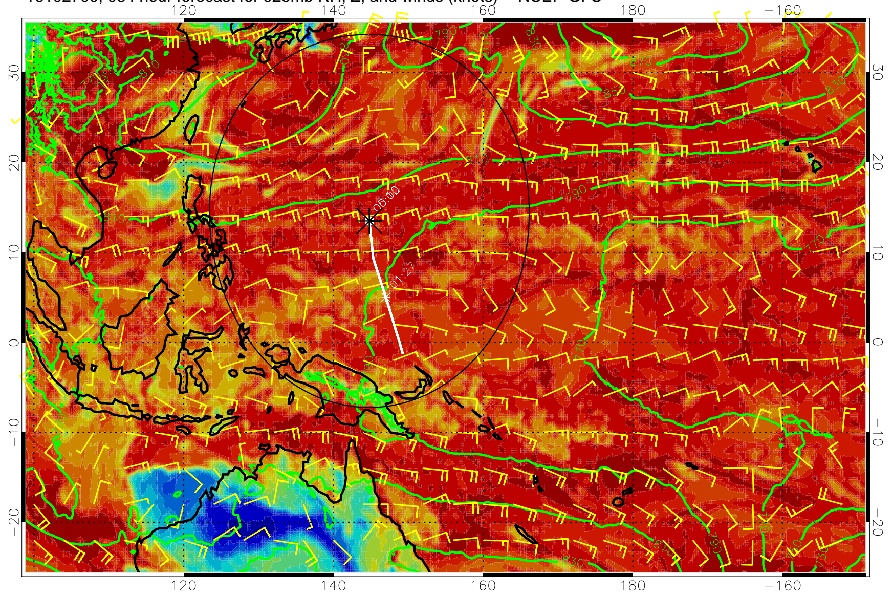
16102700, 084 hour forecast for 925mb RH, Z, and winds (knots) -- NCEP GFS
