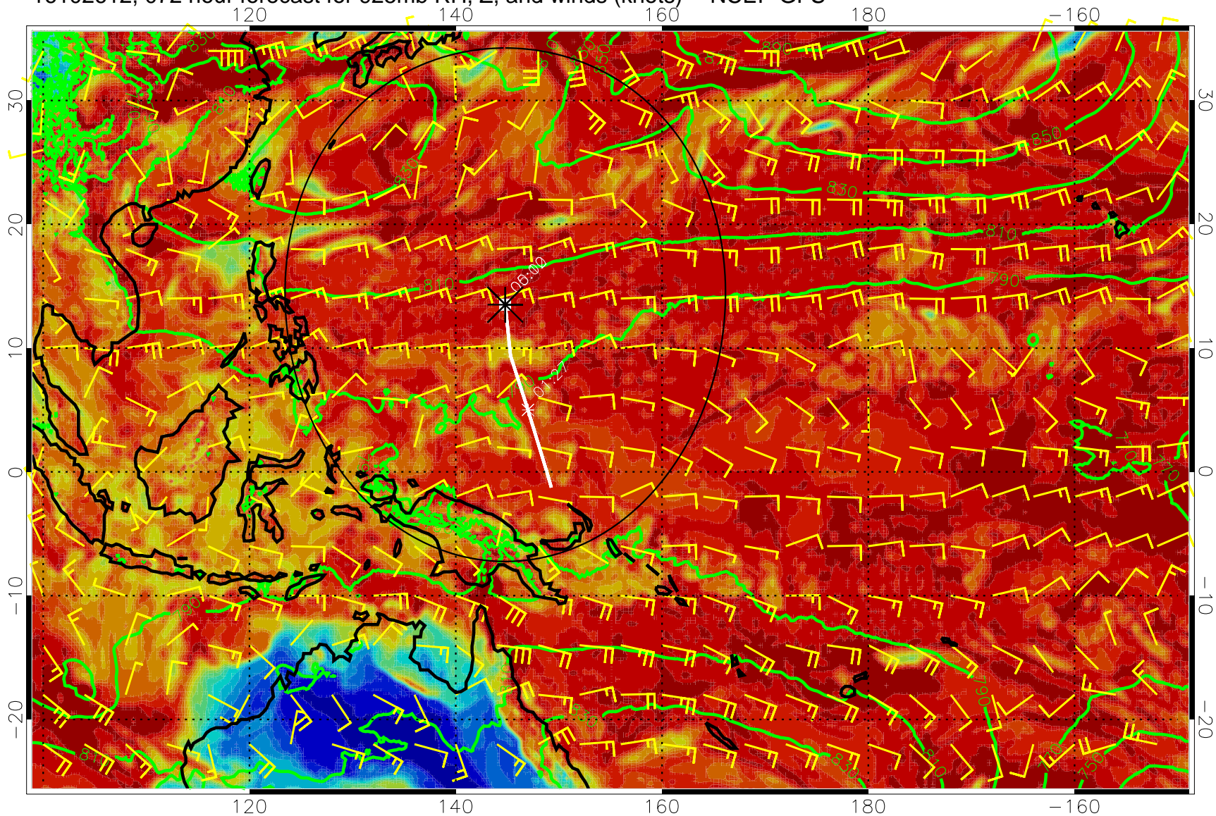
16102612, 072 hour forecast for 925mb RH, Z, and winds (knots) -- NCEP GFS
