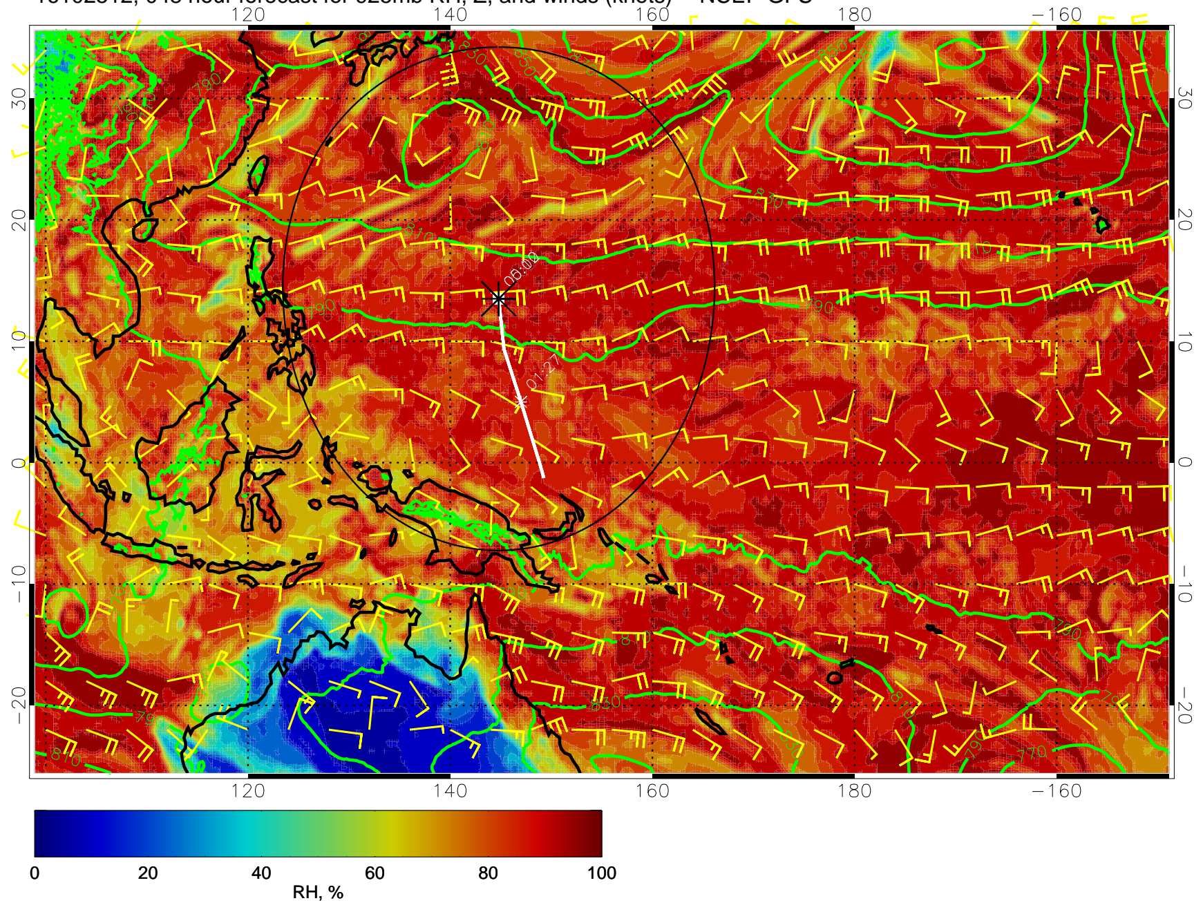
16102512, 048 hour forecast for 925mb RH, Z, and winds (knots) -- NCEP GFS
