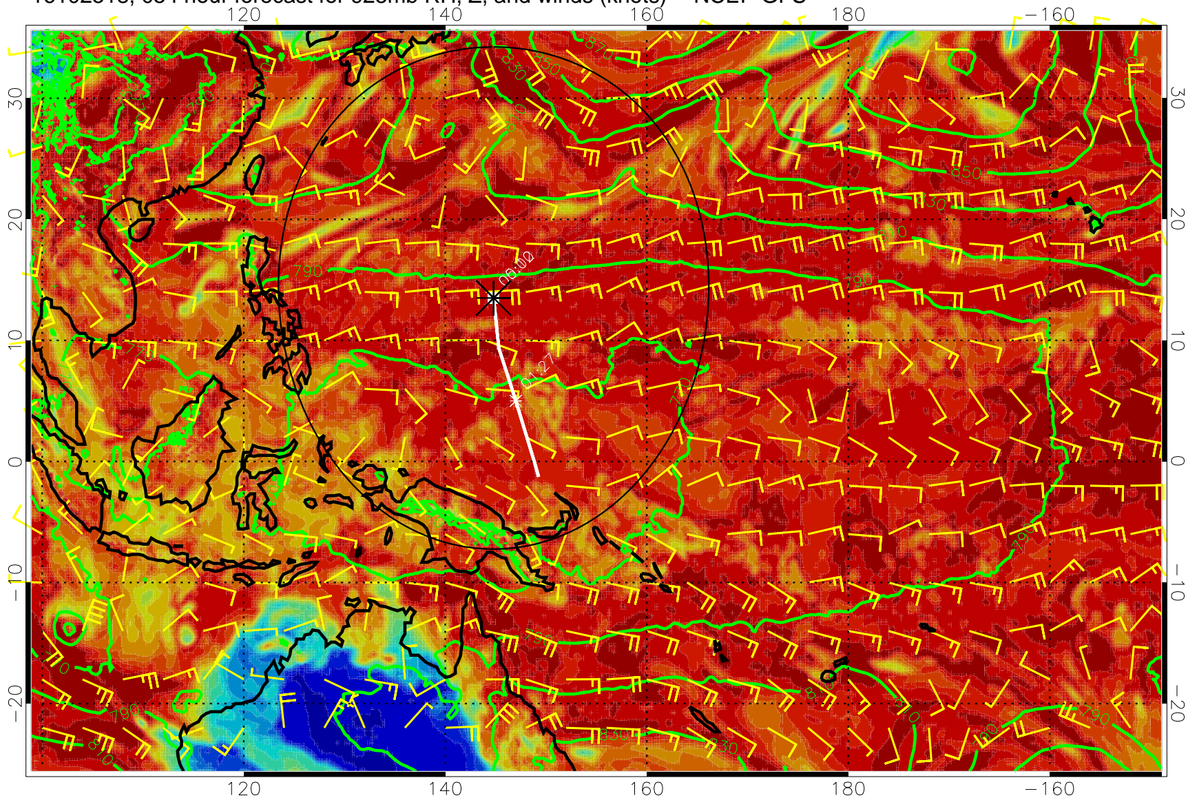
16102518, 054 hour forecast for 925mb RH, Z, and winds (knots) -- NCEP GFS
