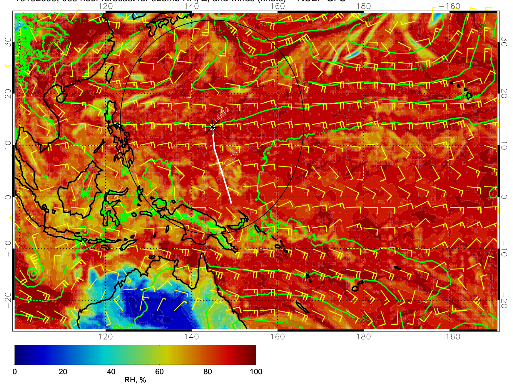
16102600, 060 hour forecast for 925mb RH, Z, and winds (knots) -- NCEP GFS
