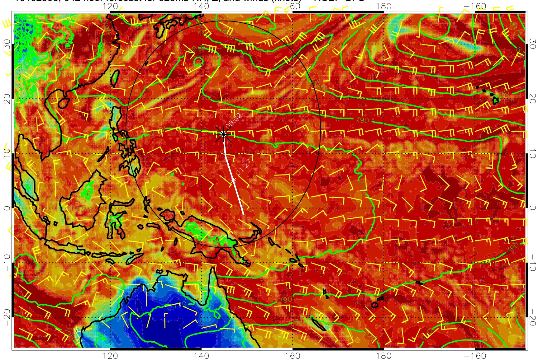
16102506, 042 hour forecast for 925mb RH, Z, and winds (knots) -- NCEP GFS
