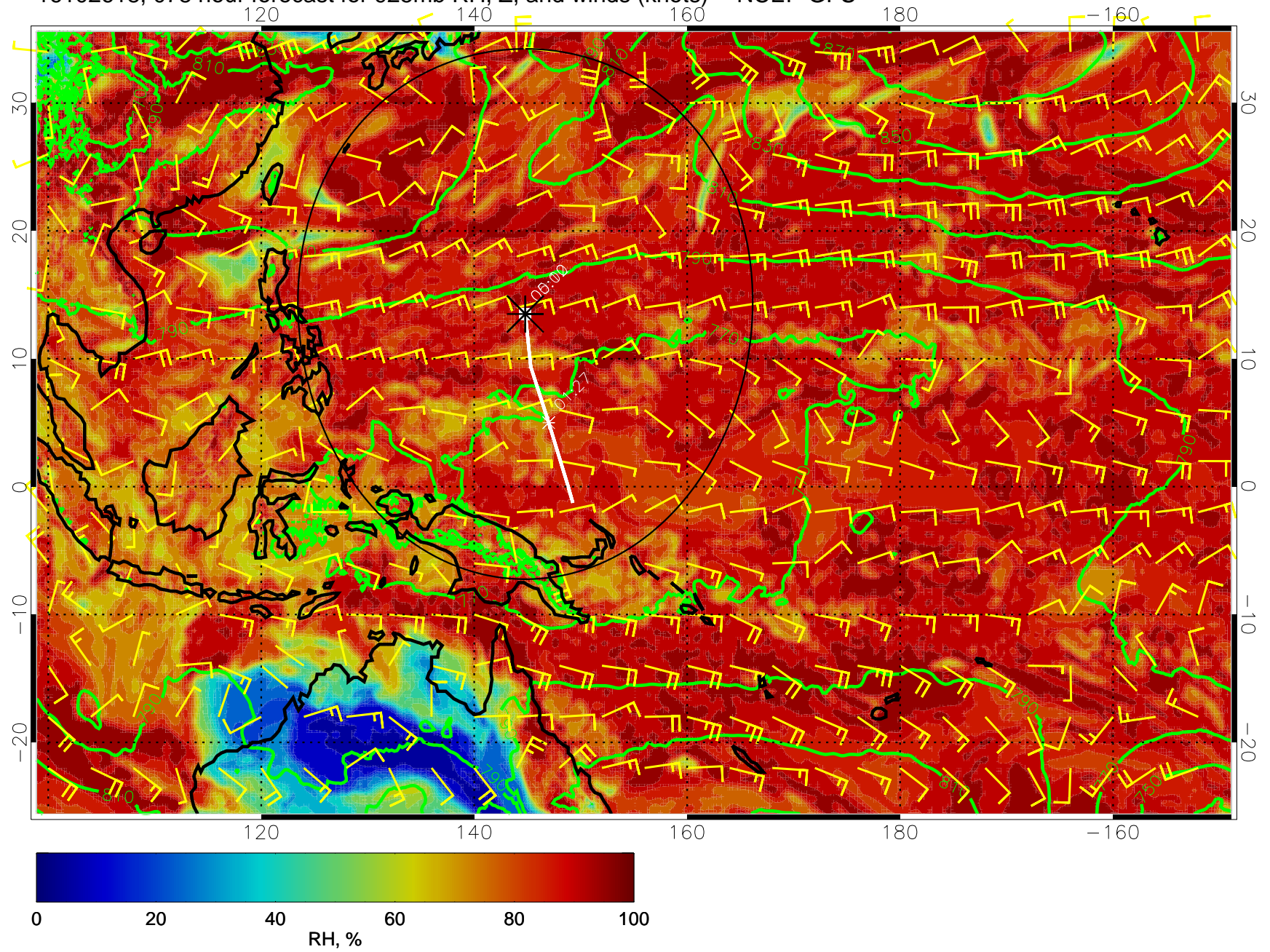
16102618, 078 hour forecast for 925mb RH, Z, and winds (knots) -- NCEP GFS
