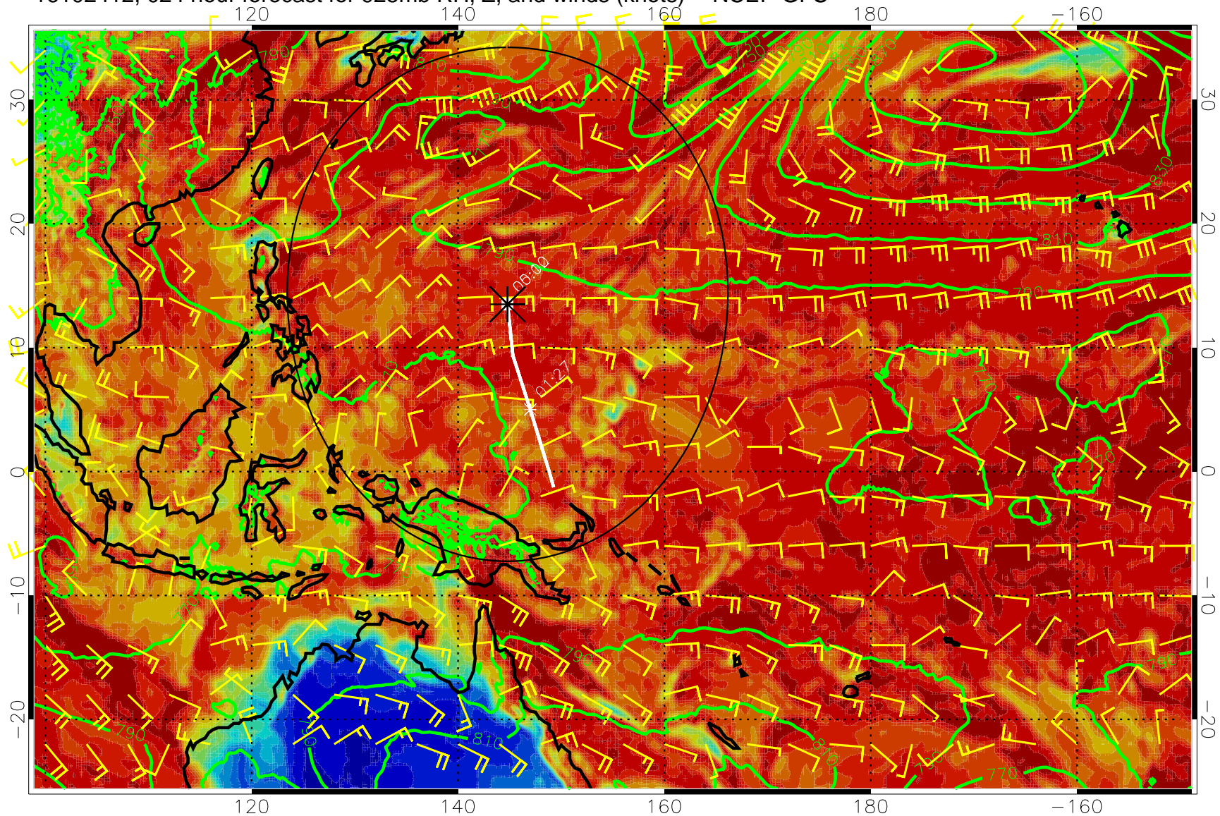
16102412, 024 hour forecast for 925mb RH, Z, and winds (knots) -- NCEP GFS
