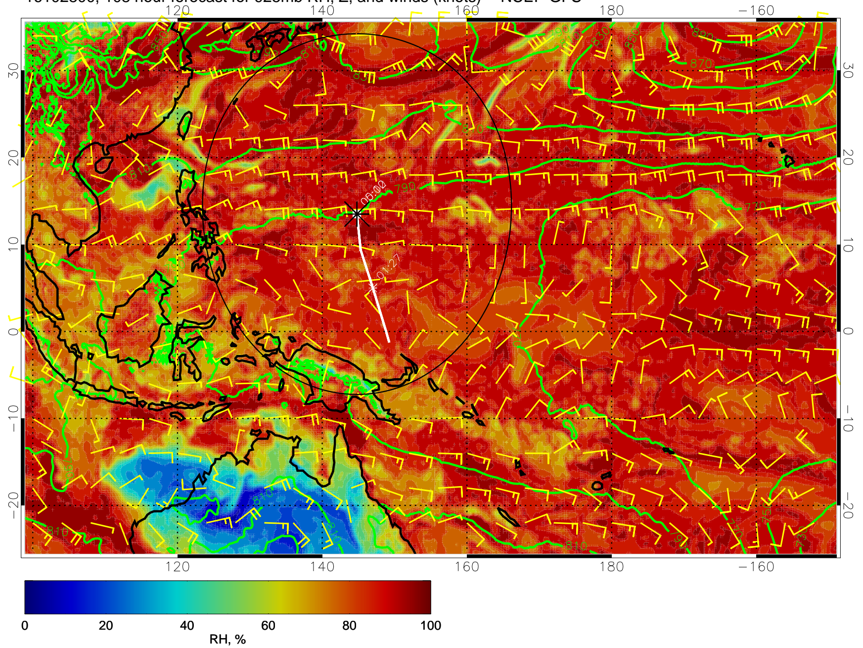
16102800, 108 hour forecast for 925mb RH, Z, and winds (knots) -- NCEP GFS
