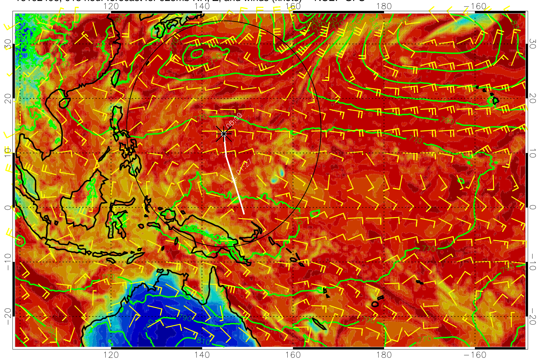
16102406, 018 hour forecast for 925mb RH, Z, and winds (knots) -- NCEP GFS
