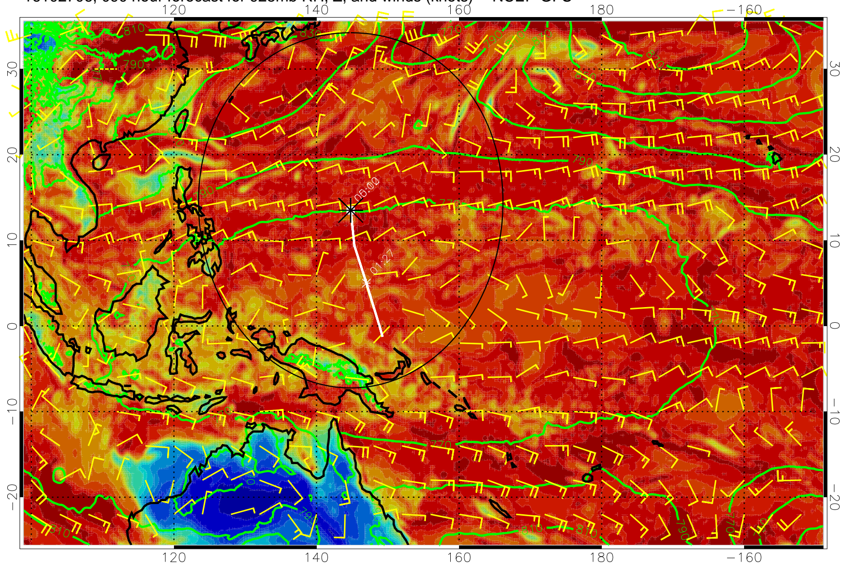
16102706, 090 hour forecast for 925mb RH, Z, and winds (knots) -- NCEP GFS
