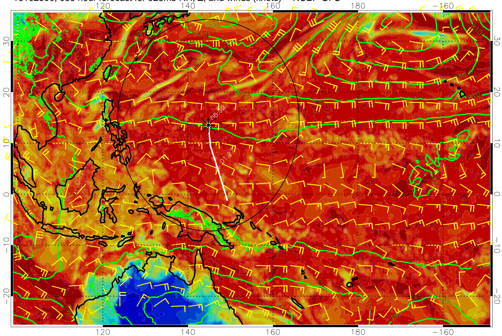
16102500, 036 hour forecast for 925mb RH, Z, and winds (knots) -- NCEP GFS
