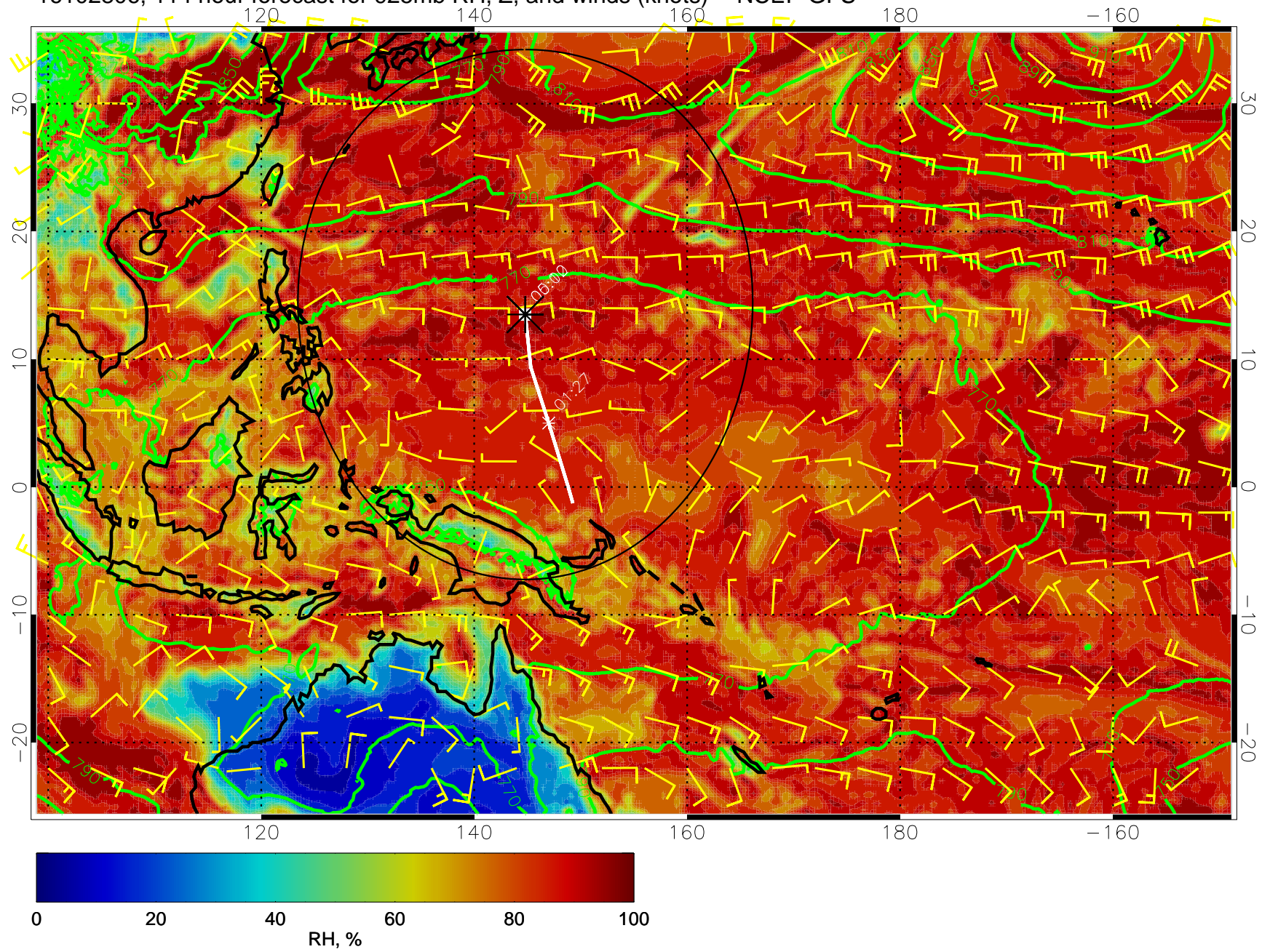
16102806, 114 hour forecast for 925mb RH, Z, and winds (knots) -- NCEP GFS
