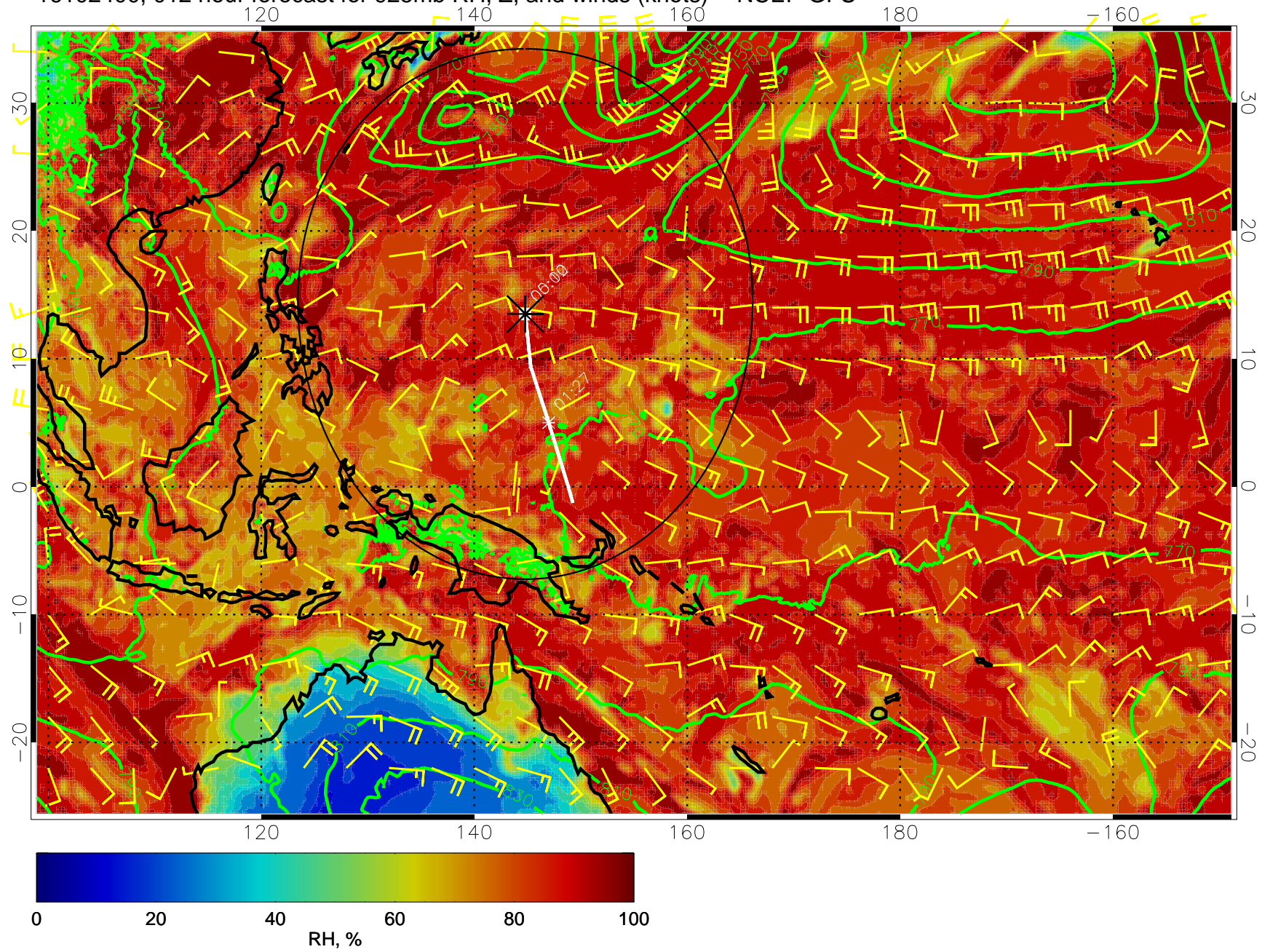
16102400, 012 hour forecast for 925mb RH, Z, and winds (knots) -- NCEP GFS
