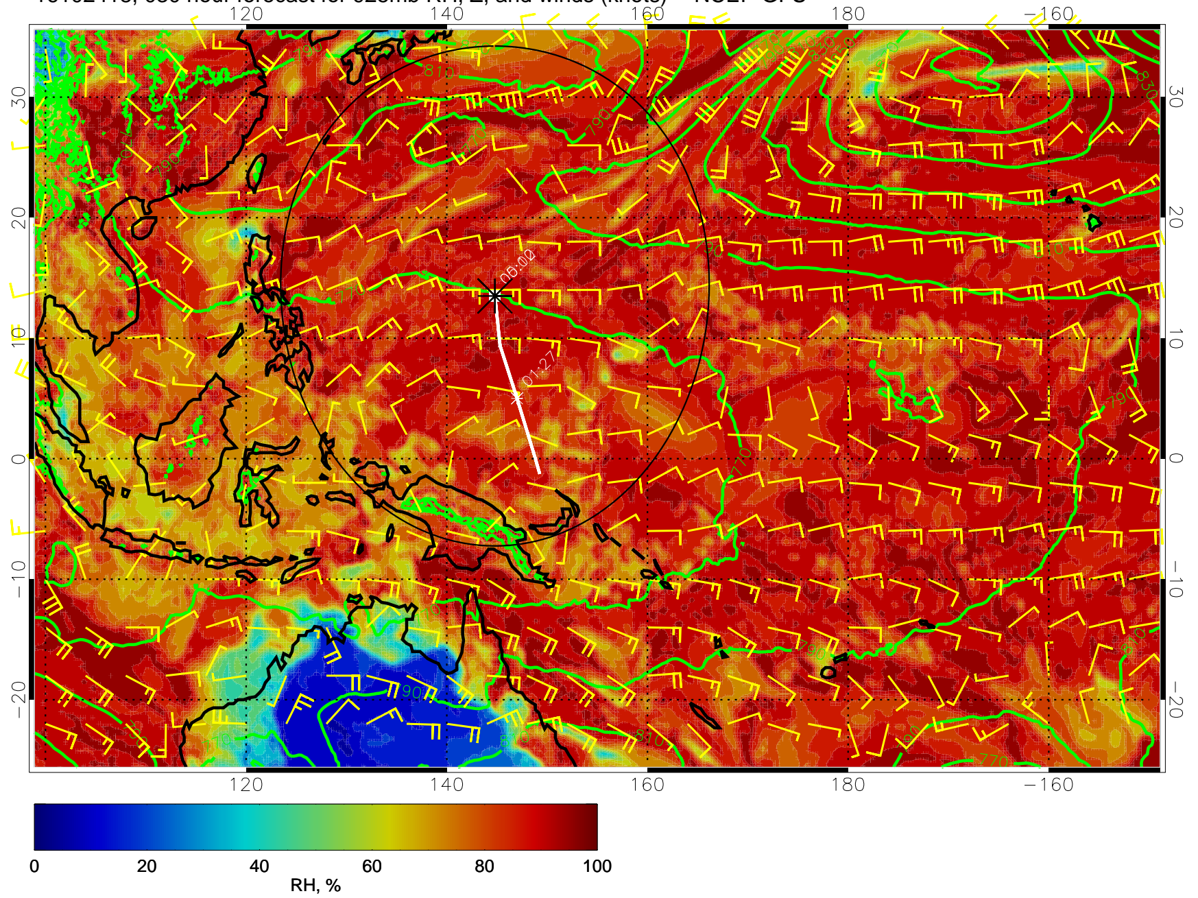
16102418, 030 hour forecast for 925mb RH, Z, and winds (knots) -- NCEP GFS
