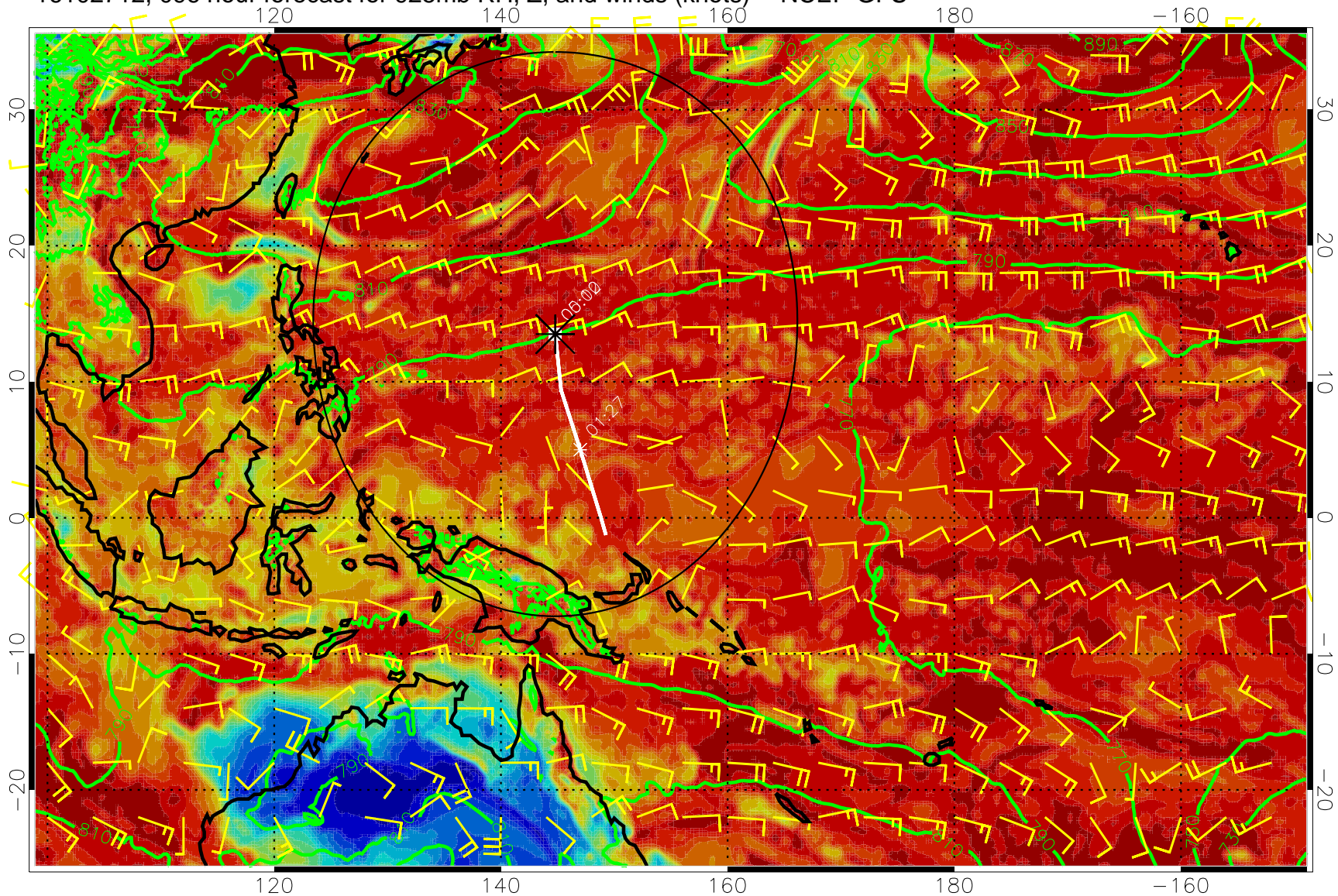
16102712, 096 hour forecast for 925mb RH, Z, and winds (knots) -- NCEP GFS
