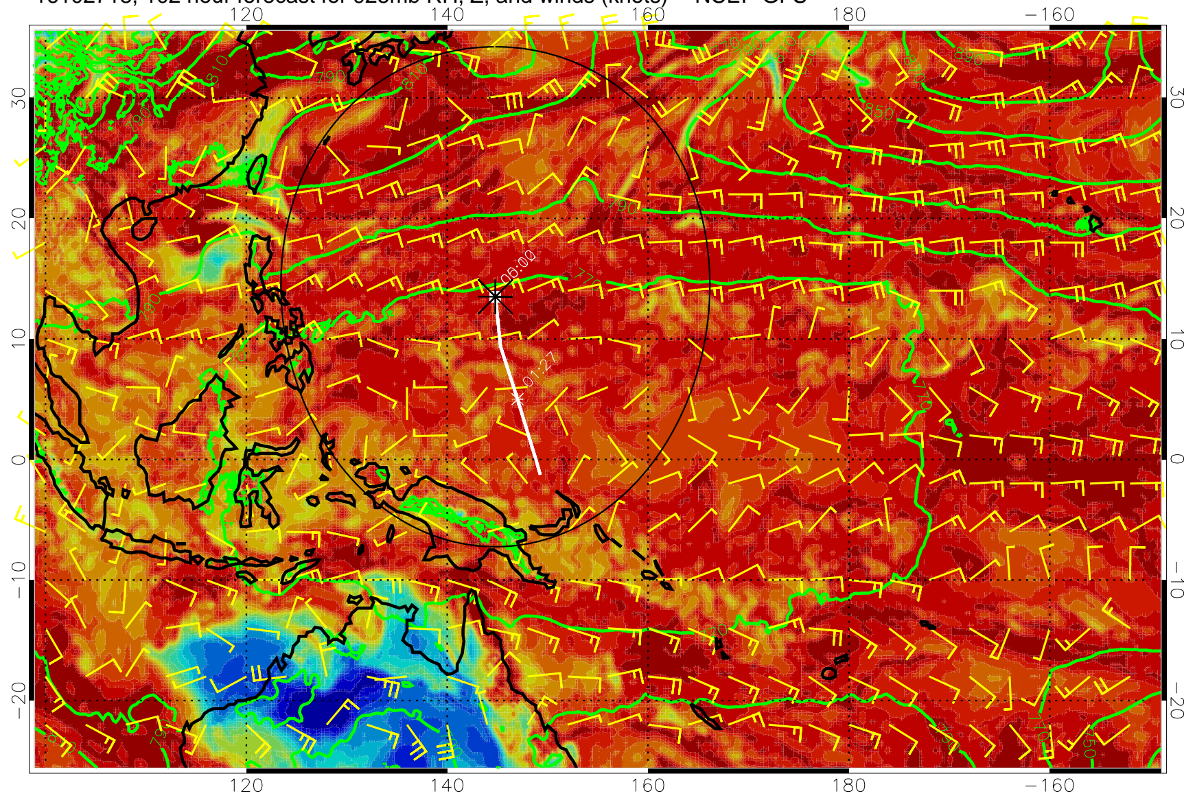
16102718, 102 hour forecast for 925mb RH, Z, and winds (knots) -- NCEP GFS
