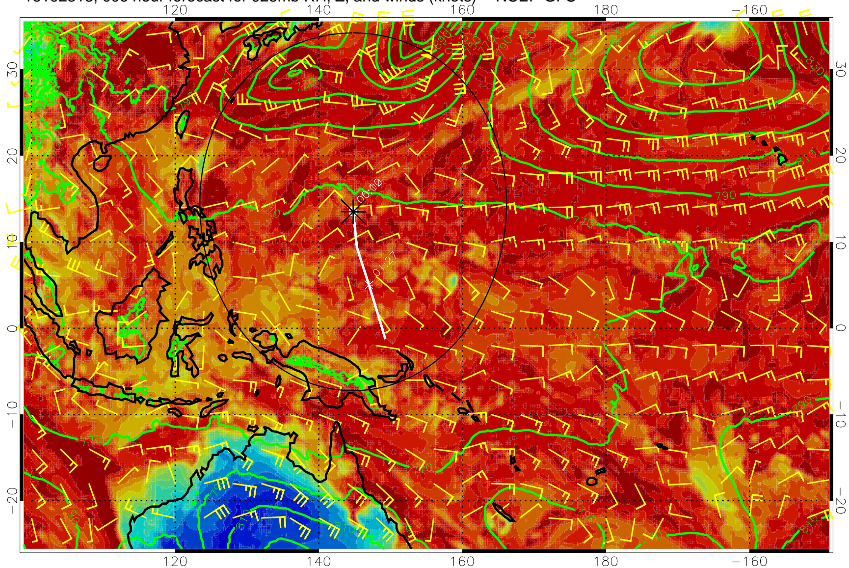
16102318, 006 hour forecast for 925mb RH, Z, and winds (knots) -- NCEP GFS
