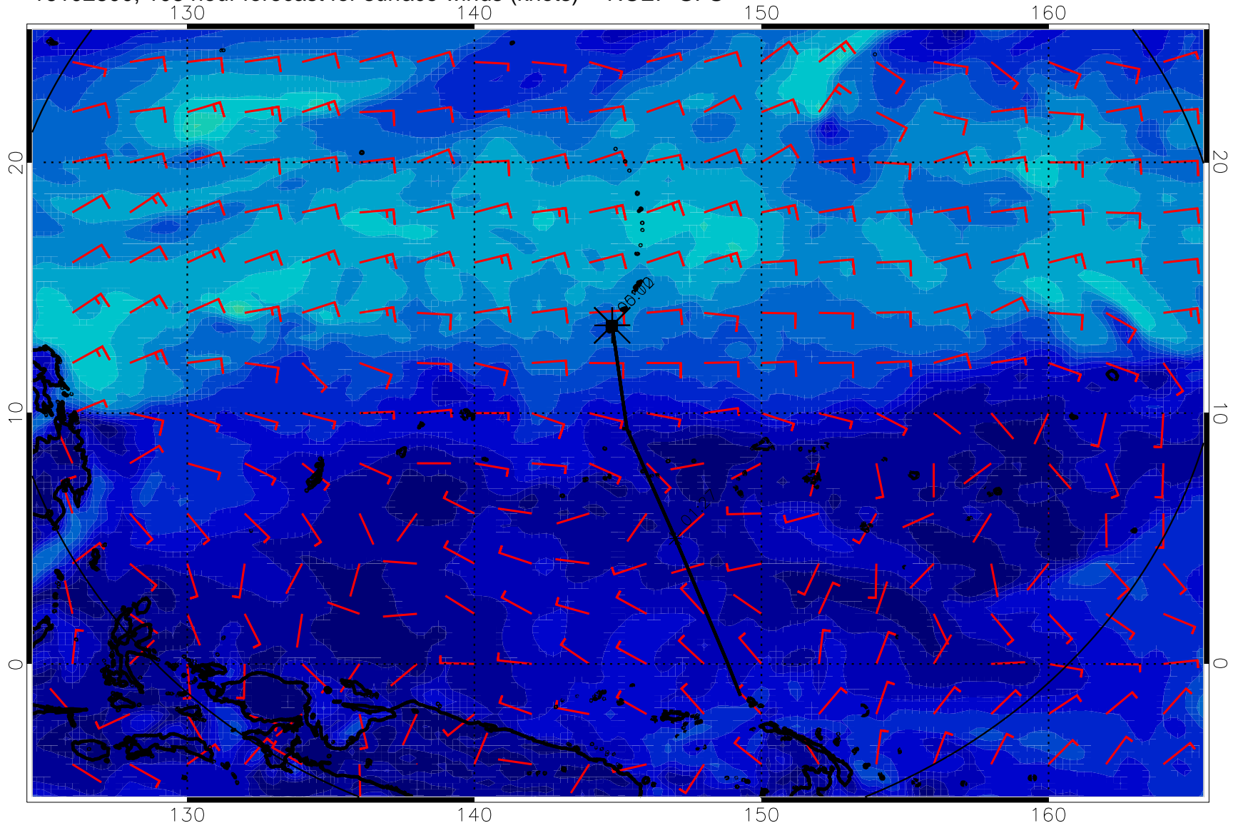
16102800, 108 hour forecast for surface winds (knots) -- NCEP GFS
