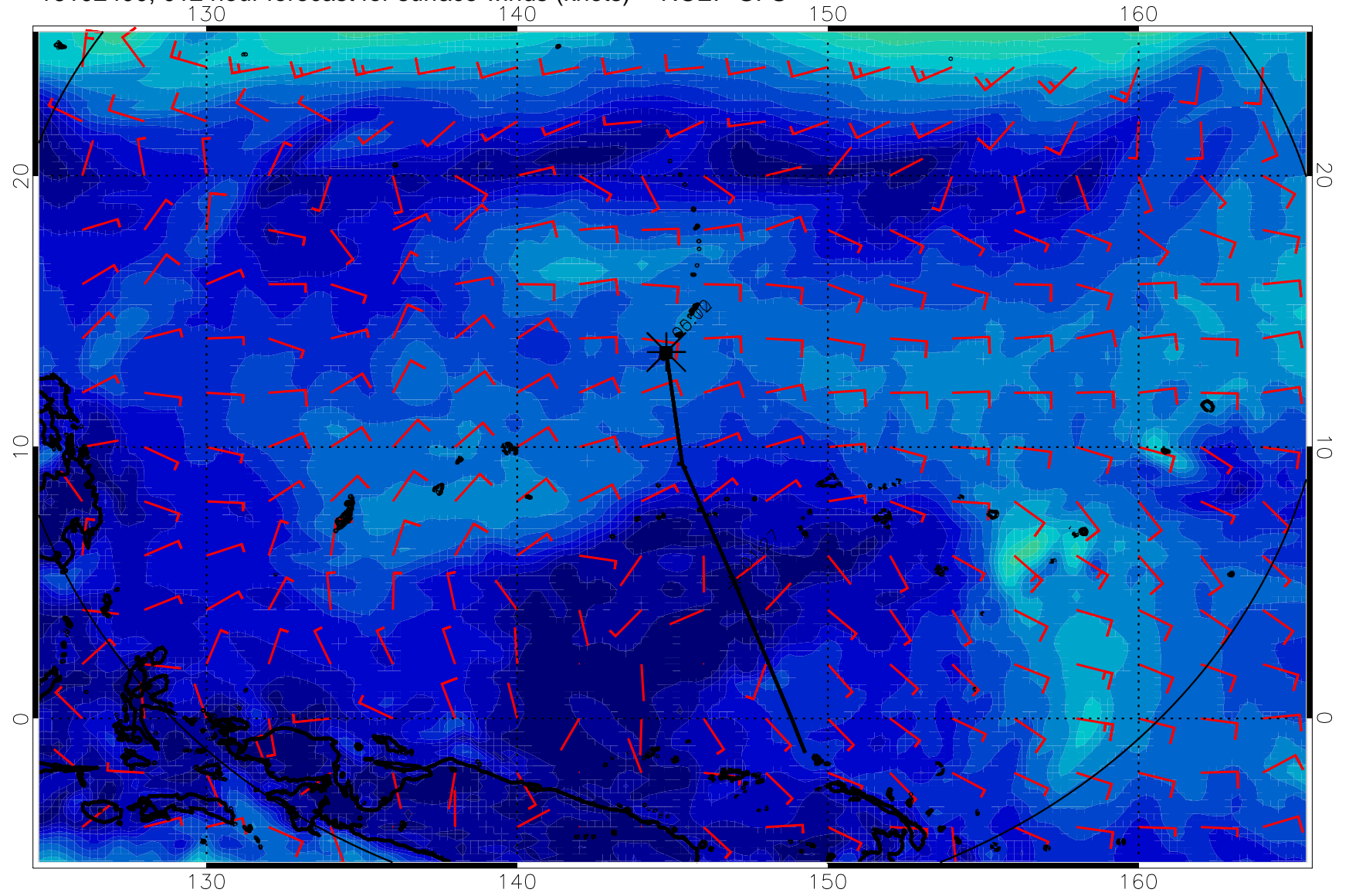
16102400, 012 hour forecast for surface winds (knots) -- NCEP GFS
