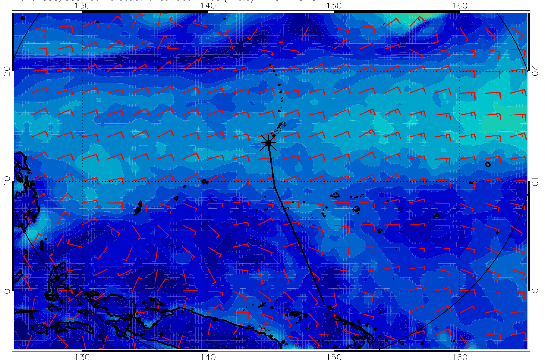
16102606, 066 hour forecast for surface winds (knots) -- NCEP GFS
