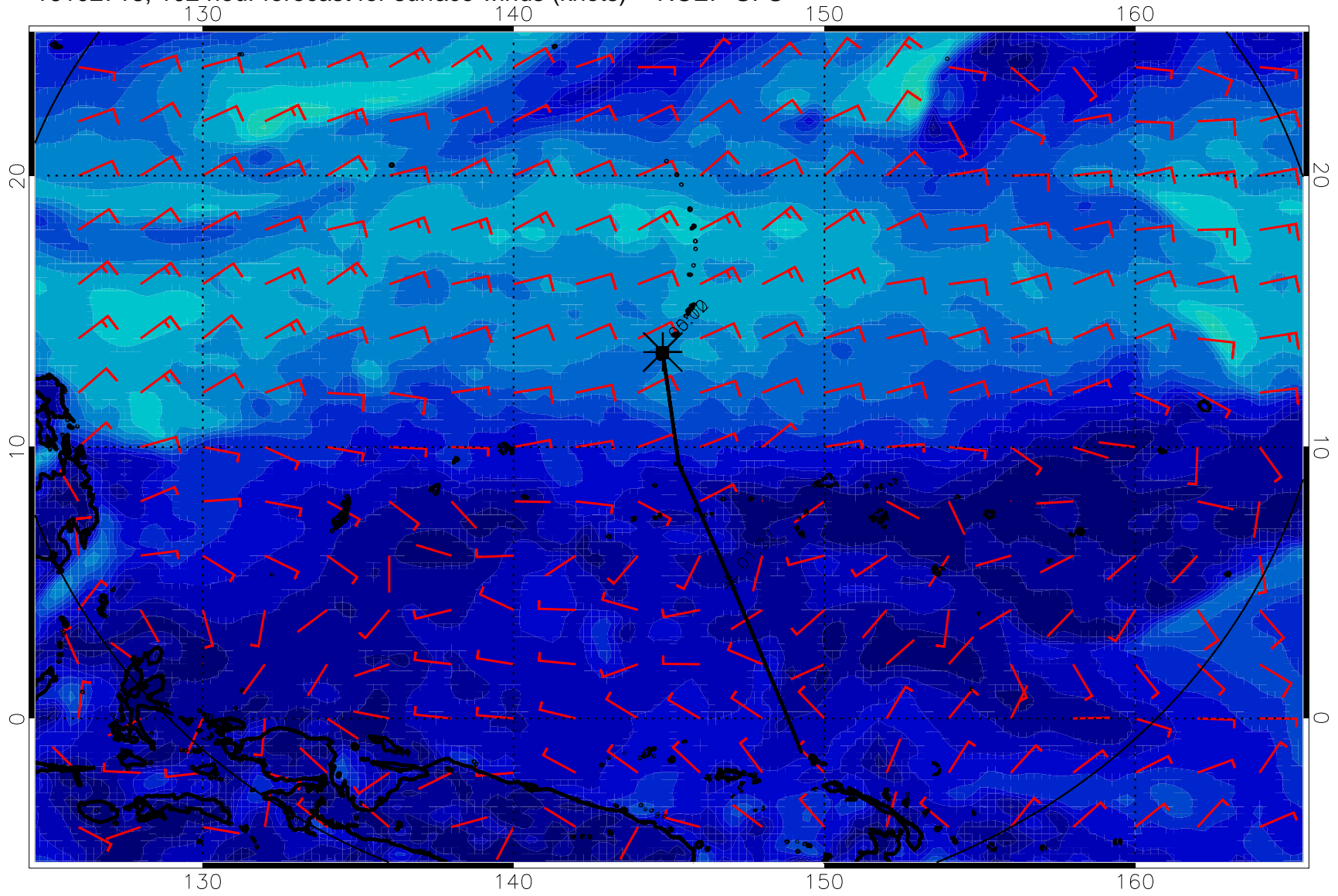
16102718, 102 hour forecast for surface winds (knots) -- NCEP GFS
