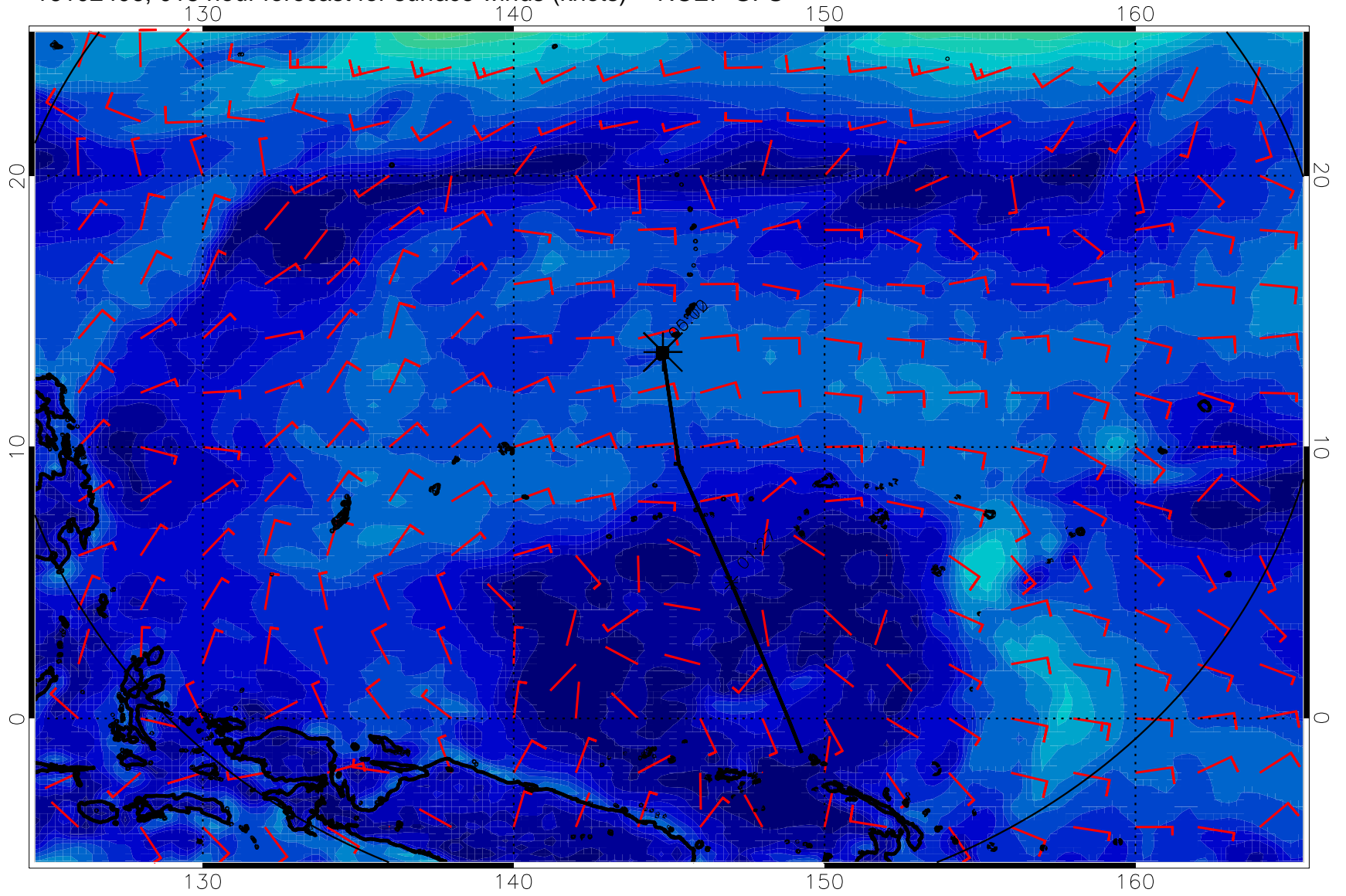
16102406, 018 hour forecast for surface winds (knots) -- NCEP GFS
