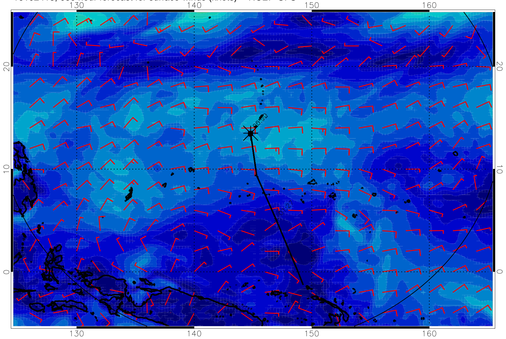
16102418, 030 hour forecast for surface winds (knots) -- NCEP GFS
