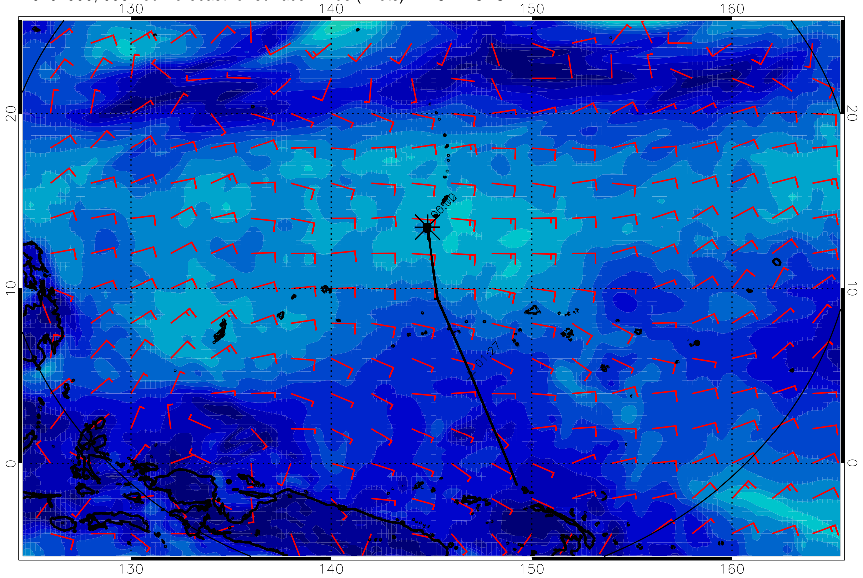
16102500, 036 hour forecast for surface winds (knots) -- NCEP GFS
