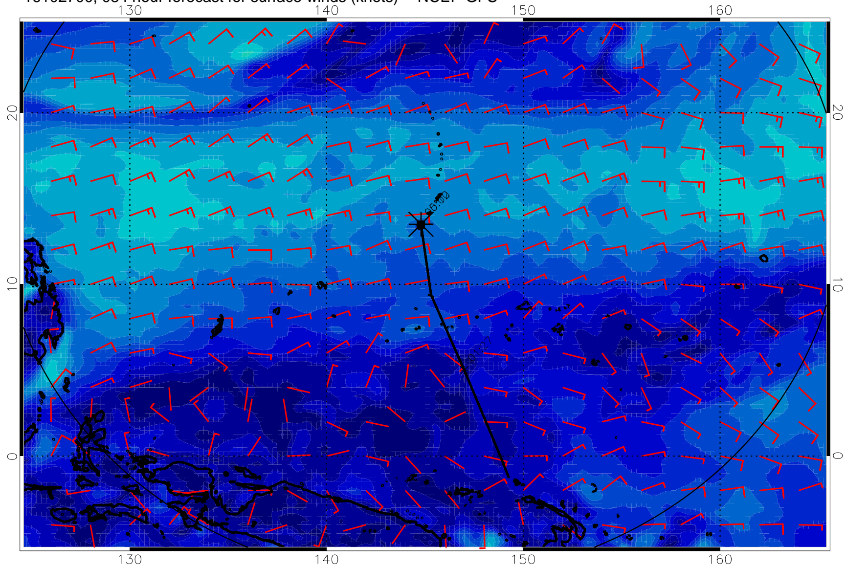
16102700, 084 hour forecast for surface winds (knots) -- NCEP GFS
