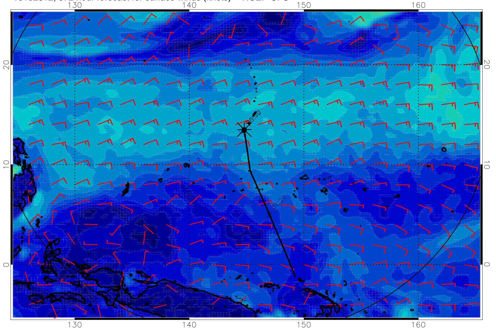
16102612, 072 hour forecast for surface winds (knots) -- NCEP GFS
