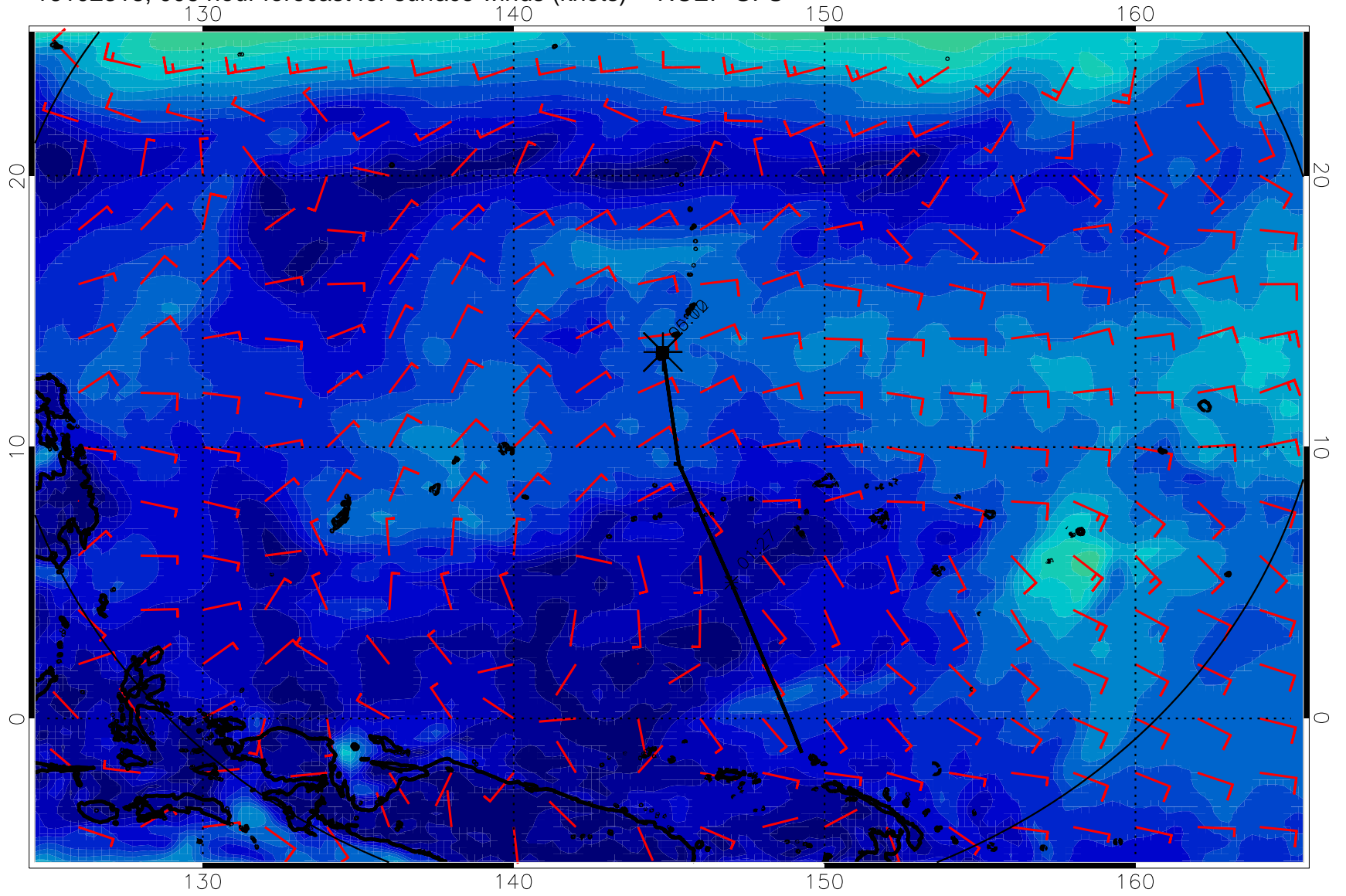
16102318, 006 hour forecast for surface winds (knots) -- NCEP GFS
