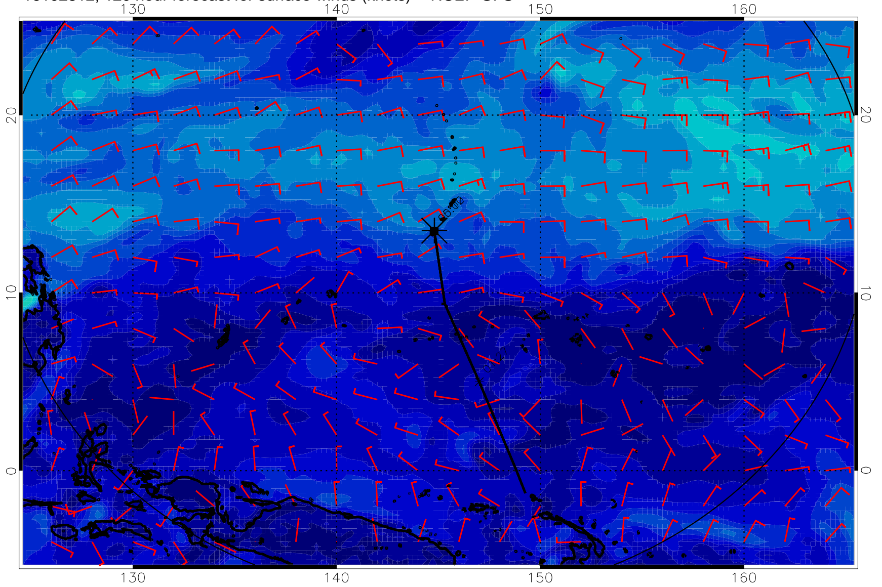
16102812, 120 hour forecast for surface winds (knots) -- NCEP GFS
