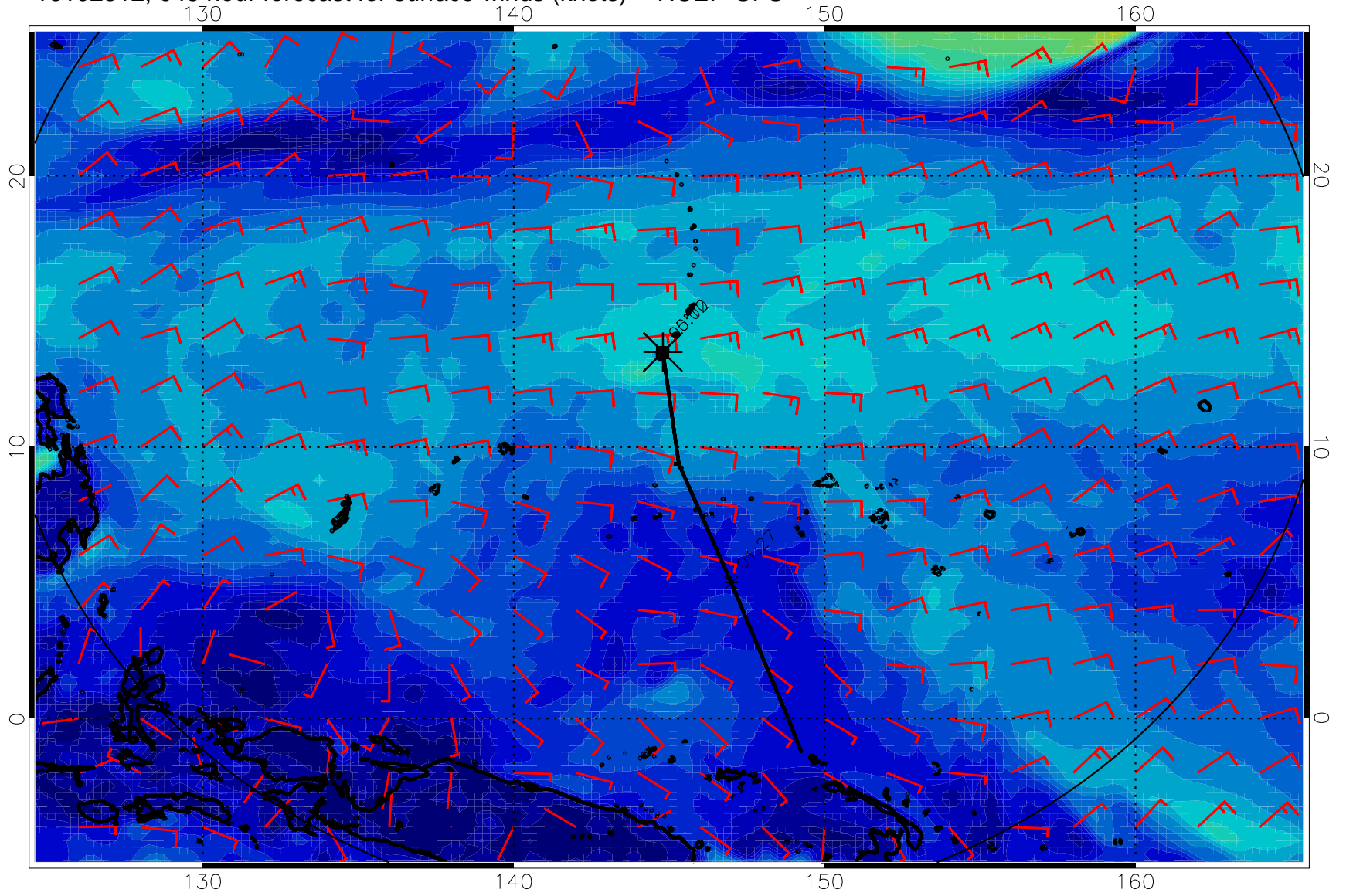
16102512, 048 hour forecast for surface winds (knots) -- NCEP GFS
