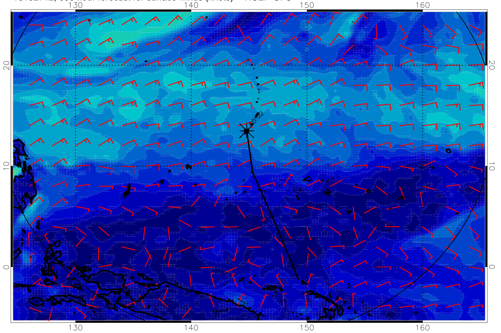
16102712, 096 hour forecast for surface winds (knots) -- NCEP GFS
