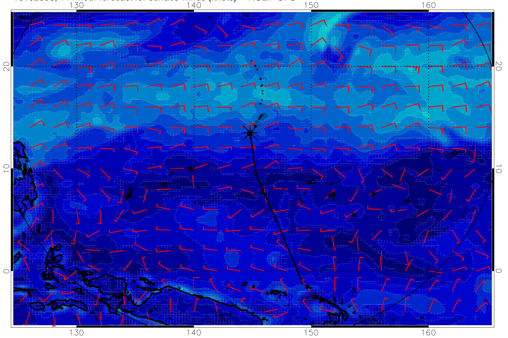
16102806, 114 hour forecast for surface winds (knots) -- NCEP GFS
