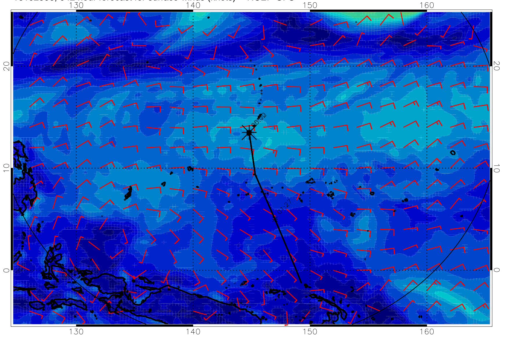
16102506, 042 hour forecast for surface winds (knots) -- NCEP GFS
