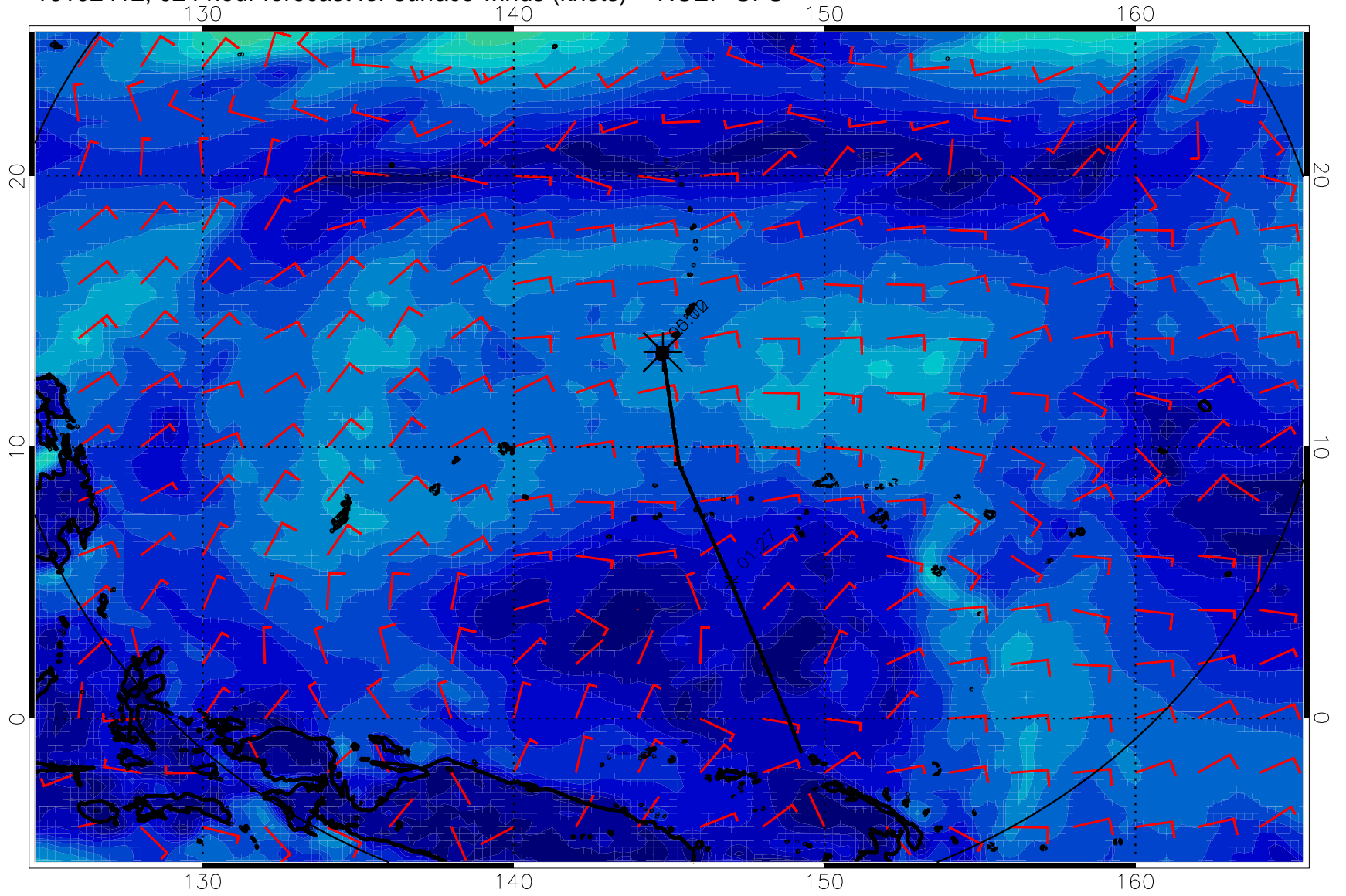
16102412, 024 hour forecast for surface winds (knots) -- NCEP GFS
