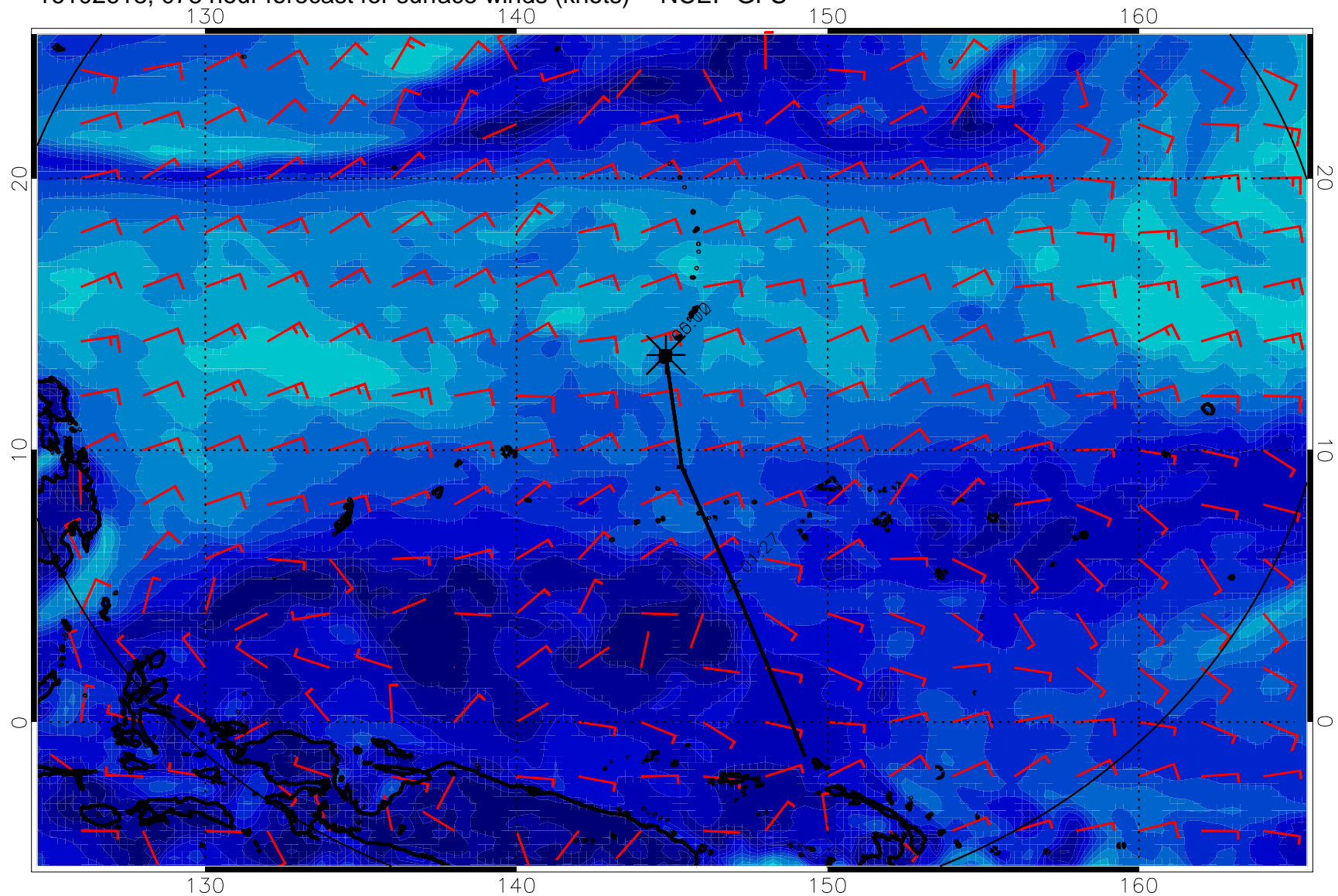
16102618, 078 hour forecast for surface winds (knots) -- NCEP GFS
