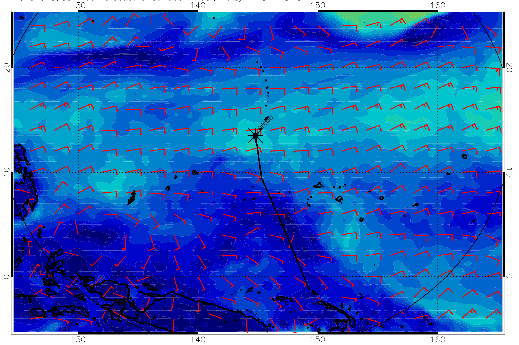
16102518, 054 hour forecast for surface winds (knots) -- NCEP GFS
