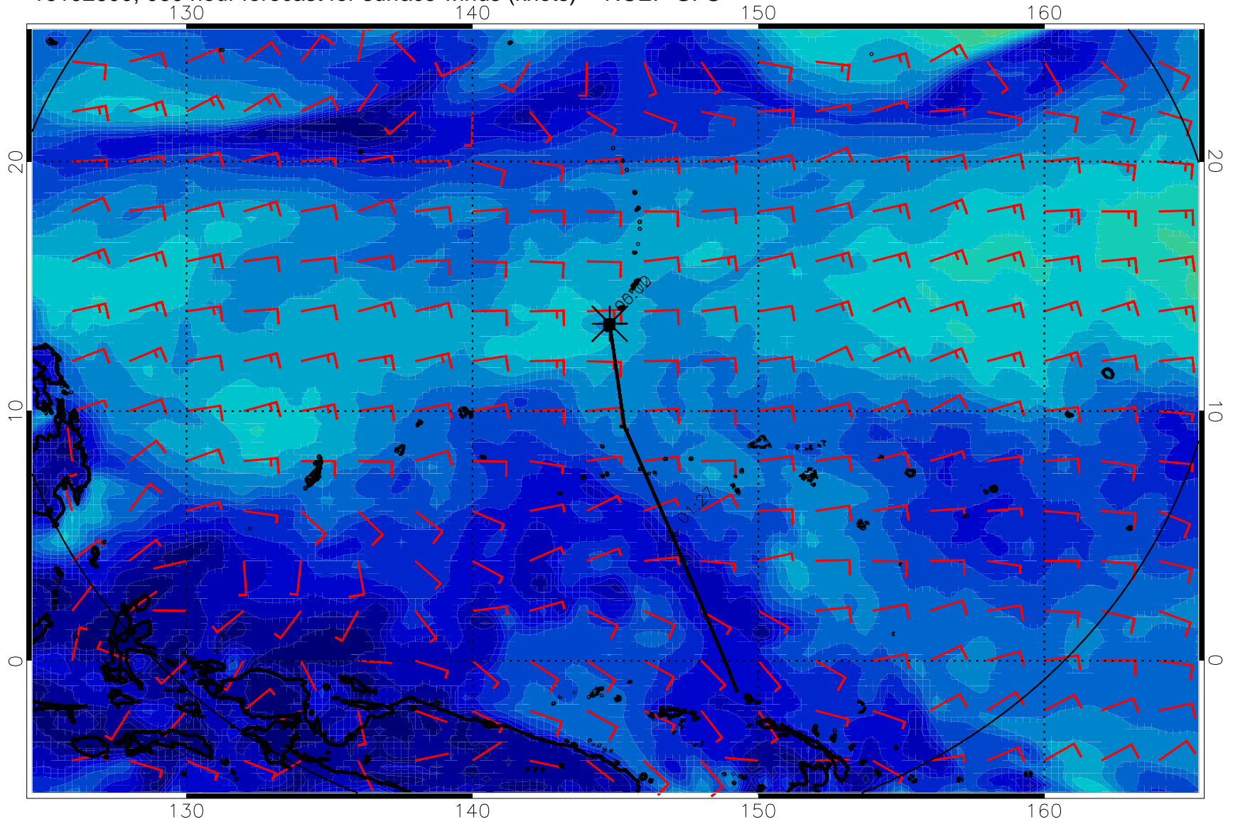
16102600, 060 hour forecast for surface winds (knots) -- NCEP GFS
