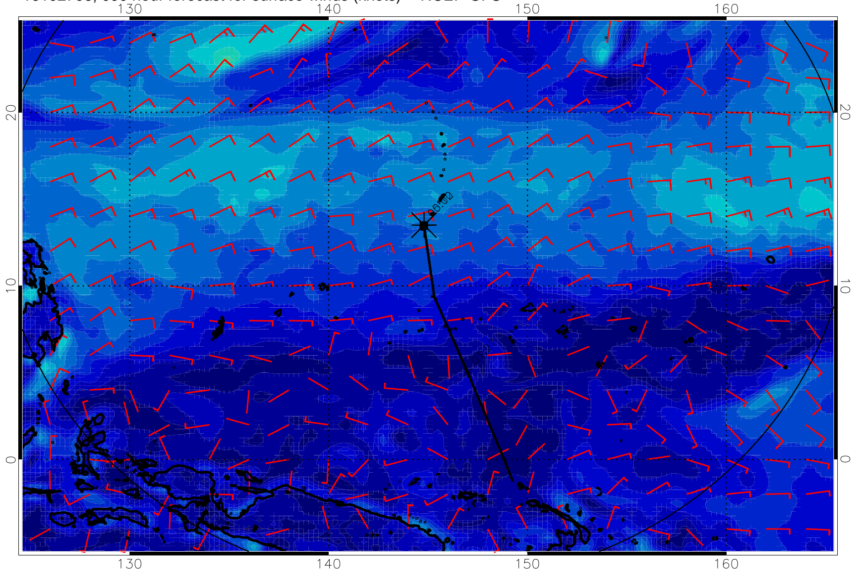
16102706, 090 hour forecast for surface winds (knots) -- NCEP GFS
