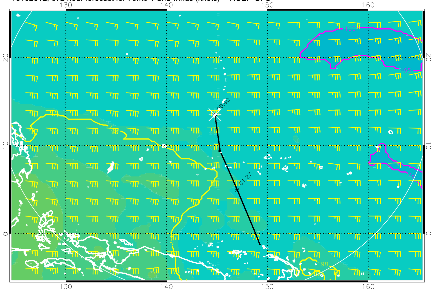
16102612, 072 hour forecast for 70mb T and winds (knots) -- NCEP GFS
