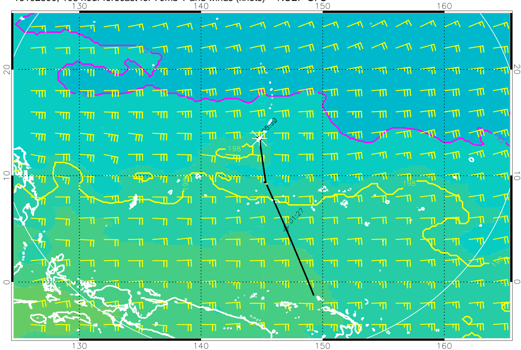
16102800, 108 hour forecast for 70mb T and winds (knots) -- NCEP GFS
