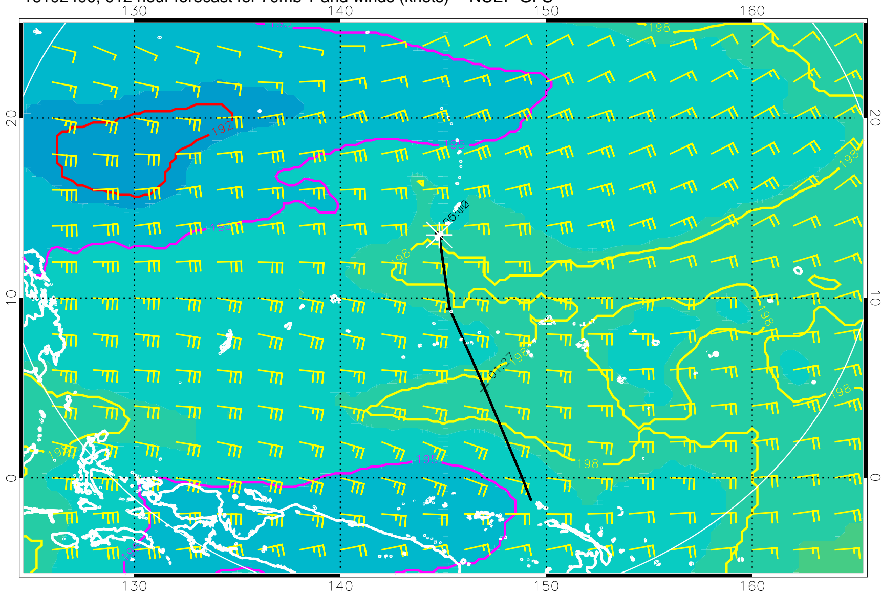
16102400, 012 hour forecast for 70mb T and winds (knots) -- NCEP GFS
