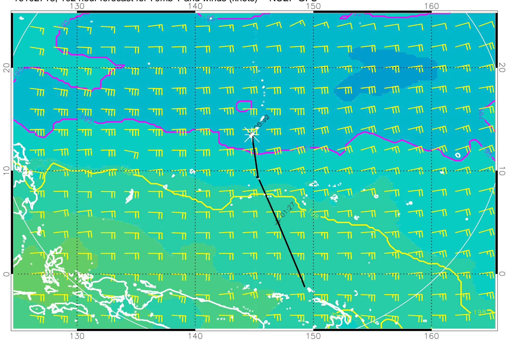
16102718, 102 hour forecast for 70mb T and winds (knots) -- NCEP GFS
