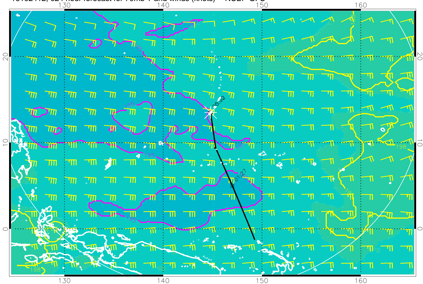
16102412, 024 hour forecast for 70mb T and winds (knots) -- NCEP GFS
