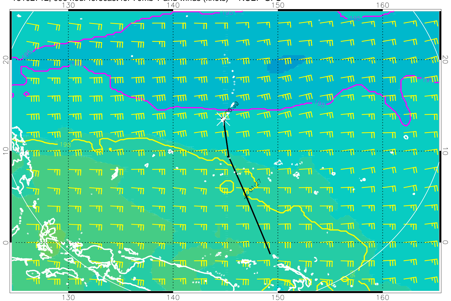
16102712, 096 hour forecast for 70mb T and winds (knots) -- NCEP GFS
