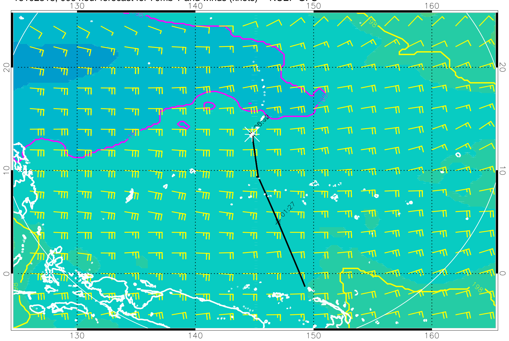
16102318, 006 hour forecast for 70mb T and winds (knots) -- NCEP GFS
