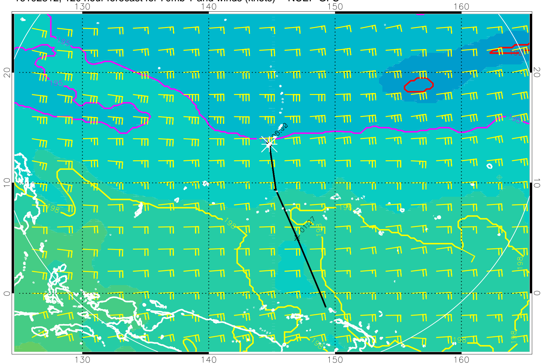
16102812, 120 hour forecast for 70mb T and winds (knots) -- NCEP GFS
