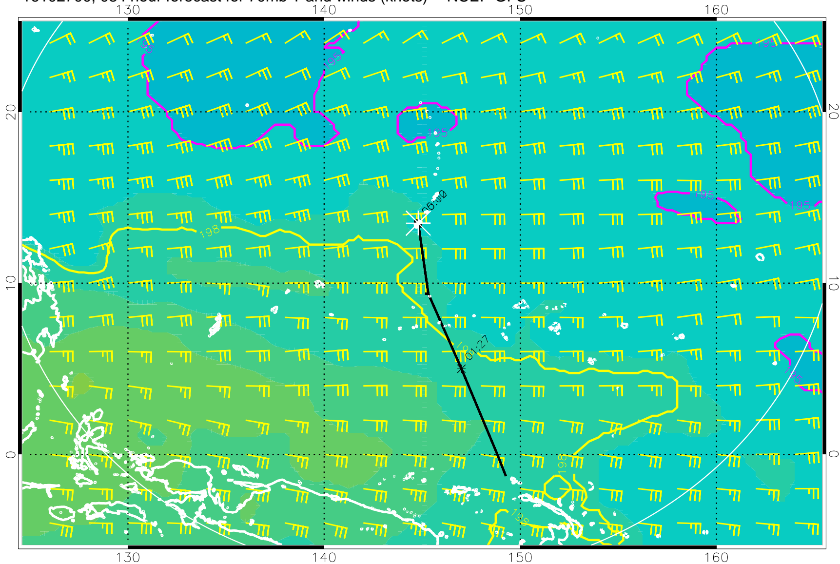
16102700, 084 hour forecast for 70mb T and winds (knots) -- NCEP GFS
