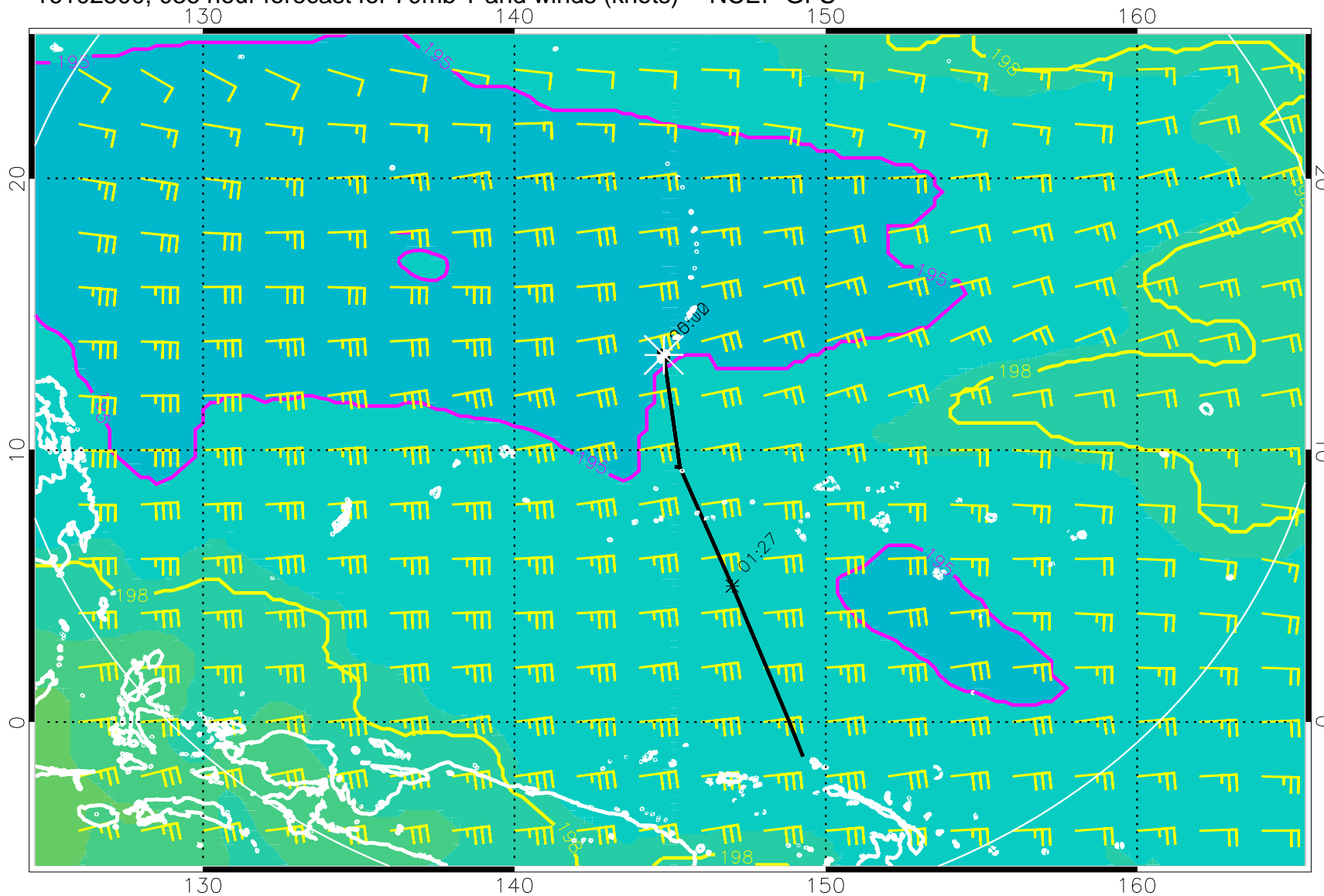
16102500, 036 hour forecast for 70mb T and winds (knots) -- NCEP GFS
