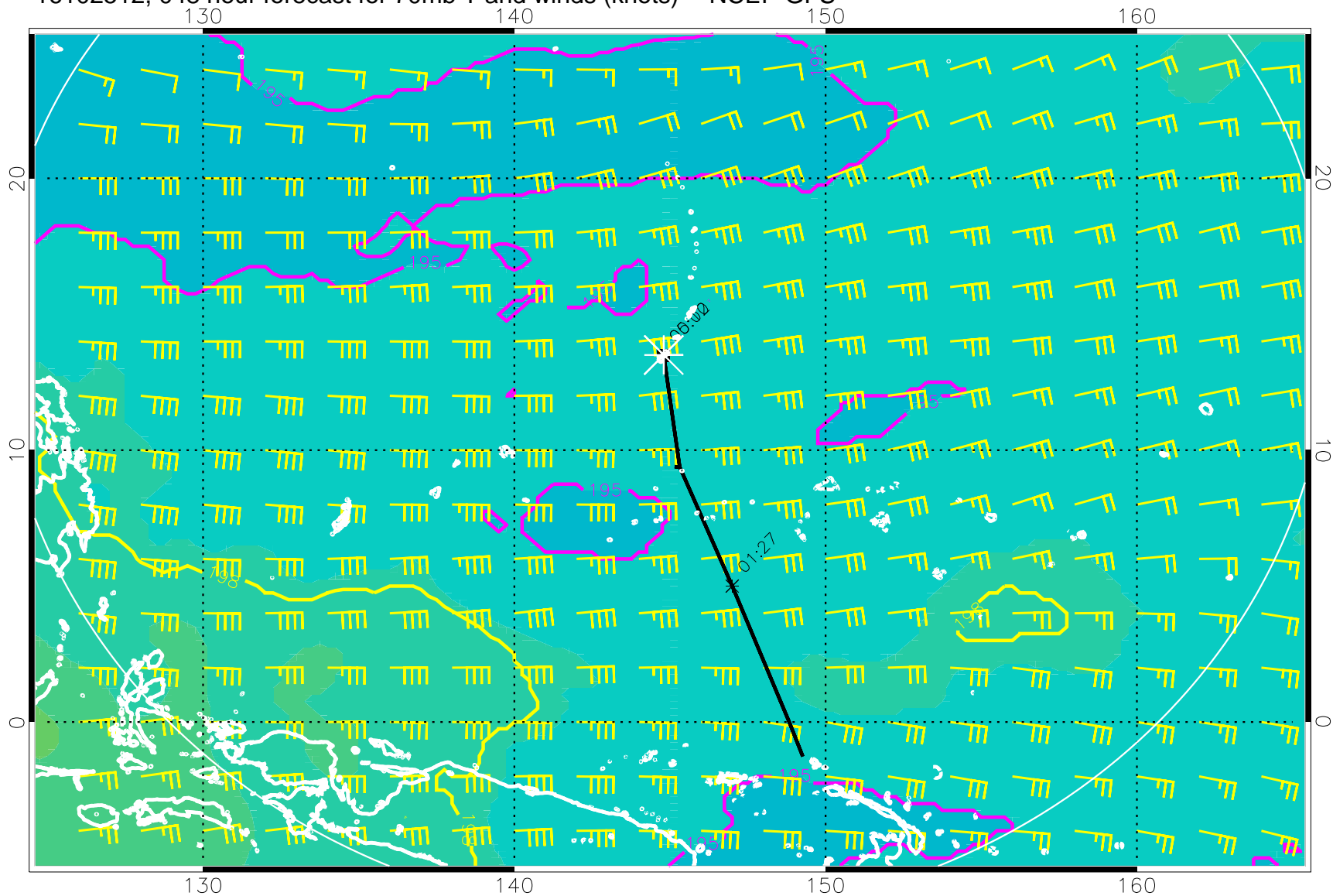
16102512, 048 hour forecast for 70mb T and winds (knots) -- NCEP GFS
