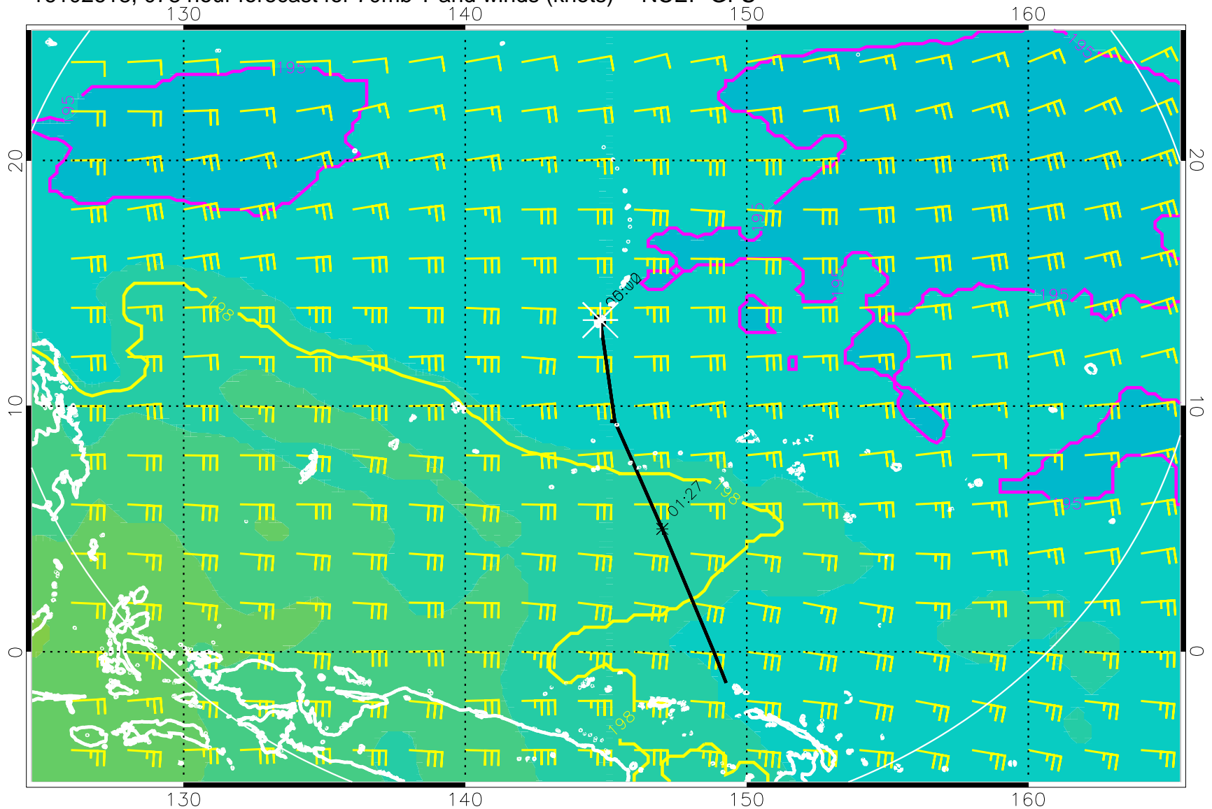
16102618, 078 hour forecast for 70mb T and winds (knots) -- NCEP GFS
