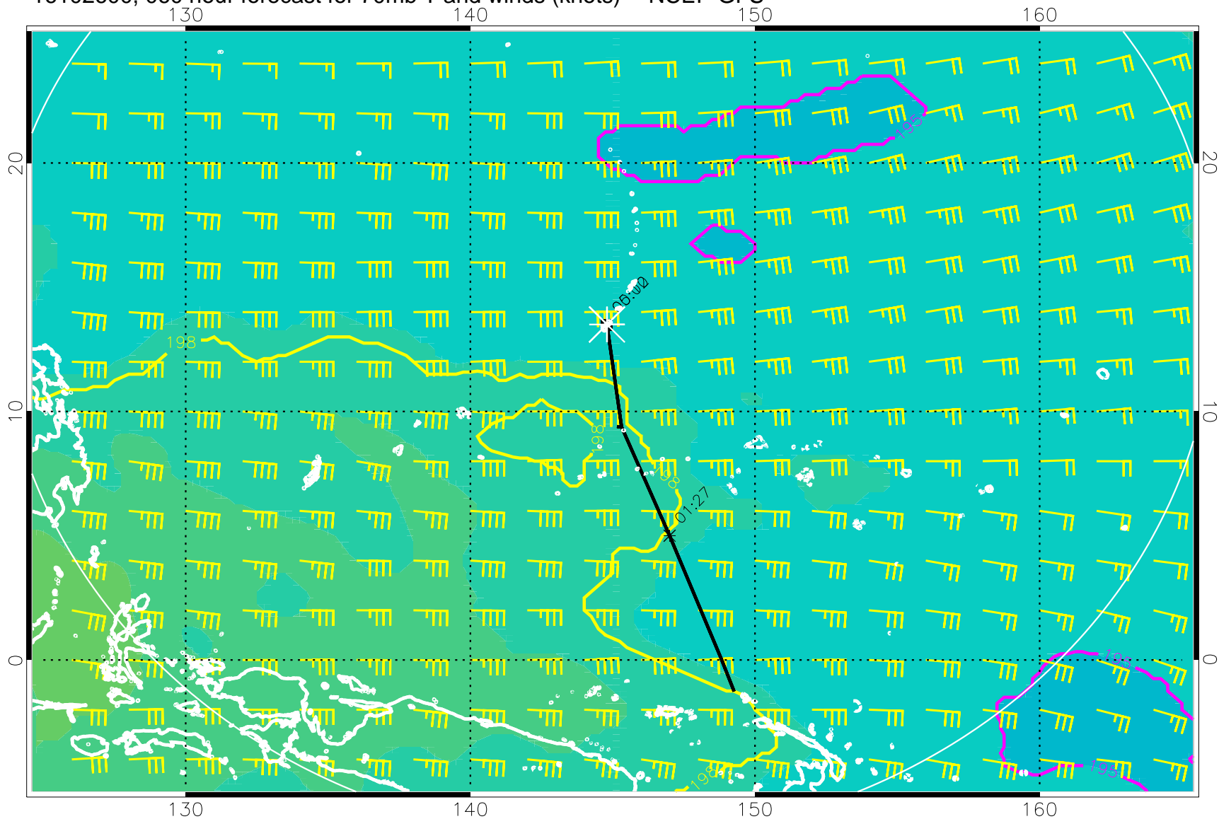
16102600, 060 hour forecast for 70mb T and winds (knots) -- NCEP GFS
