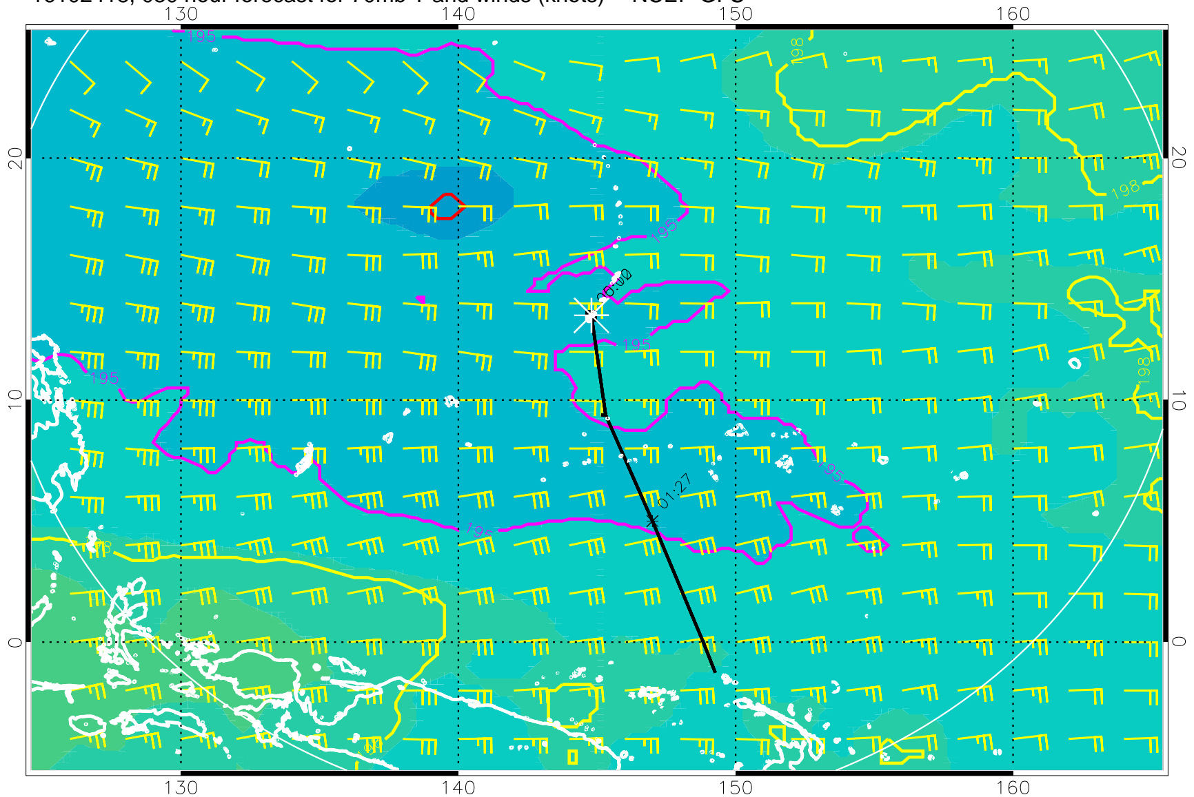
16102418, 030 hour forecast for 70mb T and winds (knots) -- NCEP GFS
