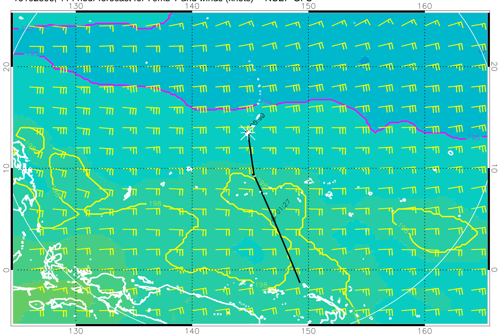
16102806, 114 hour forecast for 70mb T and winds (knots) -- NCEP GFS
