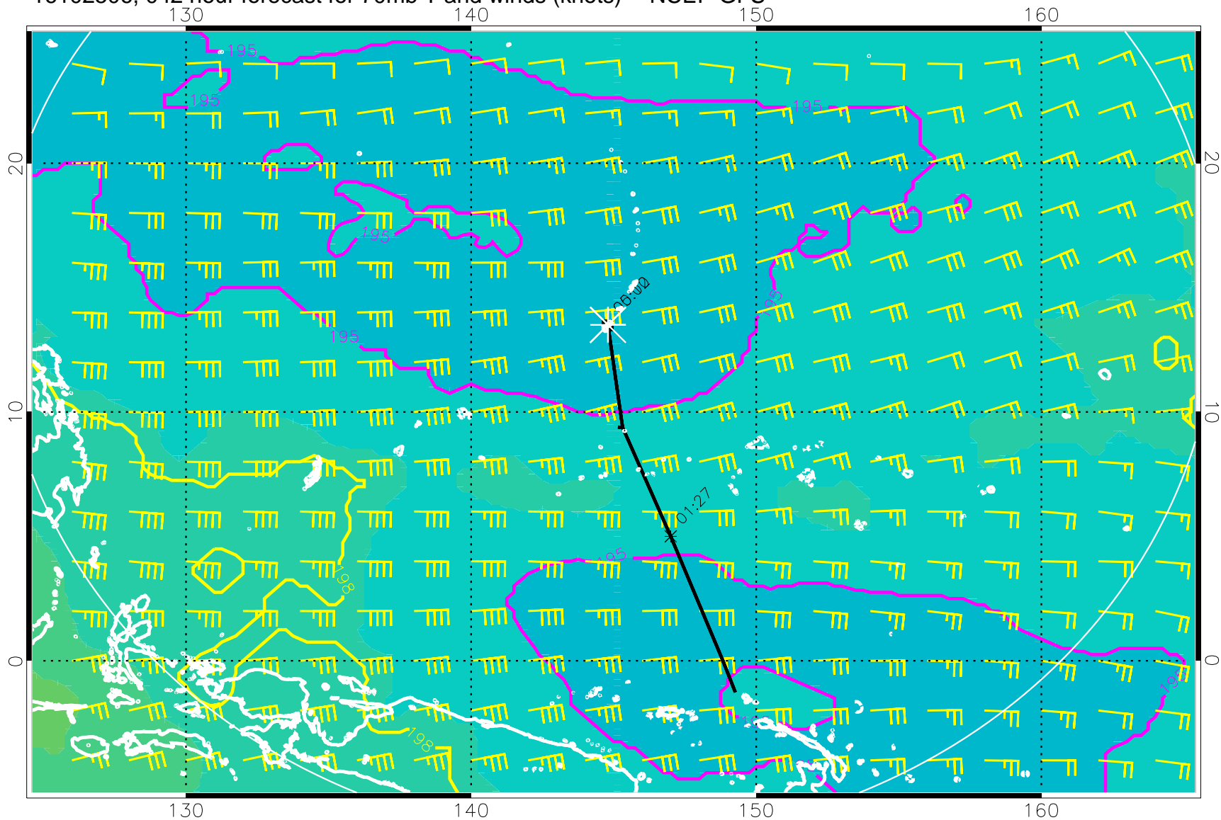
16102506, 042 hour forecast for 70mb T and winds (knots) -- NCEP GFS
