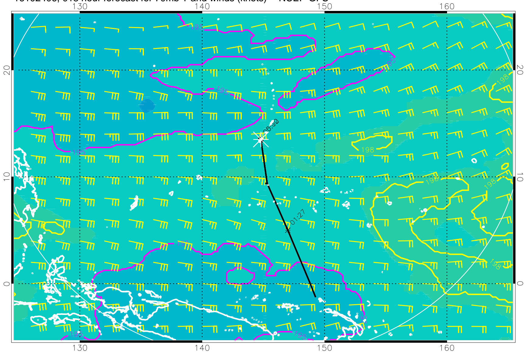
16102406, 018 hour forecast for 70mb T and winds (knots) -- NCEP GFS
