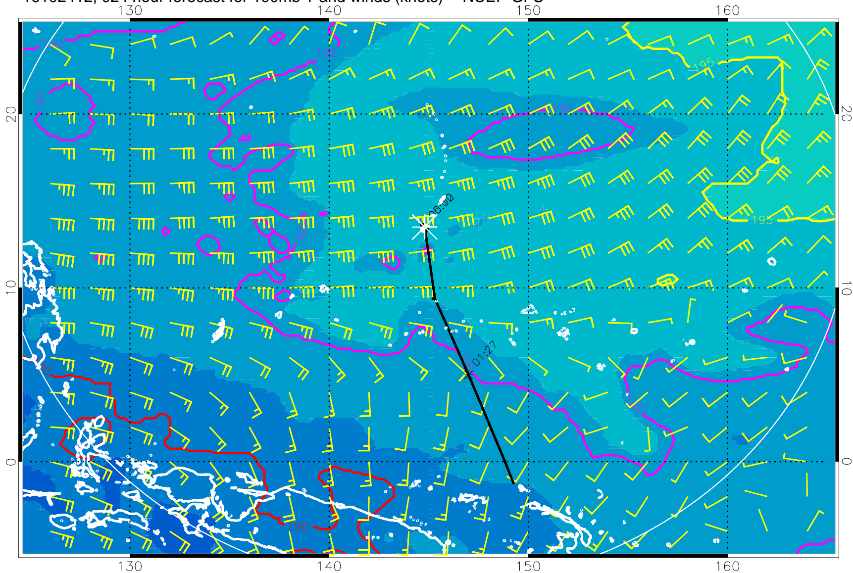
16102412, 024 hour forecast for 100mb T and winds (knots) -- NCEP GFS
