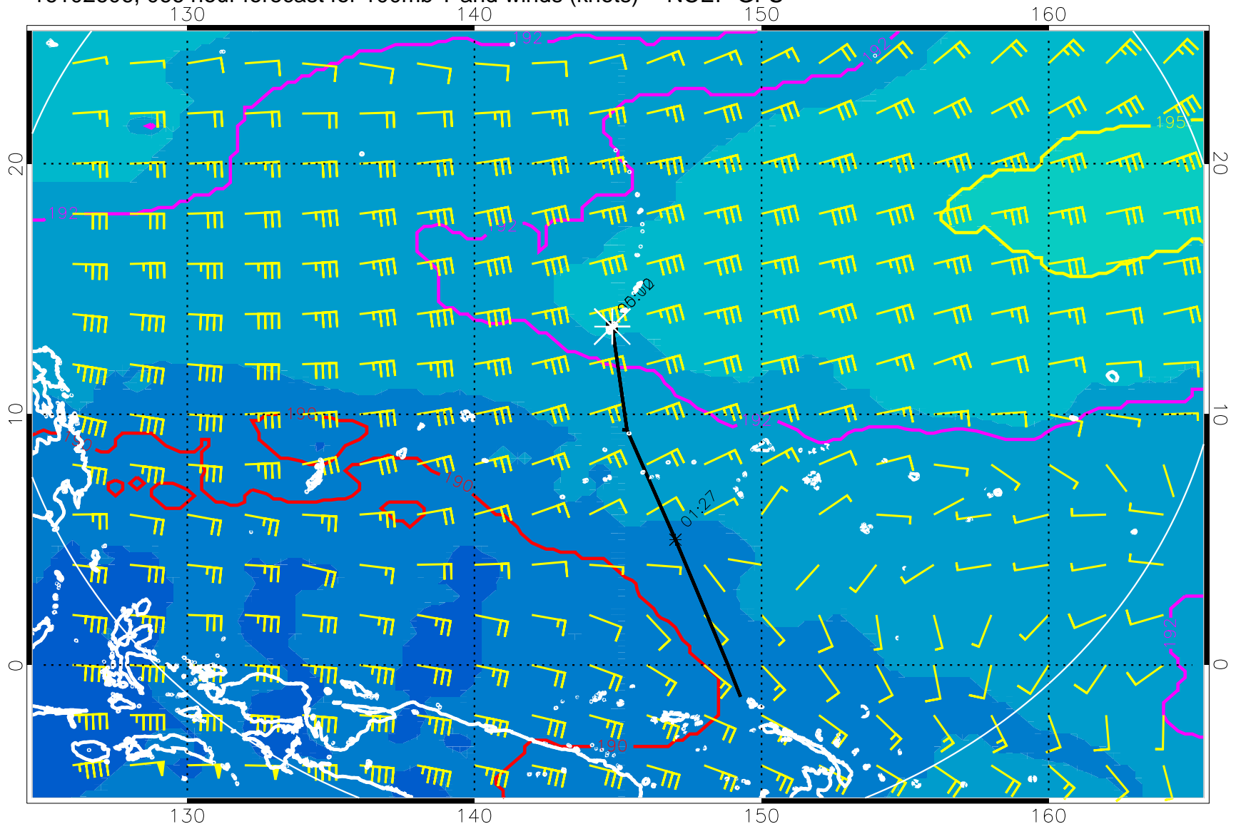
16102606, 066 hour forecast for 100mb T and winds (knots) -- NCEP GFS
