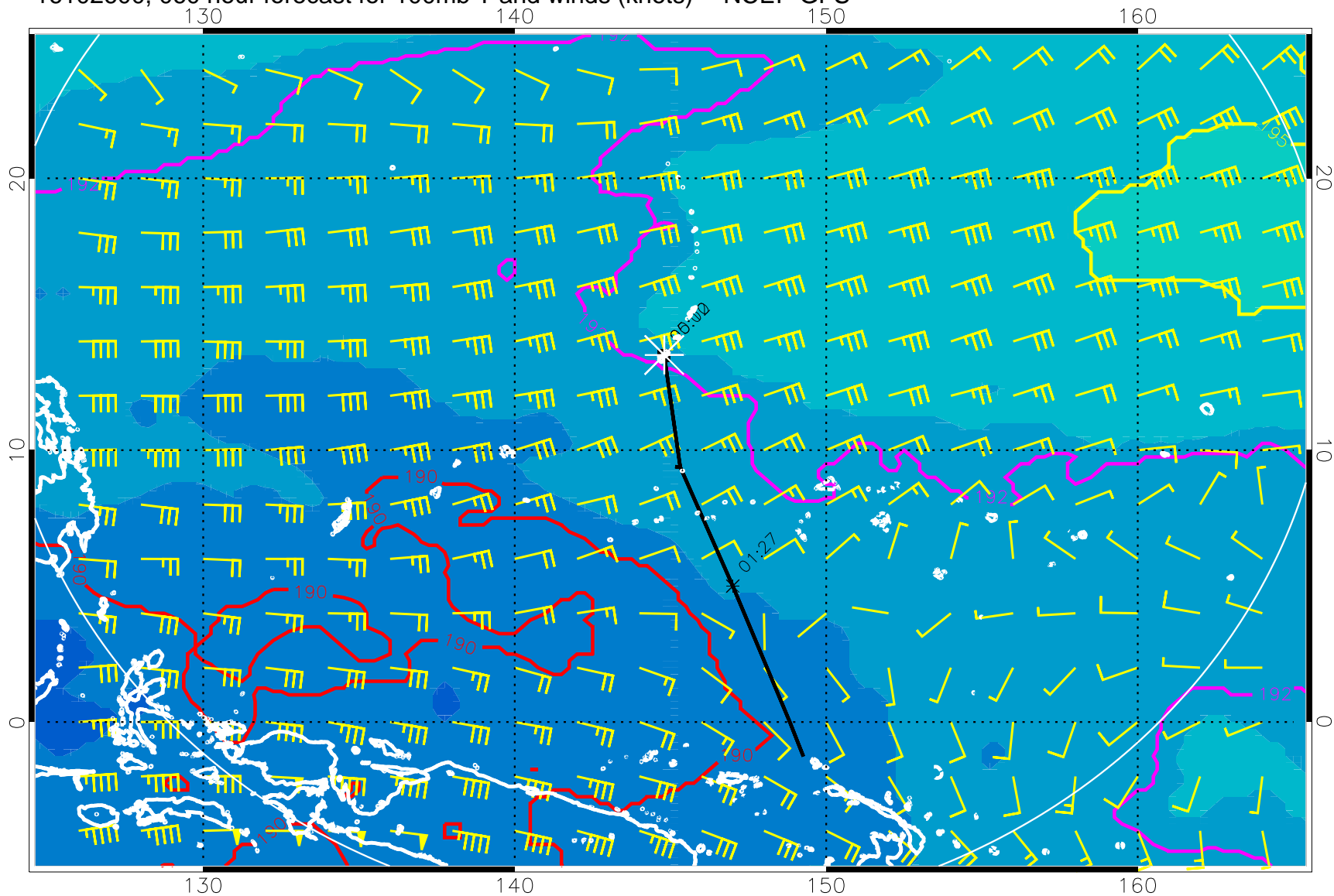
16102600, 060 hour forecast for 100mb T and winds (knots) -- NCEP GFS
