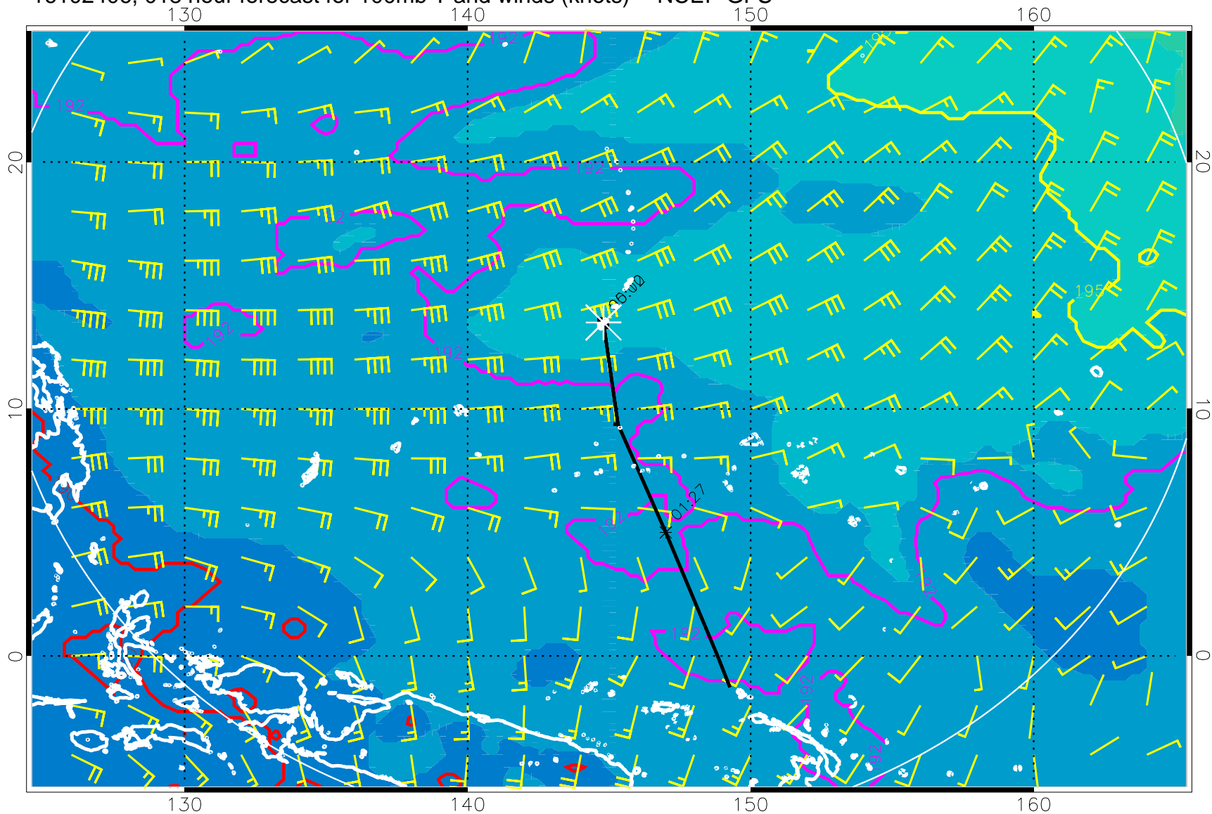
16102406, 018 hour forecast for 100mb T and winds (knots) -- NCEP GFS
