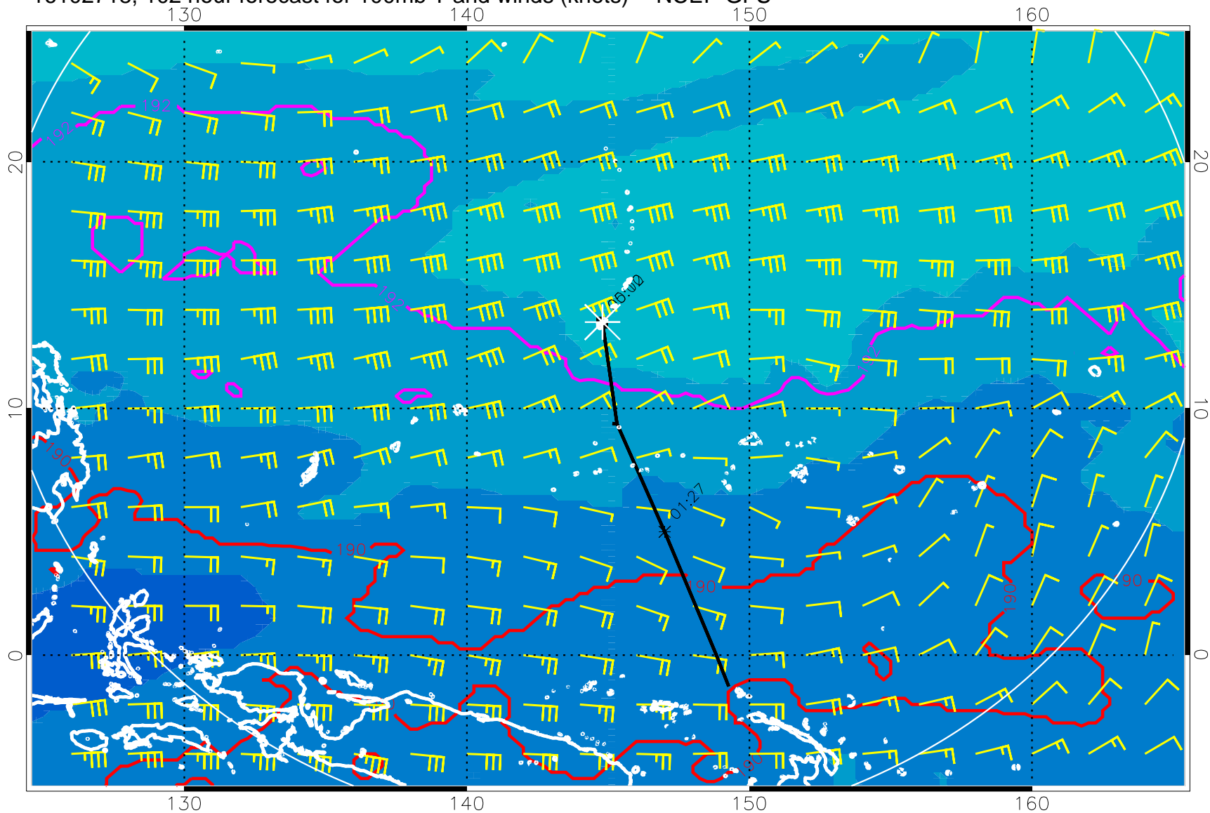
16102718, 102 hour forecast for 100mb T and winds (knots) -- NCEP GFS
