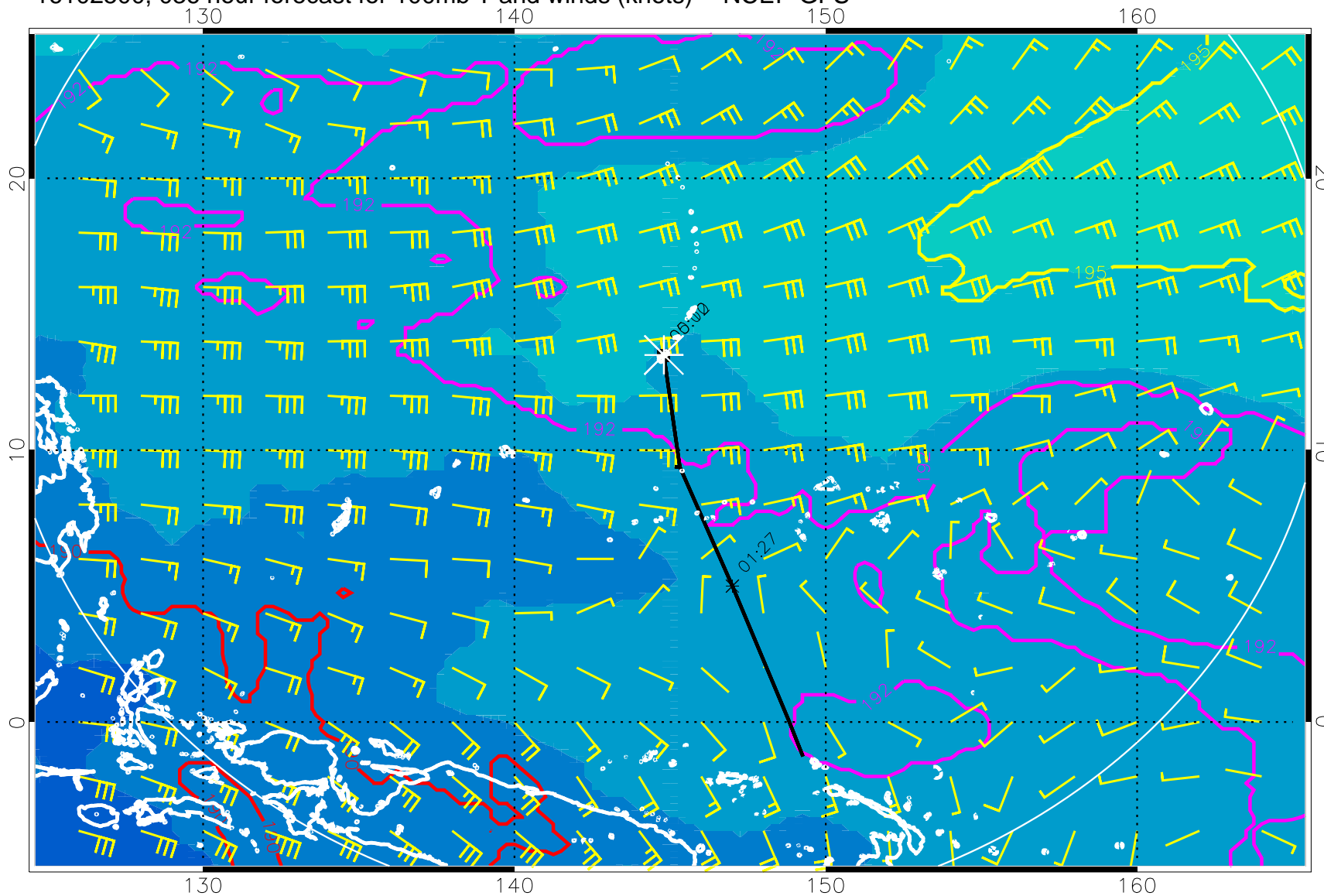
16102500, 036 hour forecast for 100mb T and winds (knots) -- NCEP GFS
