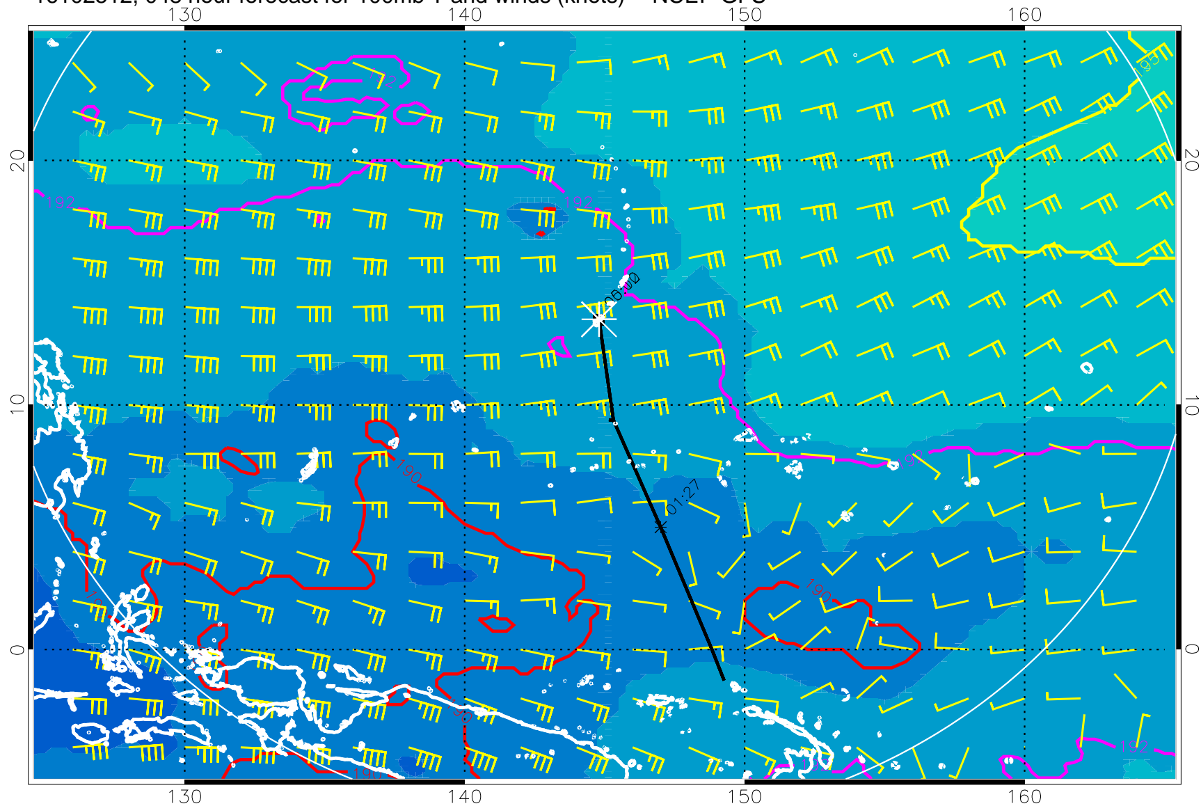
16102512, 048 hour forecast for 100mb T and winds (knots) -- NCEP GFS
