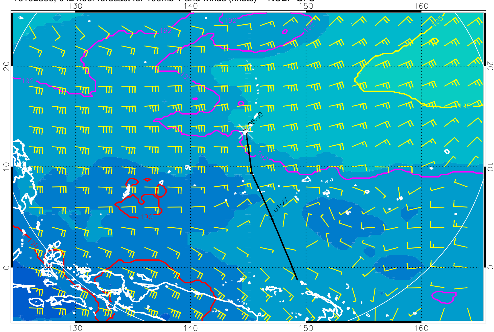
16102506, 042 hour forecast for 100mb T and winds (knots) -- NCEP GFS
