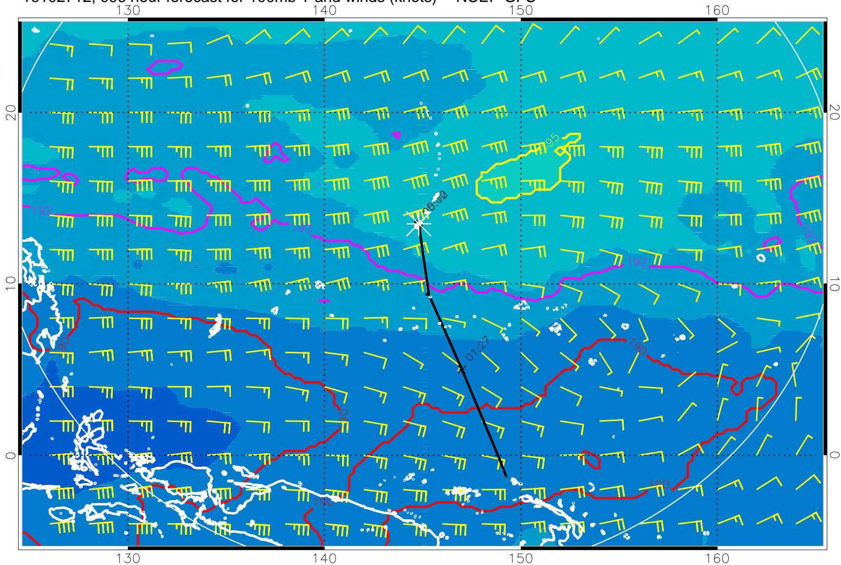
16102712, 096 hour forecast for 100mb T and winds (knots) -- NCEP GFS
