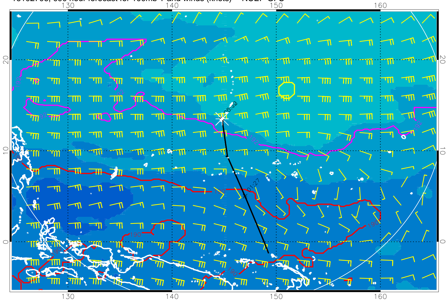
16102706, 090 hour forecast for 100mb T and winds (knots) -- NCEP GFS
