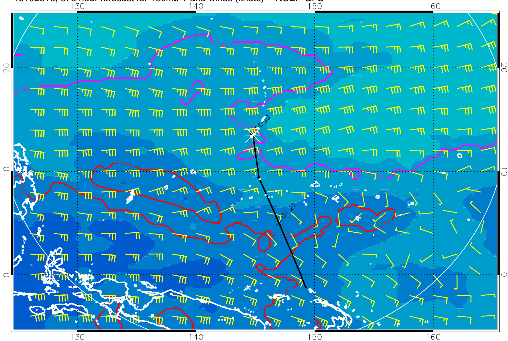
16102618, 078 hour forecast for 100mb T and winds (knots) -- NCEP GFS
