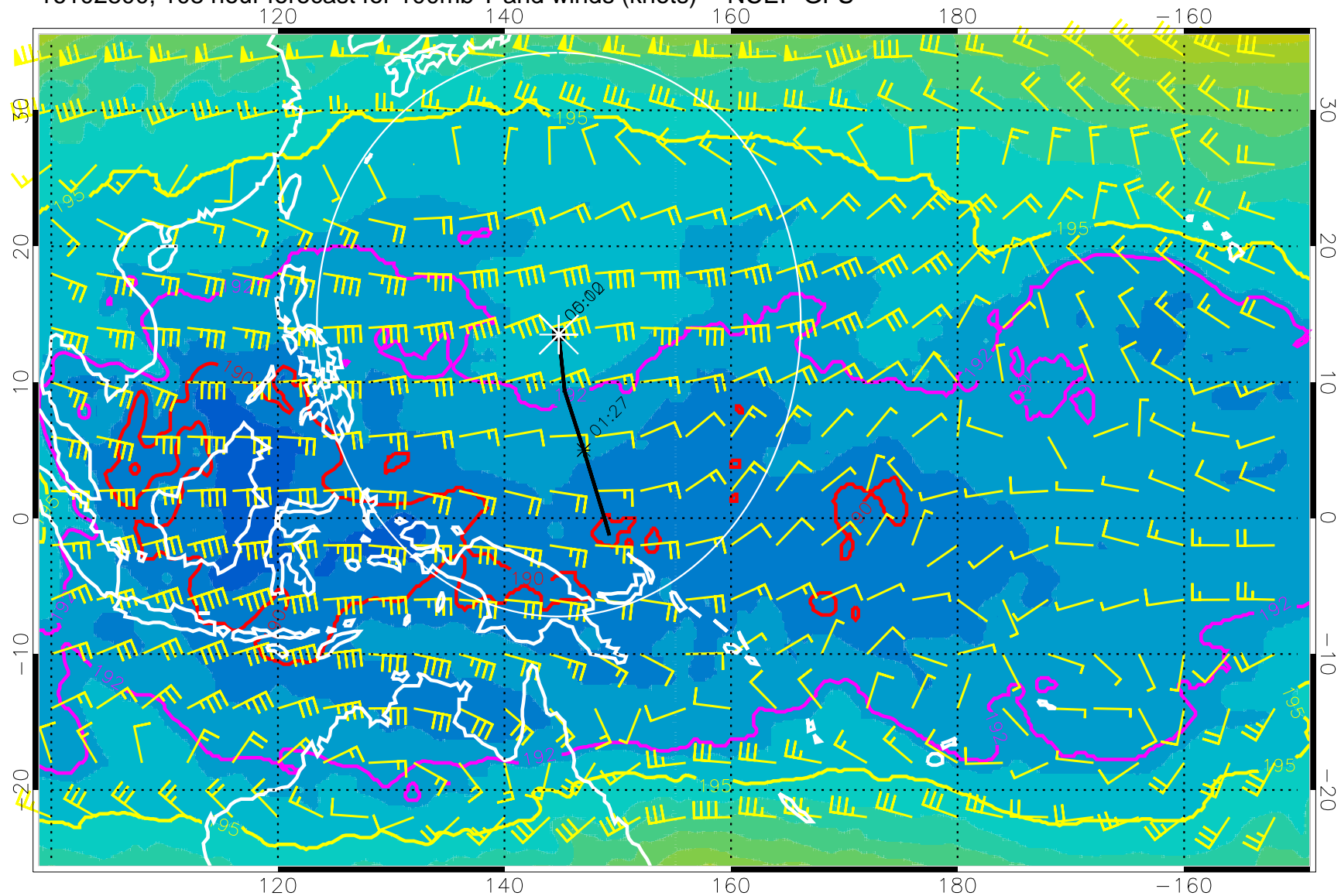
16102800, 108 hour forecast for 100mb T and winds (knots) -- NCEP GFS
