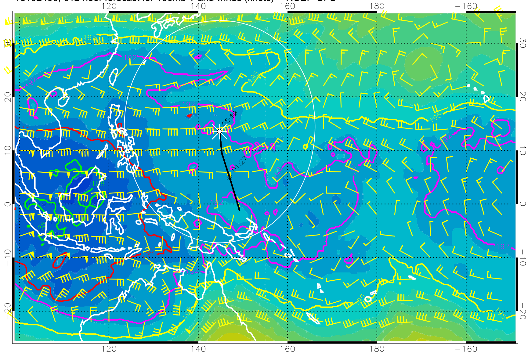
16102400, 012 hour forecast for 100mb T and winds (knots) -- NCEP GFS
