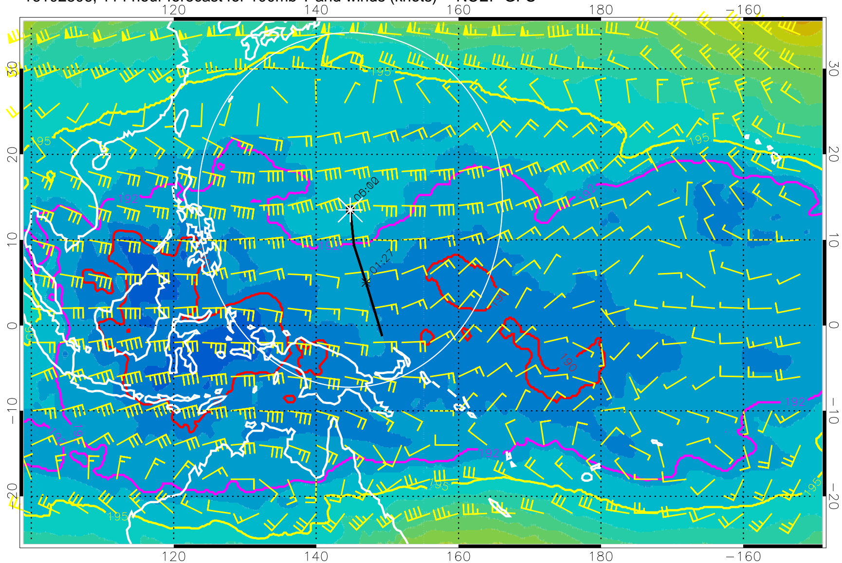
16102806, 114 hour forecast for 100mb T and winds (knots) -- NCEP GFS
