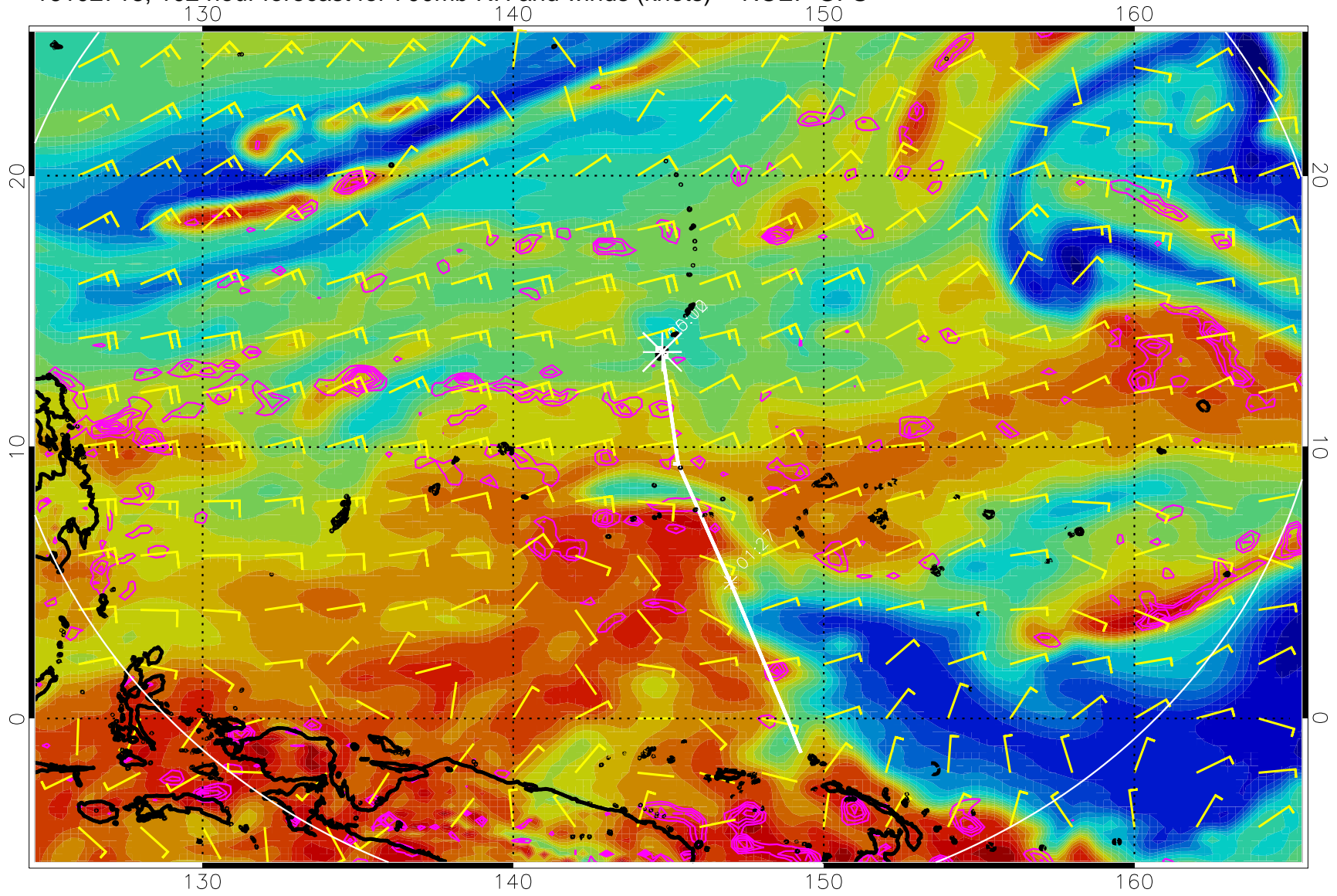
16102718, 102 hour forecast for 700mb RH and winds (knots) -- NCEP GFS
