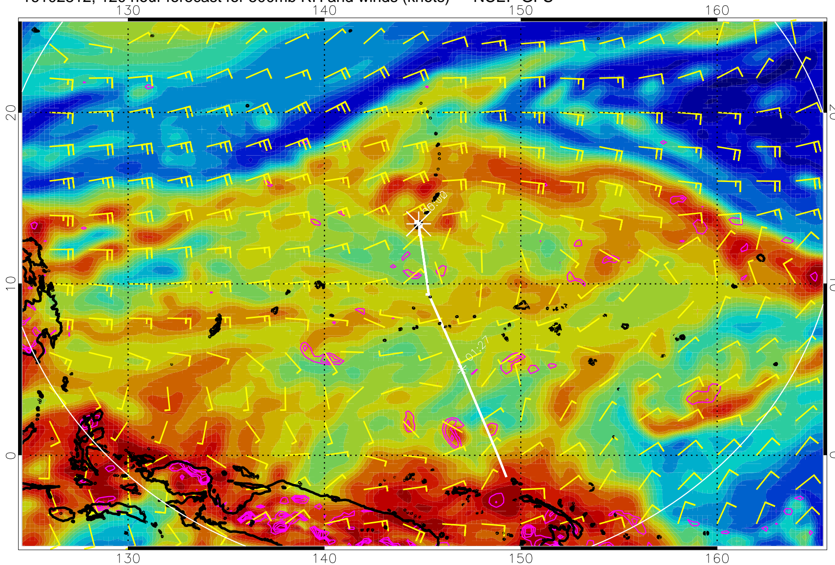
16102812, 120 hour forecast for 500mb RH and winds (knots) -- NCEP GFS
