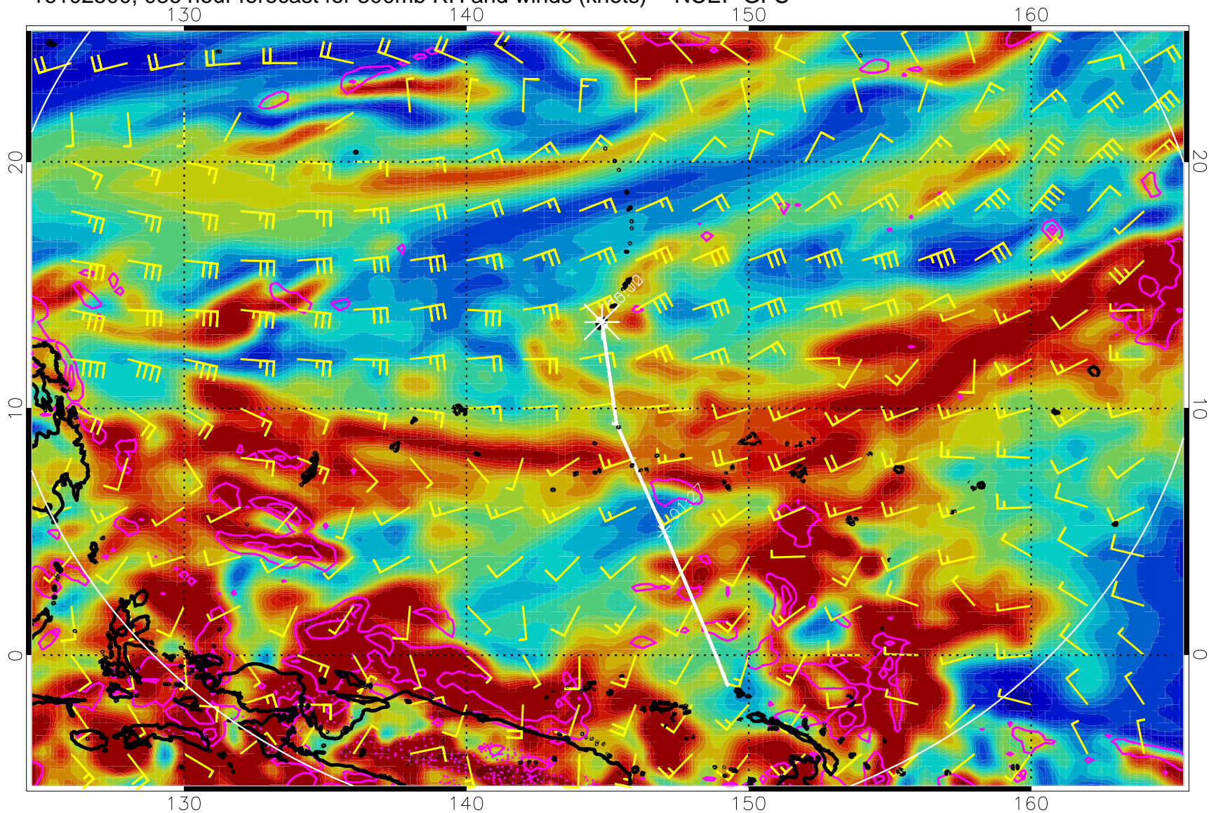
16102500, 036 hour forecast for 300mb RH and winds (knots) -- NCEP GFS
