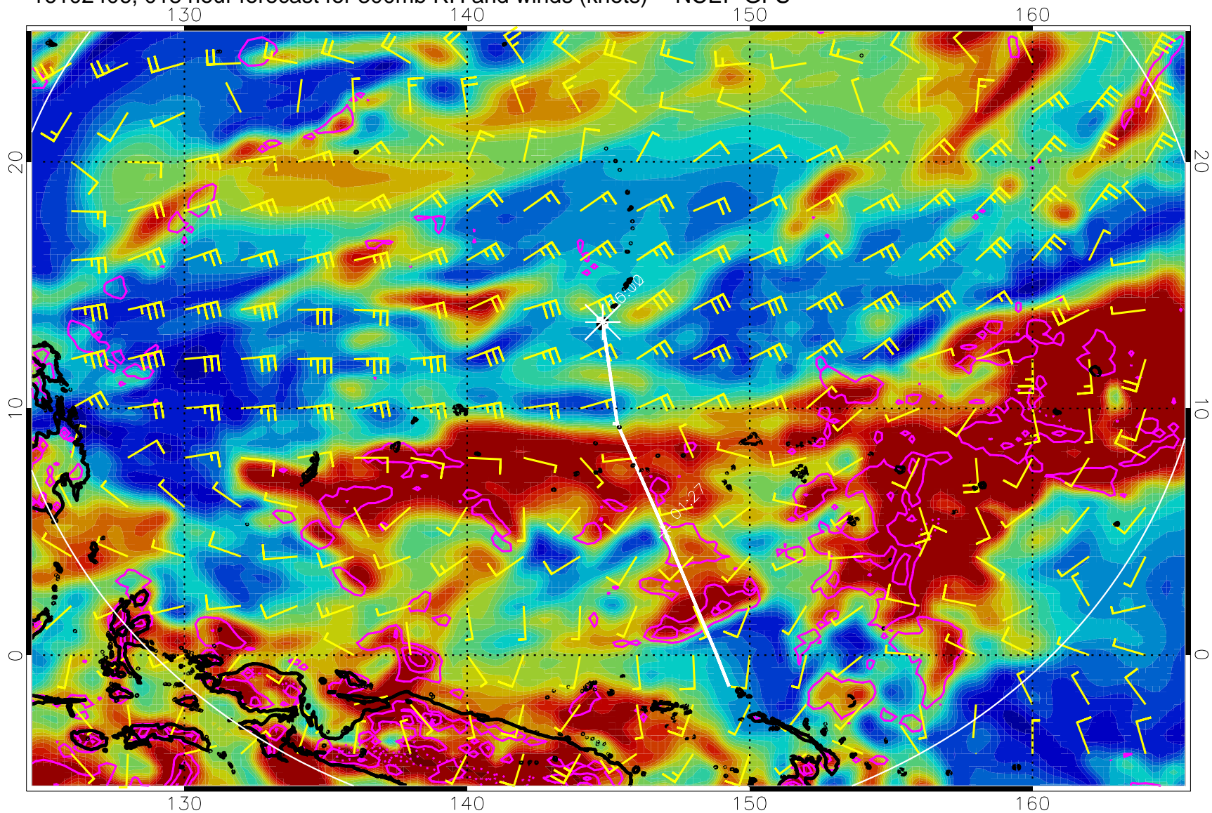
16102406, 018 hour forecast for 300mb RH and winds (knots) -- NCEP GFS
