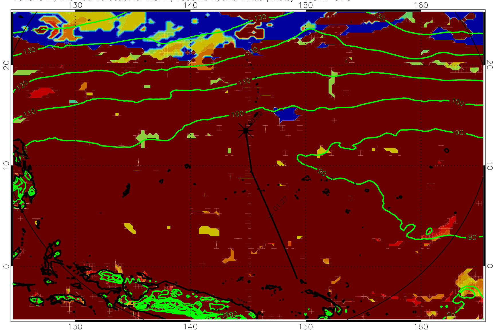
16102812, 120 hour forecast for HCAL, 1000mb Z, and winds (knots) -- NCEP GFS
