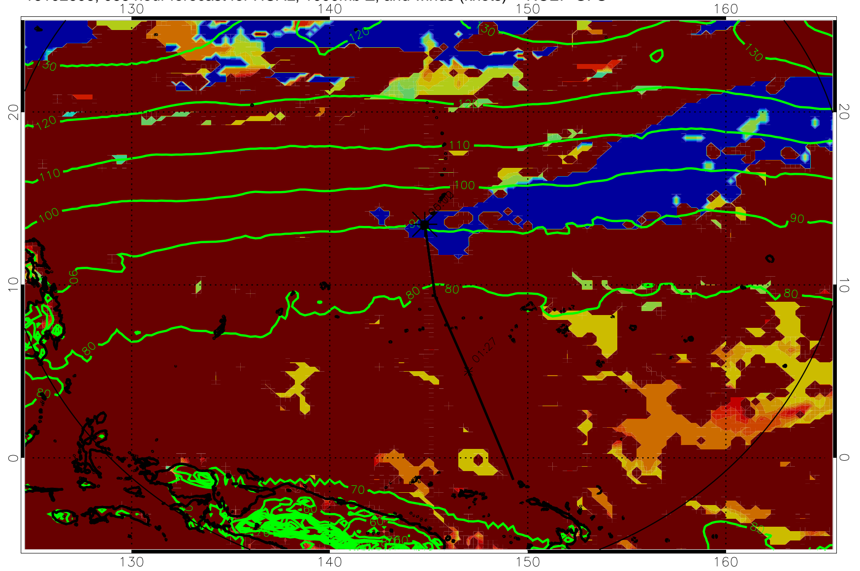
16102606, 066 hour forecast for HCAL, 1000mb Z, and winds (knots) -- NCEP GFS
