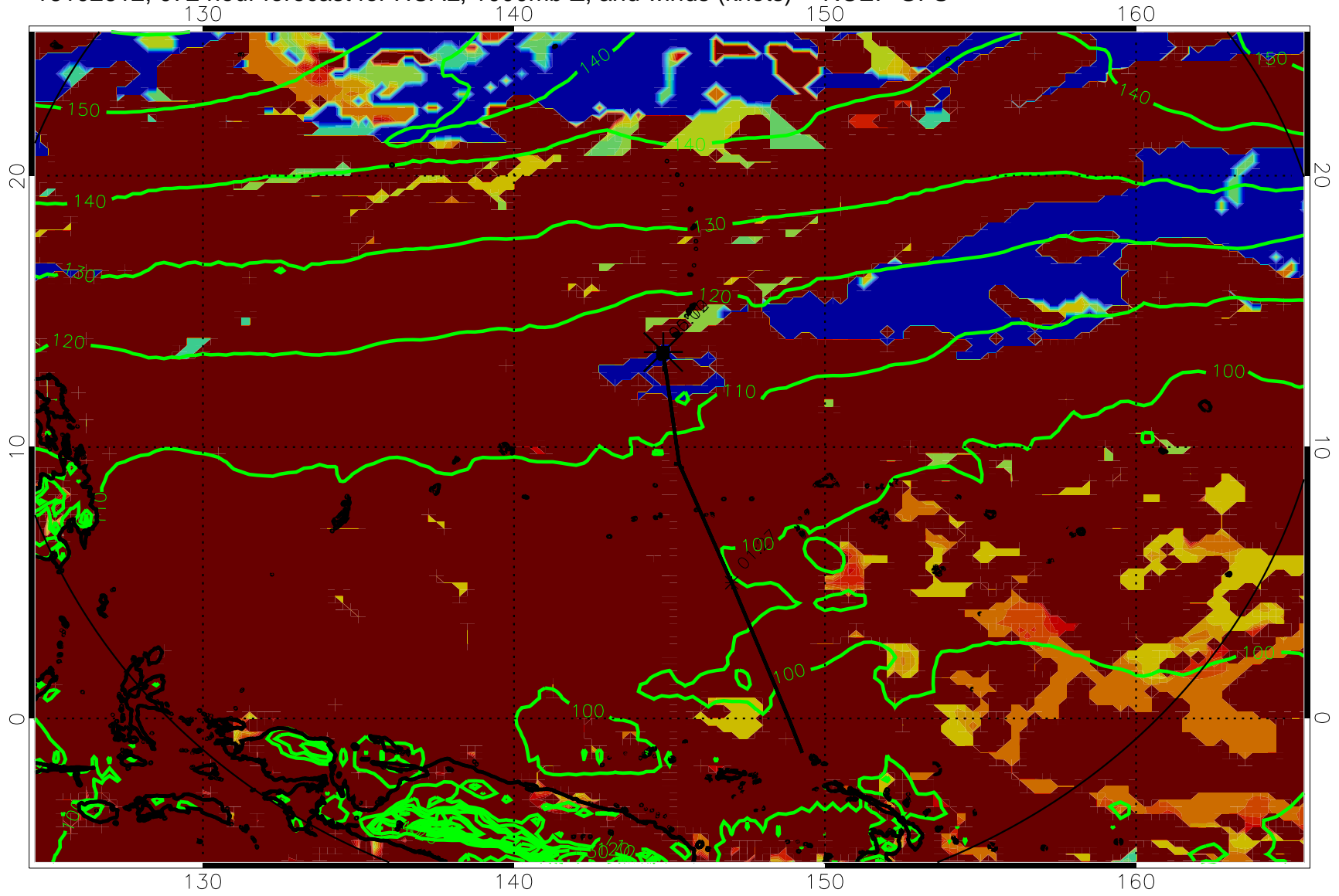
16102612, 072 hour forecast for HCAL, 1000mb Z, and winds (knots) -- NCEP GFS
