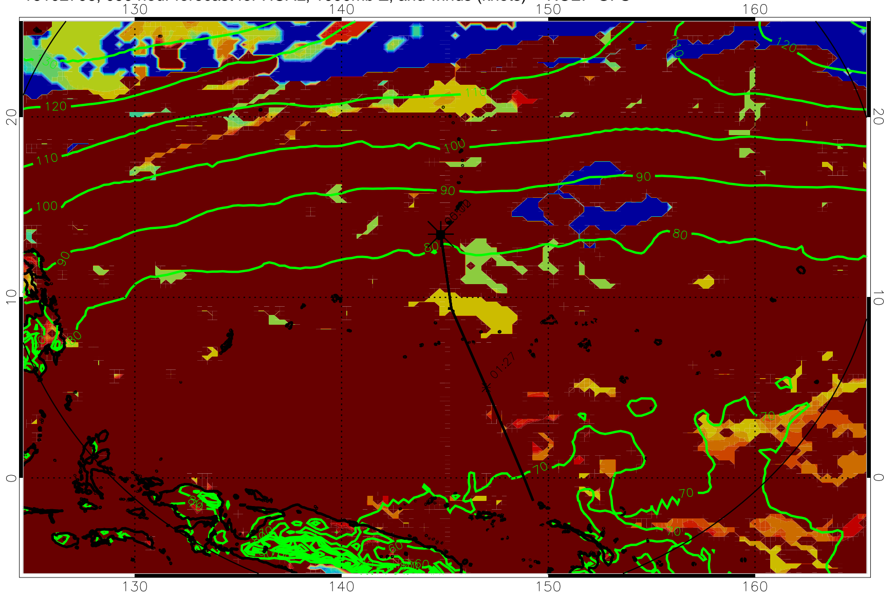
16102706, 090 hour forecast for HCAL, 1000mb Z, and winds (knots) -- NCEP GFS
