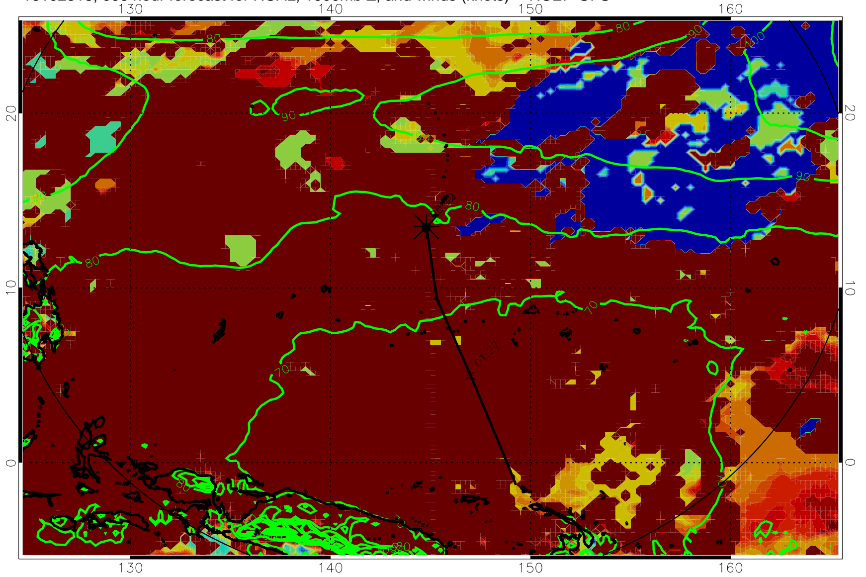
16102318, 006 hour forecast for HCAL, 1000mb Z, and winds (knots) -- NCEP GFS
