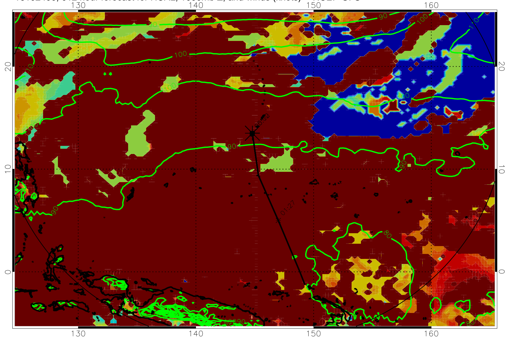
16102400, 012 hour forecast for HCAL, 1000mb Z, and winds (knots) -- NCEP GFS
