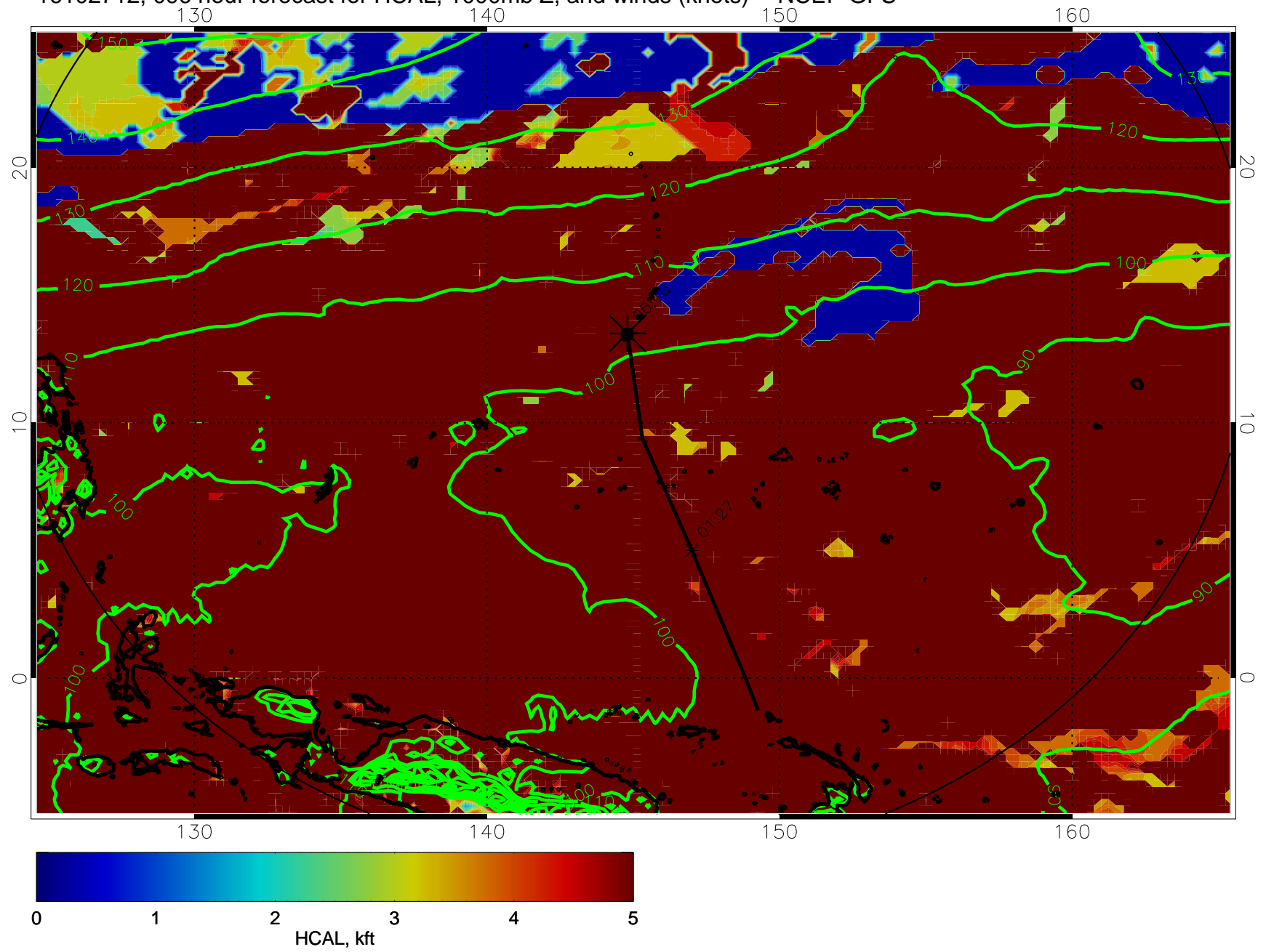
16102712, 096 hour forecast for HCAL, 1000mb Z, and winds (knots) -- NCEP GFS
