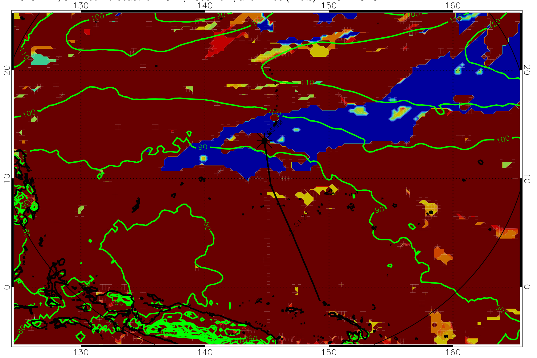
16102412, 024 hour forecast for HCAL, 1000mb Z, and winds (knots) -- NCEP GFS
