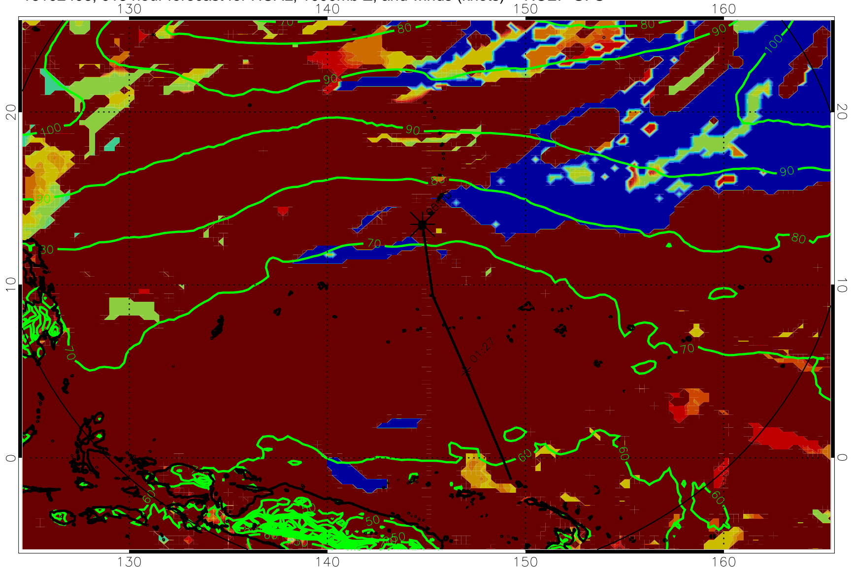
16102406, 018 hour forecast for HCAL, 1000mb Z, and winds (knots) -- NCEP GFS
