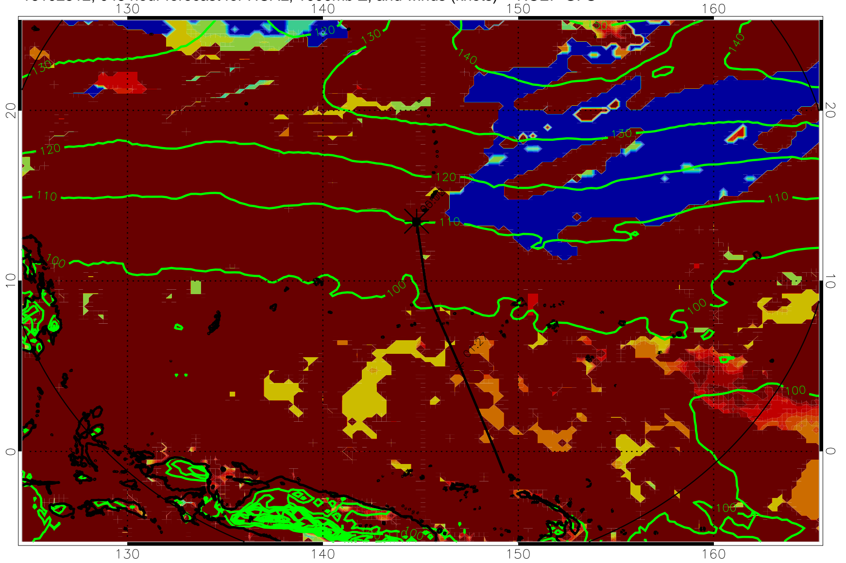
16102512, 048 hour forecast for HCAL, 1000mb Z, and winds (knots) -- NCEP GFS
