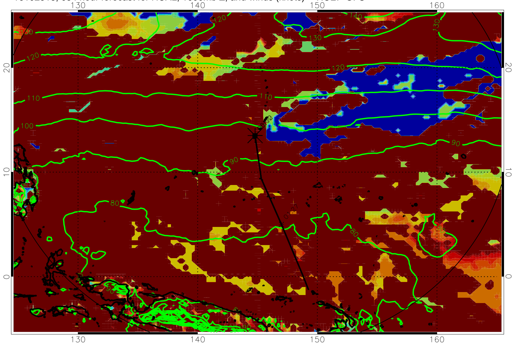
16102518, 054 hour forecast for HCAL, 1000mb Z, and winds (knots) -- NCEP GFS
