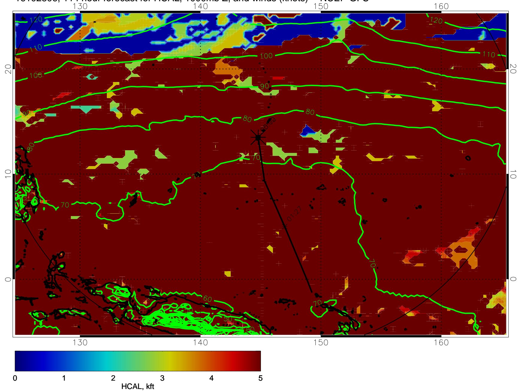
16102806, 114 hour forecast for HCAL, 1000mb Z, and winds (knots) -- NCEP GFS
