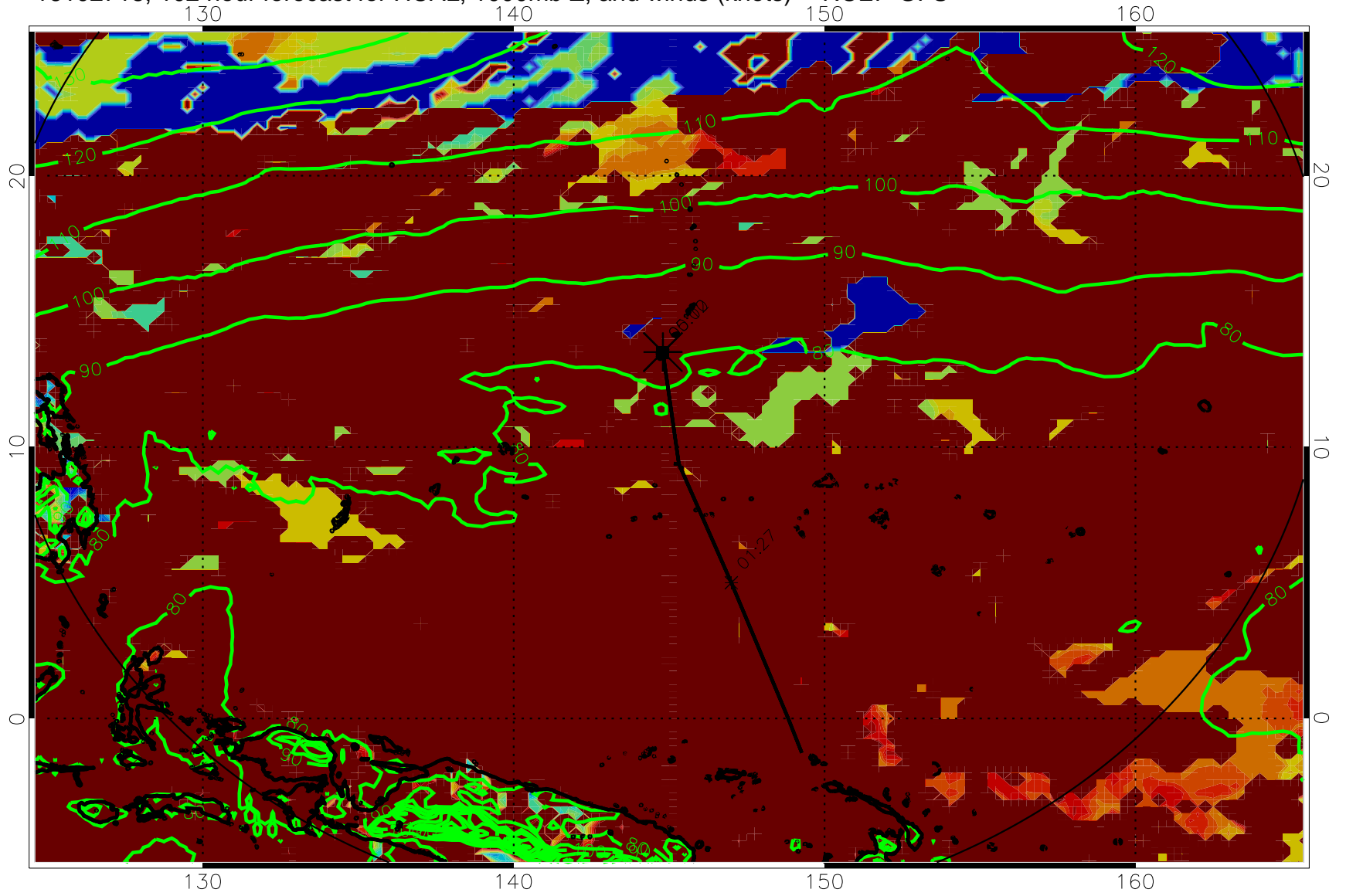
16102718, 102 hour forecast for HCAL, 1000mb Z, and winds (knots) -- NCEP GFS
