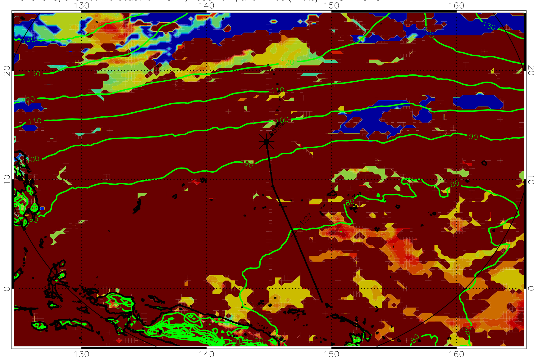
16102618, 078 hour forecast for HCAL, 1000mb Z, and winds (knots) -- NCEP GFS
