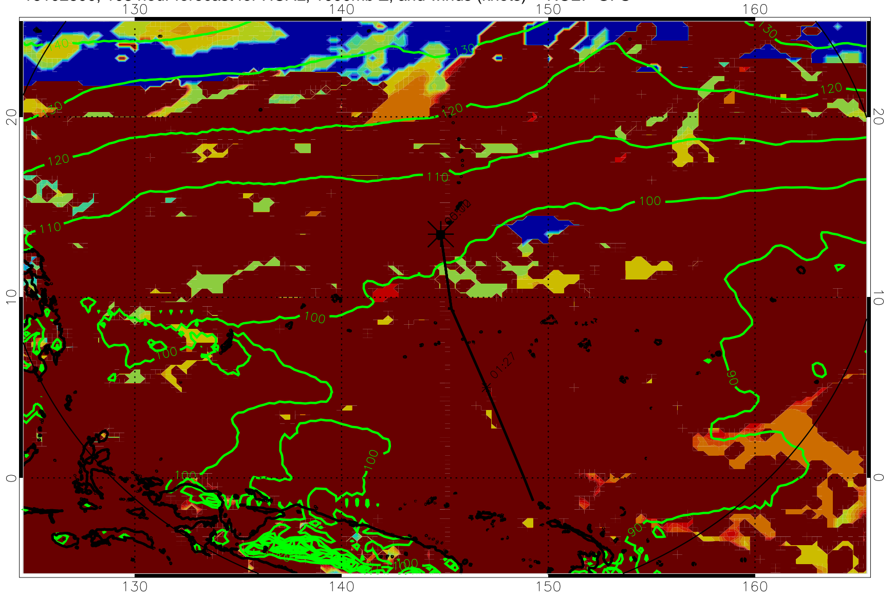
16102800, 108 hour forecast for HCAL, 1000mb Z, and winds (knots) -- NCEP GFS
