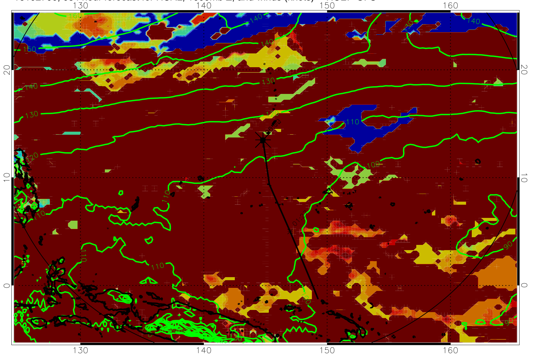
16102700, 084 hour forecast for HCAL, 1000mb Z, and winds (knots) -- NCEP GFS
