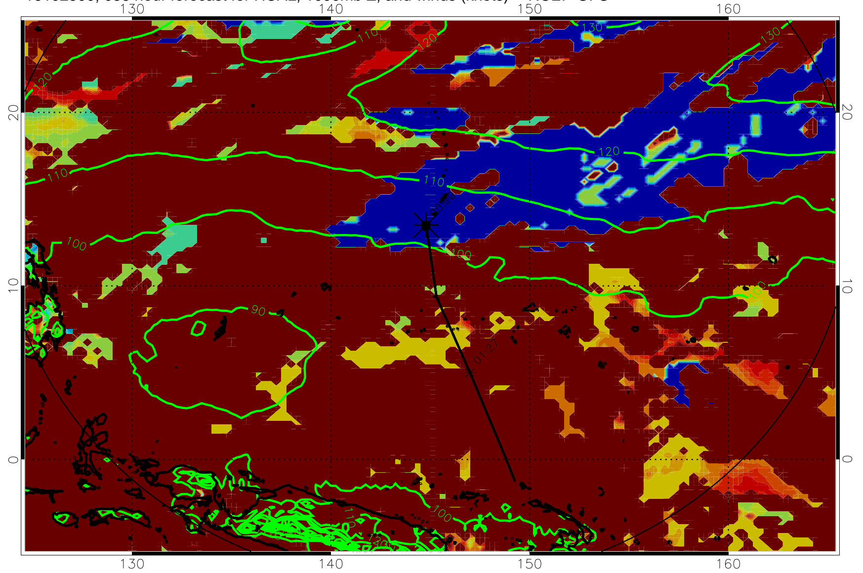
16102500, 036 hour forecast for HCAL, 1000mb Z, and winds (knots) -- NCEP GFS
