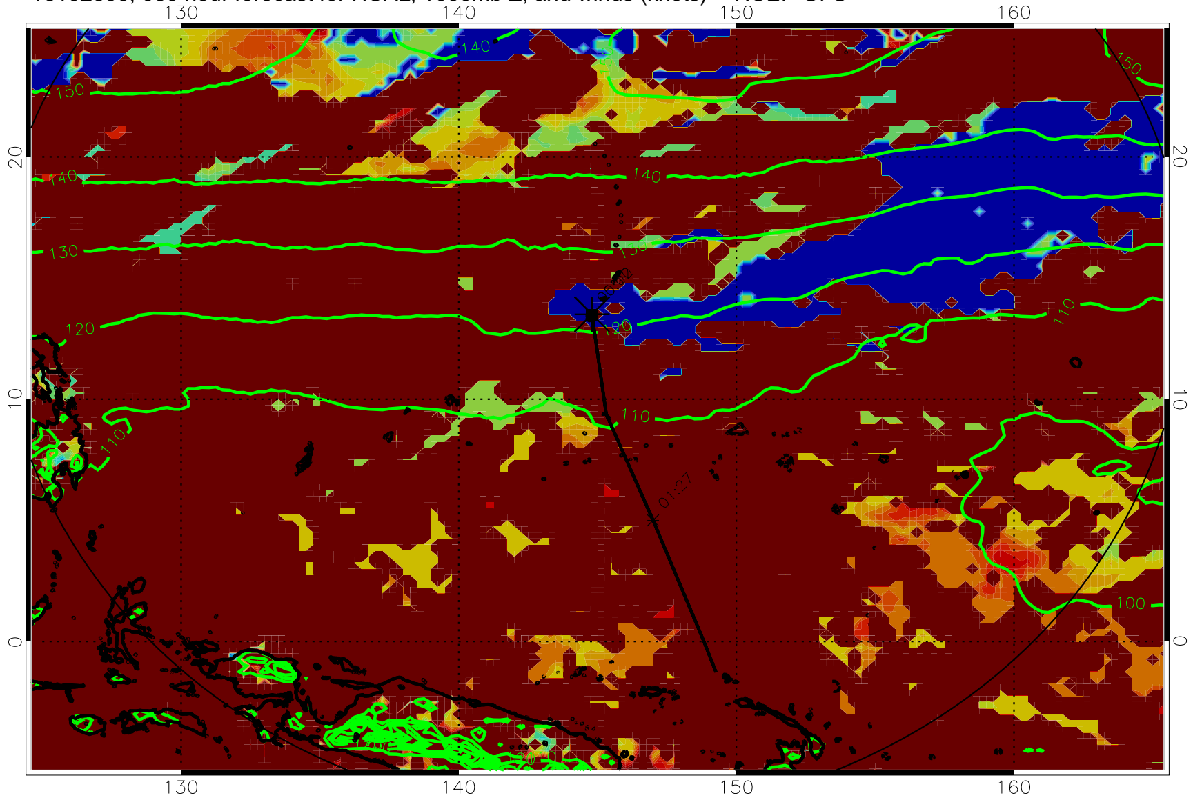
16102600, 060 hour forecast for HCAL, 1000mb Z, and winds (knots) -- NCEP GFS
