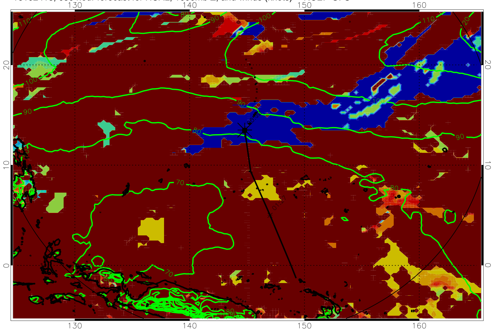
16102418, 030 hour forecast for HCAL, 1000mb Z, and winds (knots) -- NCEP GFS
