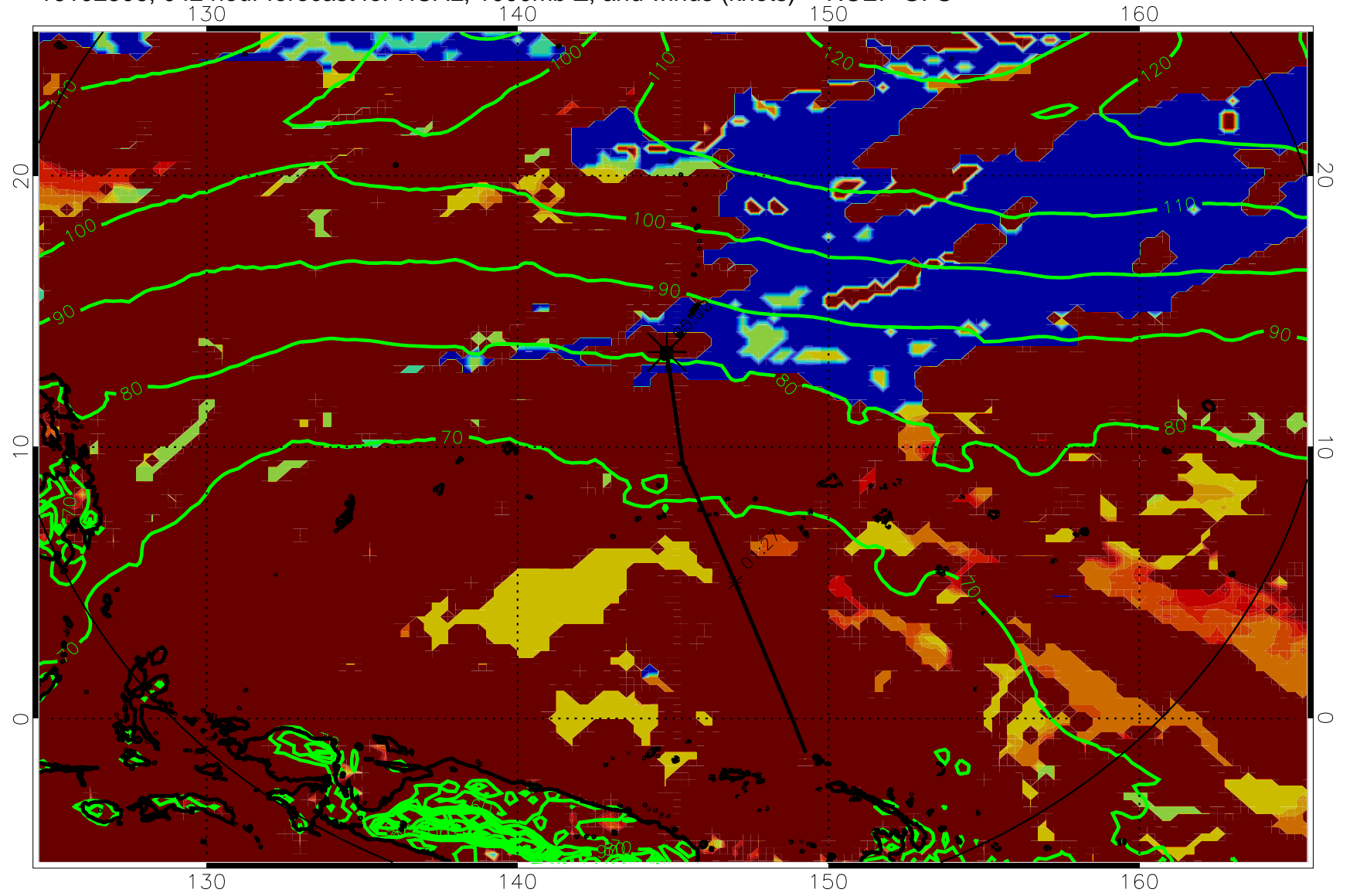
16102506, 042 hour forecast for HCAL, 1000mb Z, and winds (knots) -- NCEP GFS
