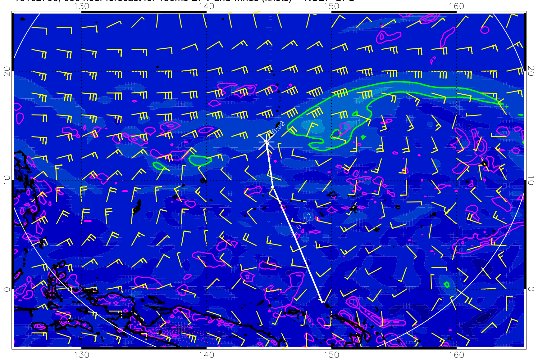
16102706, 090 hour forecast for 150mb EPV and winds (knots) -- NCEP GFS
