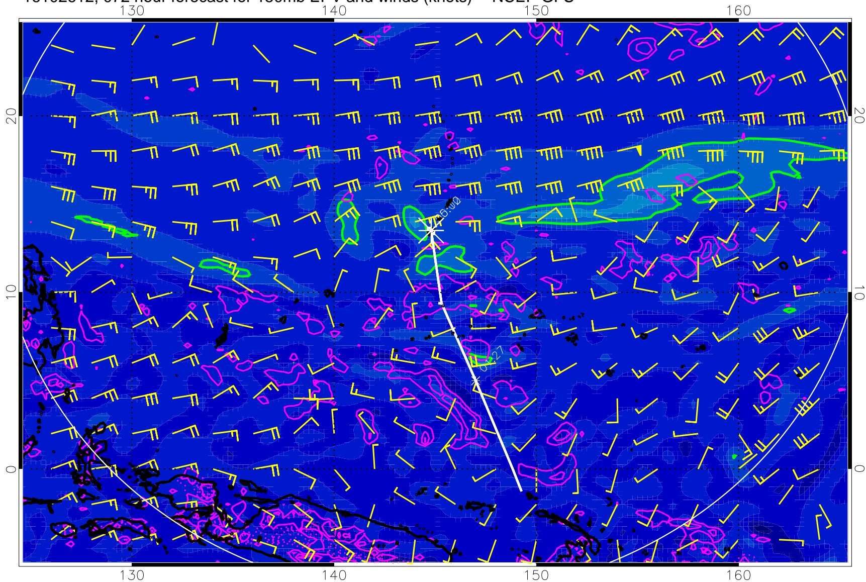
16102612, 072 hour forecast for 150mb EPV and winds (knots) -- NCEP GFS
