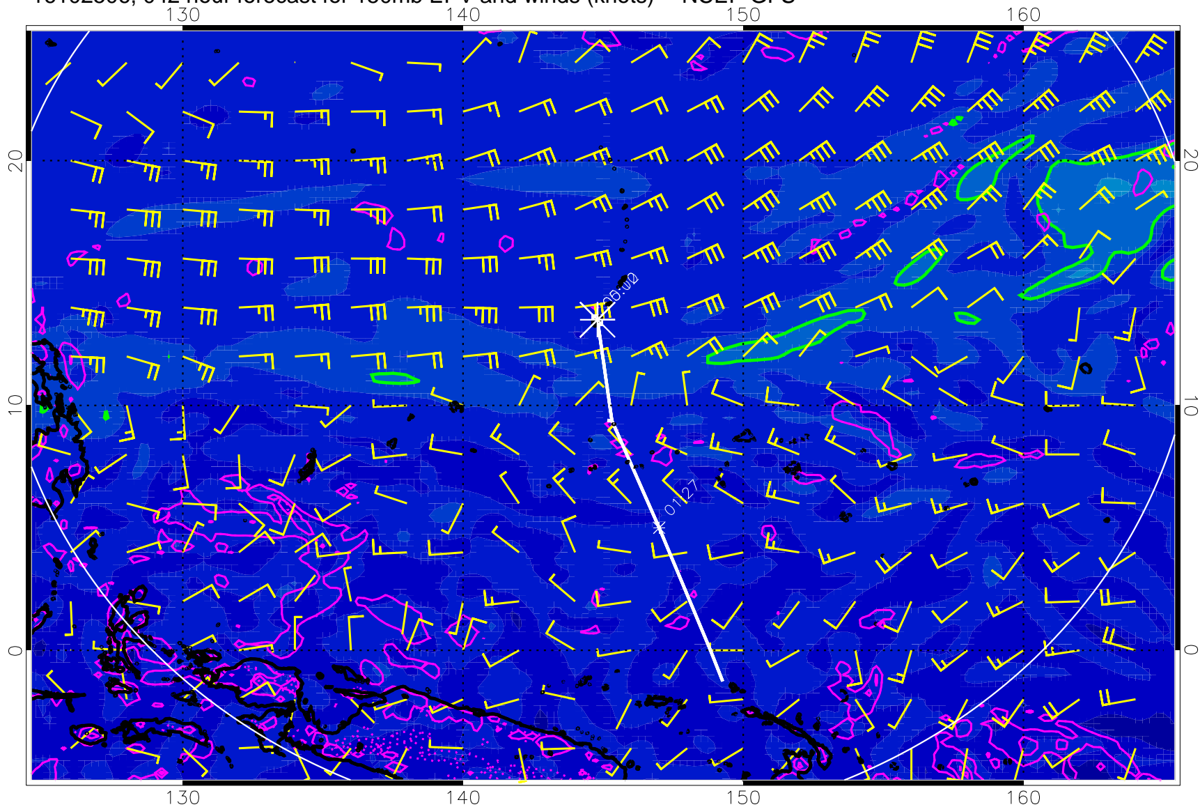
16102506, 042 hour forecast for 150mb EPV and winds (knots) -- NCEP GFS
