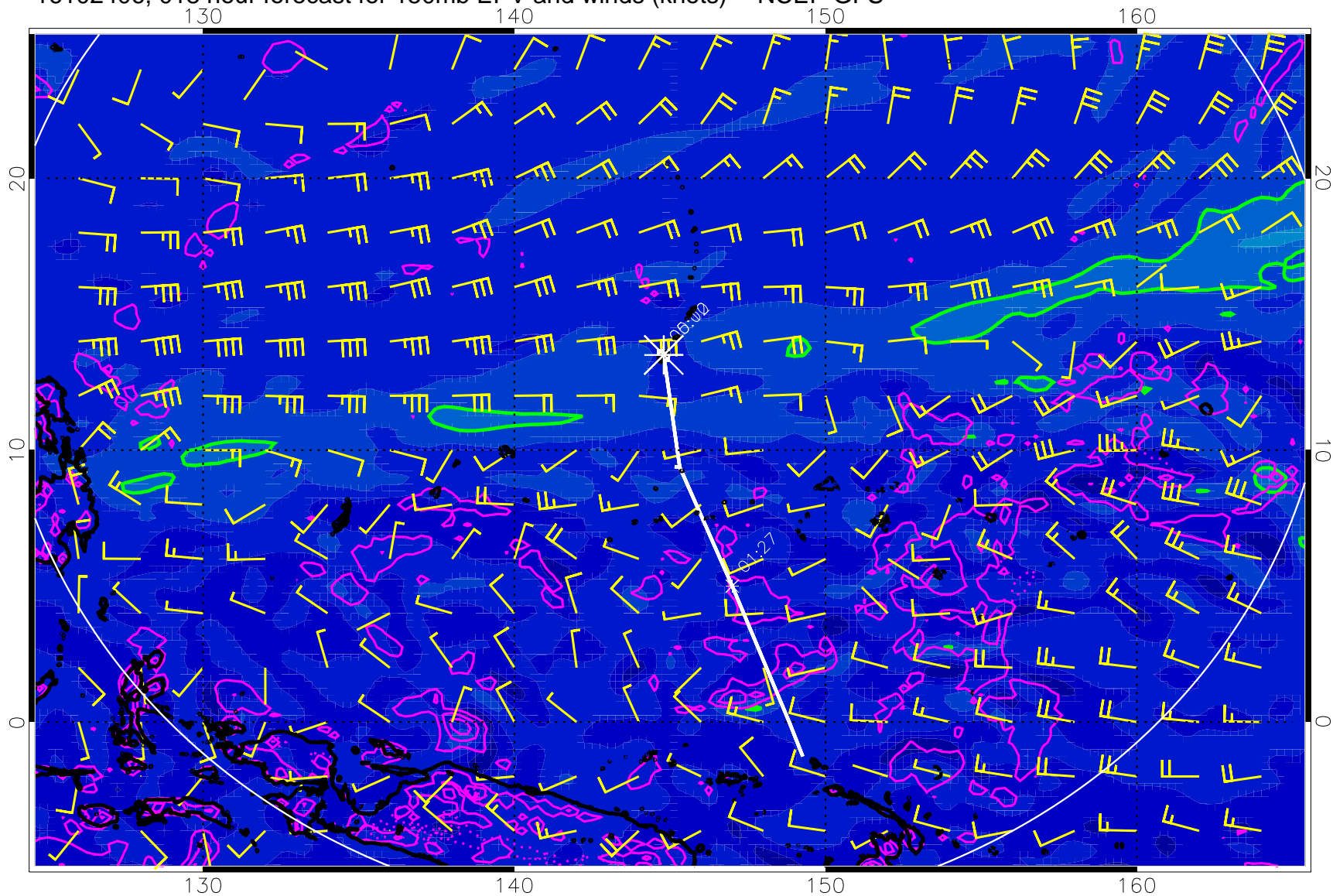
16102406, 018 hour forecast for 150mb EPV and winds (knots) -- NCEP GFS
