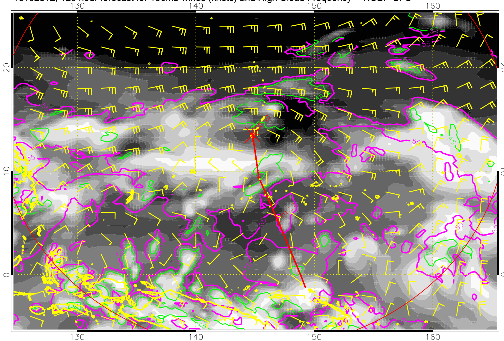
16102812, 120 hour forecast for 150mb winds (knots) and High Cloud Frequency -- NCEP GFS
