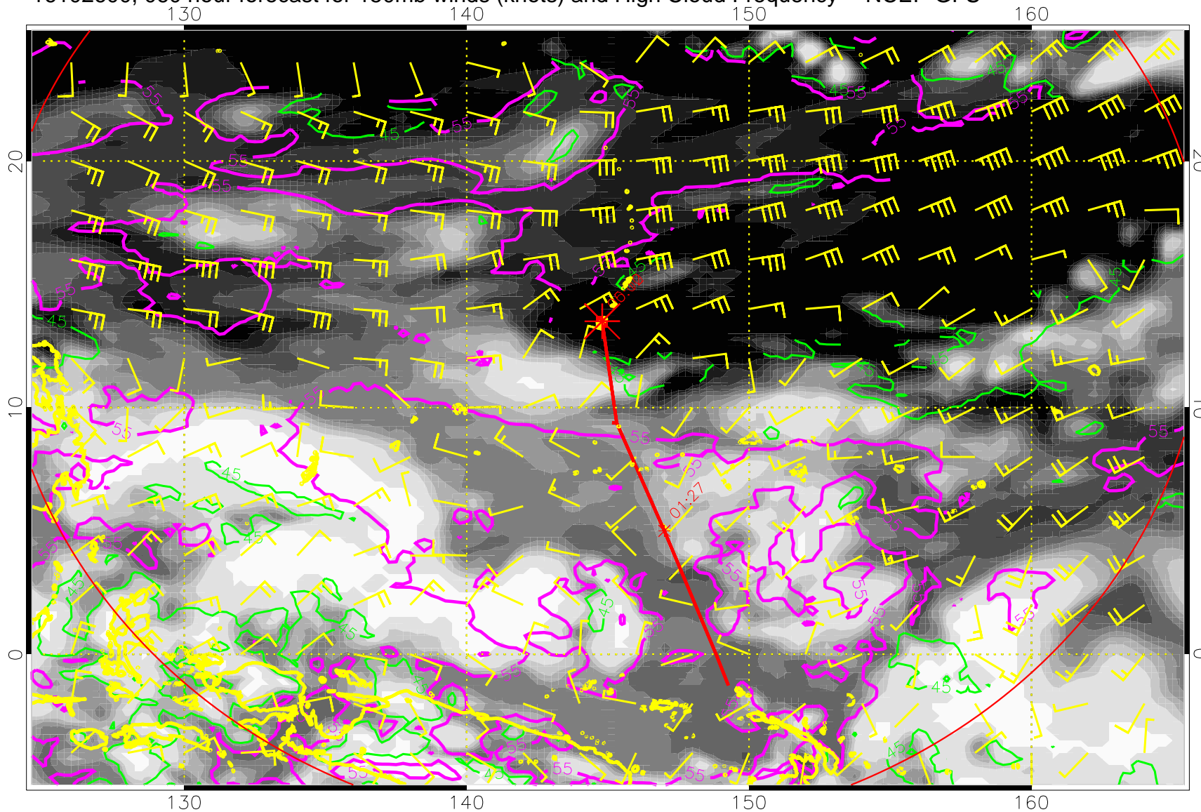
16102600, 060 hour forecast for 150mb winds (knots) and High Cloud Frequency -- NCEP GFS
