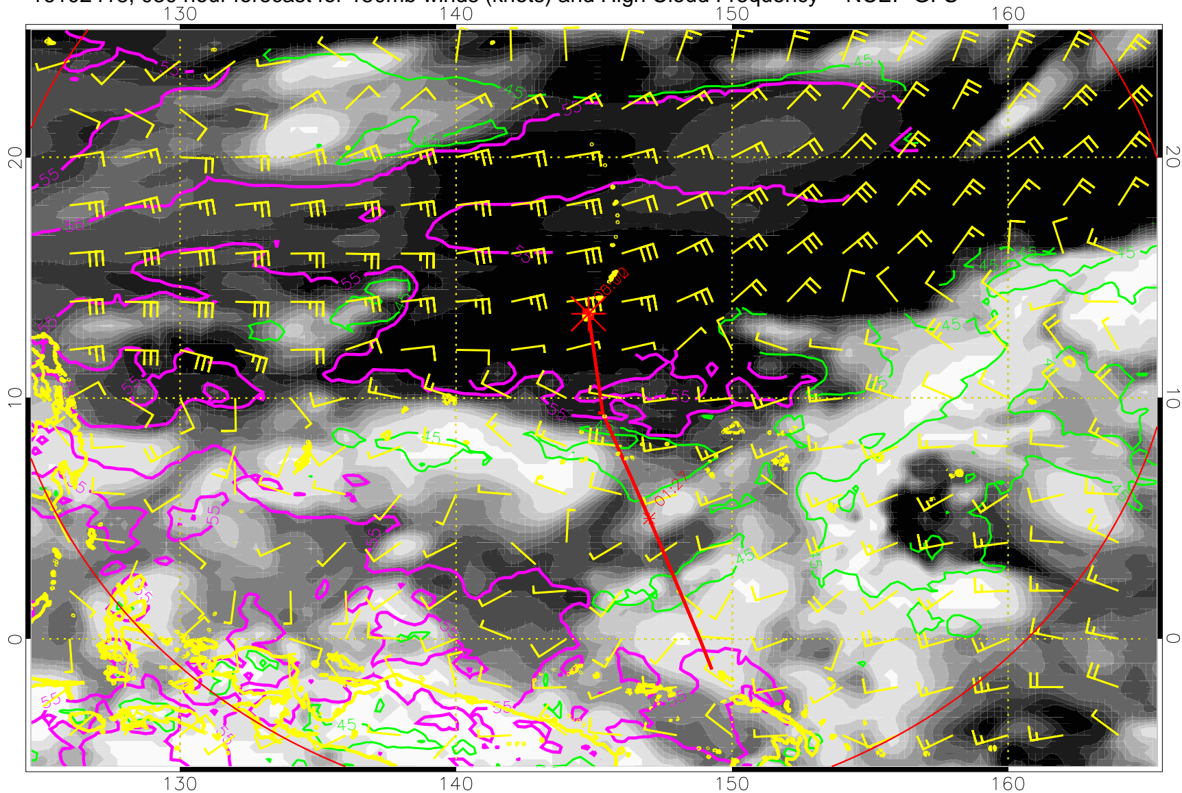
16102418, 030 hour forecast for 150mb winds (knots) and High Cloud Frequency -- NCEP GFS
