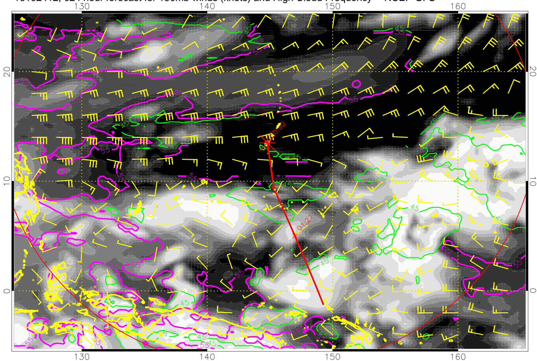
16102412, 024 hour forecast for 150mb winds (knots) and High Cloud Frequency -- NCEP GFS
