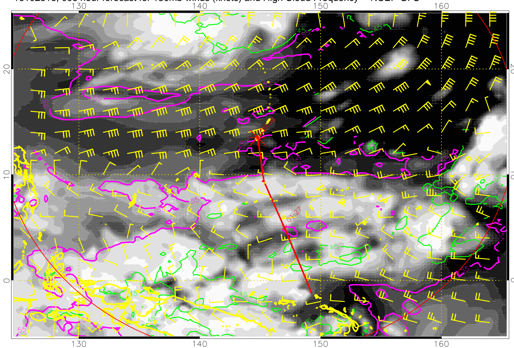
16102318, 006 hour forecast for 150mb winds (knots) and High Cloud Frequency -- NCEP GFS
