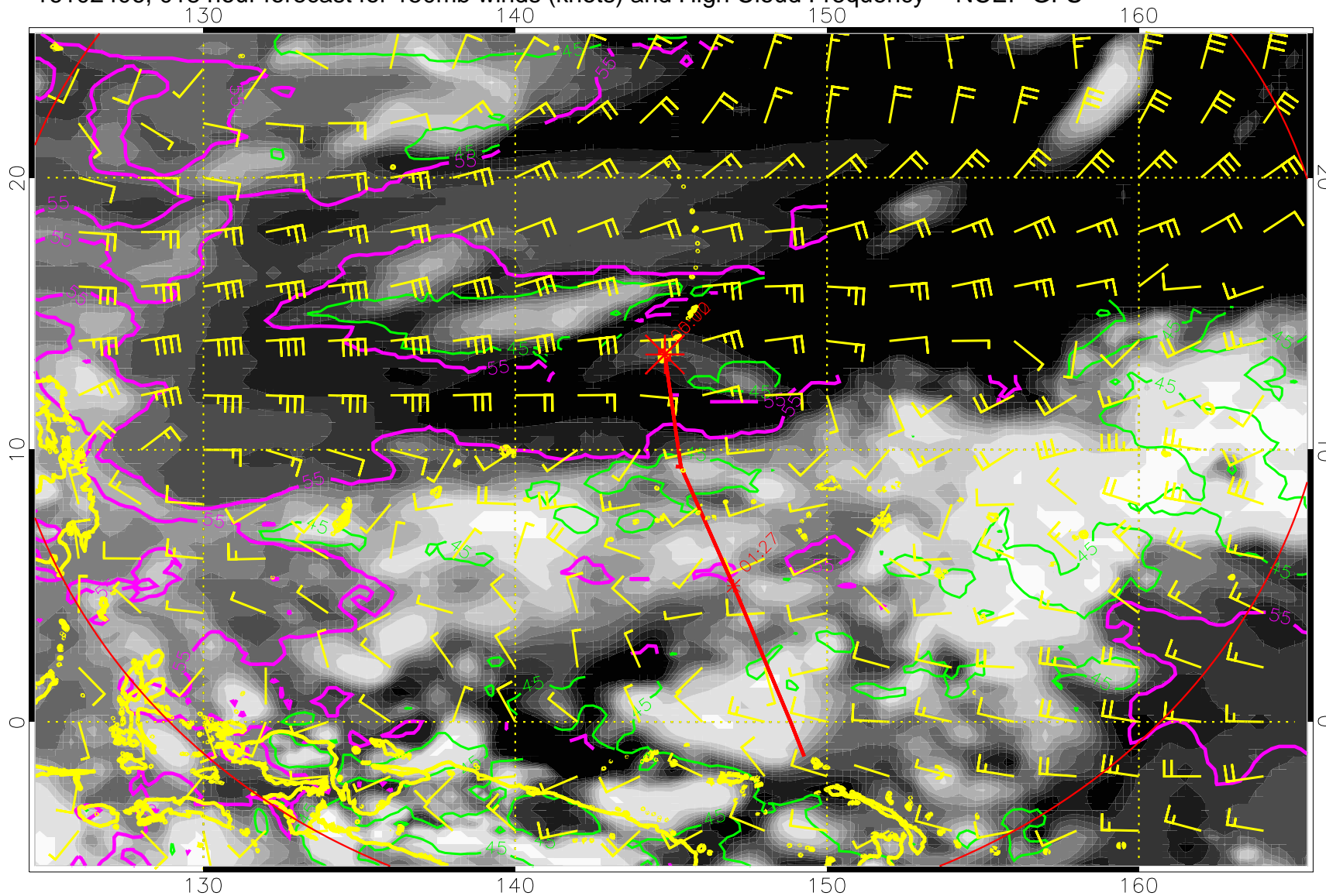
16102406, 018 hour forecast for 150mb winds (knots) and High Cloud Frequency -- NCEP GFS
