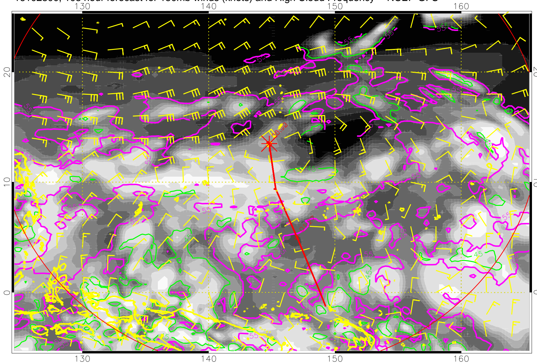
16102800, 108 hour forecast for 150mb winds (knots) and High Cloud Frequency -- NCEP GFS
