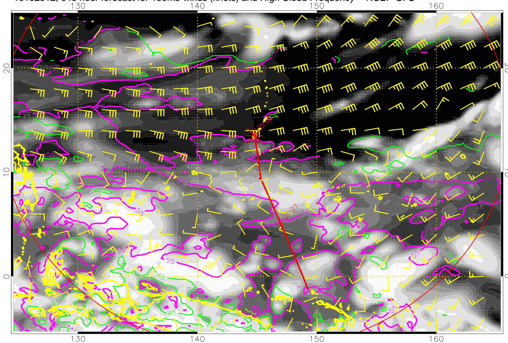
16102512, 048 hour forecast for 150mb winds (knots) and High Cloud Frequency -- NCEP GFS
