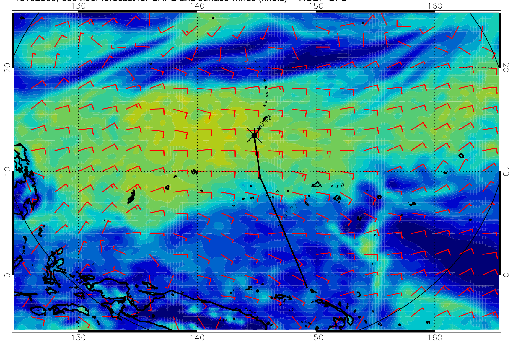
16102500, 036 hour forecast for CAPE and surface winds (knots) -- NCEP GFS
