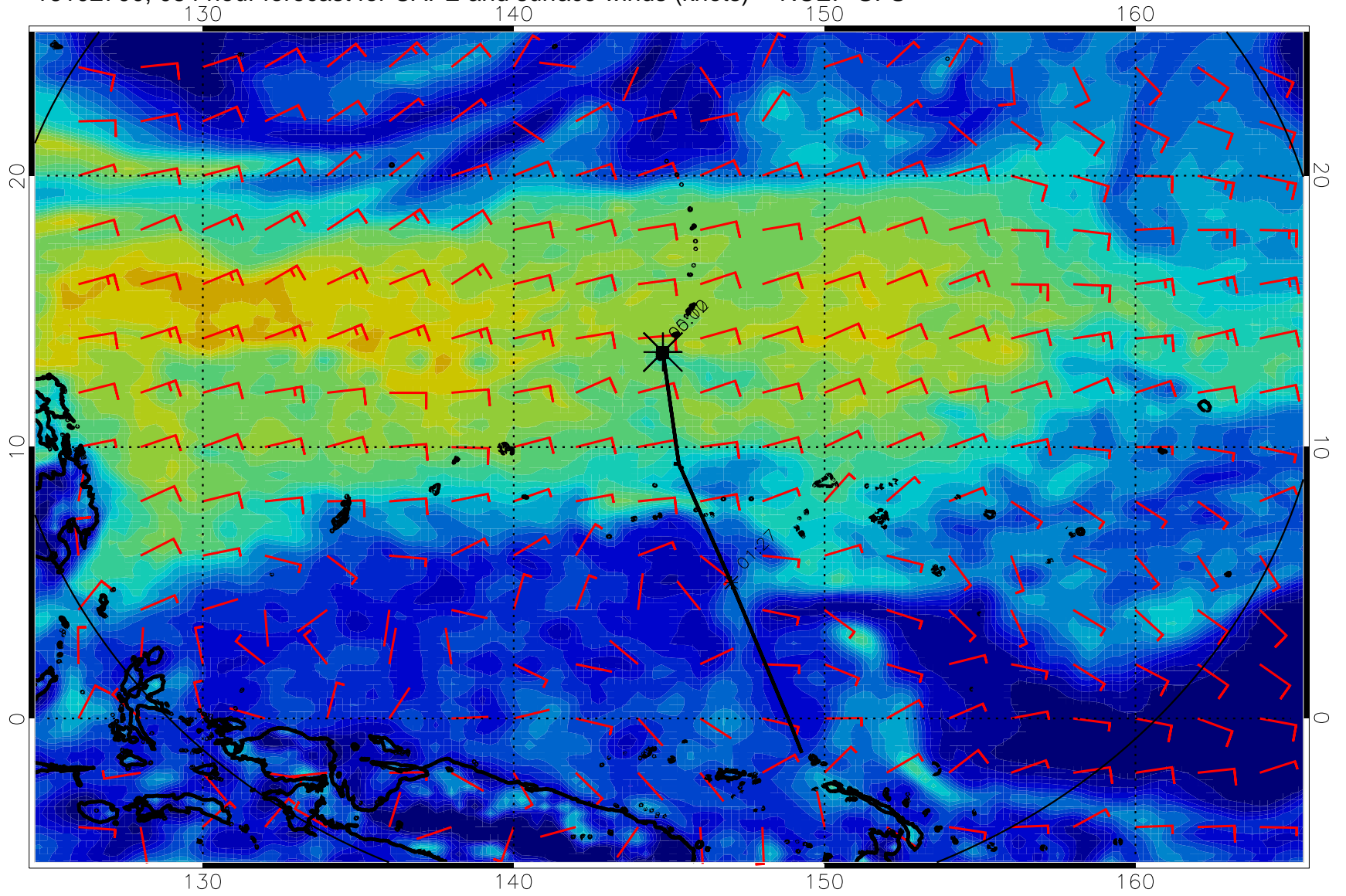
16102700, 084 hour forecast for CAPE and surface winds (knots) -- NCEP GFS
