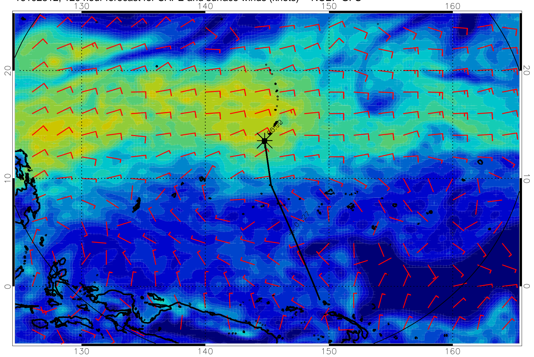
16102812, 120 hour forecast for CAPE and surface winds (knots) -- NCEP GFS
