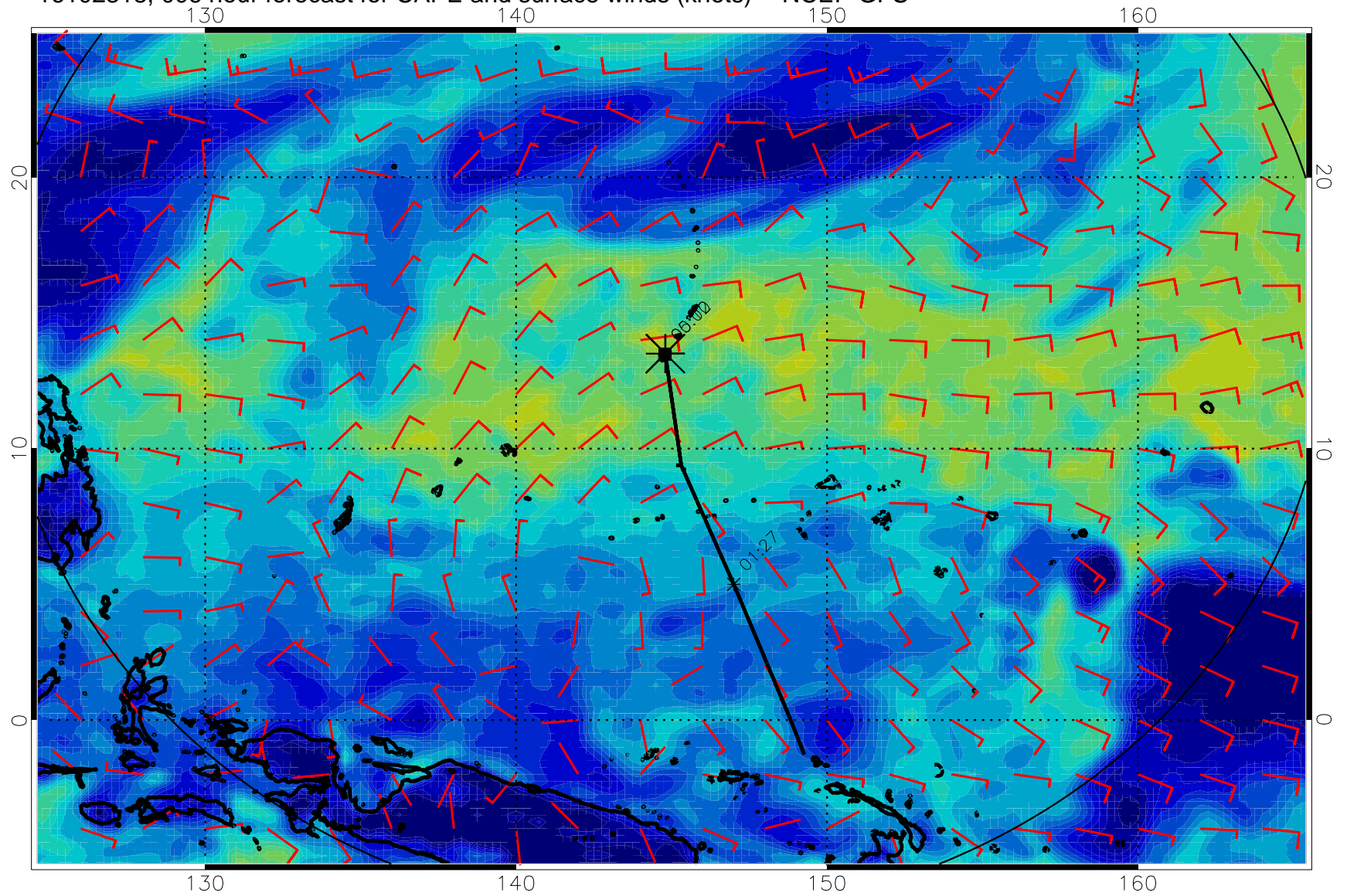
16102318, 006 hour forecast for CAPE and surface winds (knots) -- NCEP GFS
