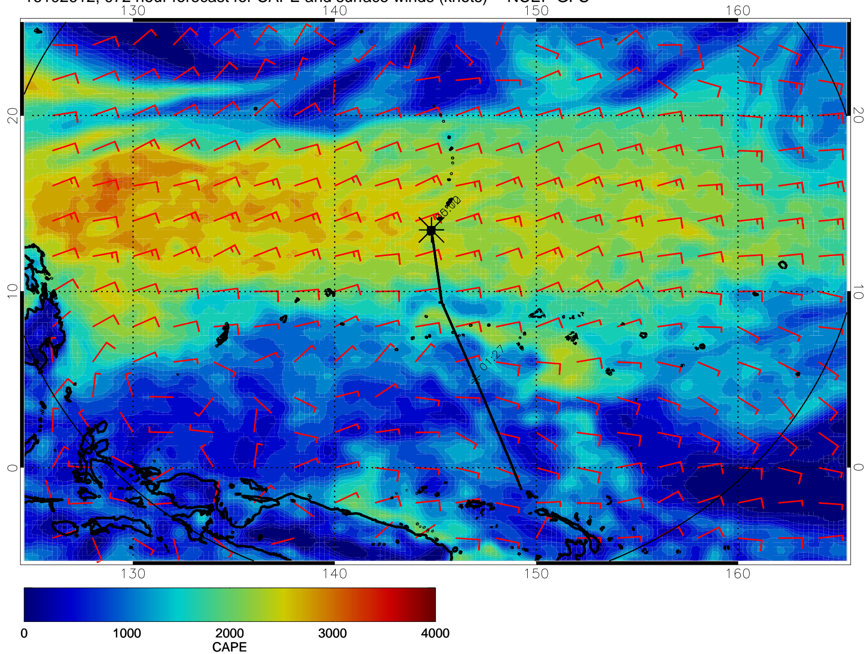
16102612, 072 hour forecast for CAPE and surface winds (knots) -- NCEP GFS
