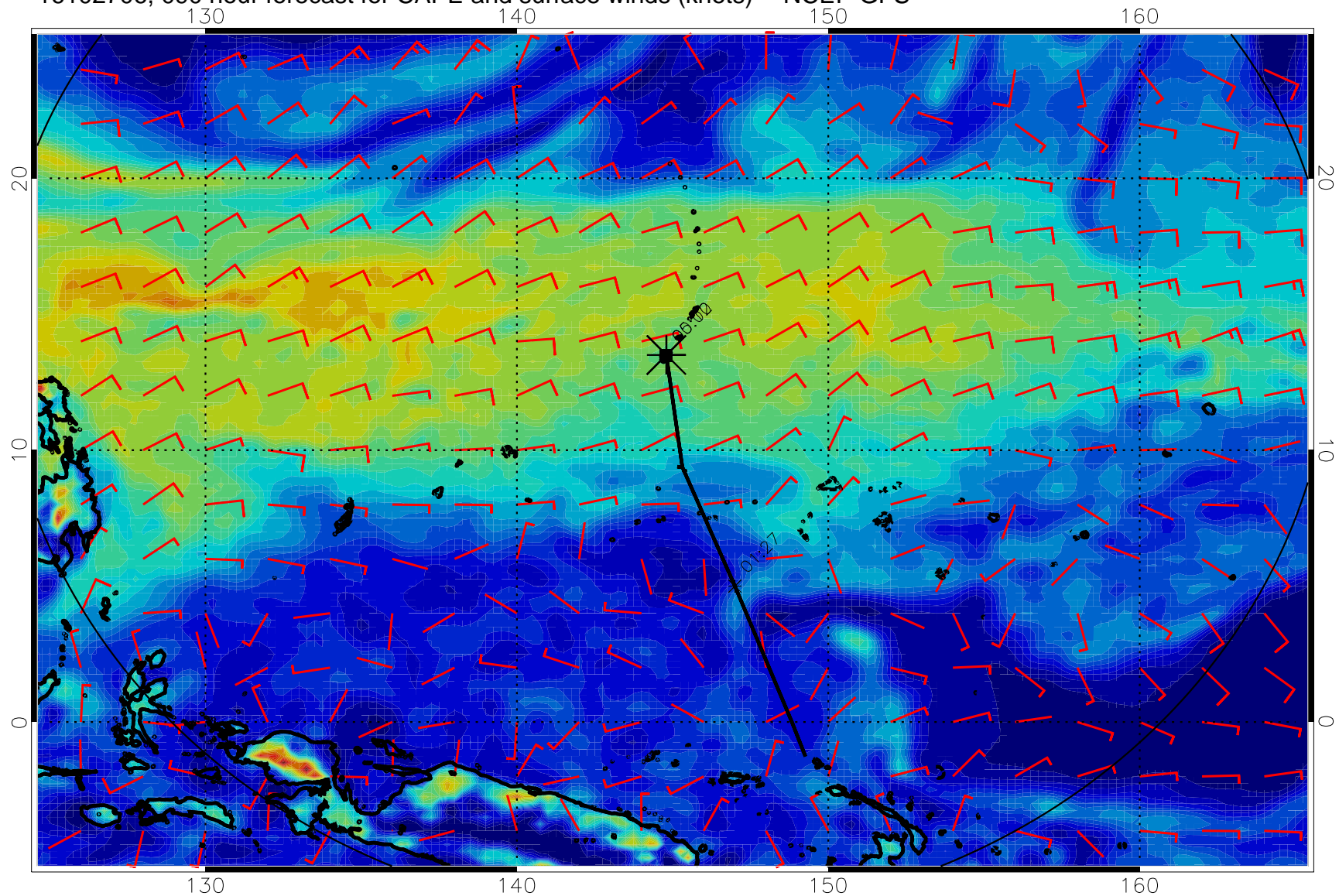
16102706, 090 hour forecast for CAPE and surface winds (knots) -- NCEP GFS
