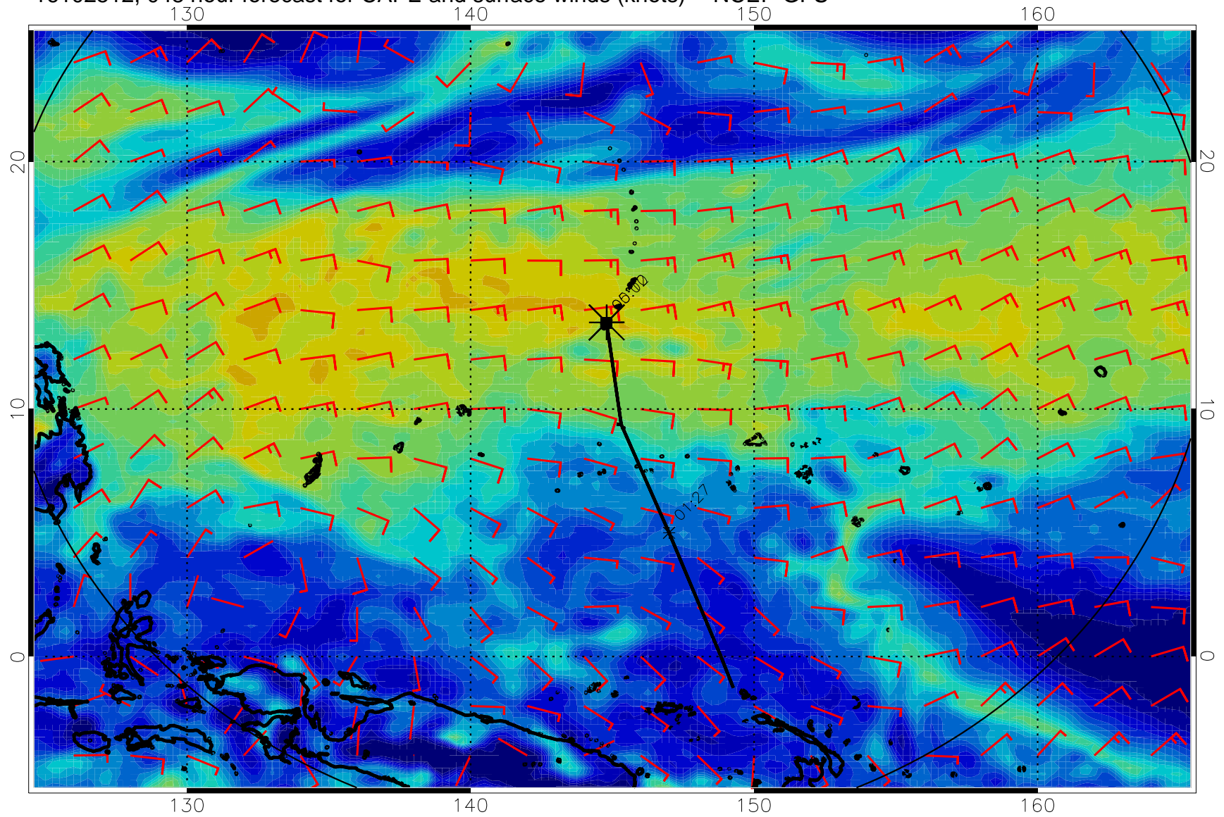
16102512, 048 hour forecast for CAPE and surface winds (knots) -- NCEP GFS
