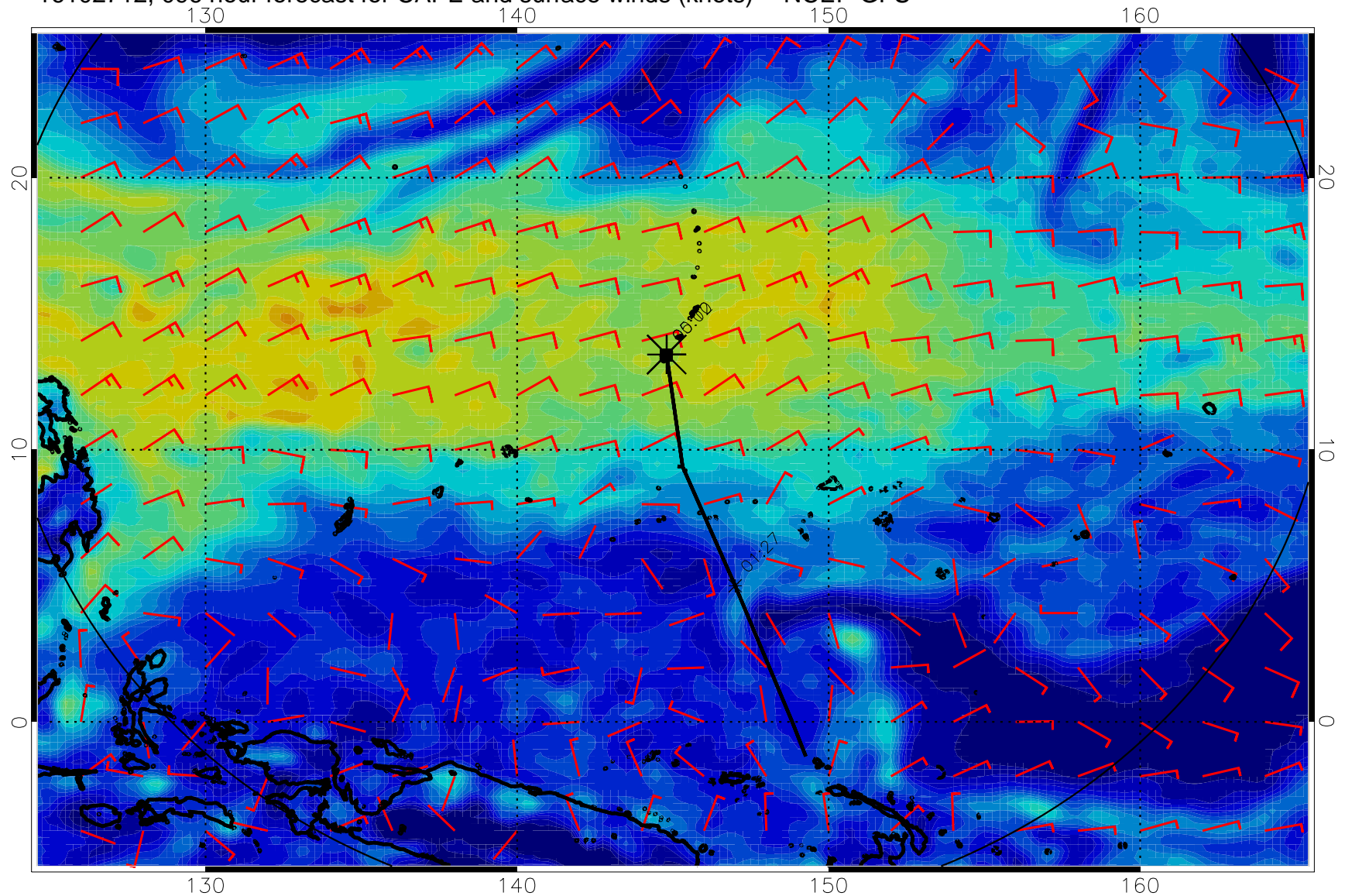
16102712, 096 hour forecast for CAPE and surface winds (knots) -- NCEP GFS
