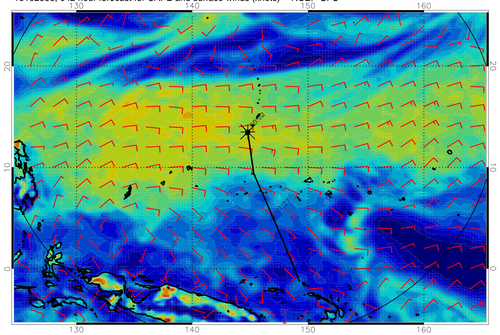
16102506, 042 hour forecast for CAPE and surface winds (knots) -- NCEP GFS
