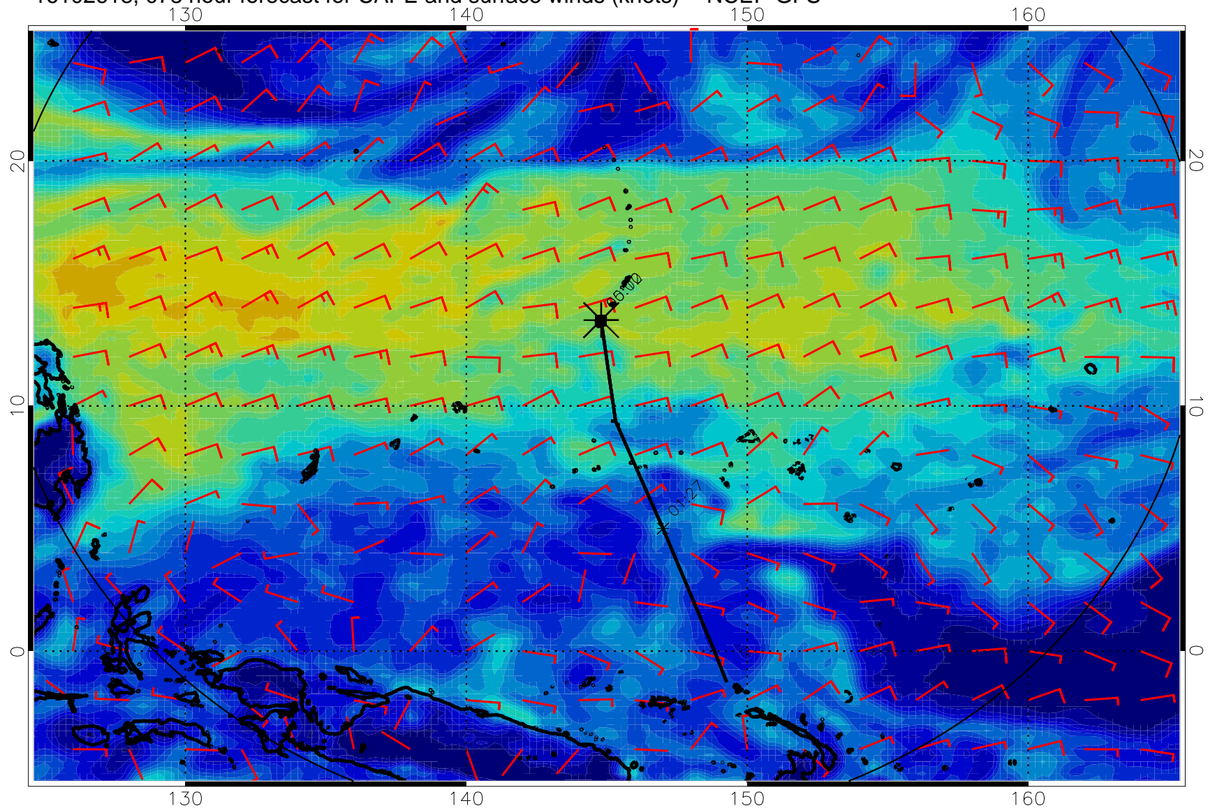
16102618, 078 hour forecast for CAPE and surface winds (knots) -- NCEP GFS
