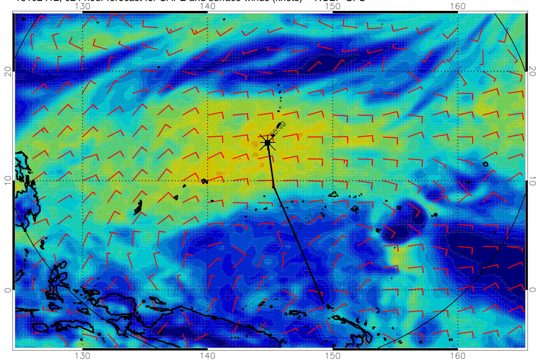
16102412, 024 hour forecast for CAPE and surface winds (knots) -- NCEP GFS
