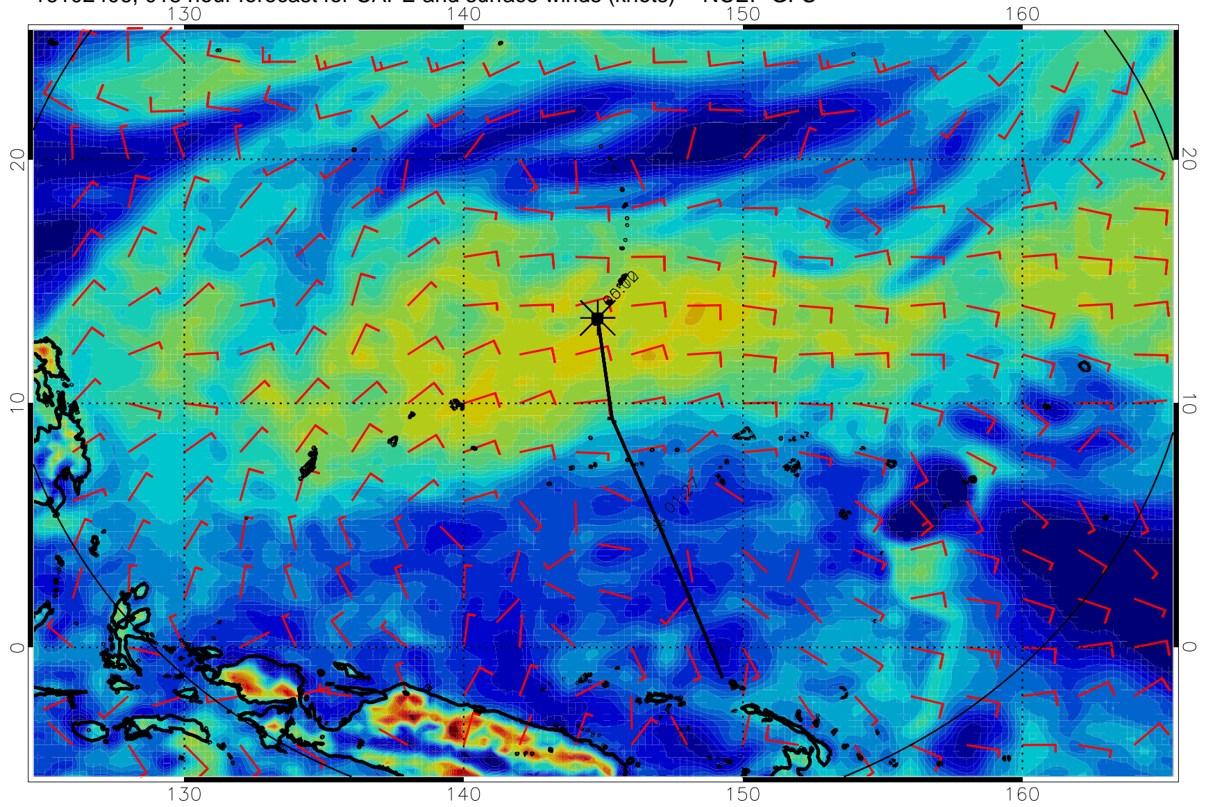
16102406, 018 hour forecast for CAPE and surface winds (knots) -- NCEP GFS
