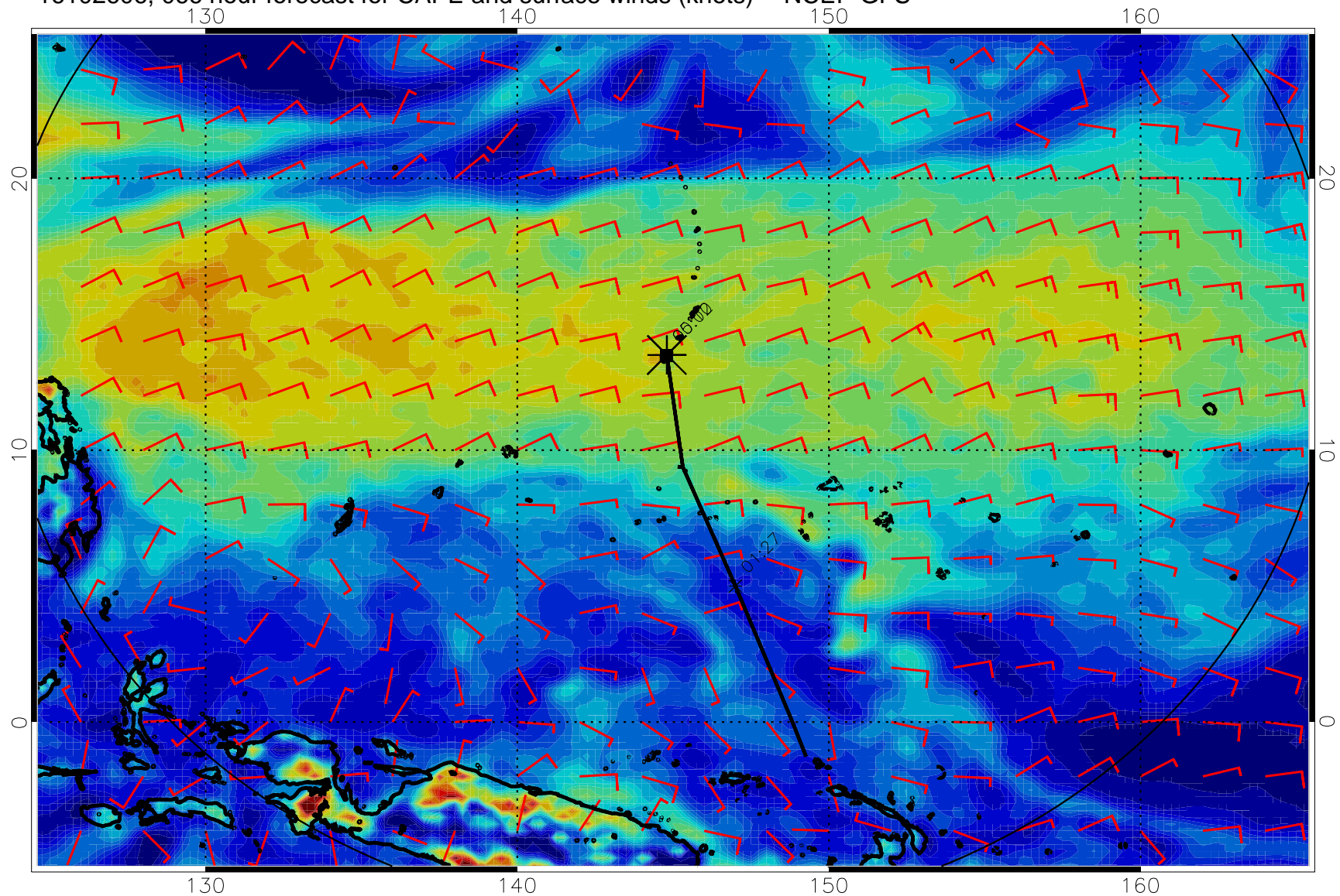
16102606, 066 hour forecast for CAPE and surface winds (knots) -- NCEP GFS
