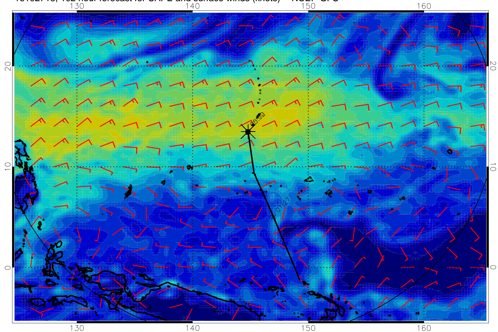
16102718, 102 hour forecast for CAPE and surface winds (knots) -- NCEP GFS
