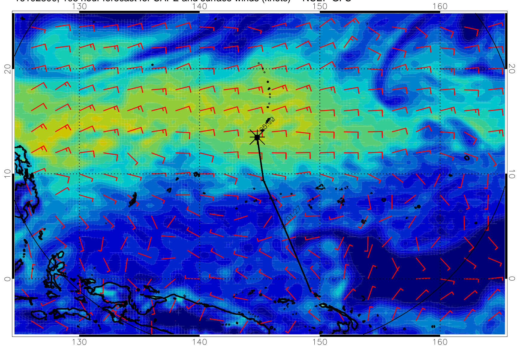
16102800, 108 hour forecast for CAPE and surface winds (knots) -- NCEP GFS
