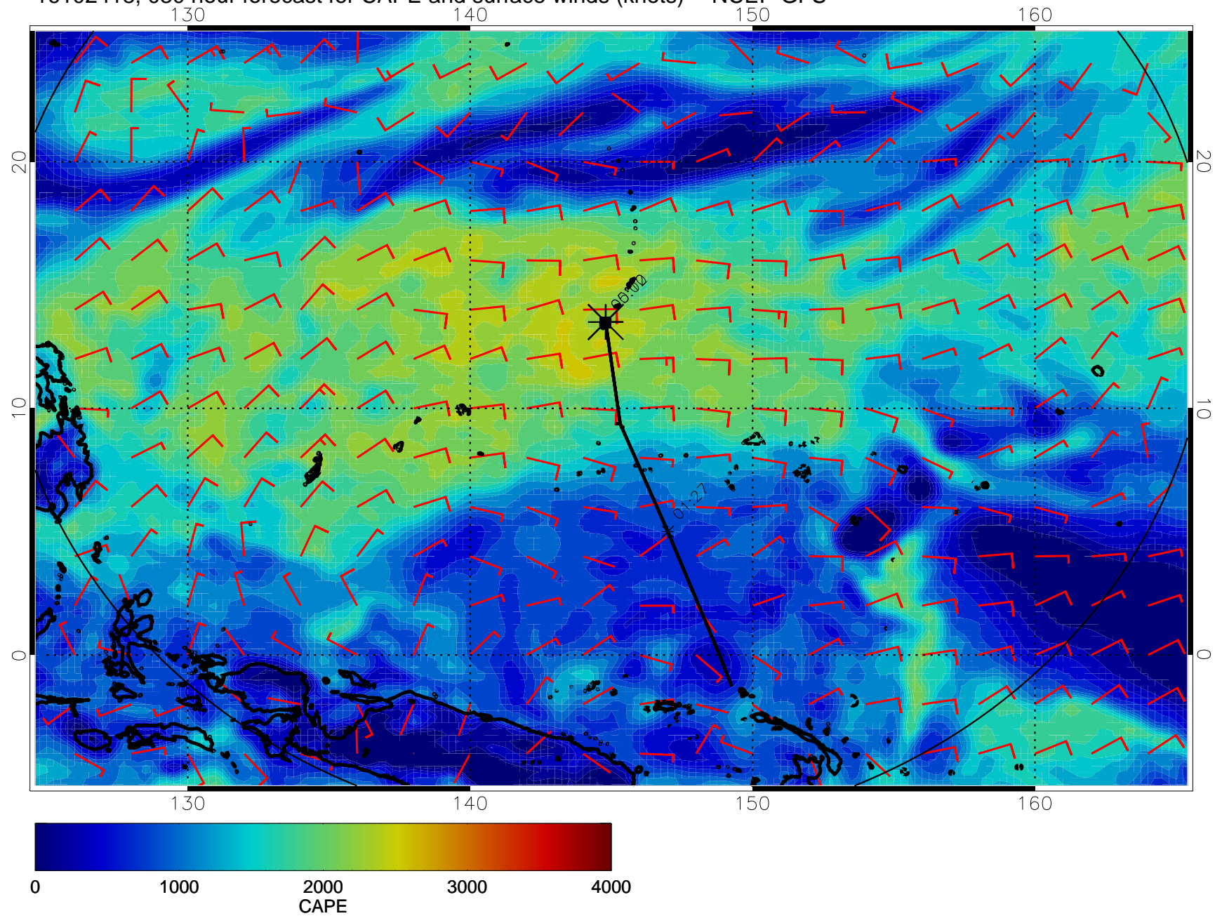
16102418, 030 hour forecast for CAPE and surface winds (knots) -- NCEP GFS
