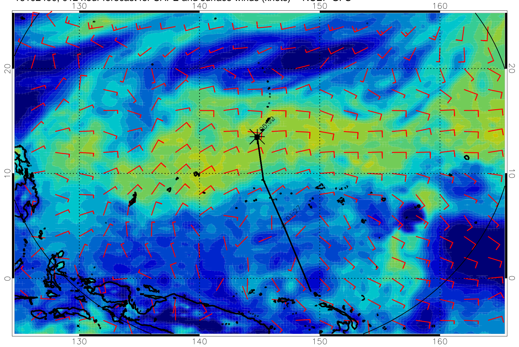
16102400, 012 hour forecast for CAPE and surface winds (knots) -- NCEP GFS
