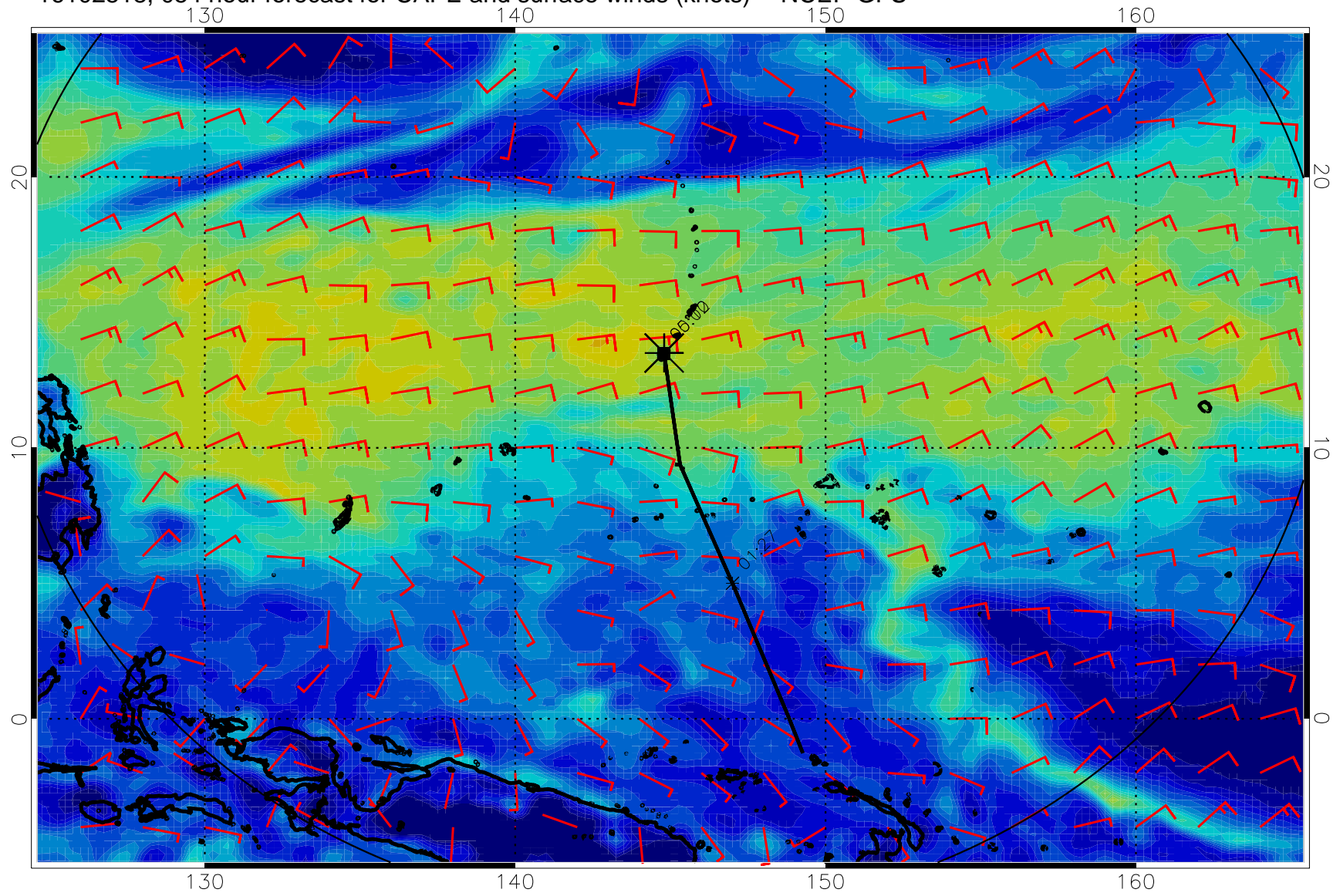
16102518, 054 hour forecast for CAPE and surface winds (knots) -- NCEP GFS
