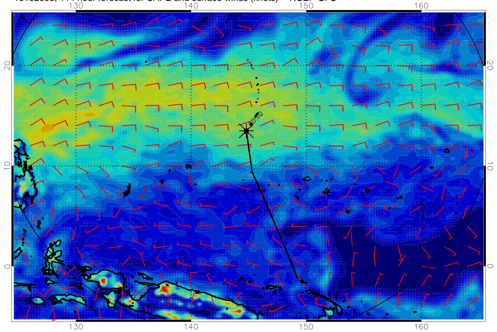
16102806, 114 hour forecast for CAPE and surface winds (knots) -- NCEP GFS
