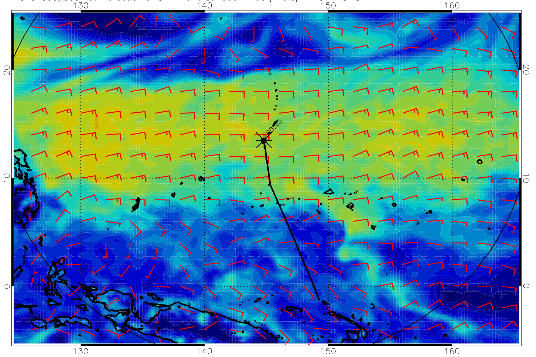
16102600, 060 hour forecast for CAPE and surface winds (knots) -- NCEP GFS
