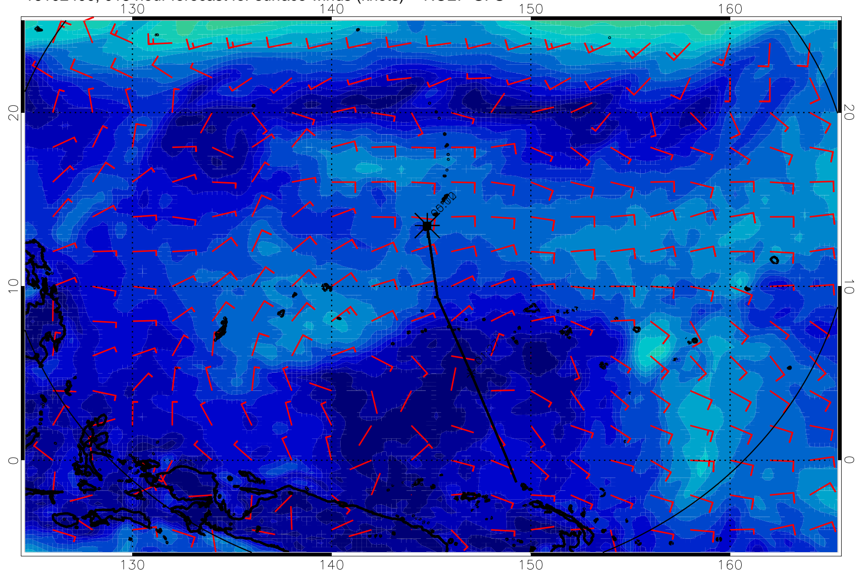
16102400, 018 hour forecast for surface winds (knots) -- NCEP GFS
