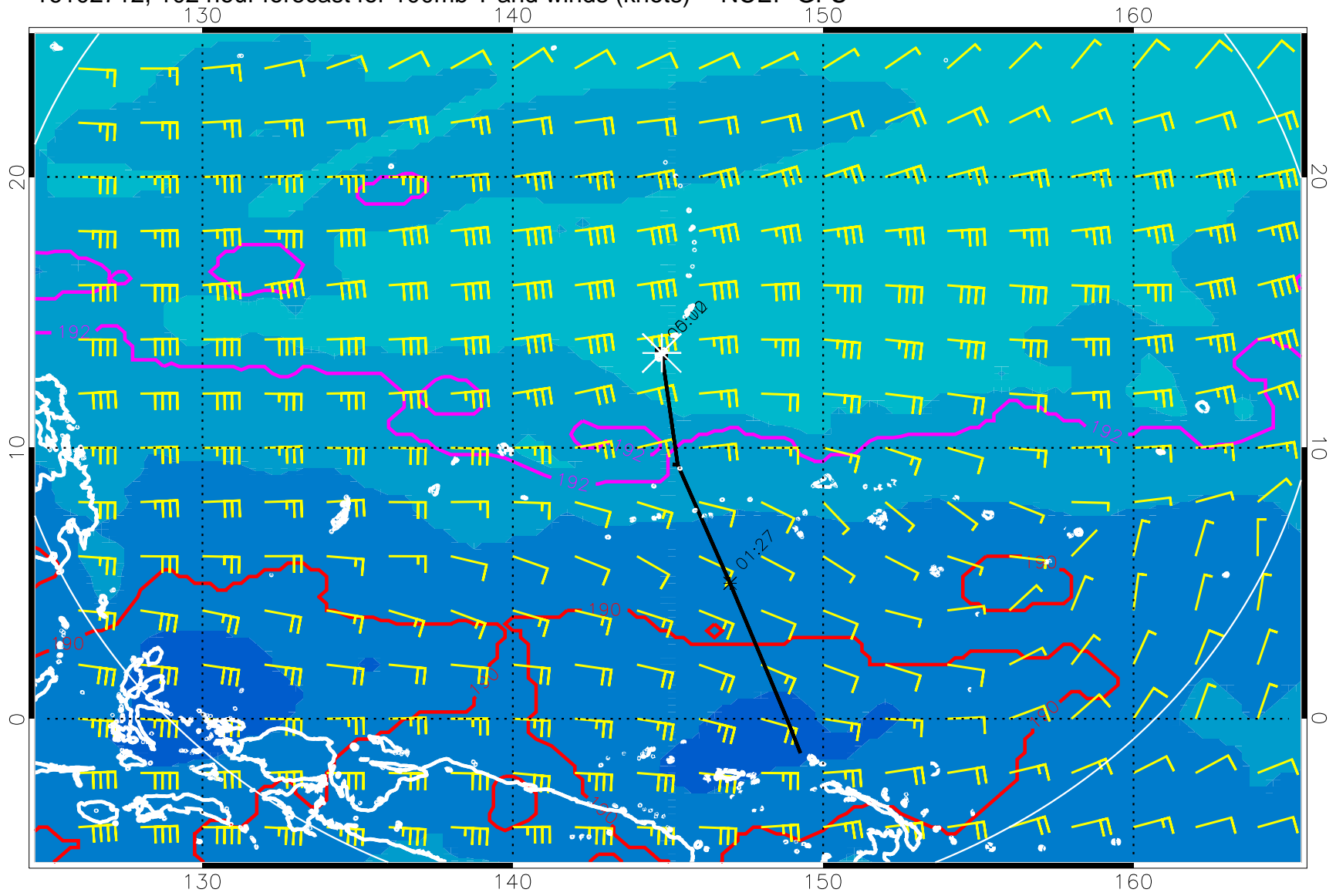
16102712, 102 hour forecast for 100mb T and winds (knots) -- NCEP GFS
