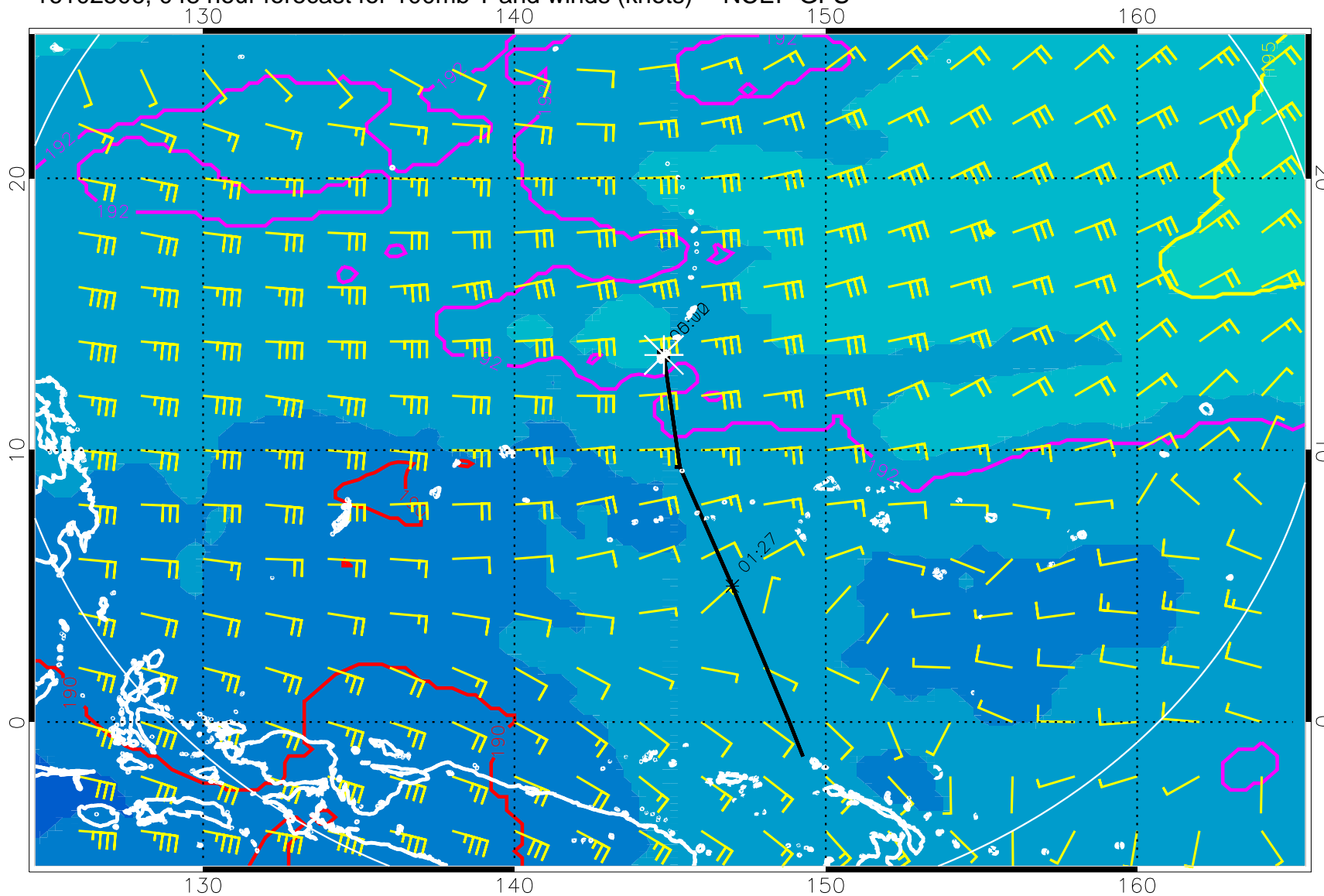
16102506, 048 hour forecast for 100mb T and winds (knots) -- NCEP GFS
