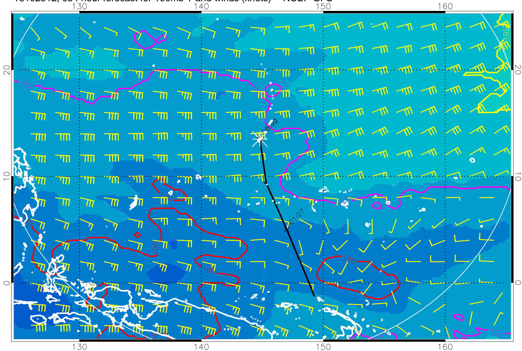
16102512, 054 hour forecast for 100mb T and winds (knots) -- NCEP GFS
