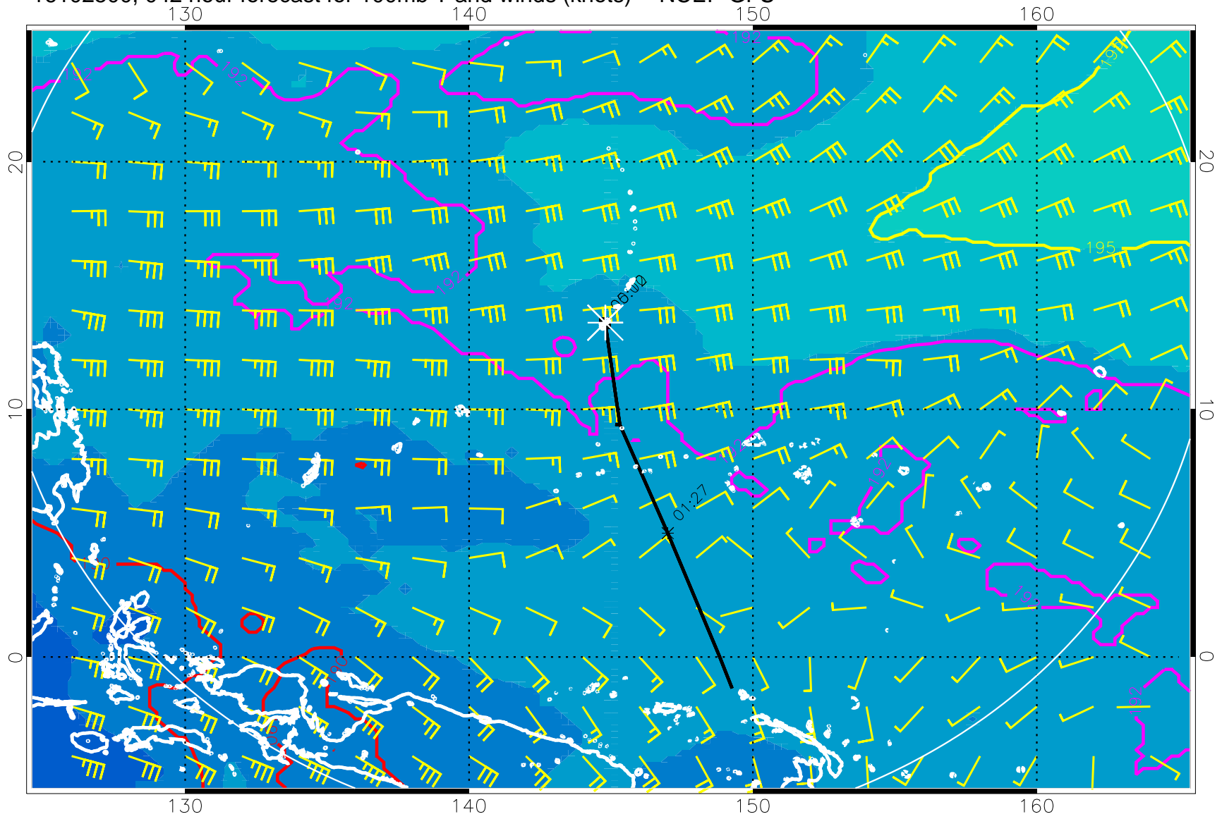
16102500, 042 hour forecast for 100mb T and winds (knots) -- NCEP GFS
