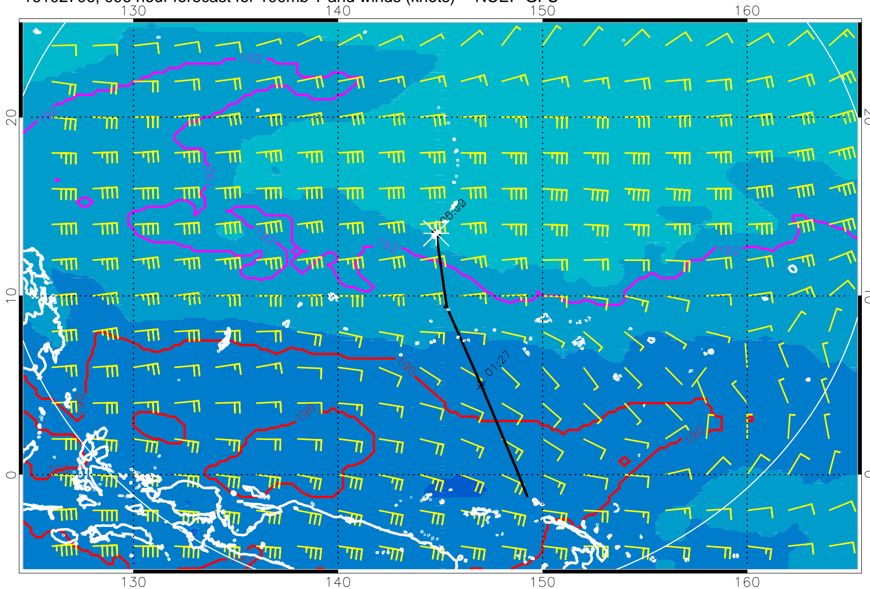
16102706, 096 hour forecast for 100mb T and winds (knots) -- NCEP GFS
