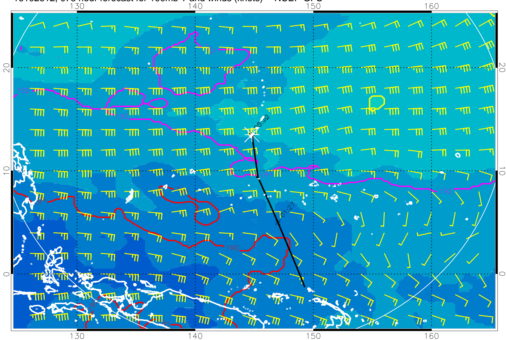
16102612, 078 hour forecast for 100mb T and winds (knots) -- NCEP GFS
