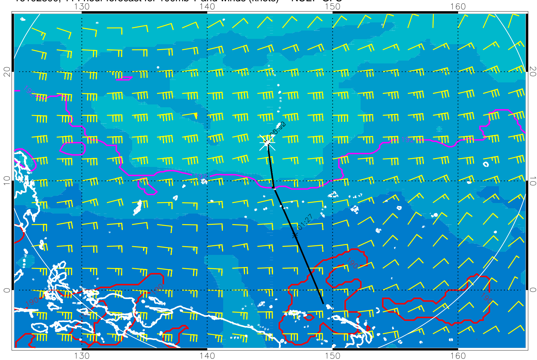
16102800, 114 hour forecast for 100mb T and winds (knots) -- NCEP GFS
