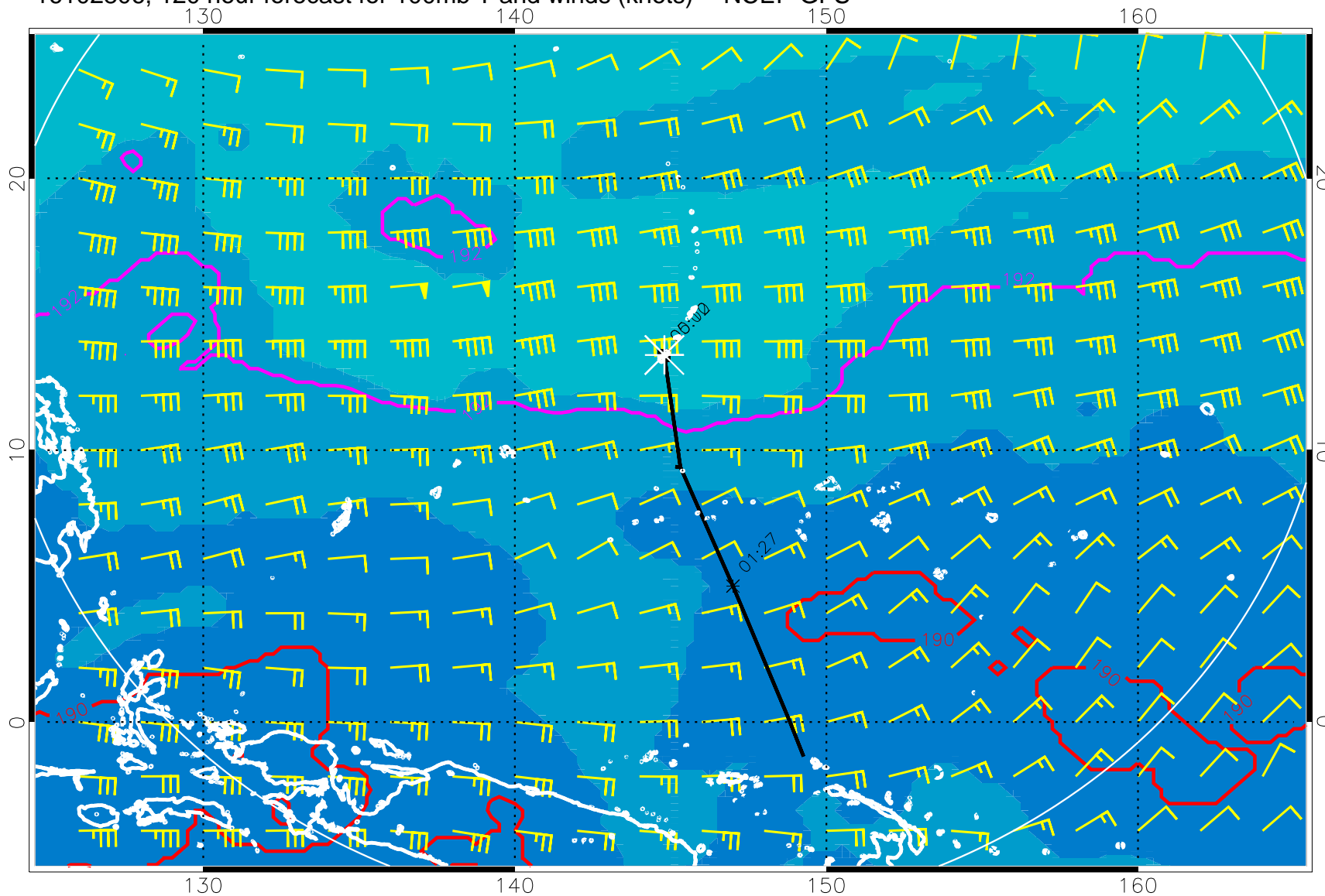
16102806, 120 hour forecast for 100mb T and winds (knots) -- NCEP GFS
