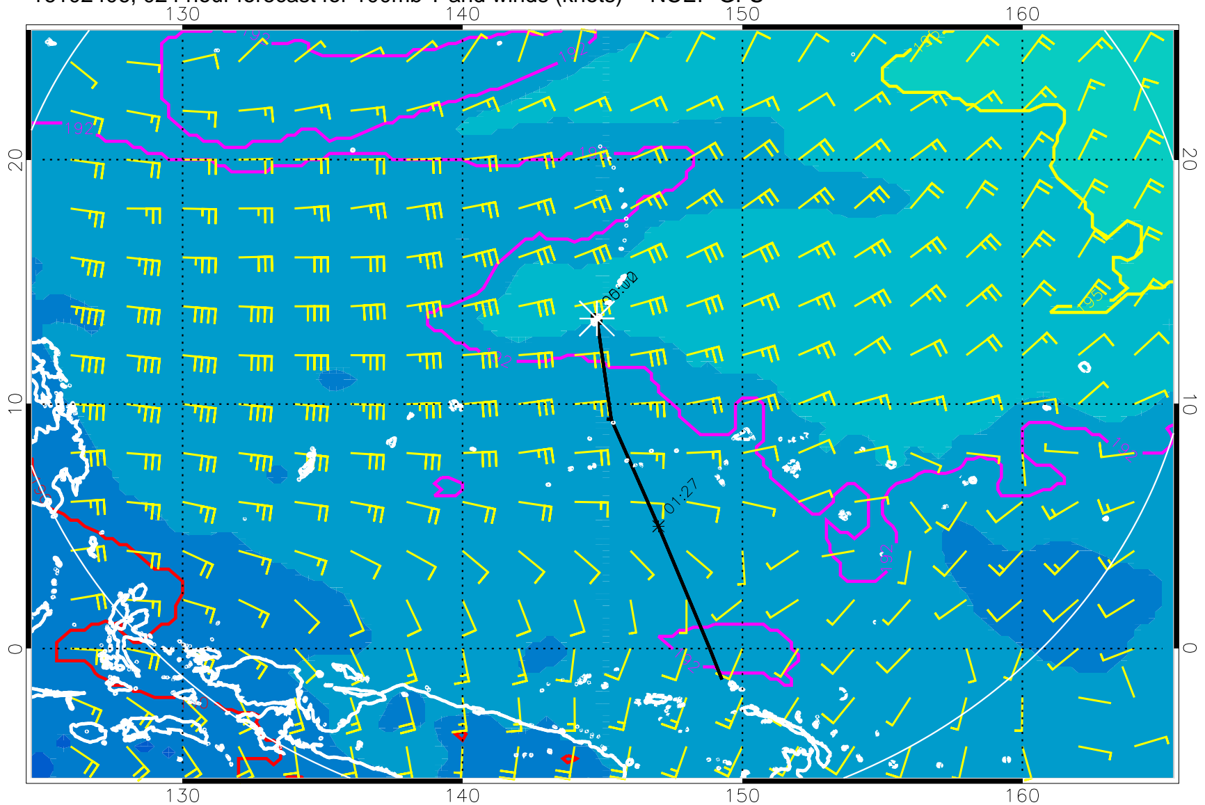
16102406, 024 hour forecast for 100mb T and winds (knots) -- NCEP GFS
