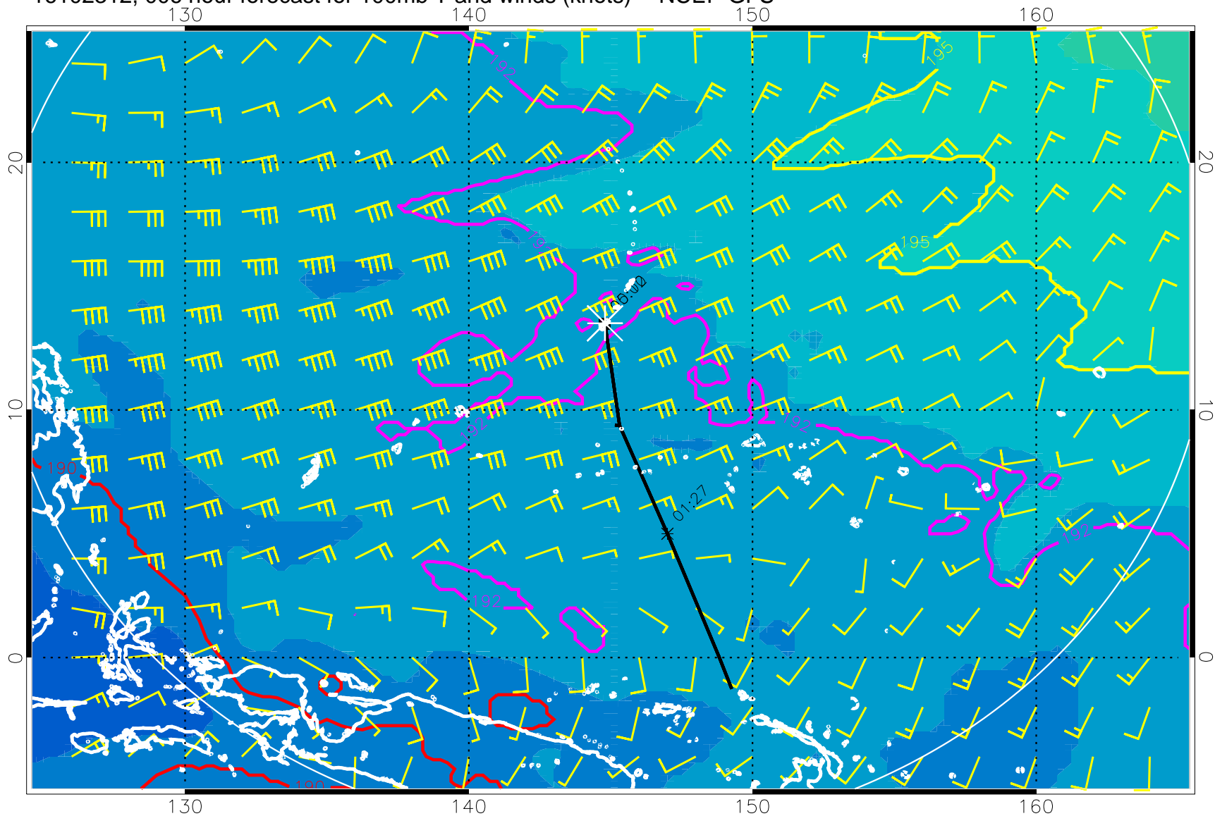
16102312, 006 hour forecast for 100mb T and winds (knots) -- NCEP GFS
