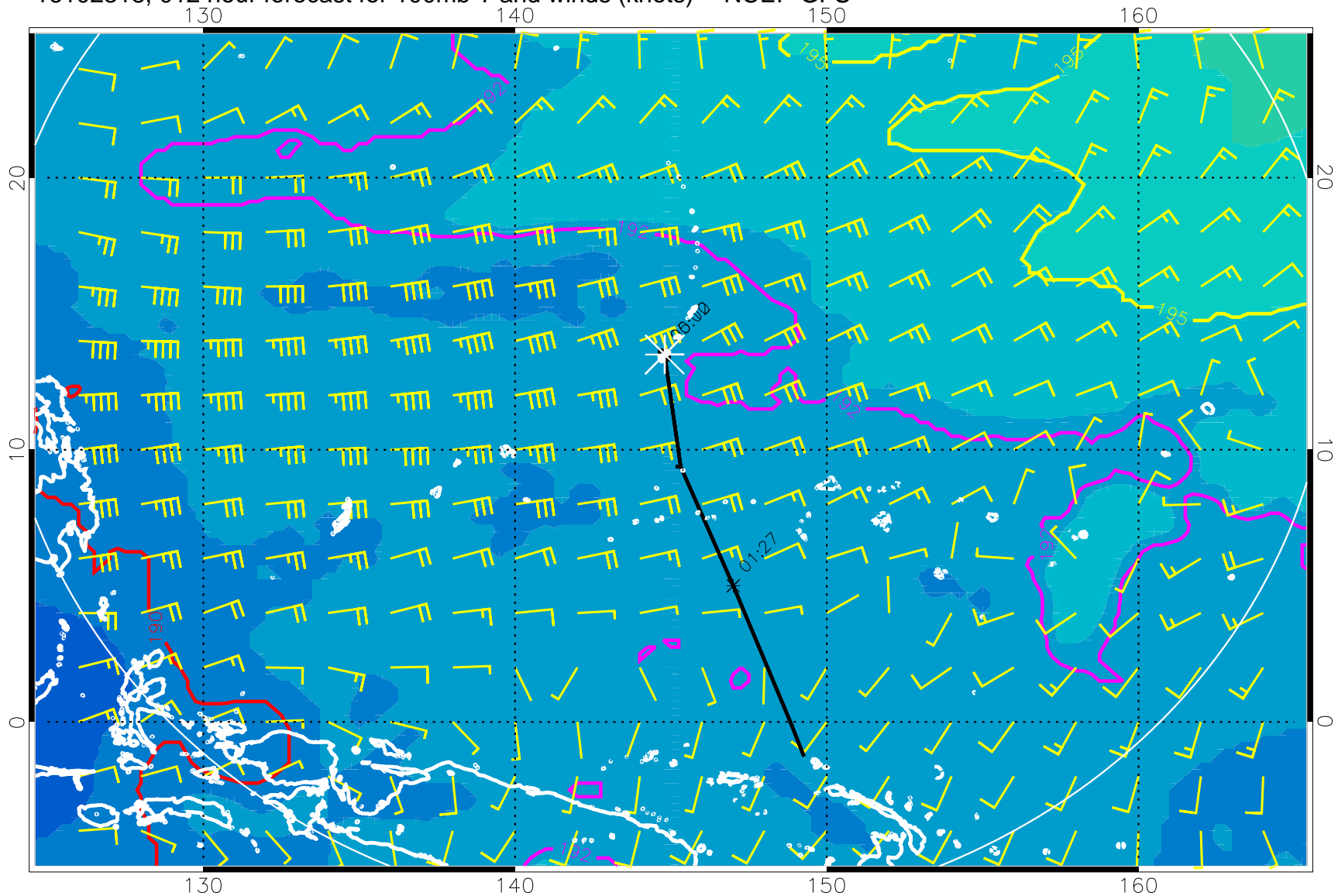
16102318, 012 hour forecast for 100mb T and winds (knots) -- NCEP GFS
