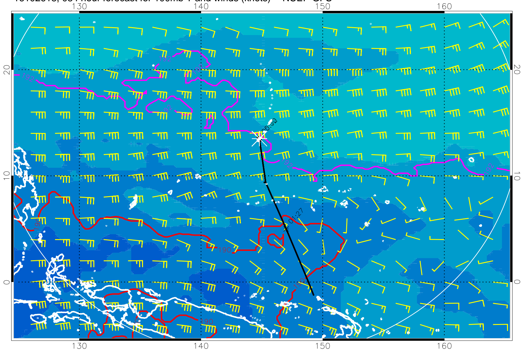
16102618, 084 hour forecast for 100mb T and winds (knots) -- NCEP GFS
