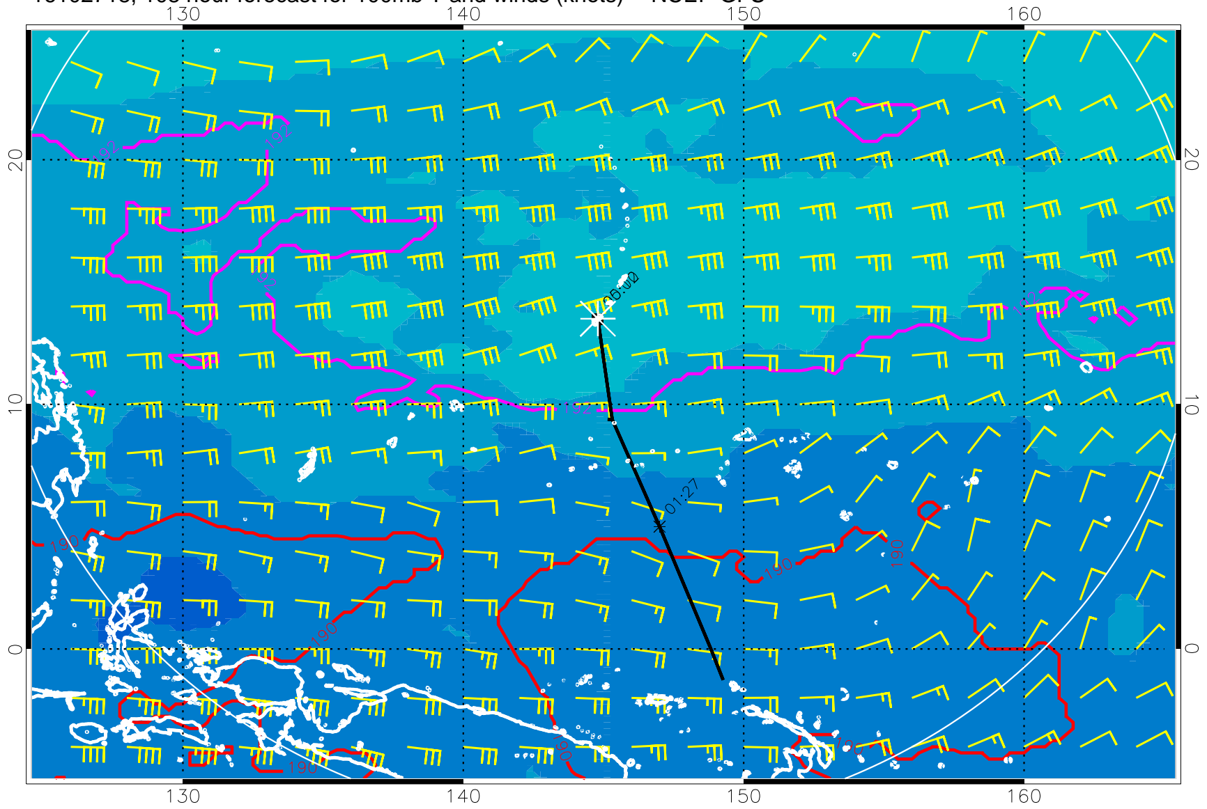
16102718, 108 hour forecast for 100mb T and winds (knots) -- NCEP GFS
