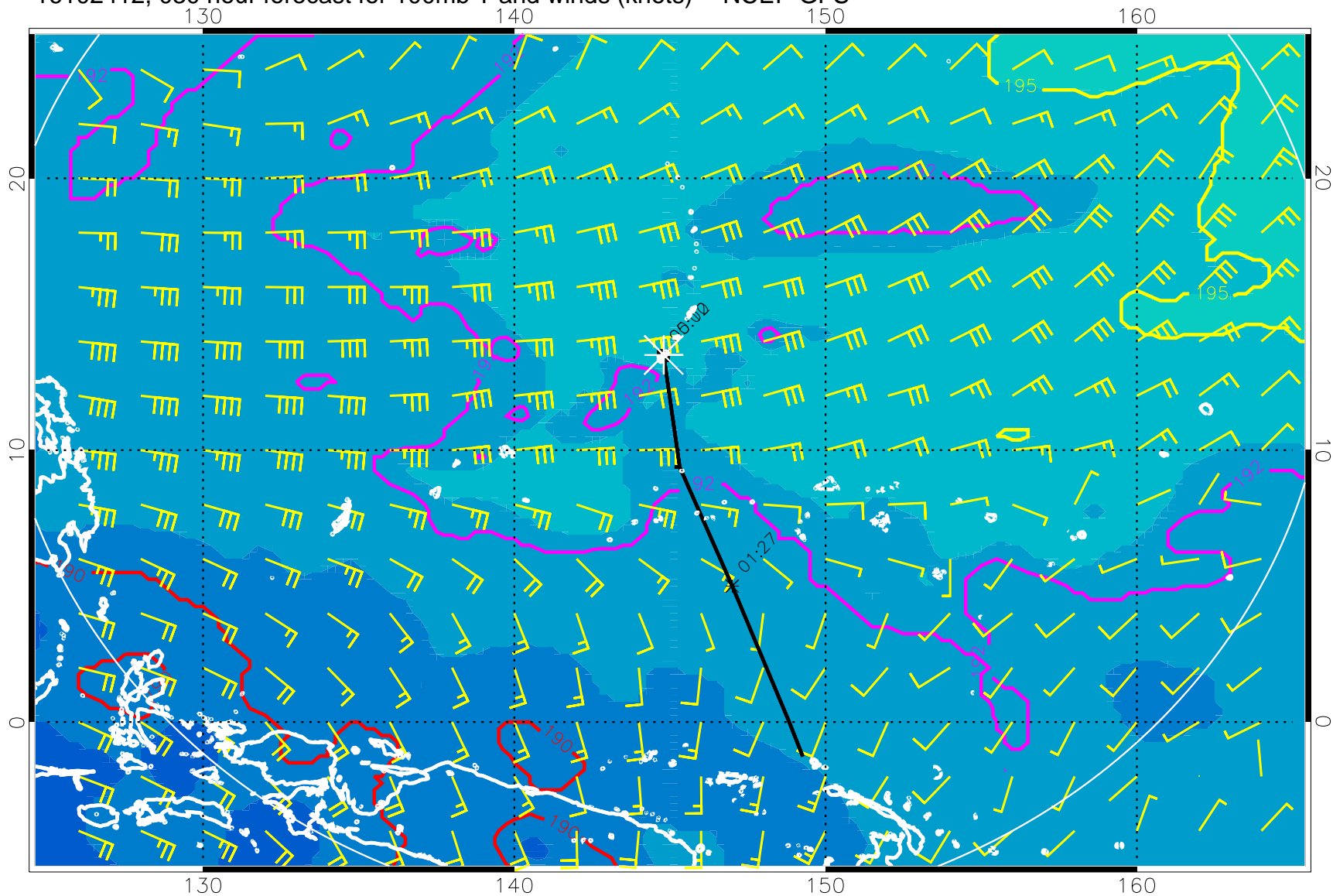
16102412, 030 hour forecast for 100mb T and winds (knots) -- NCEP GFS
