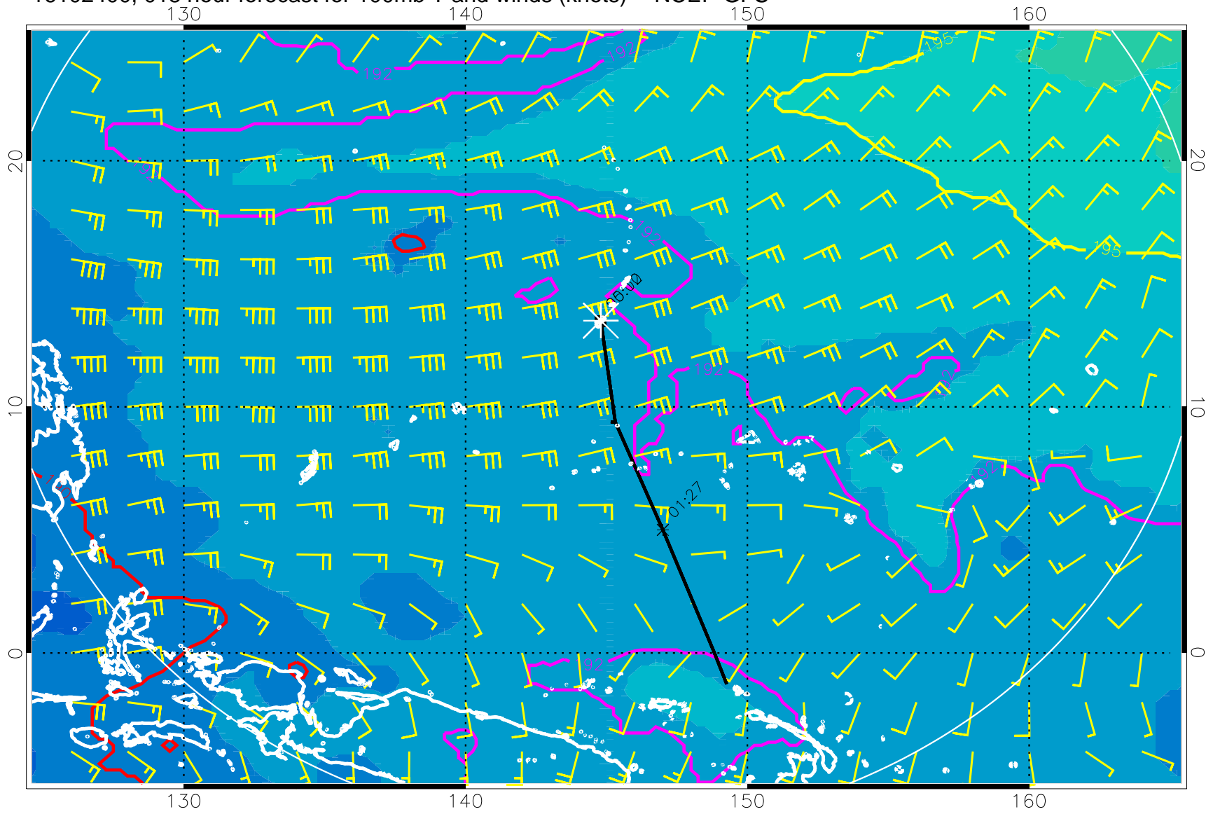
16102400, 018 hour forecast for 100mb T and winds (knots) -- NCEP GFS
