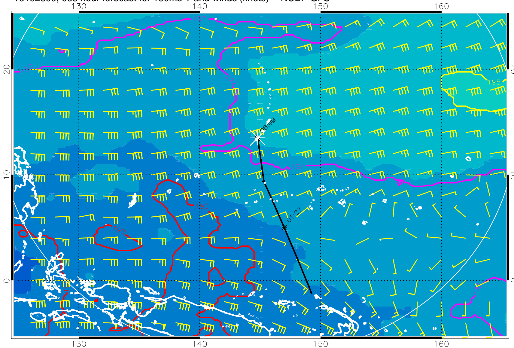
16102600, 066 hour forecast for 100mb T and winds (knots) -- NCEP GFS
