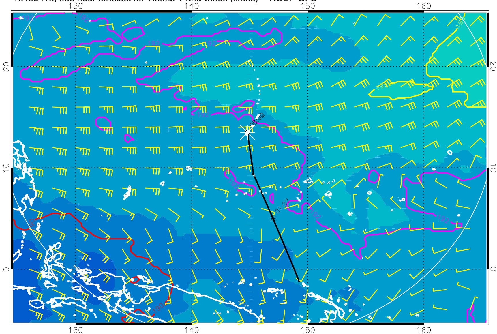
16102418, 036 hour forecast for 100mb T and winds (knots) -- NCEP GFS
