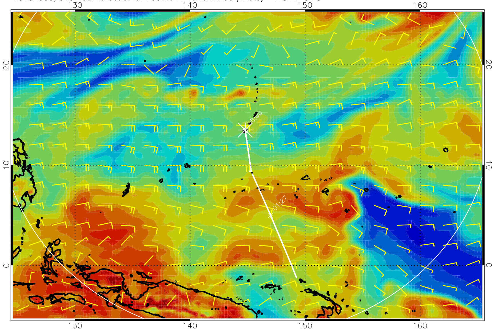
16102506, 048 hour forecast for 700mb RH and winds (knots) -- NCEP GFS
