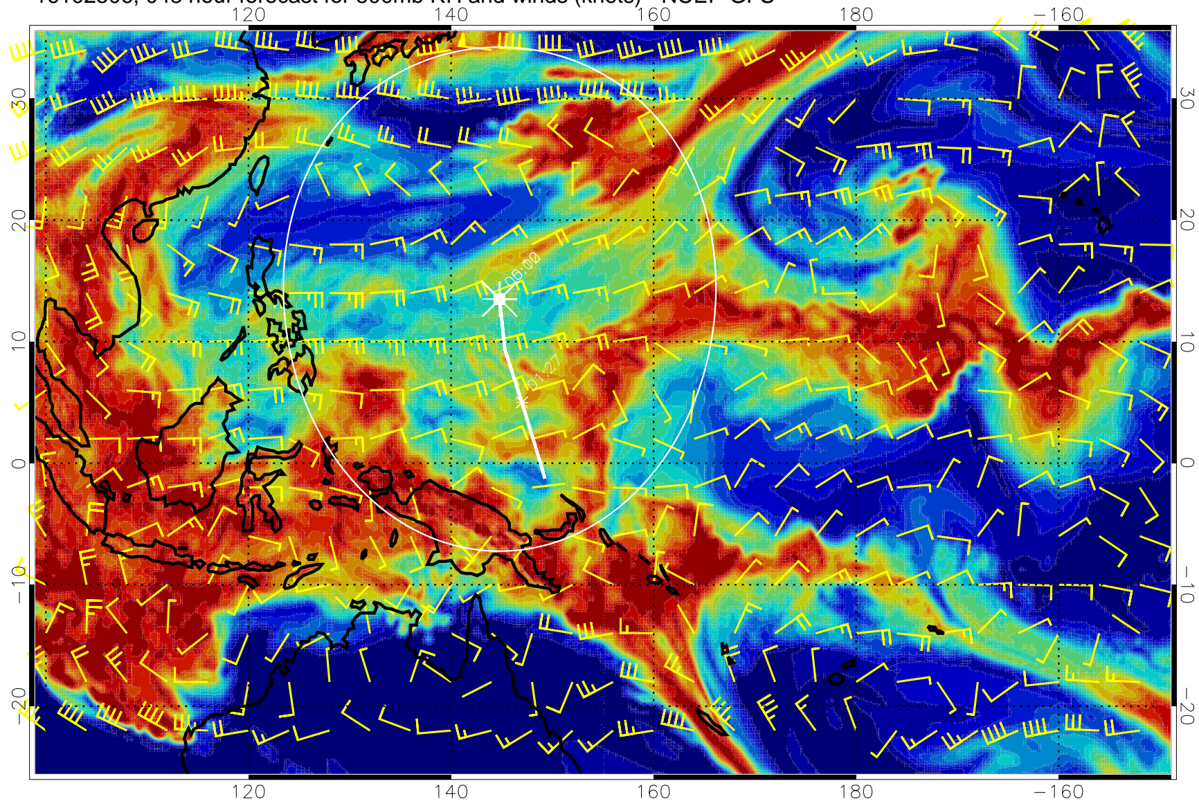
16102506, 048 hour forecast for 500mb RH and winds (knots) - NCEP GFS
