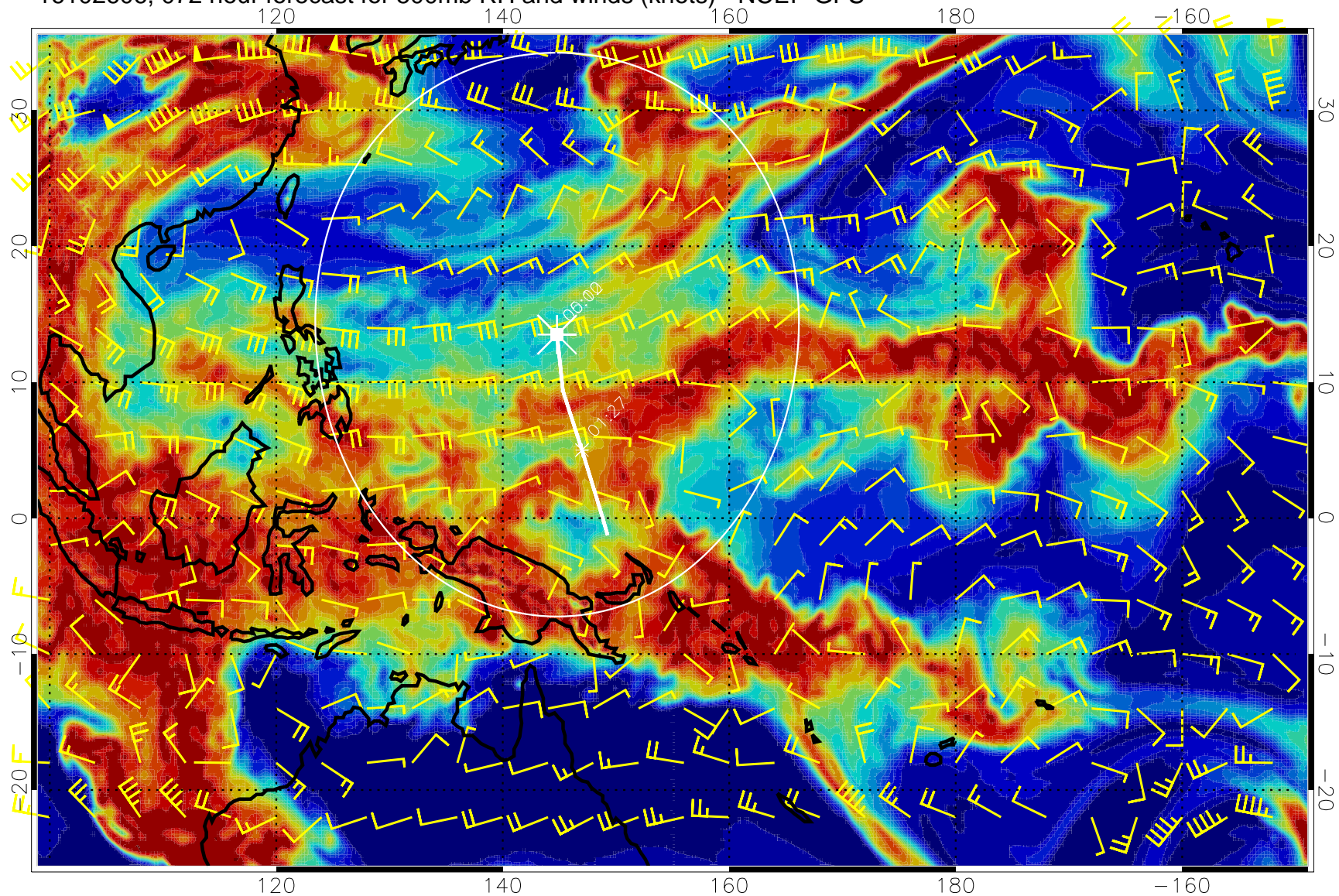
16102606, 072 hour forecast for 500mb RH and winds (knots) - NCEP GFS
