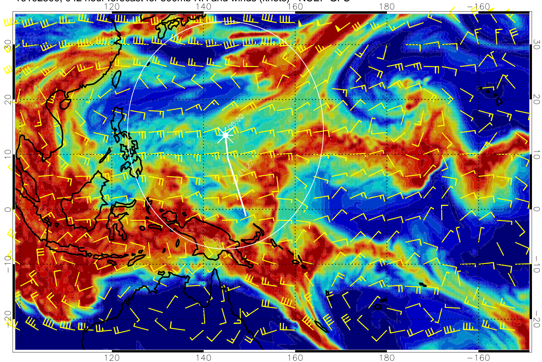
16102500, 042 hour forecast for 500mb RH and winds (knots) - NCEP GFS
