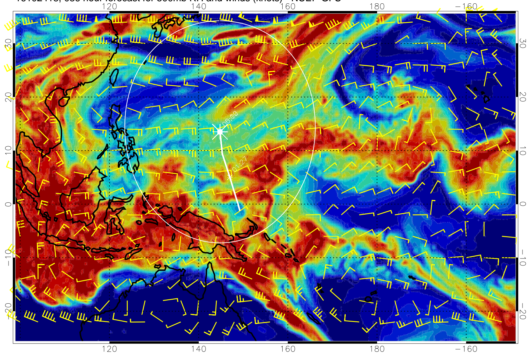
16102418, 036 hour forecast for 500mb RH and winds (knots) - NCEP GFS
