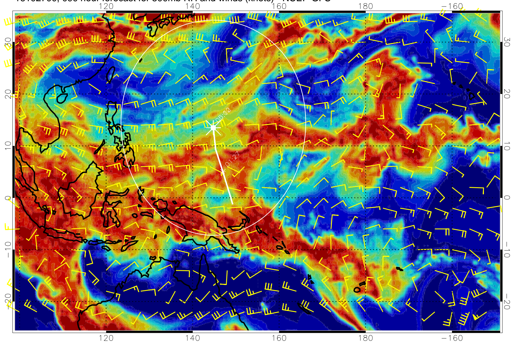
16102700, 090 hour forecast for 500mb RH and winds (knots) - NCEP GFS
