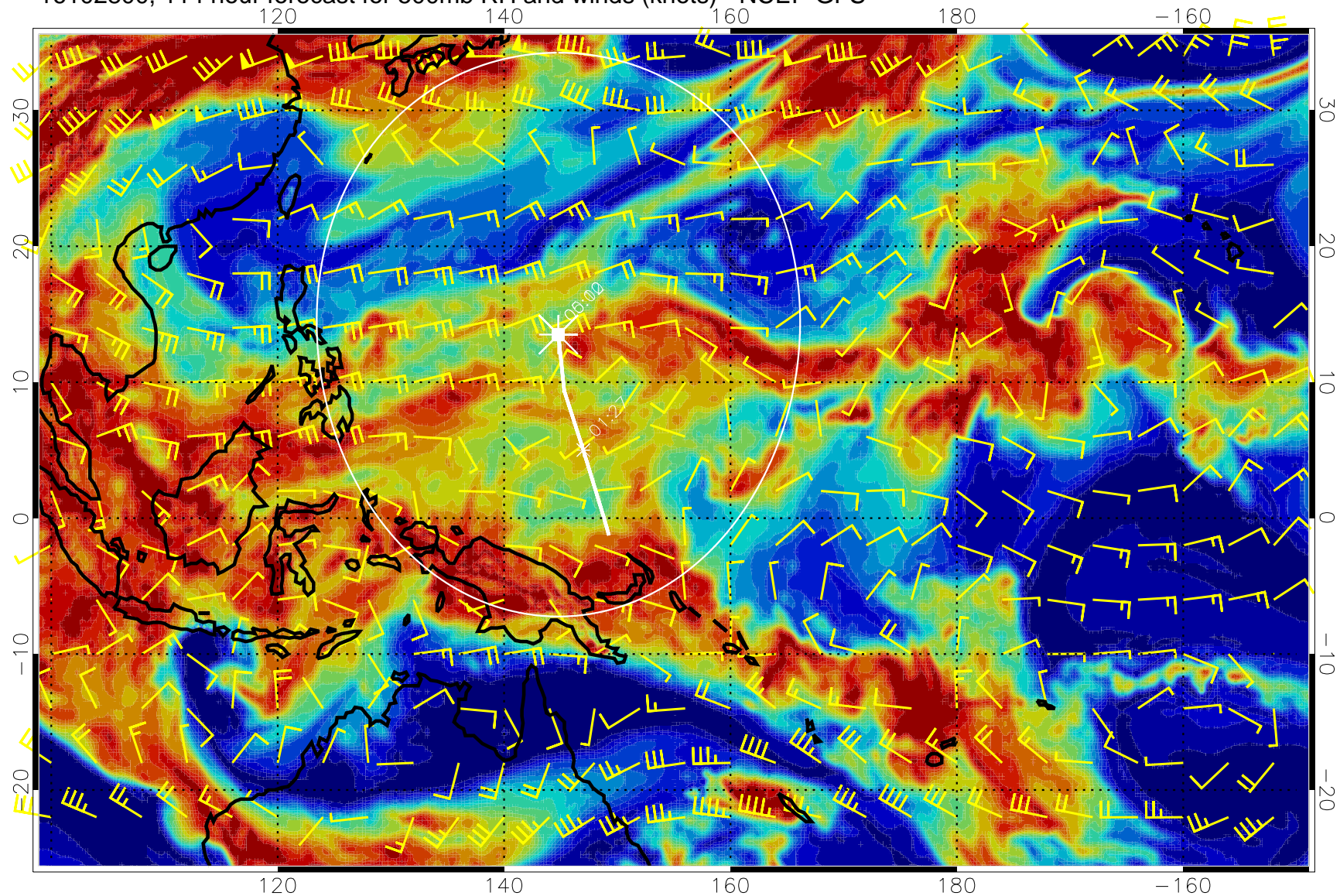
16102800, 114 hour forecast for 500mb RH and winds (knots) - NCEP GFS
