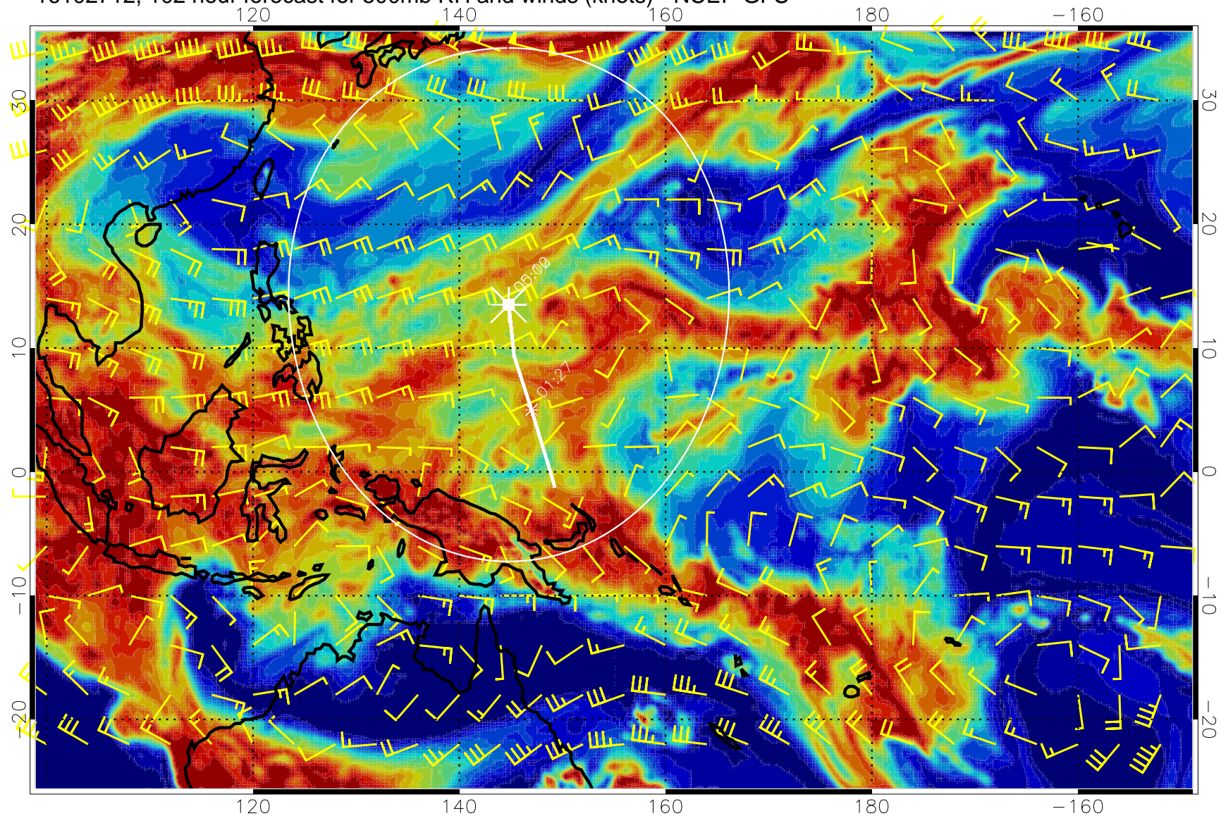
16102712, 102 hour forecast for 500mb RH and winds (knots) - NCEP GFS
