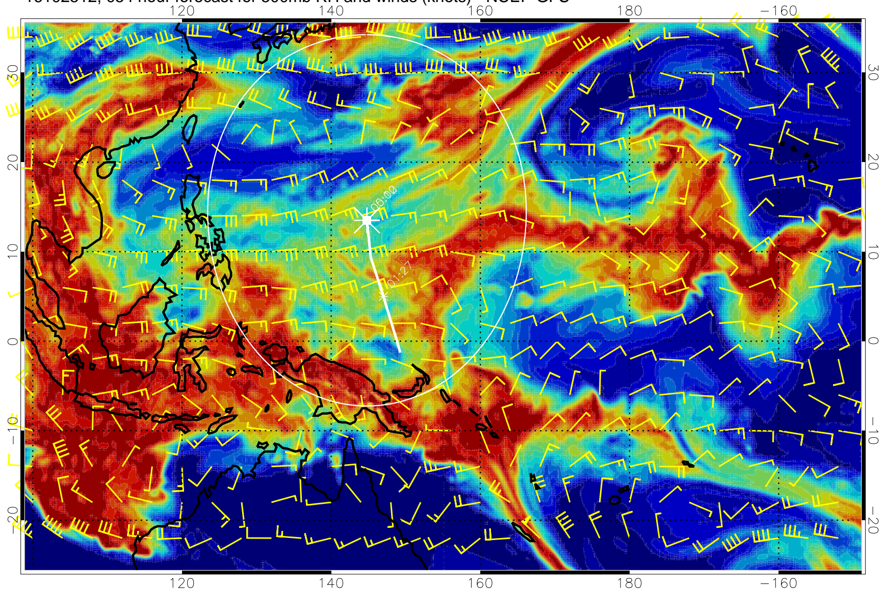
16102512, 054 hour forecast for 500mb RH and winds (knots) - NCEP GFS
