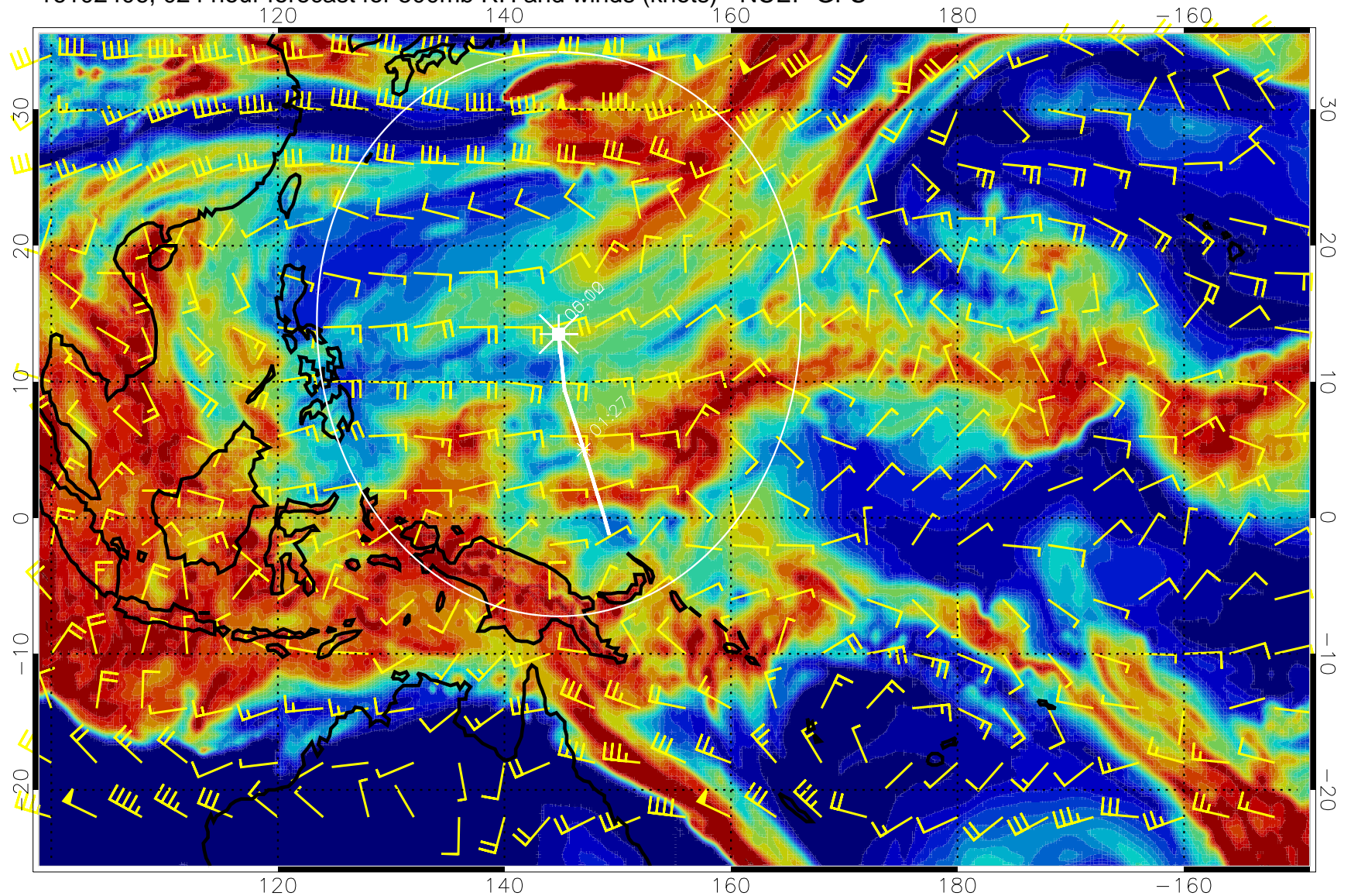
16102406, 024 hour forecast for 500mb RH and winds (knots) - NCEP GFS
