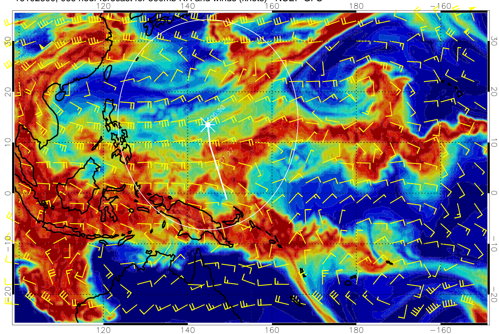
16102600, 066 hour forecast for 500mb RH and winds (knots) - NCEP GFS
