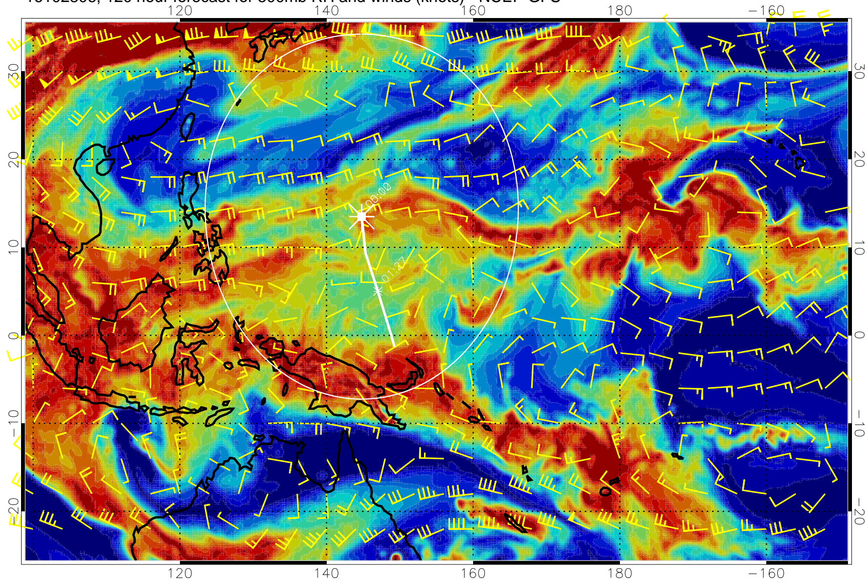
16102806, 120 hour forecast for 500mb RH and winds (knots) - NCEP GFS
