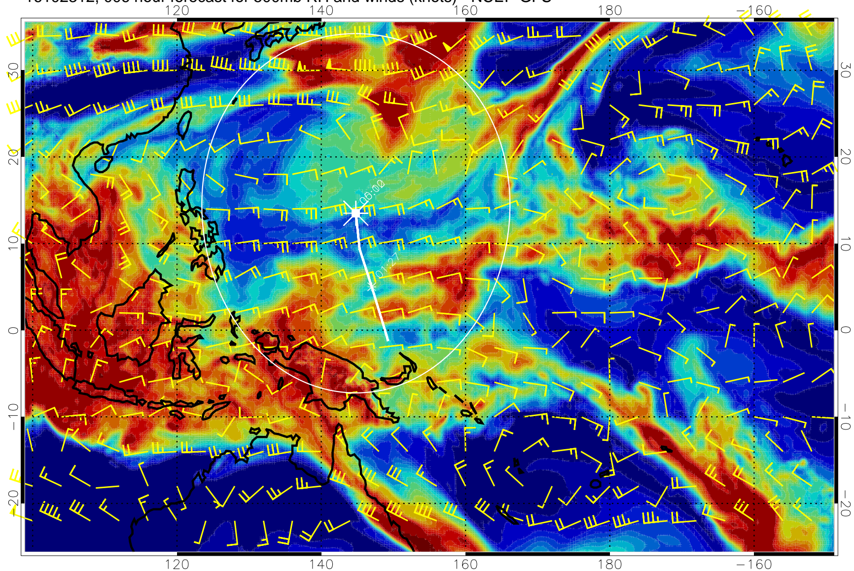
16102312, 006 hour forecast for 500mb RH and winds (knots) - NCEP GFS
