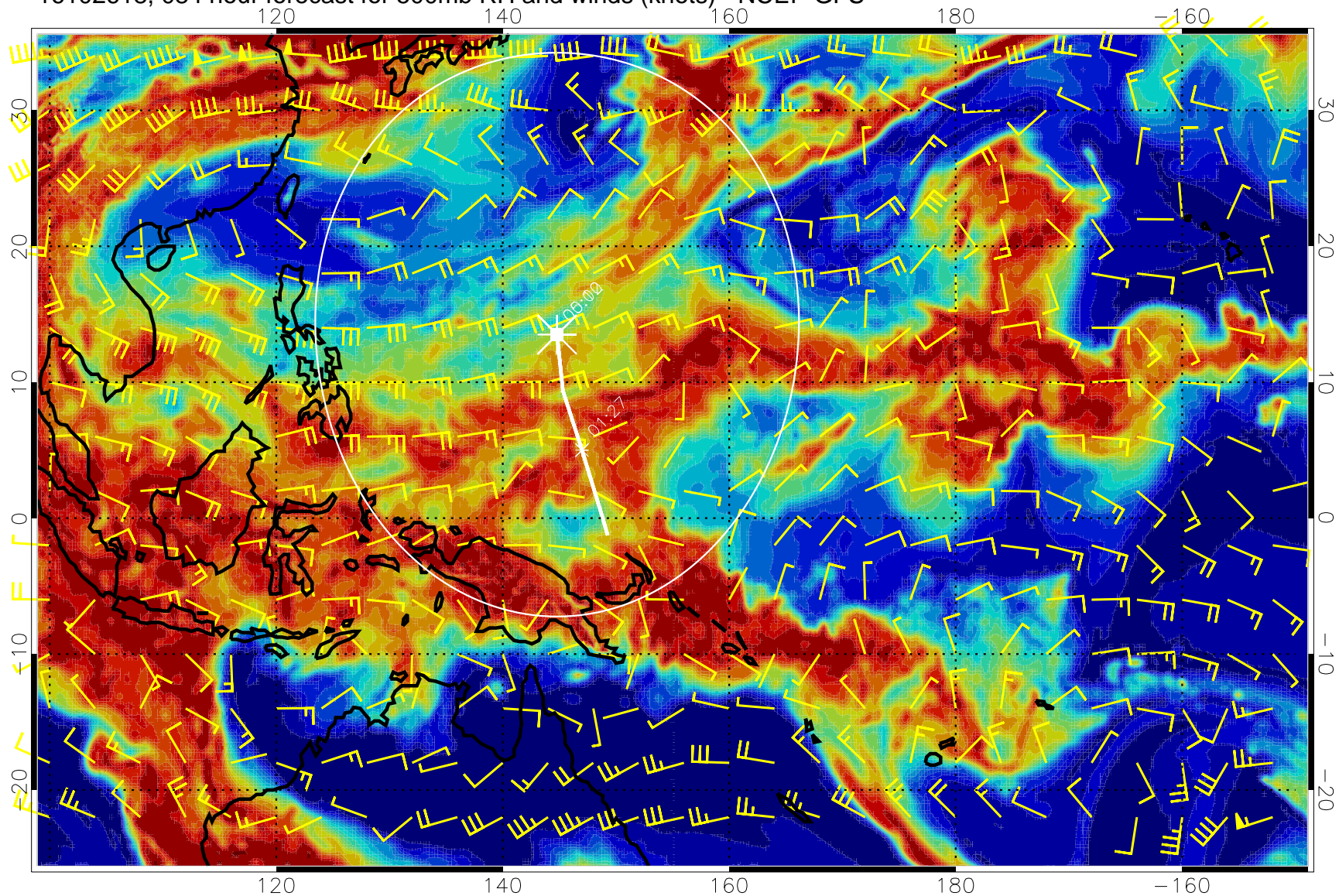
16102618, 084 hour forecast for 500mb RH and winds (knots) - NCEP GFS
