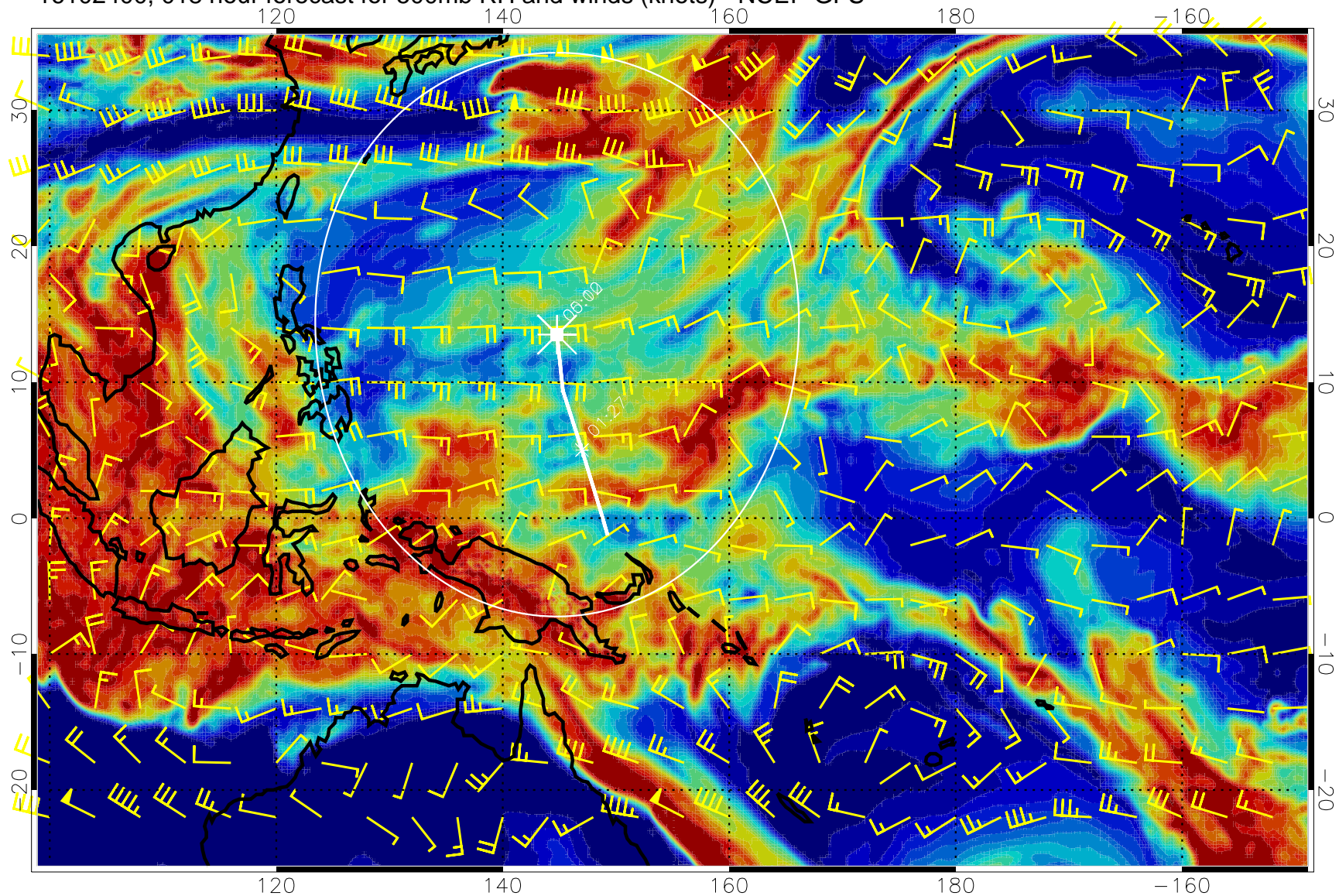
16102400, 018 hour forecast for 500mb RH and winds (knots) - NCEP GFS
