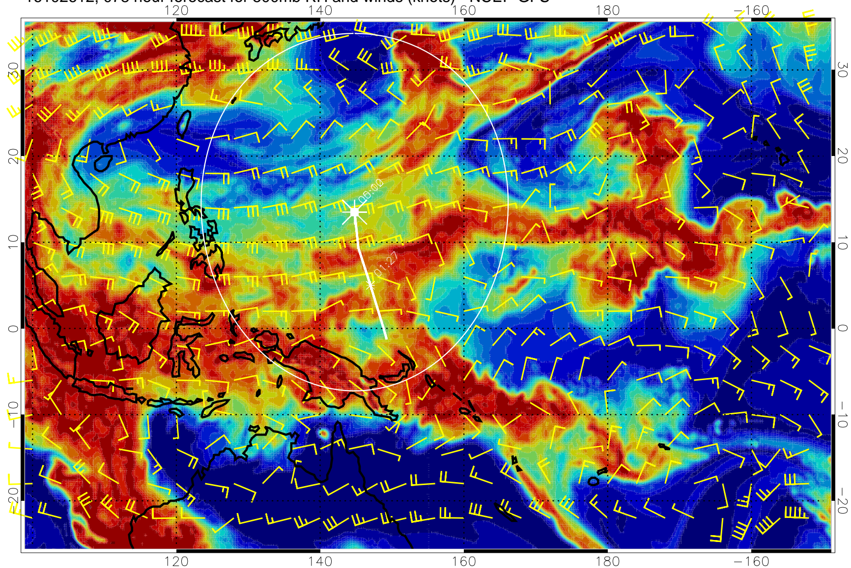
16102612, 078 hour forecast for 500mb RH and winds (knots) - NCEP GFS
