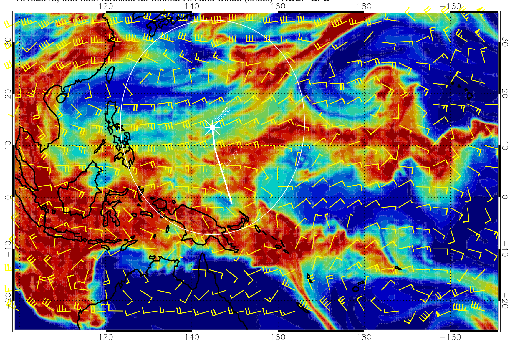
16102518, 060 hour forecast for 500mb RH and winds (knots) - NCEP GFS
