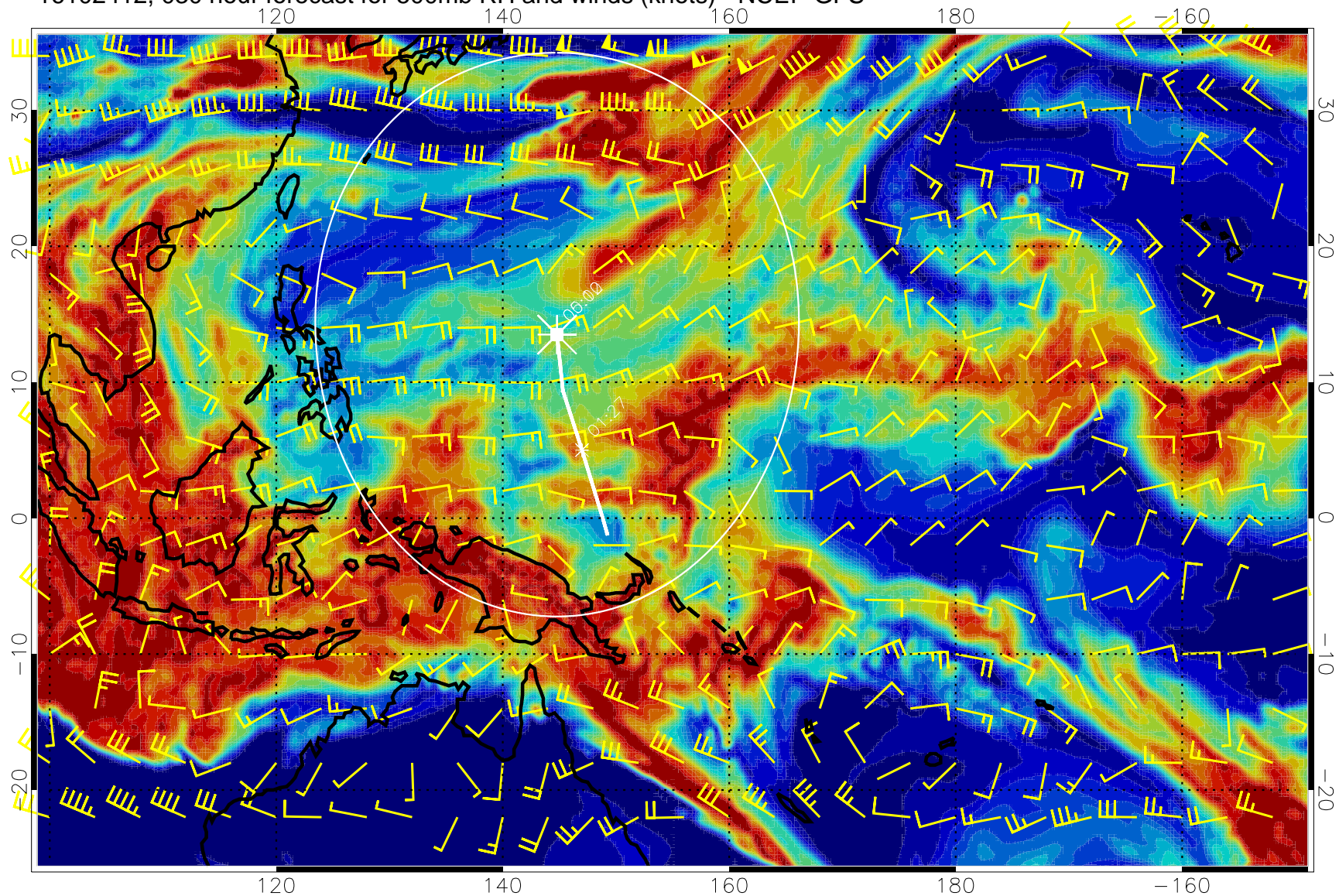
16102412, 030 hour forecast for 500mb RH and winds (knots) - NCEP GFS
