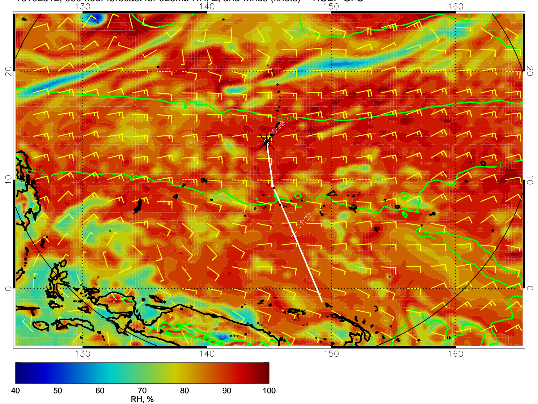
16102512, 060 hour forecast for 925mb RH, Z, and winds (knots) -- NCEP GFS
