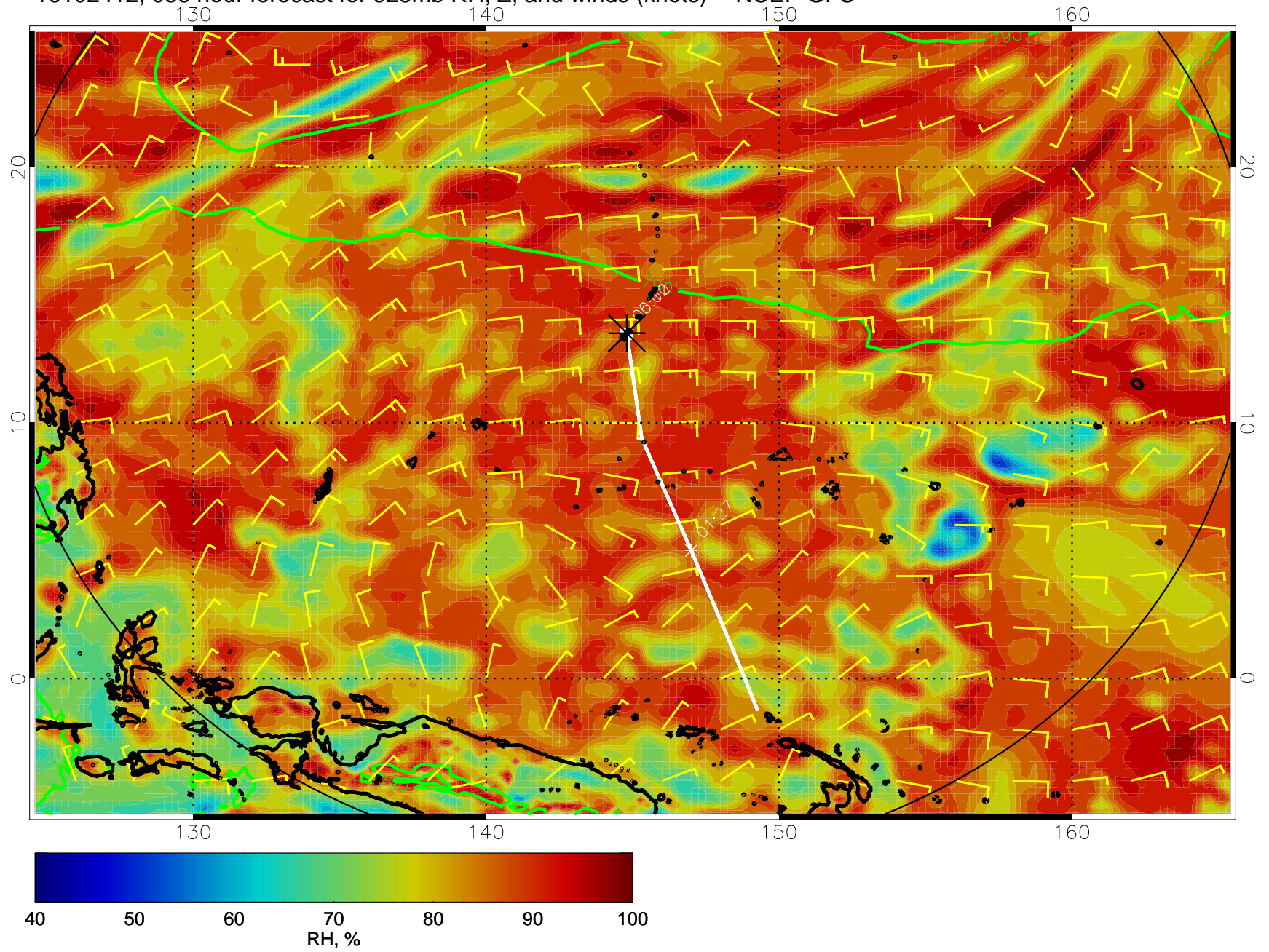
16102412, 036 hour forecast for 925mb RH, Z, and winds (knots) -- NCEP GFS
