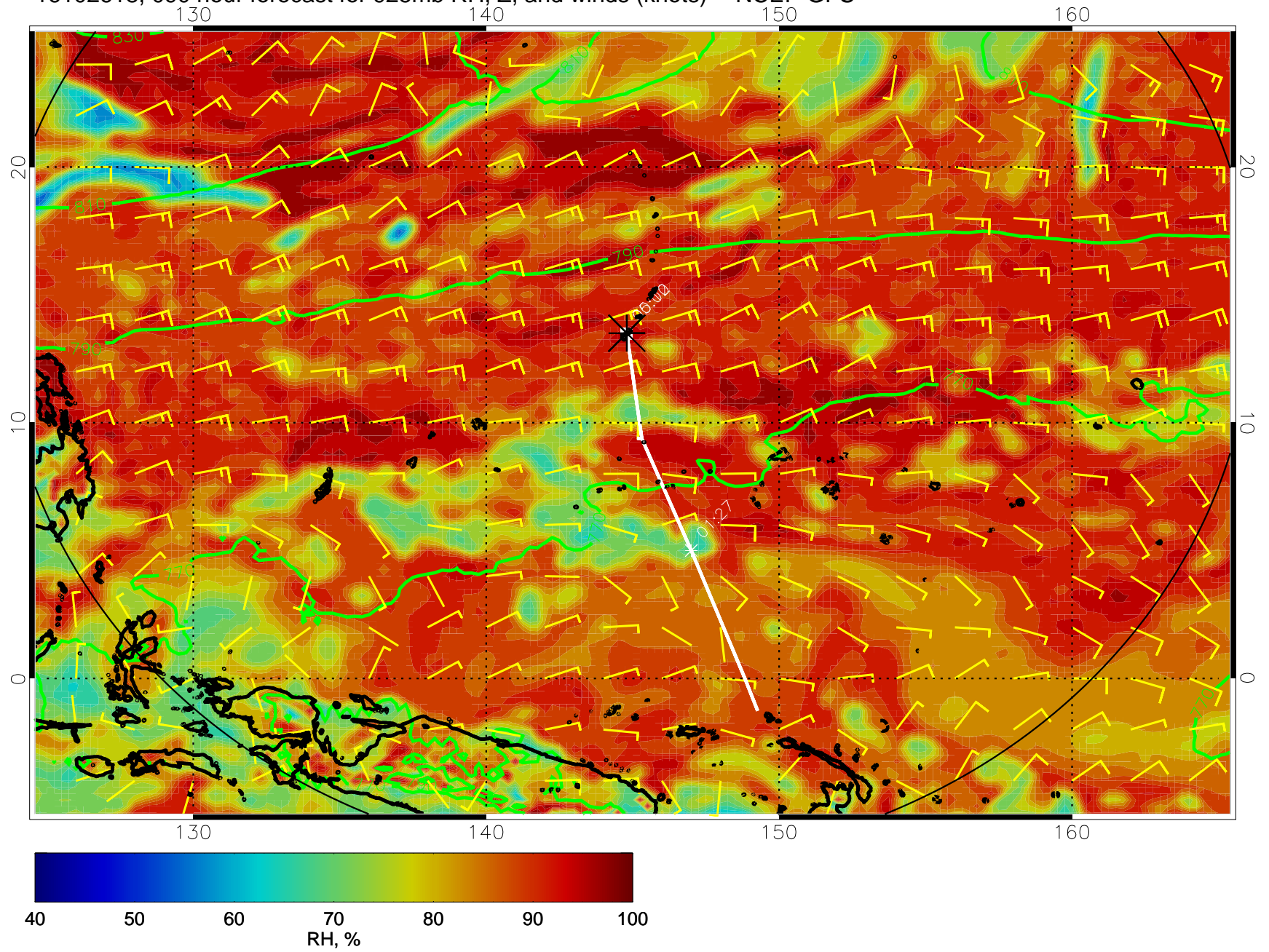
16102618, 090 hour forecast for 925mb RH, Z, and winds (knots) -- NCEP GFS
