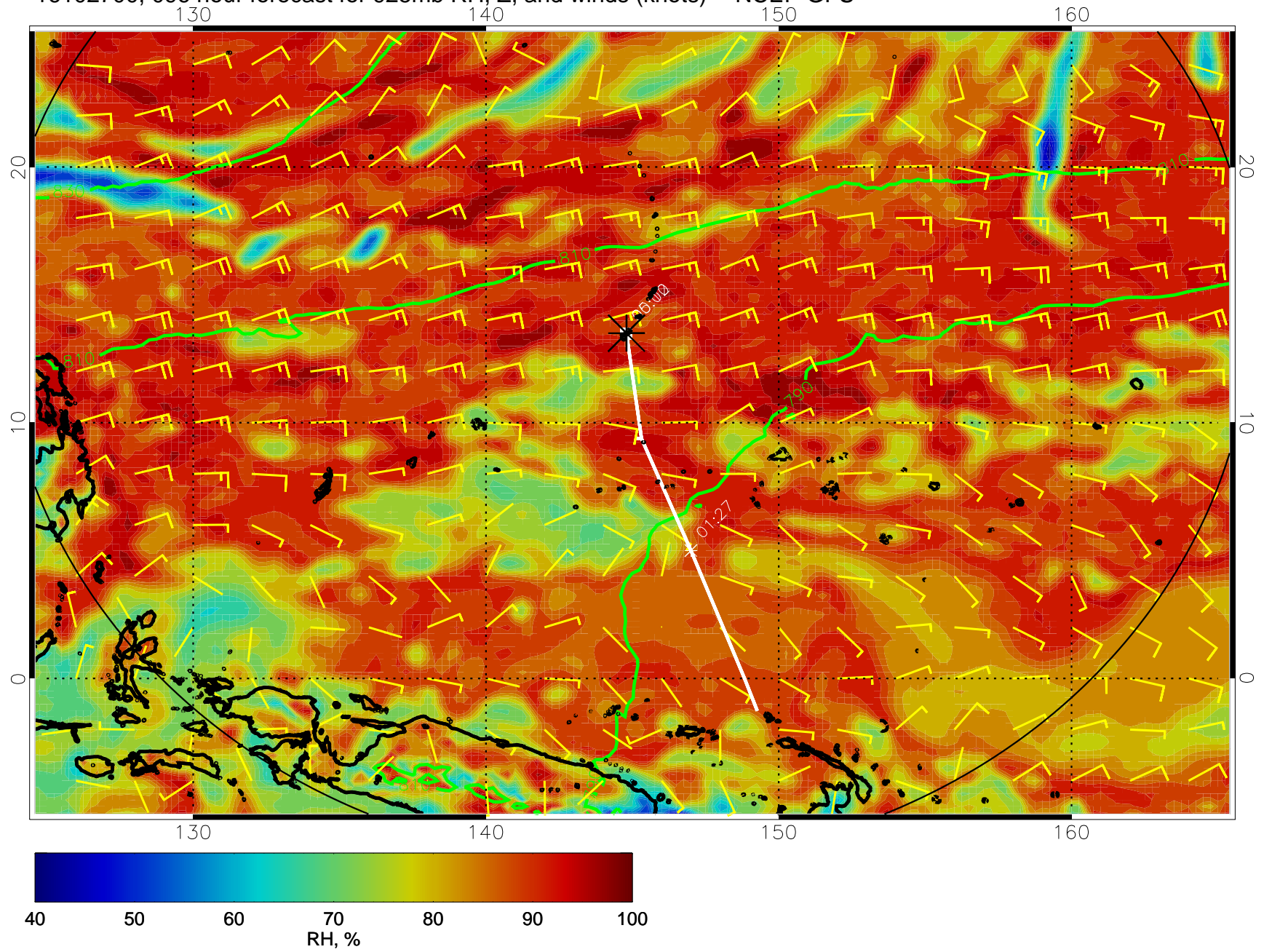
16102700, 096 hour forecast for 925mb RH, Z, and winds (knots) -- NCEP GFS
