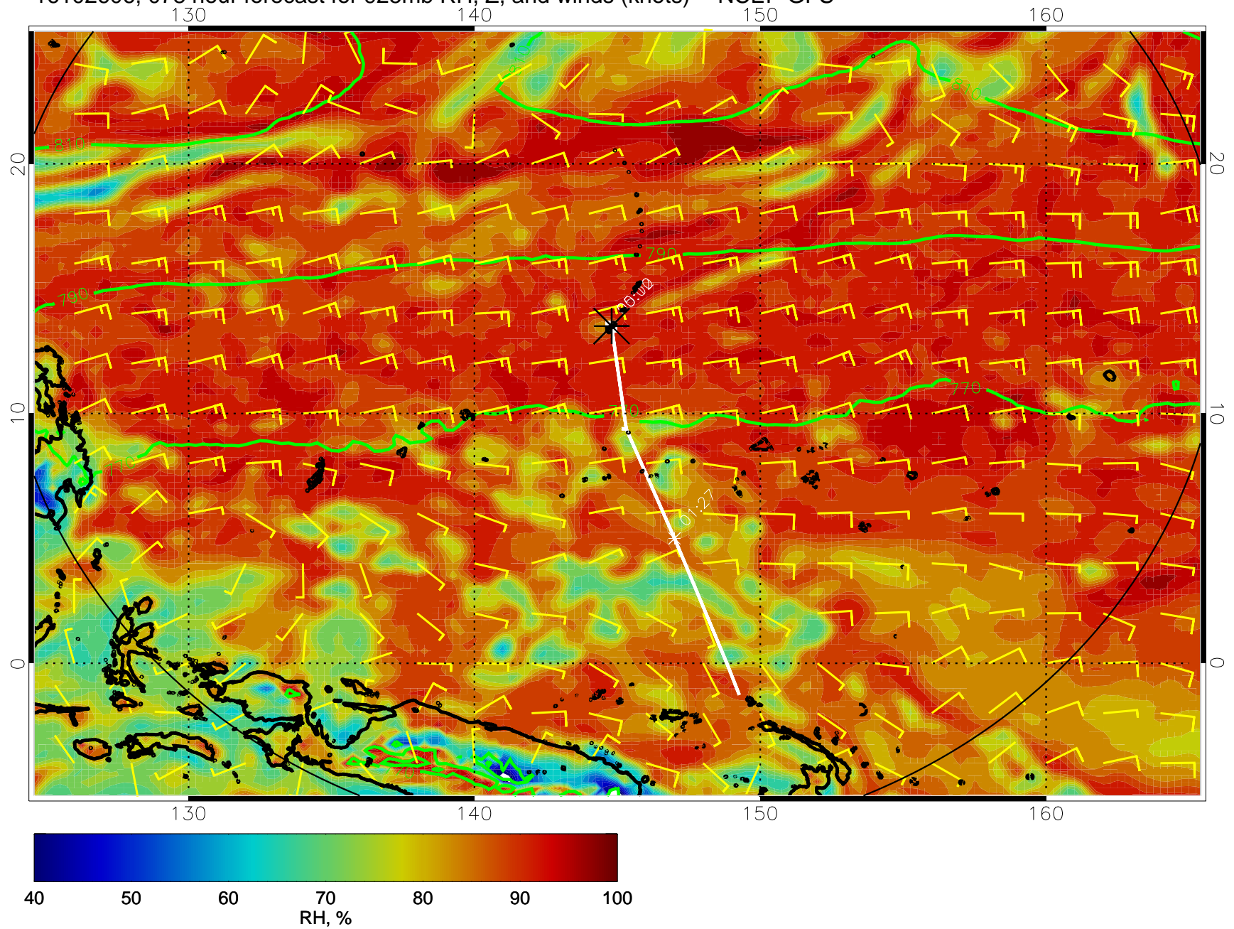
16102606, 078 hour forecast for 925mb RH, Z, and winds (knots) -- NCEP GFS
