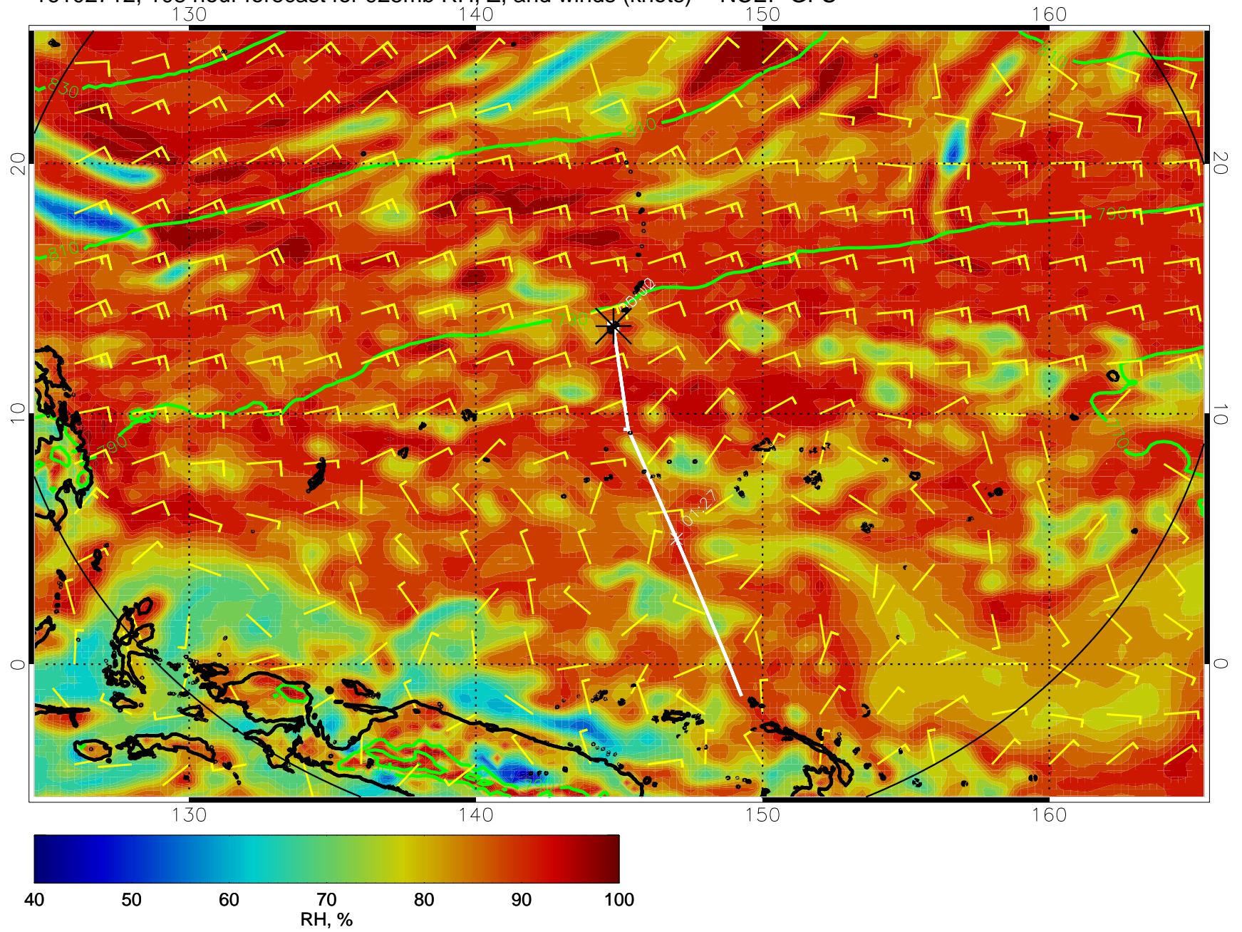
16102712, 108 hour forecast for 925mb RH, Z, and winds (knots) -- NCEP GFS
