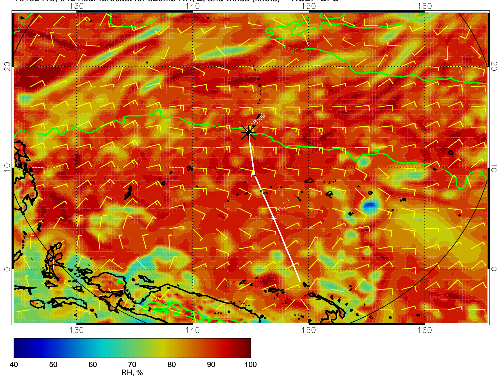
16102418, 042 hour forecast for 925mb RH, Z, and winds (knots) -- NCEP GFS
