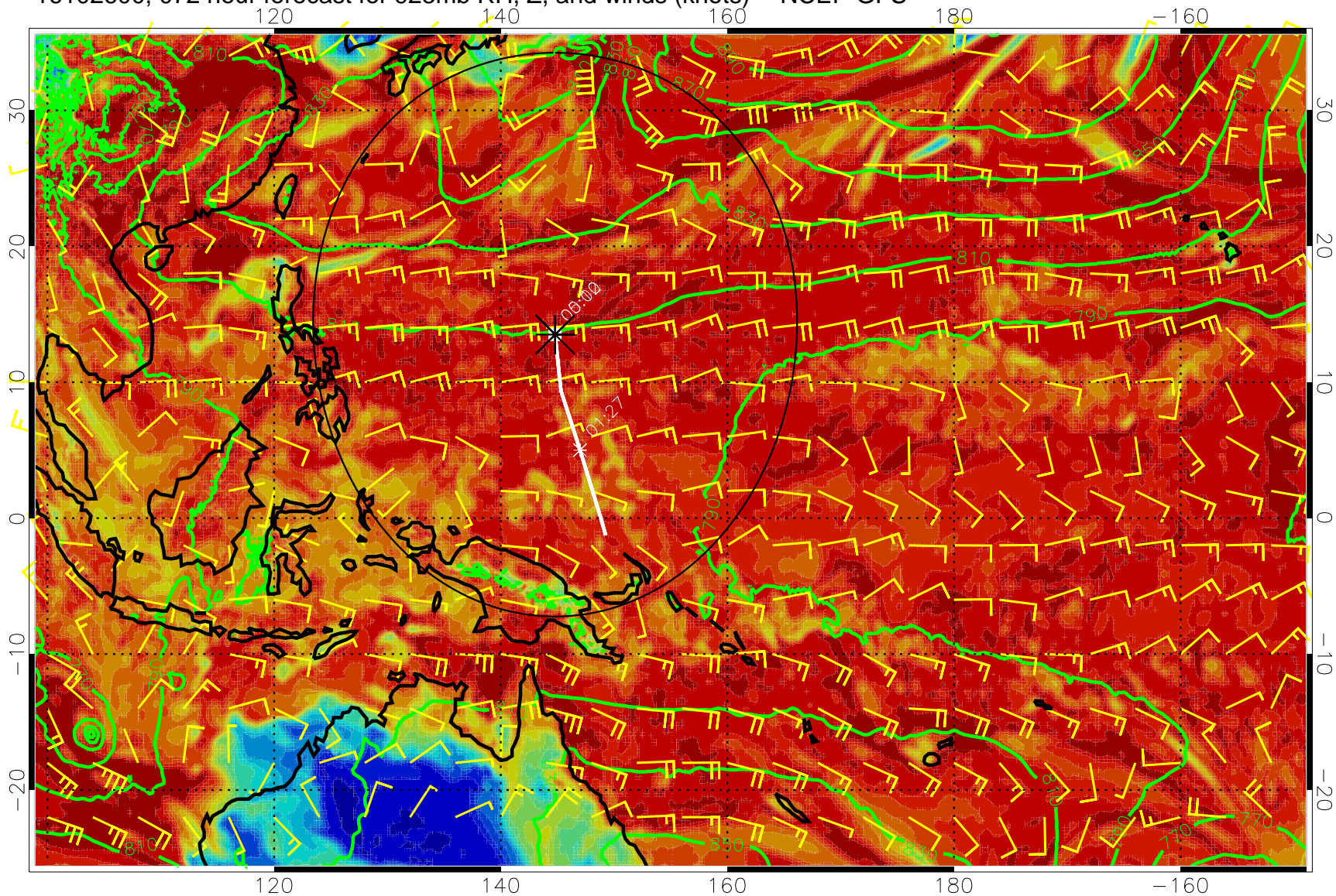
16102600, 072 hour forecast for 925mb RH, Z, and winds (knots) -- NCEP GFS
