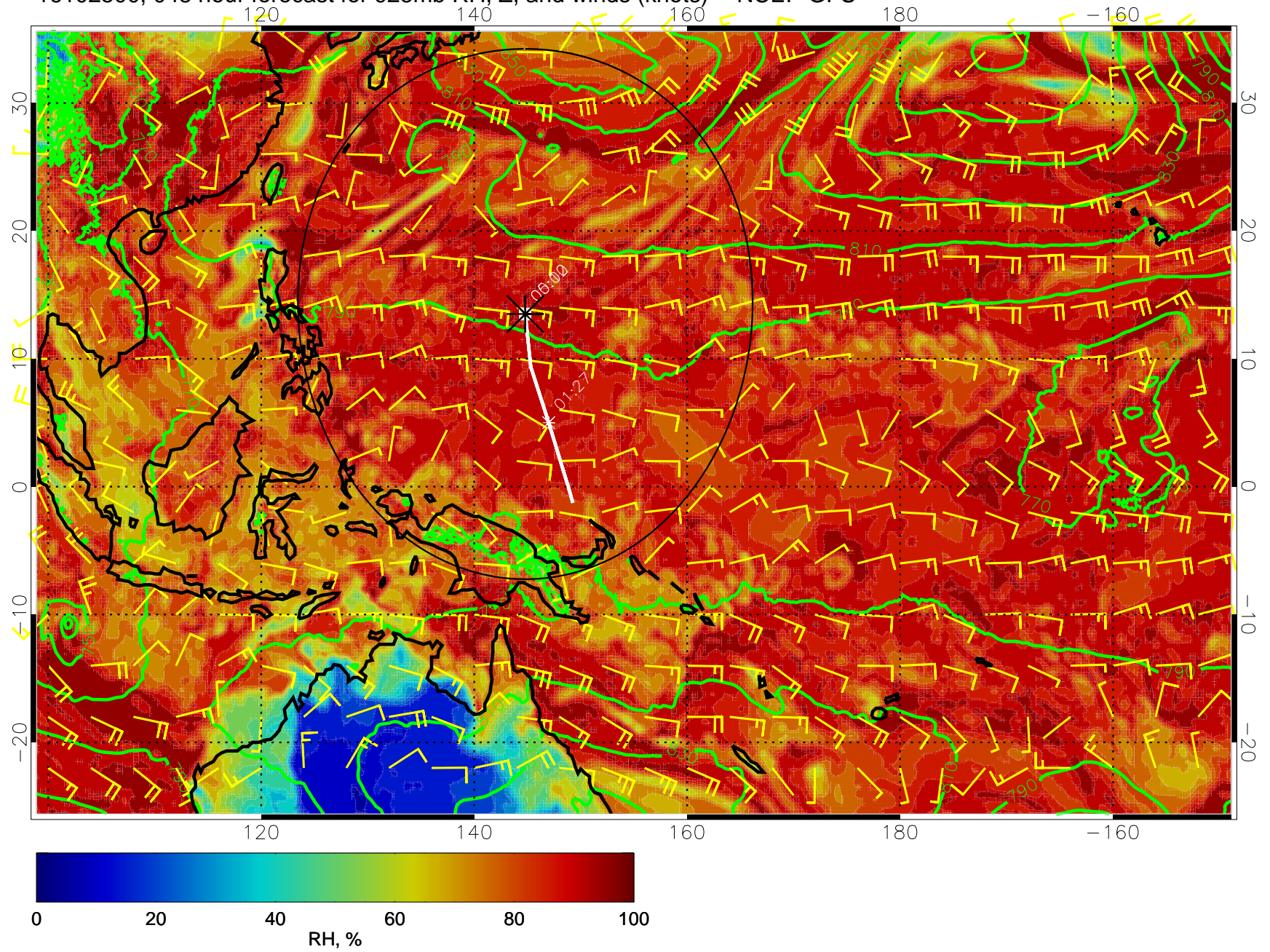
16102500, 048 hour forecast for 925mb RH, Z, and winds (knots) -- NCEP GFS
