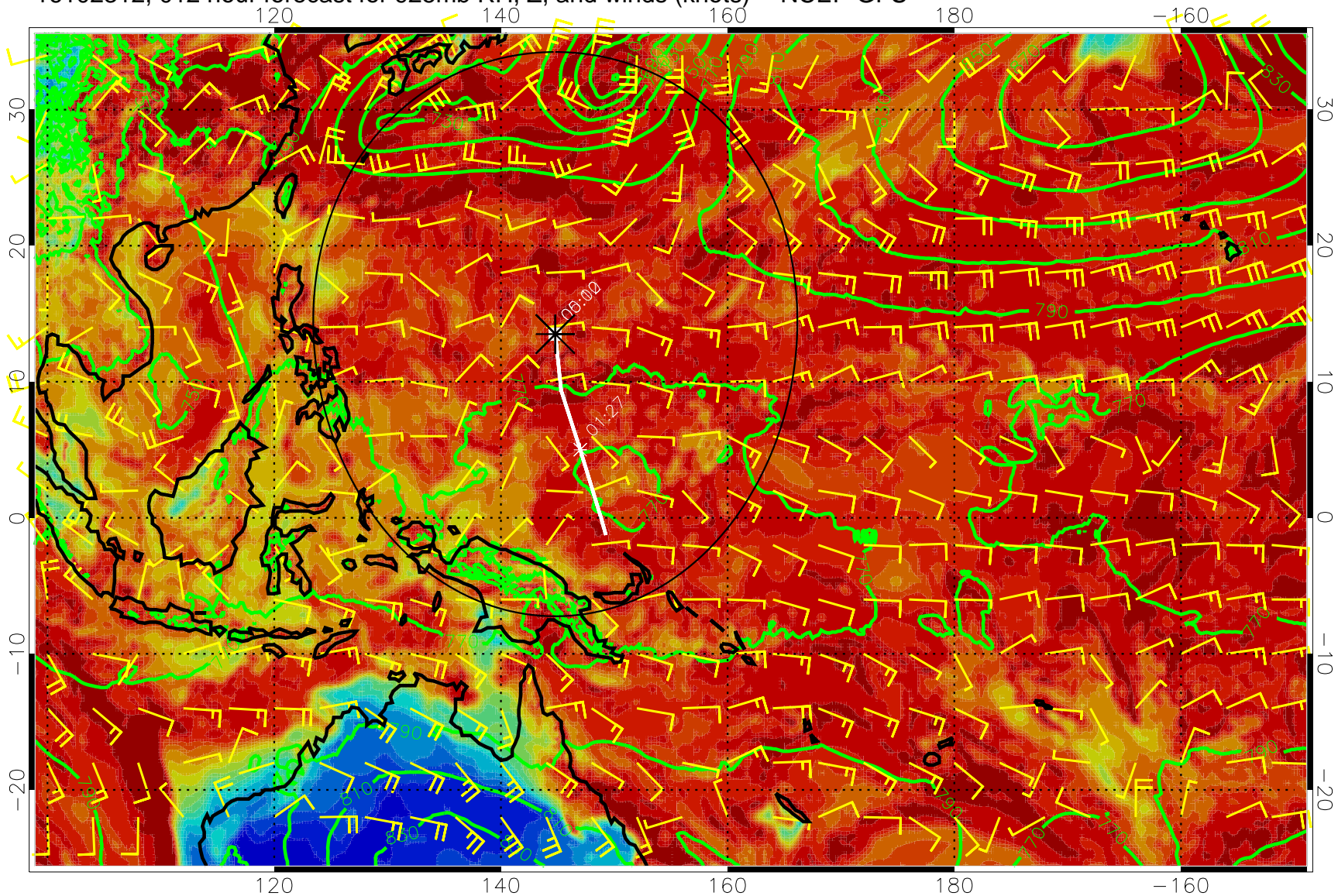
16102312, 012 hour forecast for 925mb RH, Z, and winds (knots) -- NCEP GFS
