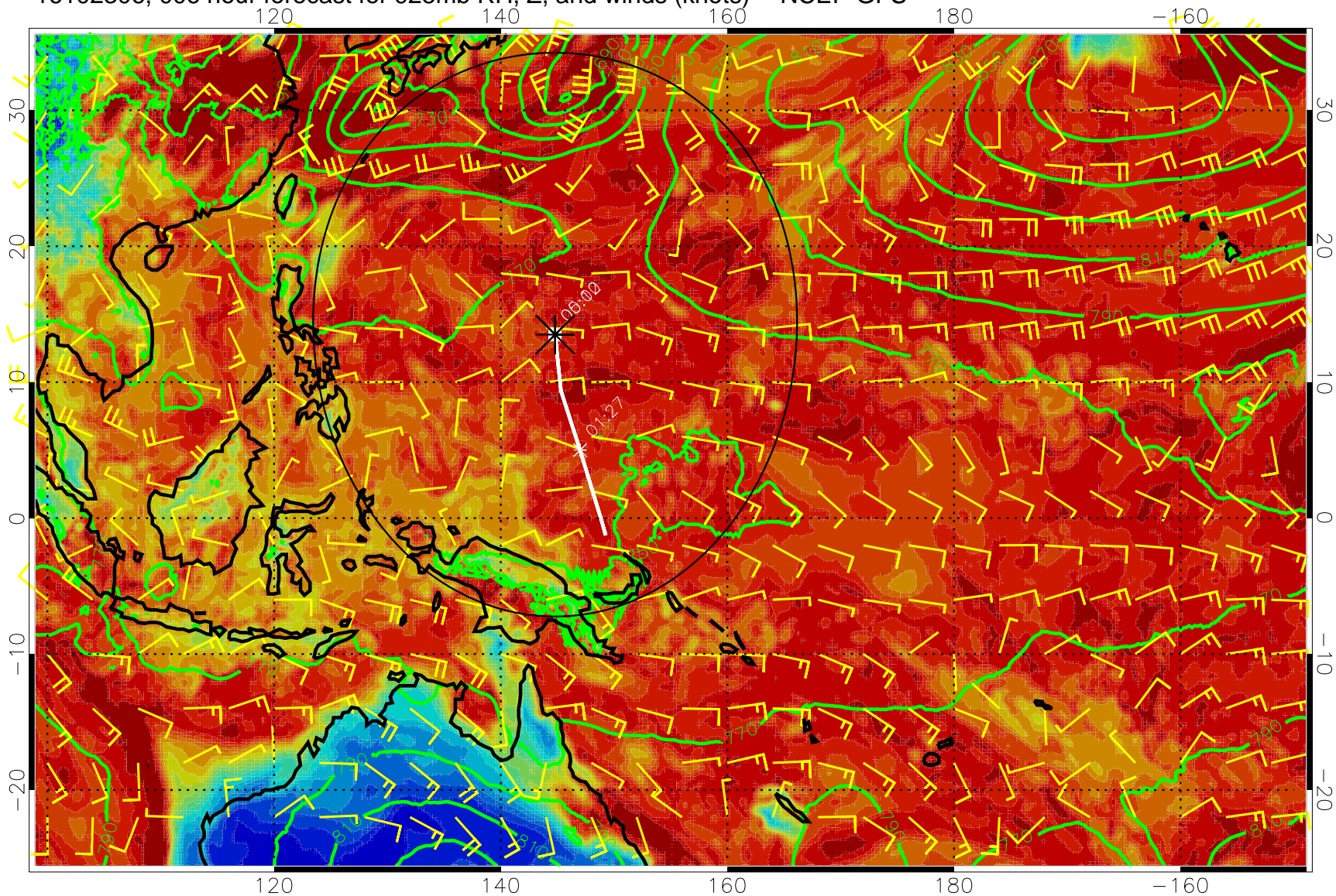
16102306, 006 hour forecast for 925mb RH, Z, and winds (knots) -- NCEP GFS
