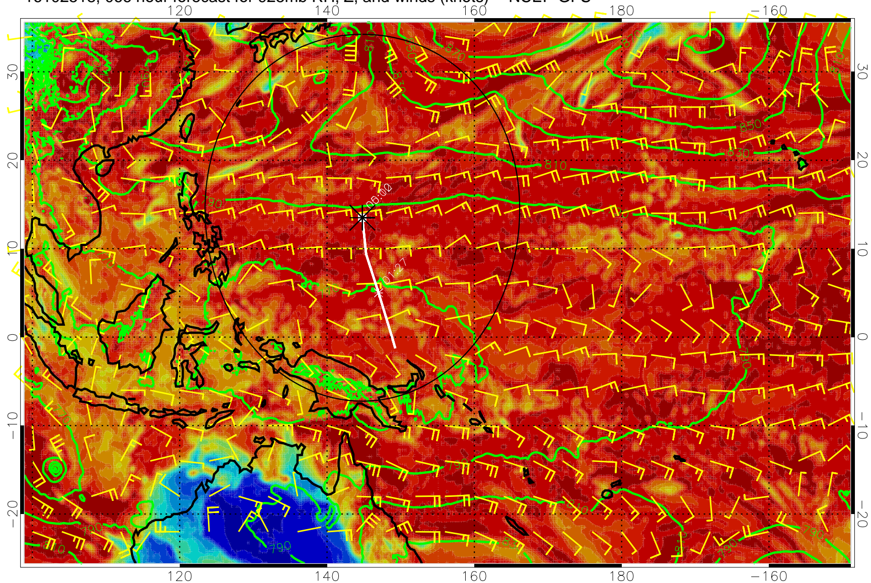
16102518, 066 hour forecast for 925mb RH, Z, and winds (knots) -- NCEP GFS
