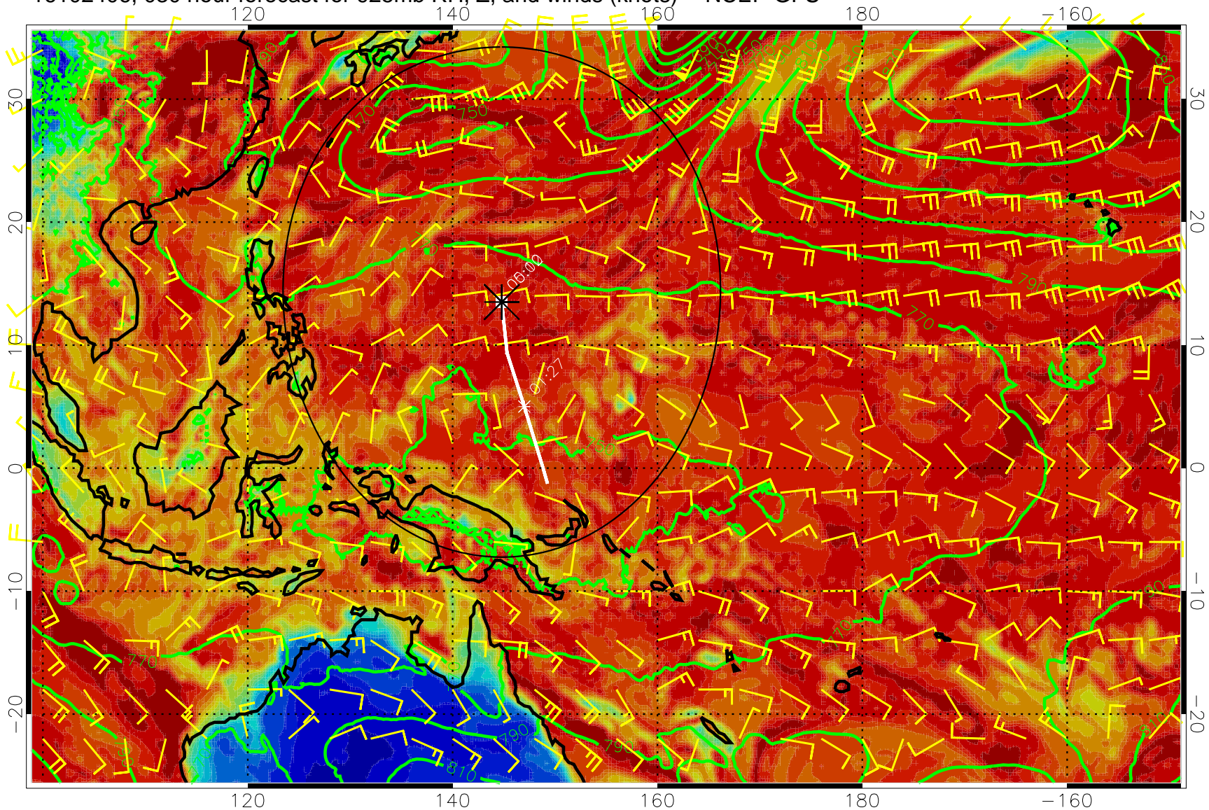
16102406, 030 hour forecast for 925mb RH, Z, and winds (knots) -- NCEP GFS
