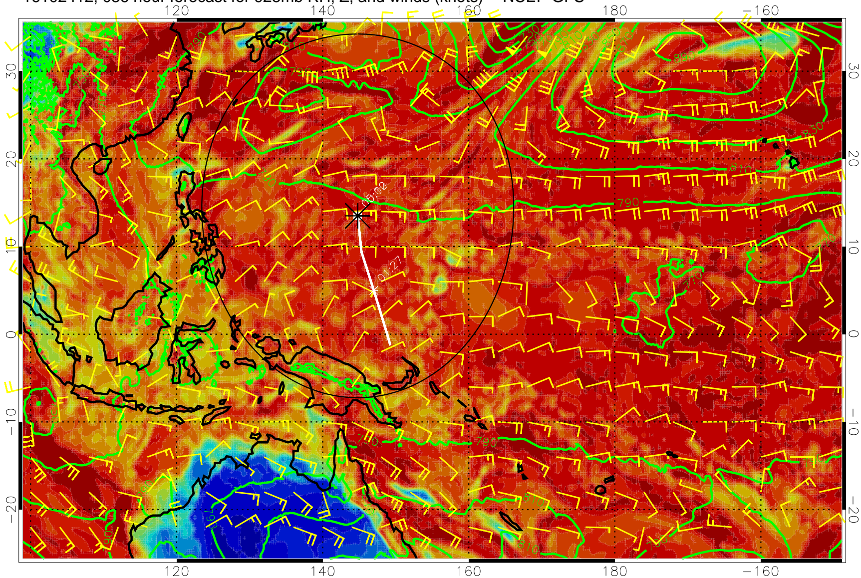
16102412, 036 hour forecast for 925mb RH, Z, and winds (knots) -- NCEP GFS
