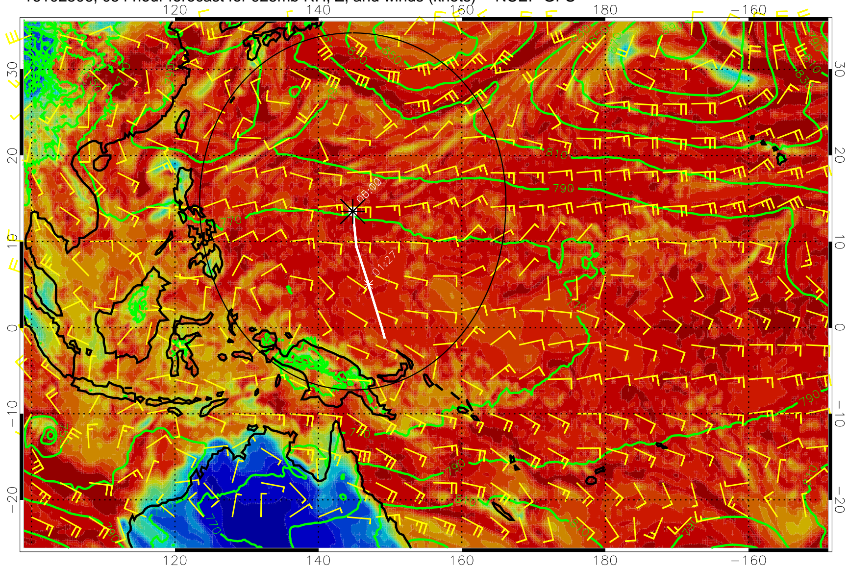
16102506, 054 hour forecast for 925mb RH, Z, and winds (knots) -- NCEP GFS
