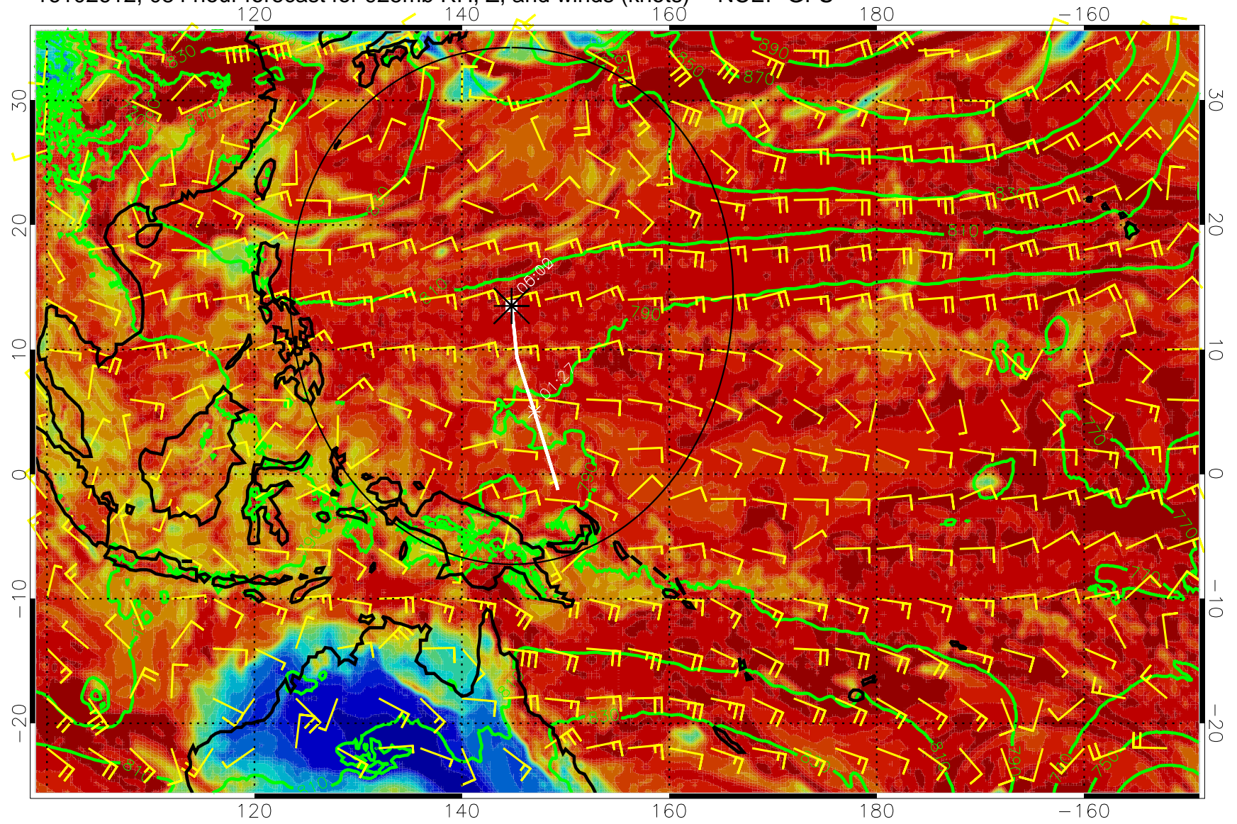
16102612, 084 hour forecast for 925mb RH, Z, and winds (knots) -- NCEP GFS
