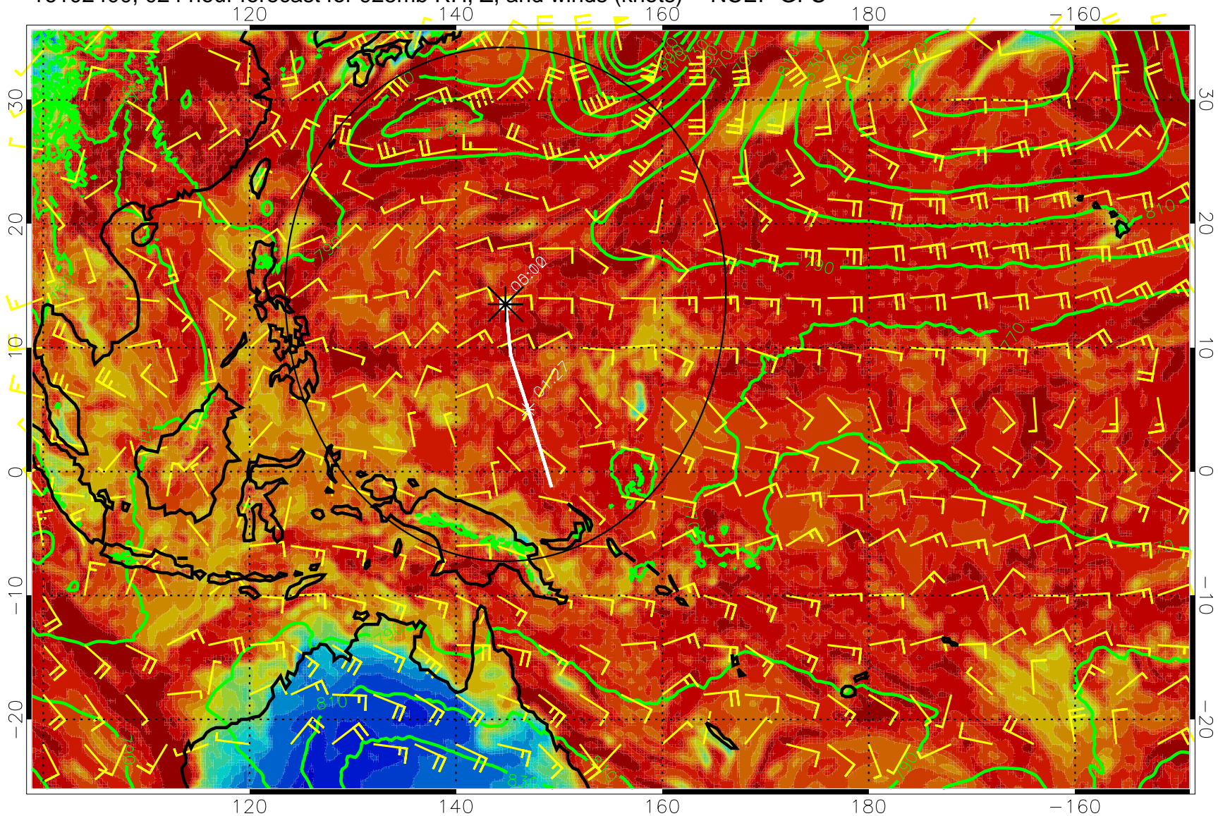
16102400, 024 hour forecast for 925mb RH, Z, and winds (knots) -- NCEP GFS
