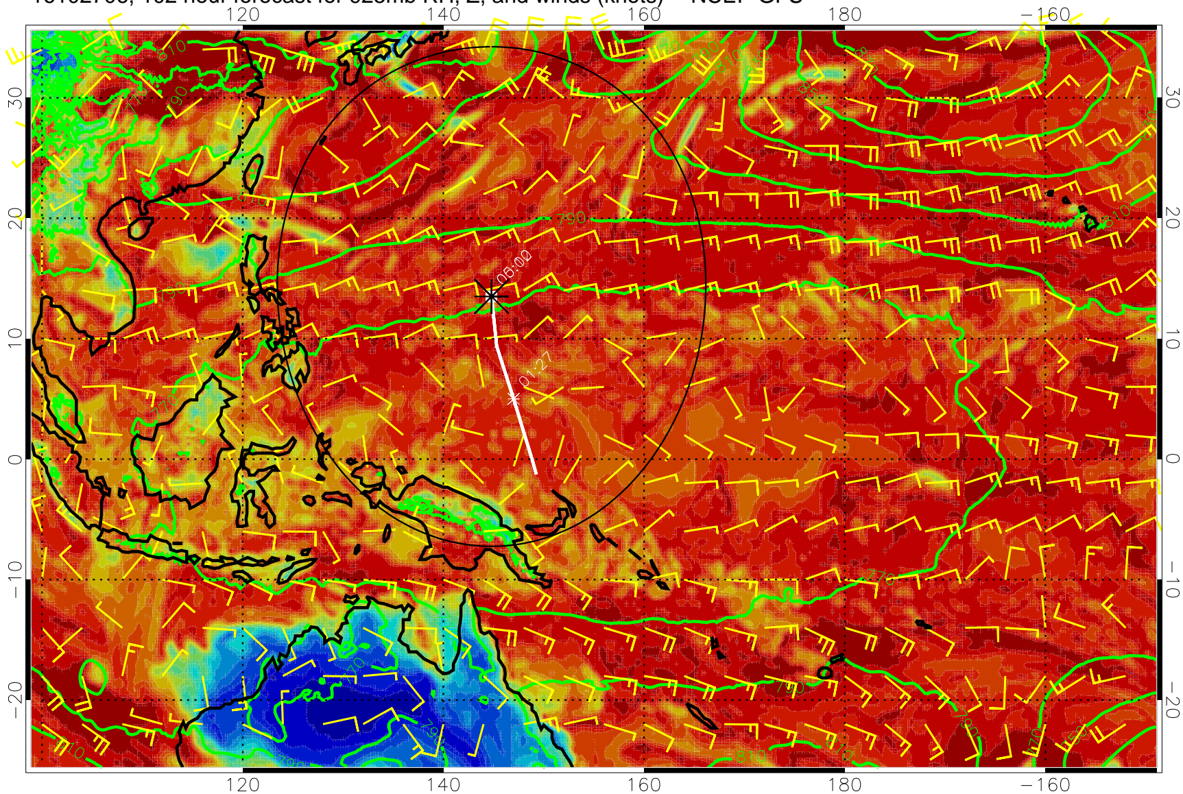
16102706, 102 hour forecast for 925mb RH, Z, and winds (knots) -- NCEP GFS
