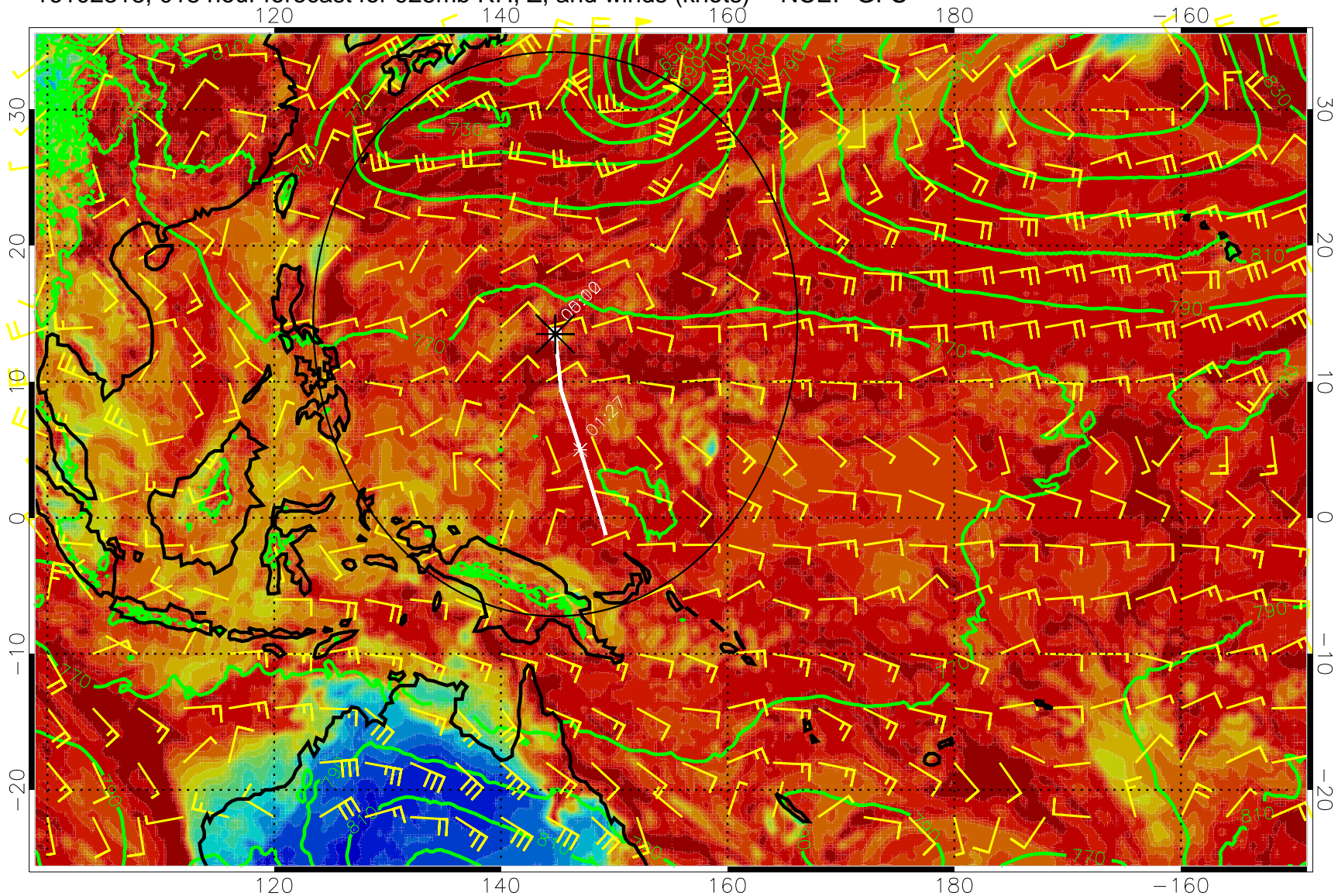
16102318, 018 hour forecast for 925mb RH, Z, and winds (knots) -- NCEP GFS
