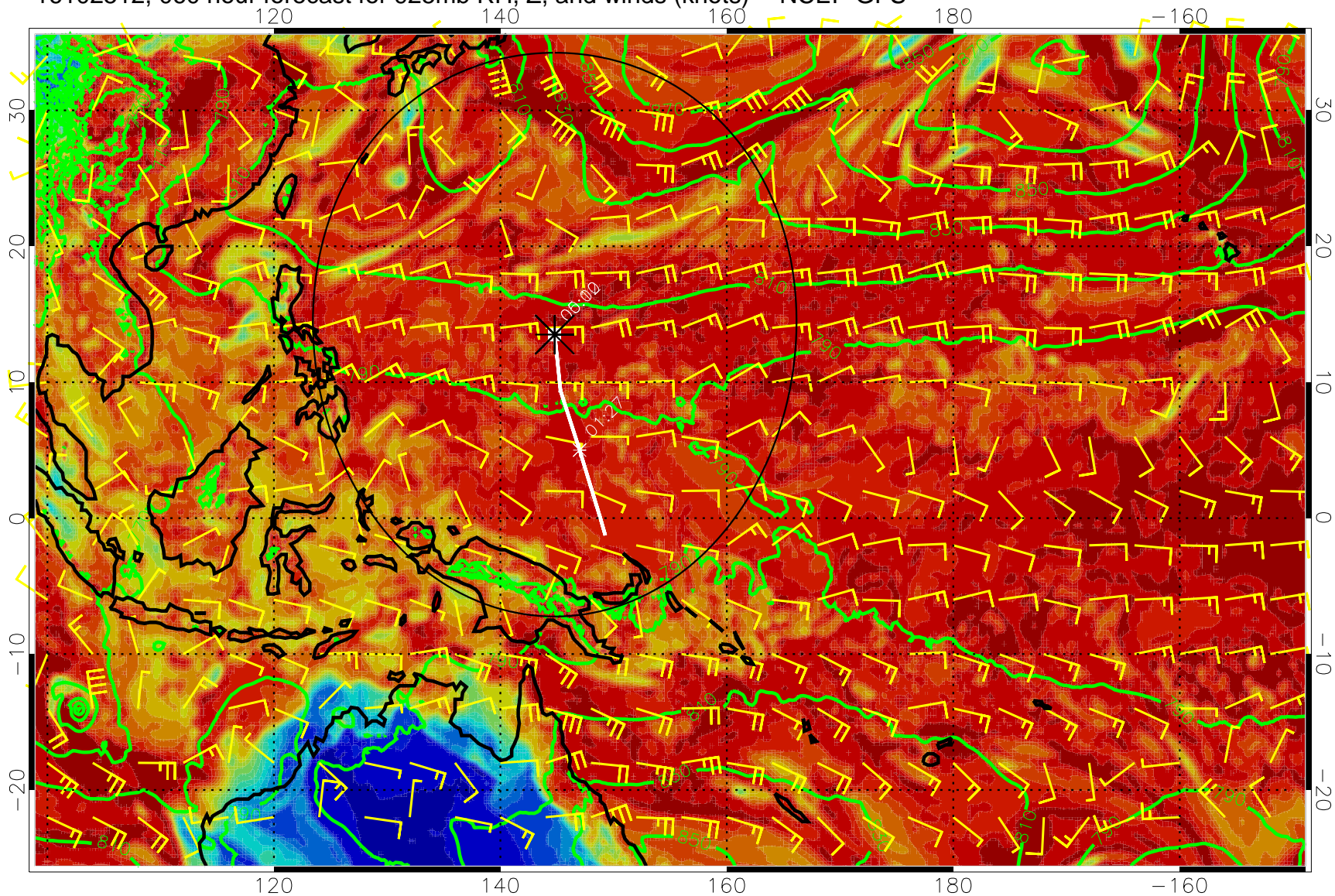
16102512, 060 hour forecast for 925mb RH, Z, and winds (knots) -- NCEP GFS
