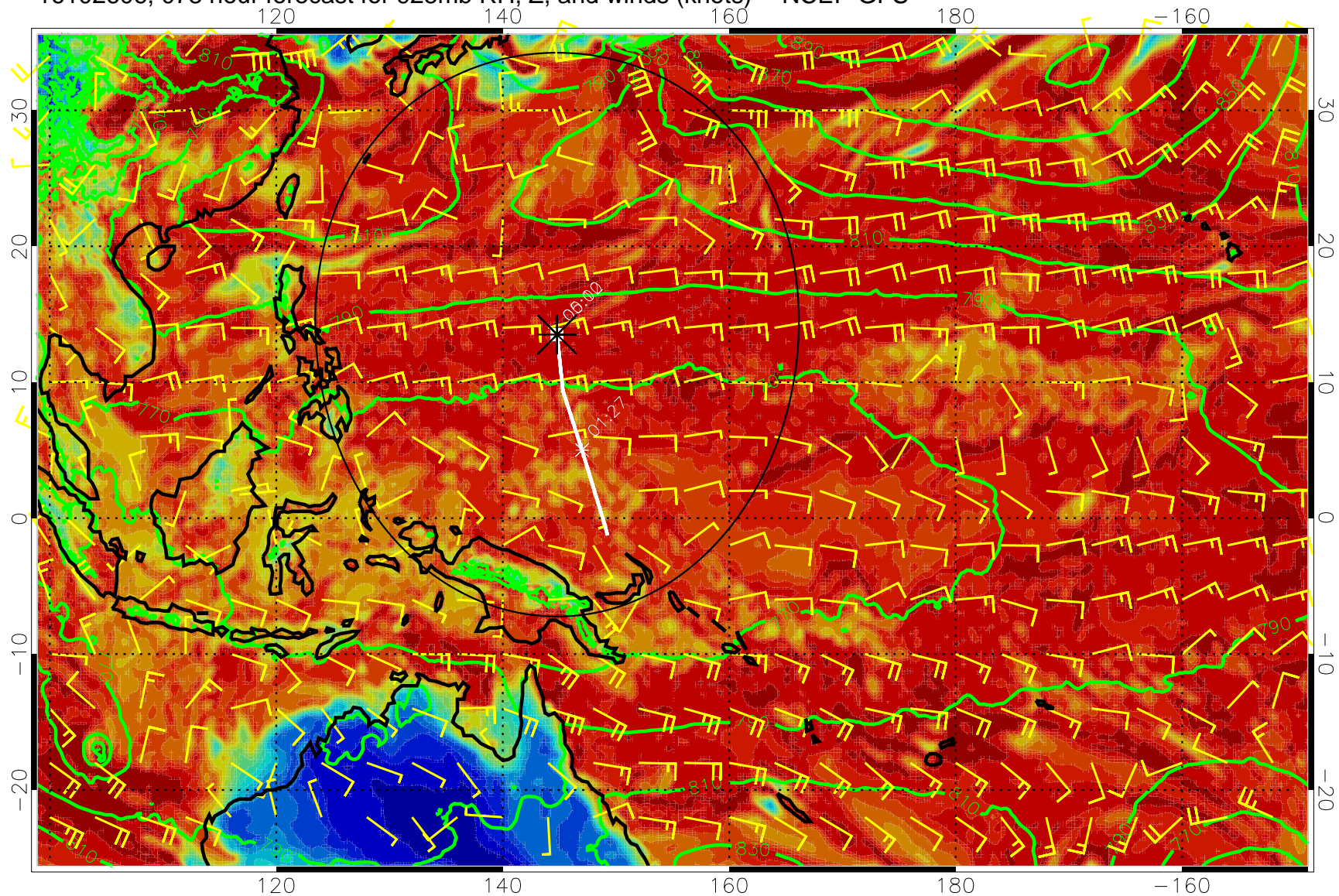
16102606, 078 hour forecast for 925mb RH, Z, and winds (knots) -- NCEP GFS
