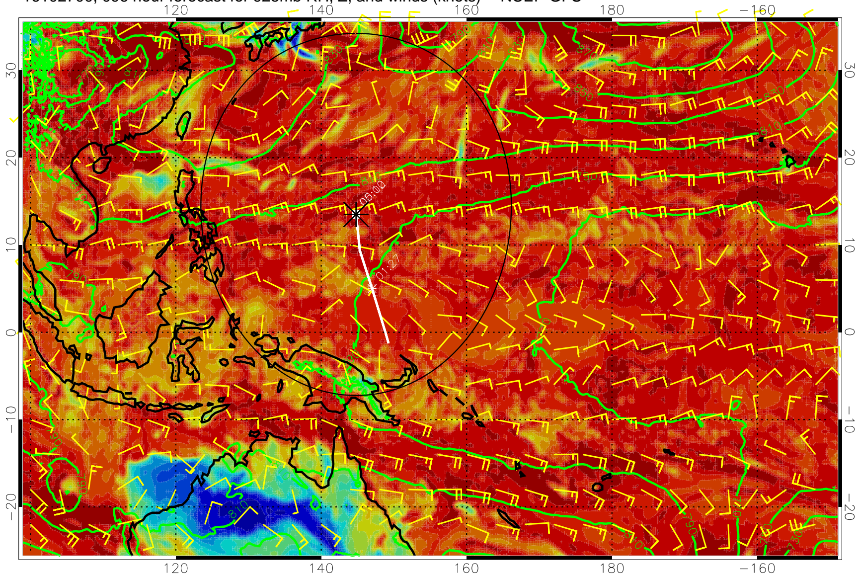
16102700, 096 hour forecast for 925mb RH, Z, and winds (knots) -- NCEP GFS
