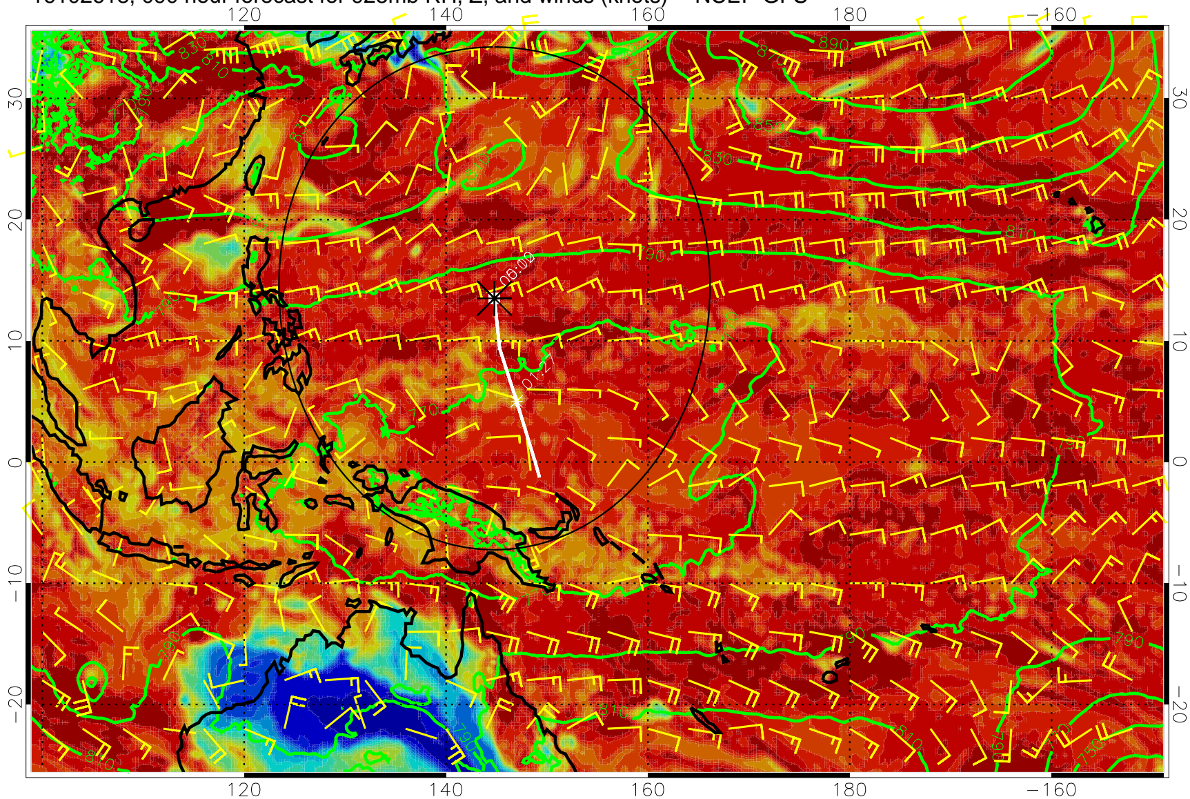
16102618, 090 hour forecast for 925mb RH, Z, and winds (knots) -- NCEP GFS
