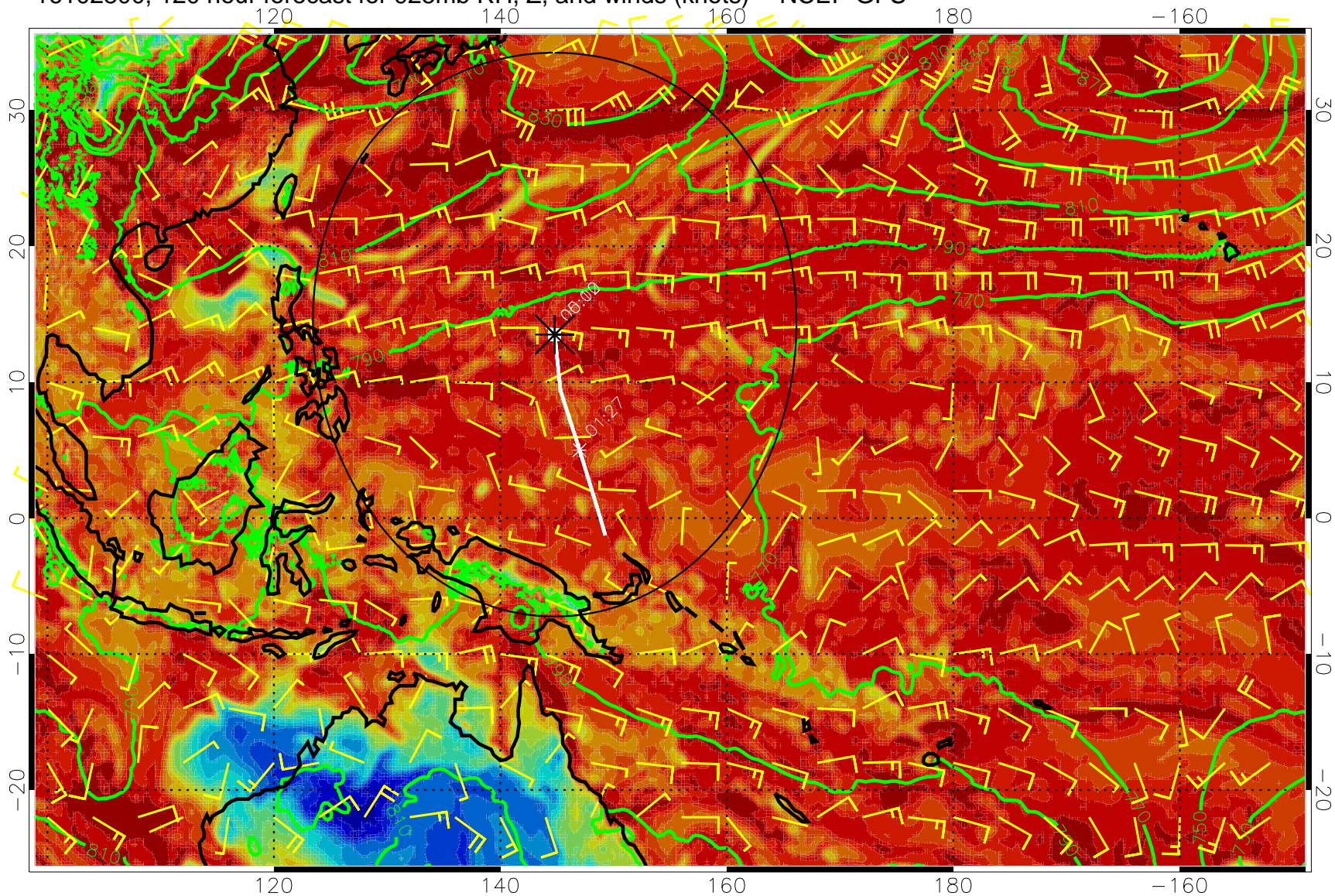
16102800, 120 hour forecast for 925mb RH, Z, and winds (knots) -- NCEP GFS
