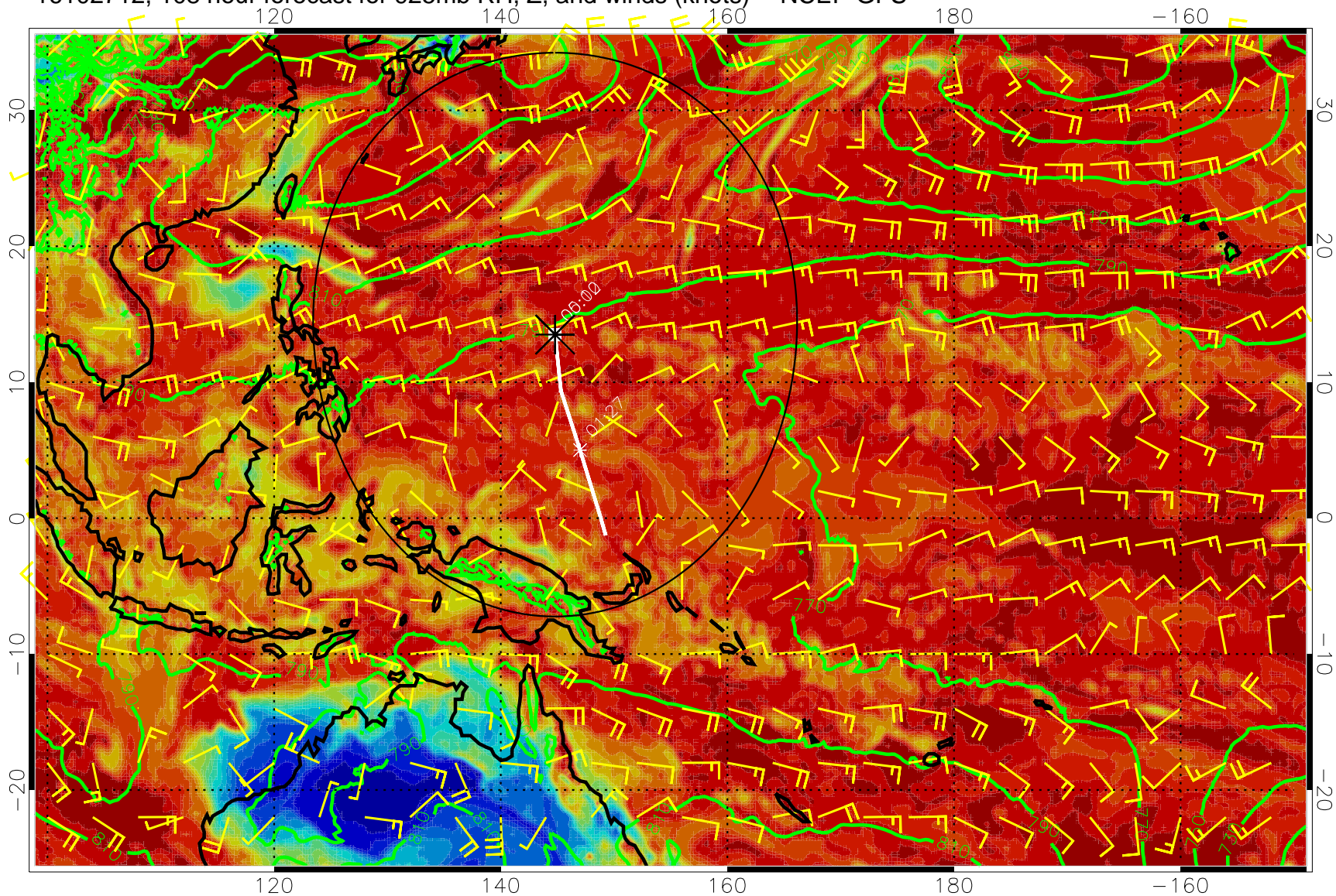
16102712, 108 hour forecast for 925mb RH, Z, and winds (knots) -- NCEP GFS
