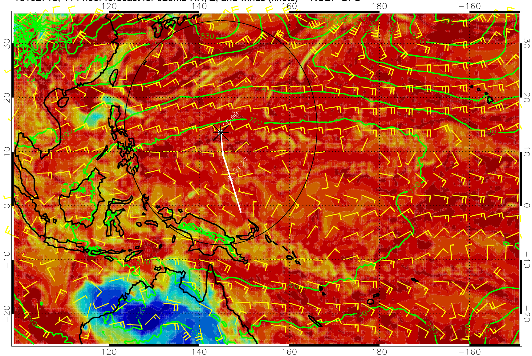
16102718, 114 hour forecast for 925mb RH, Z, and winds (knots) -- NCEP GFS
