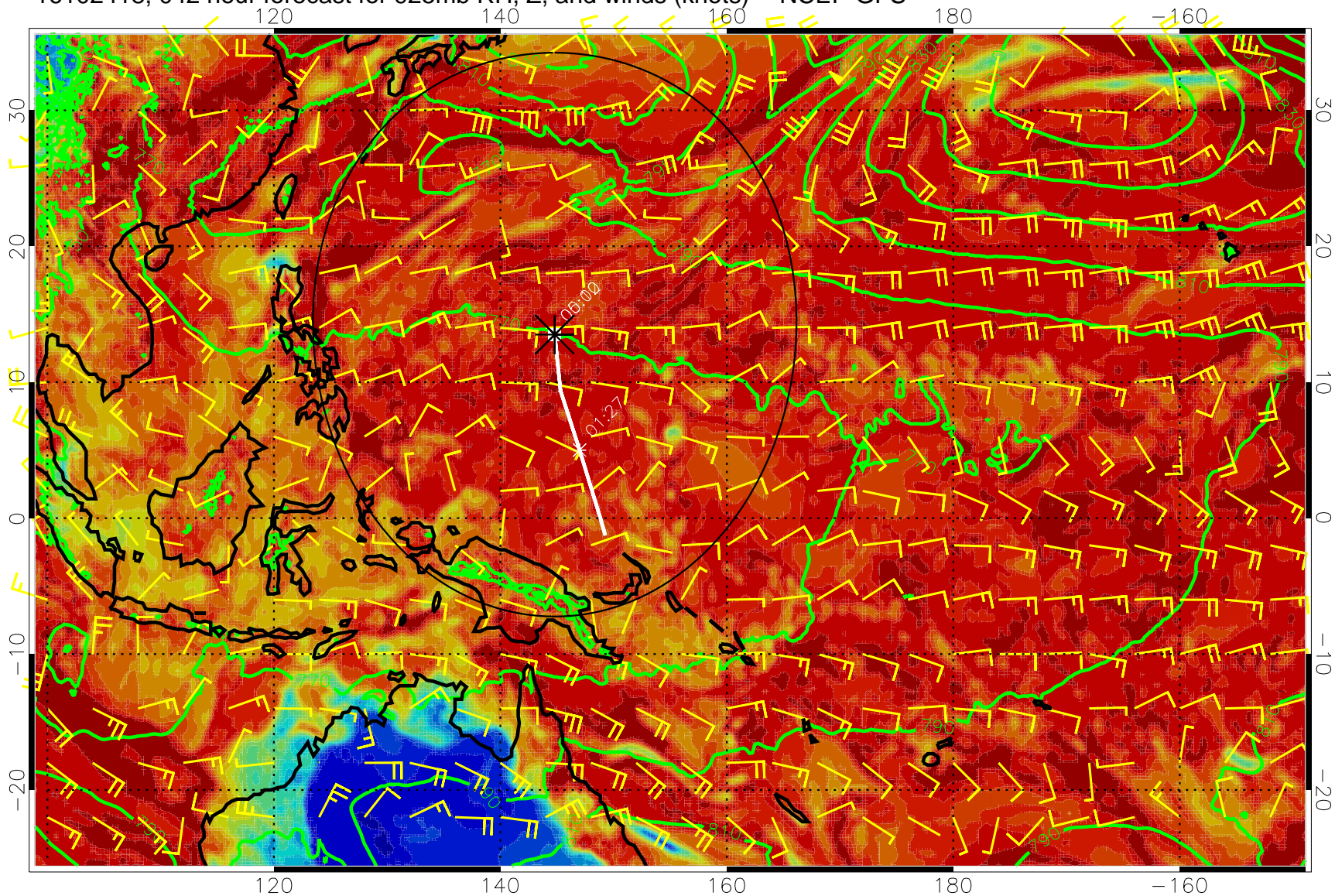
16102418, 042 hour forecast for 925mb RH, Z, and winds (knots) -- NCEP GFS
