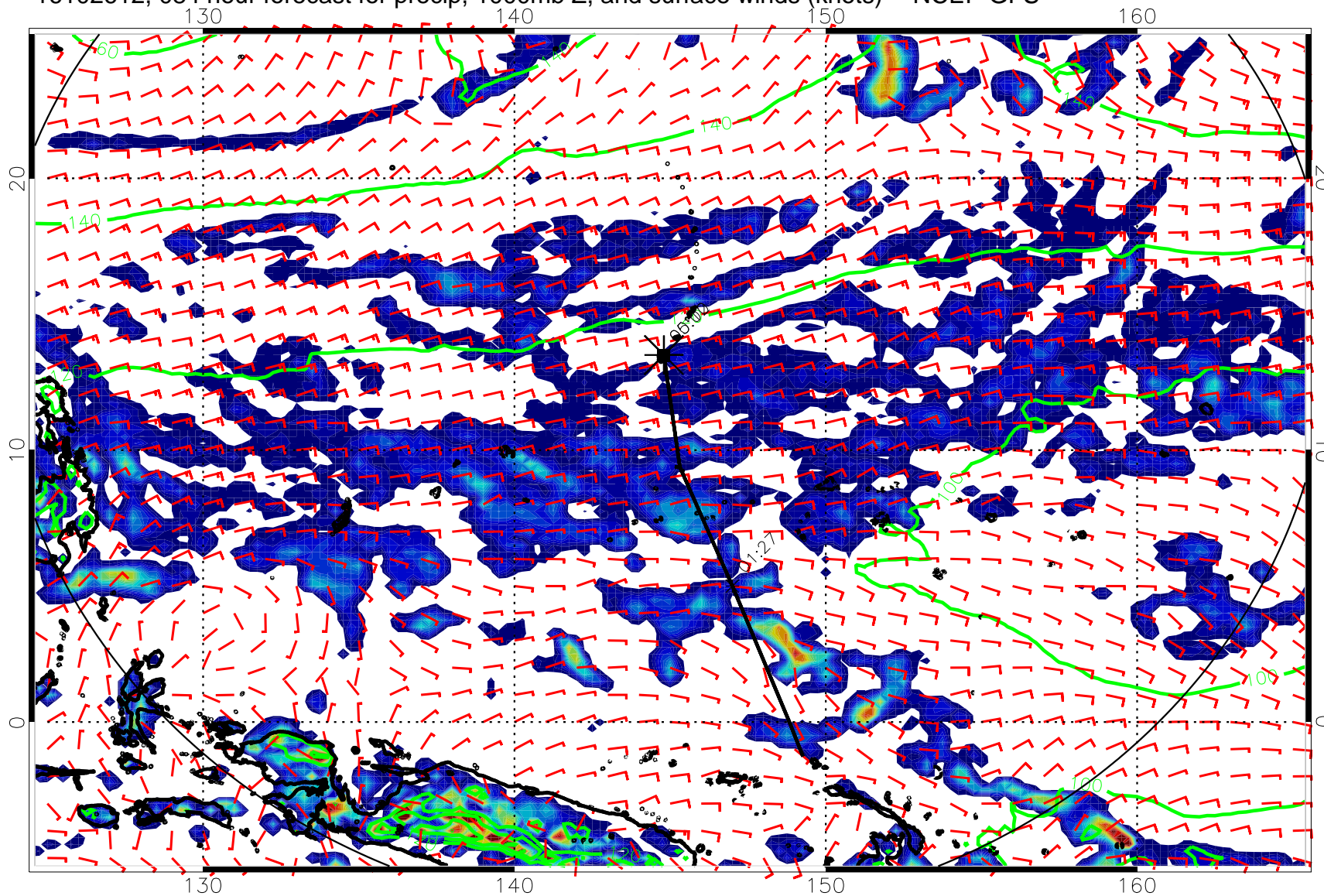
16102612, 084 hour forecast for precip, 1000mb Z, and surface winds (knots) -- NCEP GFS
