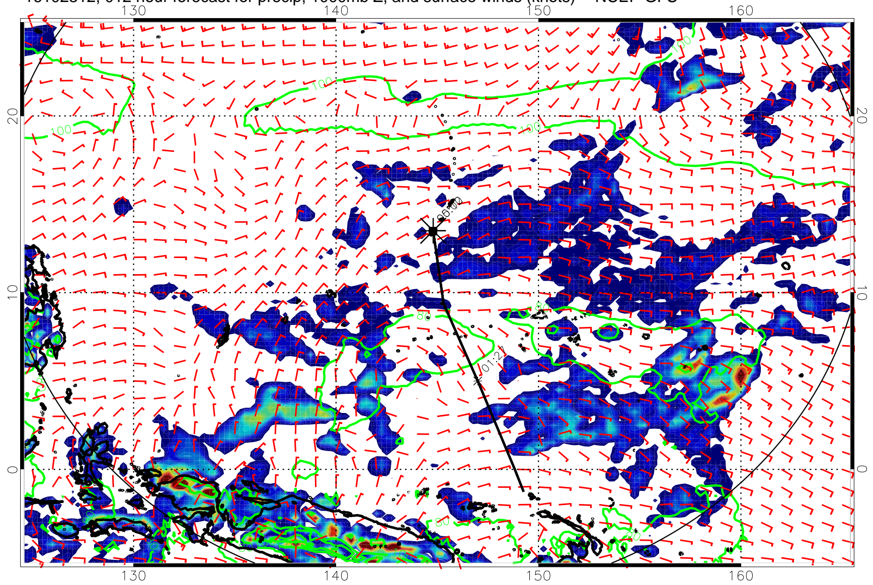
16102312, 012 hour forecast for precip, 1000mb Z, and surface winds (knots) -- NCEP GFS
