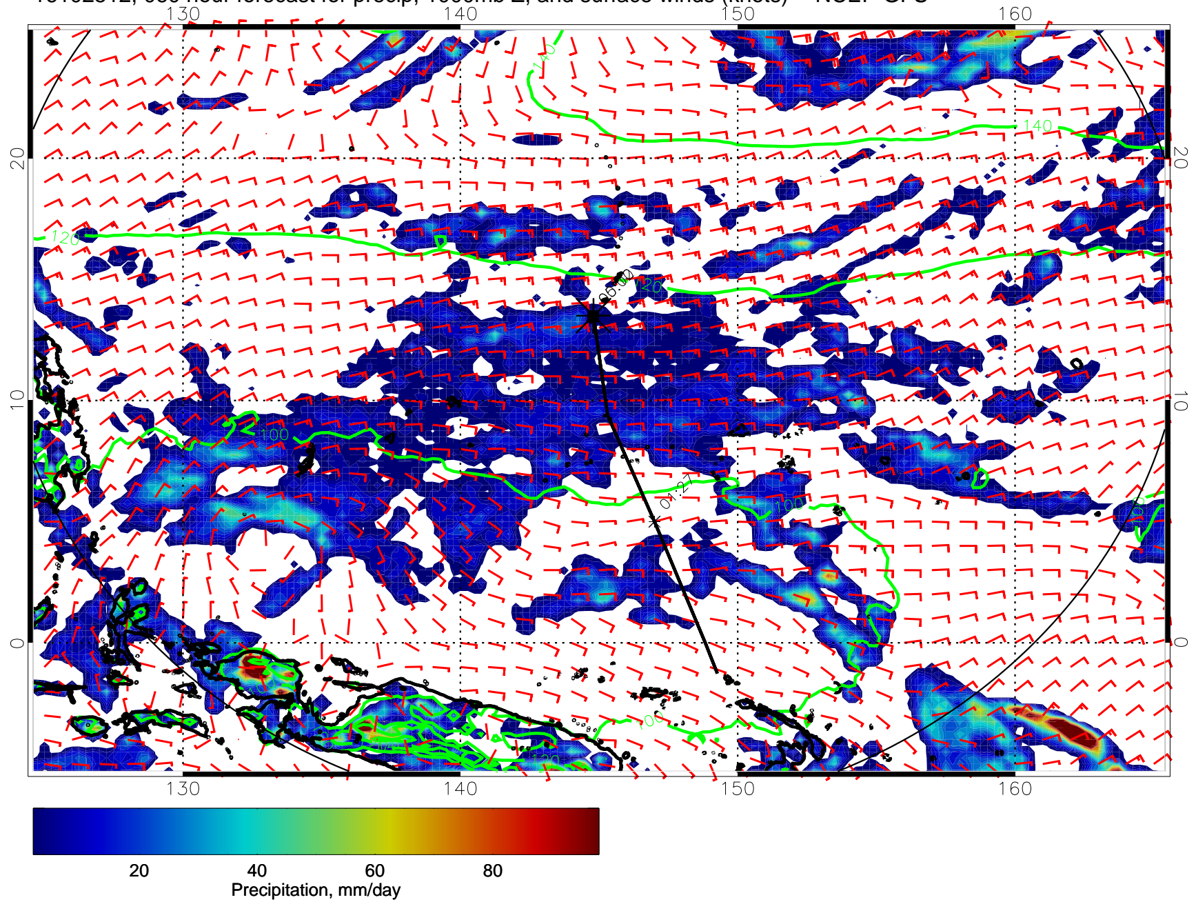
16102512, 060 hour forecast for precip, 1000mb Z, and surface winds (knots) -- NCEP GFS
