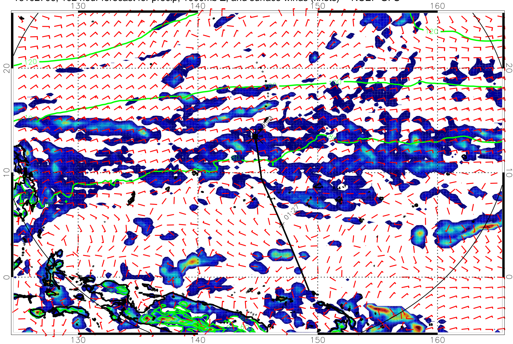
16102706, 102 hour forecast for precip, 1000mb Z, and surface winds (knots) -- NCEP GFS
