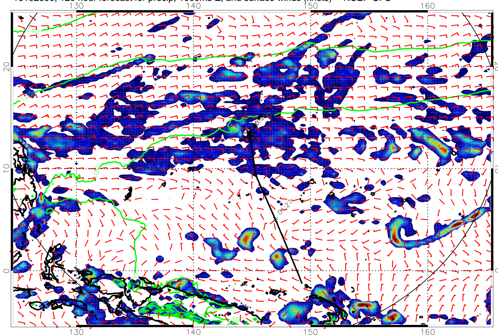
16102800, 120 hour forecast for precip, 1000mb Z, and surface winds (knots) -- NCEP GFS
