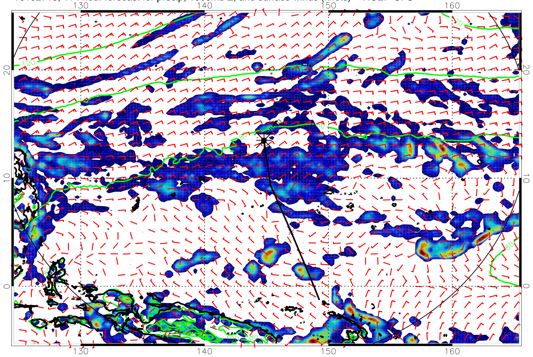
16102718, 114 hour forecast for precip, 1000mb Z, and surface winds (knots) -- NCEP GFS
