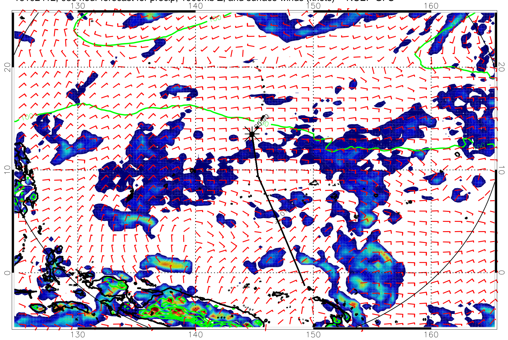
16102412, 036 hour forecast for precip, 1000mb Z, and surface winds (knots) -- NCEP GFS
