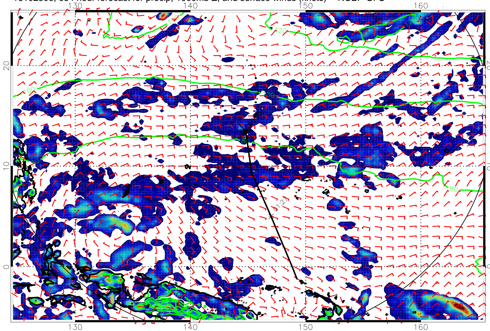
16102506, 054 hour forecast for precip, 1000mb Z, and surface winds (knots) -- NCEP GFS
