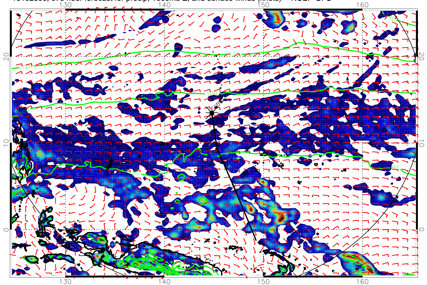
16102606, 078 hour forecast for precip, 1000mb Z, and surface winds (knots) -- NCEP GFS
