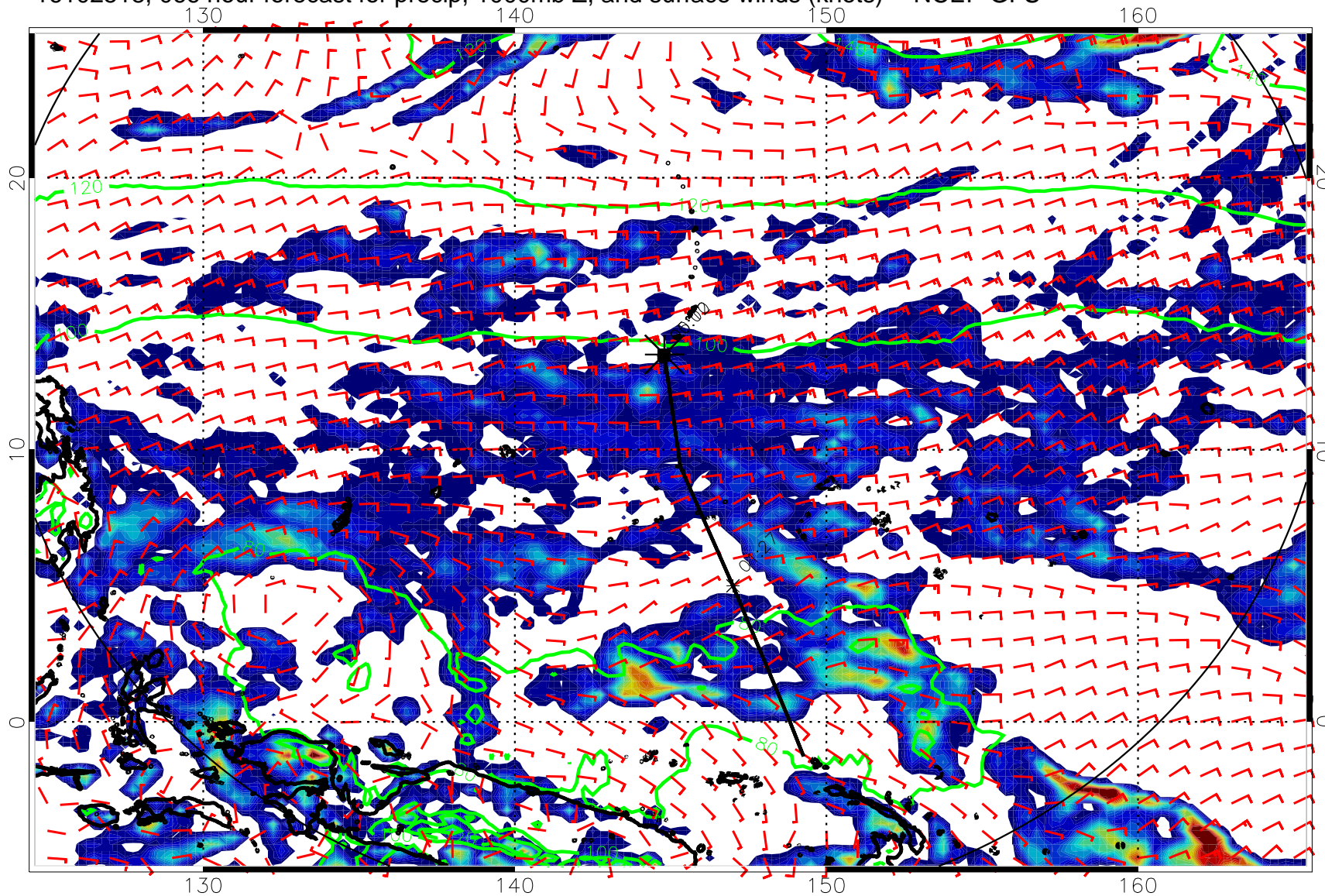
16102518, 066 hour forecast for precip, 1000mb Z, and surface winds (knots) -- NCEP GFS
