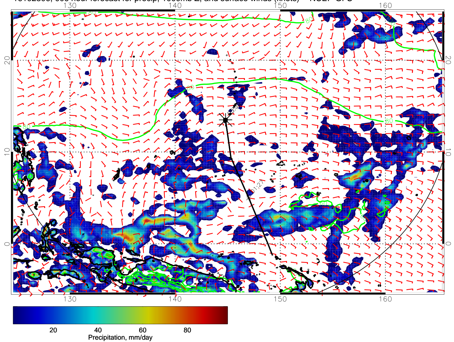
16102306, 006 hour forecast for precip, 1000mb Z, and surface winds (knots) -- NCEP GFS
