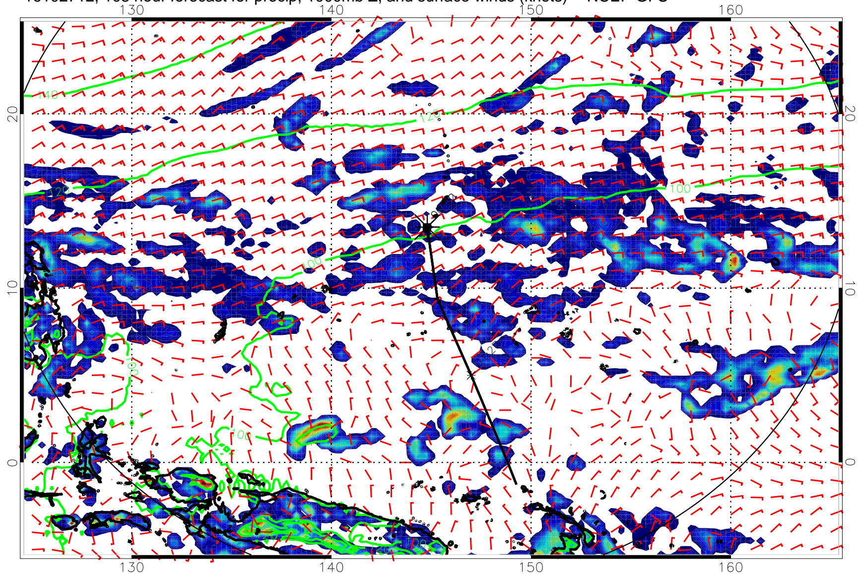
16102712, 108 hour forecast for precip, 1000mb Z, and surface winds (knots) -- NCEP GFS
