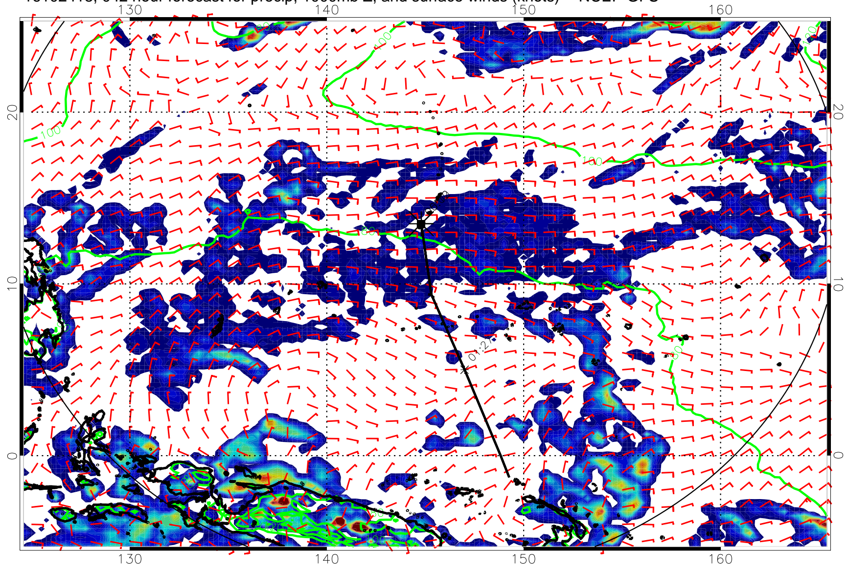
16102418, 042 hour forecast for precip, 1000mb Z, and surface winds (knots) -- NCEP GFS
