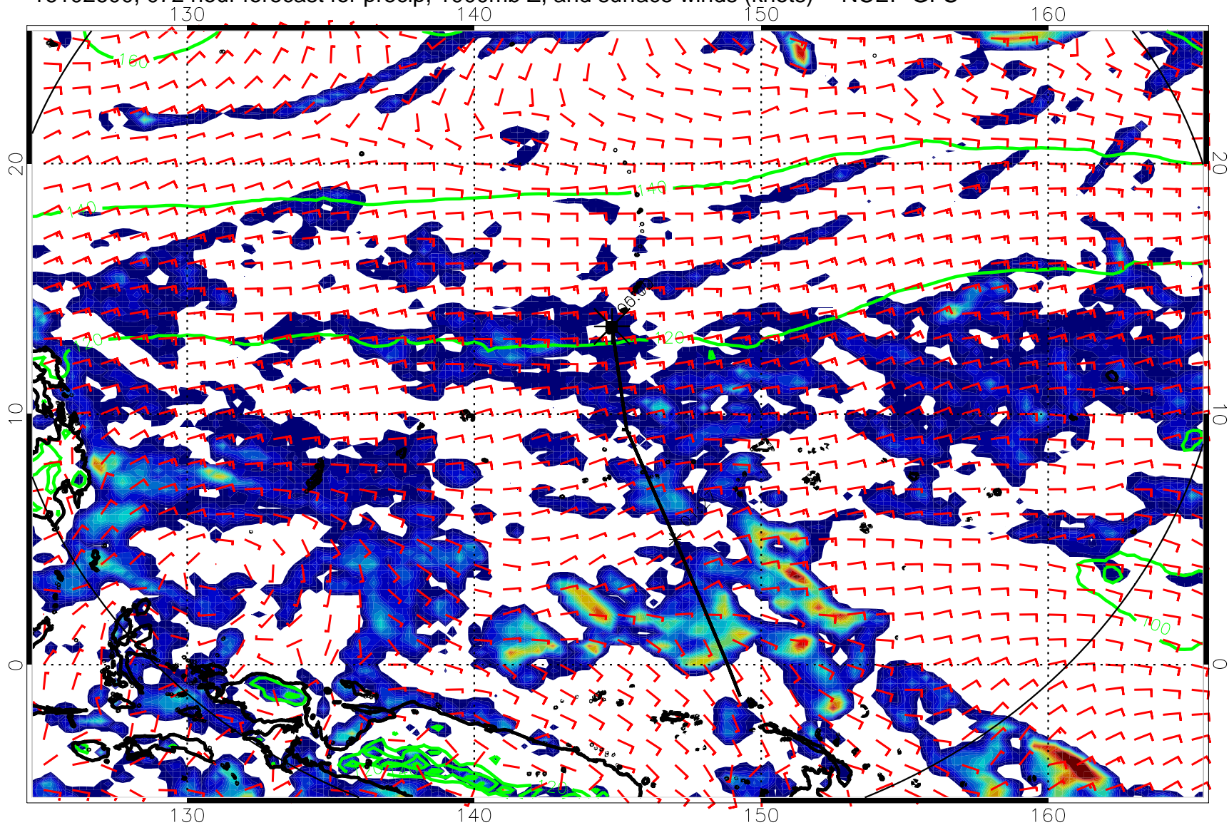
16102600, 072 hour forecast for precip, 1000mb Z, and surface winds (knots) -- NCEP GFS
