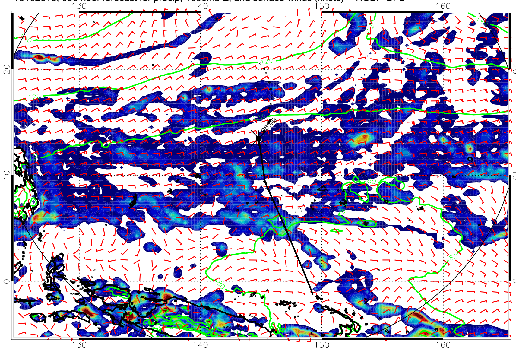
16102618, 090 hour forecast for precip, 1000mb Z, and surface winds (knots) -- NCEP GFS
