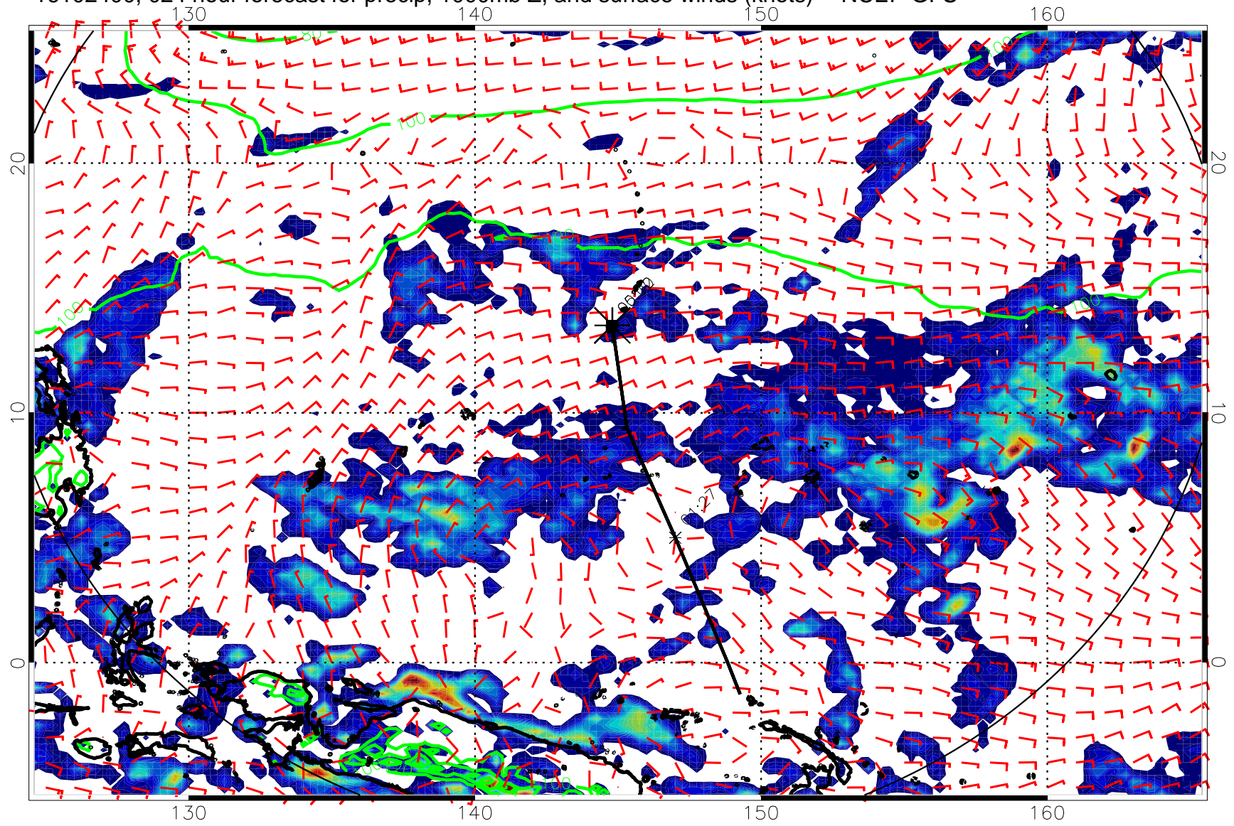
16102400, 024 hour forecast for precip, 1000mb Z, and surface winds (knots) -- NCEP GFS
