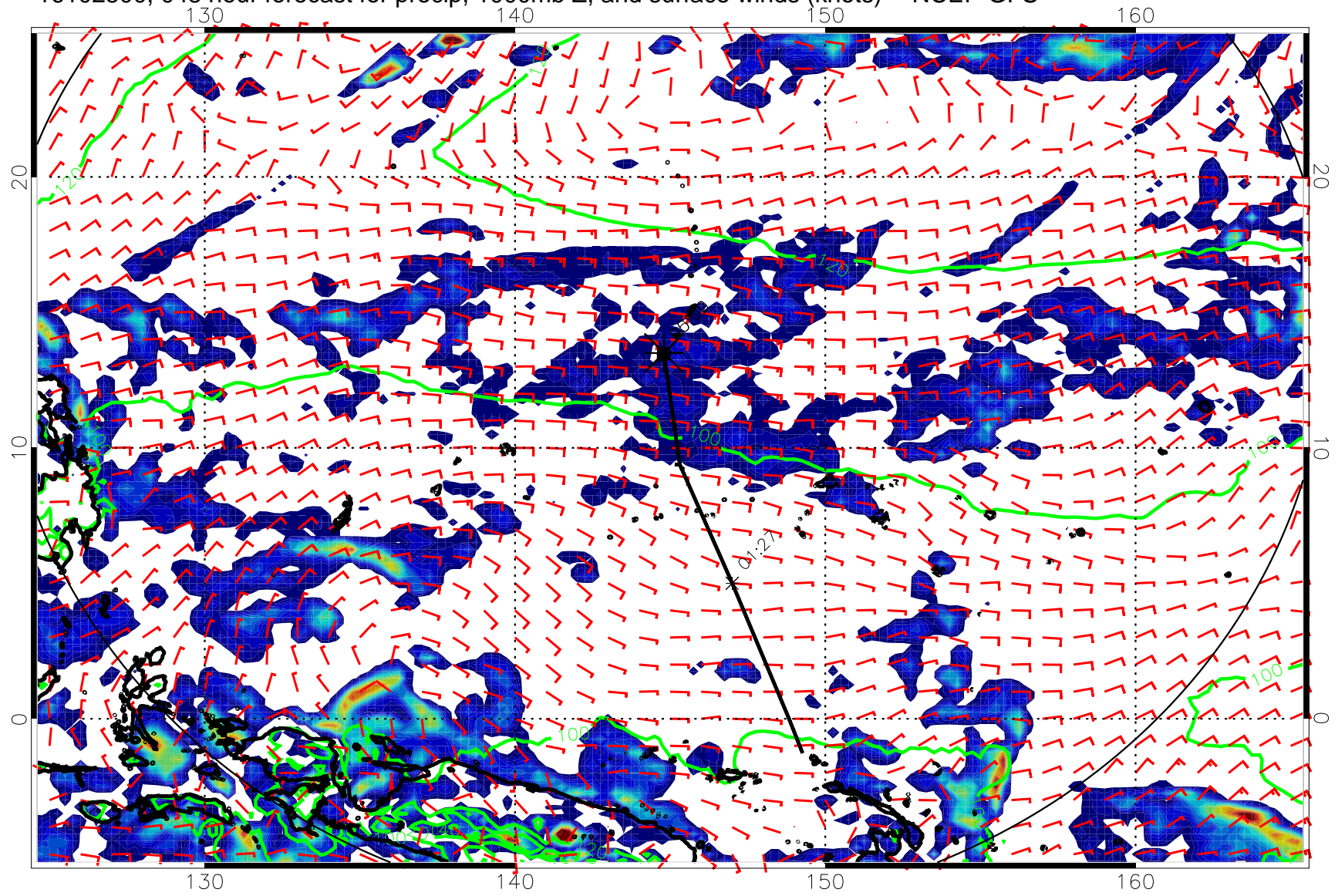
16102500, 048 hour forecast for precip, 1000mb Z, and surface winds (knots) -- NCEP GFS
