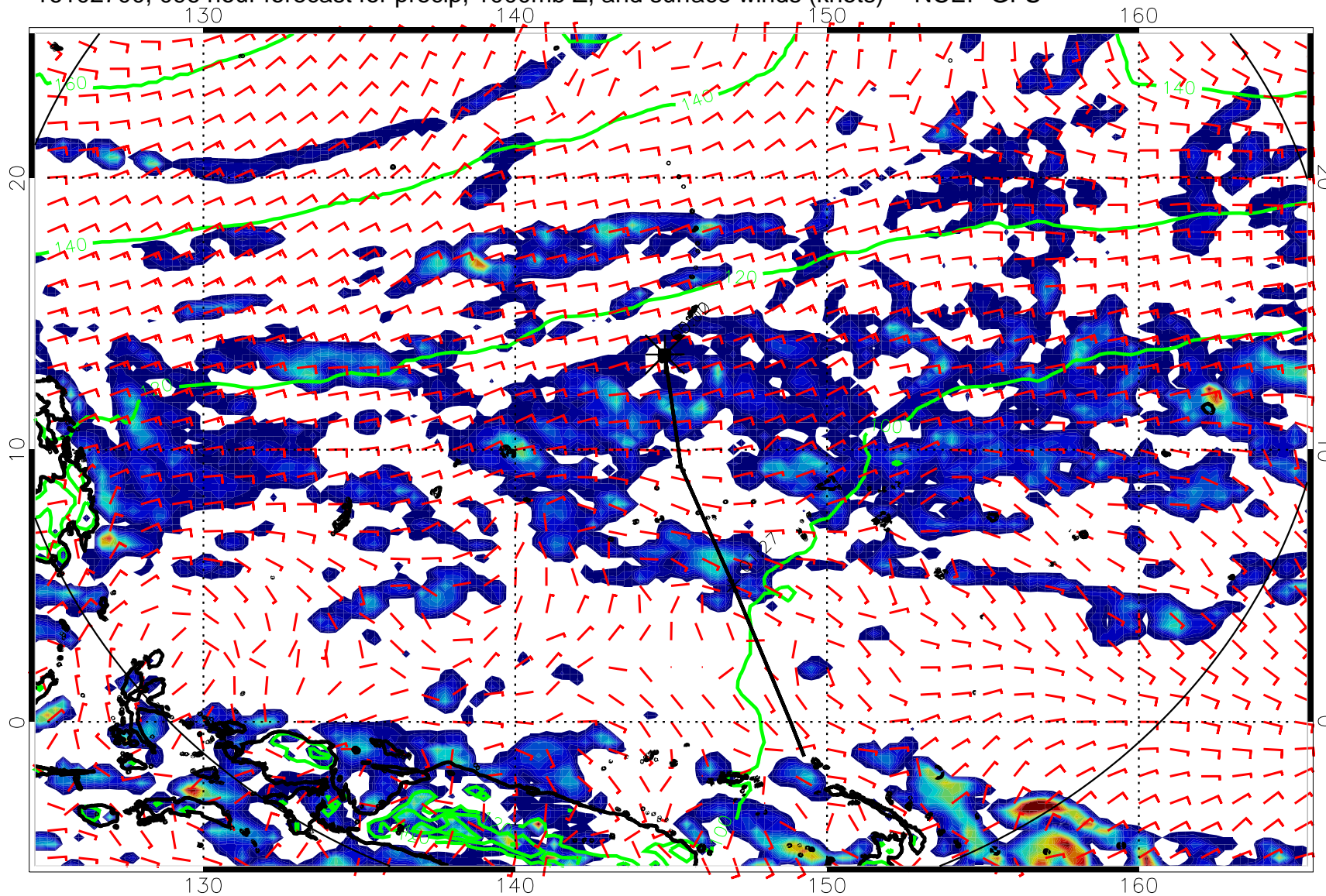
16102700, 096 hour forecast for precip, 1000mb Z, and surface winds (knots) -- NCEP GFS
