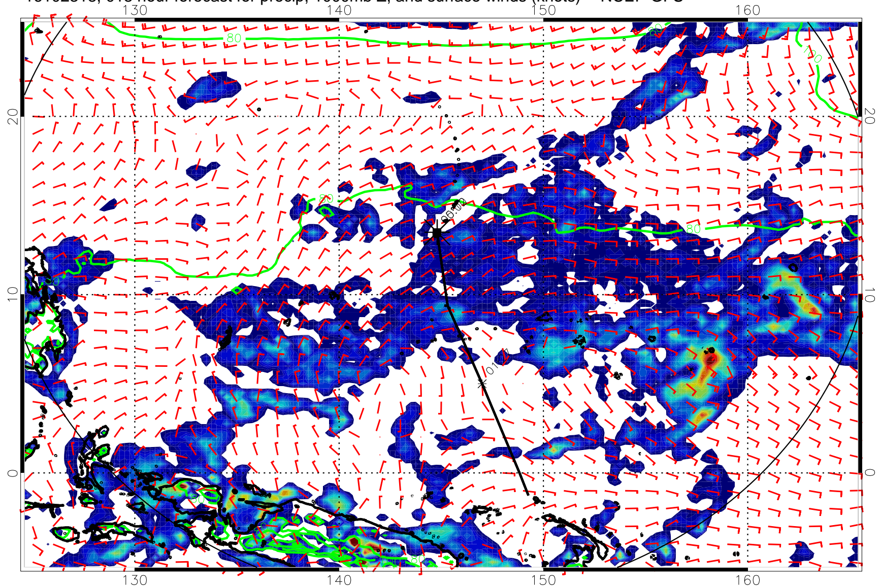
16102318, 018 hour forecast for precip, 1000mb Z, and surface winds (knots) -- NCEP GFS
