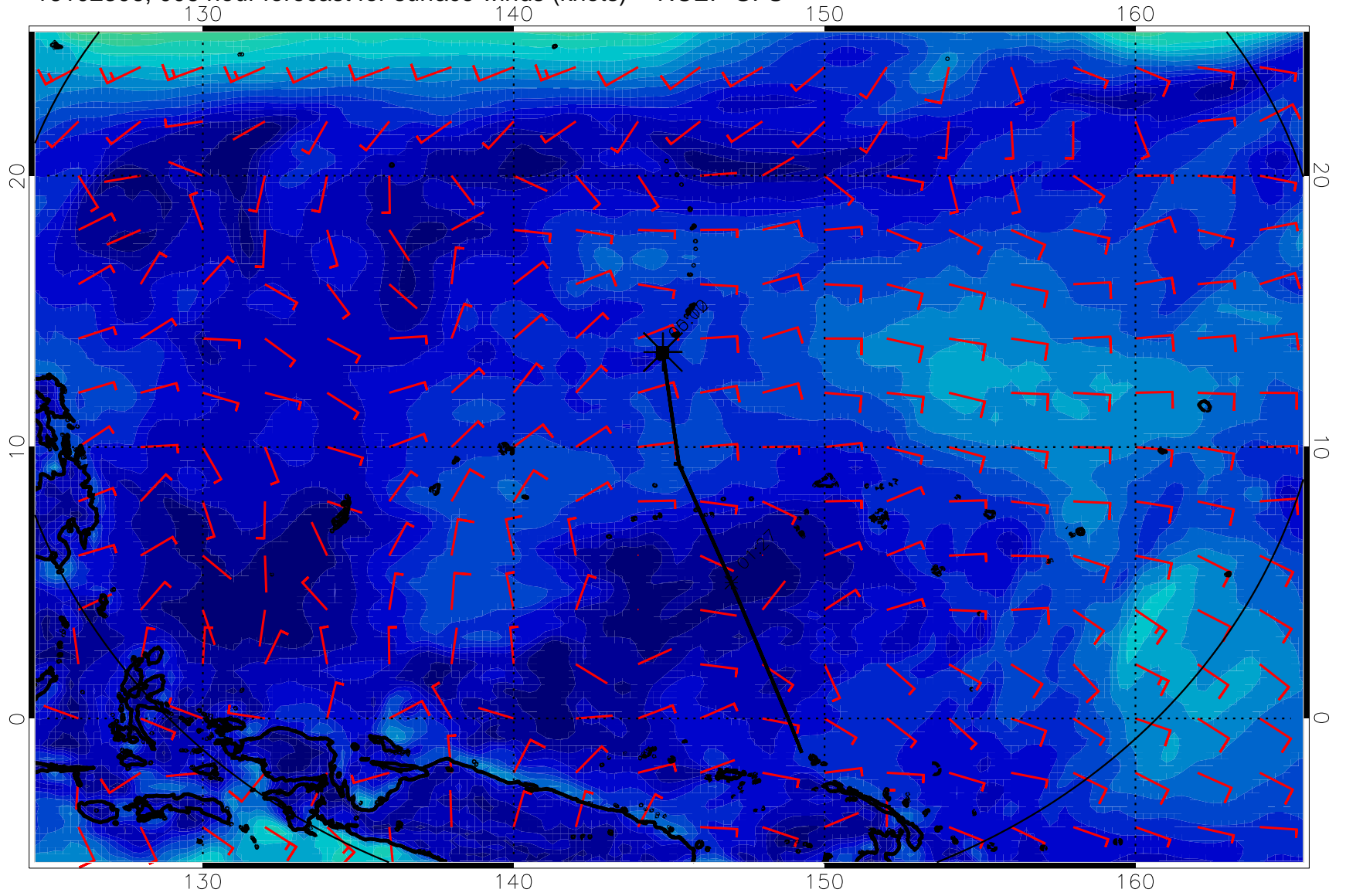
16102306, 006 hour forecast for surface winds (knots) -- NCEP GFS
