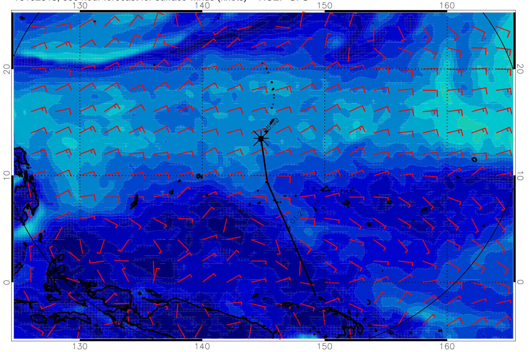
16102618, 090 hour forecast for surface winds (knots) -- NCEP GFS
