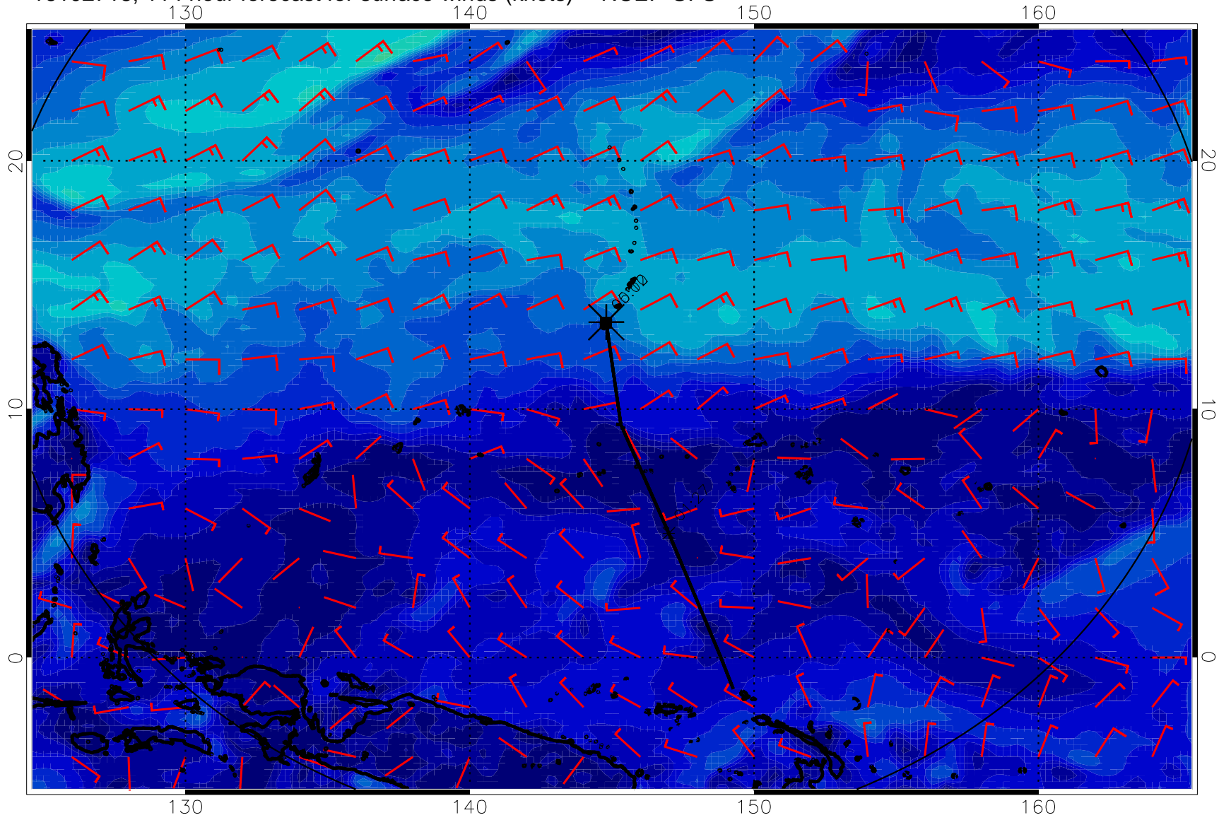
16102718, 114 hour forecast for surface winds (knots) -- NCEP GFS
