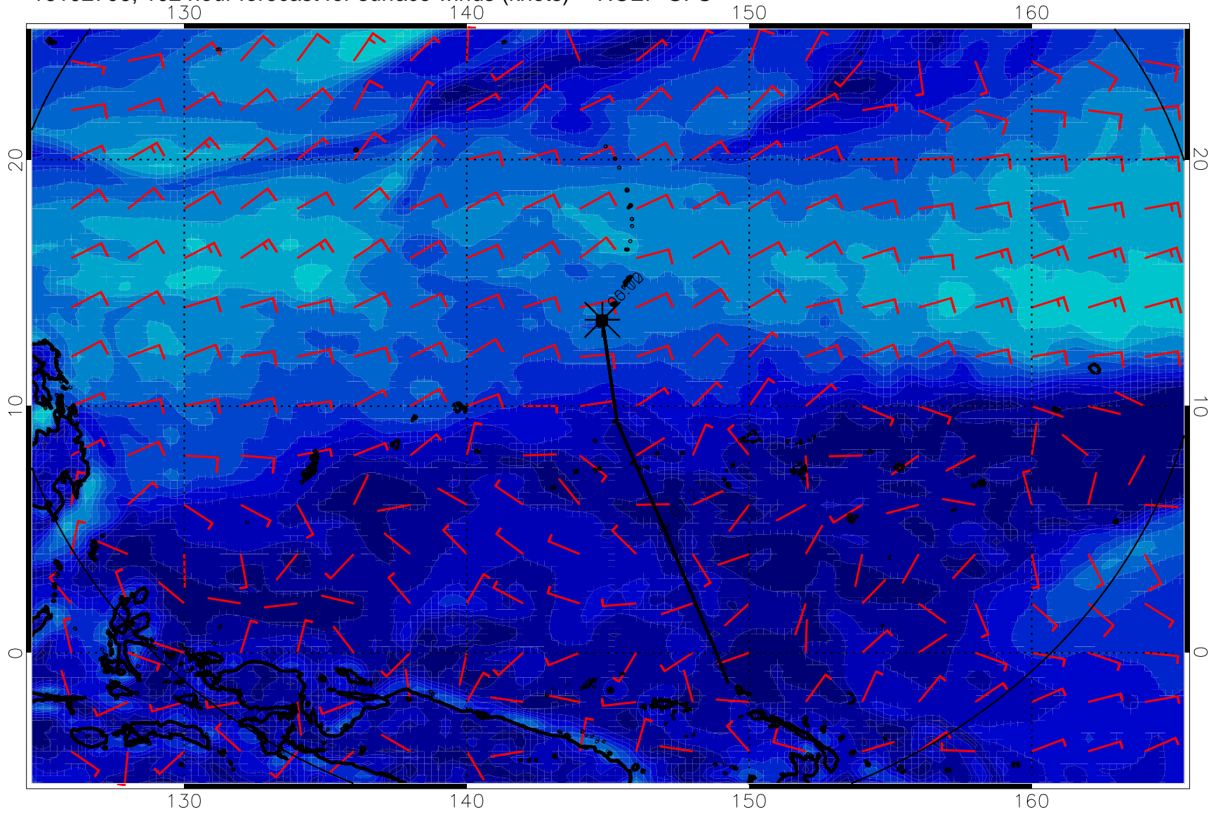
16102706, 102 hour forecast for surface winds (knots) -- NCEP GFS
