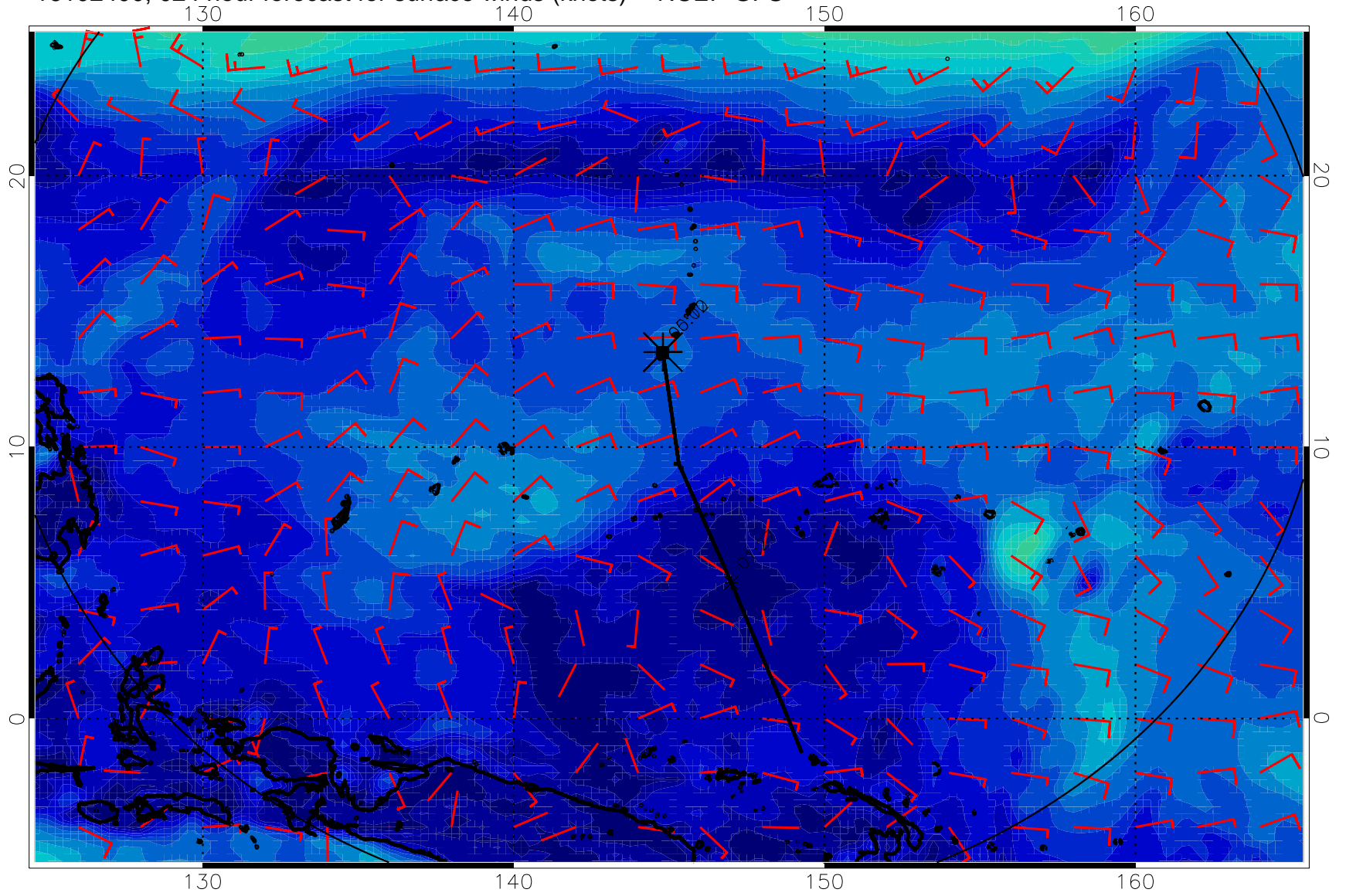
16102400, 024 hour forecast for surface winds (knots) -- NCEP GFS
