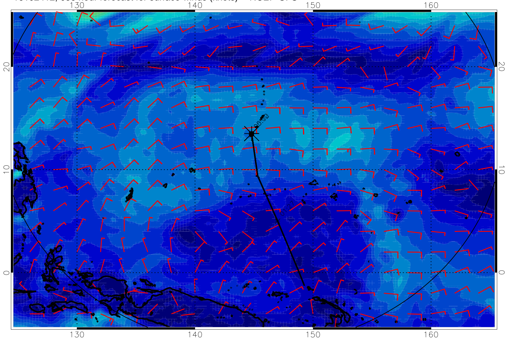
16102412, 036 hour forecast for surface winds (knots) -- NCEP GFS
