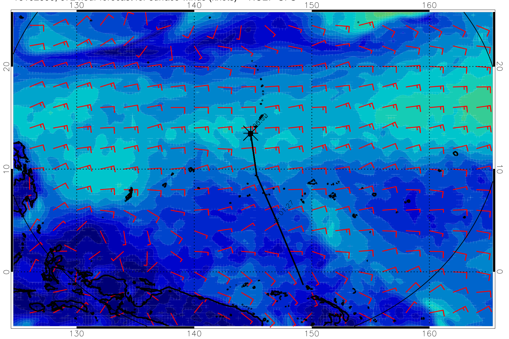
16102600, 072 hour forecast for surface winds (knots) -- NCEP GFS
