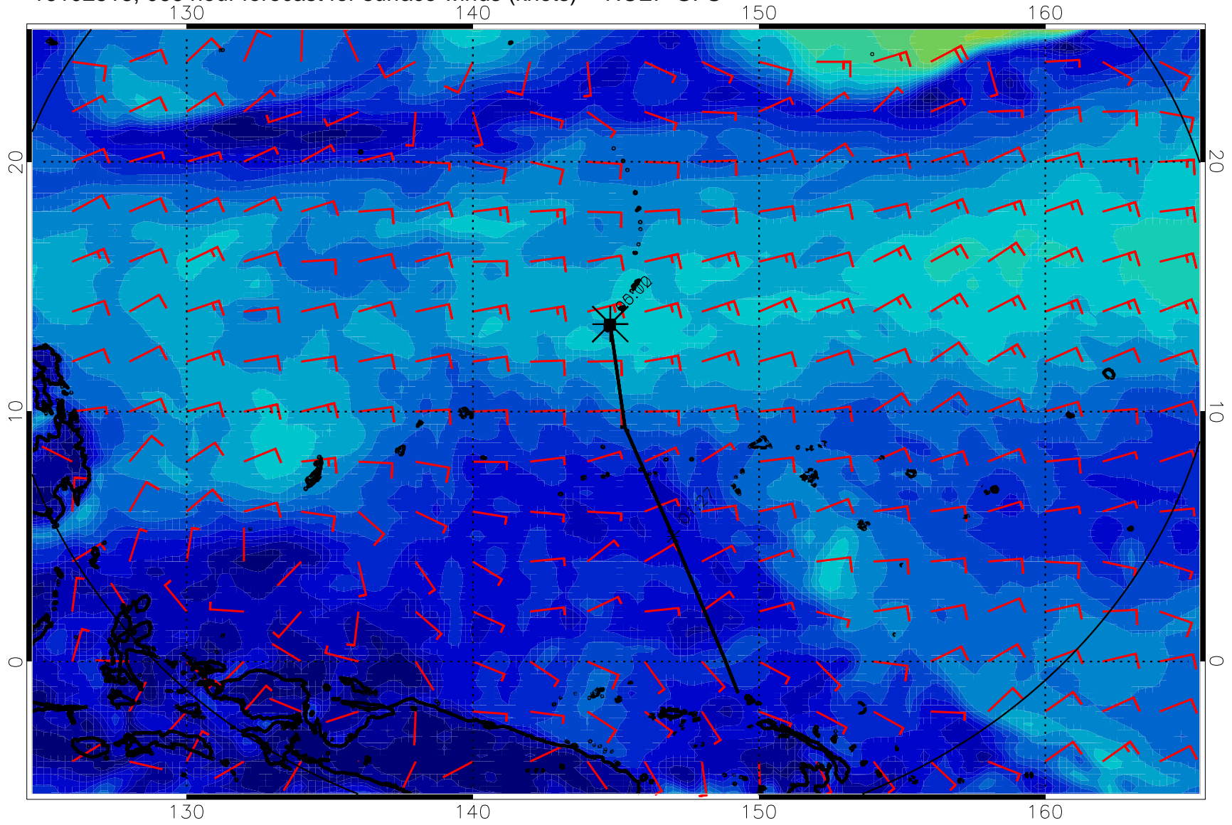
16102518, 066 hour forecast for surface winds (knots) -- NCEP GFS
