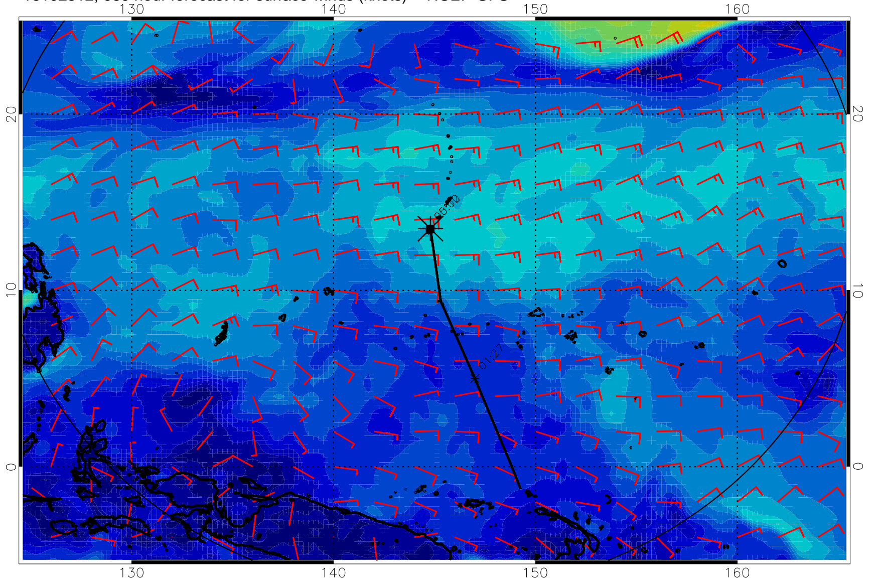
16102512, 060 hour forecast for surface winds (knots) -- NCEP GFS
