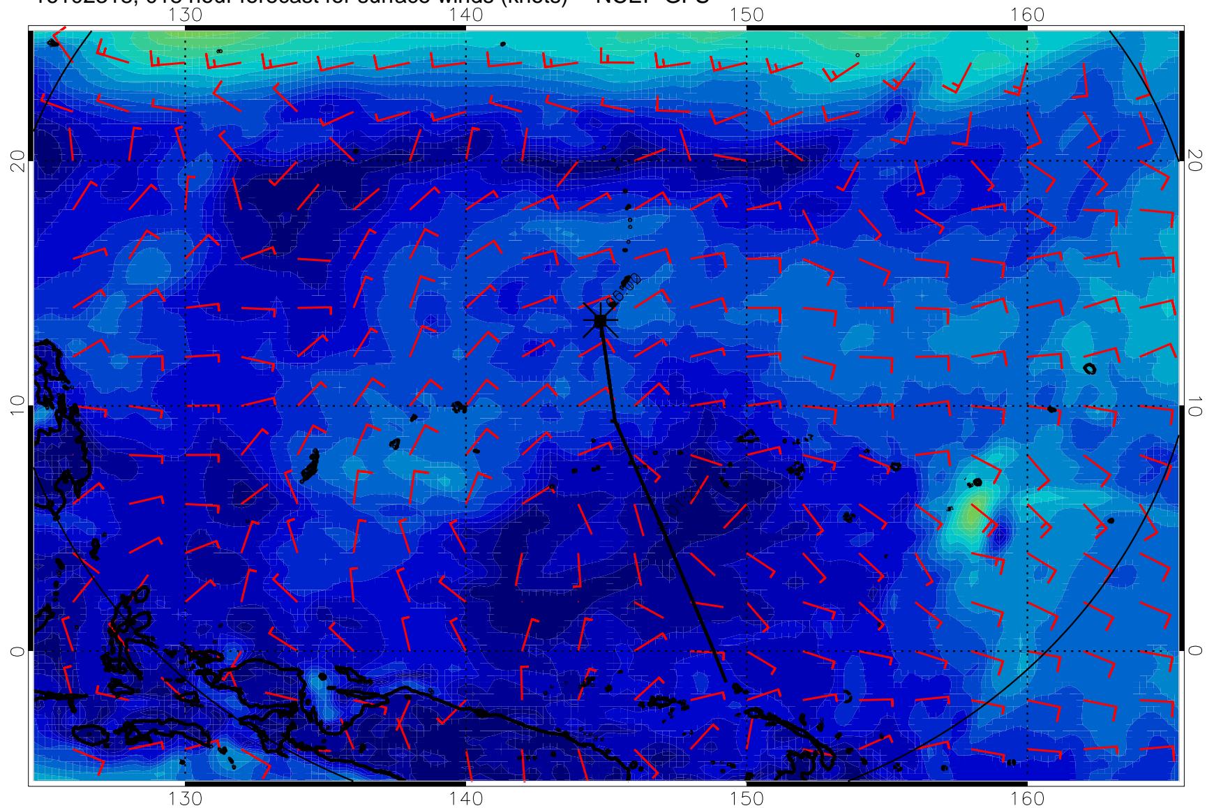
16102318, 018 hour forecast for surface winds (knots) -- NCEP GFS
