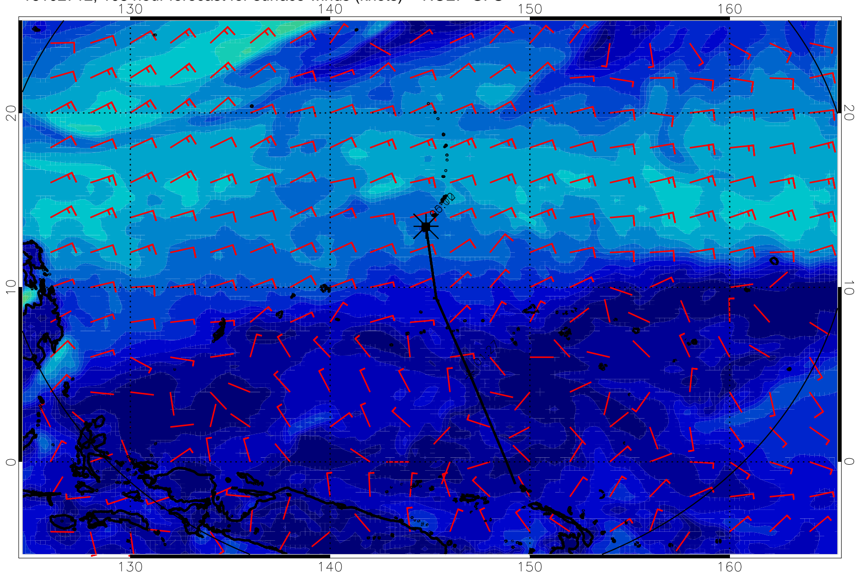
16102712, 108 hour forecast for surface winds (knots) -- NCEP GFS
