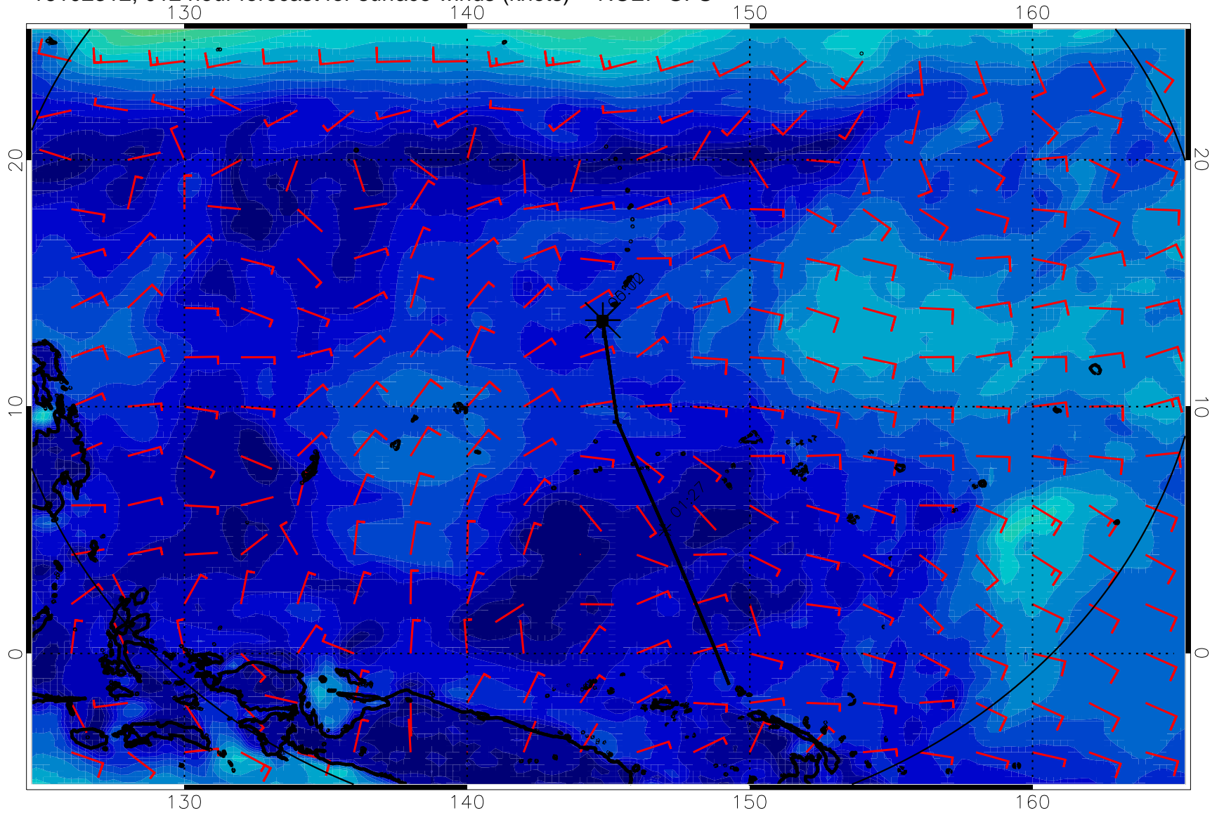
16102312, 012 hour forecast for surface winds (knots) -- NCEP GFS
