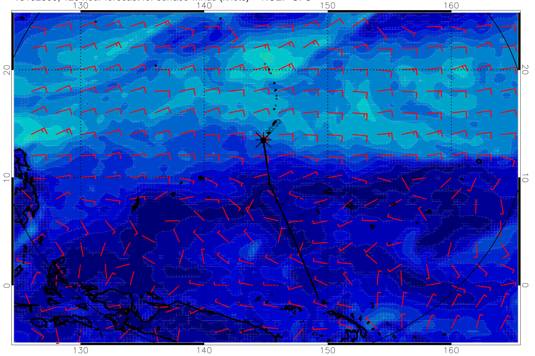
16102800, 120 hour forecast for surface winds (knots) -- NCEP GFS
