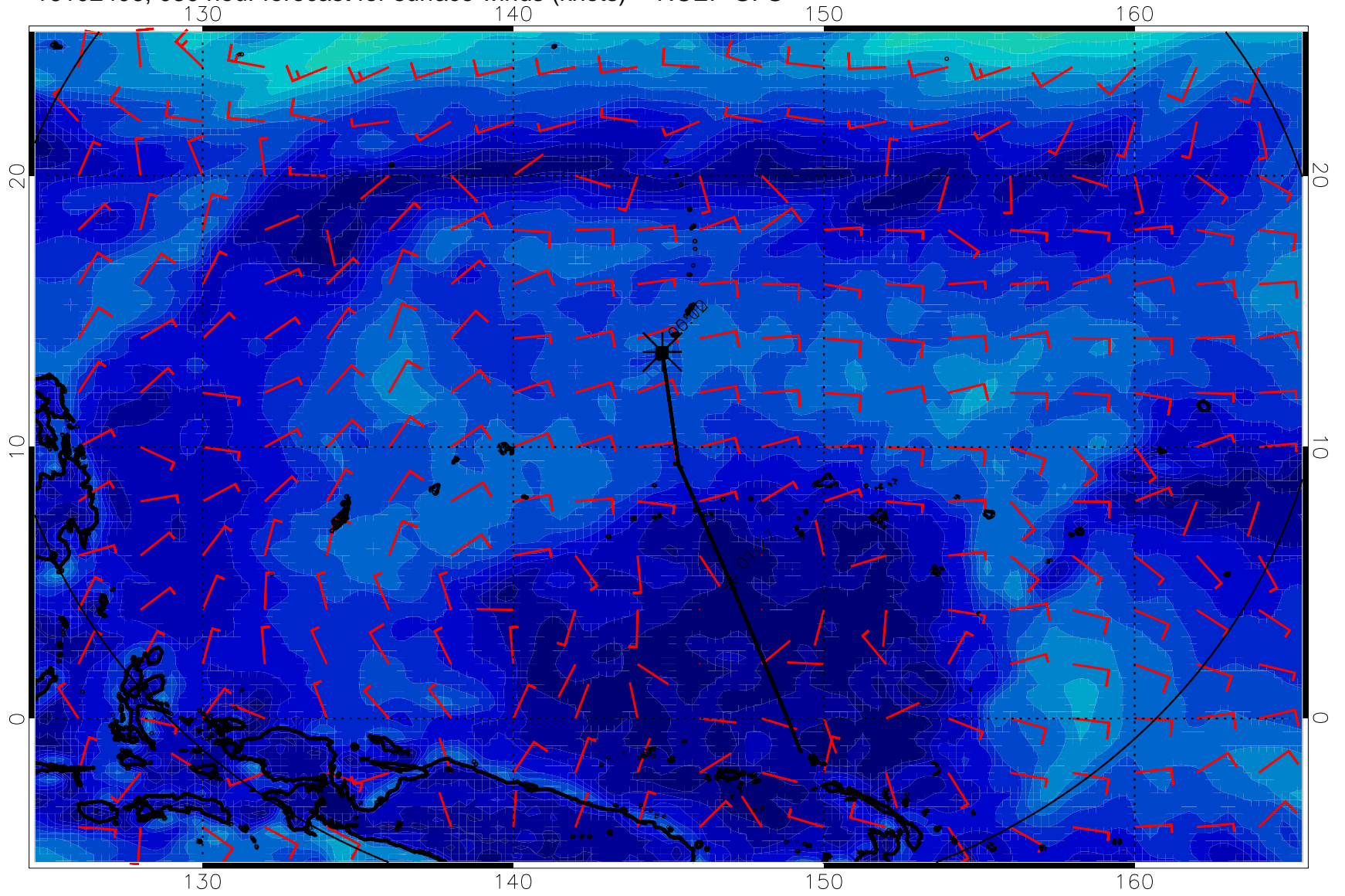
16102406, 030 hour forecast for surface winds (knots) -- NCEP GFS
