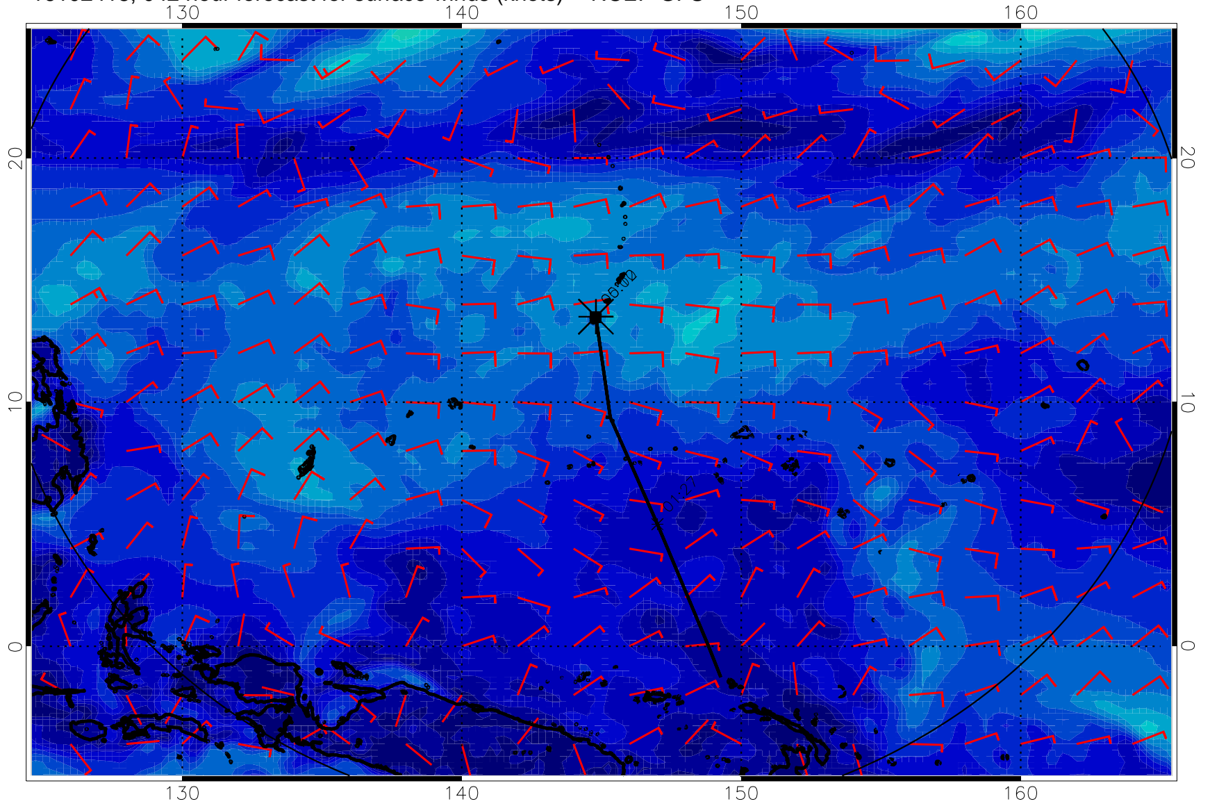
16102418, 042 hour forecast for surface winds (knots) -- NCEP GFS
