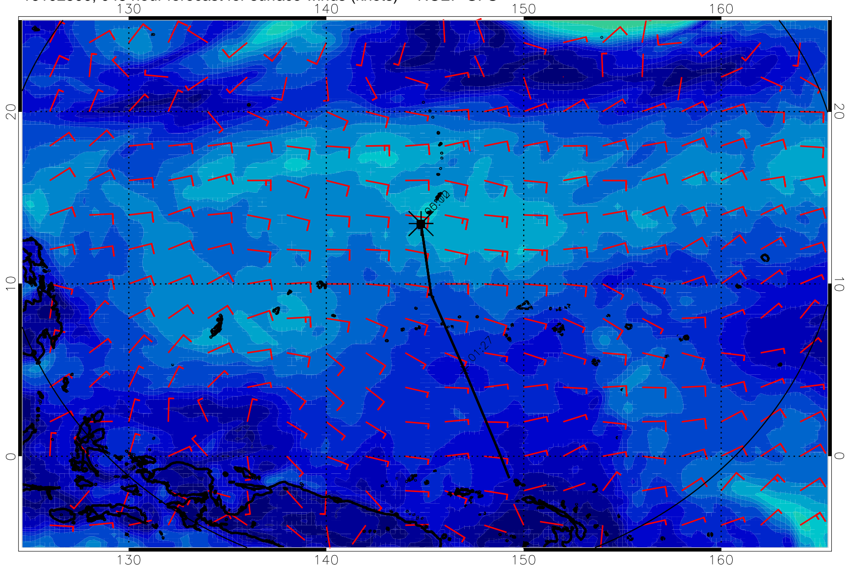
16102500, 048 hour forecast for surface winds (knots) -- NCEP GFS
