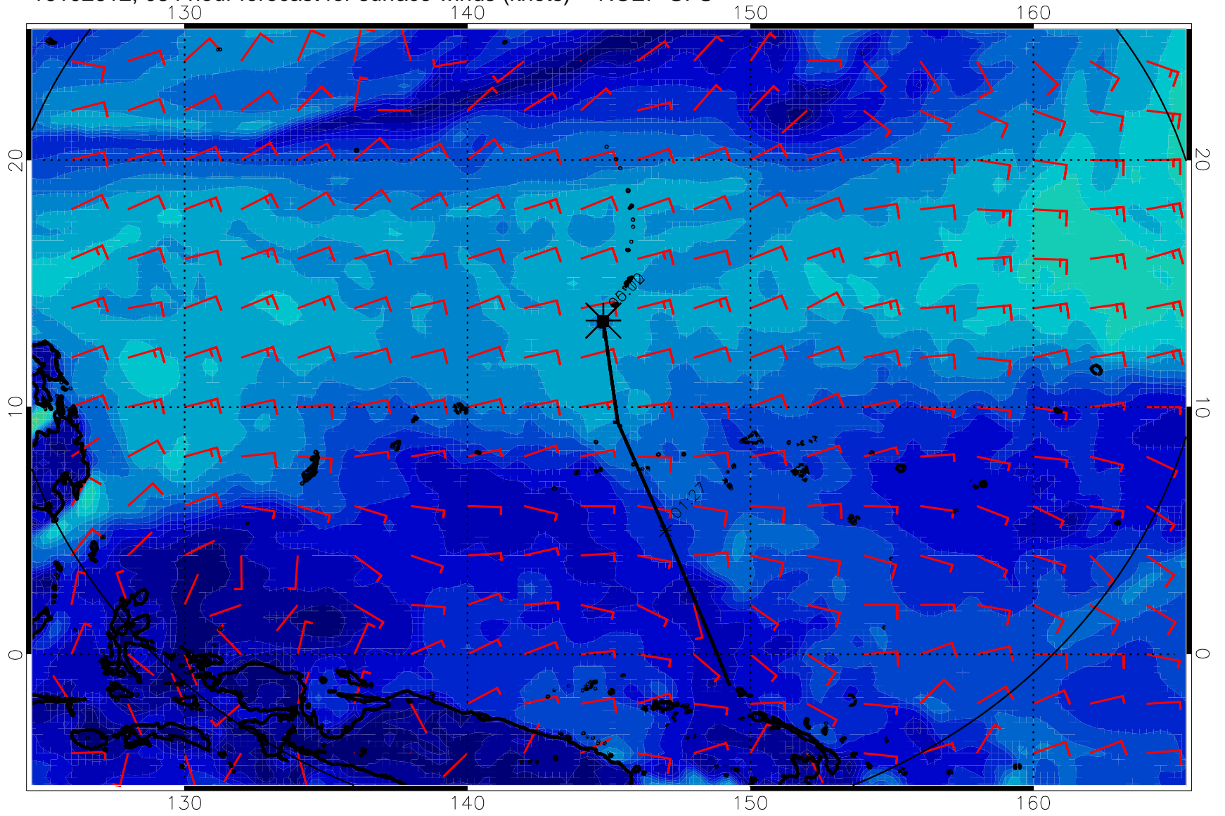
16102612, 084 hour forecast for surface winds (knots) -- NCEP GFS
