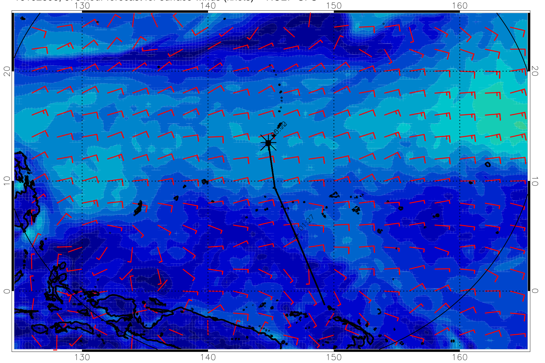
16102606, 078 hour forecast for surface winds (knots) -- NCEP GFS
