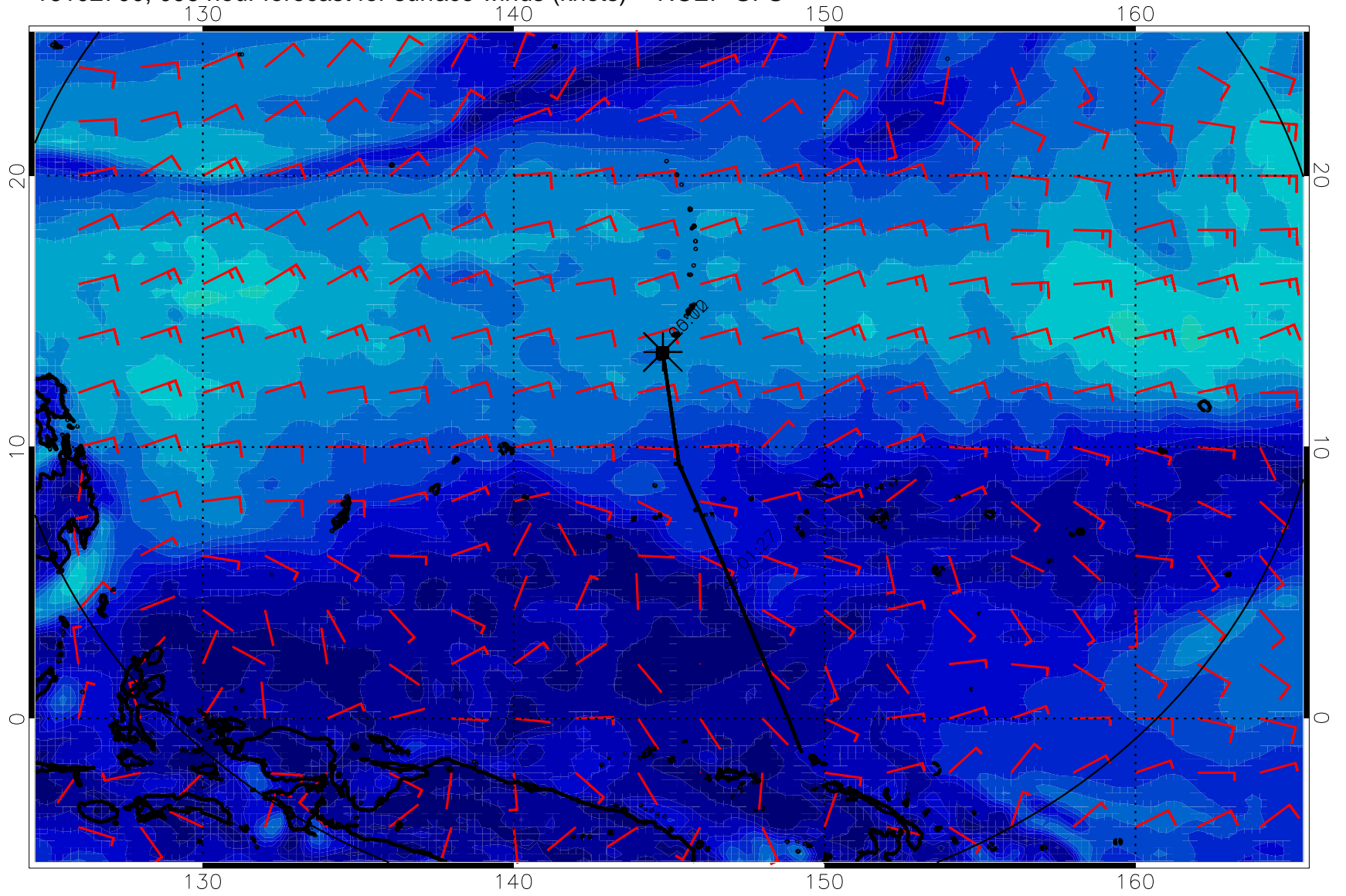
16102700, 096 hour forecast for surface winds (knots) -- NCEP GFS
