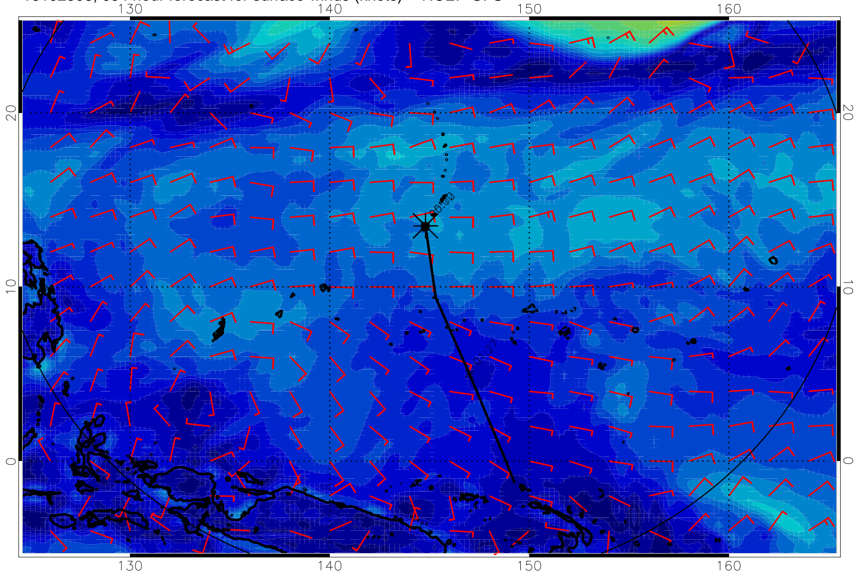
16102506, 054 hour forecast for surface winds (knots) -- NCEP GFS
