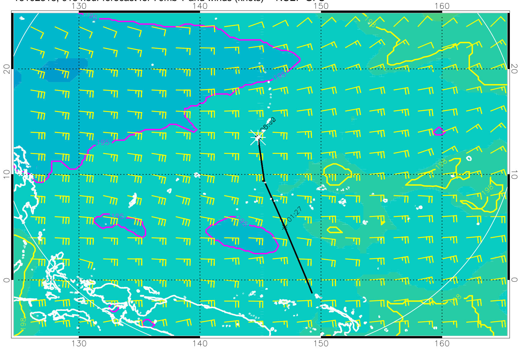
16102318, 018 hour forecast for 70mb T and winds (knots) -- NCEP GFS
