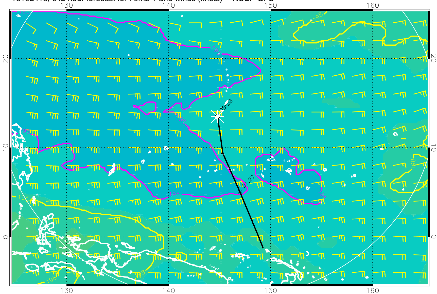
16102418, 042 hour forecast for 70mb T and winds (knots) -- NCEP GFS
