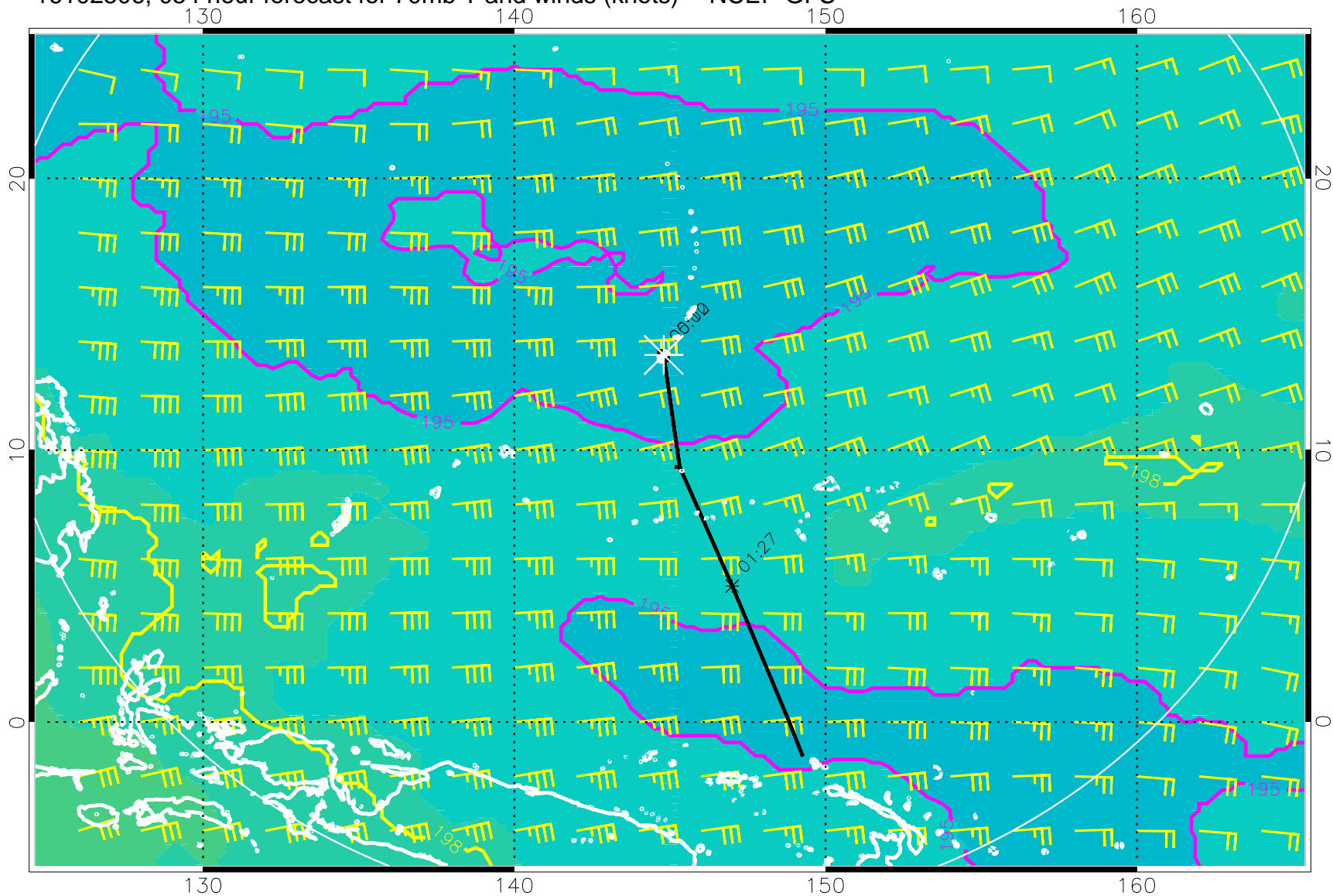
16102506, 054 hour forecast for 70mb T and winds (knots) -- NCEP GFS
