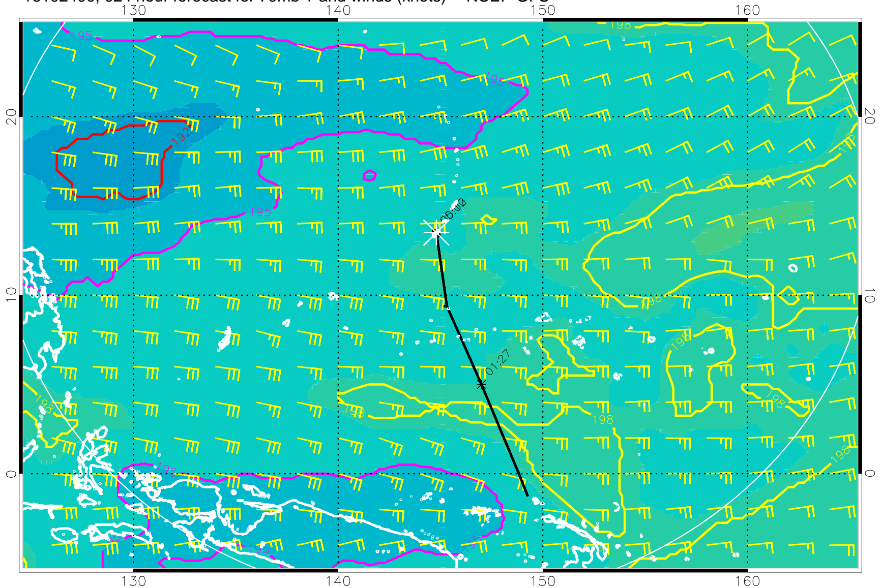
16102400, 024 hour forecast for 70mb T and winds (knots) -- NCEP GFS
