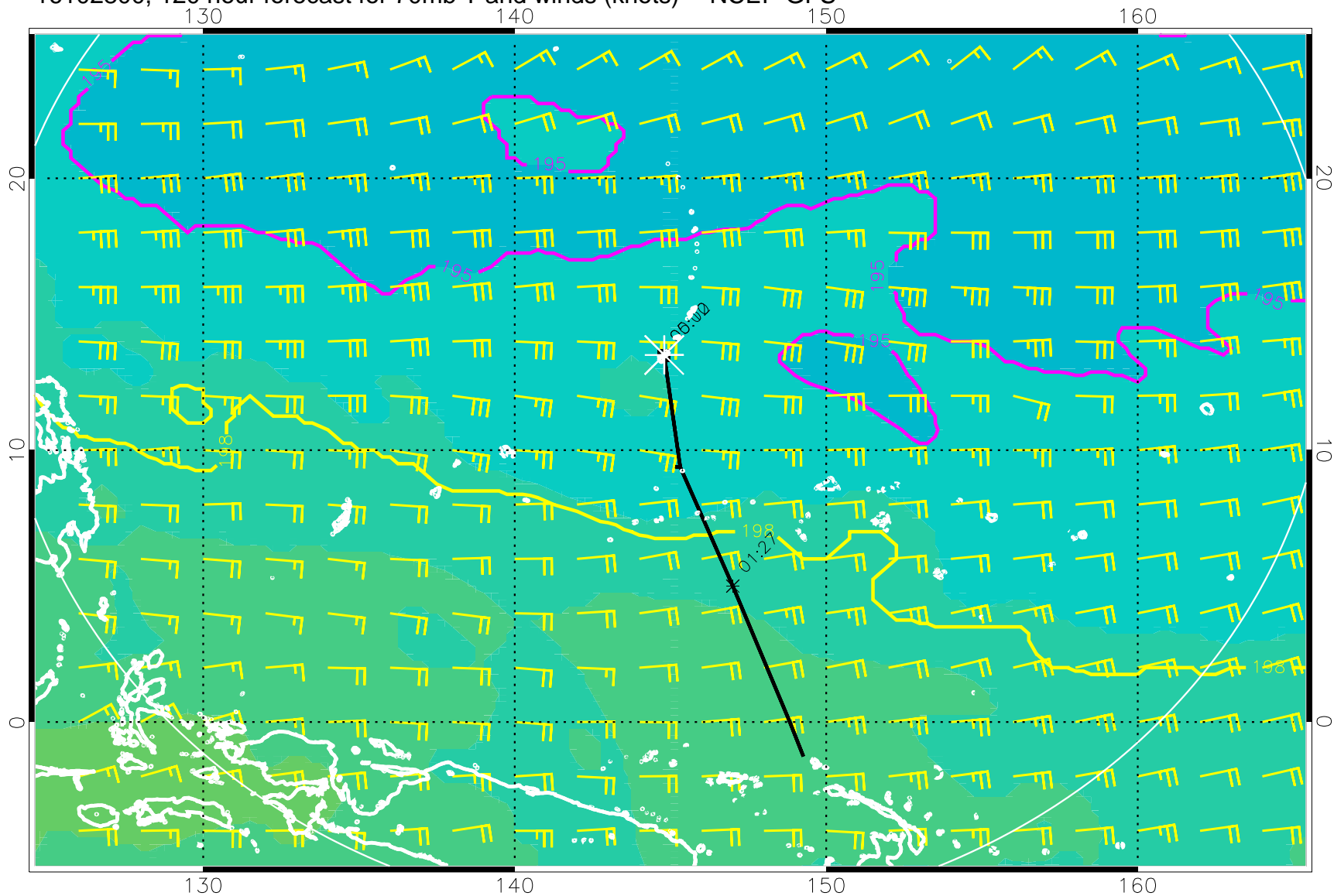
16102800, 120 hour forecast for 70mb T and winds (knots) -- NCEP GFS
