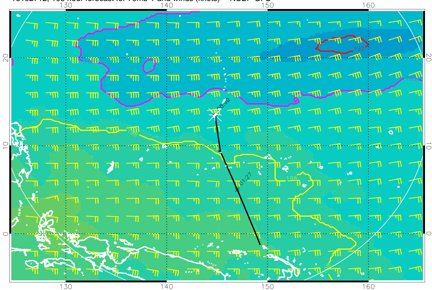
16102712, 108 hour forecast for 70mb T and winds (knots) -- NCEP GFS
