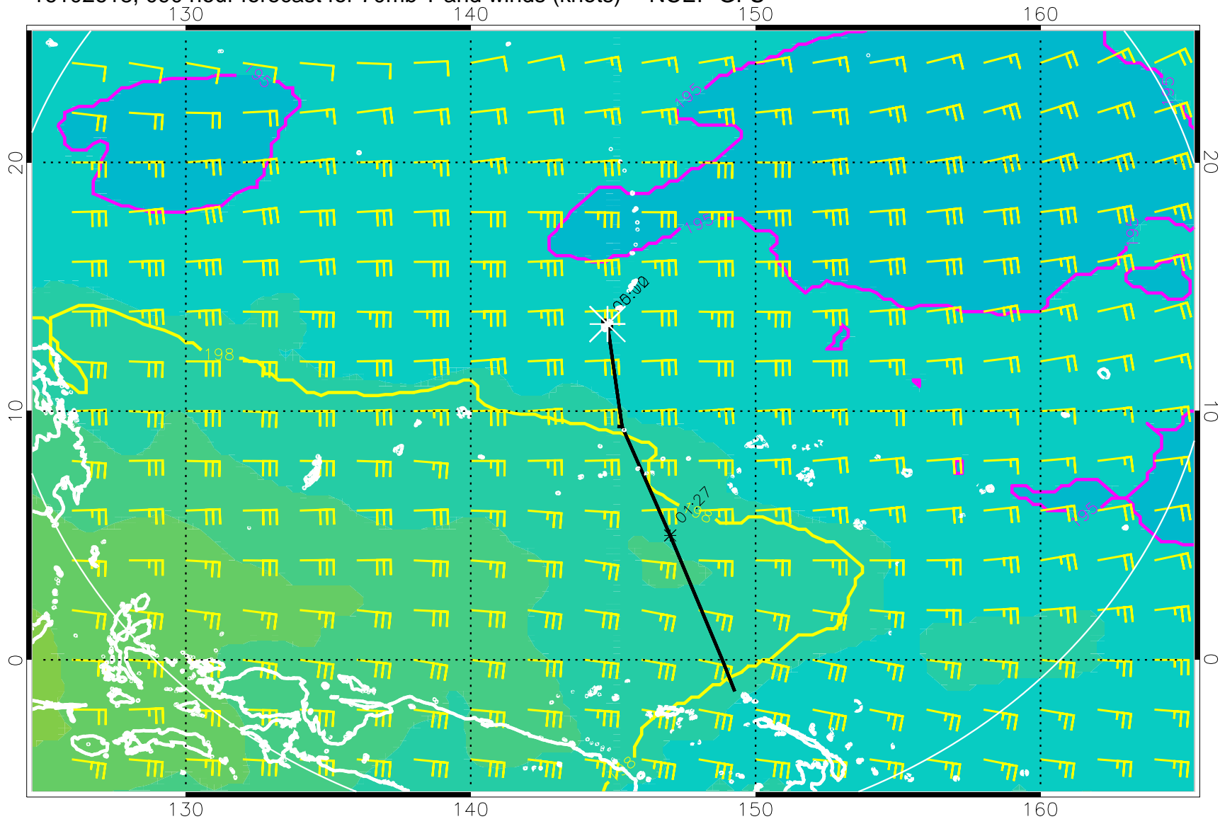
16102618, 090 hour forecast for 70mb T and winds (knots) -- NCEP GFS
