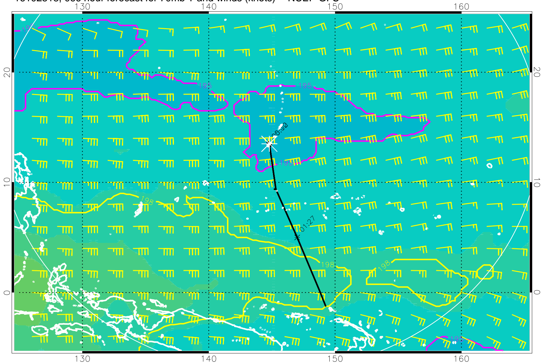
16102518, 066 hour forecast for 70mb T and winds (knots) -- NCEP GFS
