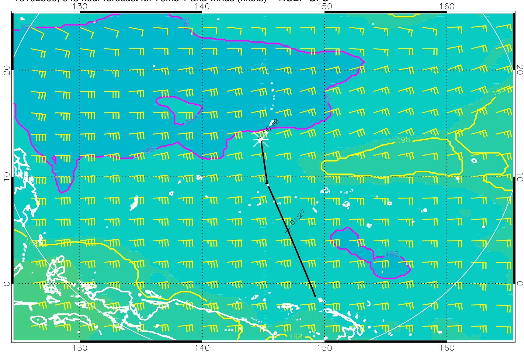
16102500, 048 hour forecast for 70mb T and winds (knots) -- NCEP GFS
