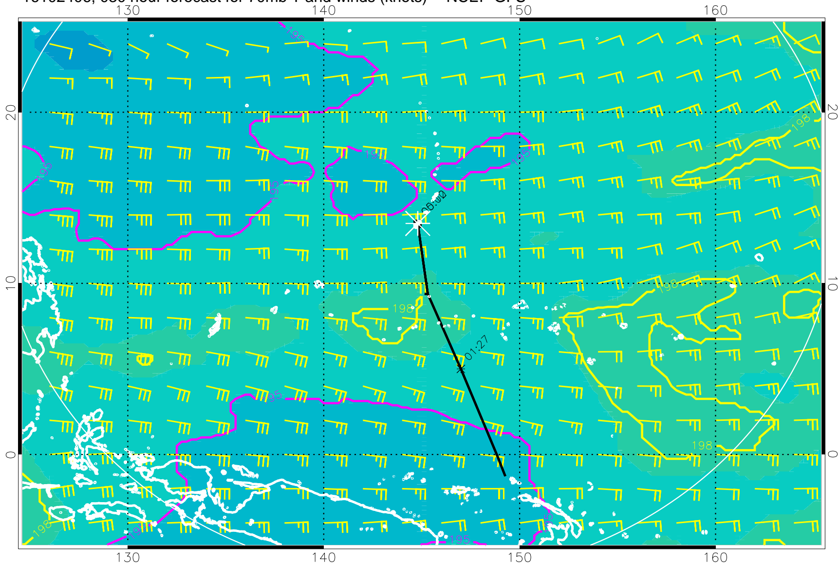
16102406, 030 hour forecast for 70mb T and winds (knots) -- NCEP GFS
