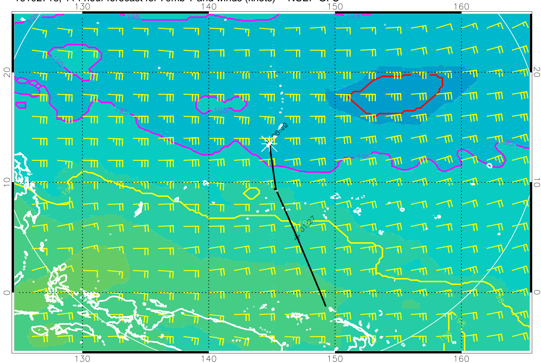
16102718, 114 hour forecast for 70mb T and winds (knots) -- NCEP GFS
