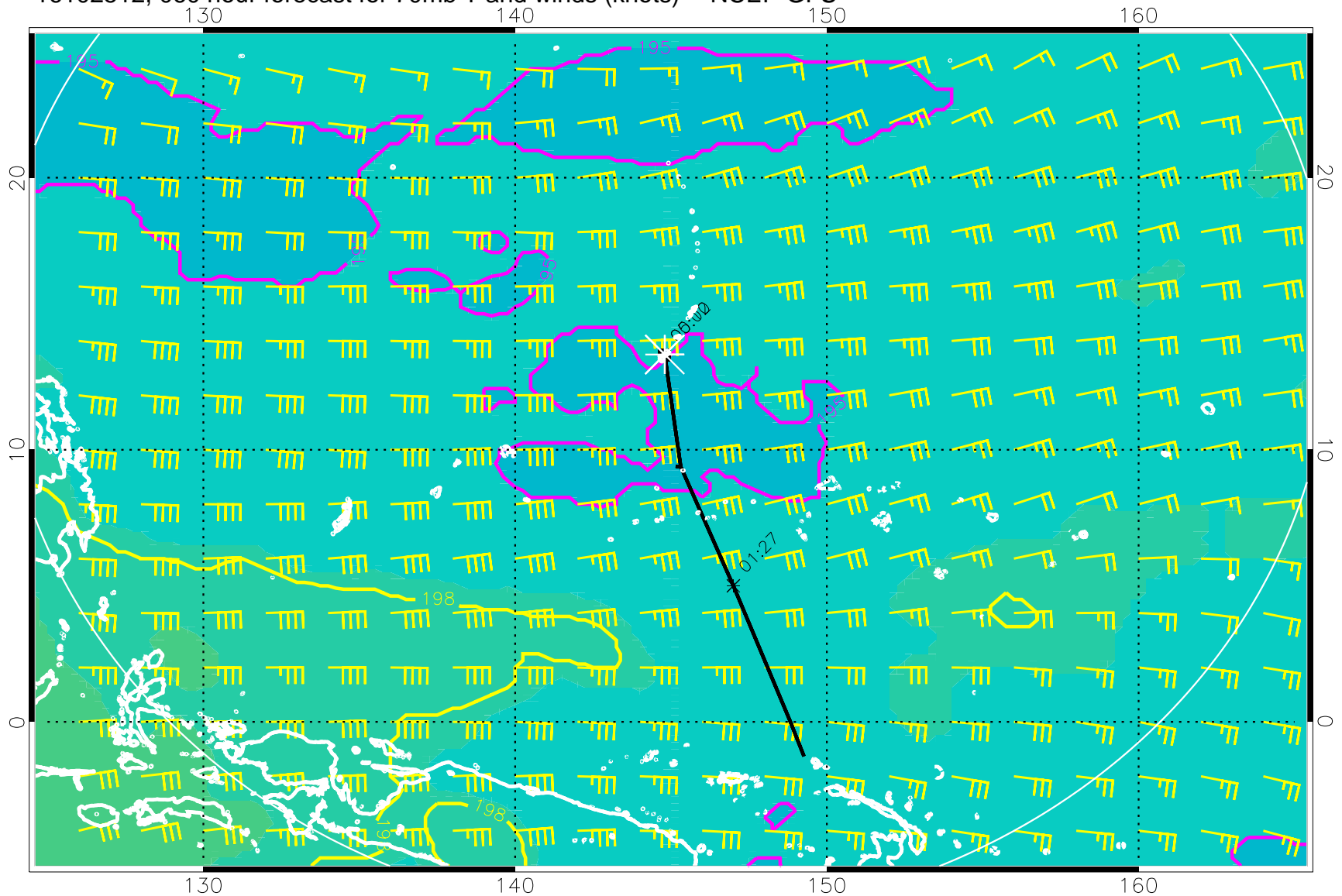
16102512, 060 hour forecast for 70mb T and winds (knots) -- NCEP GFS
