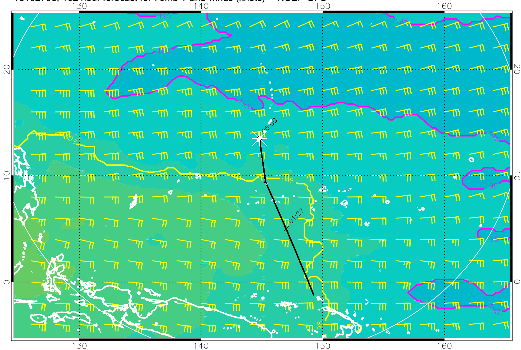
16102706, 102 hour forecast for 70mb T and winds (knots) -- NCEP GFS
