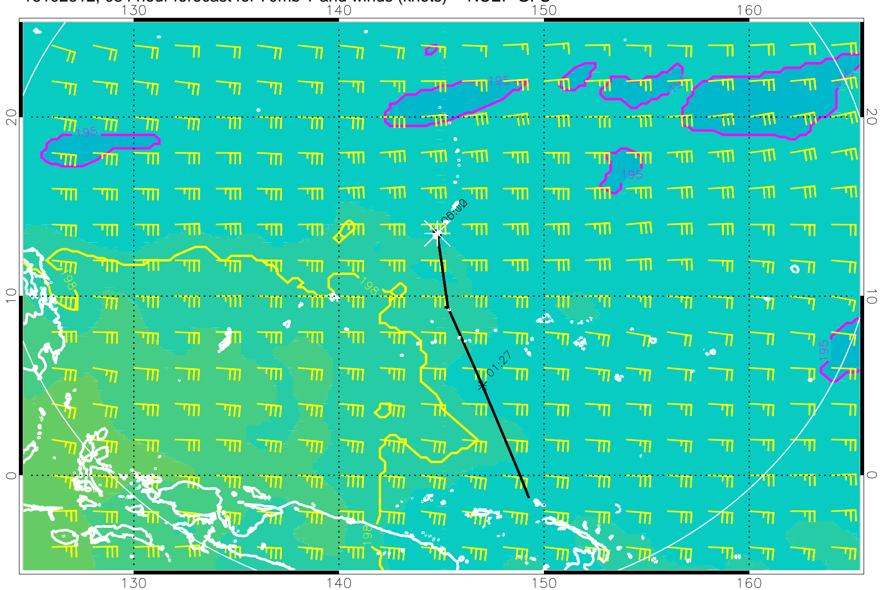
16102612, 084 hour forecast for 70mb T and winds (knots) -- NCEP GFS
