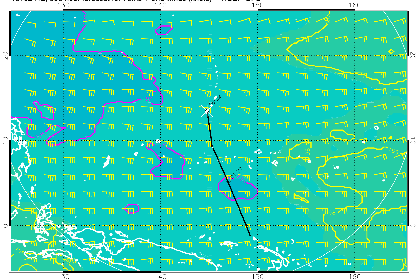
16102412, 036 hour forecast for 70mb T and winds (knots) -- NCEP GFS
