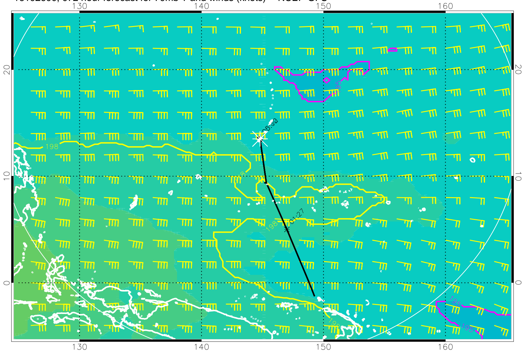
16102600, 072 hour forecast for 70mb T and winds (knots) -- NCEP GFS
