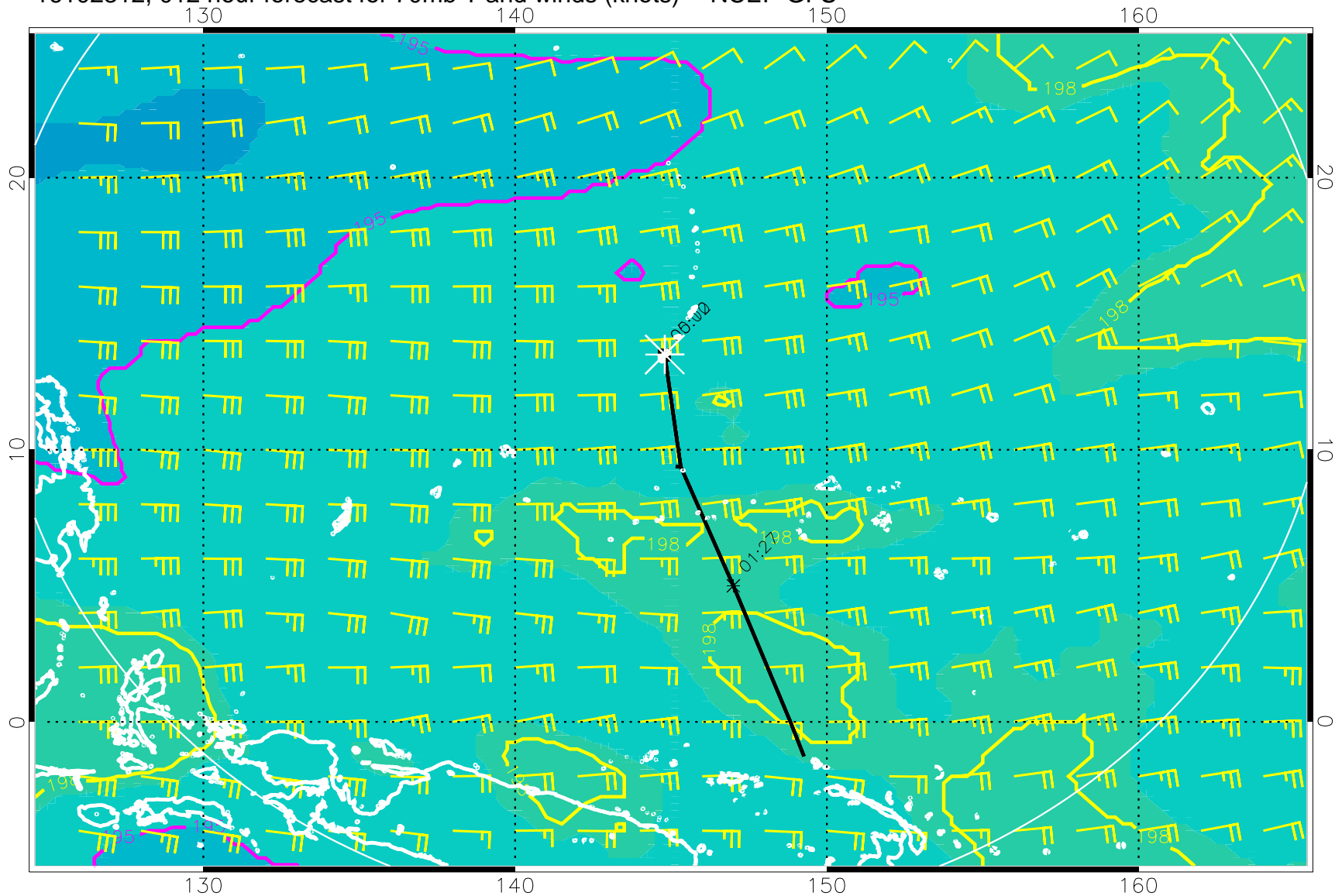
16102312, 012 hour forecast for 70mb T and winds (knots) -- NCEP GFS
