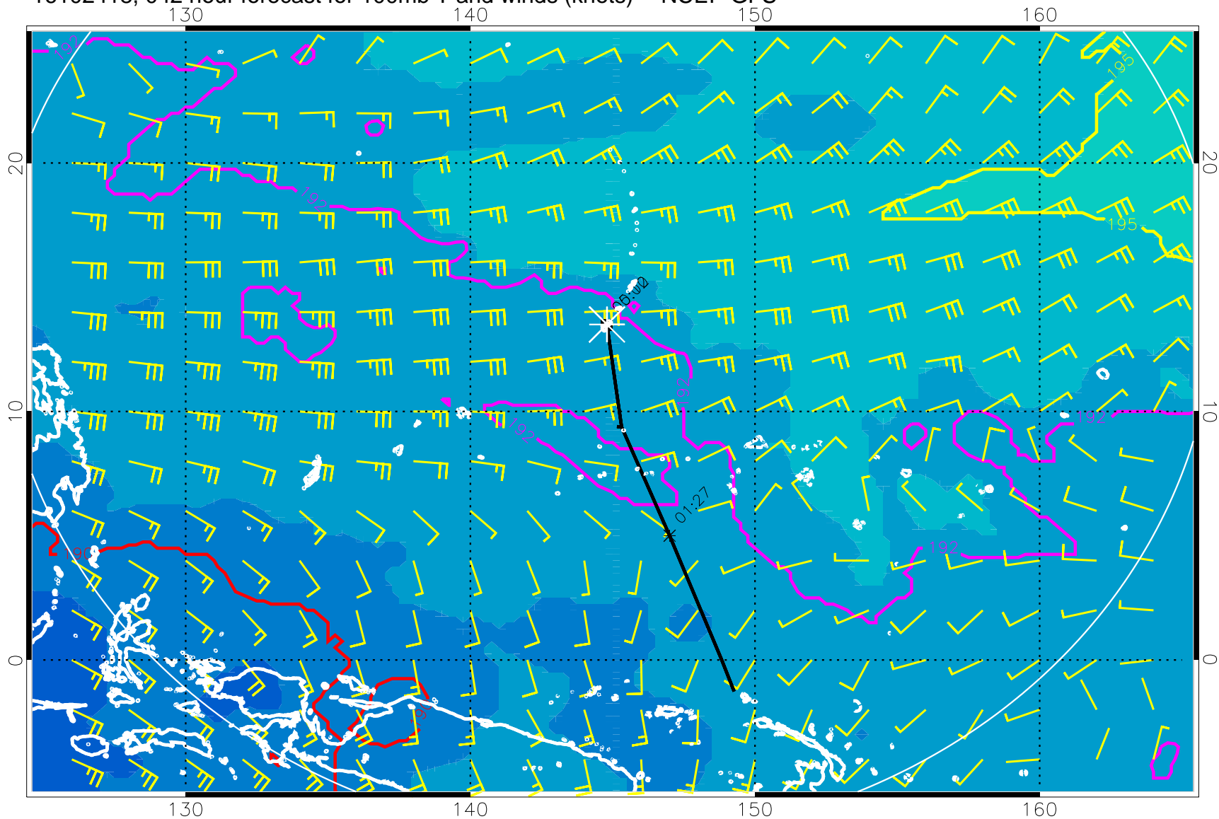
16102418, 042 hour forecast for 100mb T and winds (knots) -- NCEP GFS
