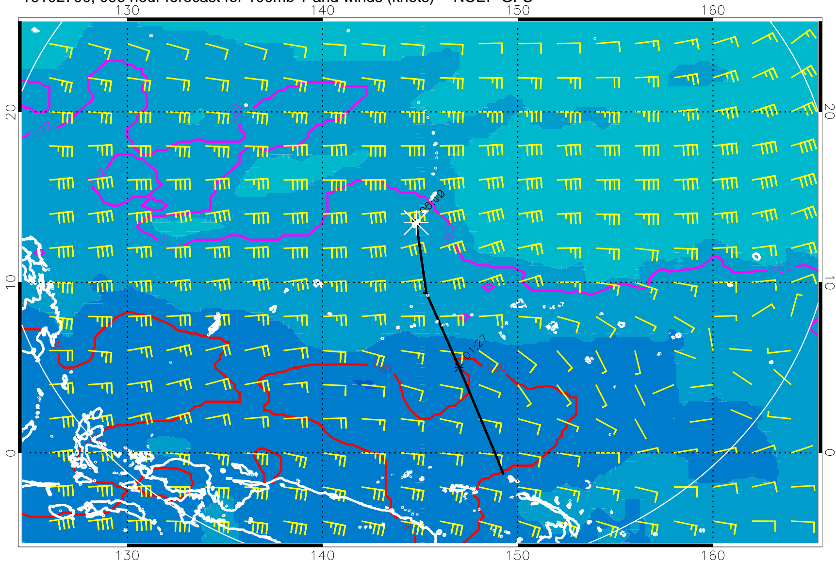
16102700, 096 hour forecast for 100mb T and winds (knots) -- NCEP GFS
