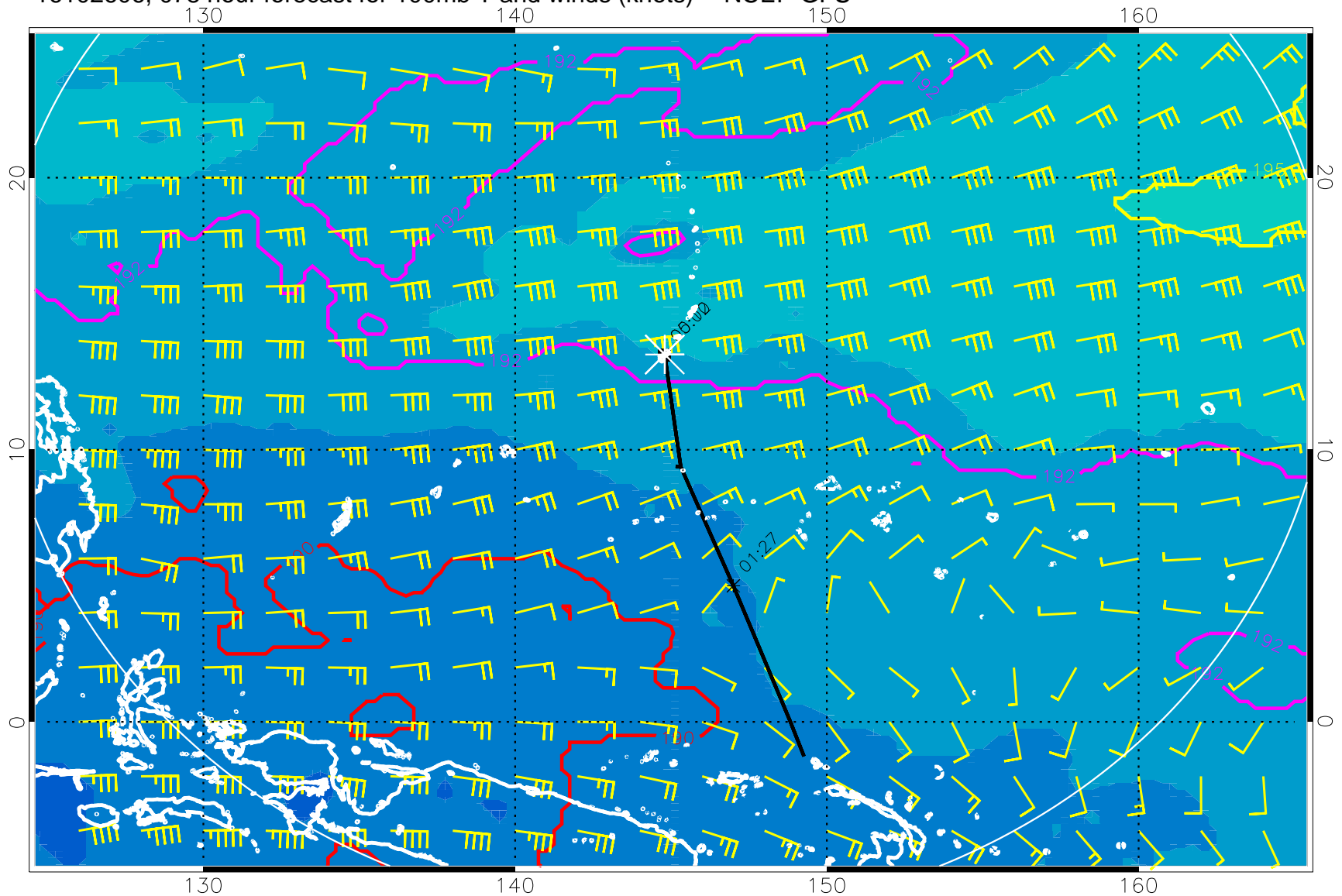
16102606, 078 hour forecast for 100mb T and winds (knots) -- NCEP GFS
