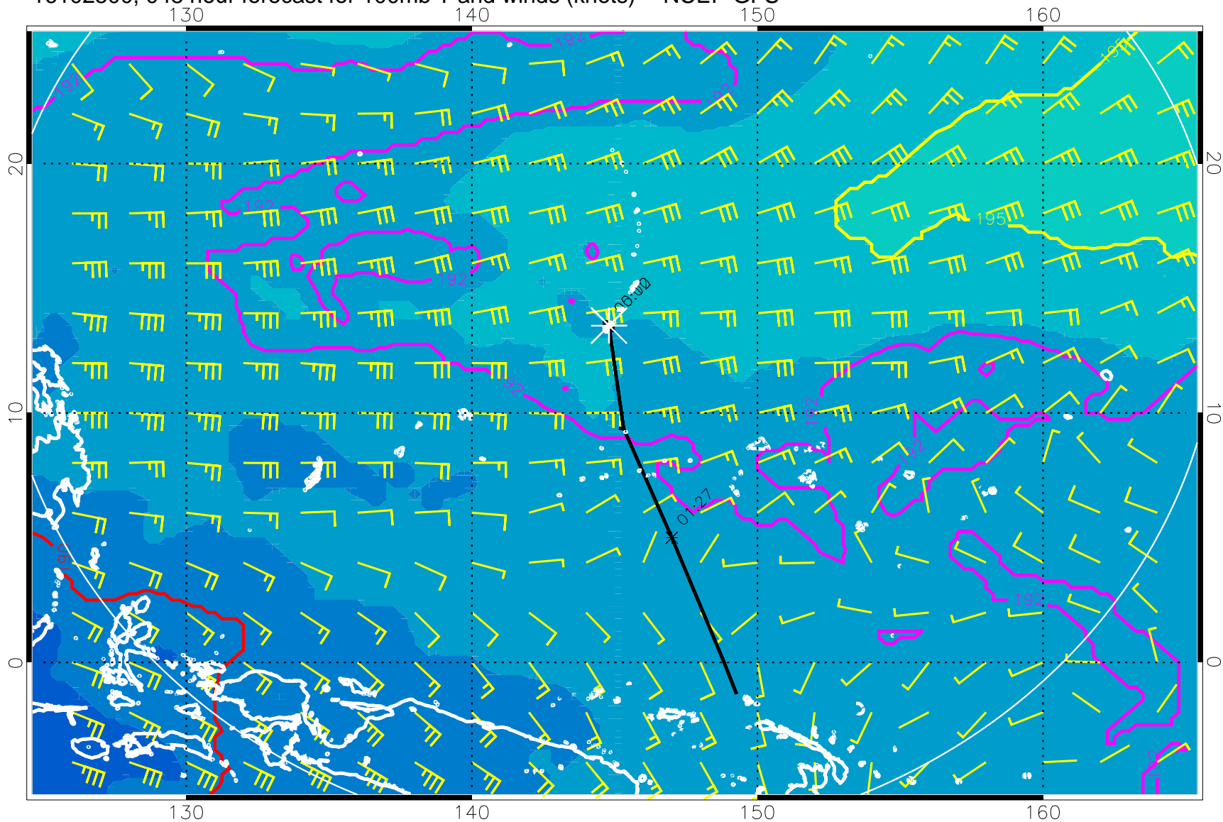
16102500, 048 hour forecast for 100mb T and winds (knots) -- NCEP GFS
