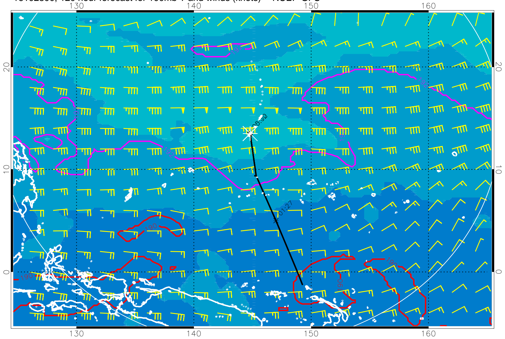
16102800, 120 hour forecast for 100mb T and winds (knots) -- NCEP GFS
