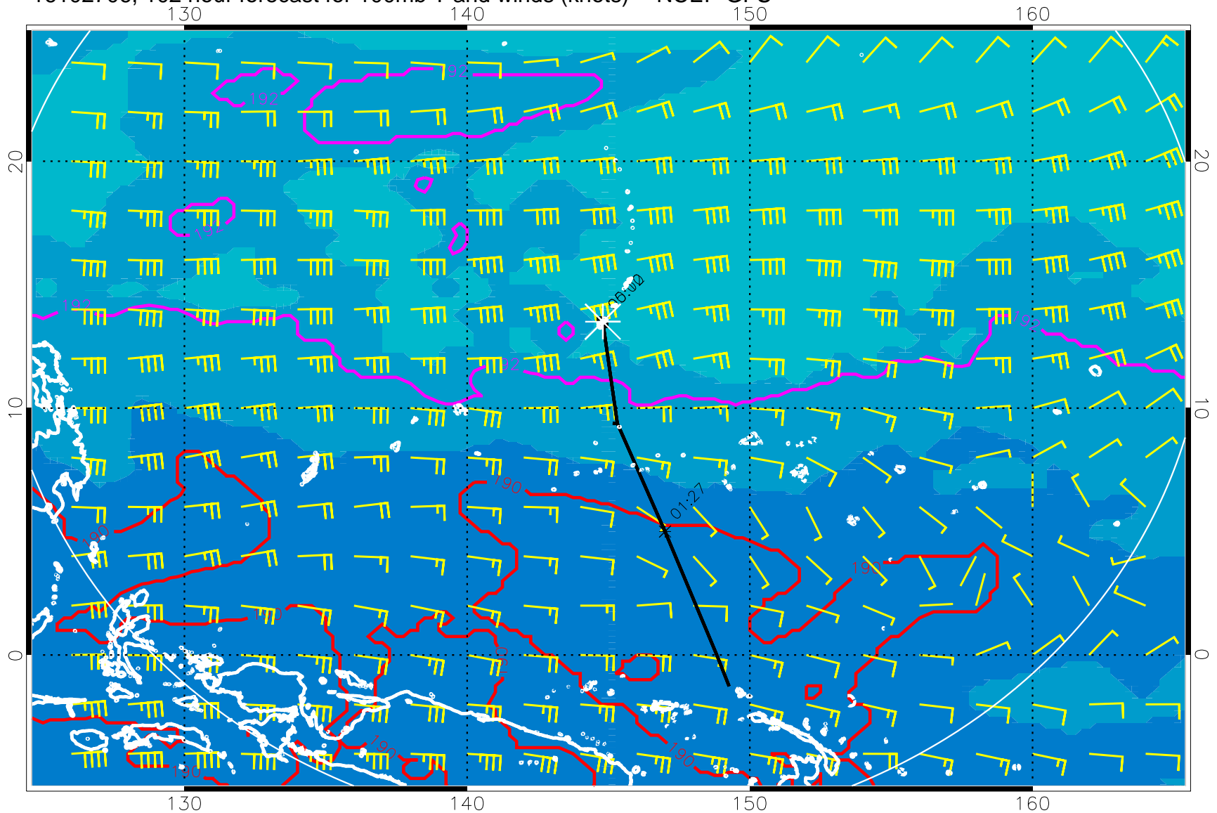
16102706, 102 hour forecast for 100mb T and winds (knots) -- NCEP GFS
