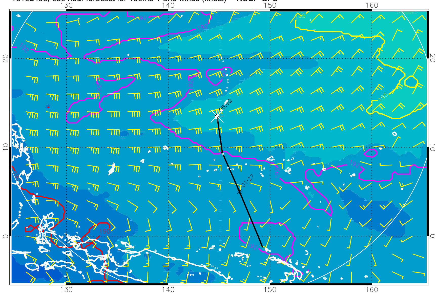
16102406, 030 hour forecast for 100mb T and winds (knots) -- NCEP GFS
