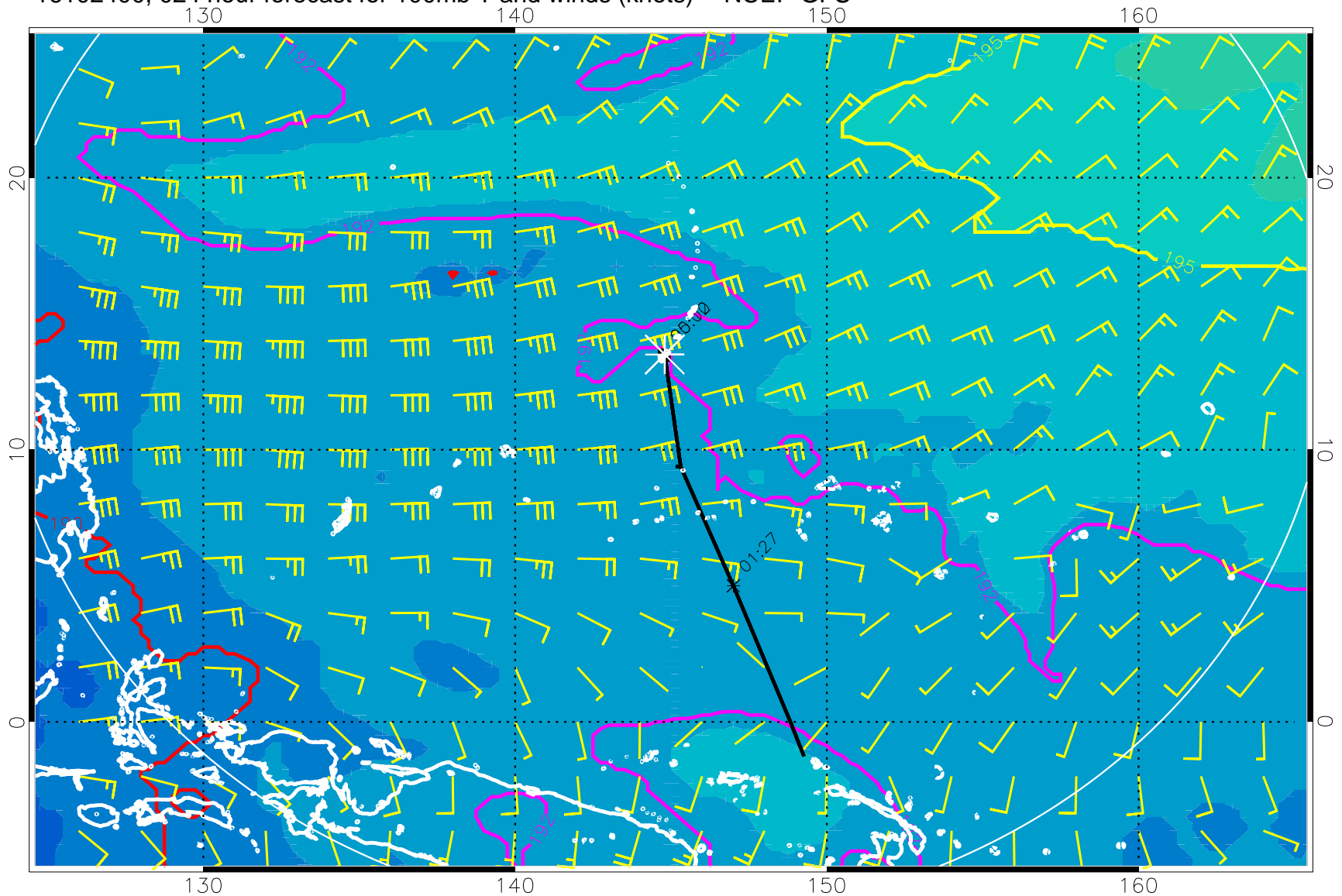
16102400, 024 hour forecast for 100mb T and winds (knots) -- NCEP GFS
