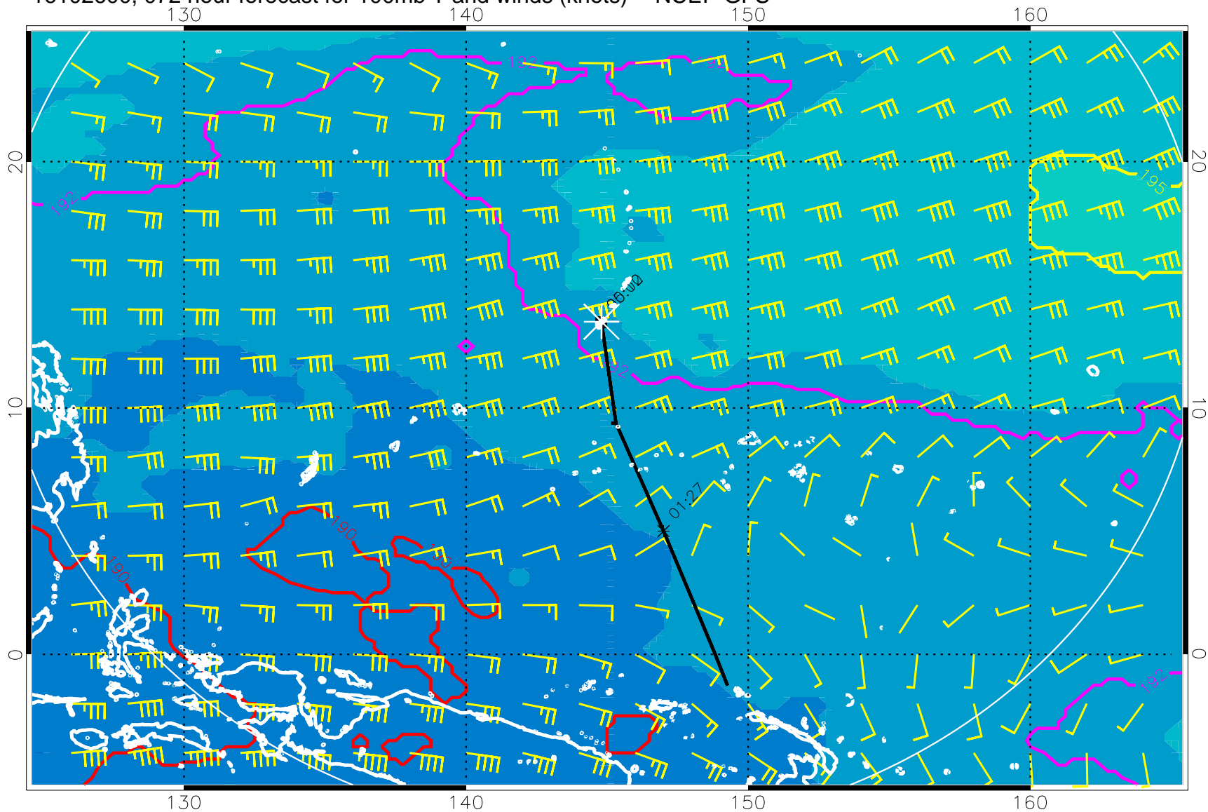
16102600, 072 hour forecast for 100mb T and winds (knots) -- NCEP GFS
