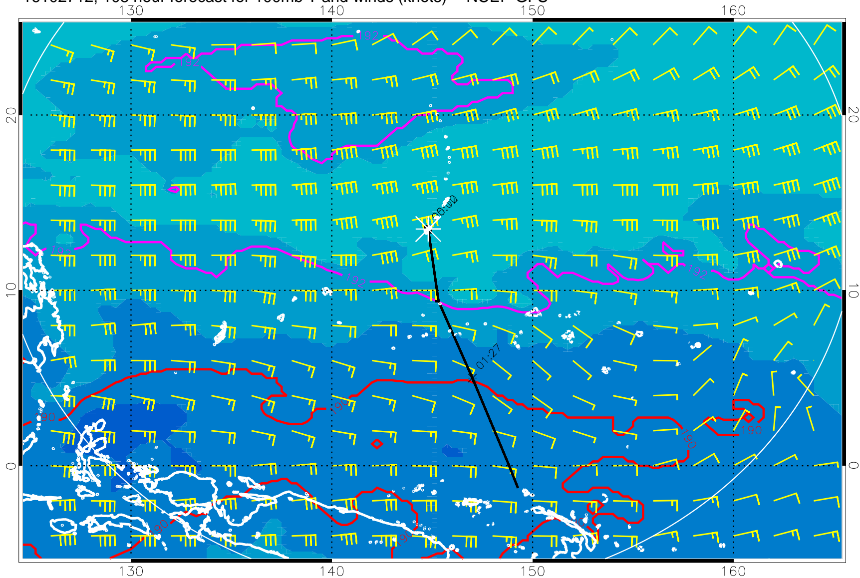
16102712, 108 hour forecast for 100mb T and winds (knots) -- NCEP GFS
