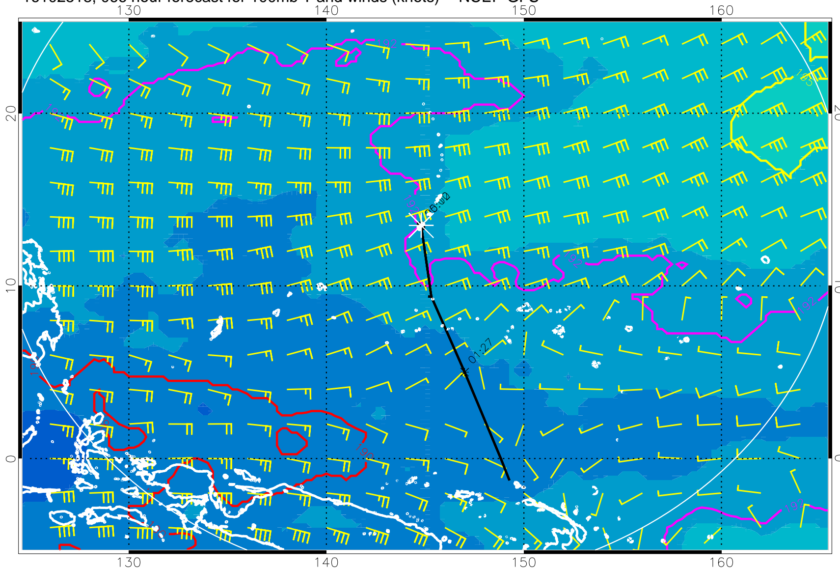
16102518, 066 hour forecast for 100mb T and winds (knots) -- NCEP GFS
