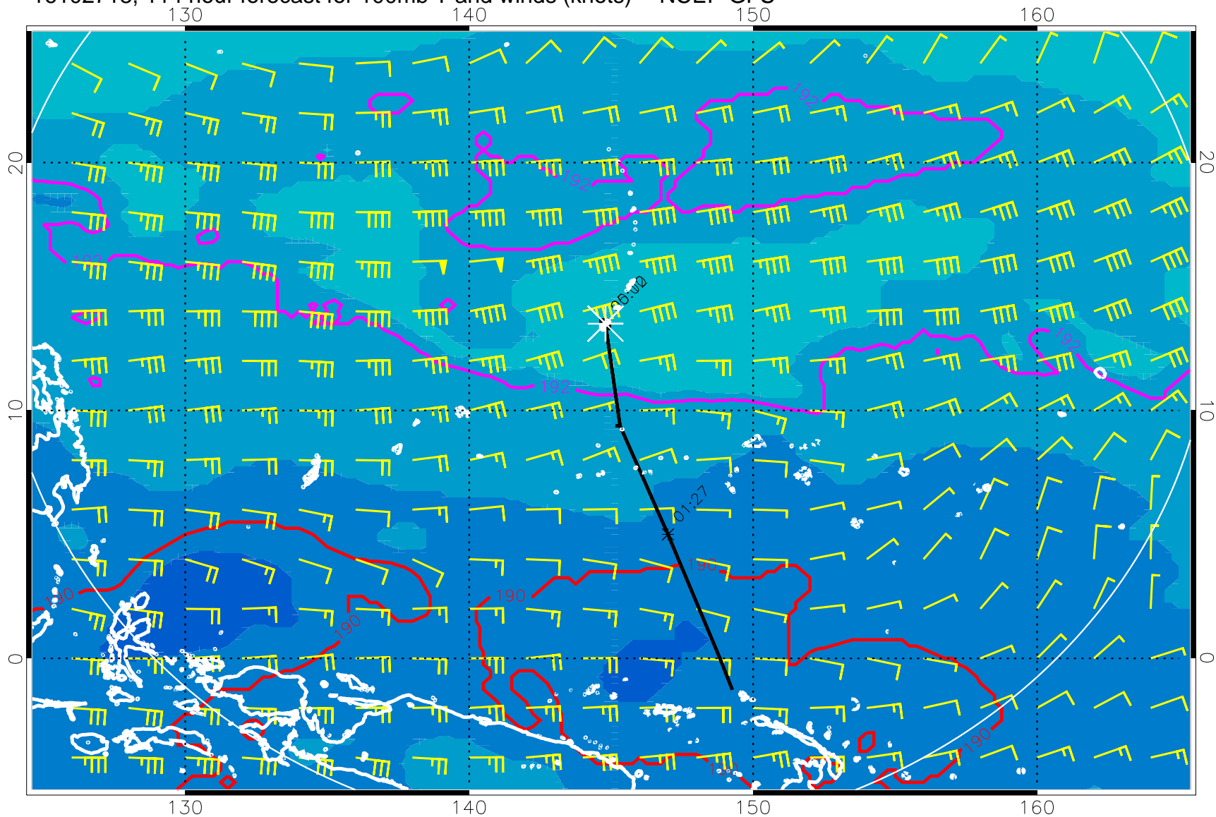
16102718, 114 hour forecast for 100mb T and winds (knots) -- NCEP GFS
