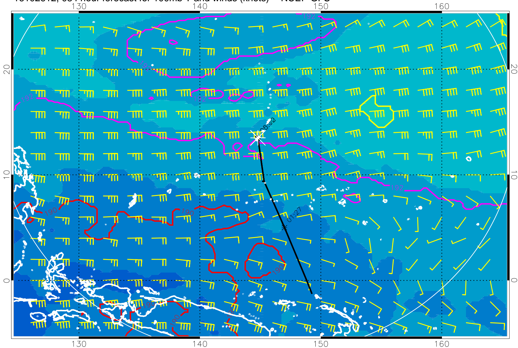
16102612, 084 hour forecast for 100mb T and winds (knots) -- NCEP GFS
