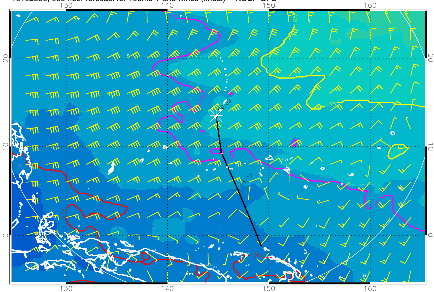
16102306, 006 hour forecast for 100mb T and winds (knots) -- NCEP GFS
