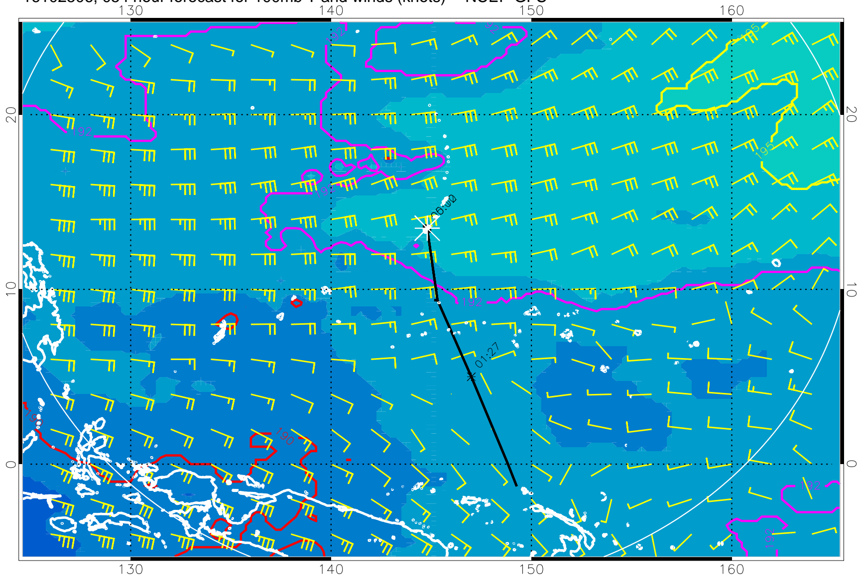
16102506, 054 hour forecast for 100mb T and winds (knots) -- NCEP GFS
