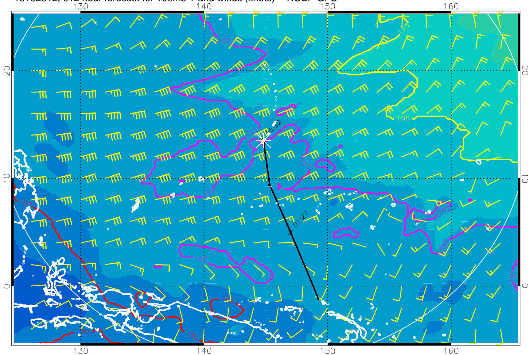
16102312, 012 hour forecast for 100mb T and winds (knots) -- NCEP GFS
