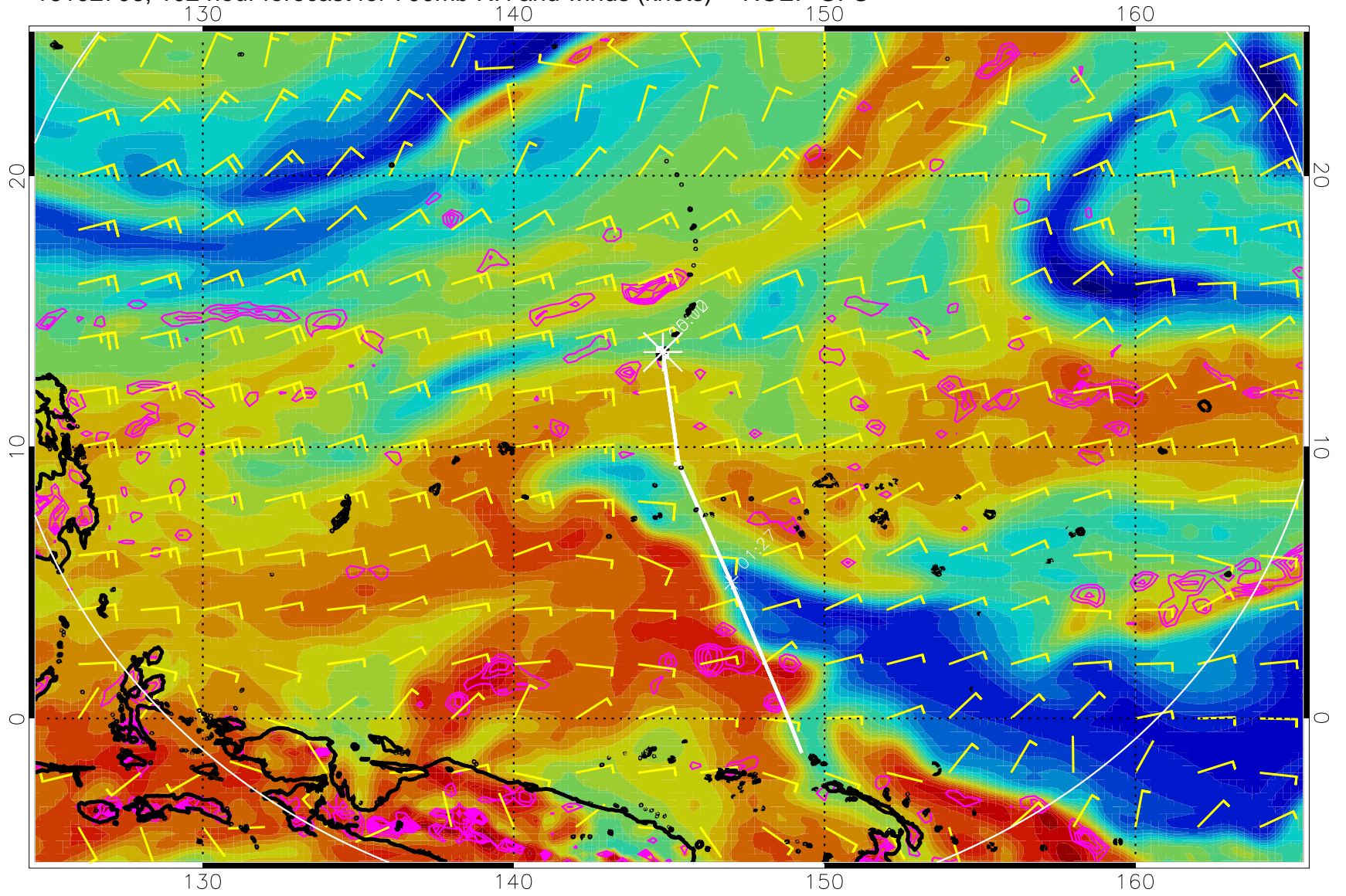
16102706, 102 hour forecast for 700mb RH and winds (knots) -- NCEP GFS
