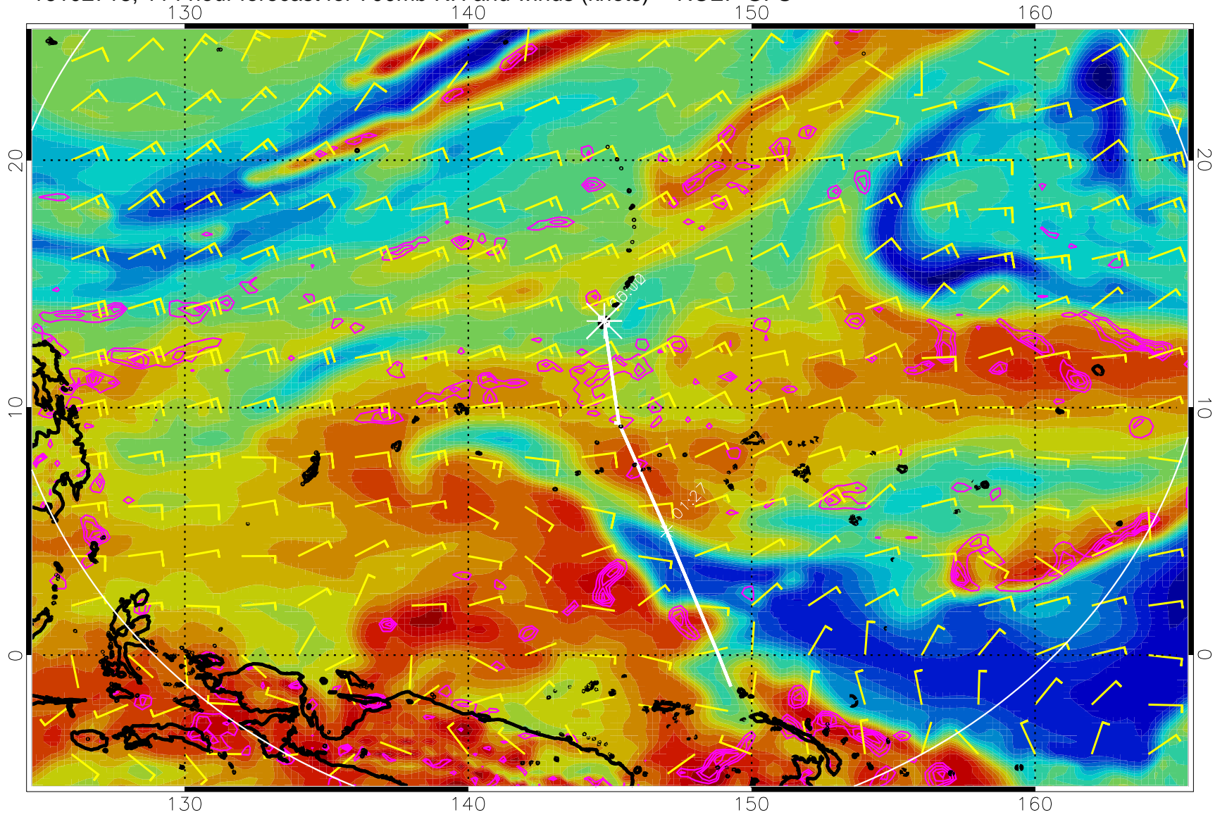
16102718, 114 hour forecast for 700mb RH and winds (knots) -- NCEP GFS
