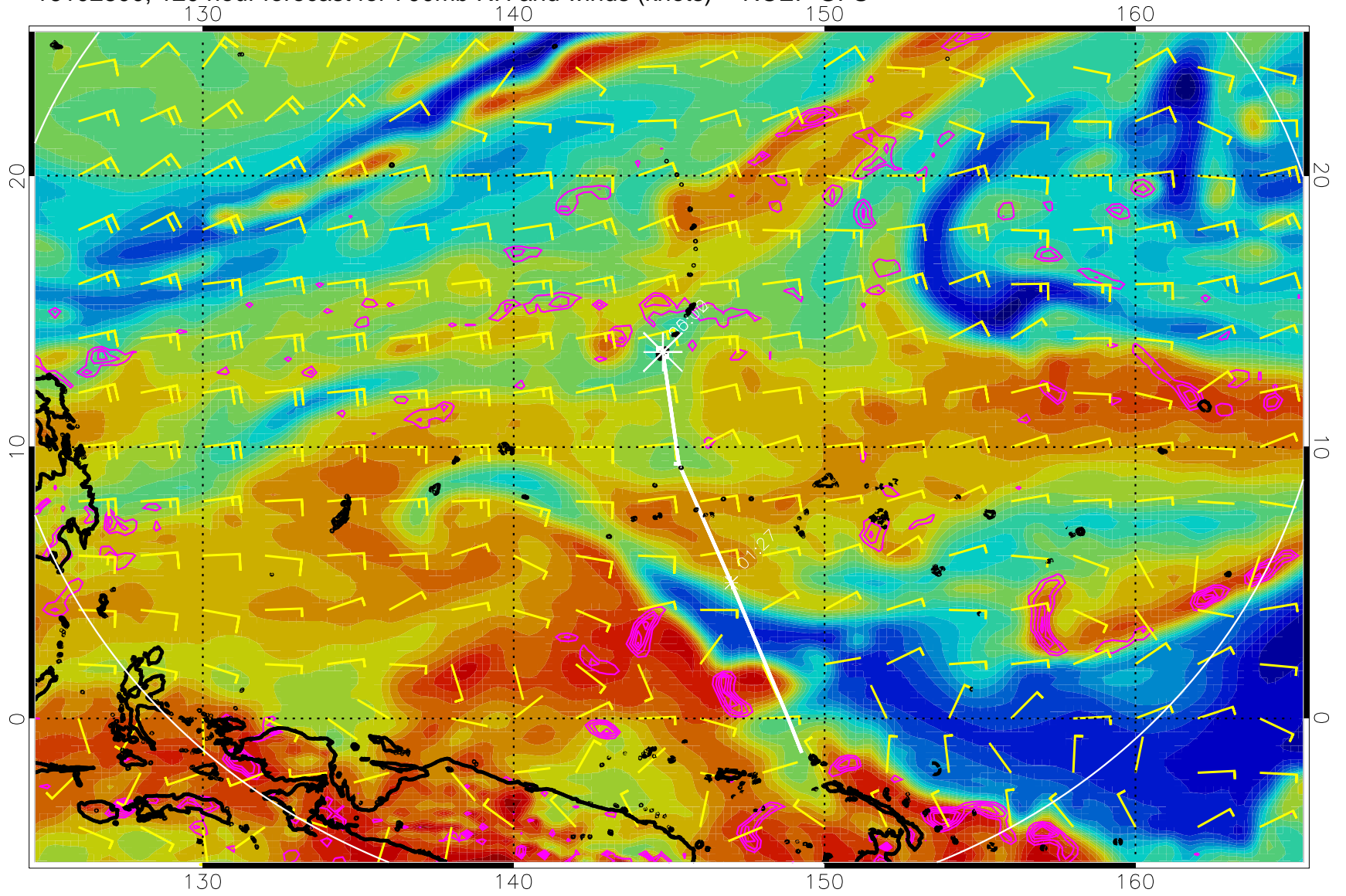
16102800, 120 hour forecast for 700mb RH and winds (knots) -- NCEP GFS
