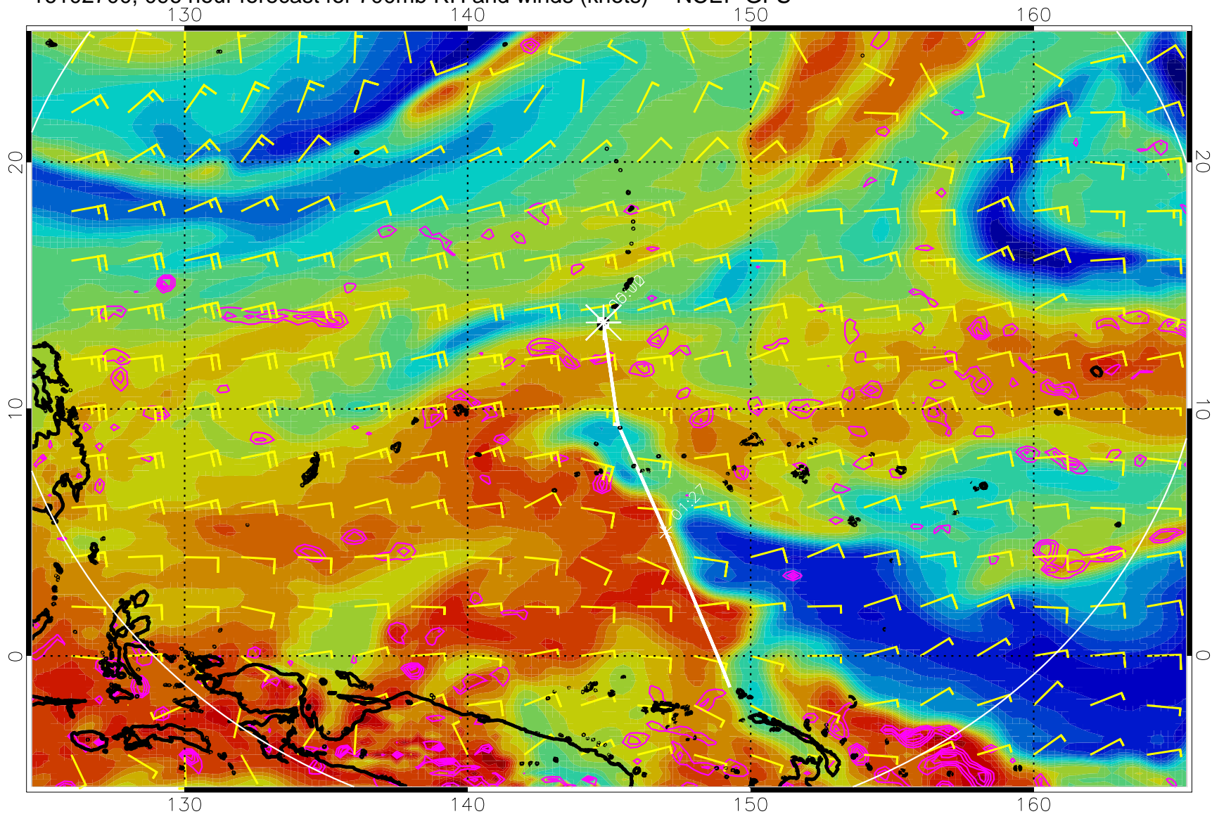
16102700, 096 hour forecast for 700mb RH and winds (knots) -- NCEP GFS
