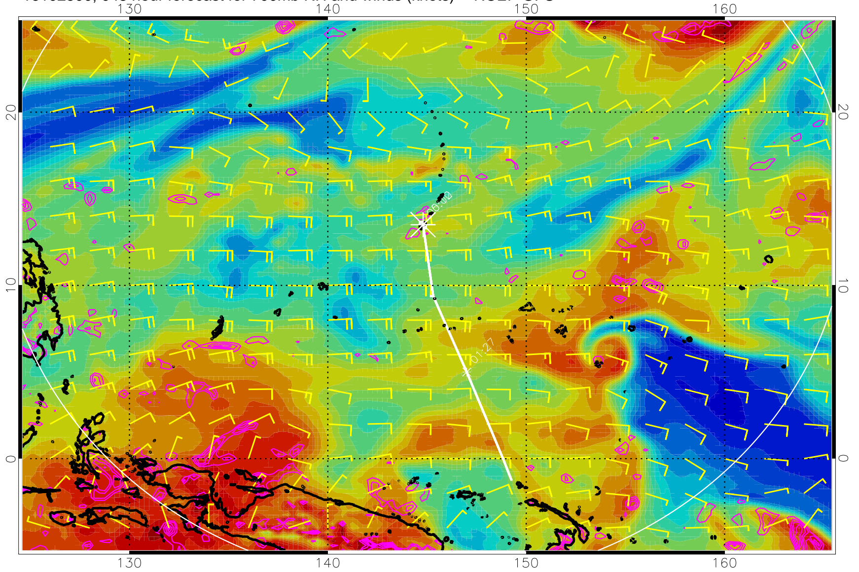
16102500, 048 hour forecast for 700mb RH and winds (knots) -- NCEP GFS
