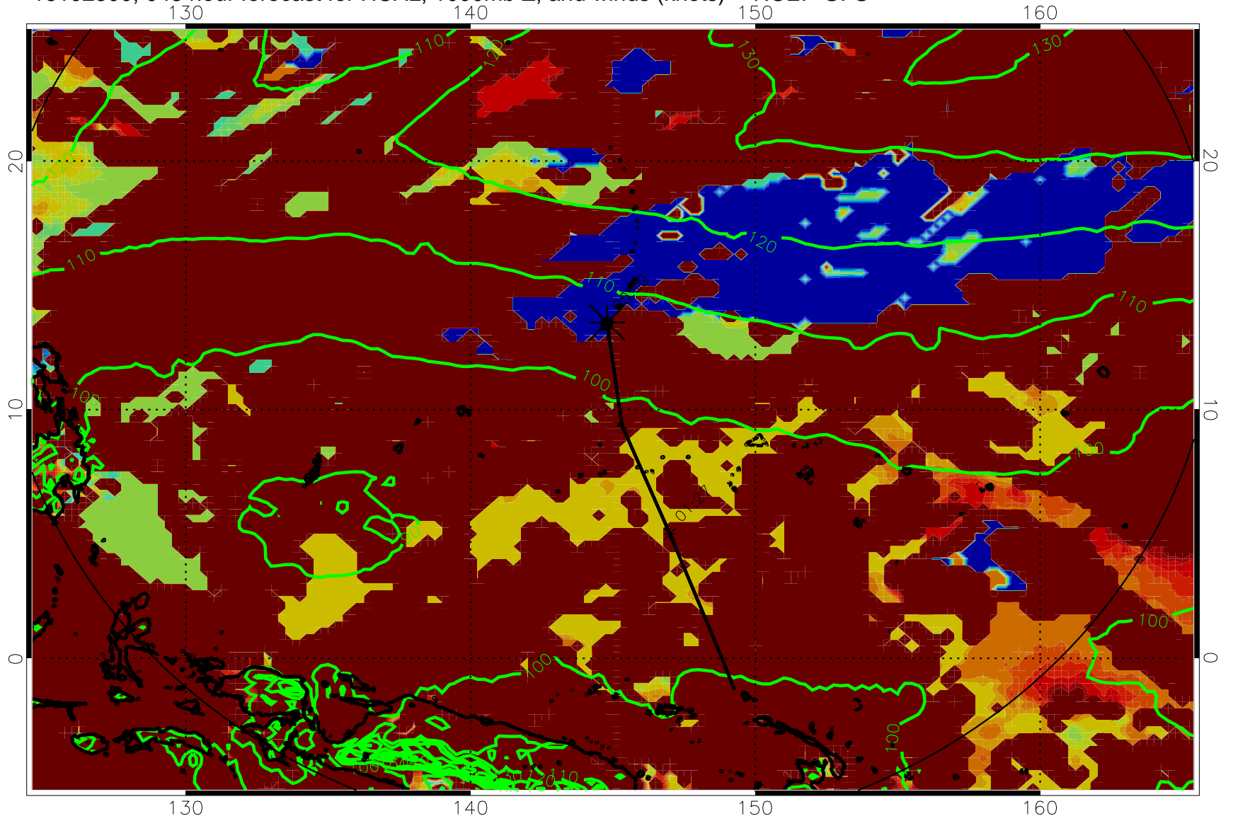
16102500, 048 hour forecast for HCAL, 1000mb Z, and winds (knots) -- NCEP GFS
