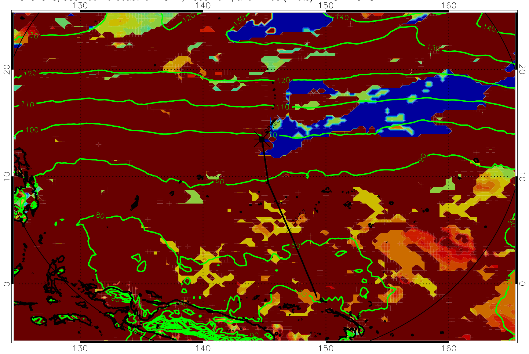
16102518, 066 hour forecast for HCAL, 1000mb Z, and winds (knots) -- NCEP GFS
