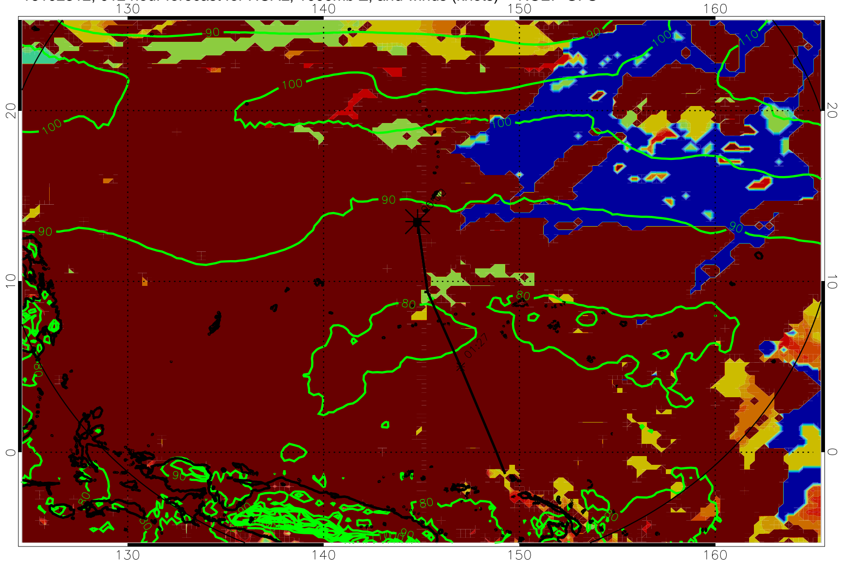
16102312, 012 hour forecast for HCAL, 1000mb Z, and winds (knots) -- NCEP GFS
