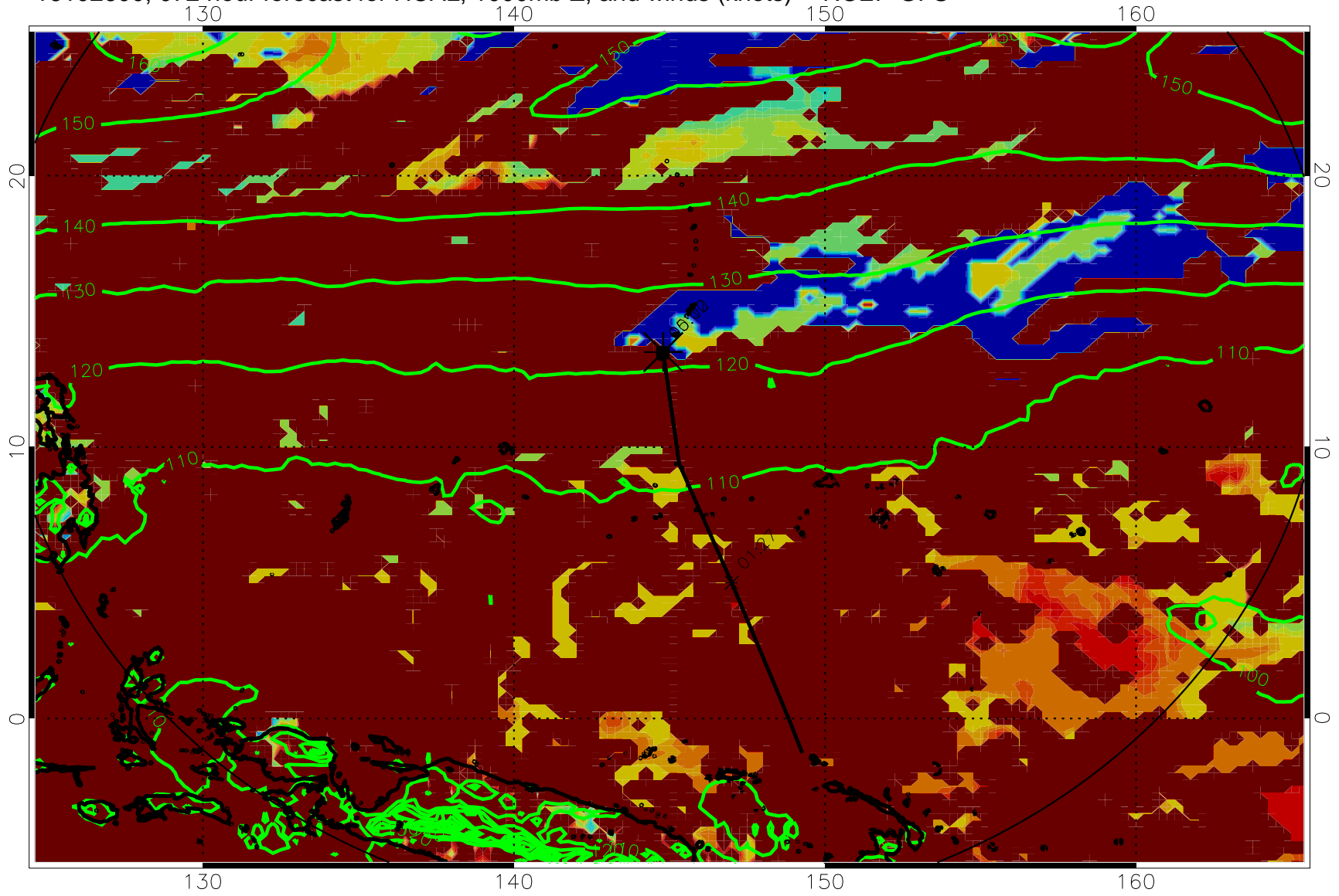
16102600, 072 hour forecast for HCAL, 1000mb Z, and winds (knots) -- NCEP GFS
