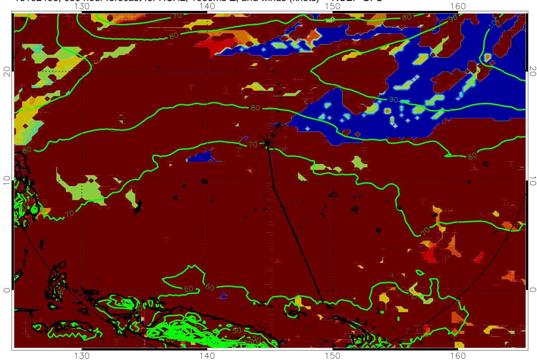
16102406, 0300 hour forecast for HCAL, 1000mb Z, and winds (knots) -- NCEP GFS
