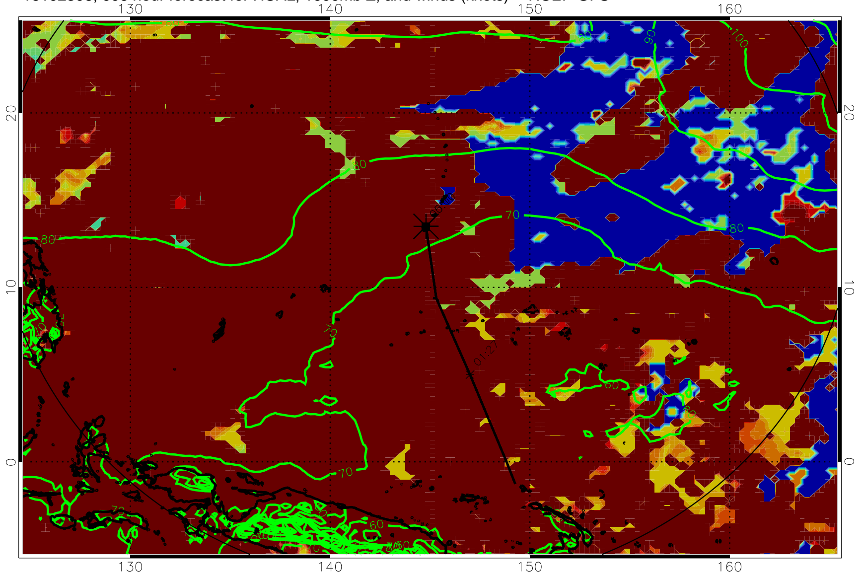
16102306, 006 hour forecast for HCAL, 1000mb Z, and winds (knots) -- NCEP GFS
