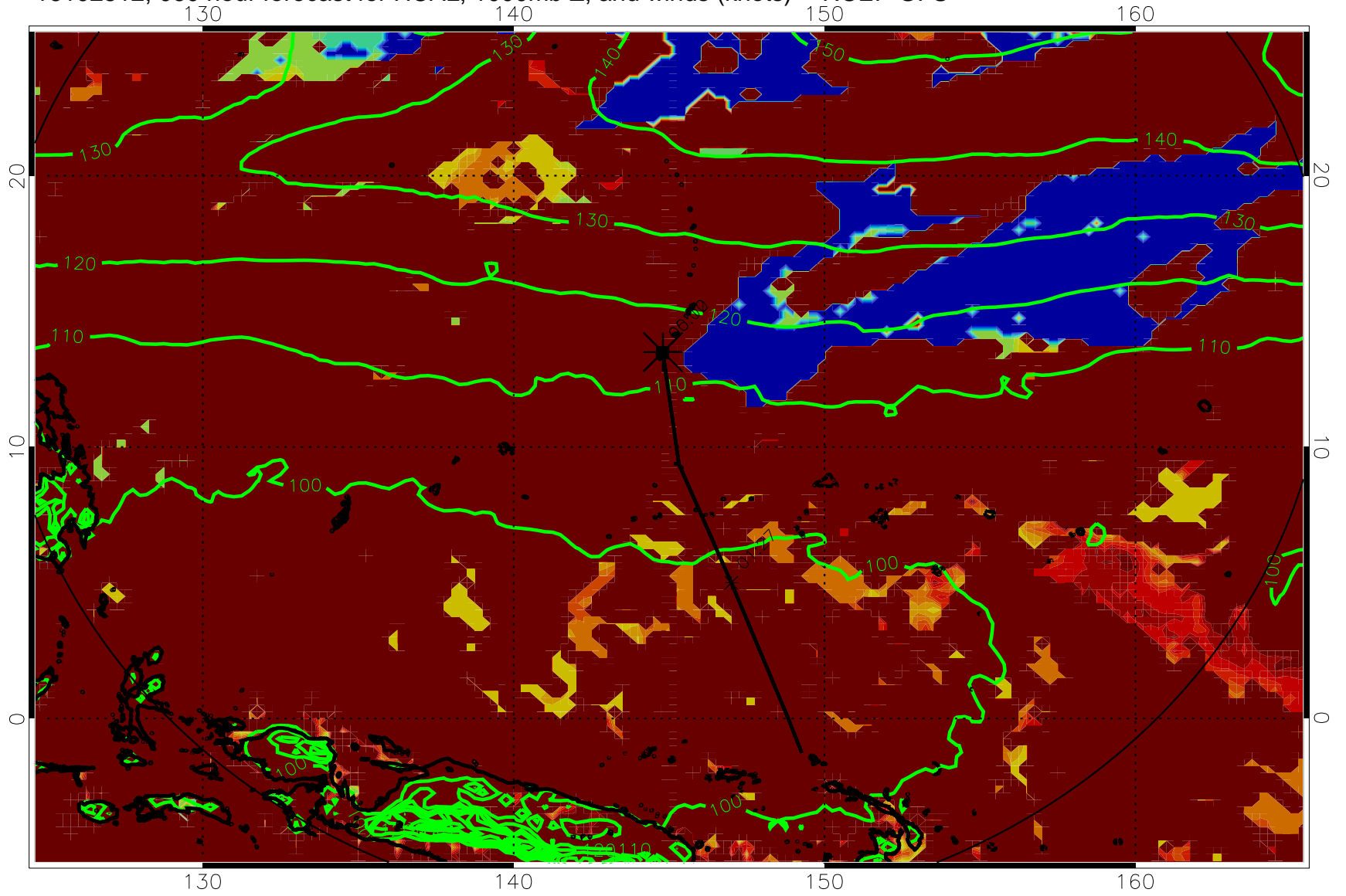
16102512, 060 hour forecast for HCAL, 1000mb Z, and winds (knots) -- NCEP GFS
