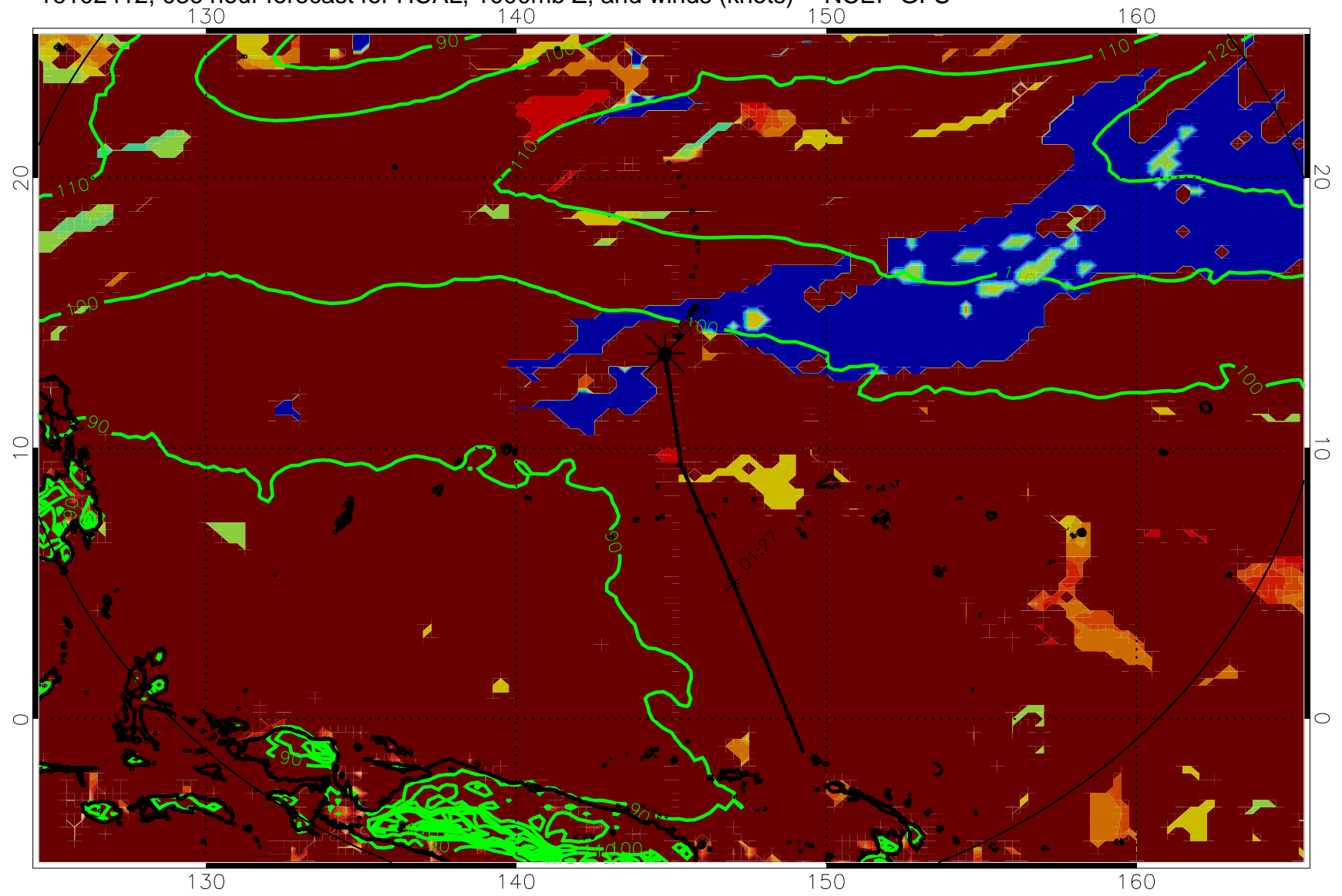
16102412, 036 hour forecast for HCAL, 1000mb Z, and winds (knots) -- NCEP GFS
