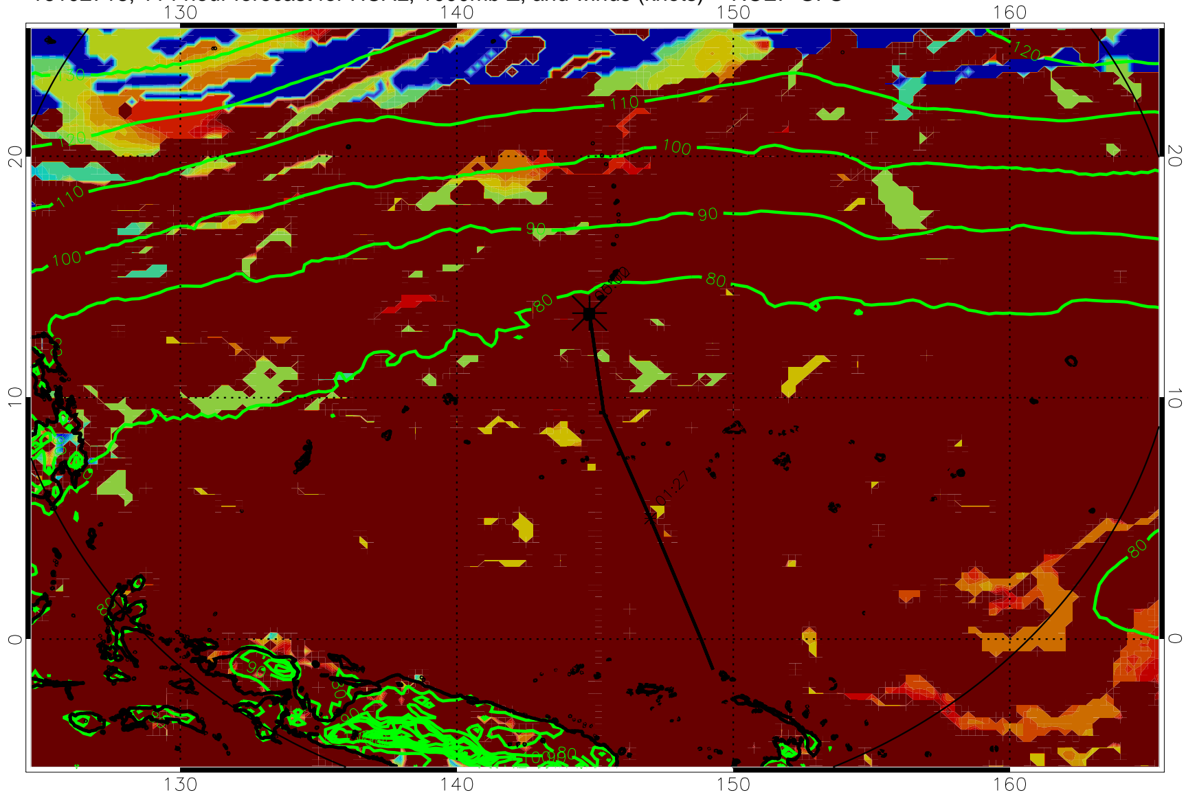
16102718, 114 hour forecast for HCAL, 1000mb Z, and winds (knots) -- NCEP GFS
