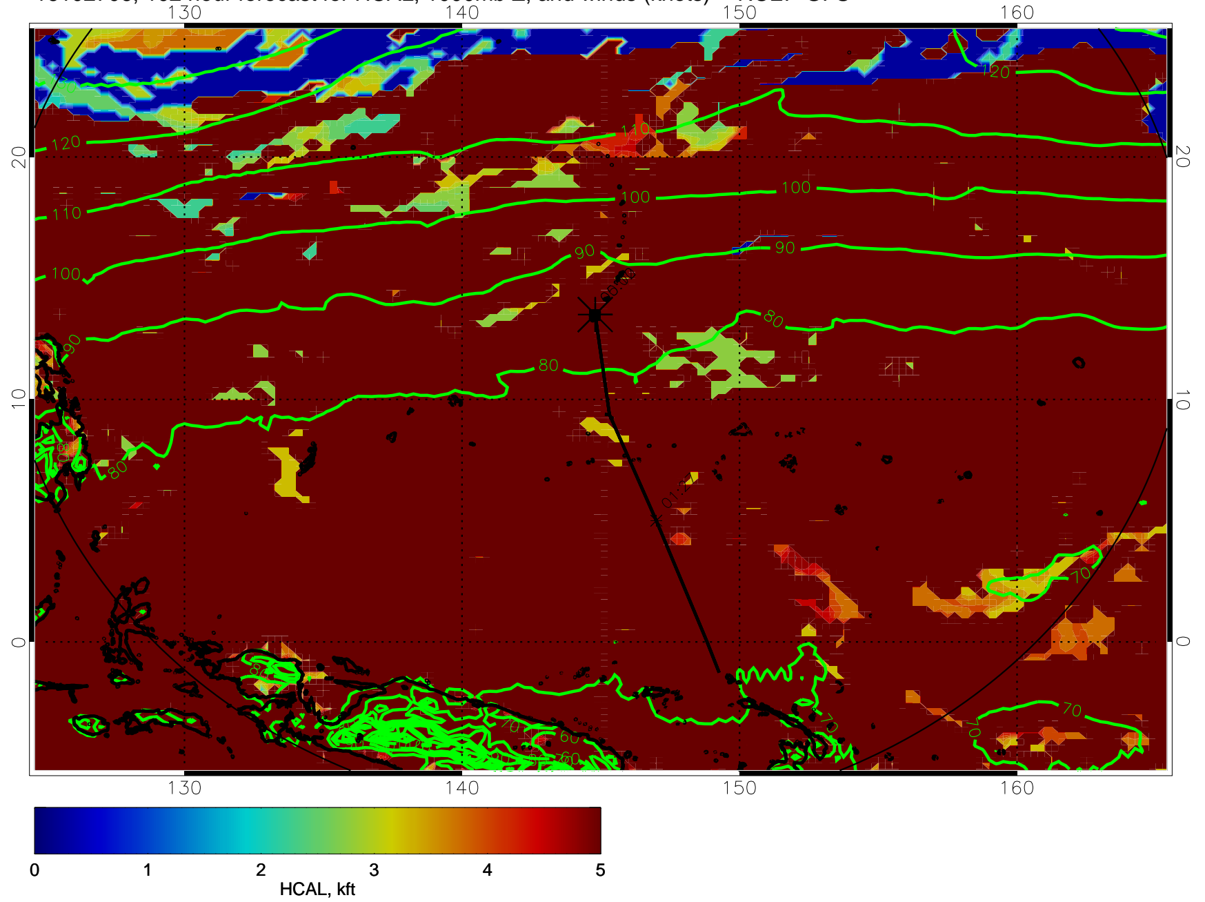
16102706, 102 hour forecast for HCAL, 1000mb Z, and winds (knots) -- NCEP GFS
