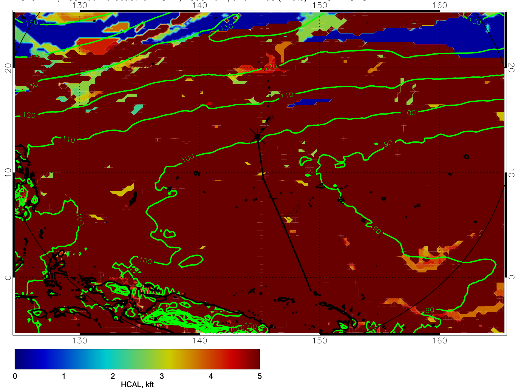
16102712, 108 hour forecast for HCAL, 1000mb Z, and winds (knots) -- NCEP GFS
