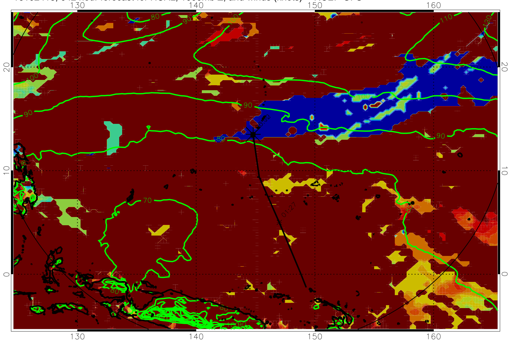
16102418, 042 hour forecast for HCAL, 1000mb Z, and winds (knots) -- NCEP GFS
