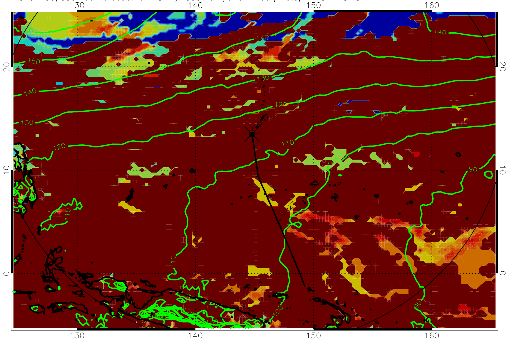
16102700, 096 hour forecast for HCAL, 1000mb Z, and winds (knots) -- NCEP GFS
