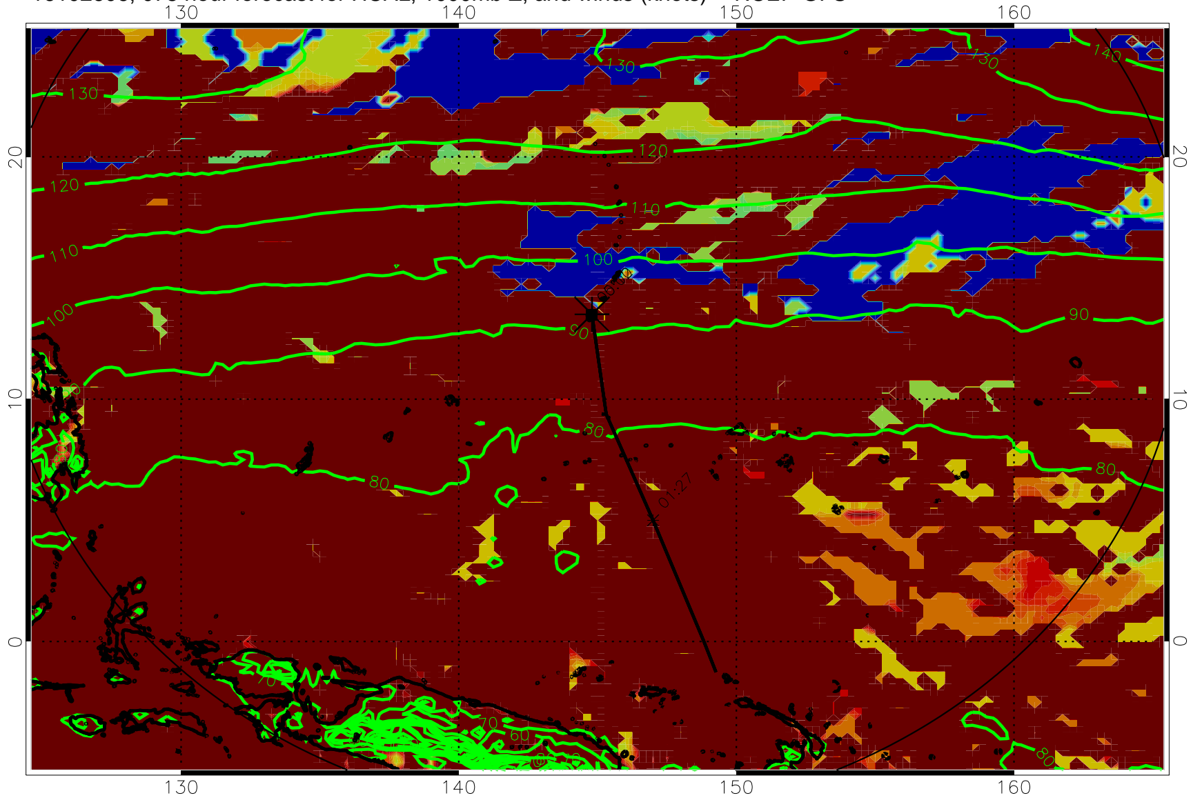
16102606, 078 hour forecast for HCAL, 1000mb Z, and winds (knots) -- NCEP GFS
