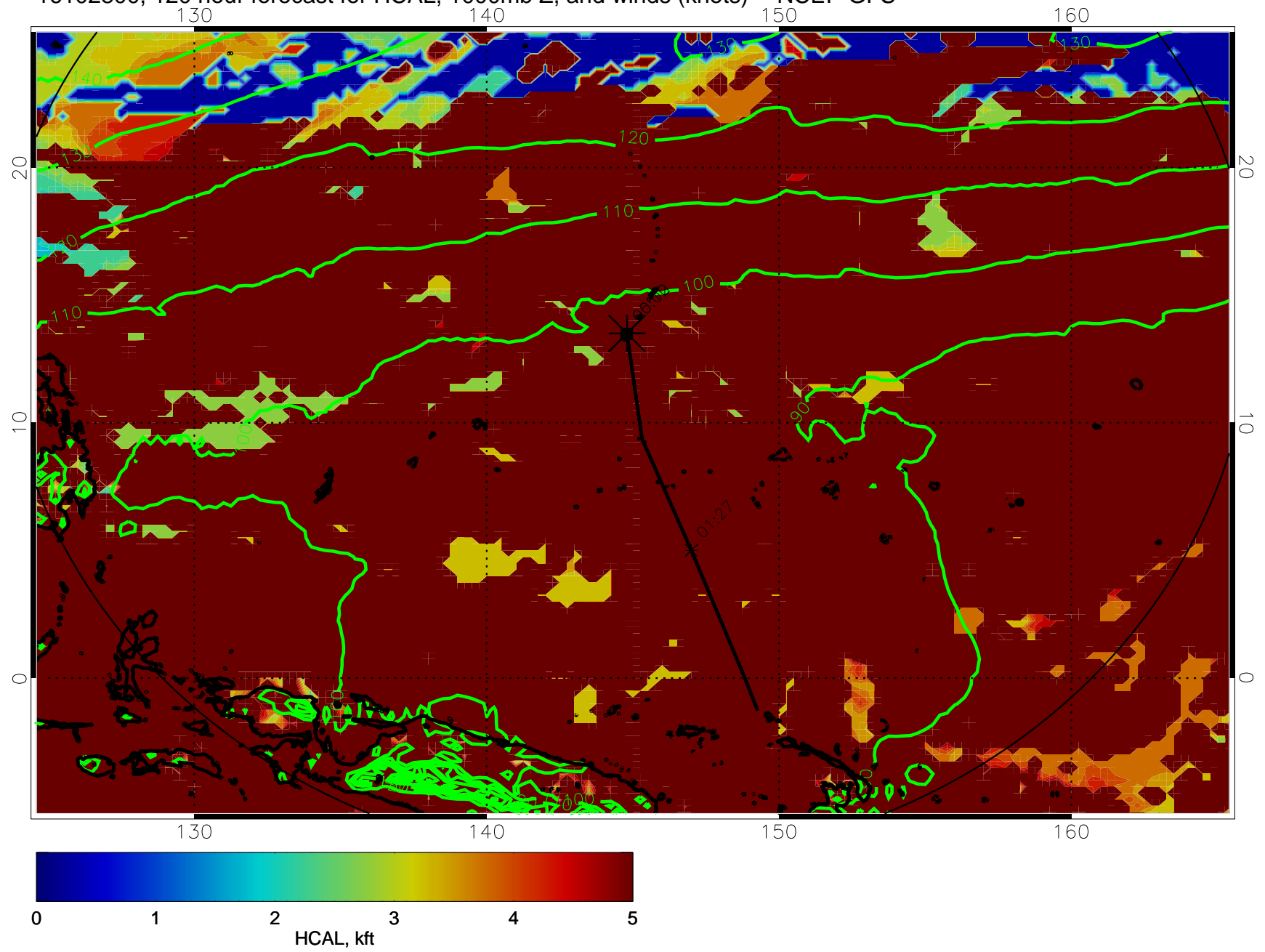
16102800, 120 hour forecast for HCAL, 1000mb Z, and winds (knots) -- NCEP GFS
