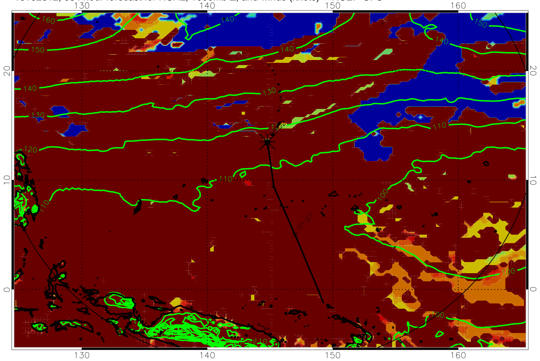
16102612, 084 hour forecast for HCAL, 1000mb Z, and winds (knots) -- NCEP GFS
