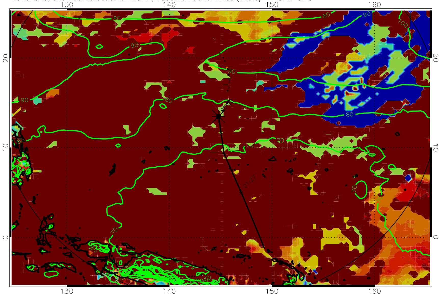
16102318, 018 hour forecast for HCAL, 1000mb Z, and winds (knots) -- NCEP GFS
