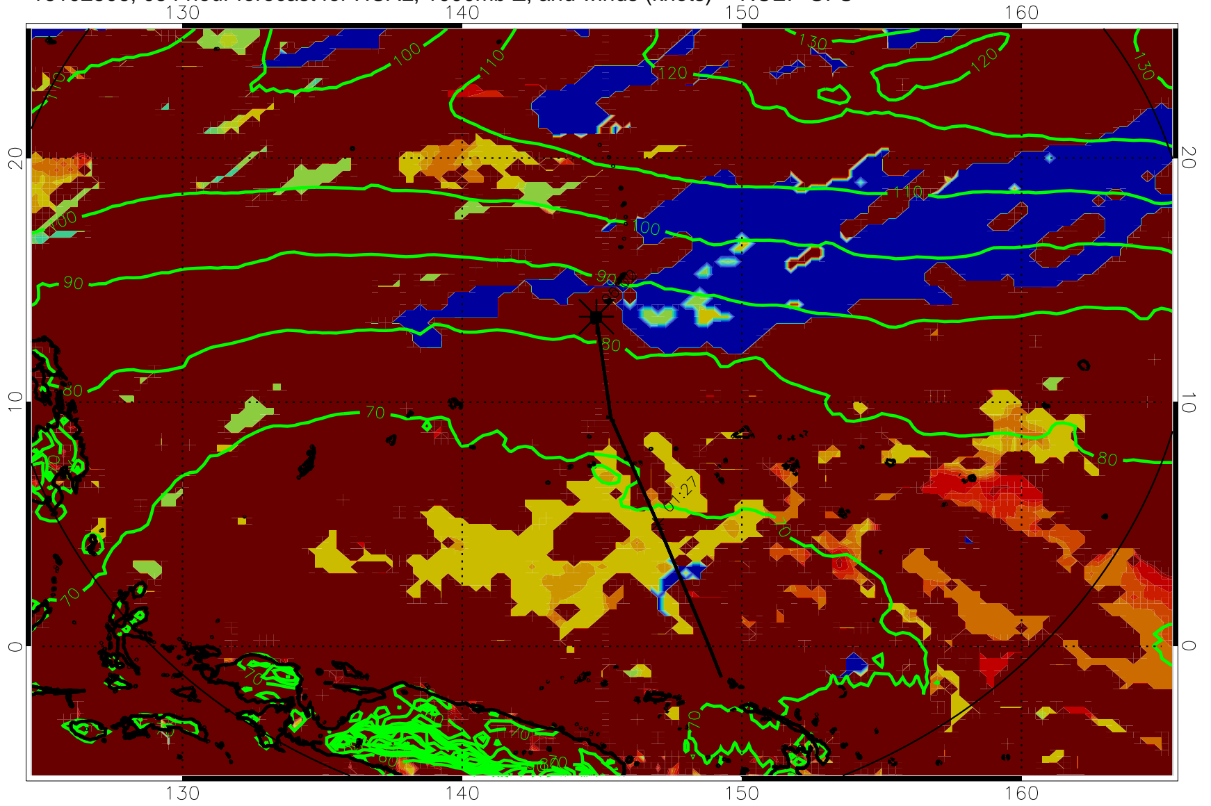
16102506, 054 hour forecast for HCAL, 1000mb Z, and winds (knots) -- NCEP GFS
