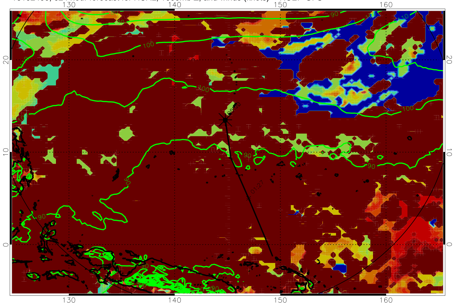
16102400, 024 hour forecast for HCAL, 1000mb Z, and winds (knots) -- NCEP GFS
