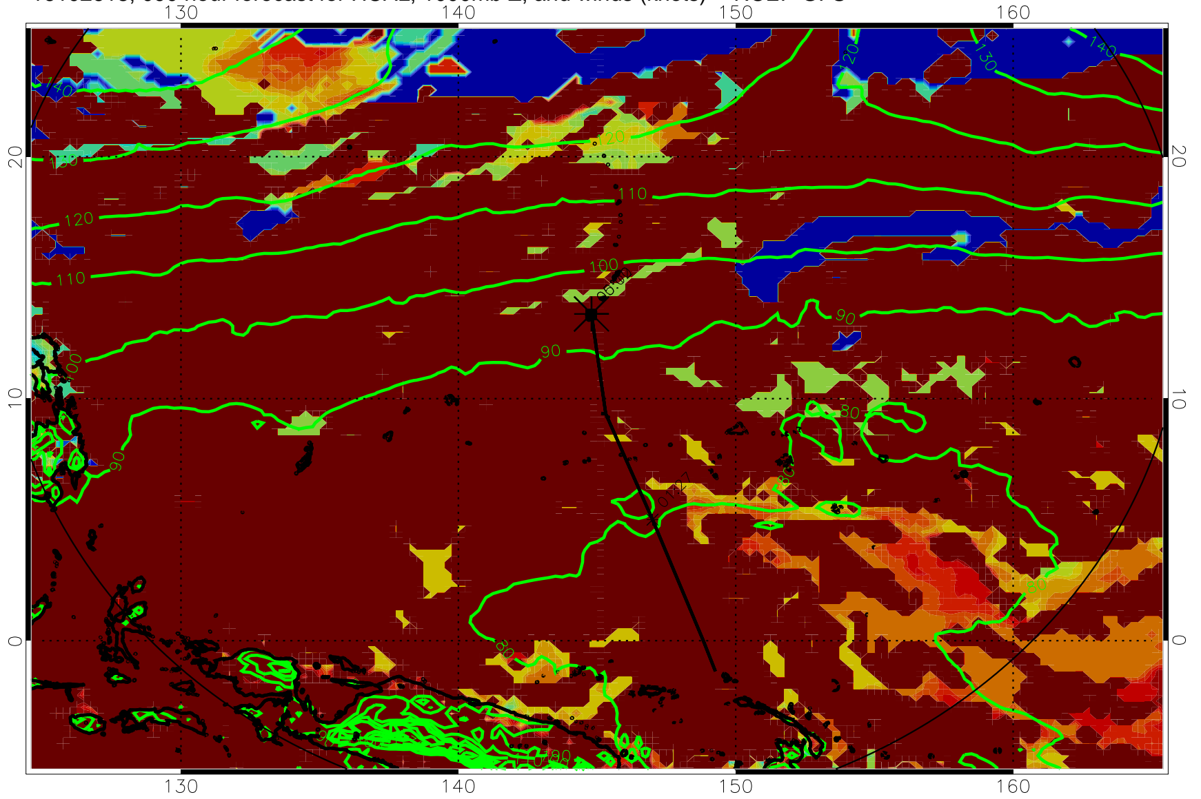
16102618, 090 hour forecast for HCAL, 1000mb Z, and winds (knots) -- NCEP GFS
