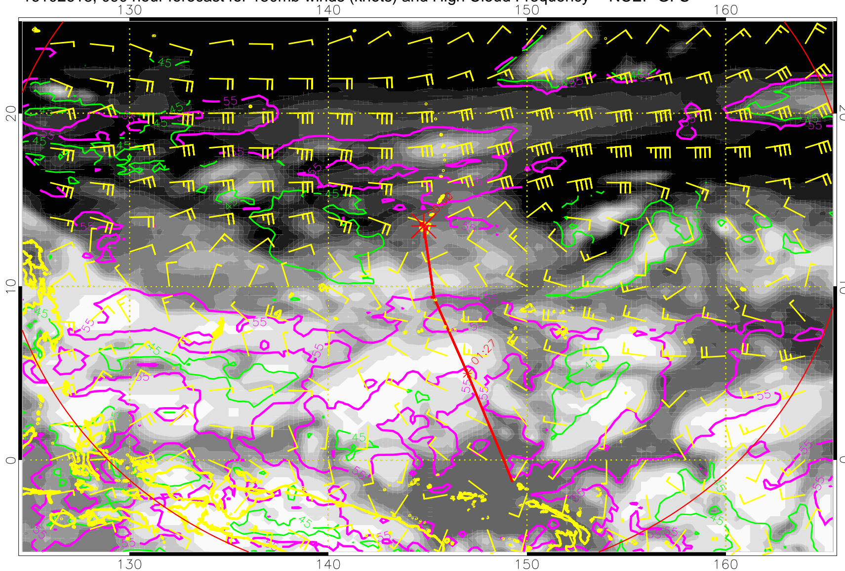
16102618, 090 hour forecast for 150mb winds (knots) and High Cloud Frequency -- NCEP GFS
