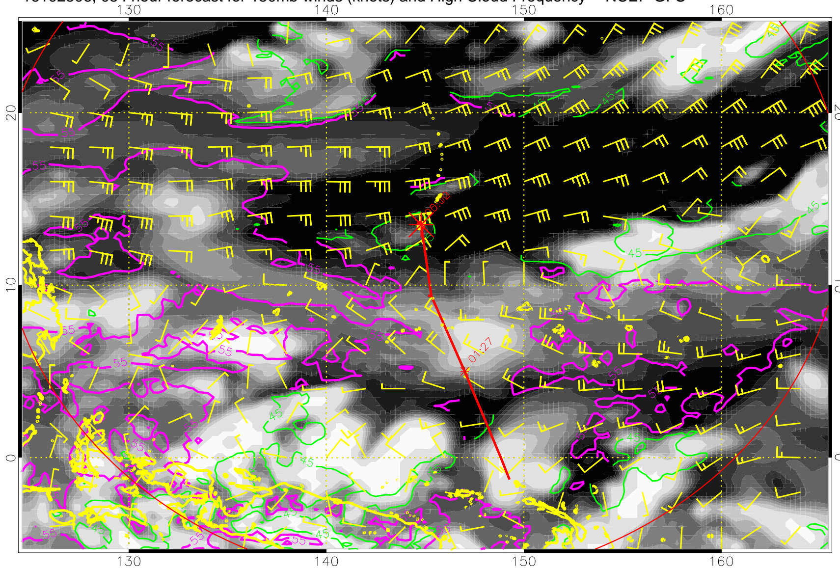
16102506, 054 hour forecast for 150mb winds (knots) and High Cloud Frequency -- NCEP GFS
