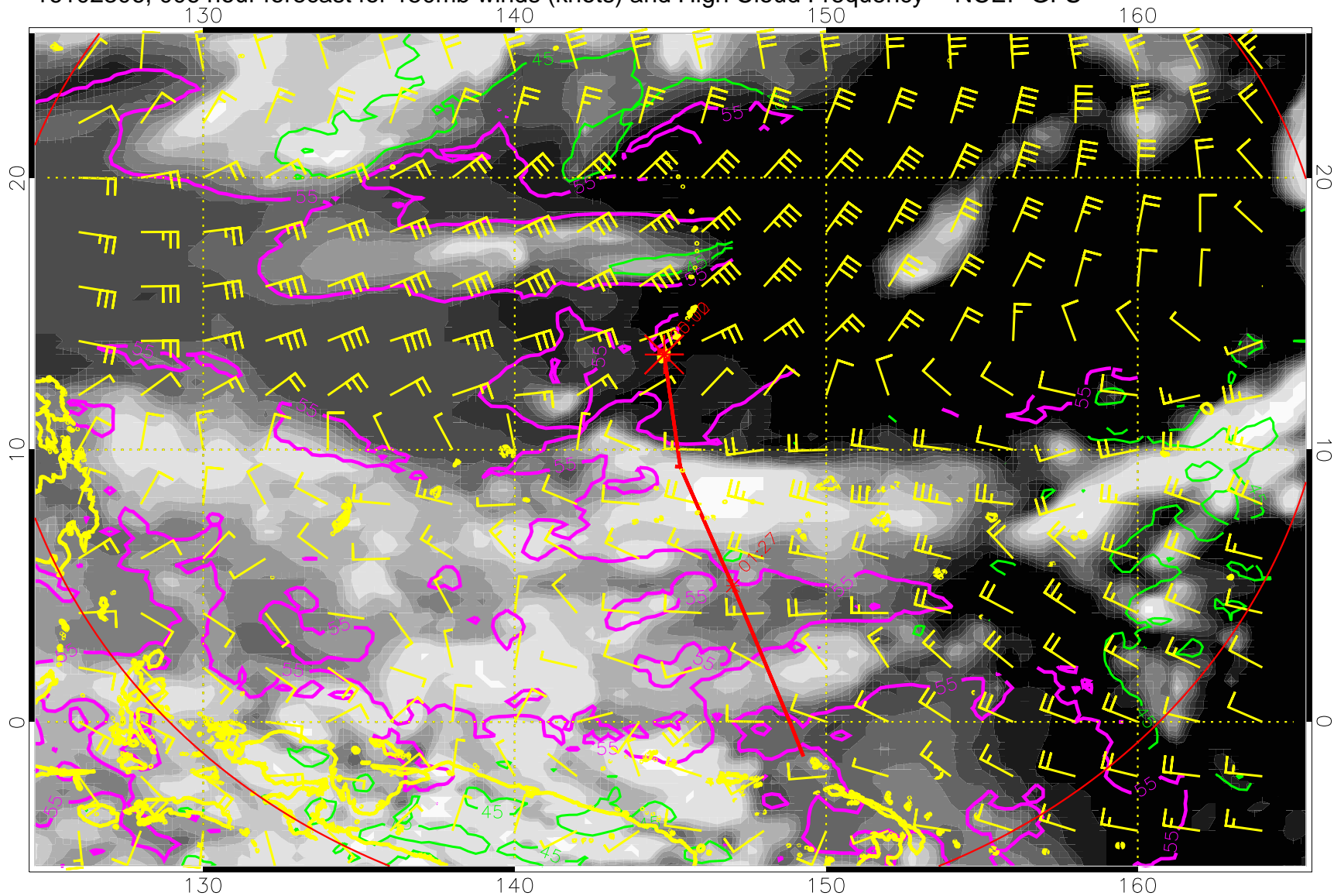
16102306, 006 hour forecast for 150mb winds (knots) and High Cloud Frequency -- NCEP GFS
