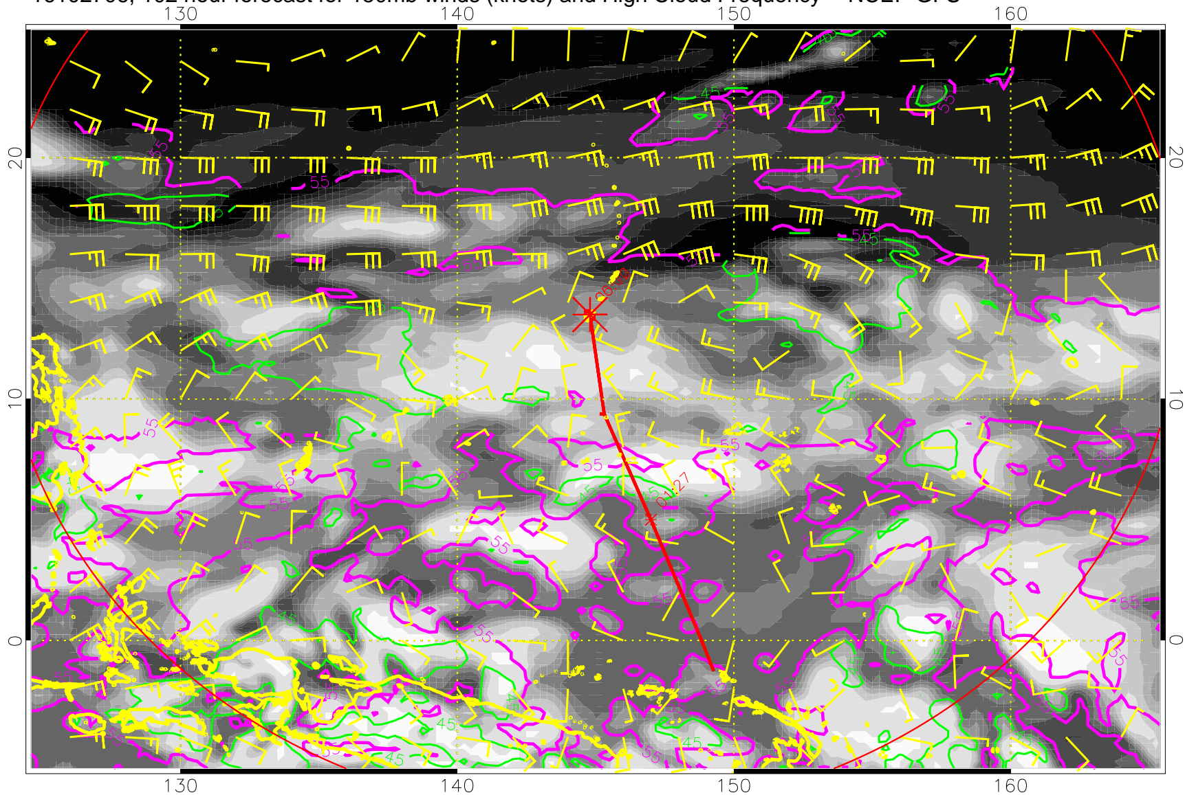
16102706, 102 hour forecast for 150mb winds (knots) and High Cloud Frequency -- NCEP GFS
