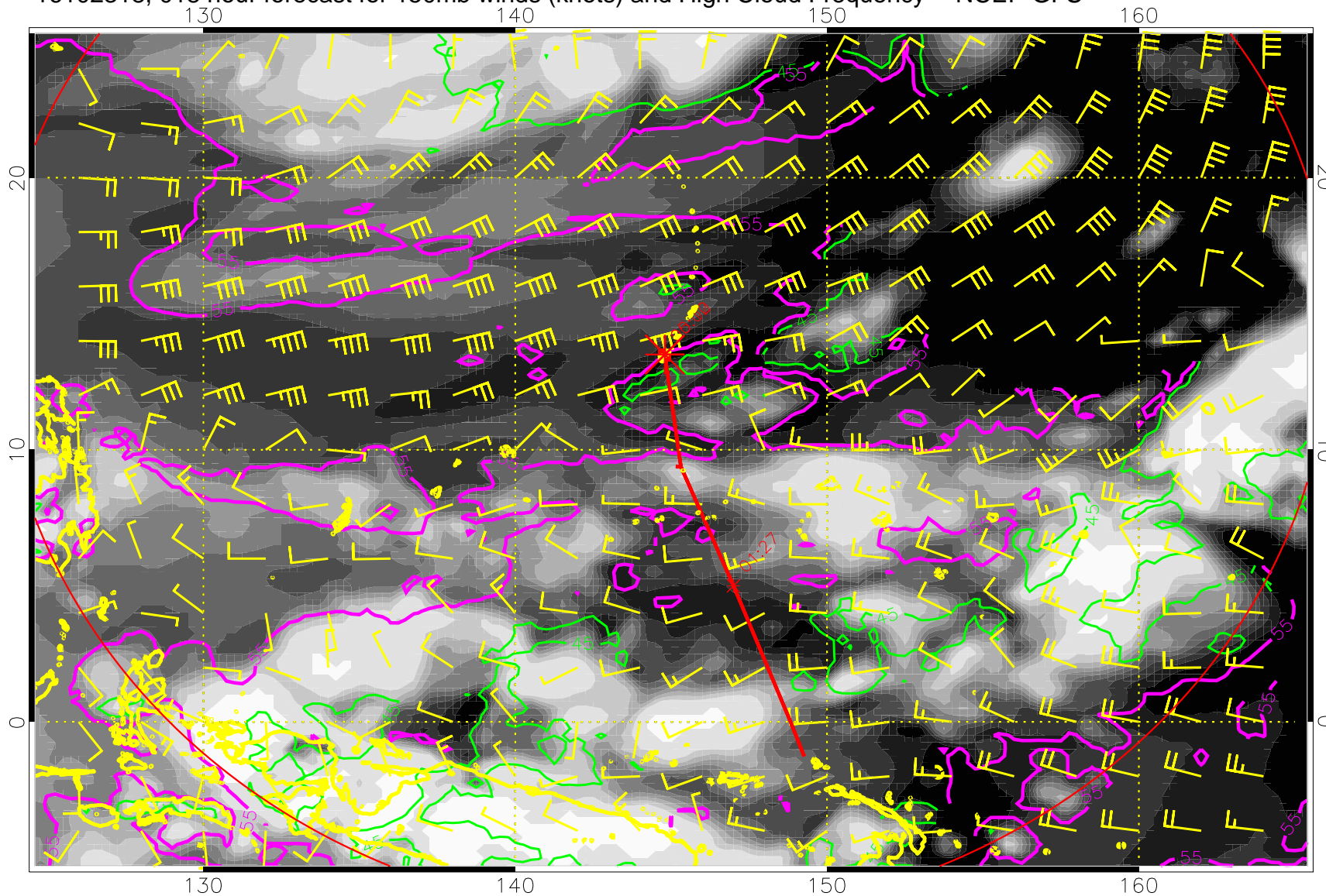
16102318, 018 hour forecast for 150mb winds (knots) and High Cloud Frequency -- NCEP GFS
