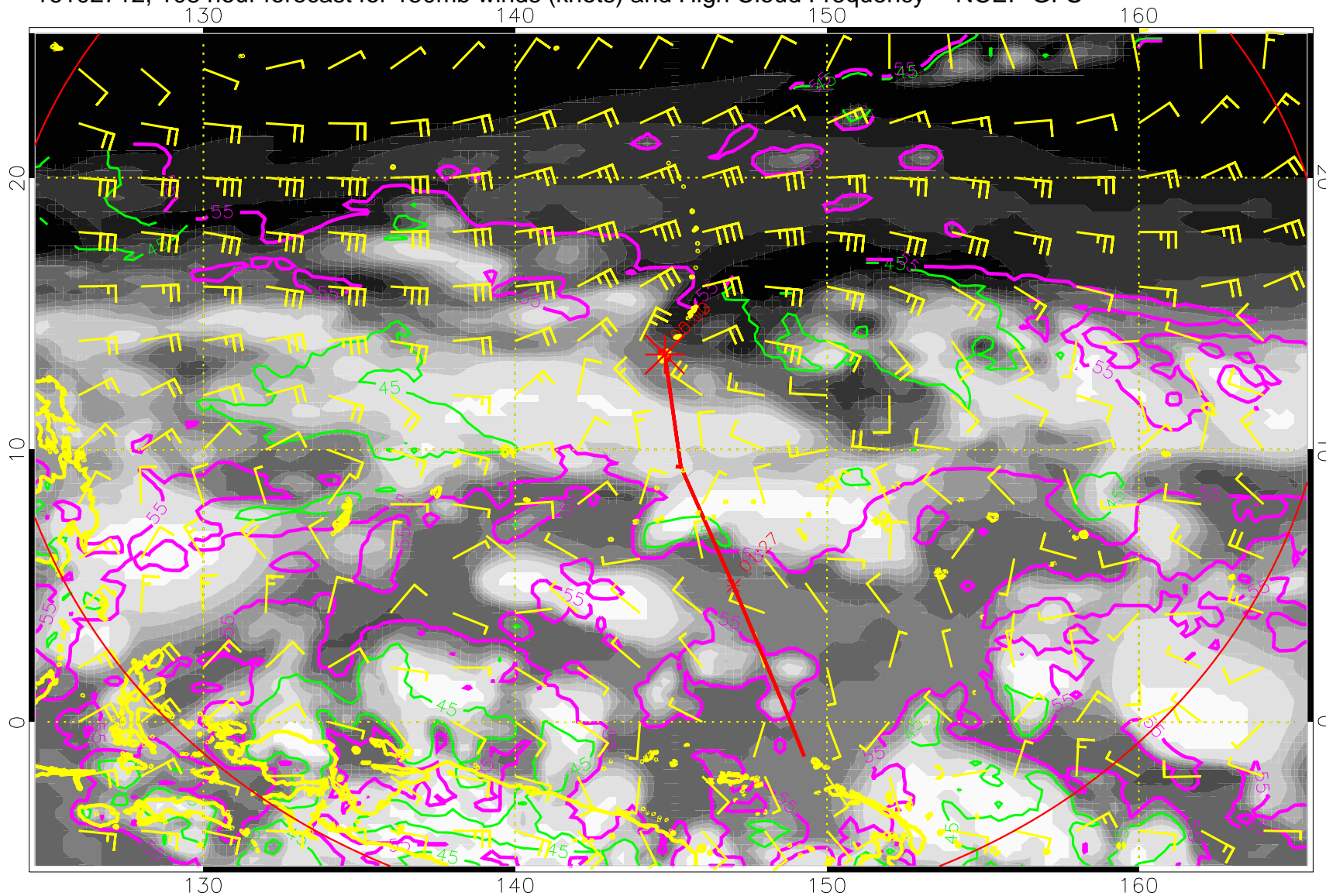
16102712, 108 hour forecast for 150mb winds (knots) and High Cloud Frequency -- NCEP GFS
