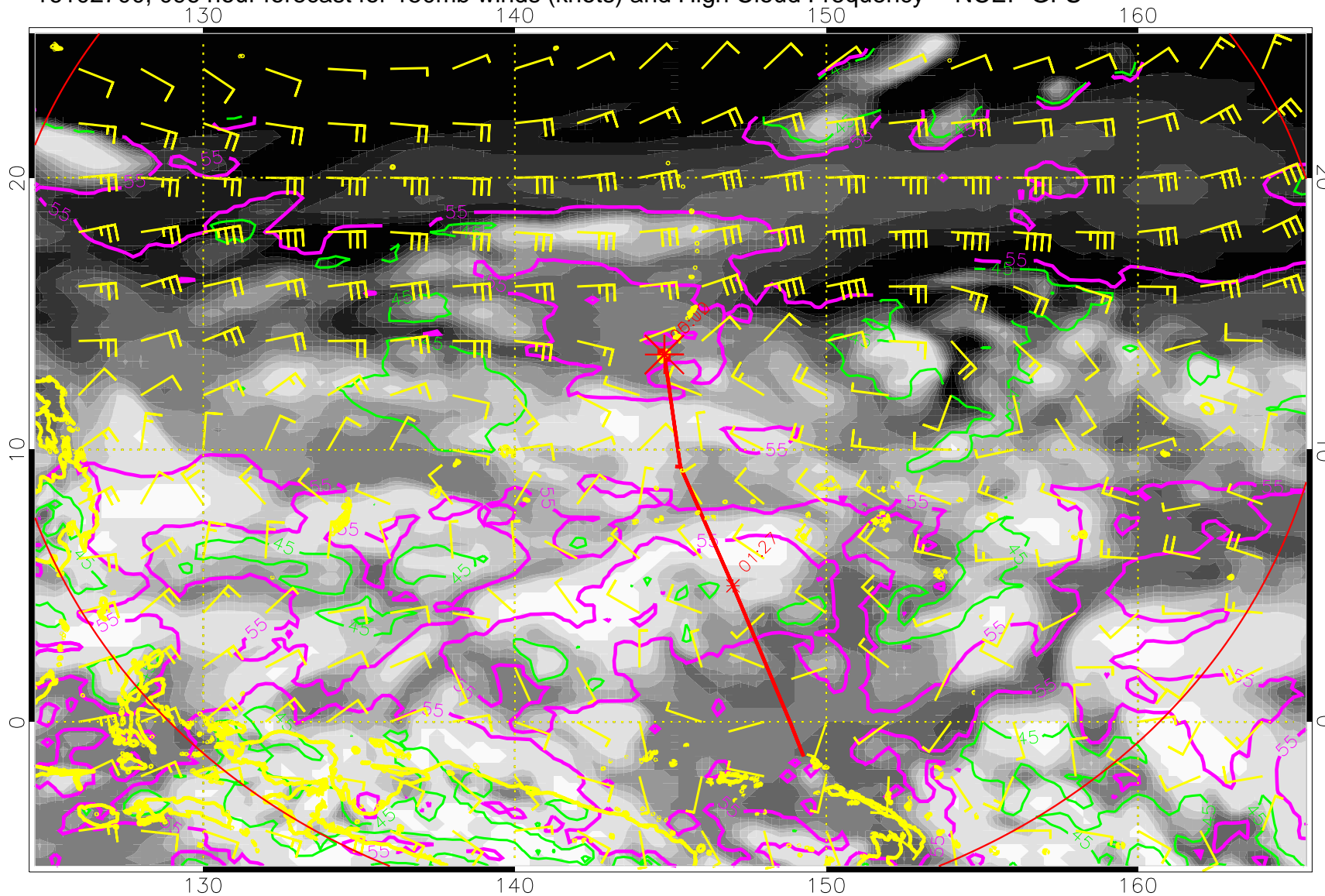
16102700, 096 hour forecast for 150mb winds (knots) and High Cloud Frequency -- NCEP GFS
