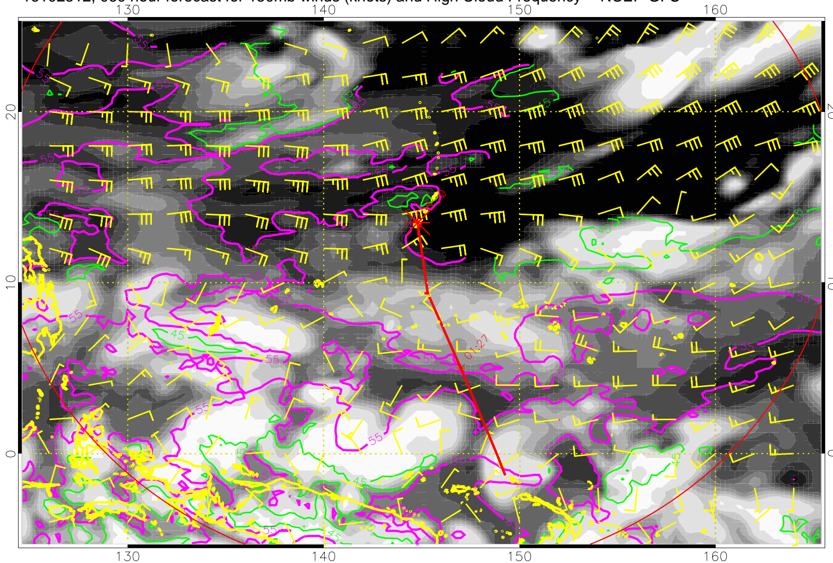
16102512, 060 hour forecast for 150mb winds (knots) and High Cloud Frequency -- NCEP GFS
