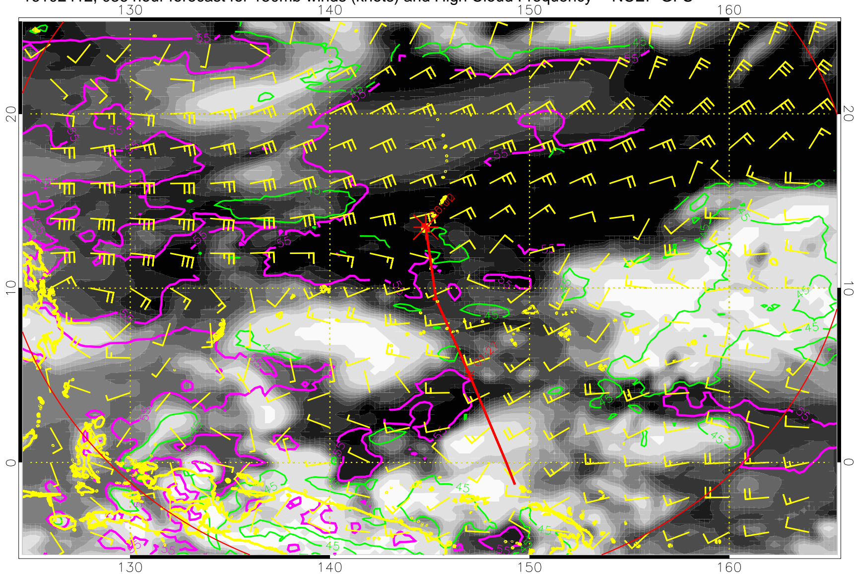
16102412, 036 hour forecast for 150mb winds (knots) and High Cloud Frequency -- NCEP GFS
