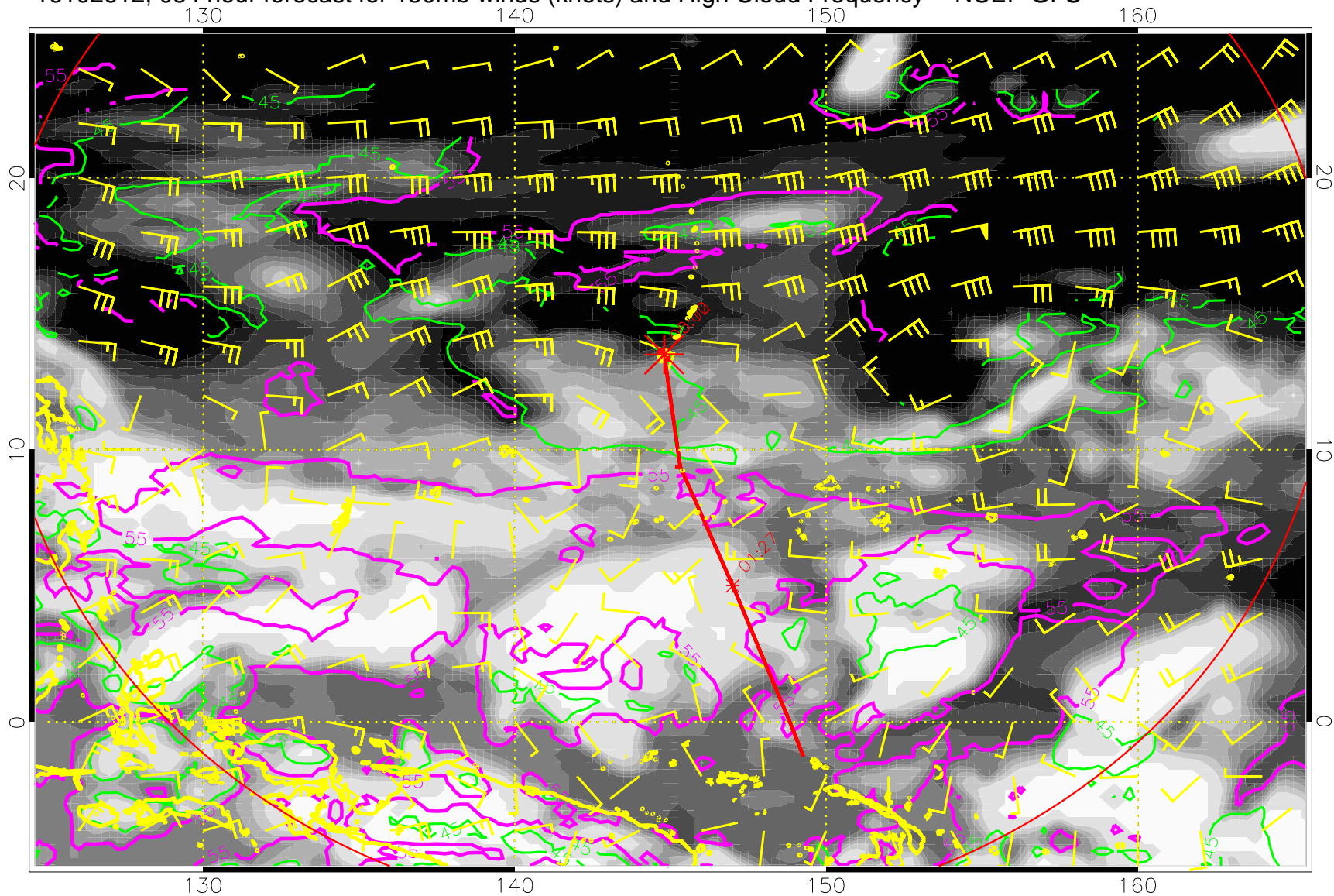
16102612, 084 hour forecast for 150mb winds (knots) and High Cloud Frequency -- NCEP GFS
