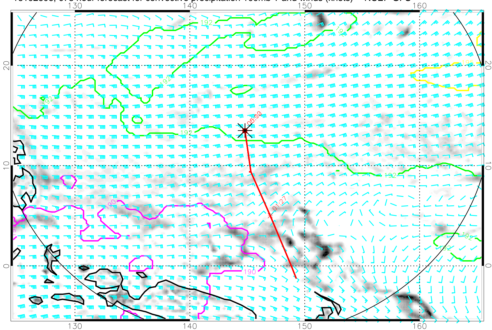
16102606, 078 hour forecast for convective precipitation 100mb T and winds (knots) -- NCEP GFS
