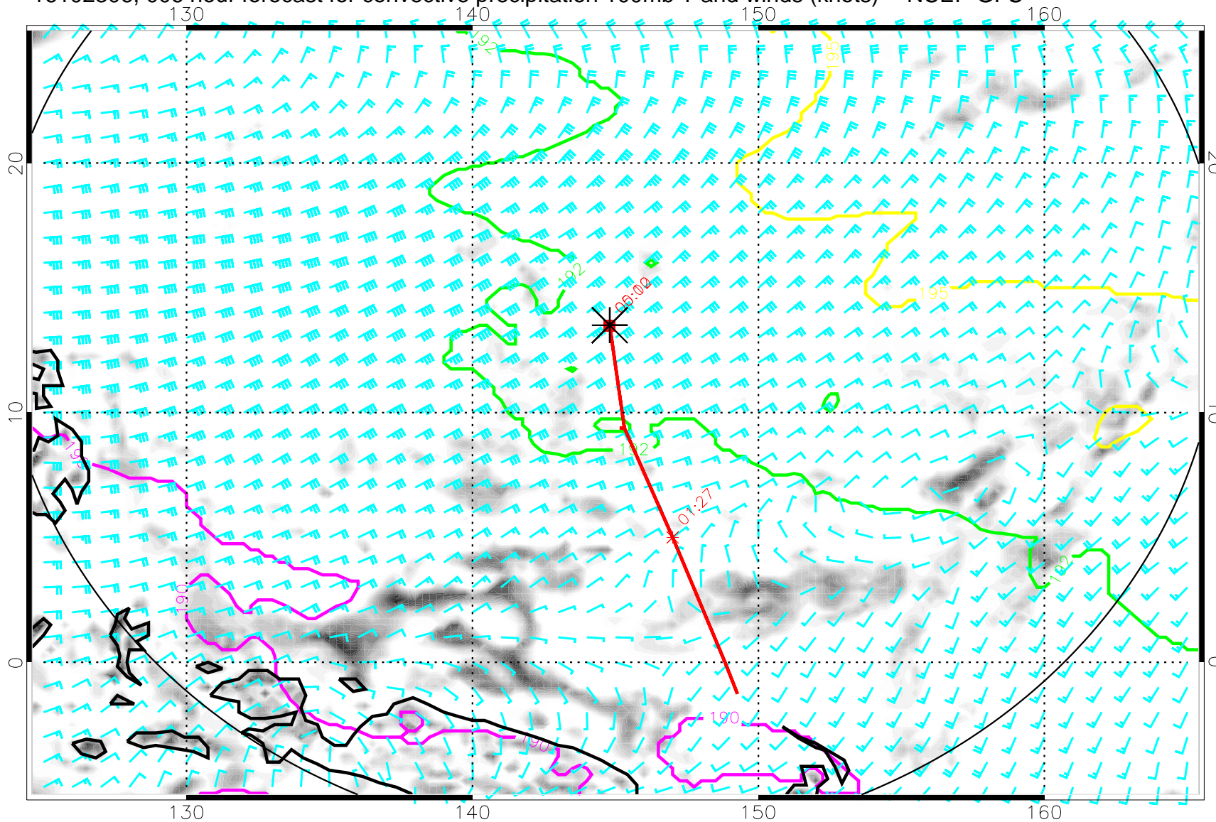
16102306, 006 hour forecast for convective precipitation 100mb T and winds (knots) -- NCEP GFS
