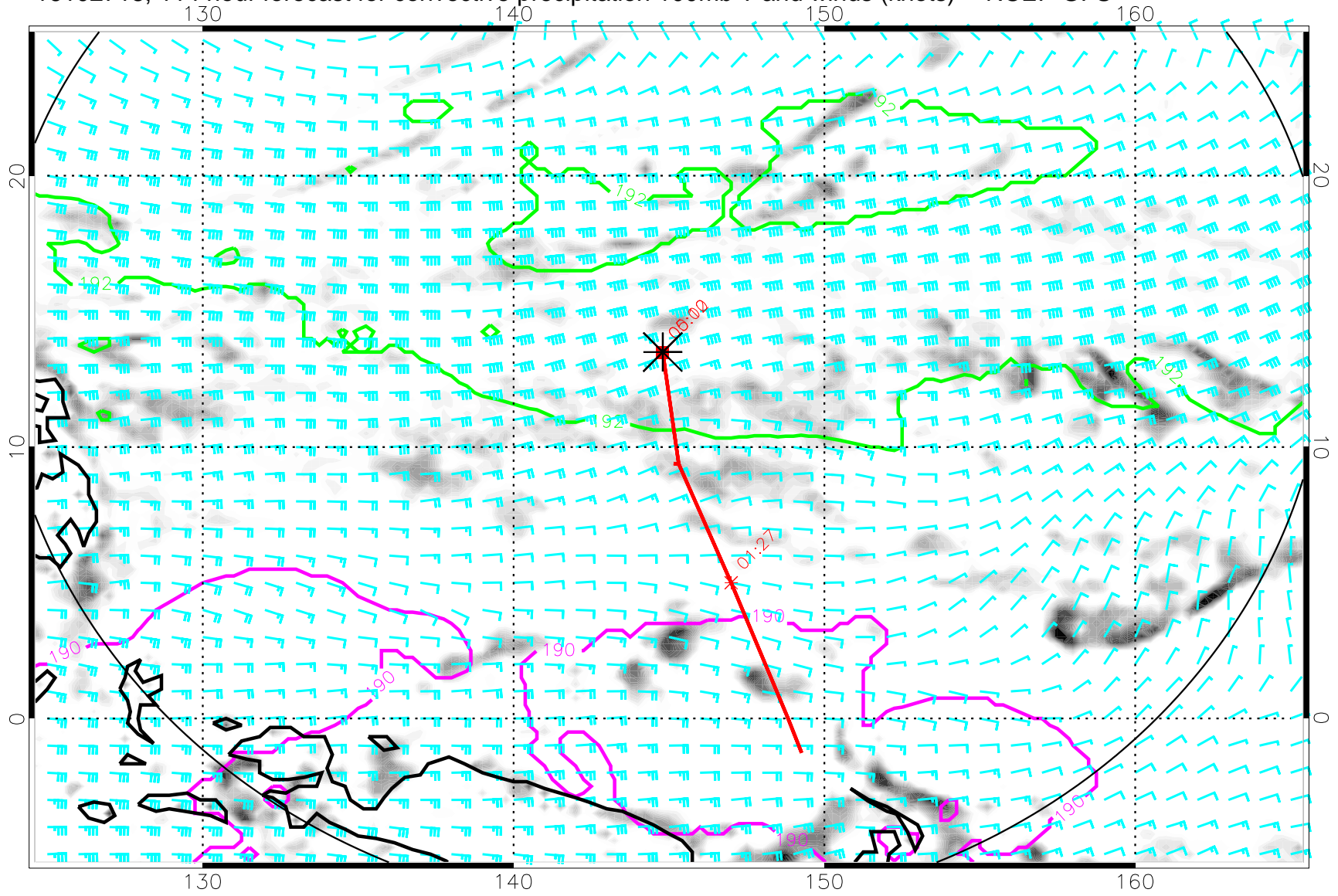
16102718, 114 hour forecast for convective precipitation 100mb T and winds (knots) -- NCEP GFS
