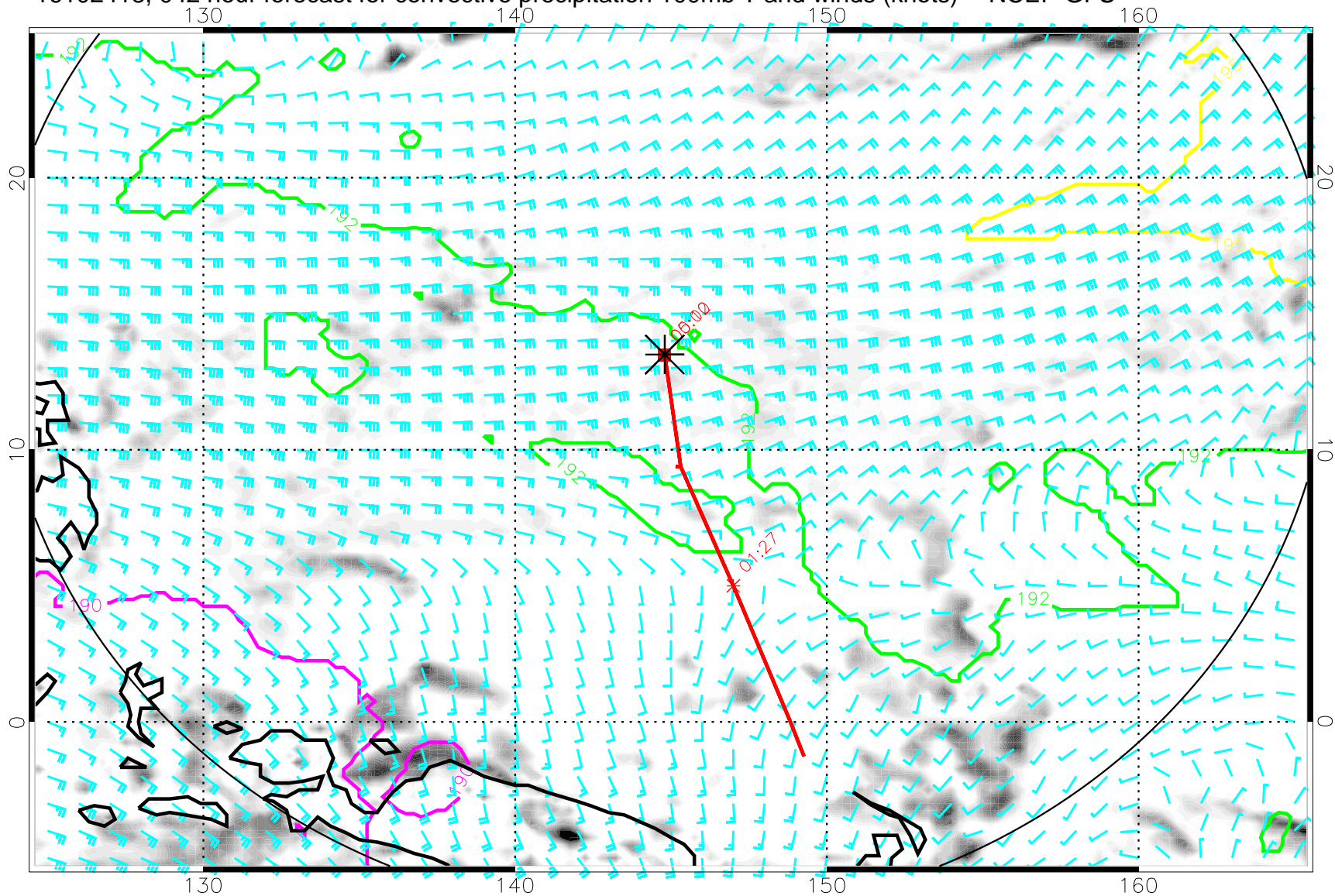
16102418, 04Z hour forecast for convective precipitation 100mb T and winds (knots) -- NCEP GFS
