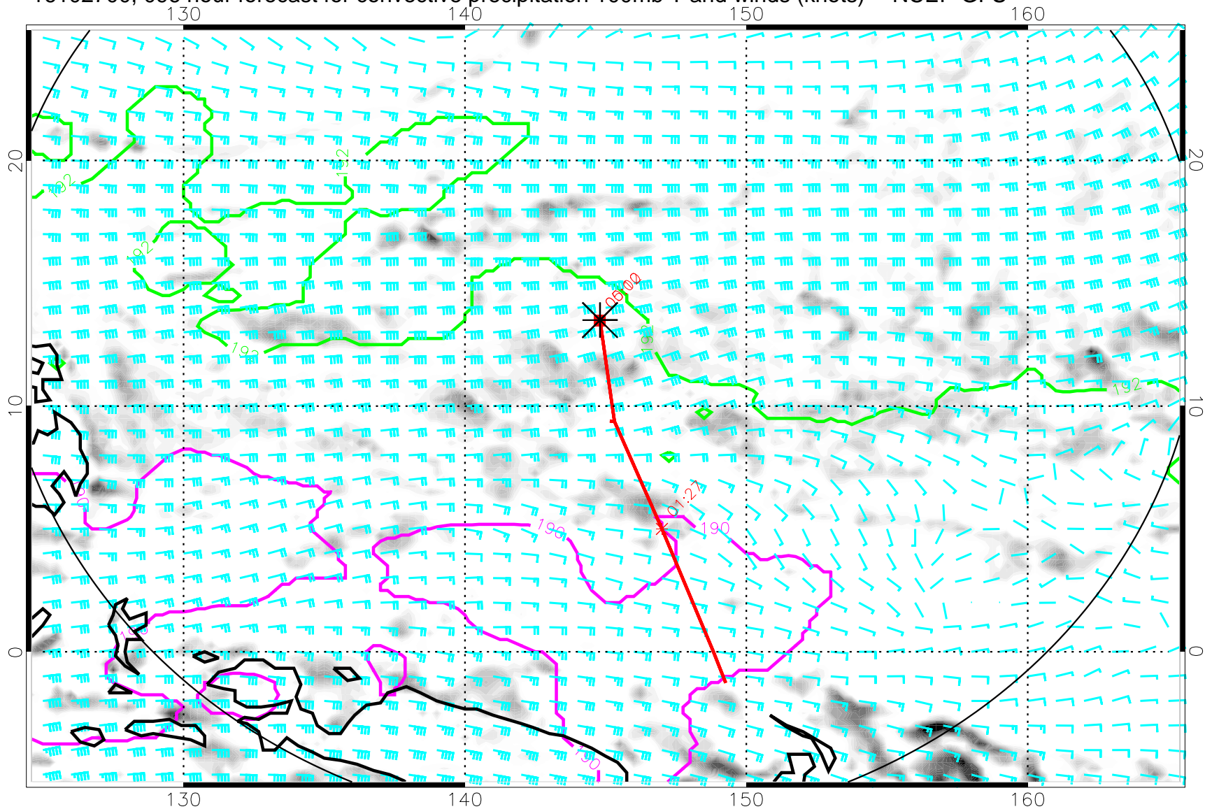
16102700, 096 hour forecast for convective precipitation 100mb T and winds (knots) -- NCEP GFS
