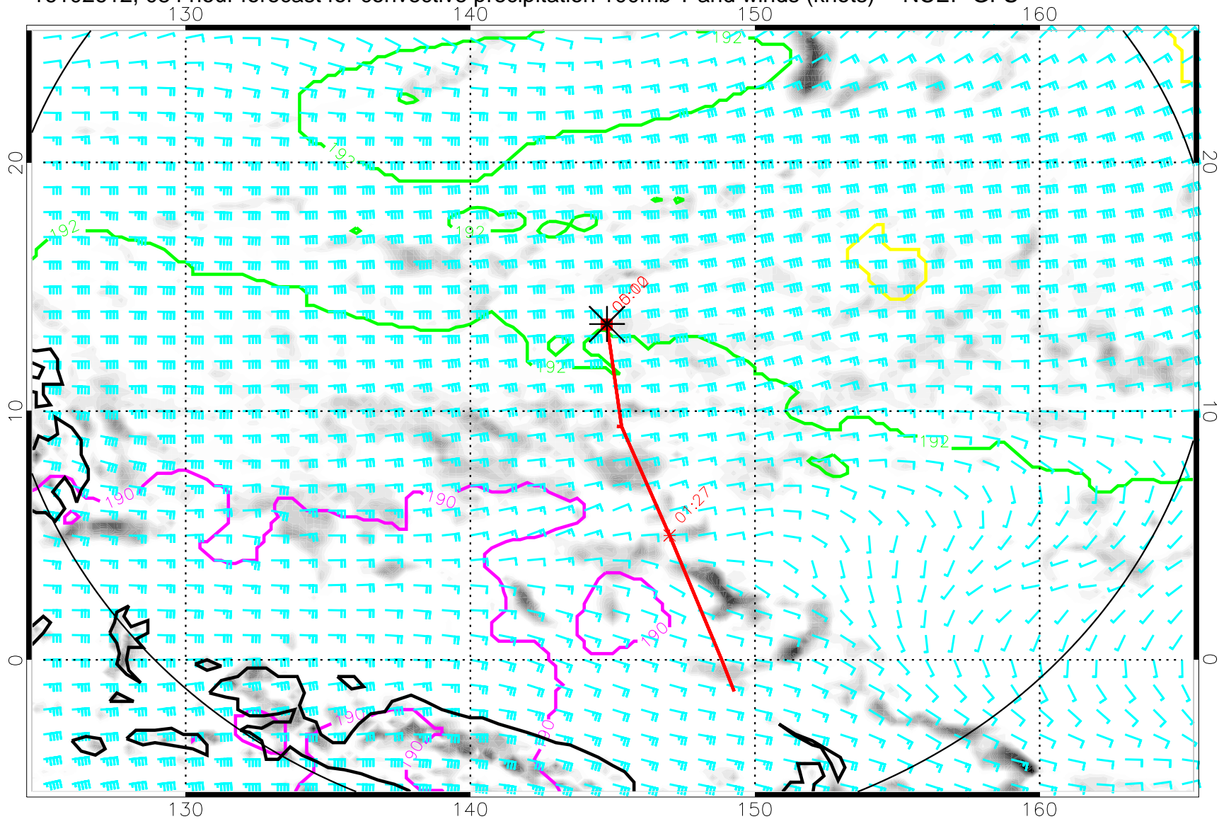
16102612, 084 hour forecast for convective precipitation 100mb T and winds (knots) -- NCEP GFS
