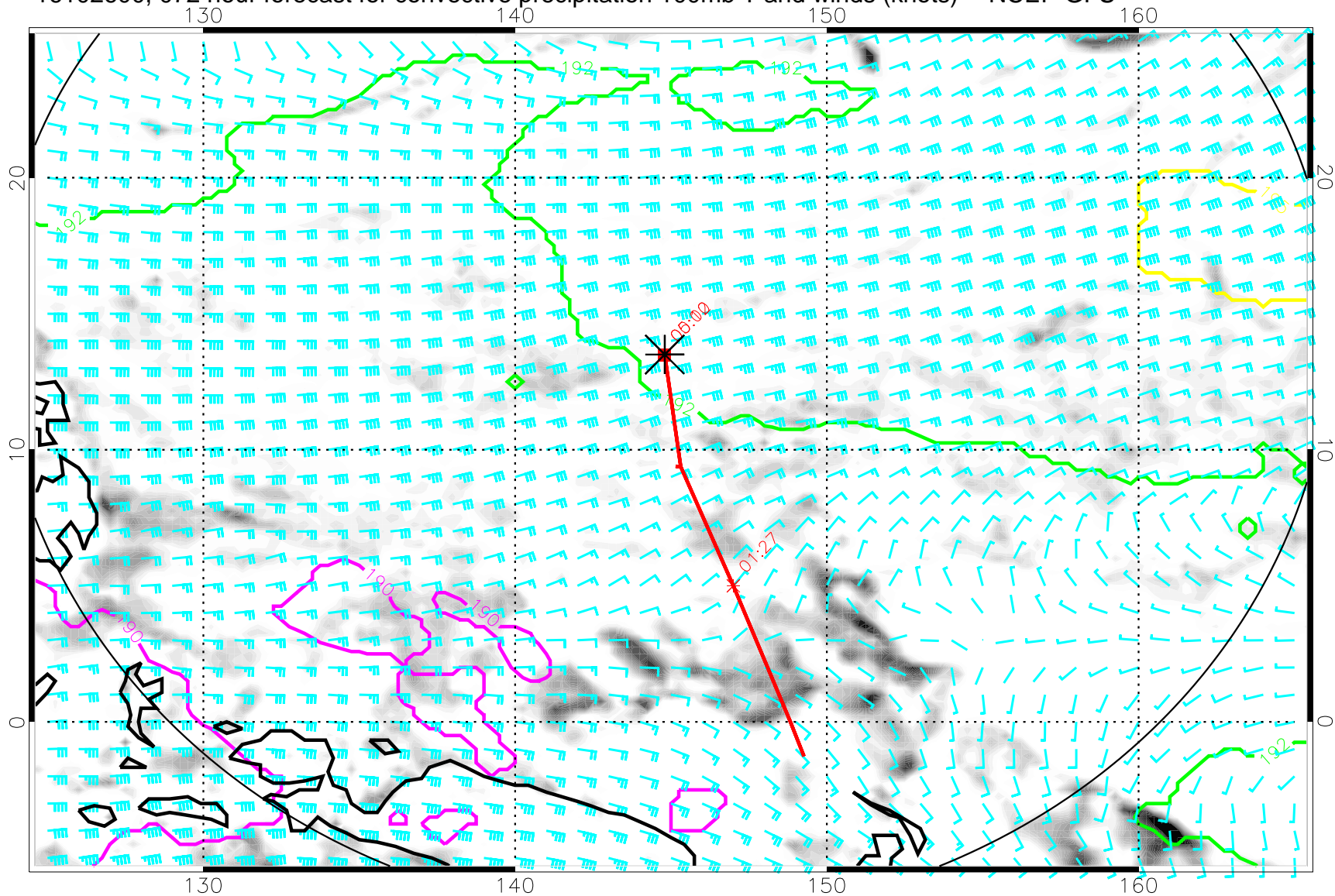
16102600, 072 hour forecast for convective precipitation 100mb T and winds (knots) -- NCEP GFS
