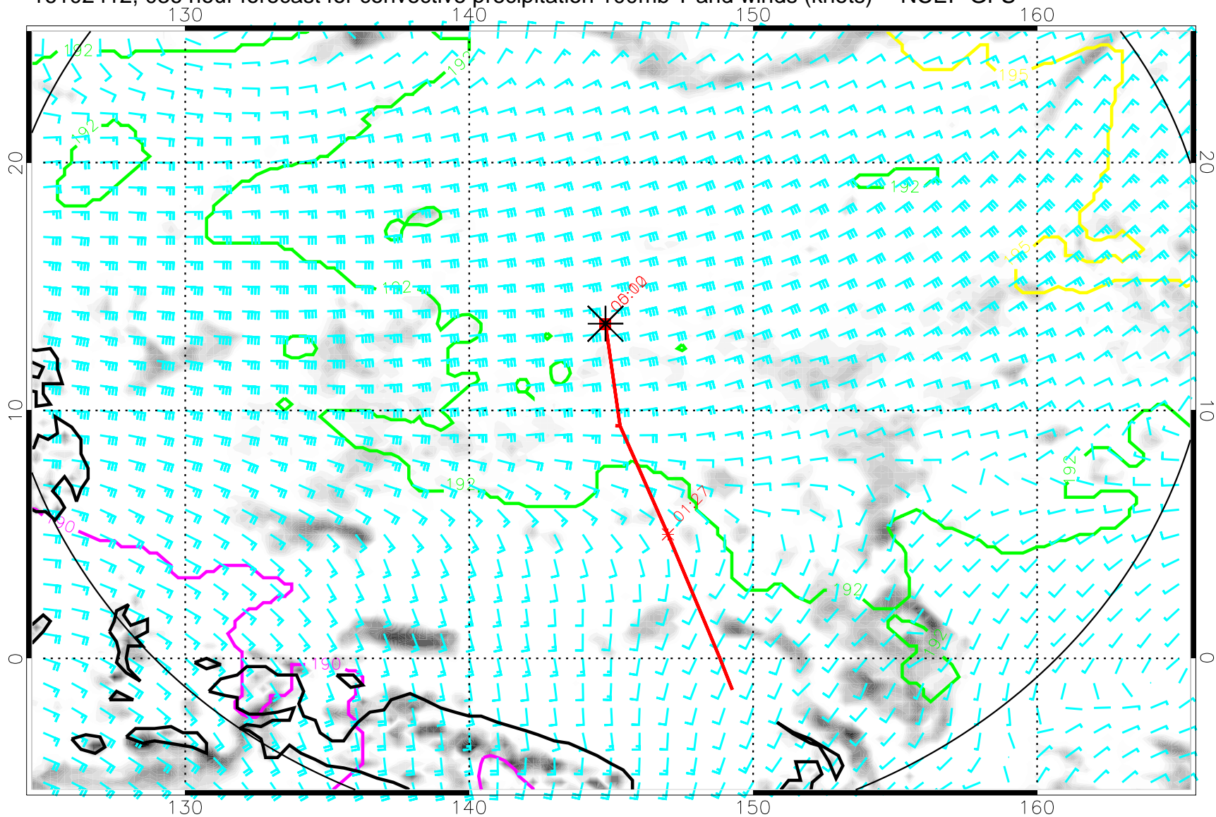
16102412, 036 hour forecast for convective precipitation 100mb T and winds (knots) -- NCEP GFS
