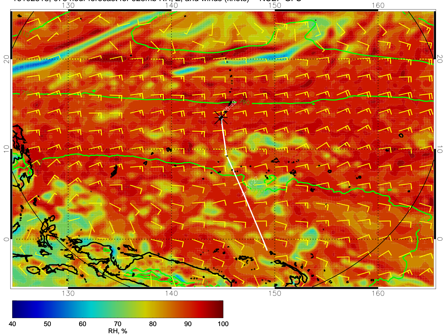
16102518, 078 hour forecast for 925mb RH, Z, and winds (knots) -- NCEP GFS
