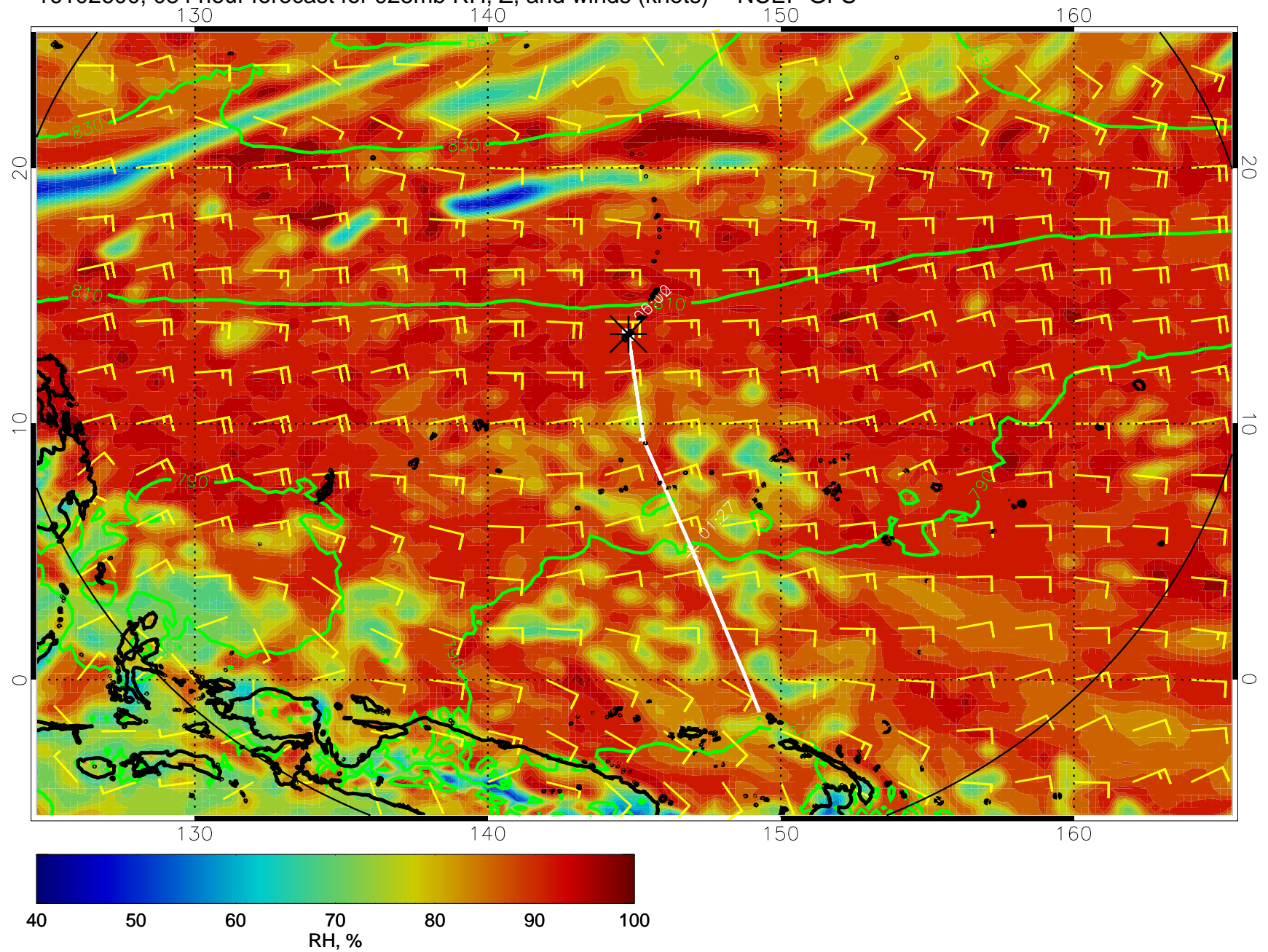
16102600, 084 hour forecast for 925mb RH, Z, and winds (knots) -- NCEP GFS
