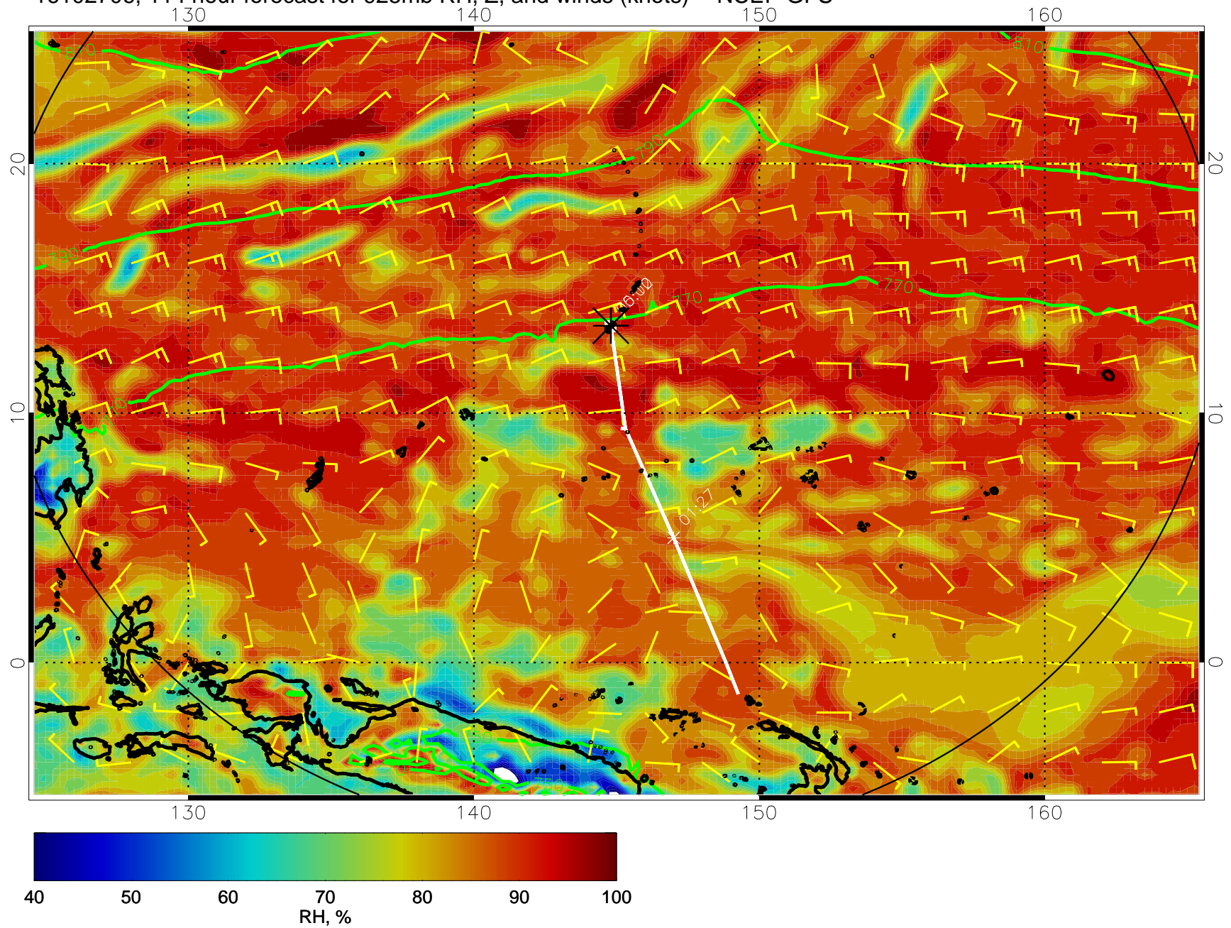
16102706, 114 hour forecast for 925mb RH, Z, and winds (knots) -- NCEP GFS
