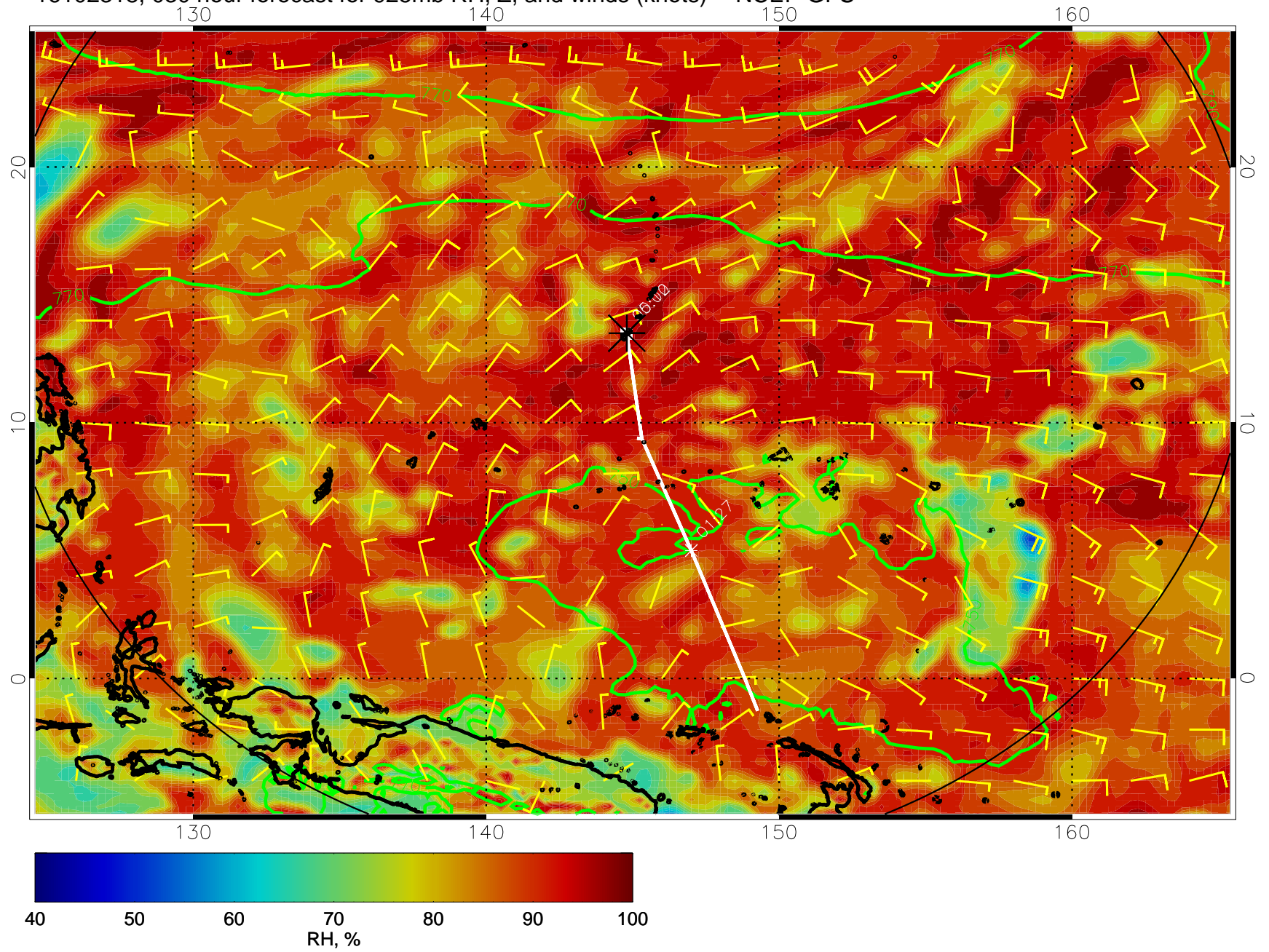
16102318, 030 hour forecast for 925mb RH, Z, and winds (knots) -- NCEP GFS
