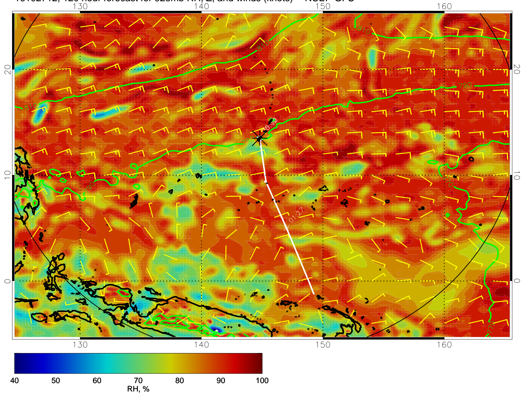
16102712, 120 hour forecast for 925mb RH, Z, and winds (knots) -- NCEP GFS
