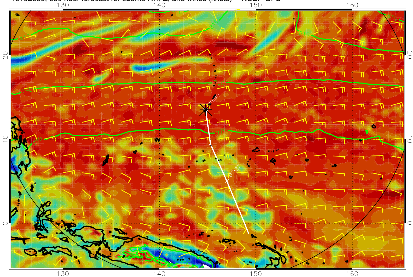
16102606, 090 hour forecast for 925mb RH, Z, and winds (knots) -- NCEP GFS
