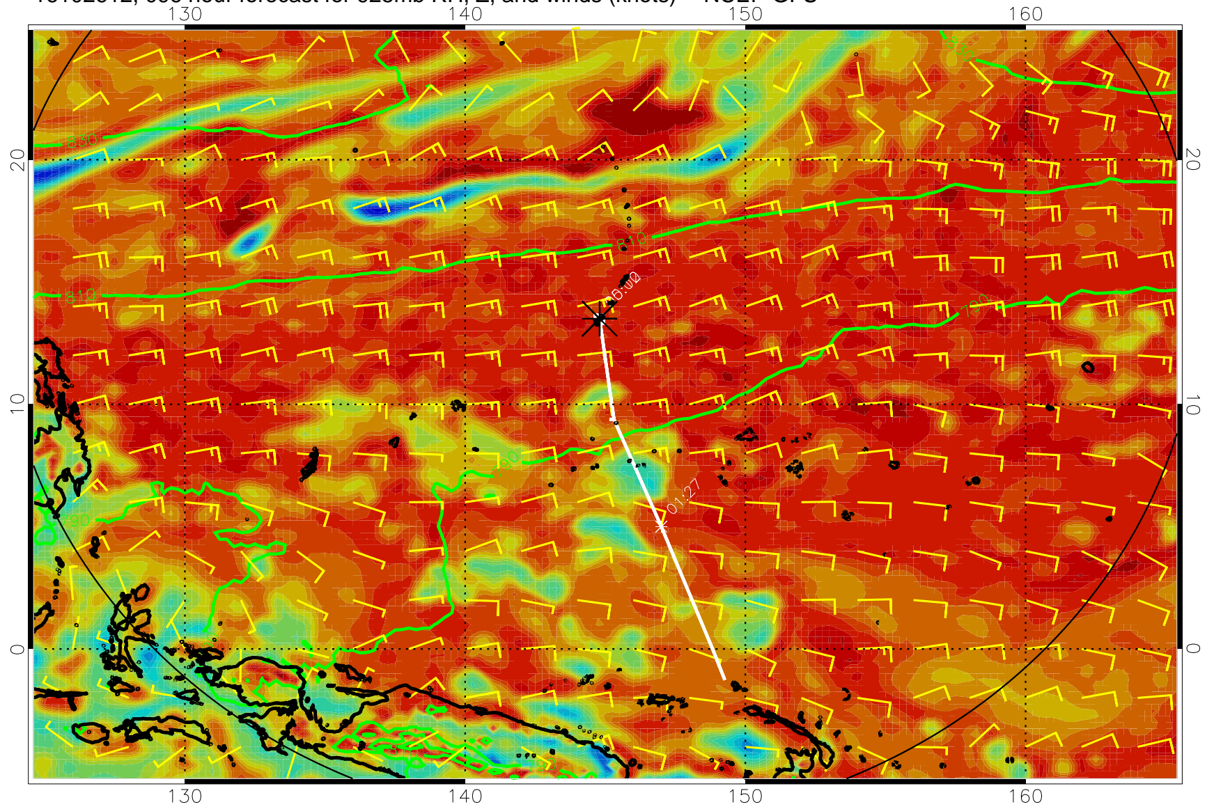
16102612, 096 hour forecast for 925mb RH, Z, and winds (knots) -- NCEP GFS
