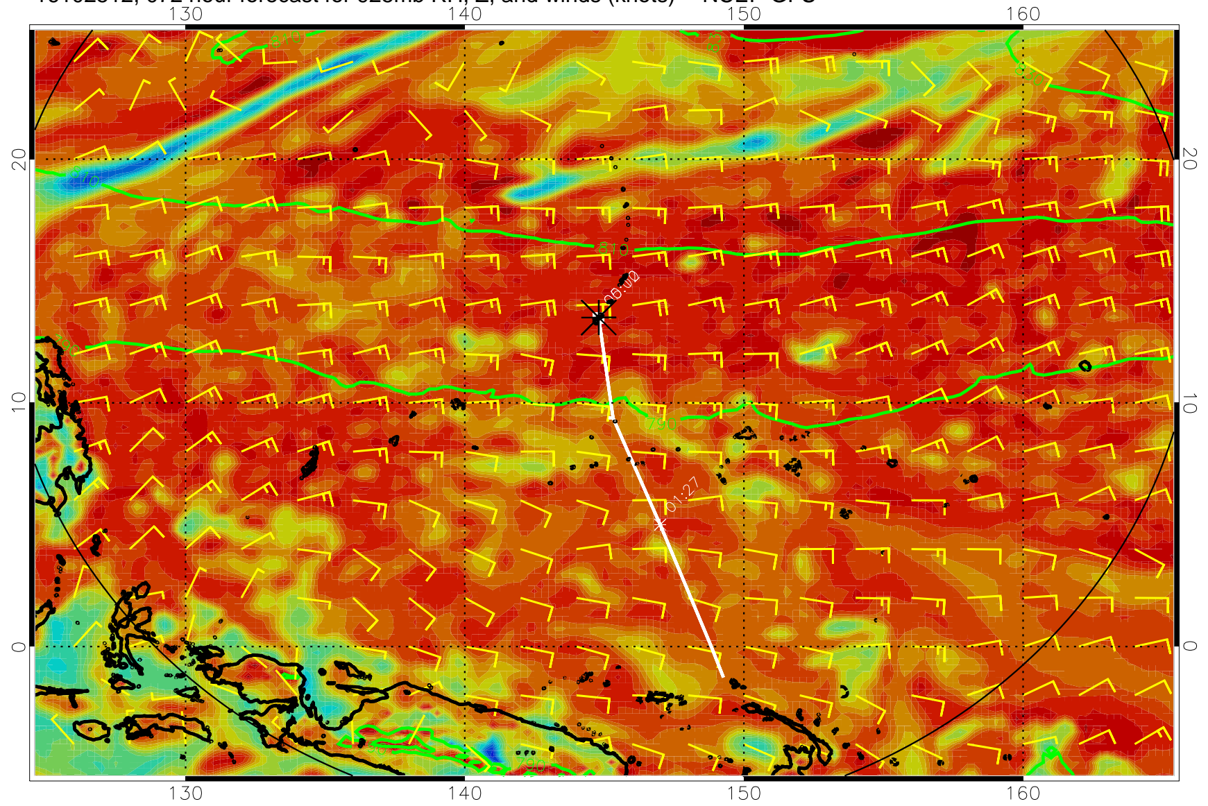
16102512, 072 hour forecast for 925mb RH, Z, and winds (knots) -- NCEP GFS
