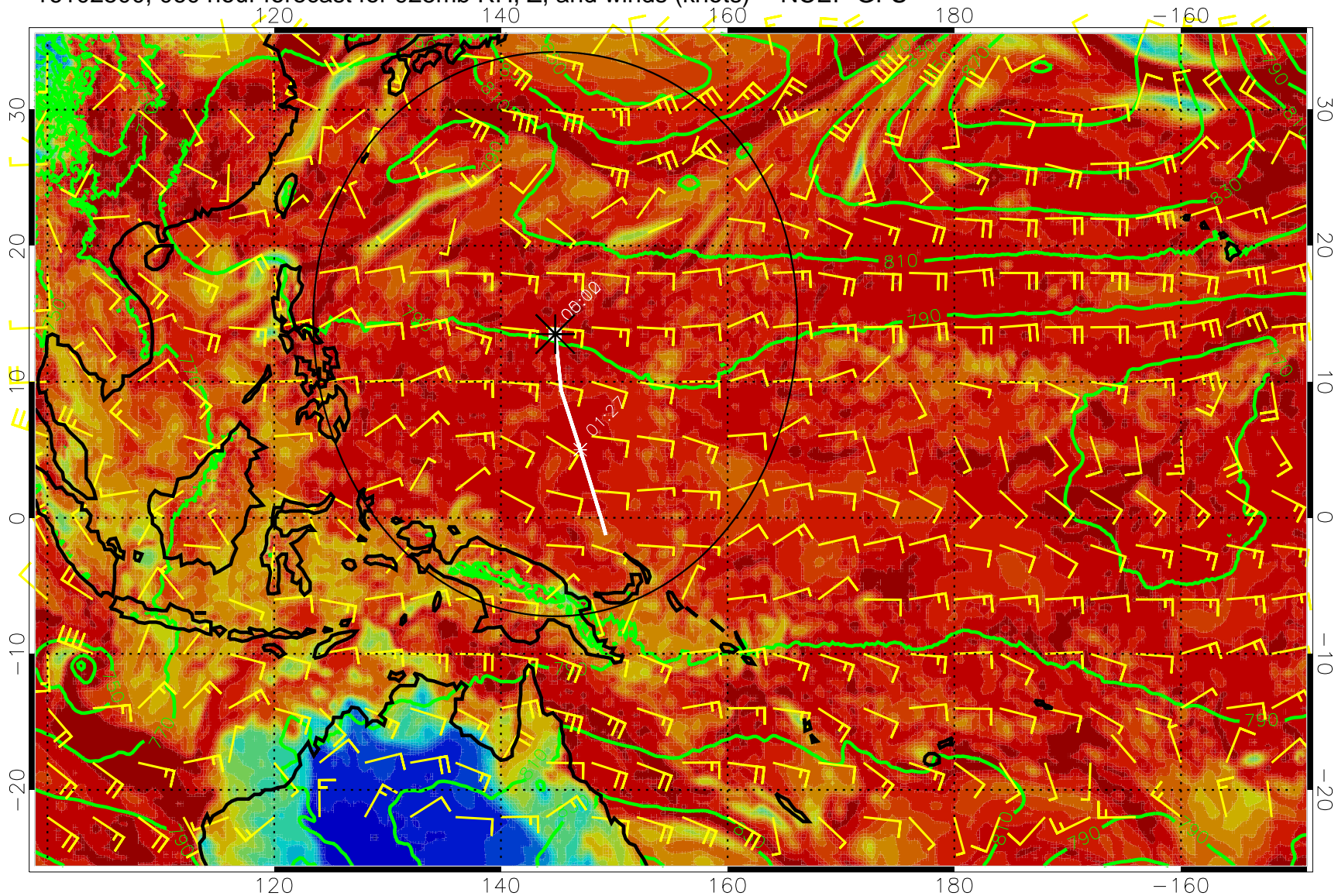
16102500, 060 hour forecast for 925mb RH, Z, and winds (knots) -- NCEP GFS
