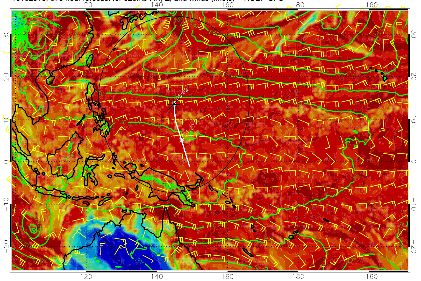
16102518, 078 hour forecast for 925mb RH, Z, and winds (knots) -- NCEP GFS
