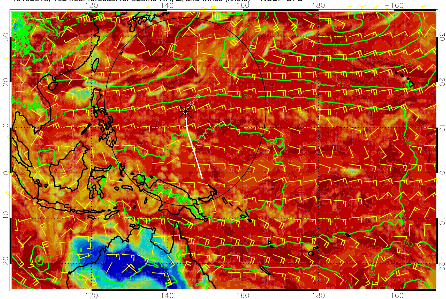
16102618, 102 hour forecast for 925mb RH, Z, and winds (knots) -- NCEP GFS
