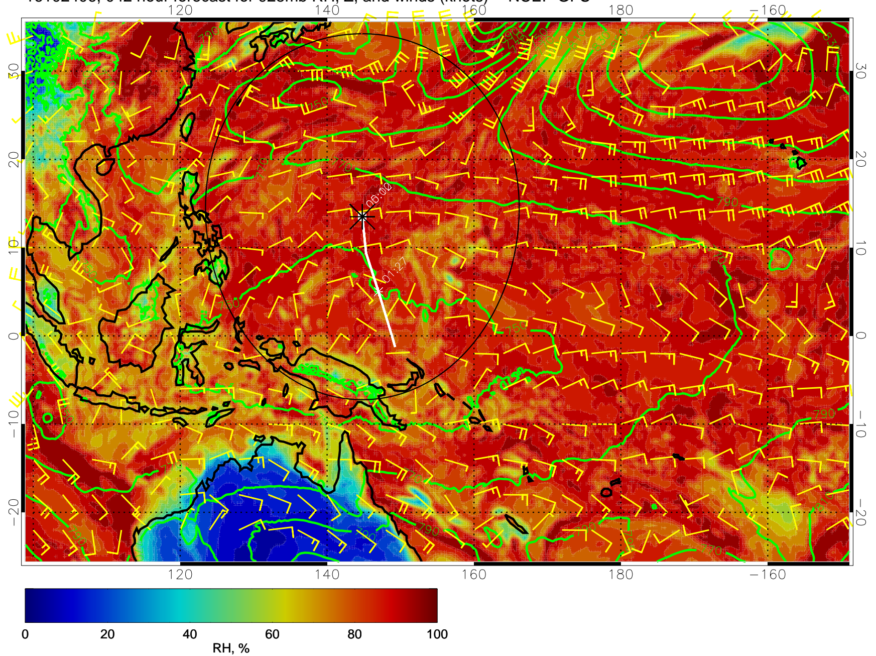
16102406, 042 hour forecast for 925mb RH, Z, and winds (knots) -- NCEP GFS
