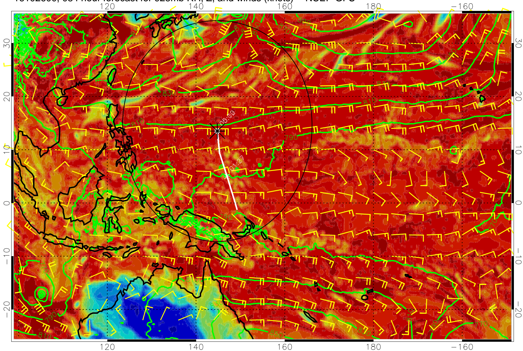
16102600, 084 hour forecast for 925mb RH, Z, and winds (knots) -- NCEP GFS
