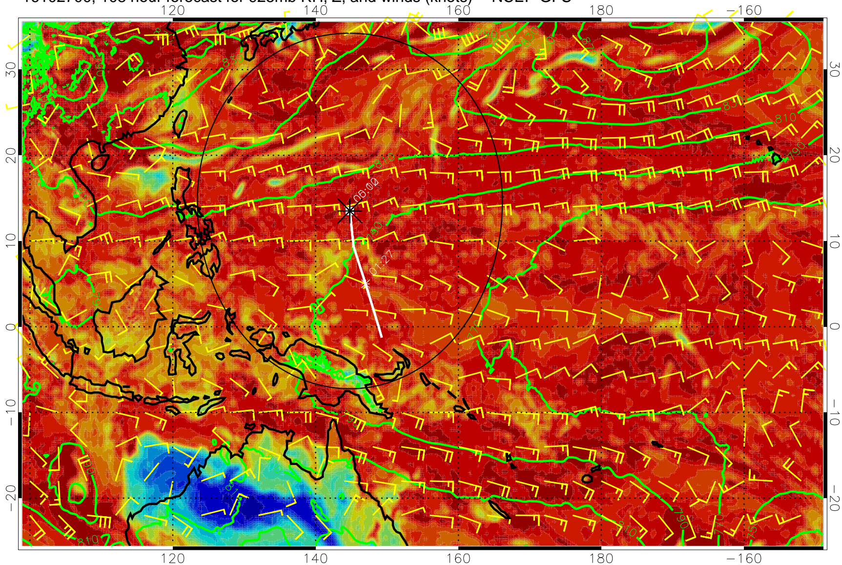
16102700, 108 hour forecast for 925mb RH, Z, and winds (knots) -- NCEP GFS
