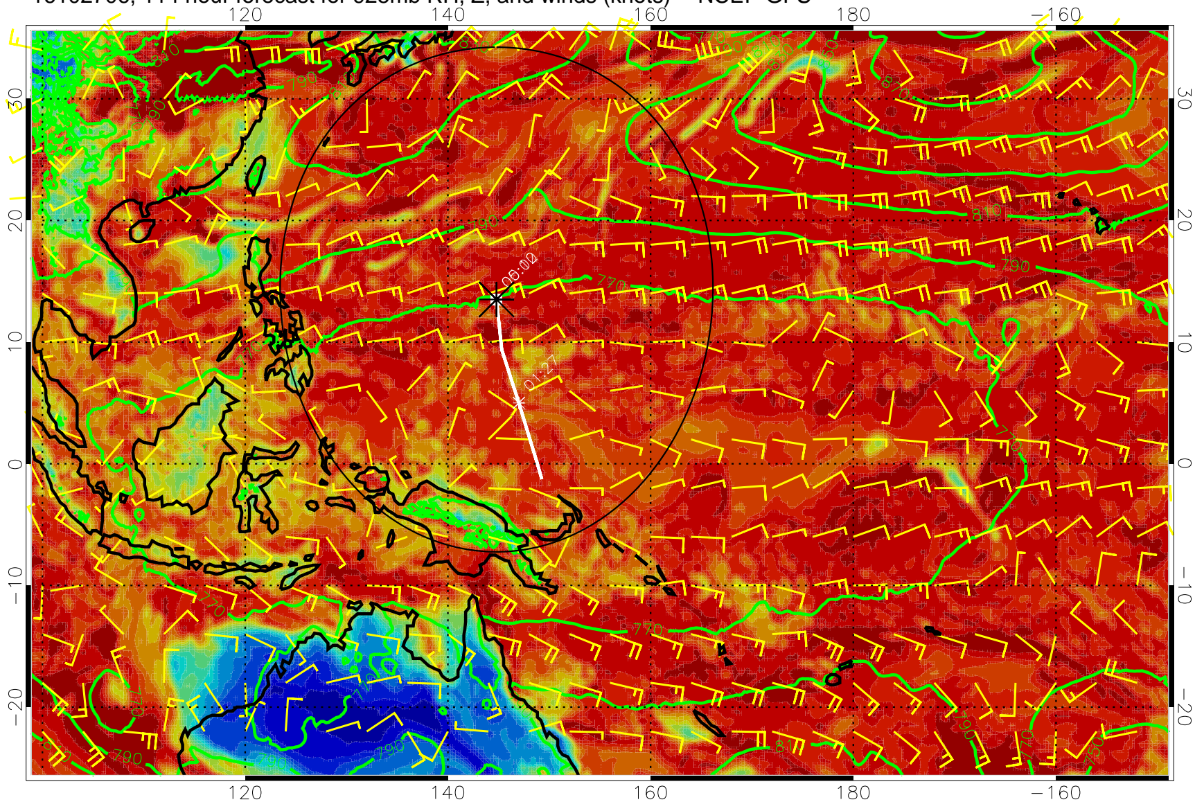
16102706, 114 hour forecast for 925mb RH, Z, and winds (knots) -- NCEP GFS
