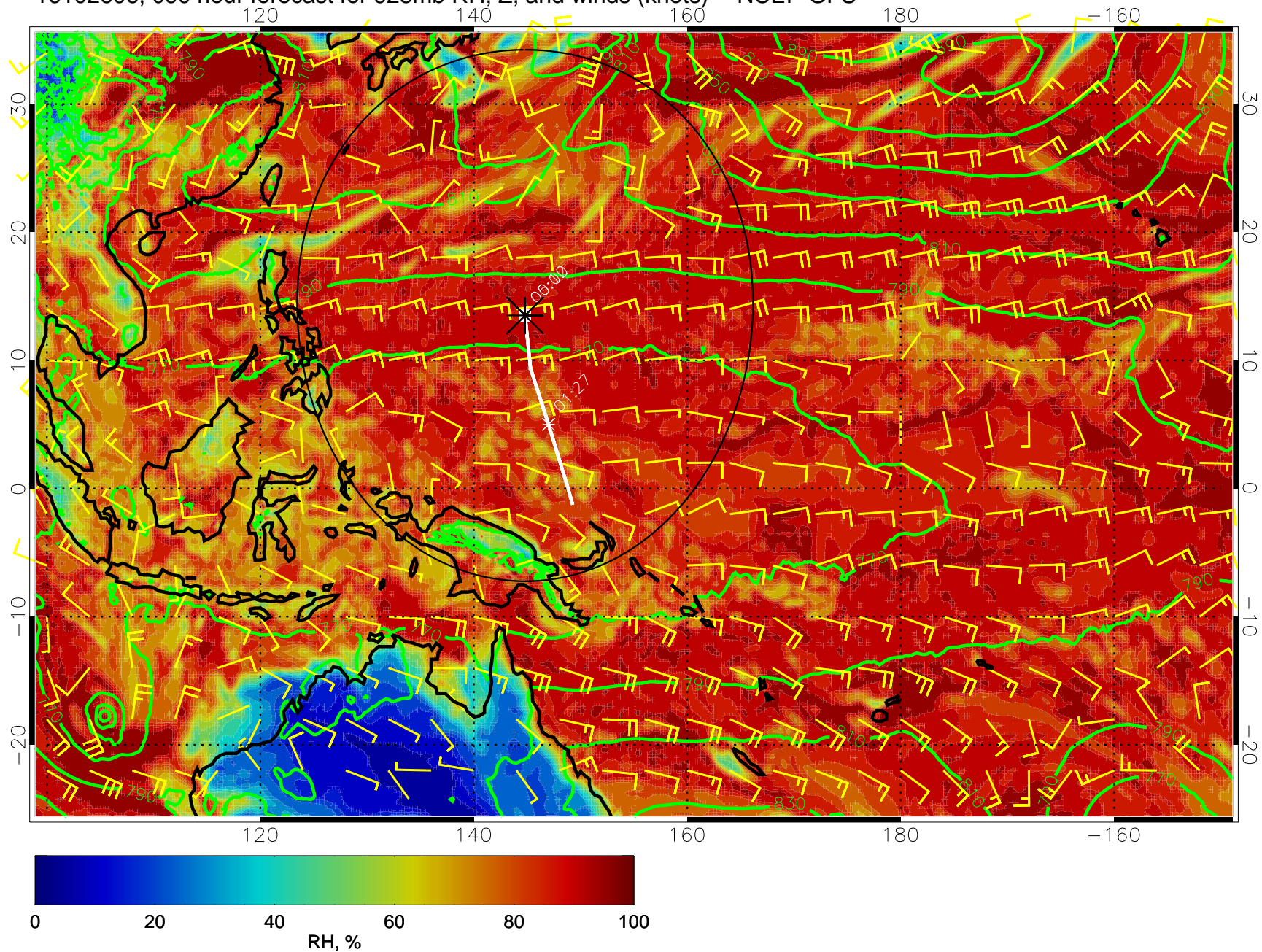
16102606, 090 hour forecast for 925mb RH, Z, and winds (knots) -- NCEP GFS
