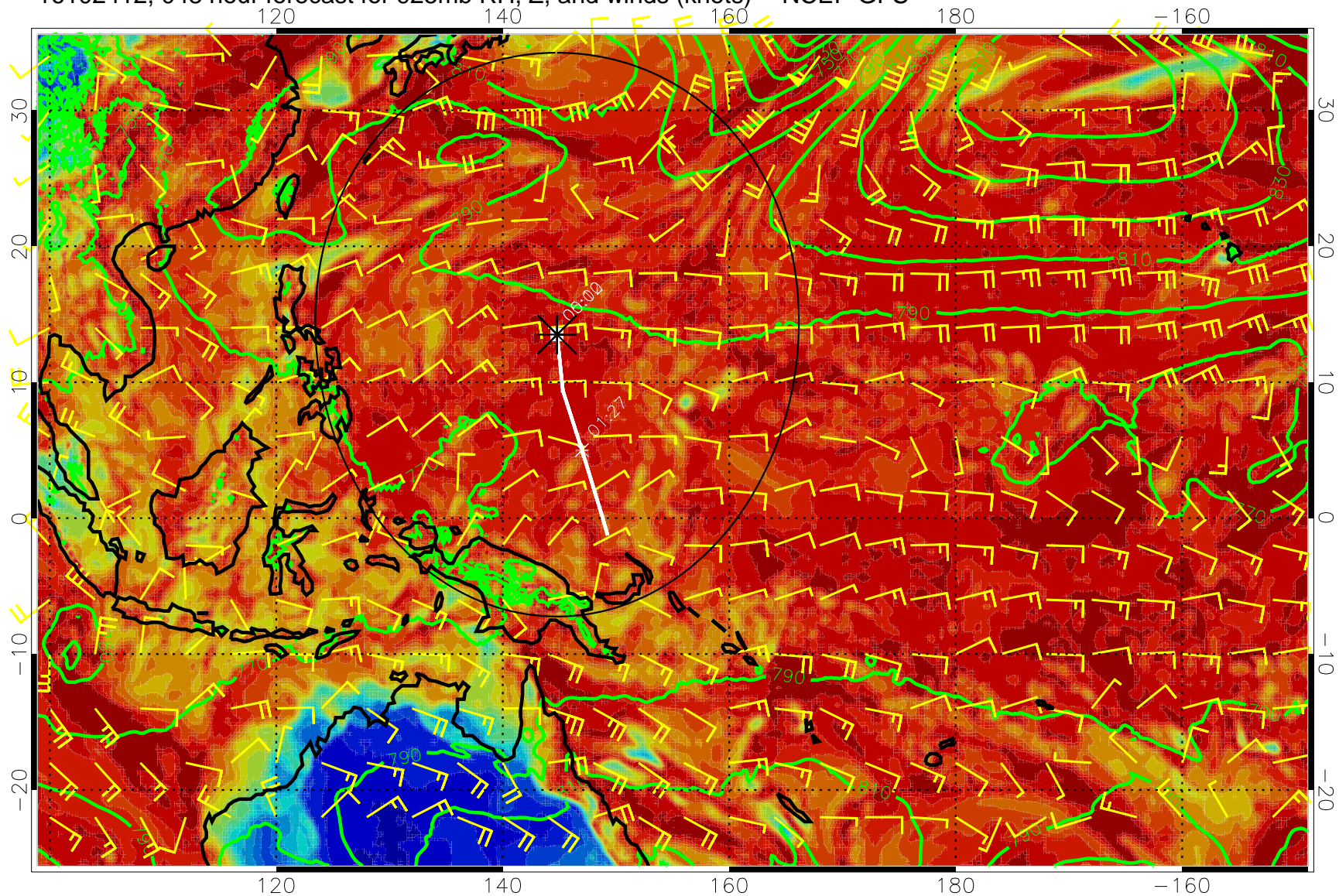
16102412, 048 hour forecast for 925mb RH, Z, and winds (knots) -- NCEP GFS
