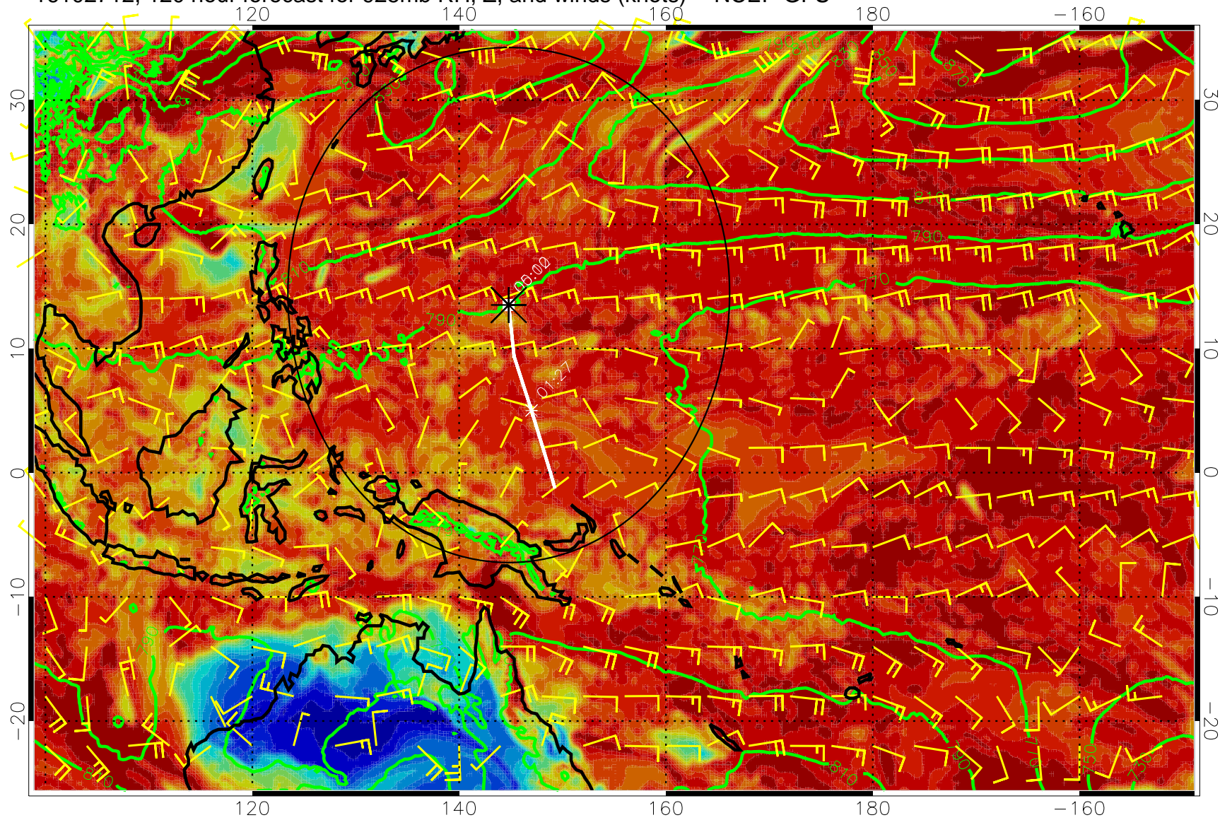
16102712, 120 hour forecast for 925mb RH, Z, and winds (knots) -- NCEP GFS
