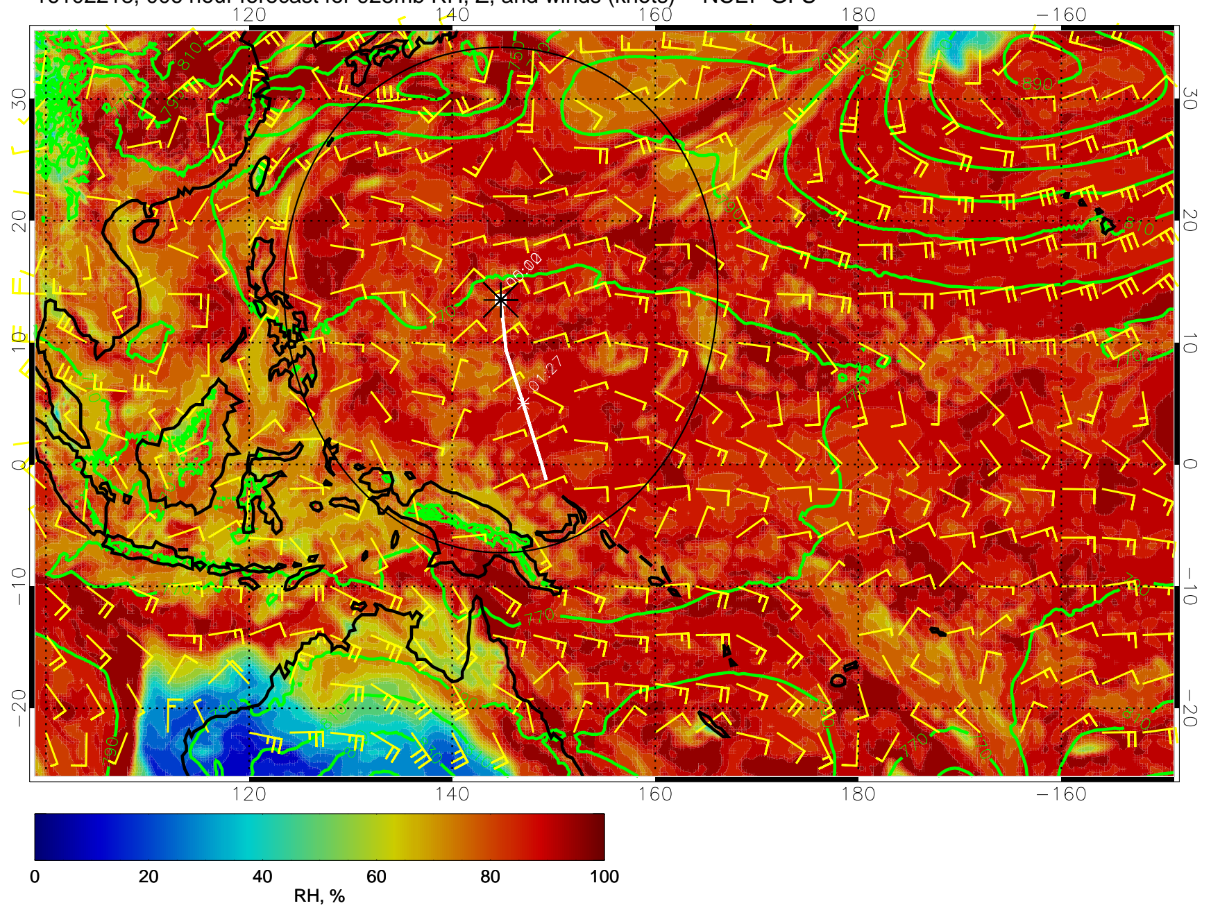
16102218, 006 hour forecast for 925mb RH, Z, and winds (knots) -- NCEP GFS
