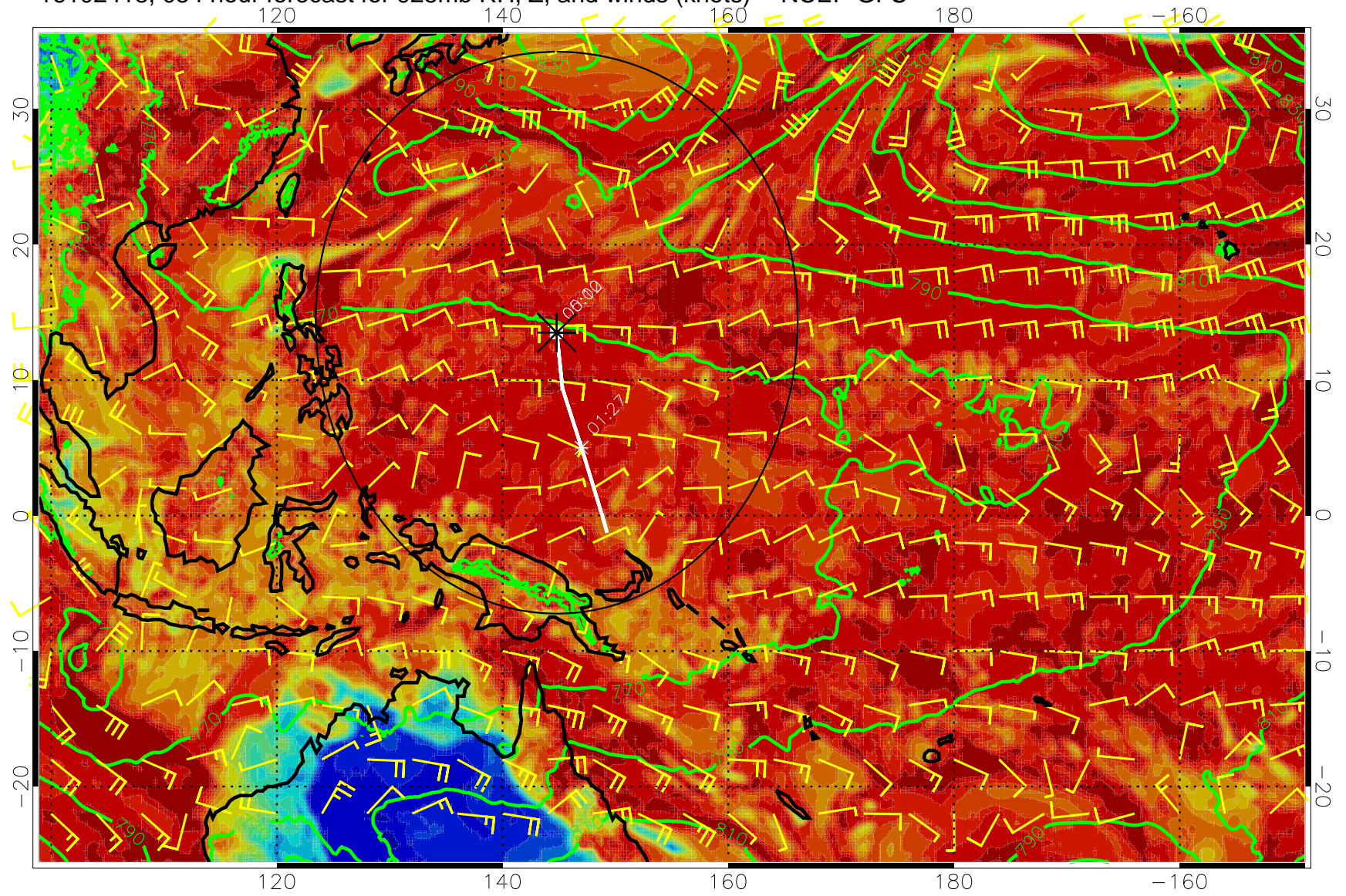
16102418, 054 hour forecast for 925mb RH, Z, and winds (knots) -- NCEP GFS
