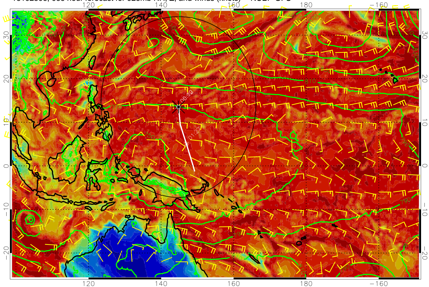
16102506, 066 hour forecast for 925mb RH, Z, and winds (knots) -- NCEP GFS
