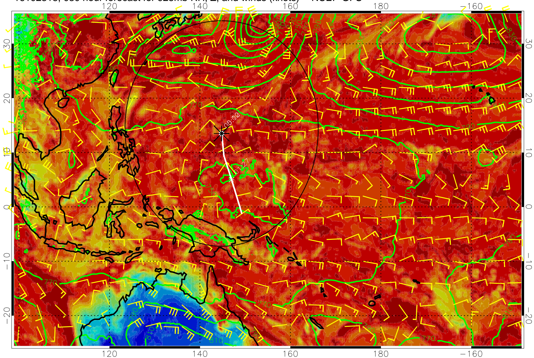
16102318, 030 hour forecast for 925mb RH, Z, and winds (knots) -- NCEP GFS
