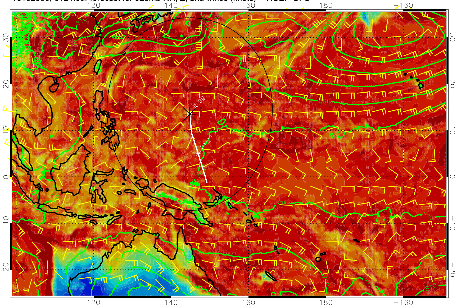
16102300, 012 hour forecast for 925mb RH, Z, and winds (knots) -- NCEP GFS
