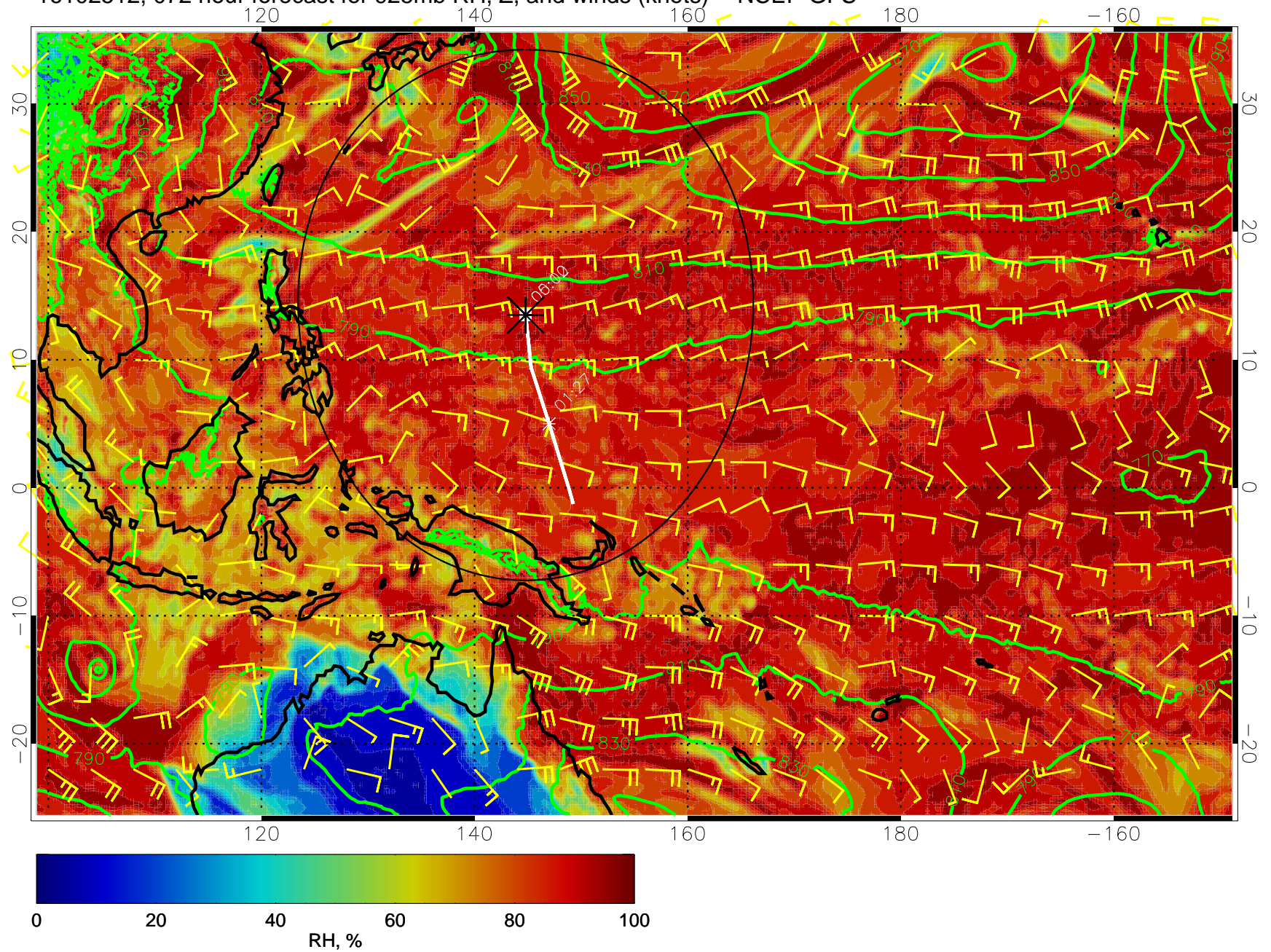
16102512, 072 hour forecast for 925mb RH, Z, and winds (knots) -- NCEP GFS
