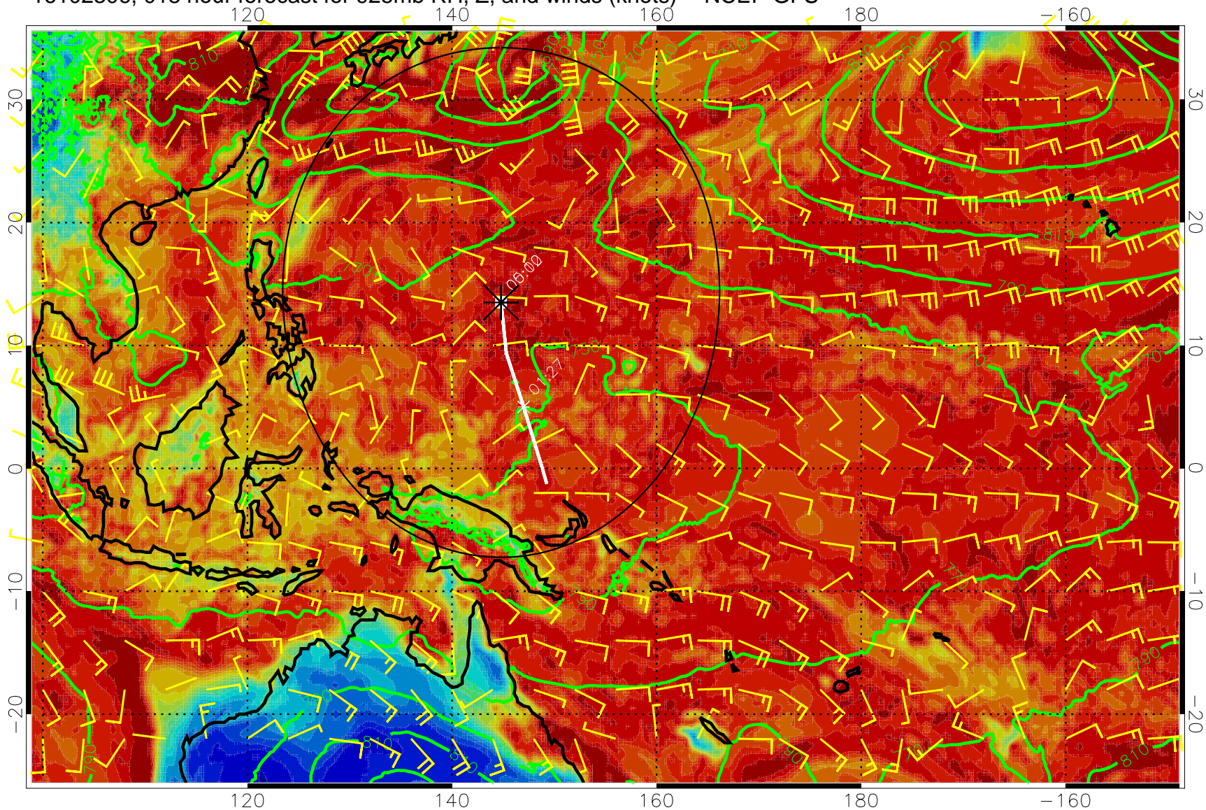
16102306, 018 hour forecast for 925mb RH, Z, and winds (knots) -- NCEP GFS
