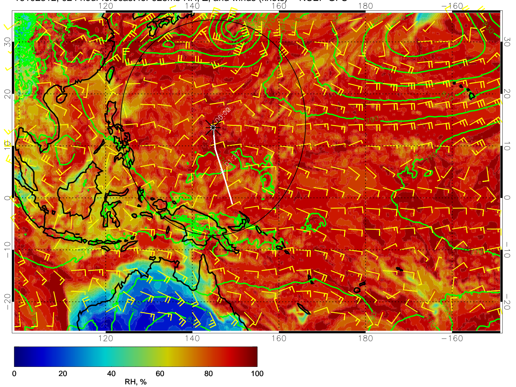
16102312, 024 hour forecast for 925mb RH, Z, and winds (knots) -- NCEP GFS
