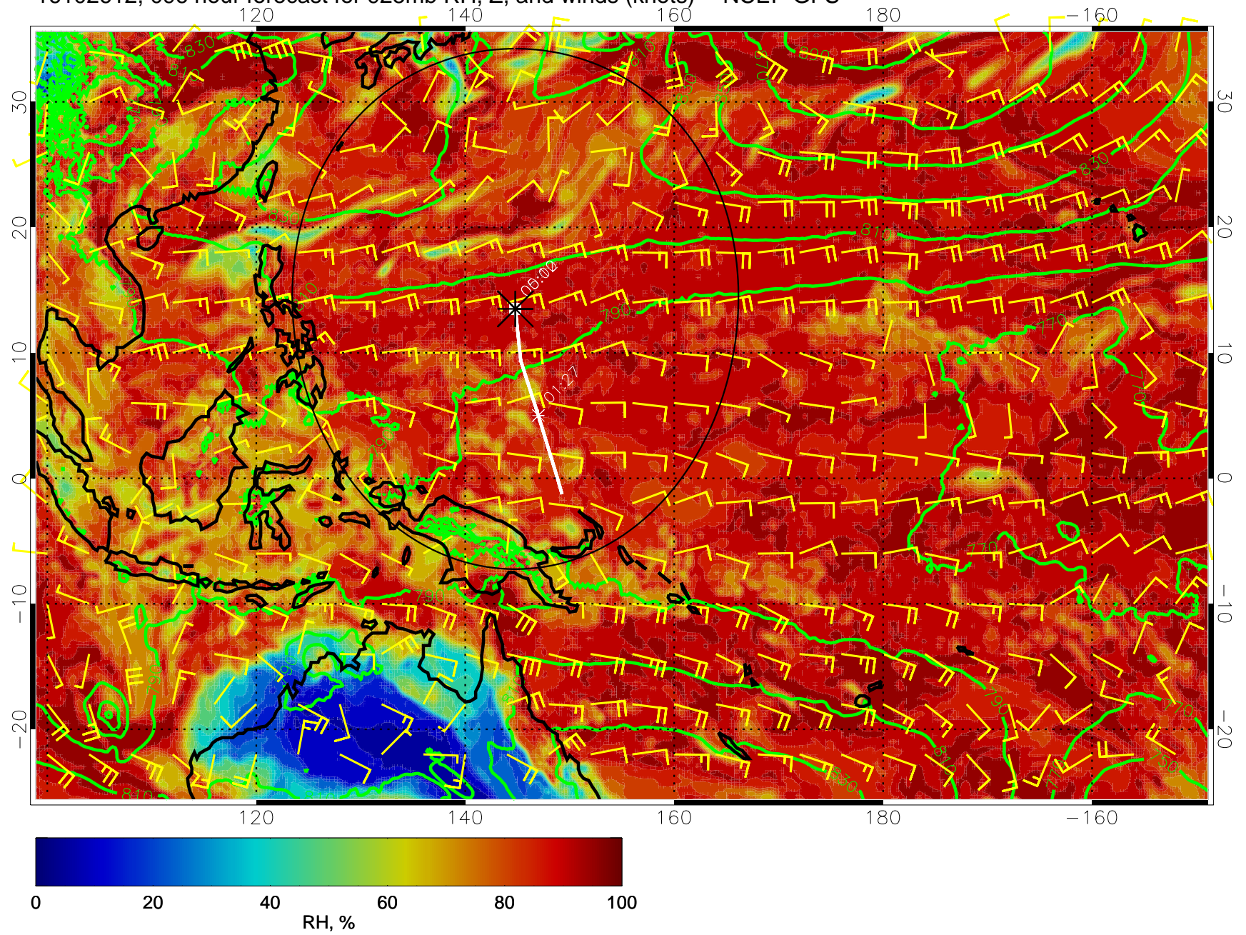
16102612, 096 hour forecast for 925mb RH, Z, and winds (knots) -- NCEP GFS
