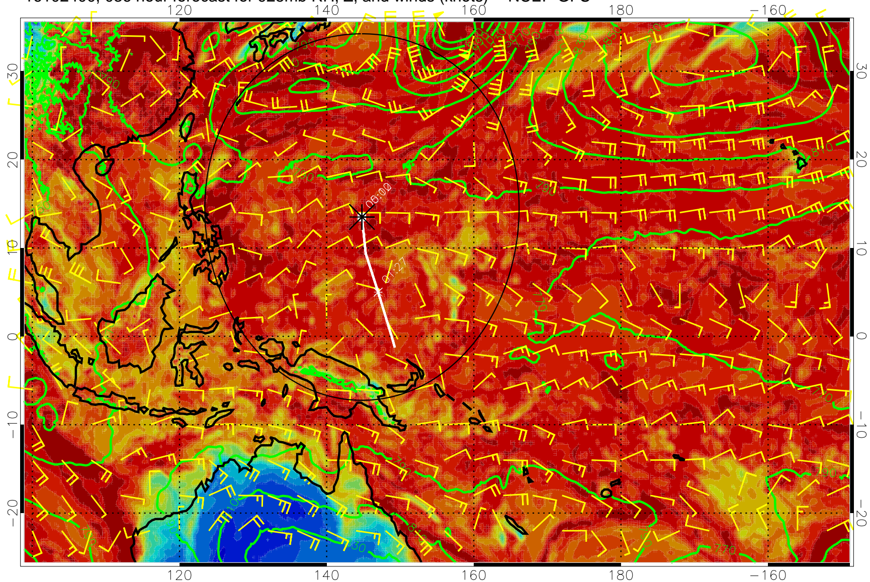
16102400, 036 hour forecast for 925mb RH, Z, and winds (knots) -- NCEP GFS
