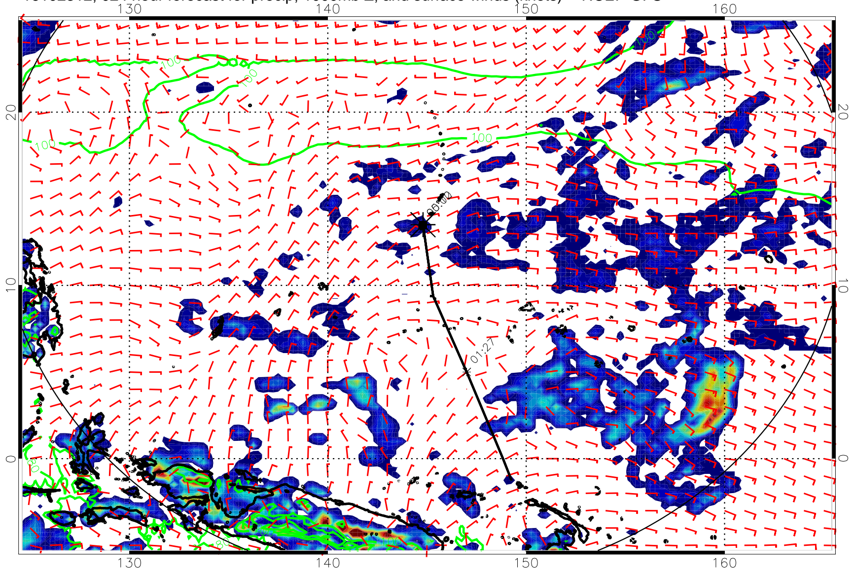
16102312, 024 hour forecast for precip, 1000mb Z, and surface winds (knots) -- NCEP GFS
