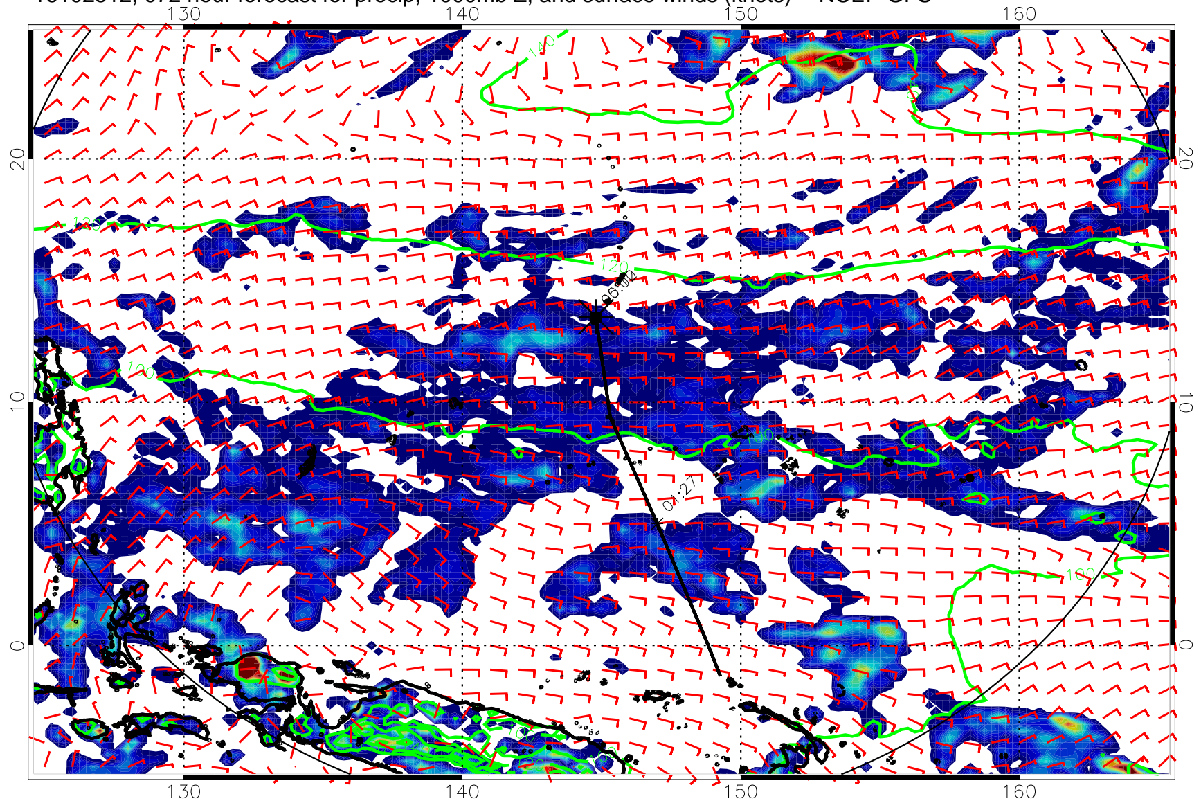
16102512, 072 hour forecast for precip, 1000mb Z, and surface winds (knots) -- NCEP GFS
