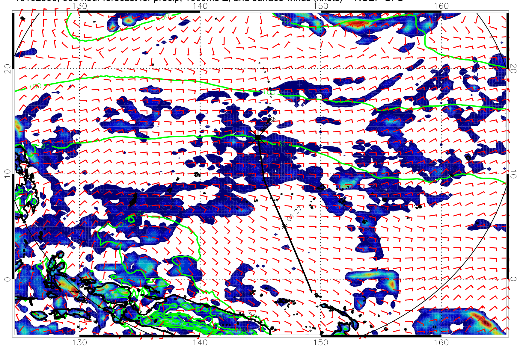
16102506, 066 hour forecast for precip, 1000mb Z, and surface winds (knots) -- NCEP GFS
