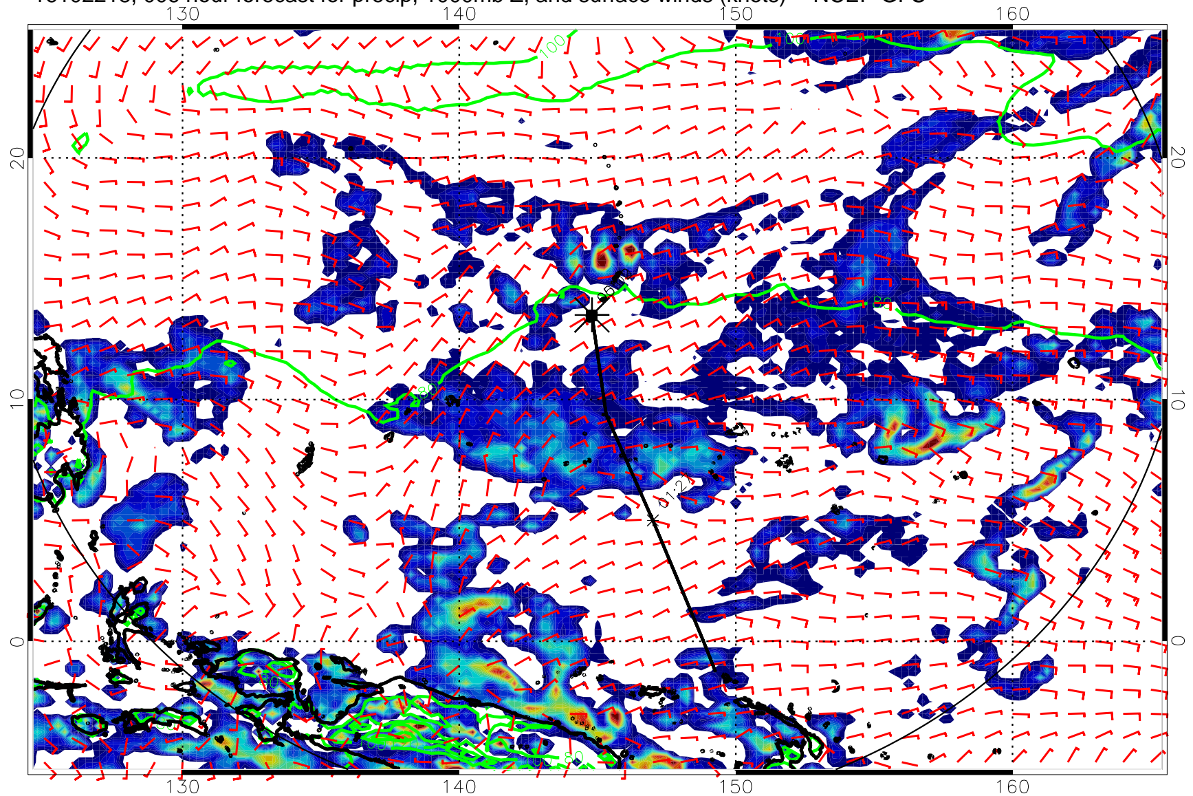
16102218, 006 hour forecast for precip, 1000mb Z, and surface winds (knots) -- NCEP GFS
