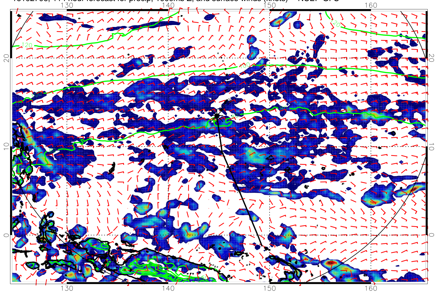
16102706, 114 hour forecast for precip, 1000mb Z, and surface winds (knots) -- NCEP GFS
