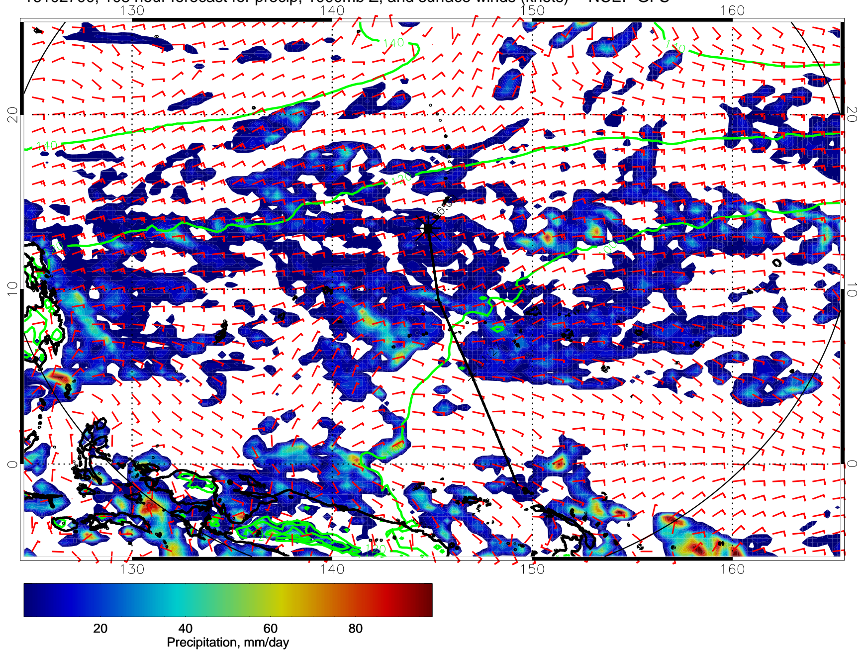
16102700, 108 hour forecast for precip, 1000mb Z, and surface winds (knots) -- NCEP GFS
