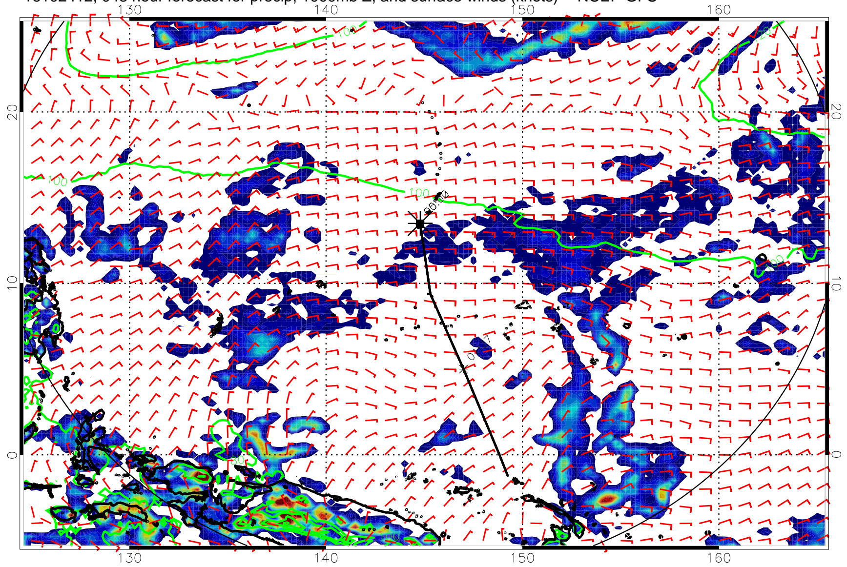
16102412, 048 hour forecast for precip, 1000mb Z, and surface winds (knots) -- NCEP GFS
