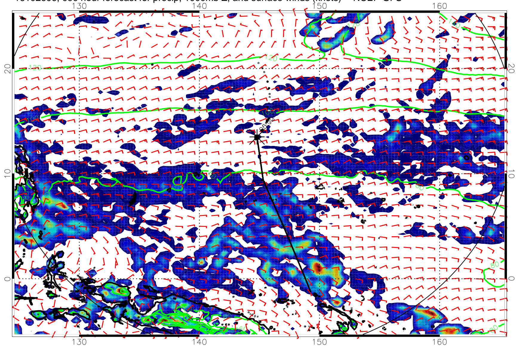
16102606, 0900 hour forecast for precip, 1000mb Z, and surface winds (knots) -- NCEP GFS
