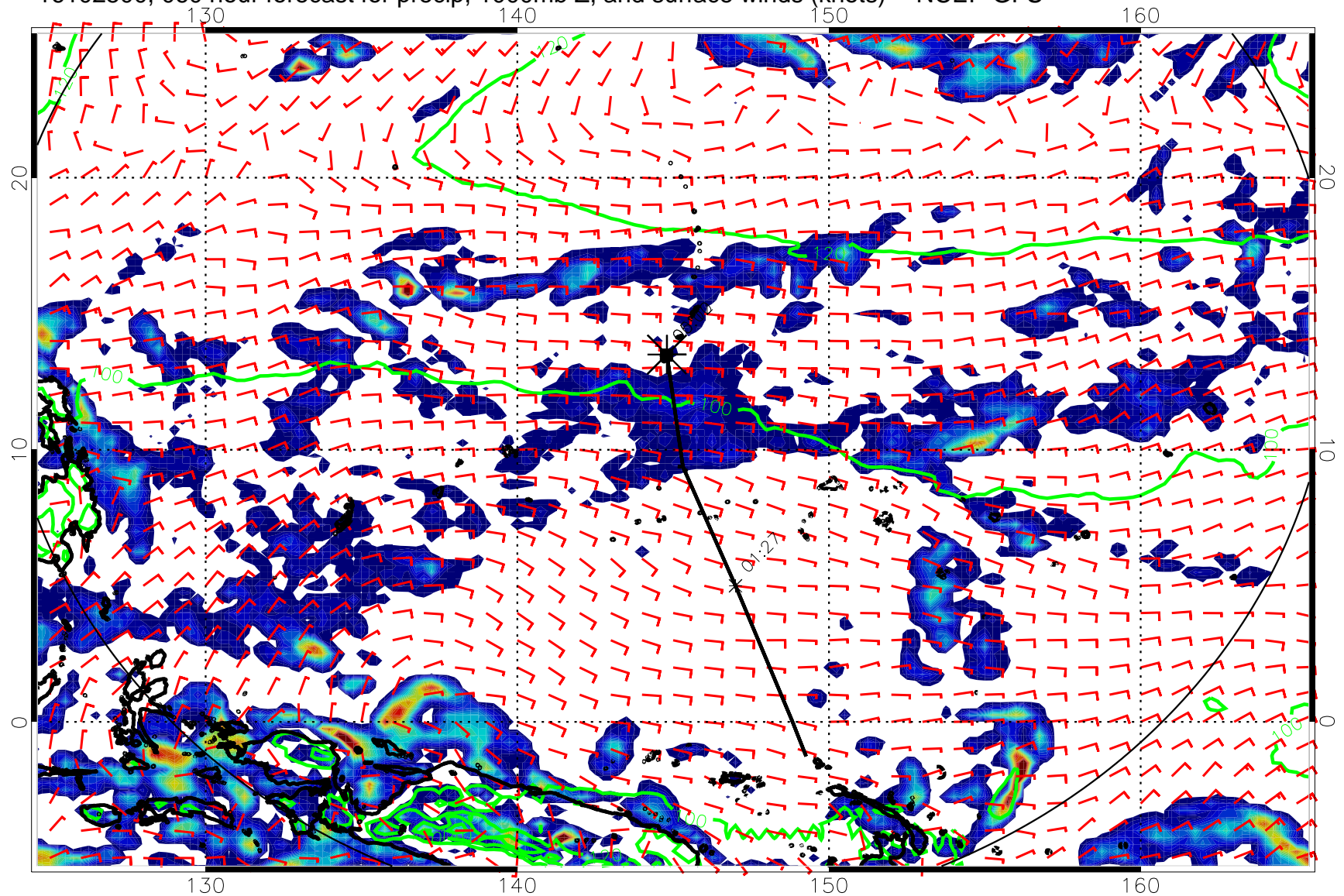
16102500, 060 hour forecast for precip, 1000mb Z, and surface winds (knots) -- NCEP GFS
