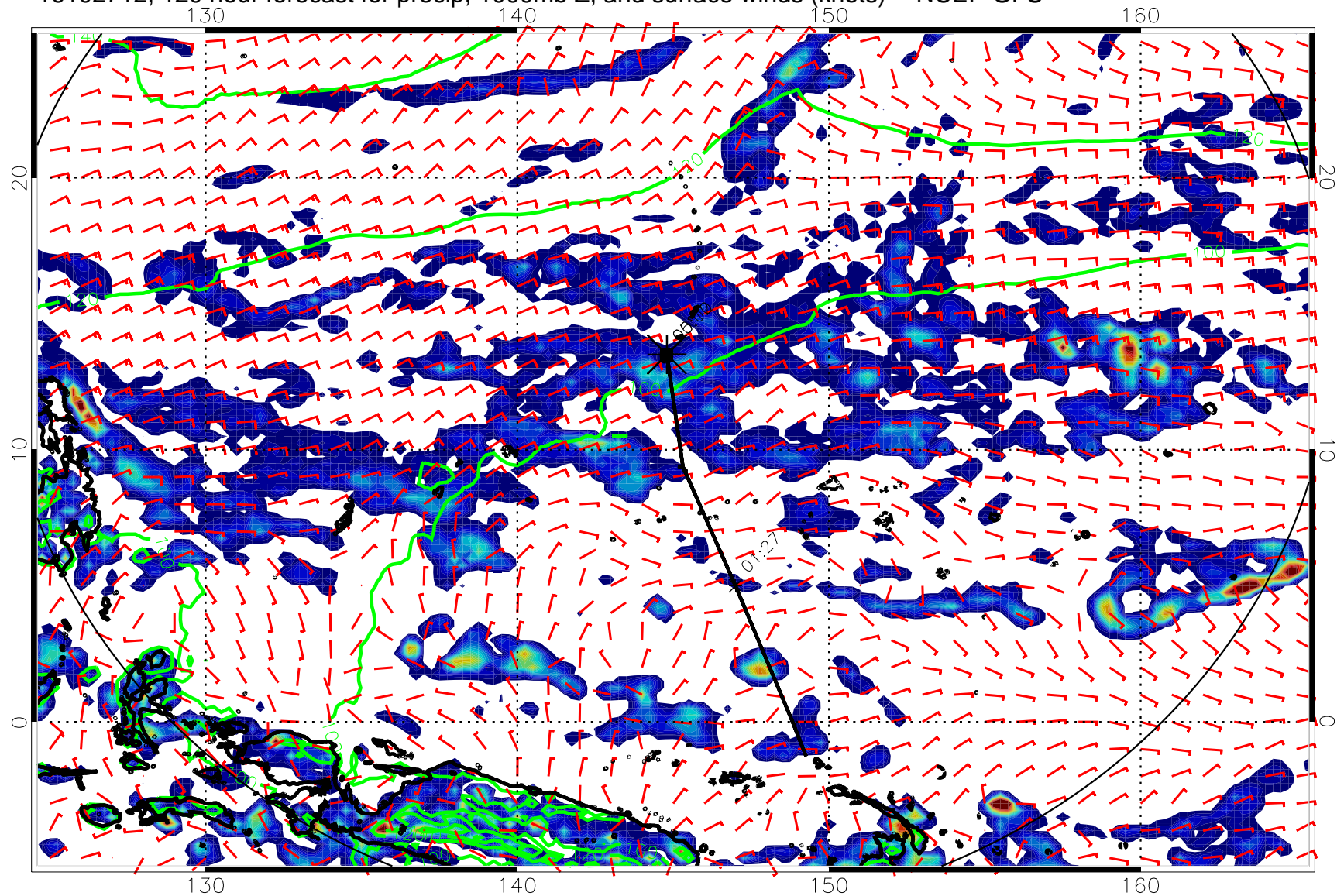
16102712, 120 hour forecast for precip, 1000mb Z, and surface winds (knots) -- NCEP GFS
