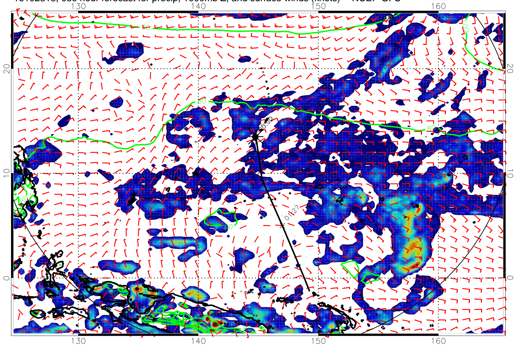
16102318, 030 hour forecast for precip, 1000mb Z, and surface winds (knots) -- NCEP GFS
