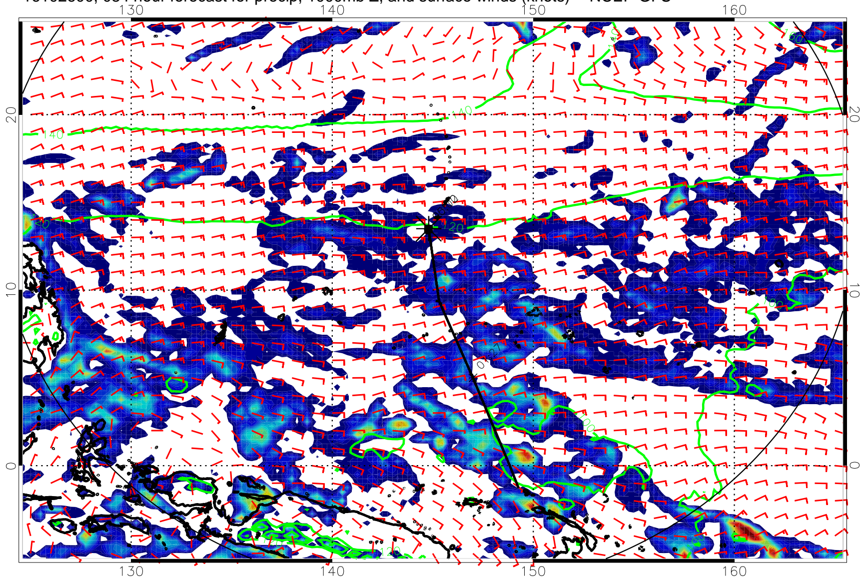
16102600, 084 hour forecast for precip, 1000mb Z, and surface winds (knots) -- NCEP GFS
