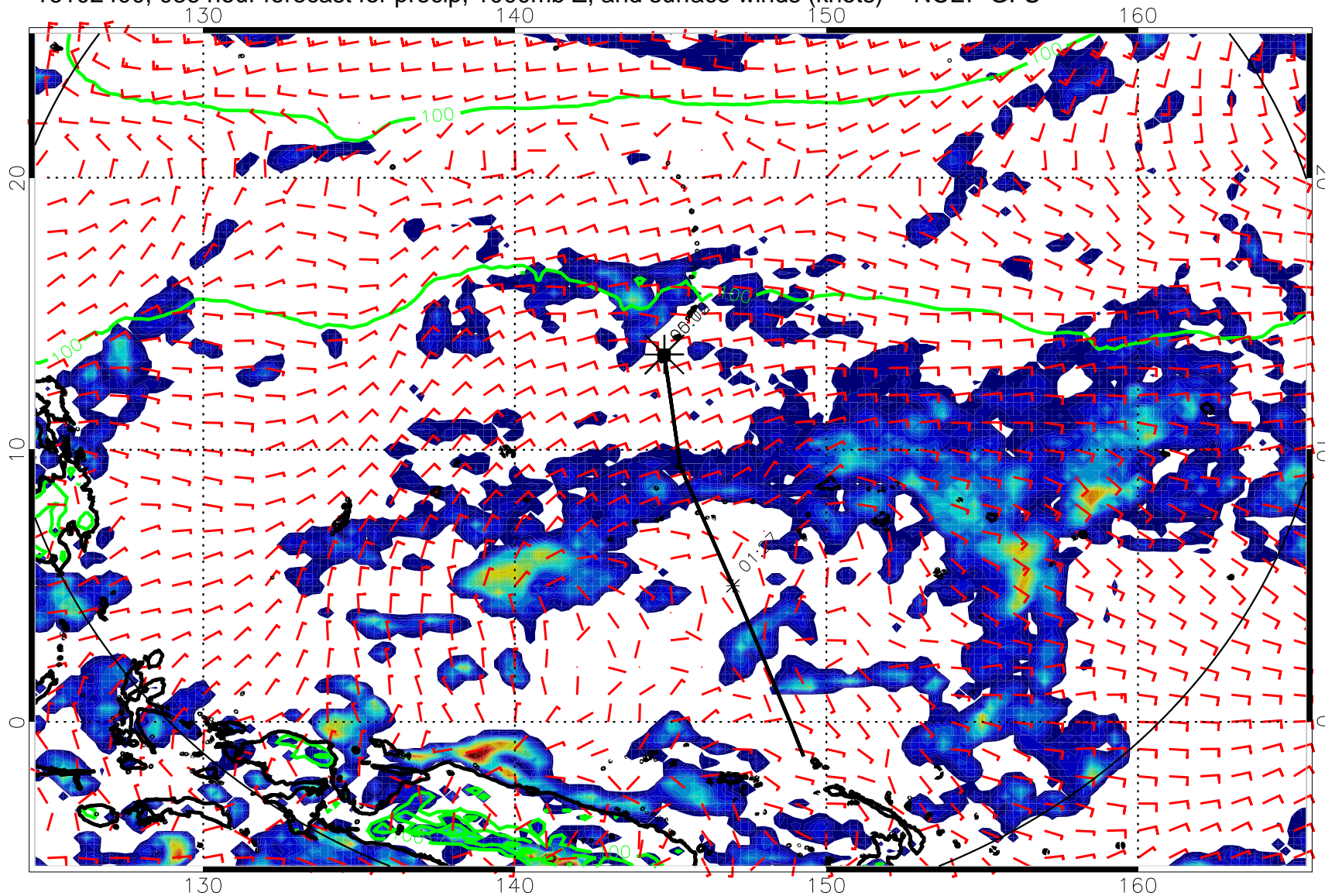
16102400, 036 hour forecast for precip, 1000mb Z, and surface winds (knots) -- NCEP GFS
