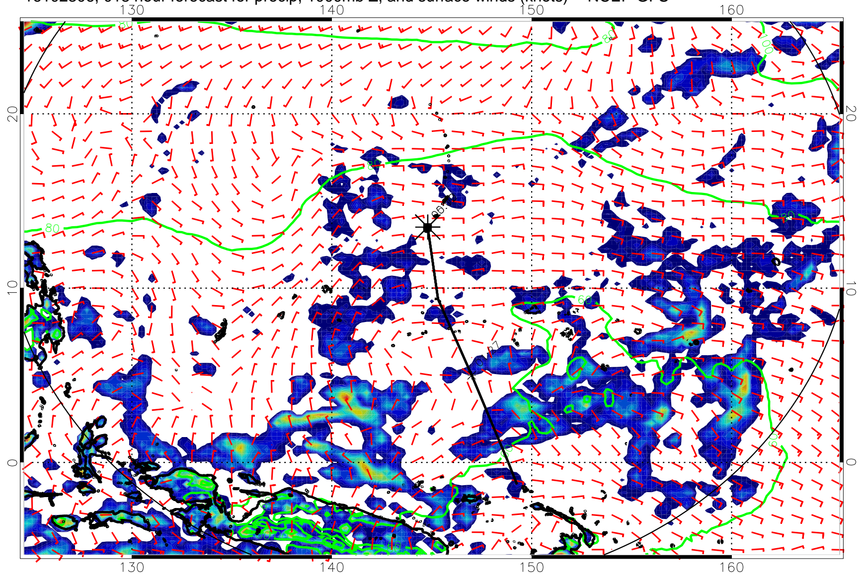
16102306, 018 hour forecast for precip, 1000mb Z, and surface winds (knots) -- NCEP GFS
