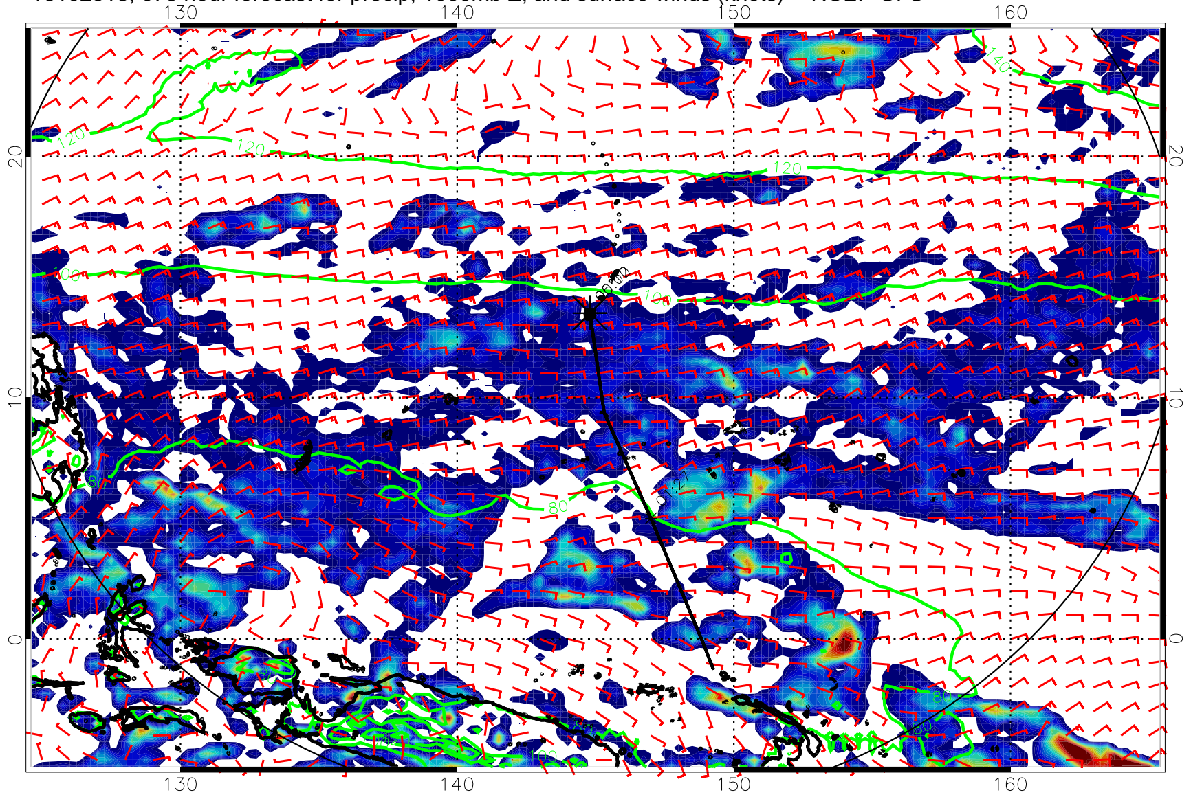
16102518, 078 hour forecast for precip, 1000mb Z, and surface winds (knots) -- NCEP GFS
