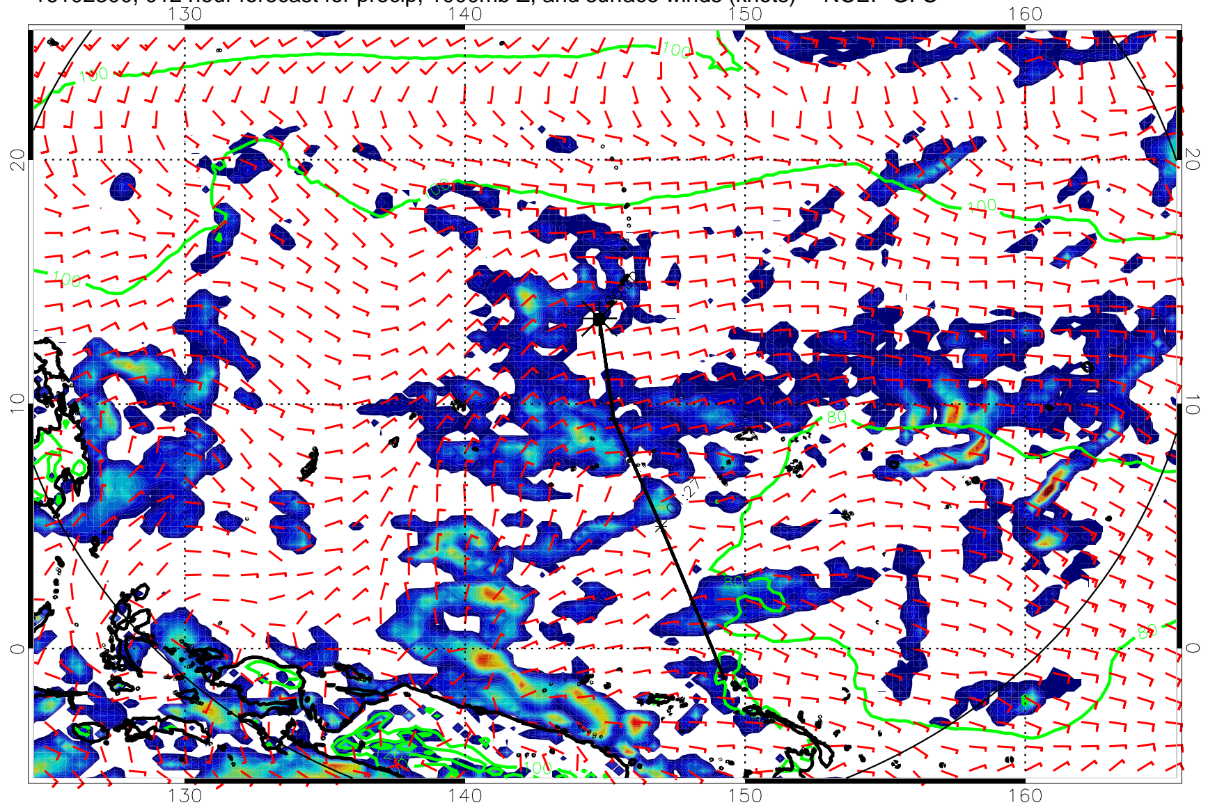
16102300, 012 hour forecast for precip, 1000mb Z, and surface winds (knots) -- NCEP GFS
