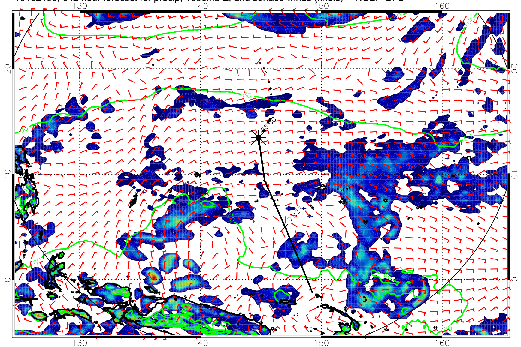
16102406, 042 hour forecast for precip, 1000mb Z, and surface winds (knots) -- NCEP GFS
