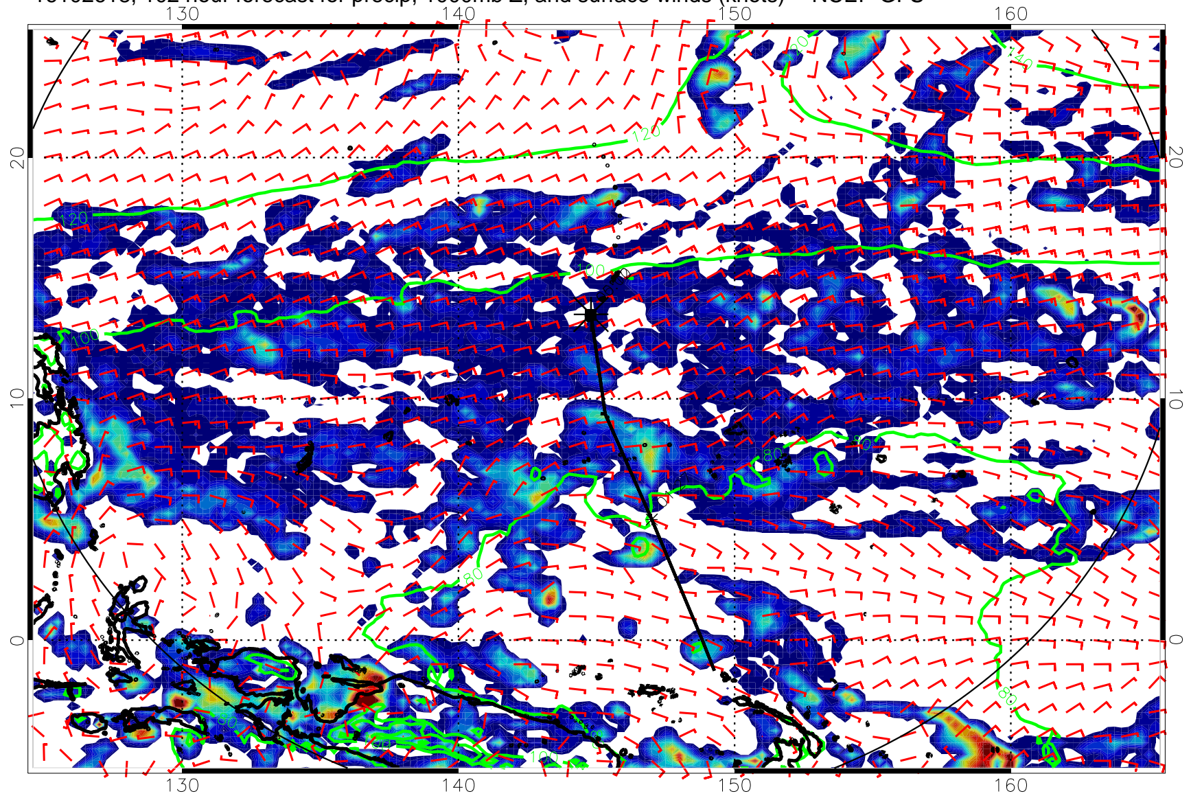
16102618, 102 hour forecast for precip, 1000mb Z, and surface winds (knots) -- NCEP GFS
