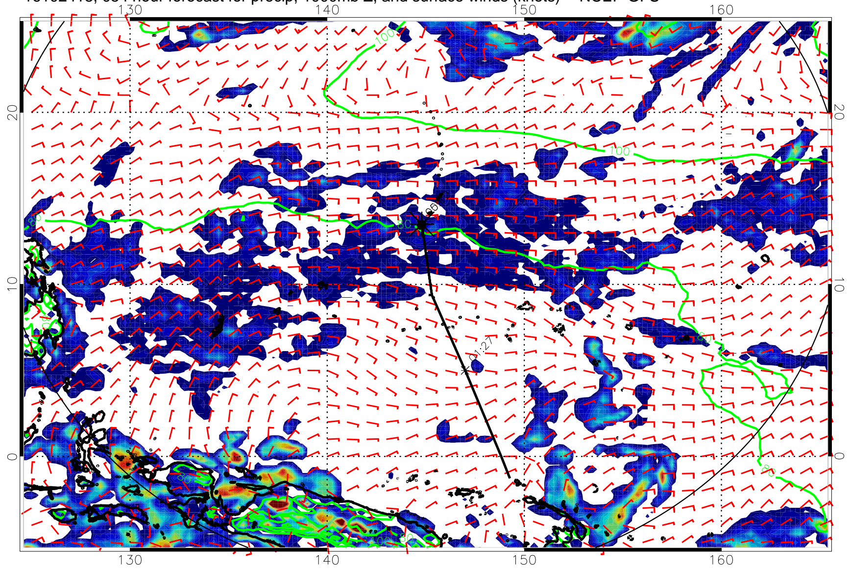
16102418, 054 hour forecast for precip, 1000mb Z, and surface winds (knots) -- NCEP GFS
