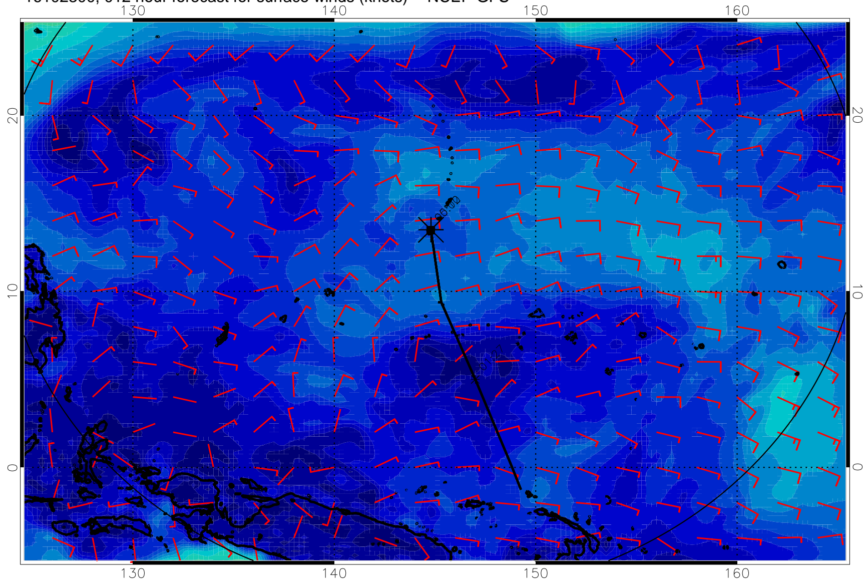
16102300, 012 hour forecast for surface winds (knots) -- NCEP GFS
