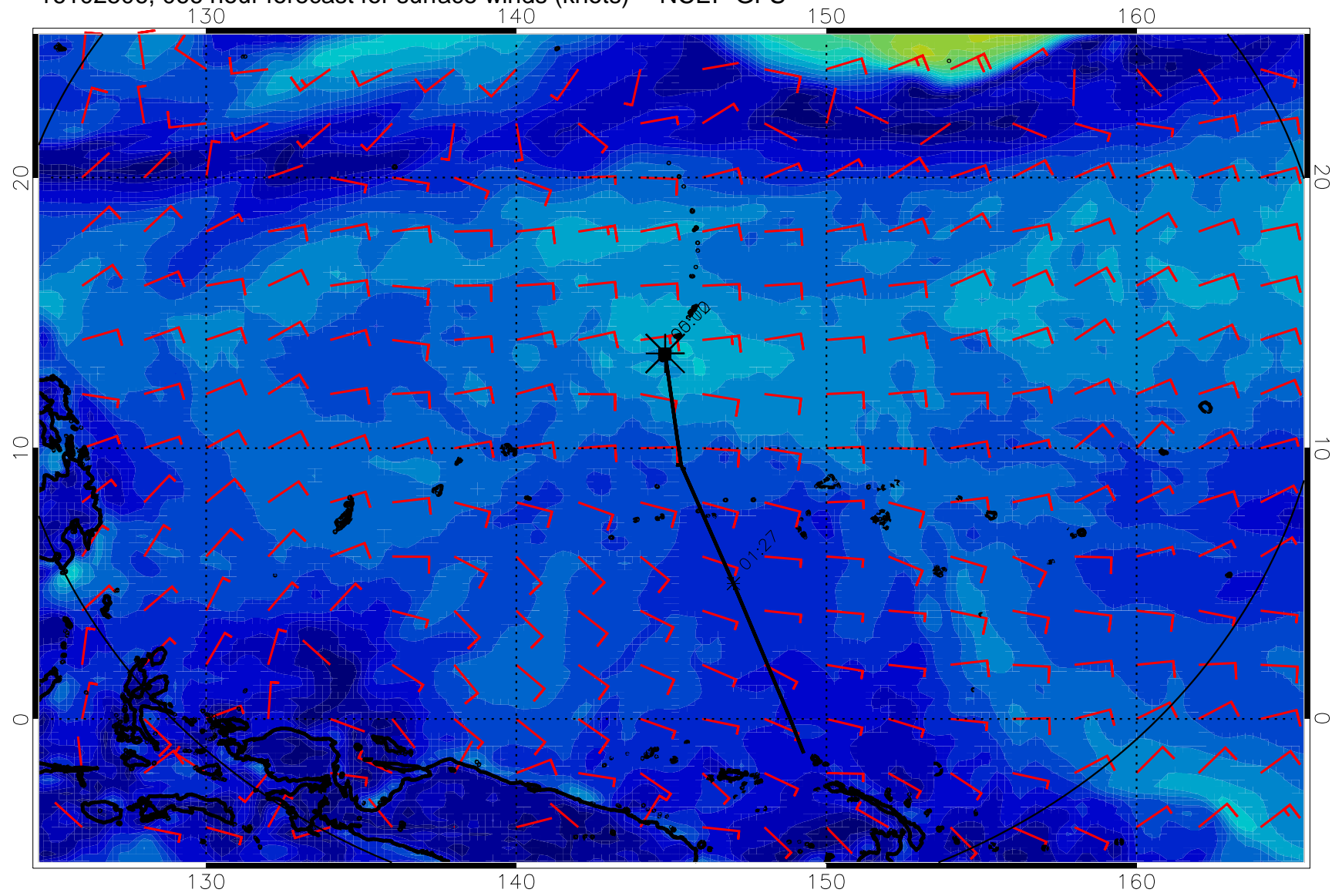
16102506, 066 hour forecast for surface winds (knots) -- NCEP GFS
