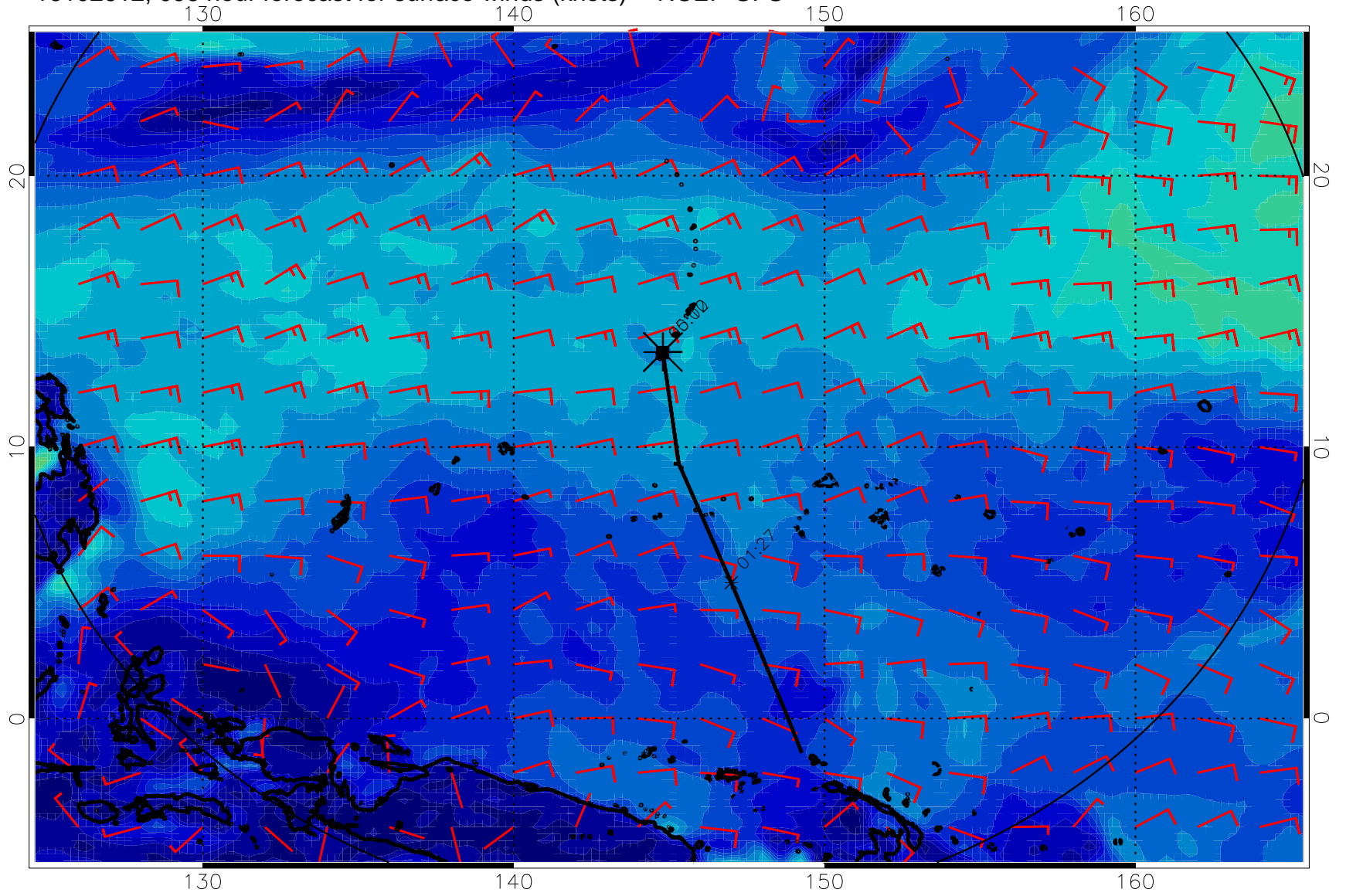
16102612, 096 hour forecast for surface winds (knots) -- NCEP GFS
