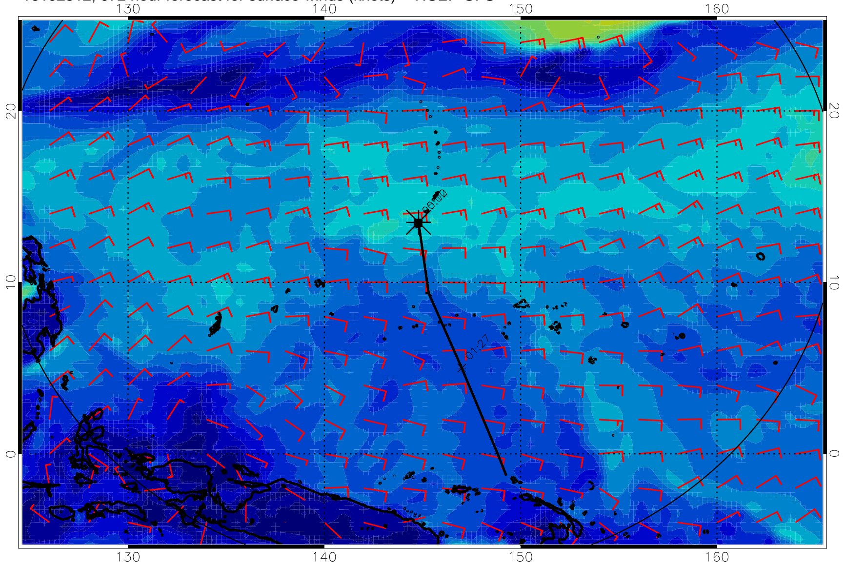
16102512, 072 hour forecast for surface winds (knots) -- NCEP GFS
