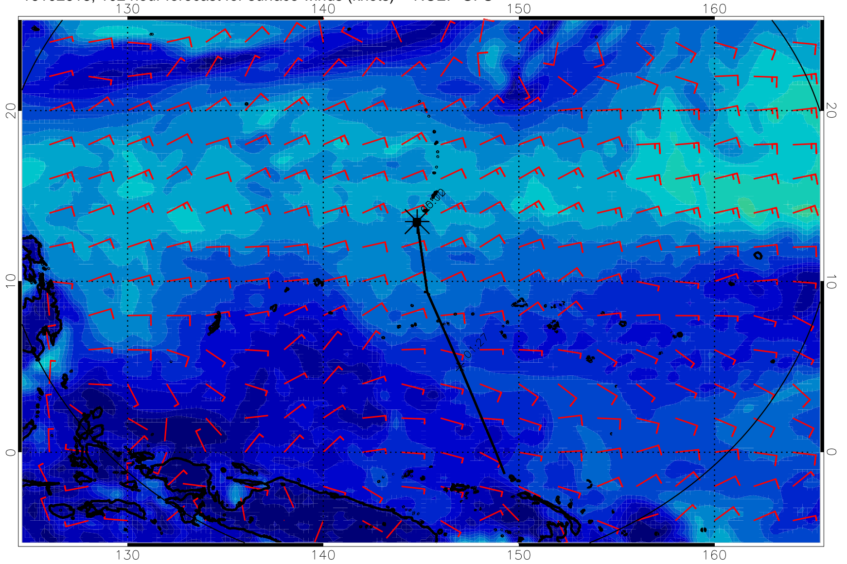
16102618, 102 hour forecast for surface winds (knots) -- NCEP GFS
