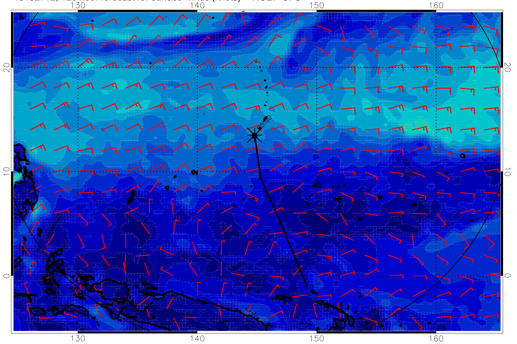
16102712, 120 hour forecast for surface winds (knots) -- NCEP GFS
