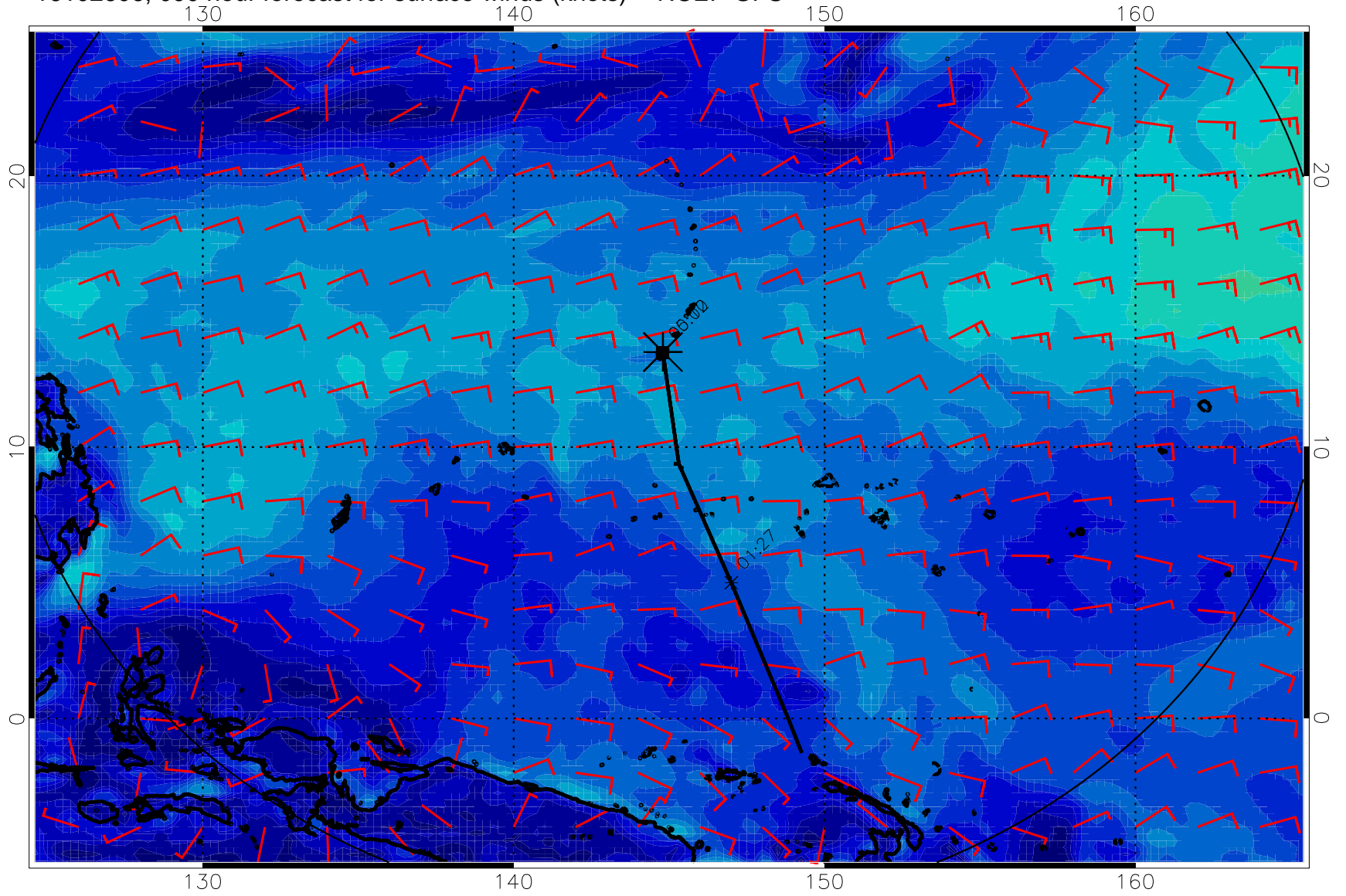
16102606, 090 hour forecast for surface winds (knots) -- NCEP GFS
