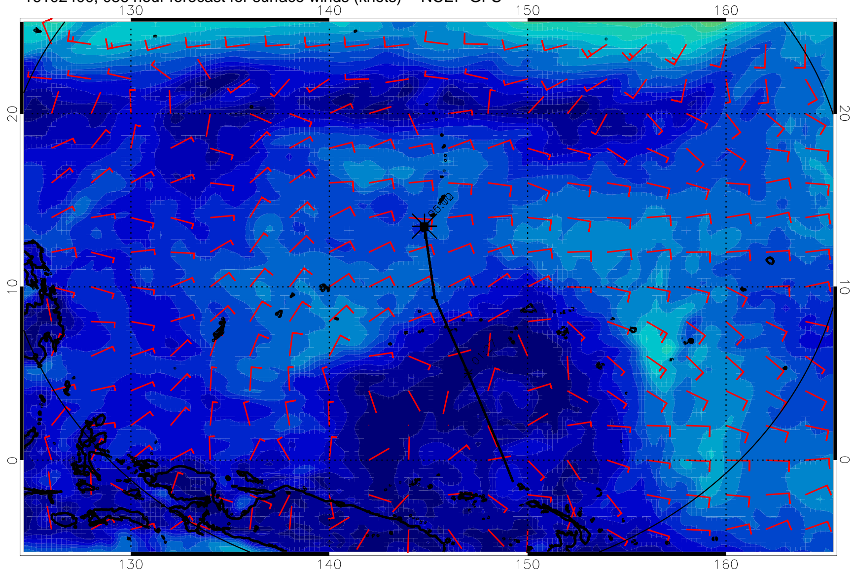
16102400, 036 hour forecast for surface winds (knots) -- NCEP GFS
