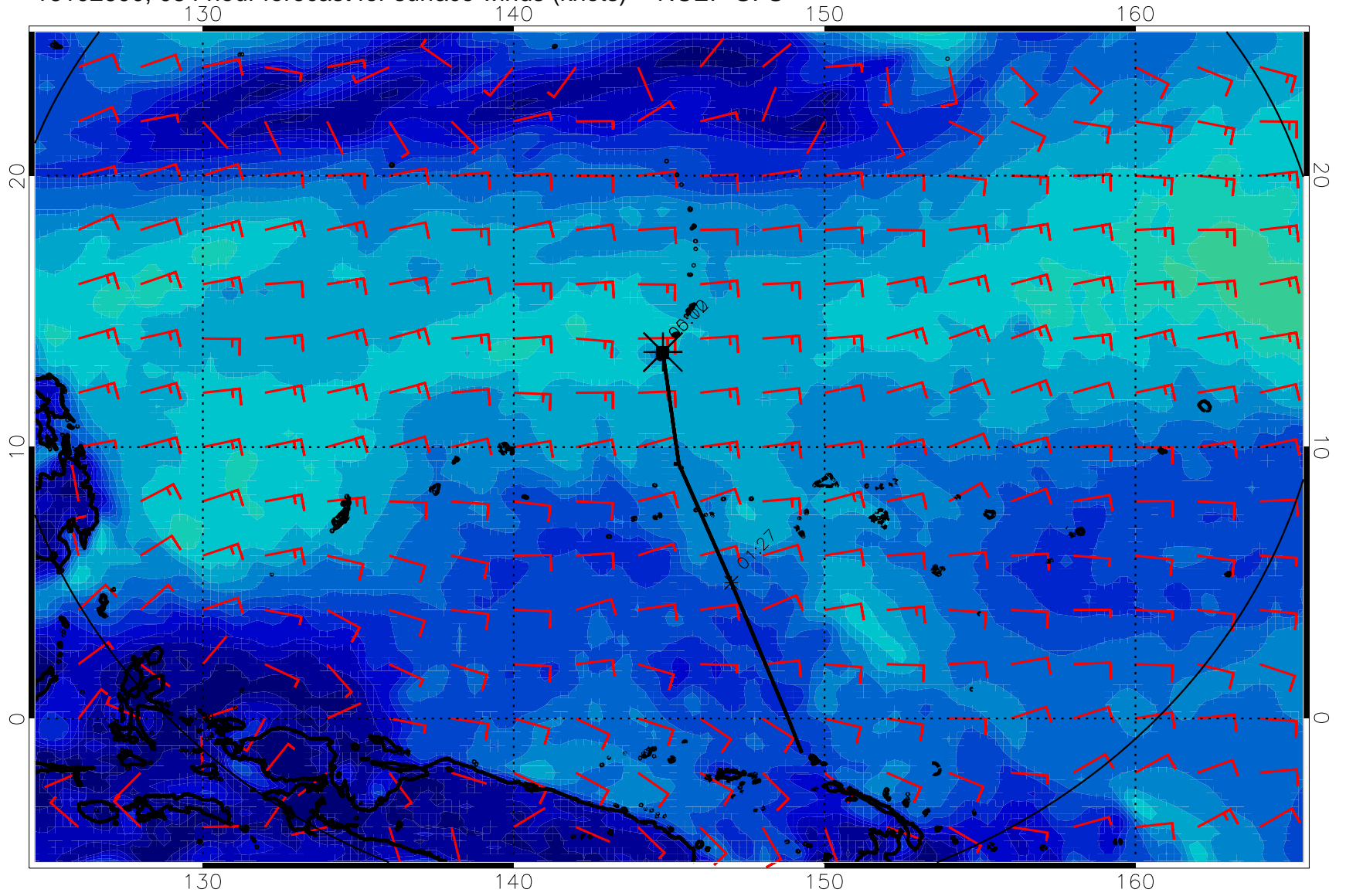
16102600, 084 hour forecast for surface winds (knots) -- NCEP GFS
