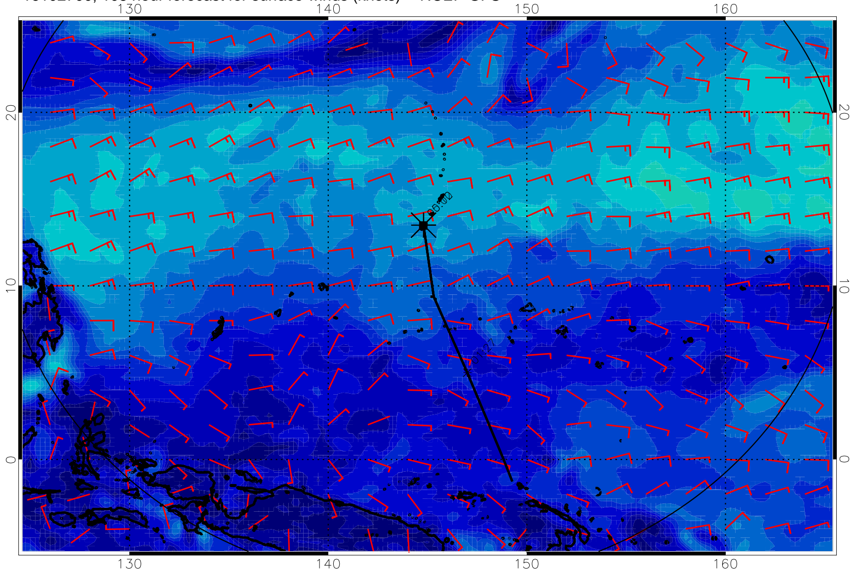
16102700, 108 hour forecast for surface winds (knots) -- NCEP GFS
