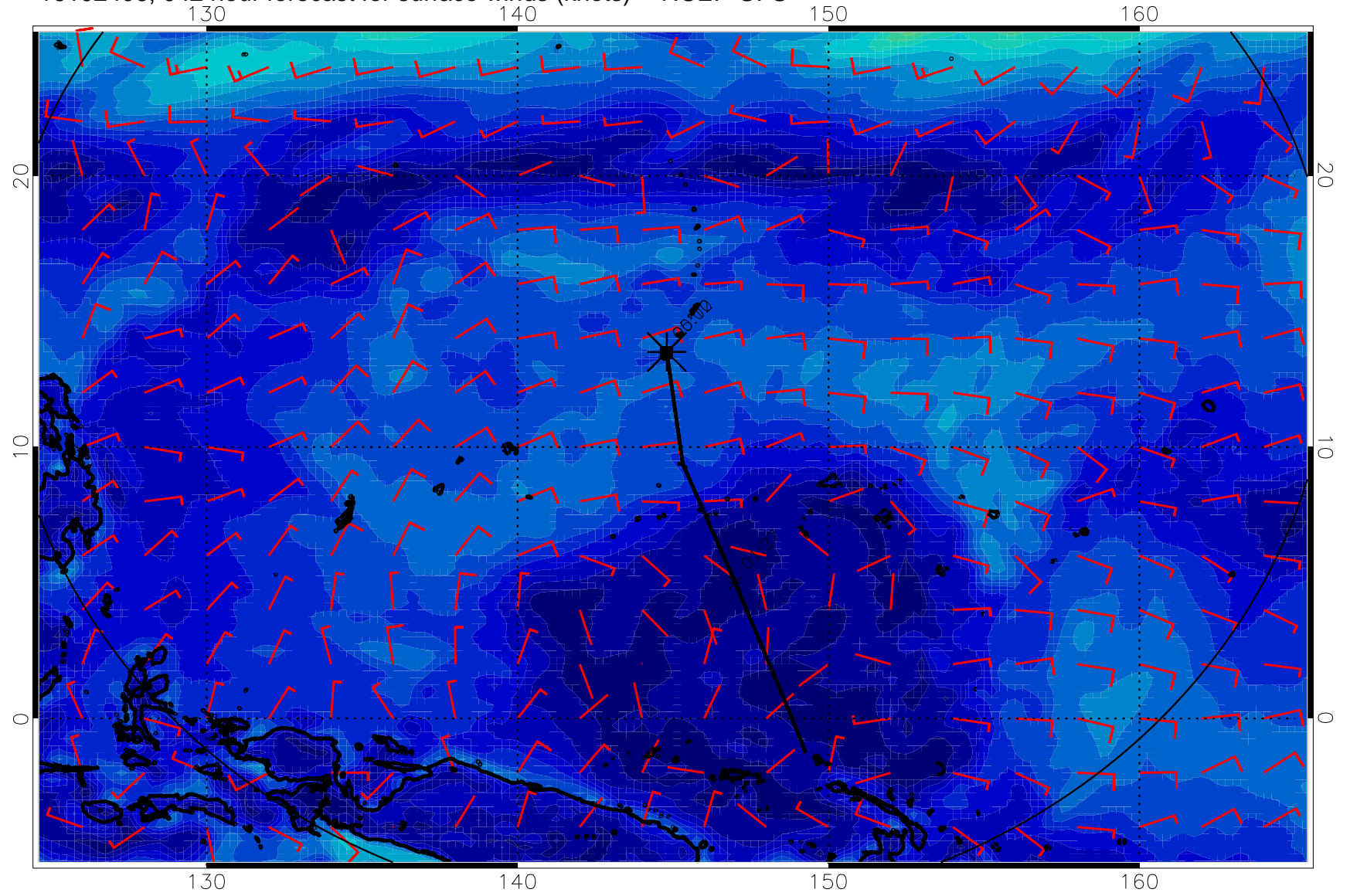
16102406, 042 hour forecast for surface winds (knots) -- NCEP GFS
