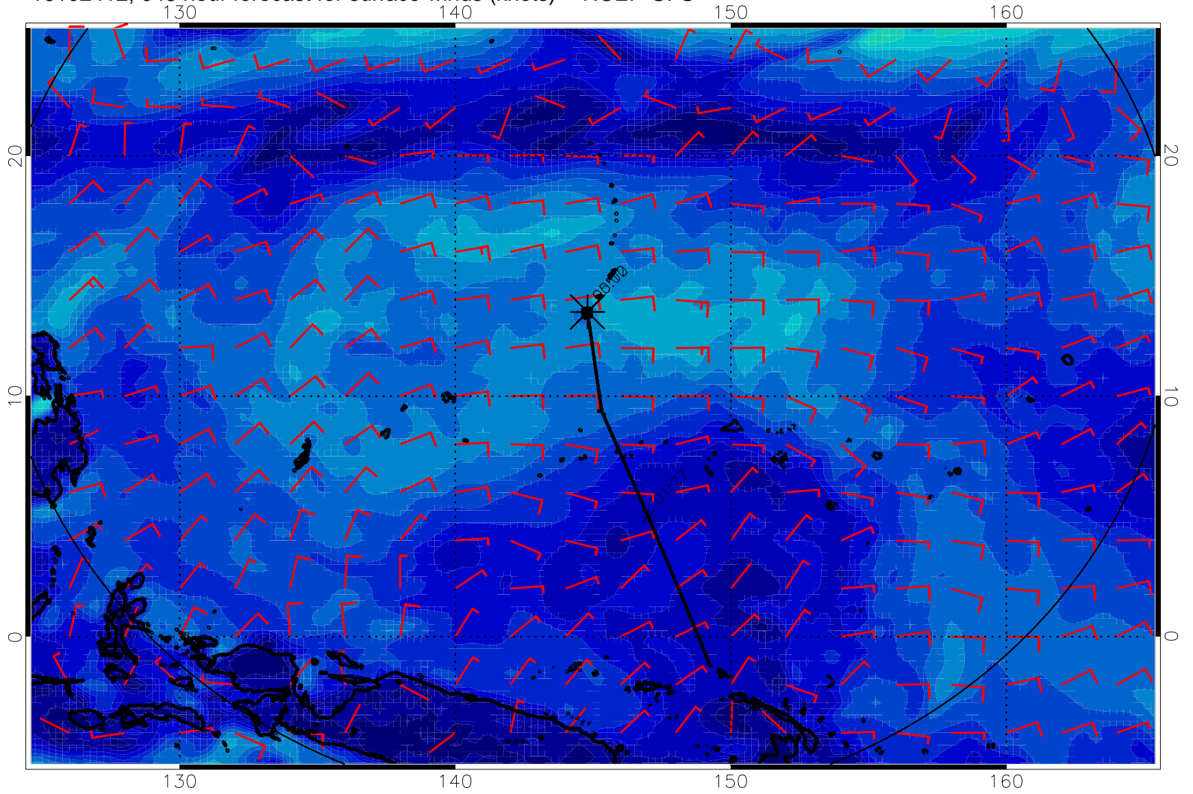
16102412, 048 hour forecast for surface winds (knots) -- NCEP GFS
