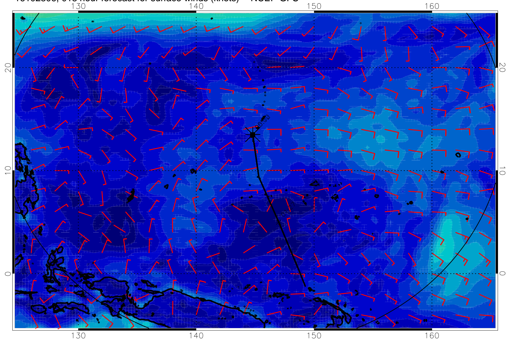
16102306, 018 hour forecast for surface winds (knots) -- NCEP GFS
