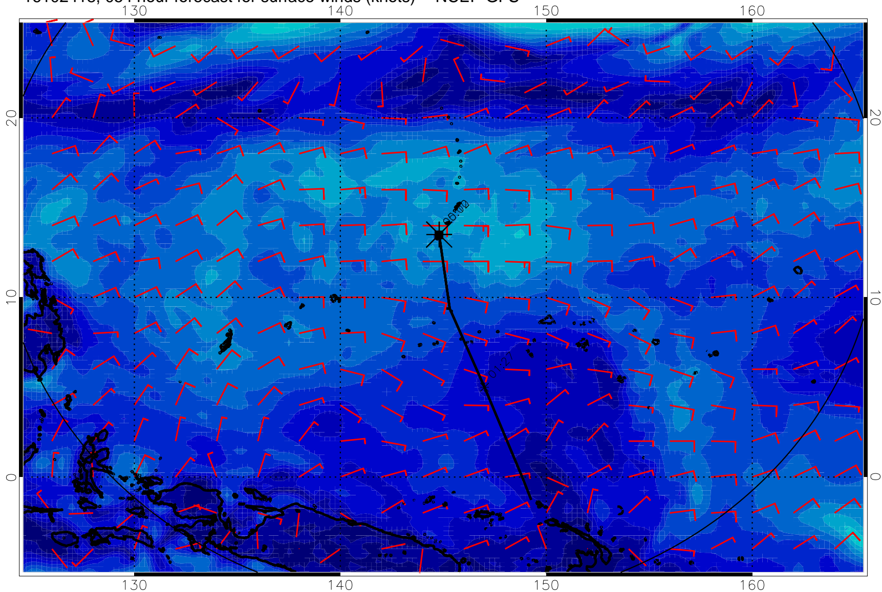
16102418, 054 hour forecast for surface winds (knots) -- NCEP GFS
