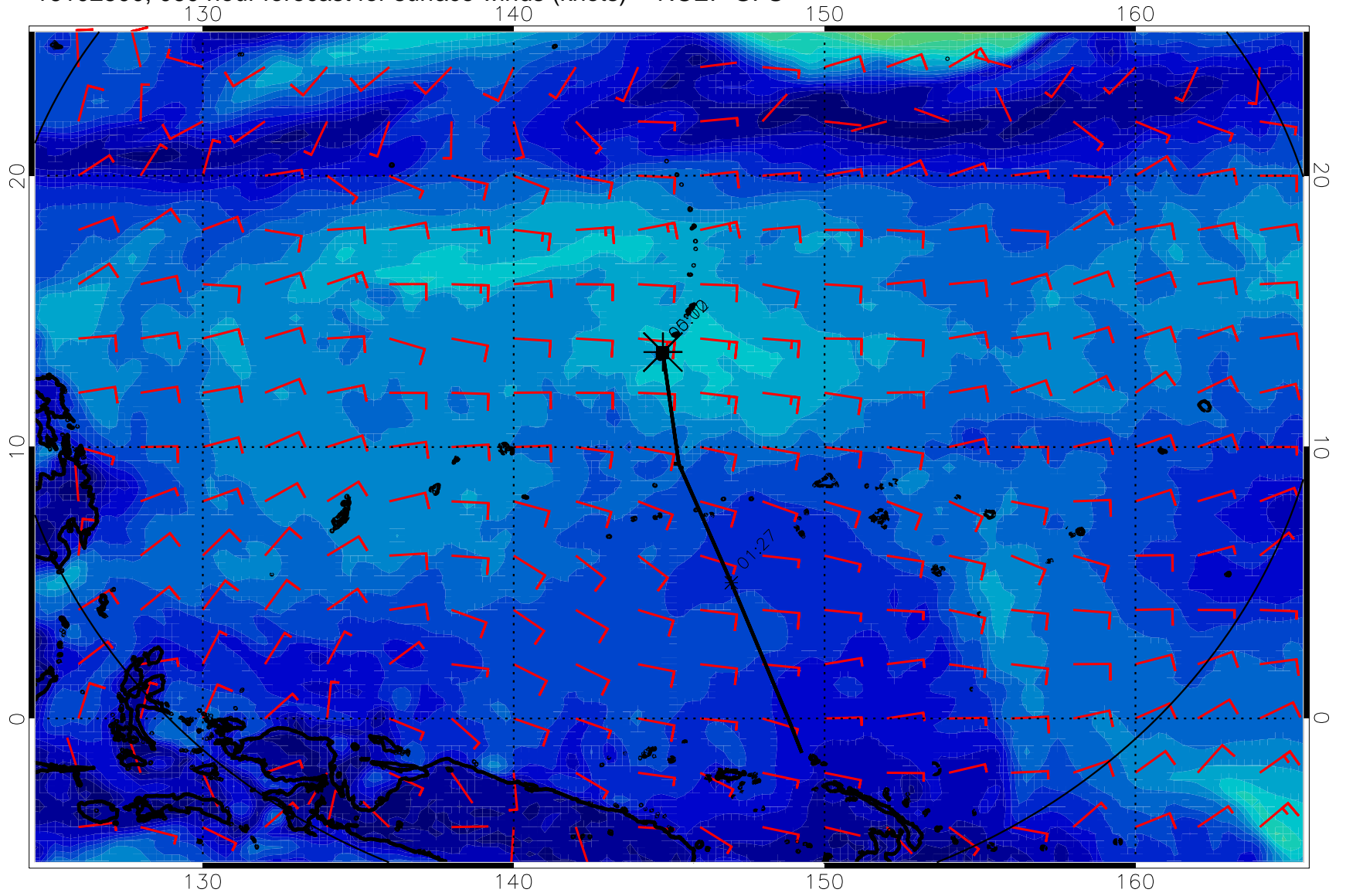
16102500, 060 hour forecast for surface winds (knots) -- NCEP GFS
