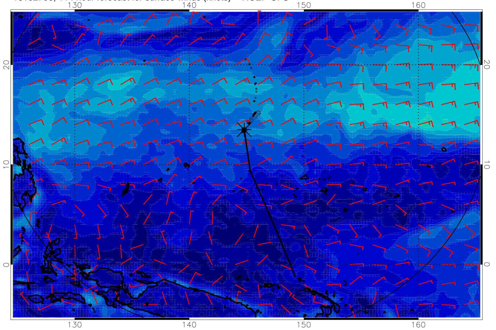
16102706, 114 hour forecast for surface winds (knots) -- NCEP GFS
