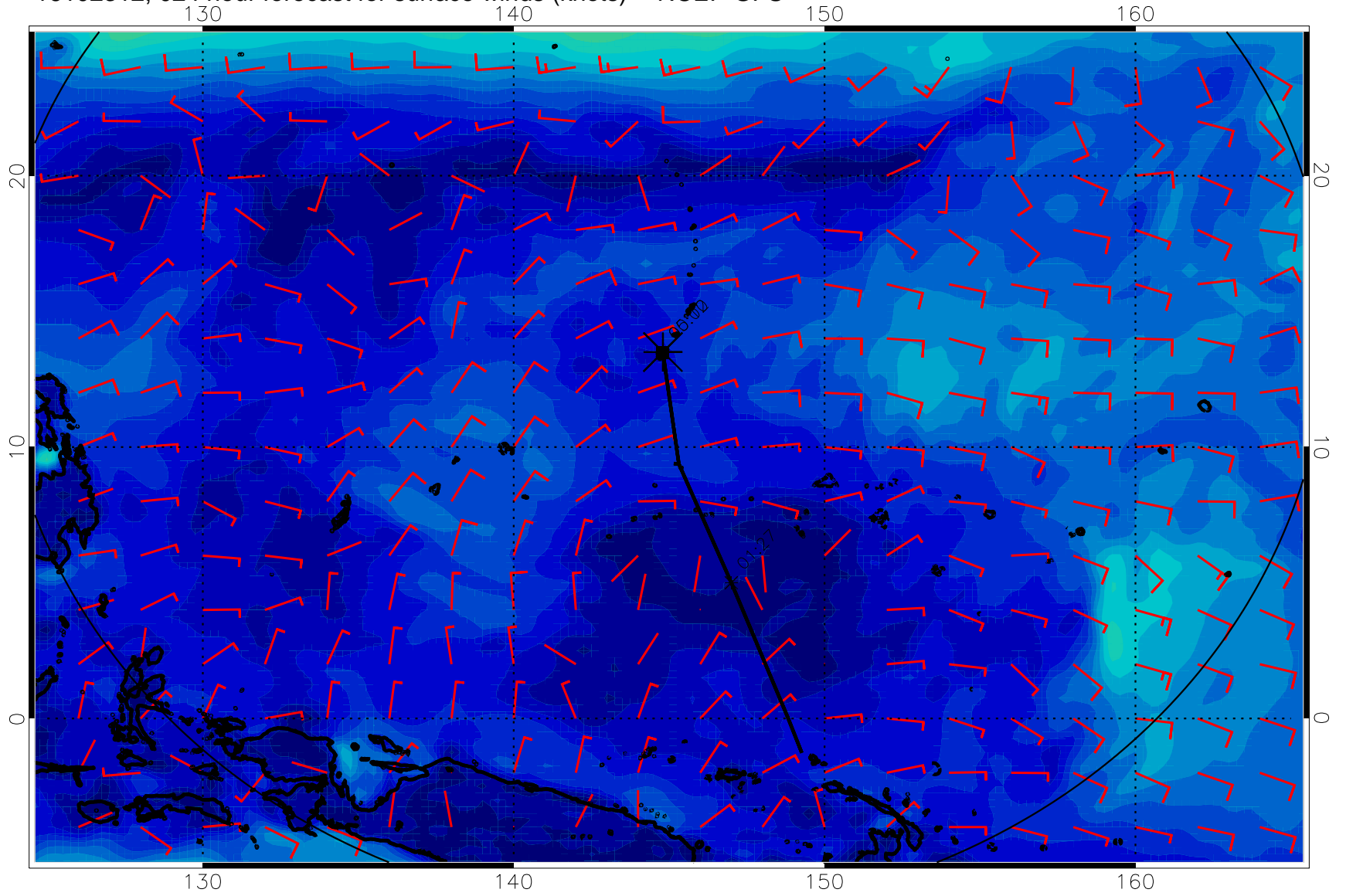
16102312, 024 hour forecast for surface winds (knots) -- NCEP GFS
