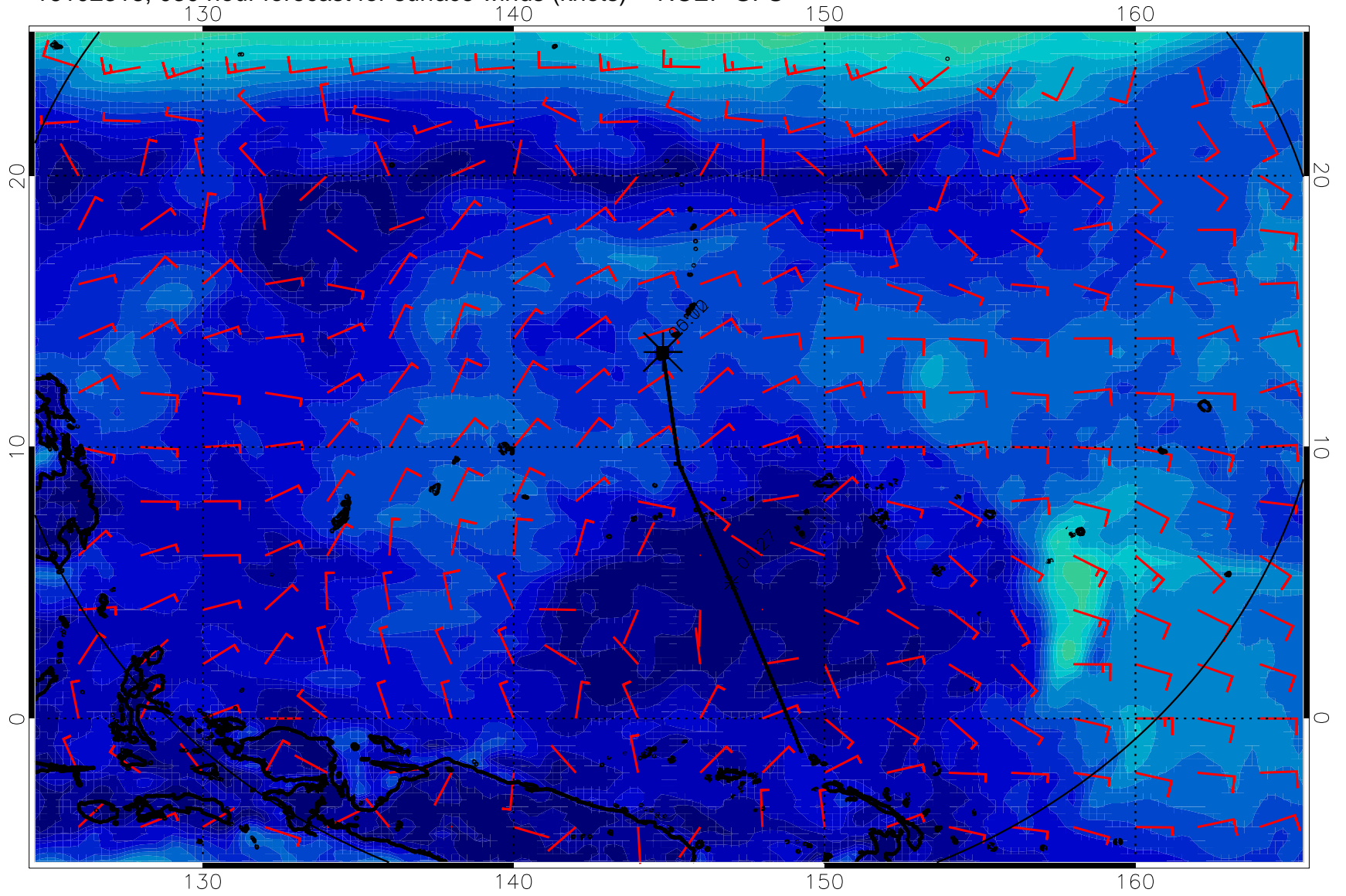
16102318, 030 hour forecast for surface winds (knots) -- NCEP GFS
