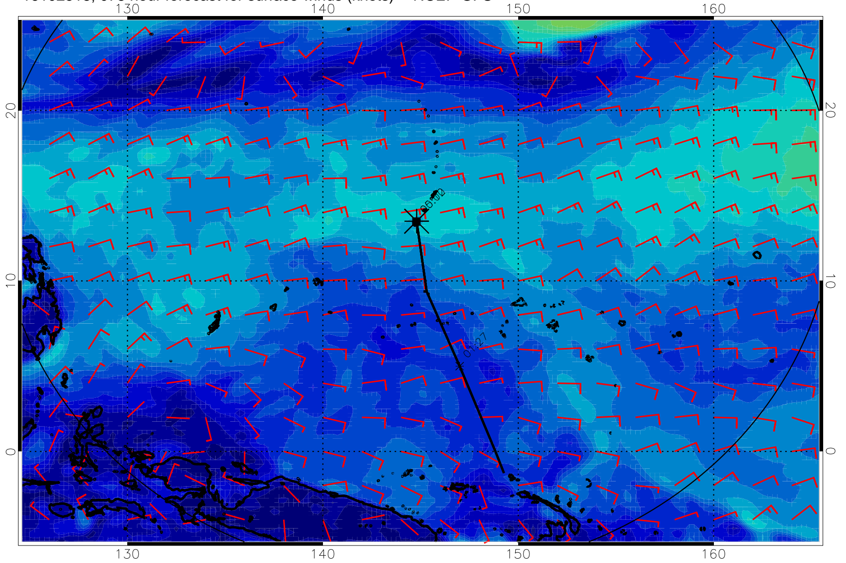
16102518, 078 hour forecast for surface winds (knots) -- NCEP GFS
