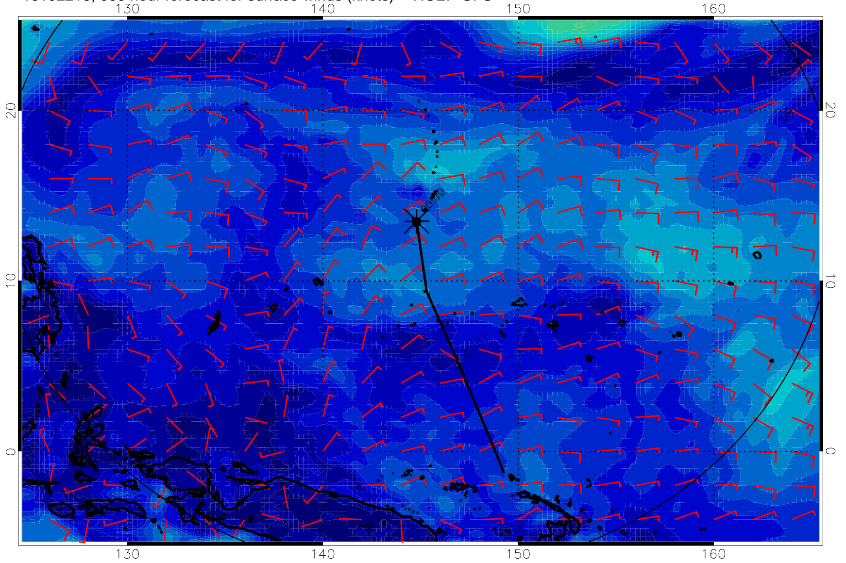
16102218, 006 hour forecast for surface winds (knots) -- NCEP GFS
