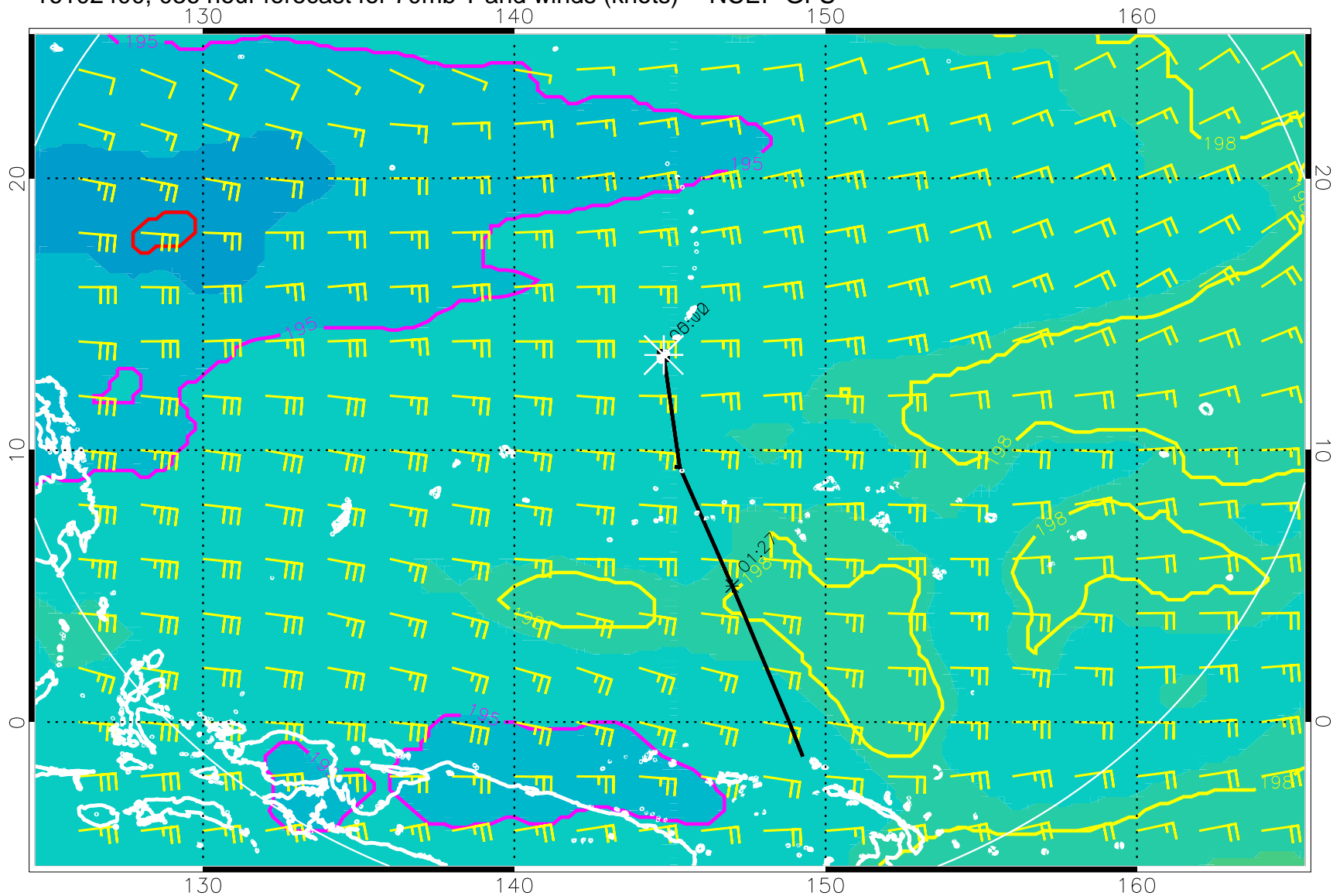
16102400, 036 hour forecast for 70mb T and winds (knots) -- NCEP GFS
