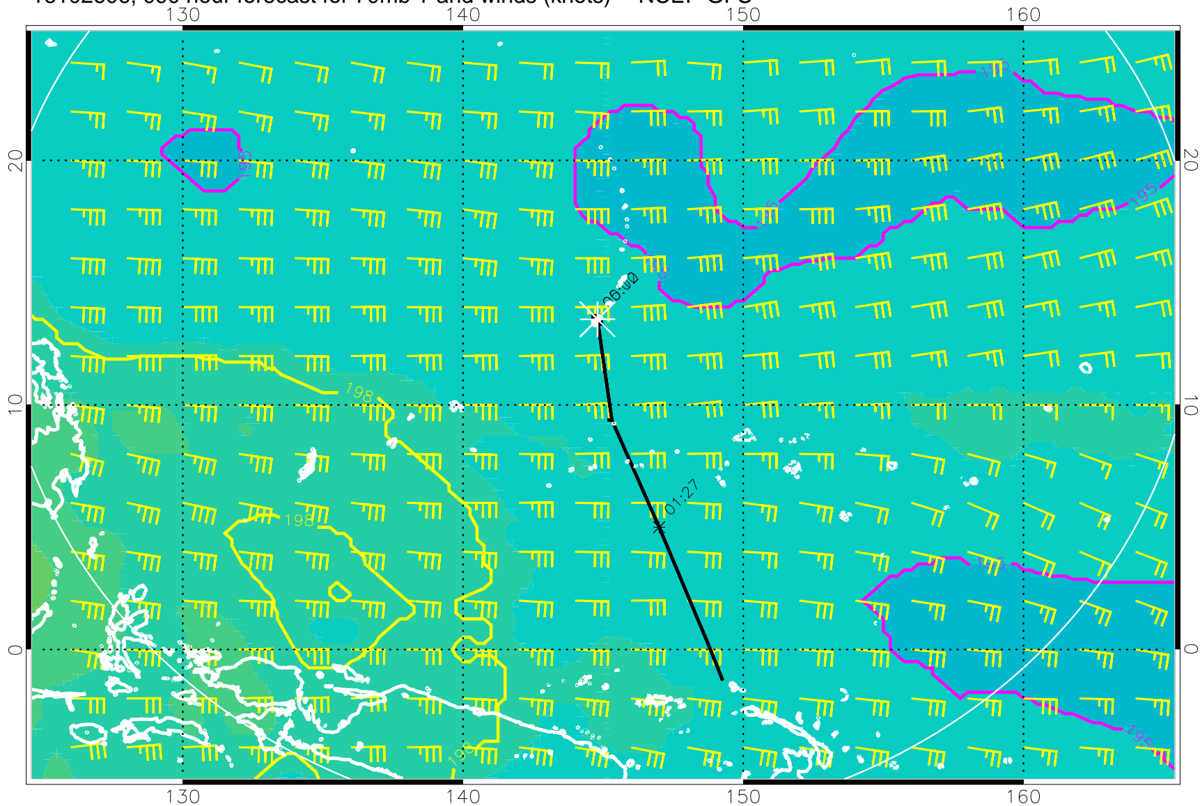
16102606, 090 hour forecast for 70mb T and winds (knots) -- NCEP GFS
