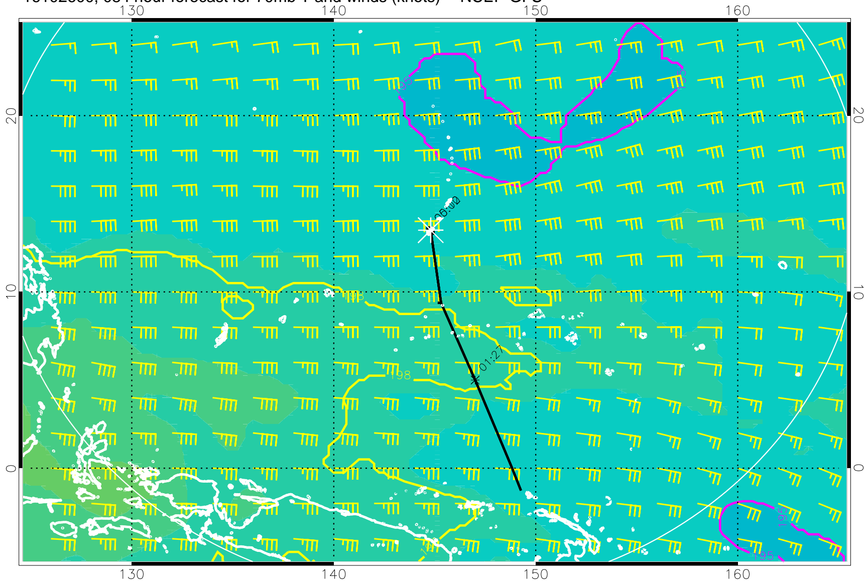
16102600, 084 hour forecast for 70mb T and winds (knots) -- NCEP GFS
