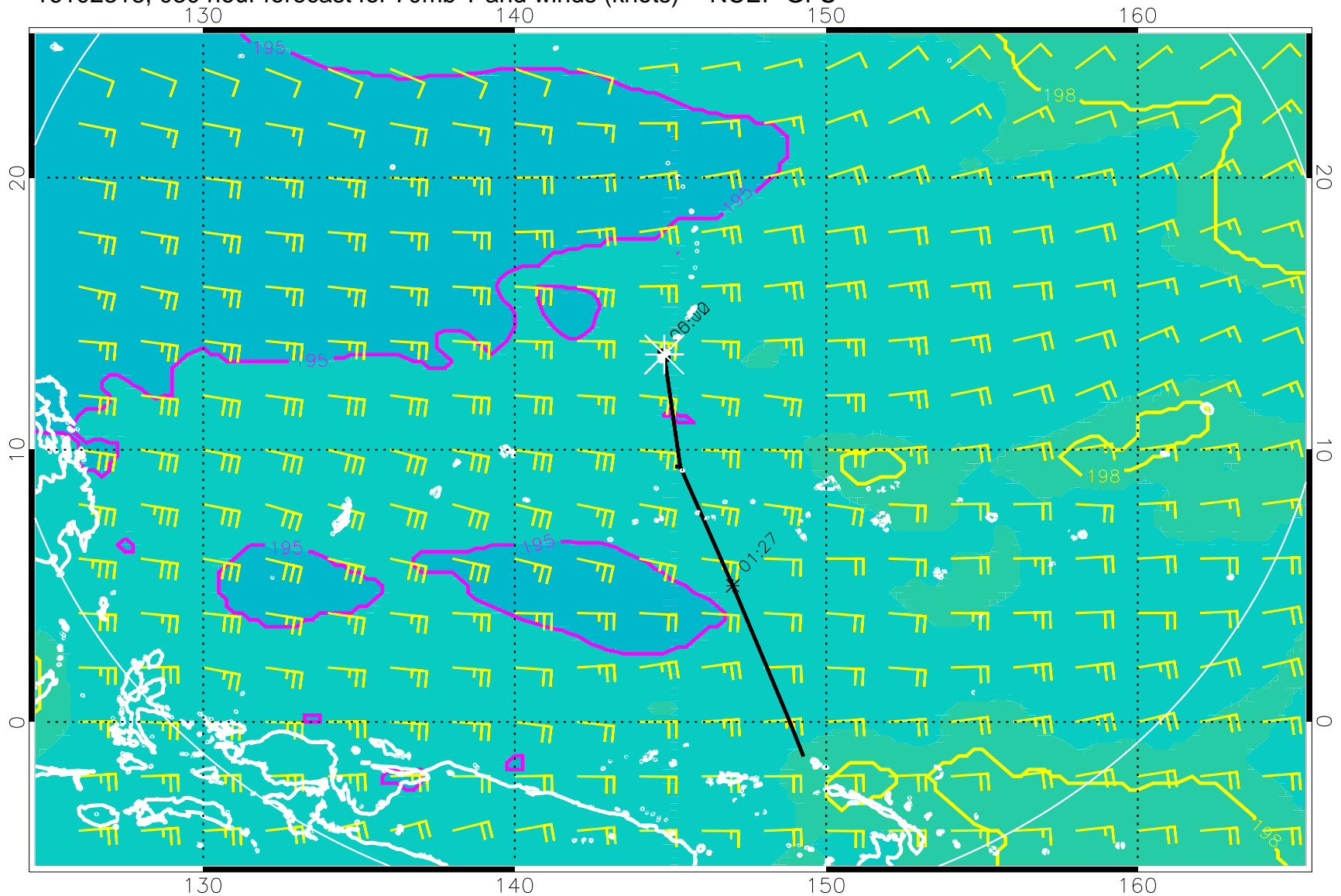
16102318, 030 hour forecast for 70mb T and winds (knots) -- NCEP GFS
