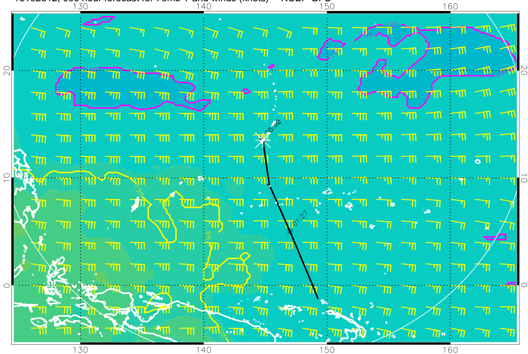
16102612, 096 hour forecast for 70mb T and winds (knots) -- NCEP GFS
