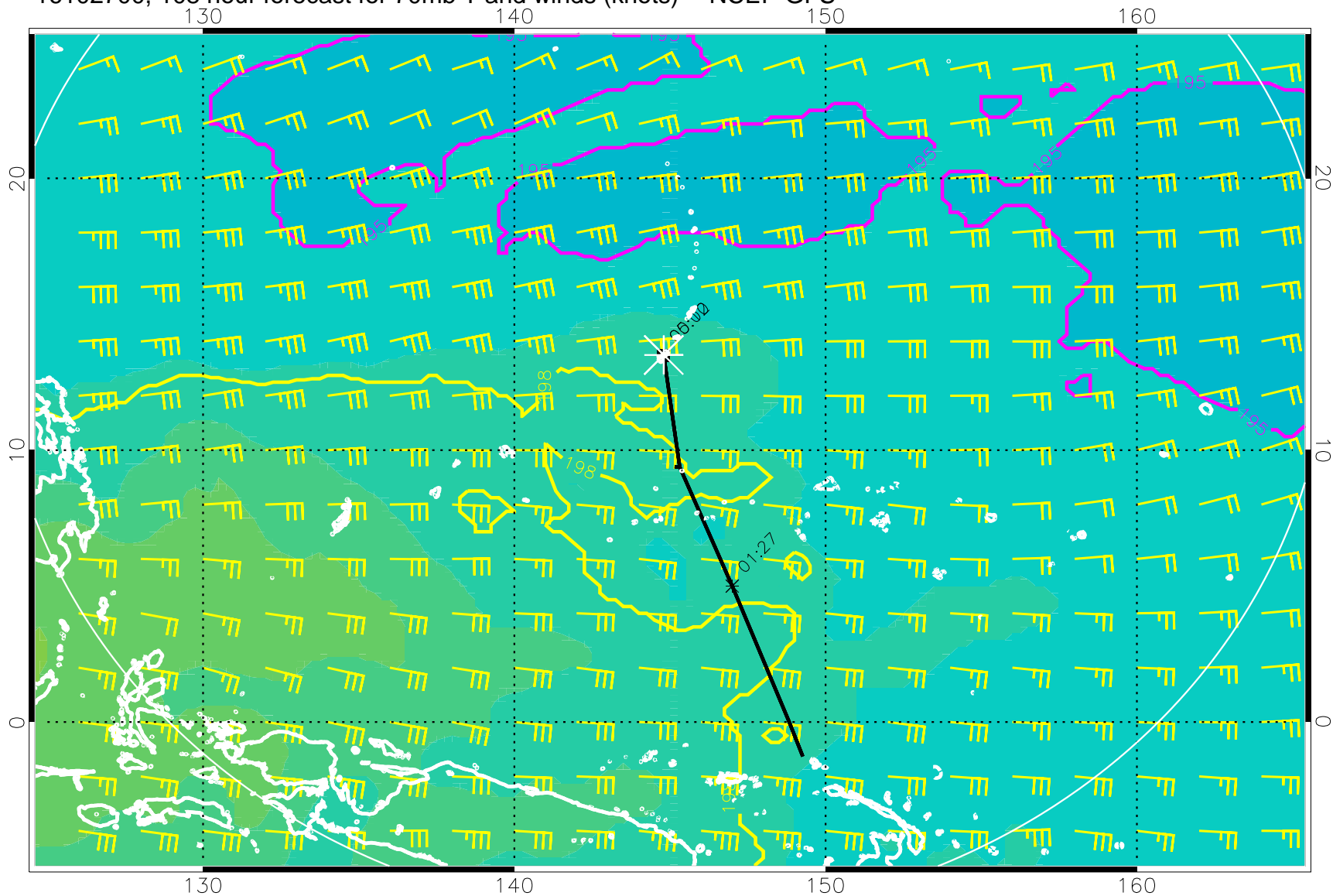
16102700, 108 hour forecast for 70mb T and winds (knots) -- NCEP GFS
