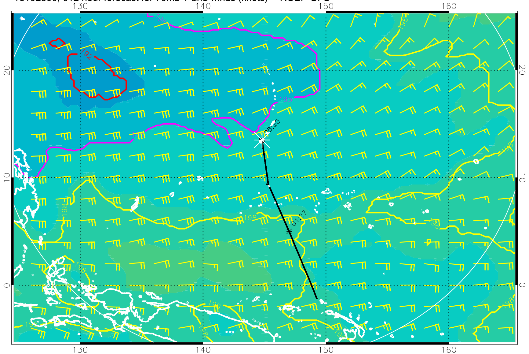
16102300, 012 hour forecast for 70mb T and winds (knots) -- NCEP GFS
