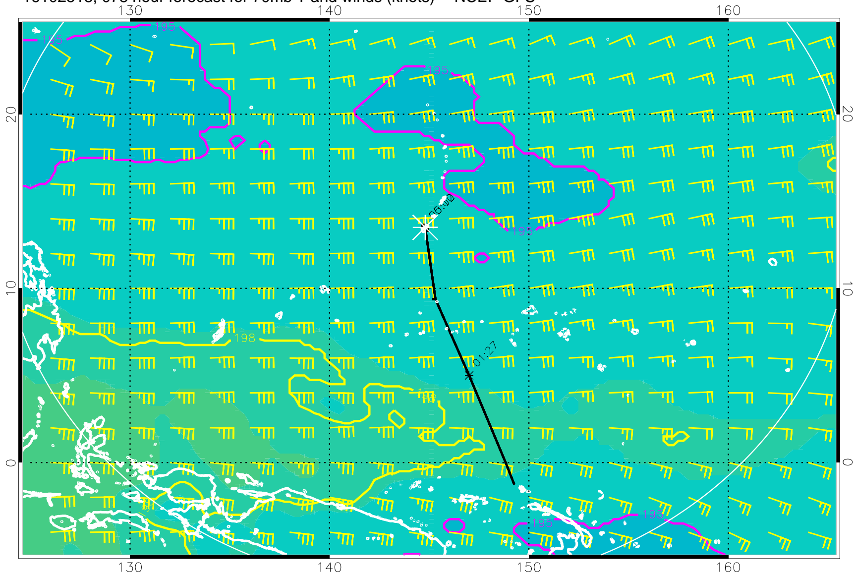
16102518, 078 hour forecast for 70mb T and winds (knots) -- NCEP GFS
