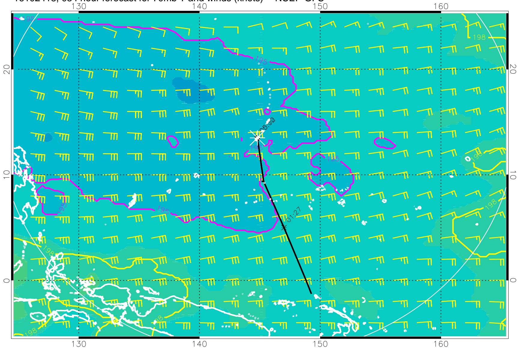
16102418, 054 hour forecast for 70mb T and winds (knots) -- NCEP GFS
