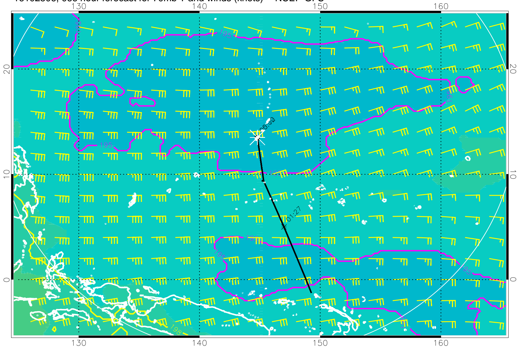
16102506, 066 hour forecast for 70mb T and winds (knots) -- NCEP GFS
