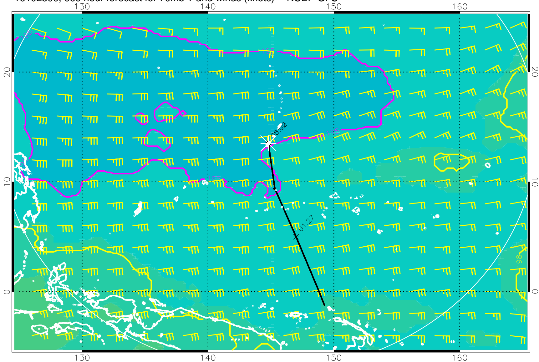
16102500, 060 hour forecast for 70mb T and winds (knots) -- NCEP GFS
