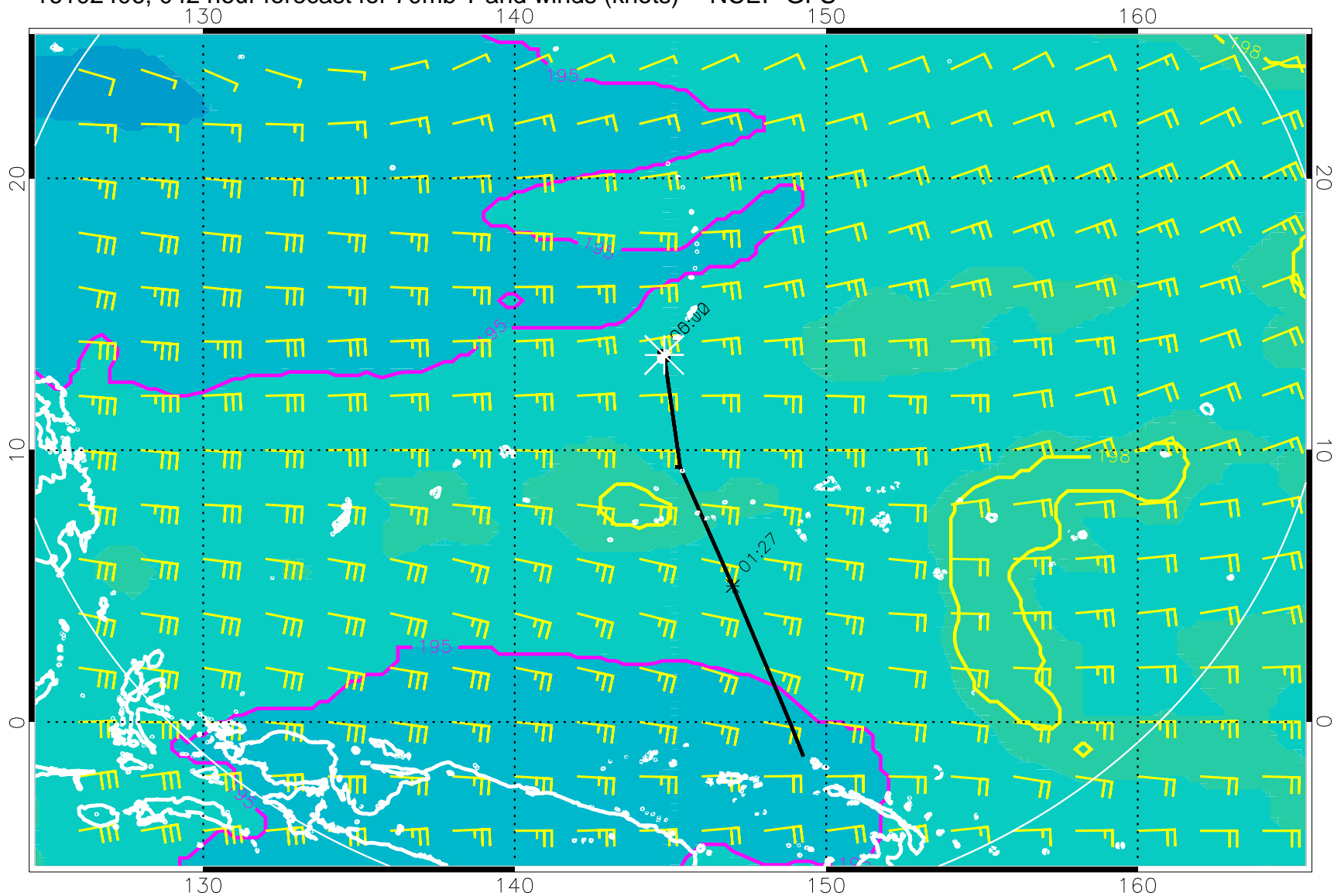
16102406, 042 hour forecast for 70mb T and winds (knots) -- NCEP GFS
