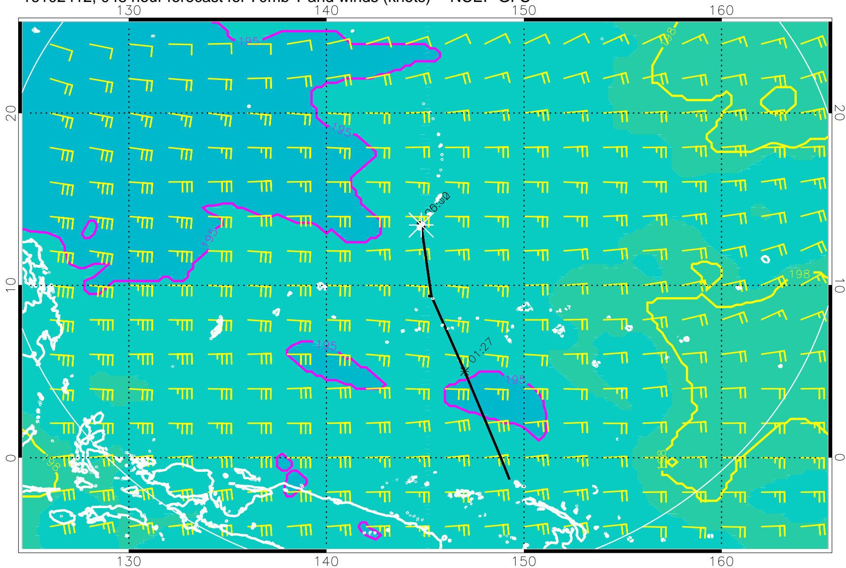
16102412, 048 hour forecast for 70mb T and winds (knots) -- NCEP GFS
