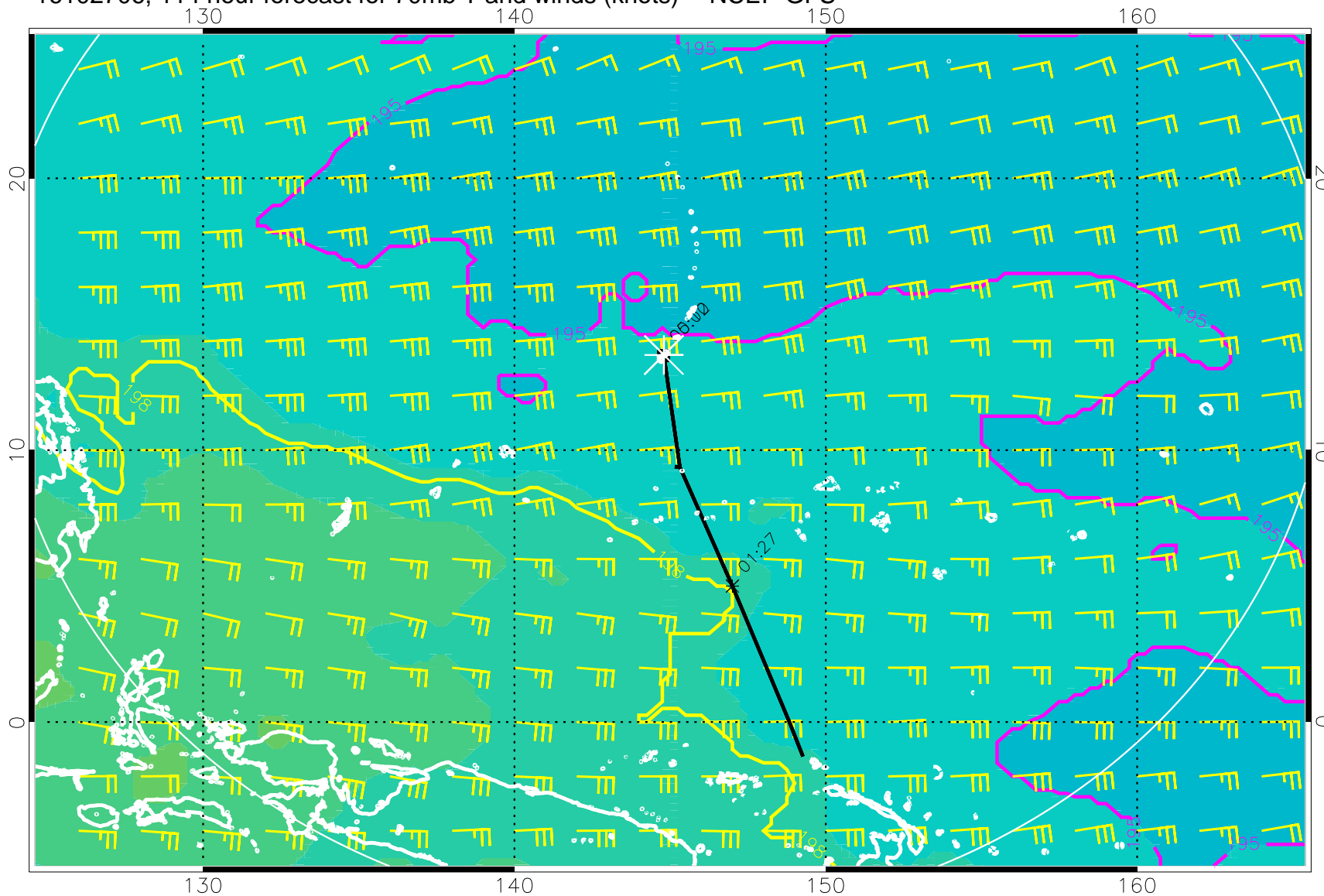
16102706, 114 hour forecast for 70mb T and winds (knots) -- NCEP GFS
