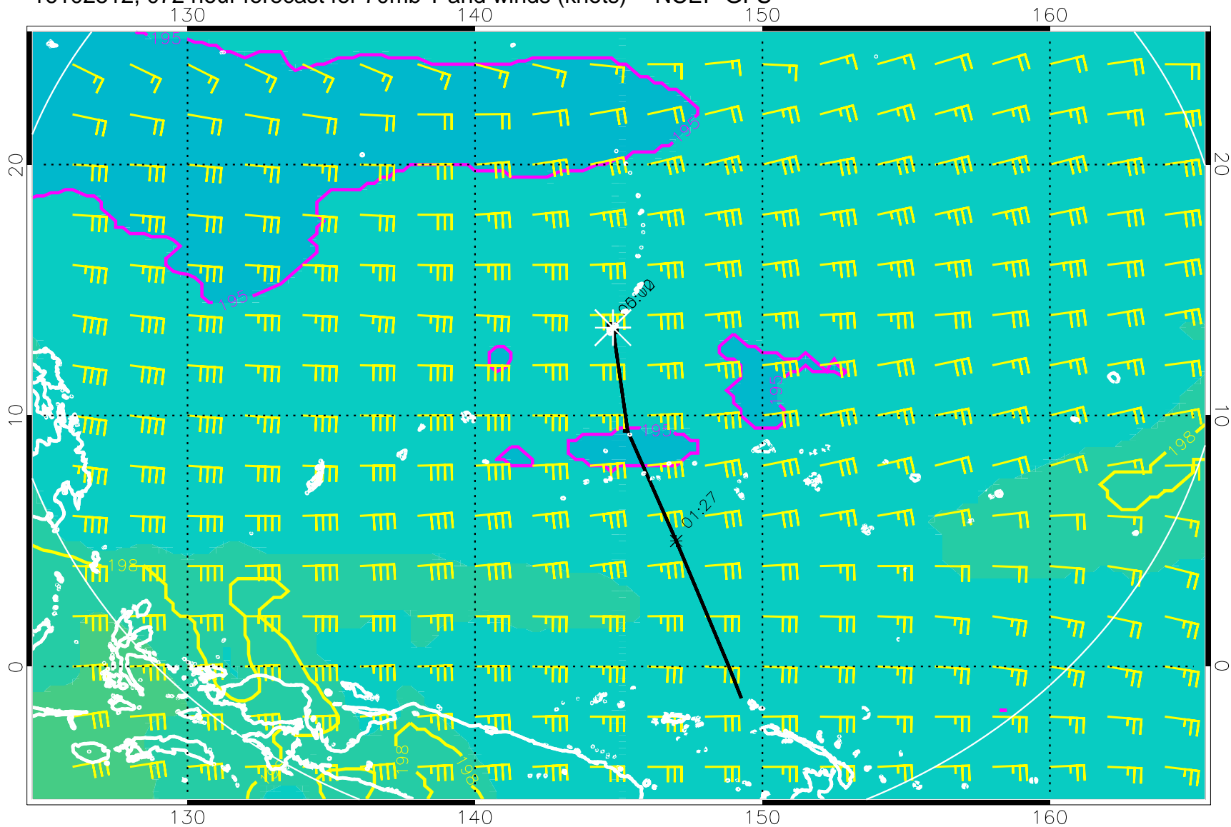
16102512, 072 hour forecast for 70mb T and winds (knots) -- NCEP GFS
