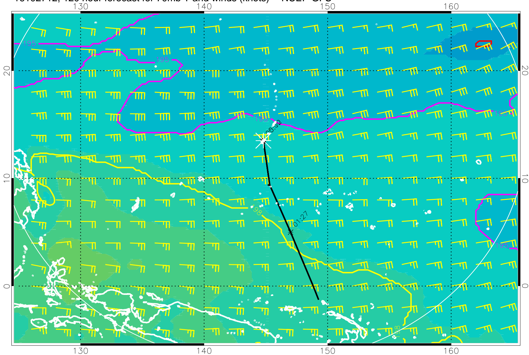
16102712, 120 hour forecast for 70mb T and winds (knots) -- NCEP GFS
