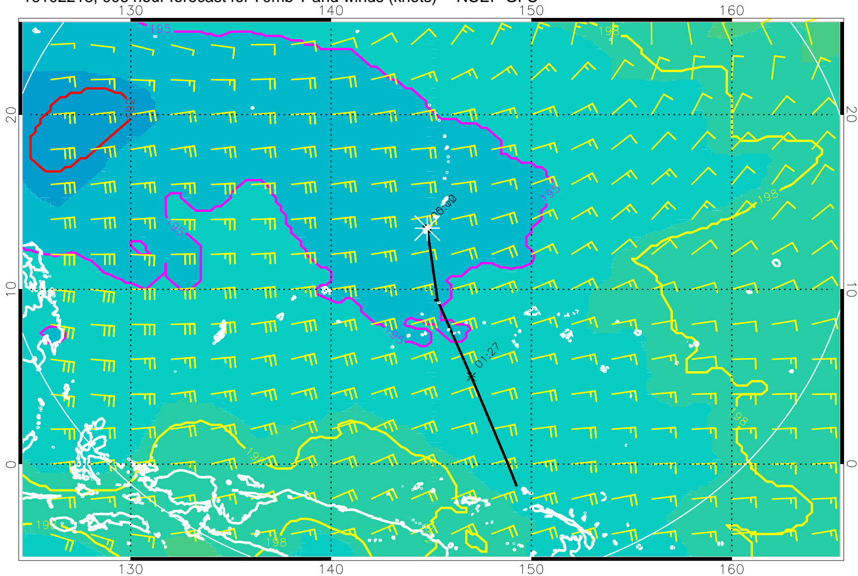
16102218, 006 hour forecast for 70mb T and winds (knots) -- NCEP GFS
