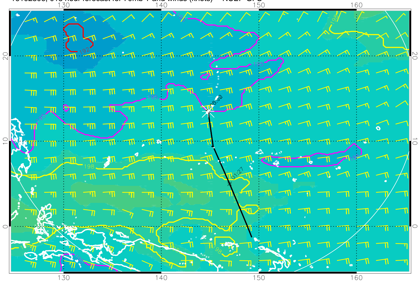
16102306, 018 hour forecast for 70mb T and winds (knots) -- NCEP GFS
