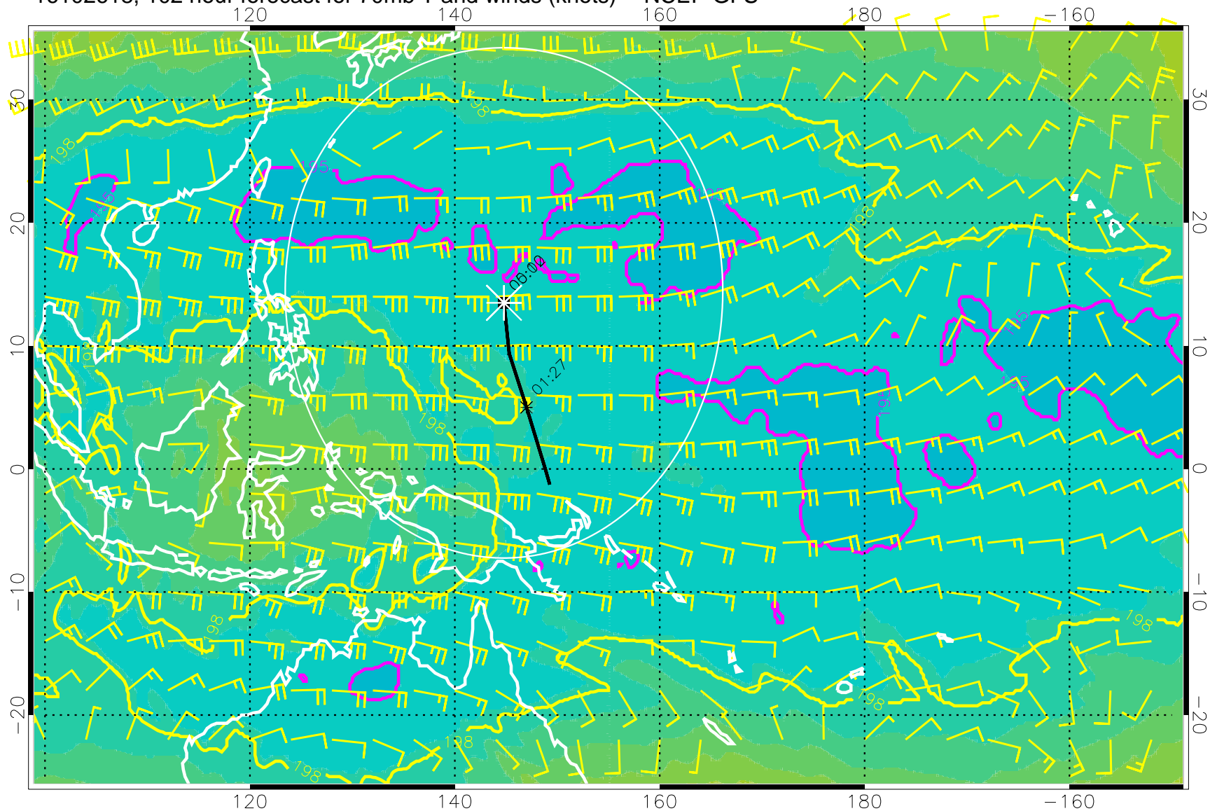
16102618, 102 hour forecast for 70mb T and winds (knots) -- NCEP GFS
