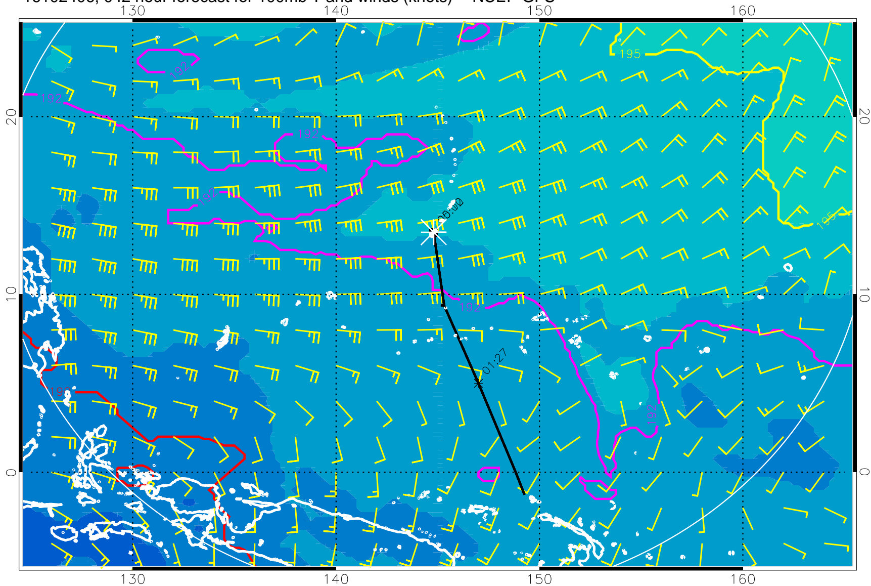
16102406, 042 hour forecast for 100mb T and winds (knots) -- NCEP GFS
