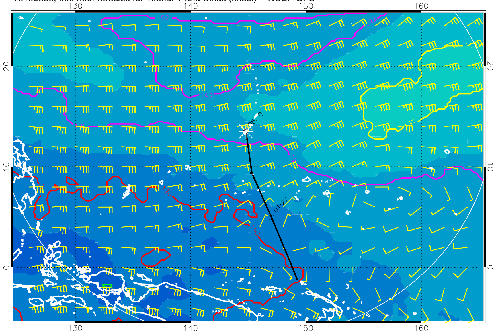
16102606, 090 hour forecast for 100mb T and winds (knots) -- NCEP GFS
