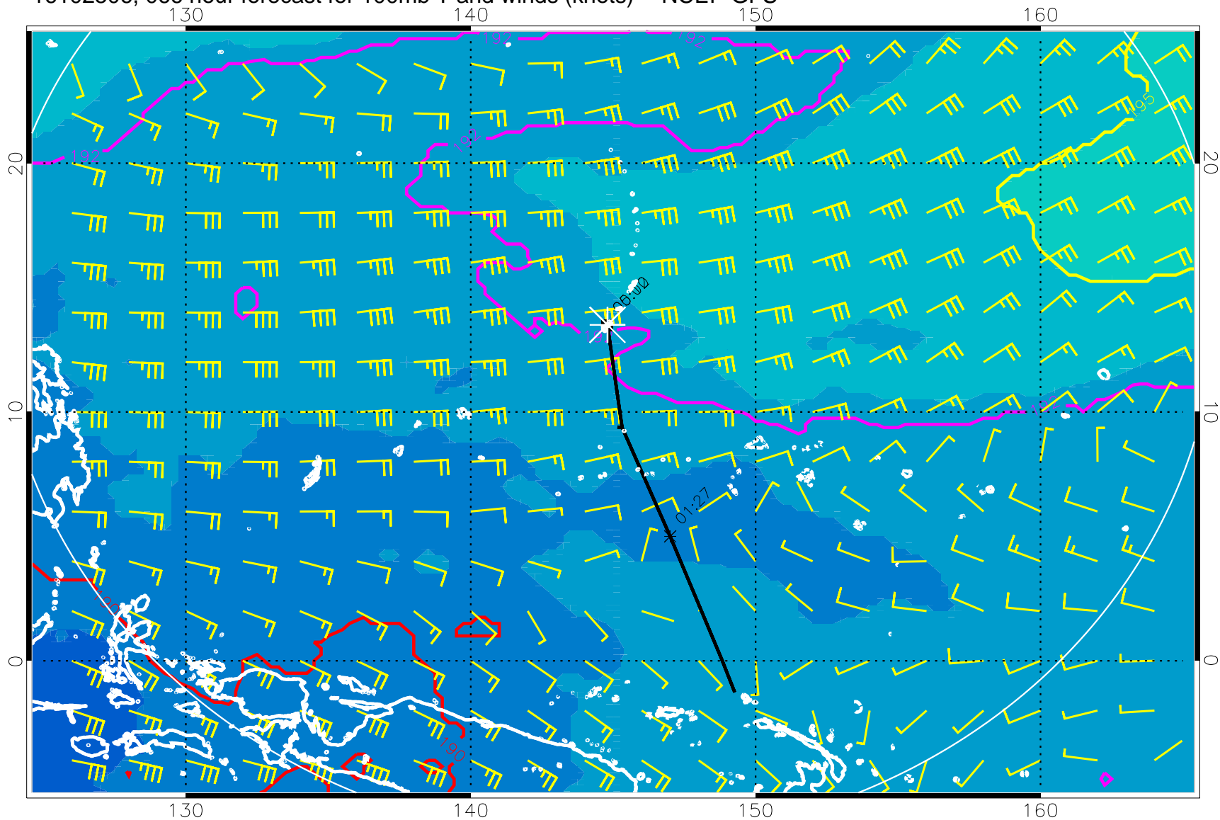
16102506, 066 hour forecast for 100mb T and winds (knots) -- NCEP GFS
