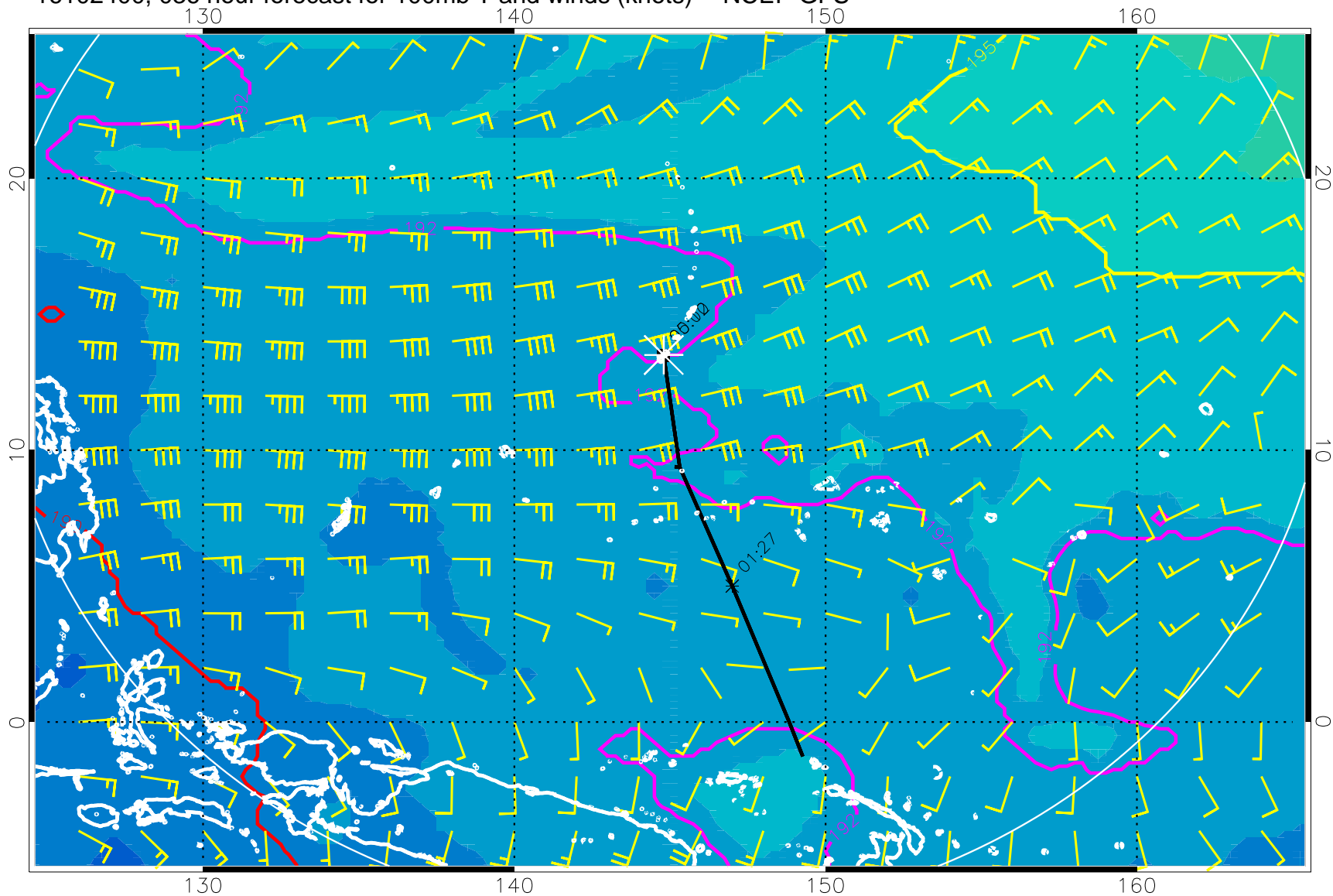
16102400, 036 hour forecast for 100mb T and winds (knots) -- NCEP GFS
