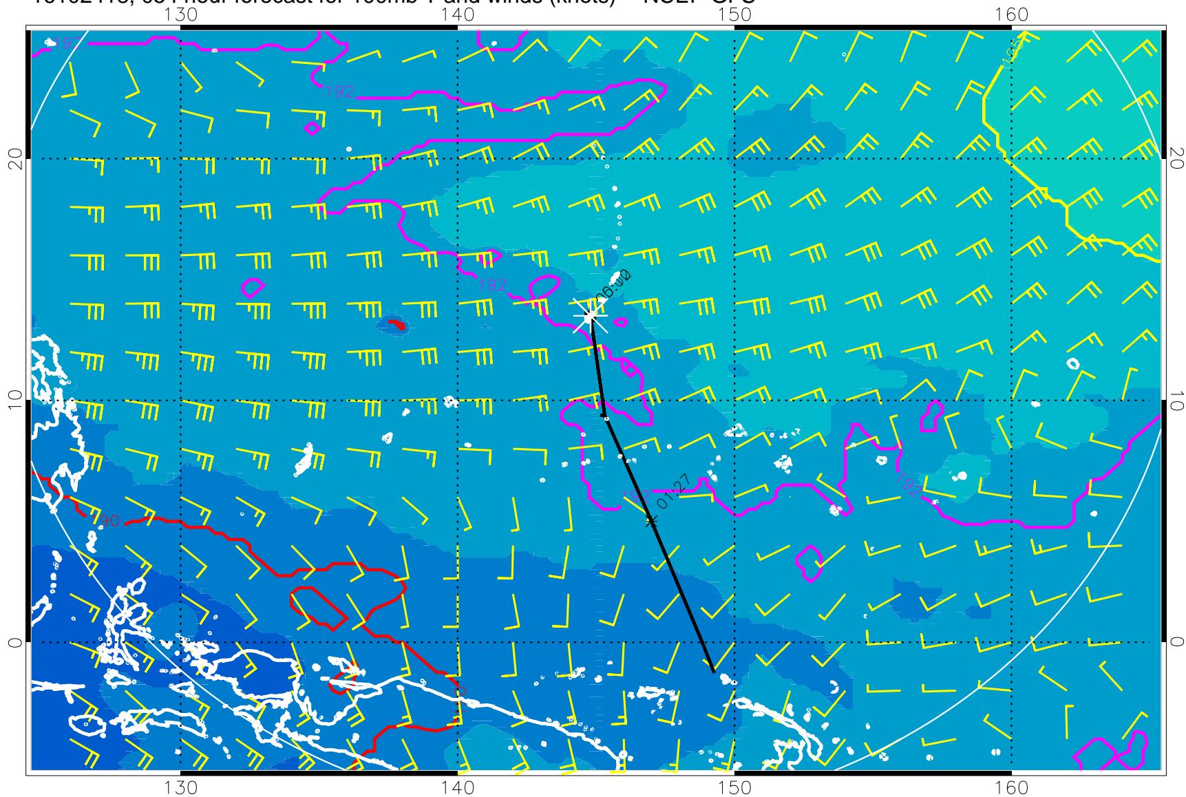
16102418, 054 hour forecast for 100mb T and winds (knots) -- NCEP GFS
