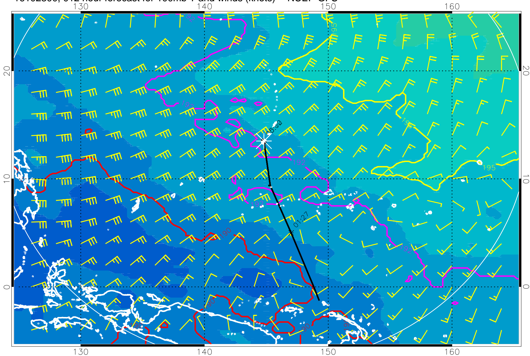
16102300, 012 hour forecast for 100mb T and winds (knots) -- NCEP GFS
