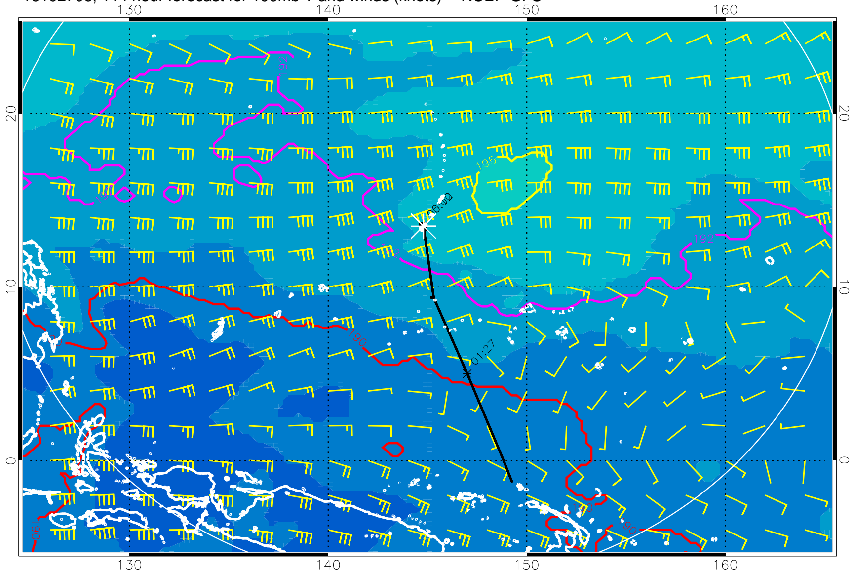
16102706, 114 hour forecast for 100mb T and winds (knots) -- NCEP GFS
