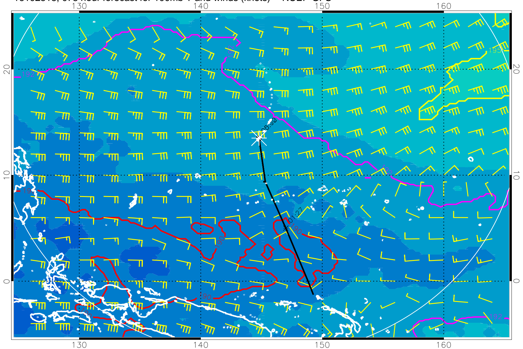
16102518, 078 hour forecast for 100mb T and winds (knots) -- NCEP GFS
