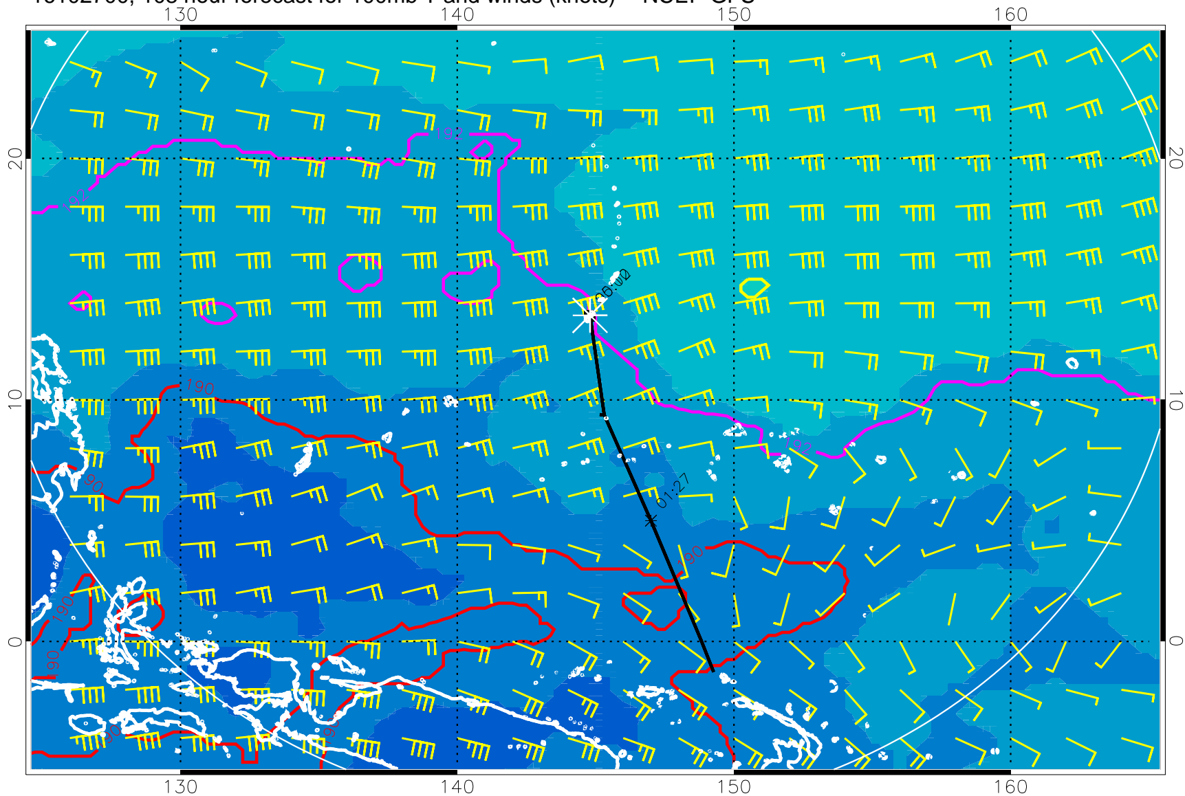
16102700, 108 hour forecast for 100mb T and winds (knots) -- NCEP GFS
