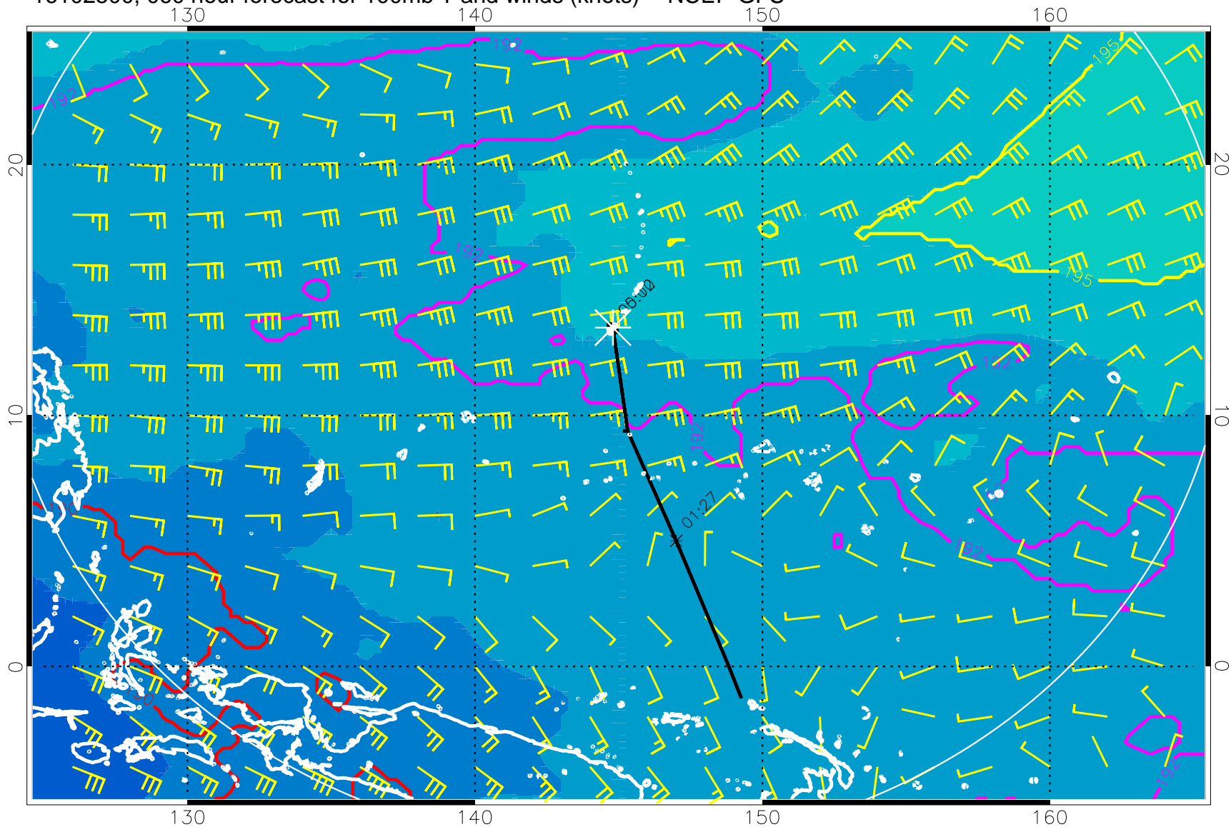
16102500, 060 hour forecast for 100mb T and winds (knots) -- NCEP GFS
