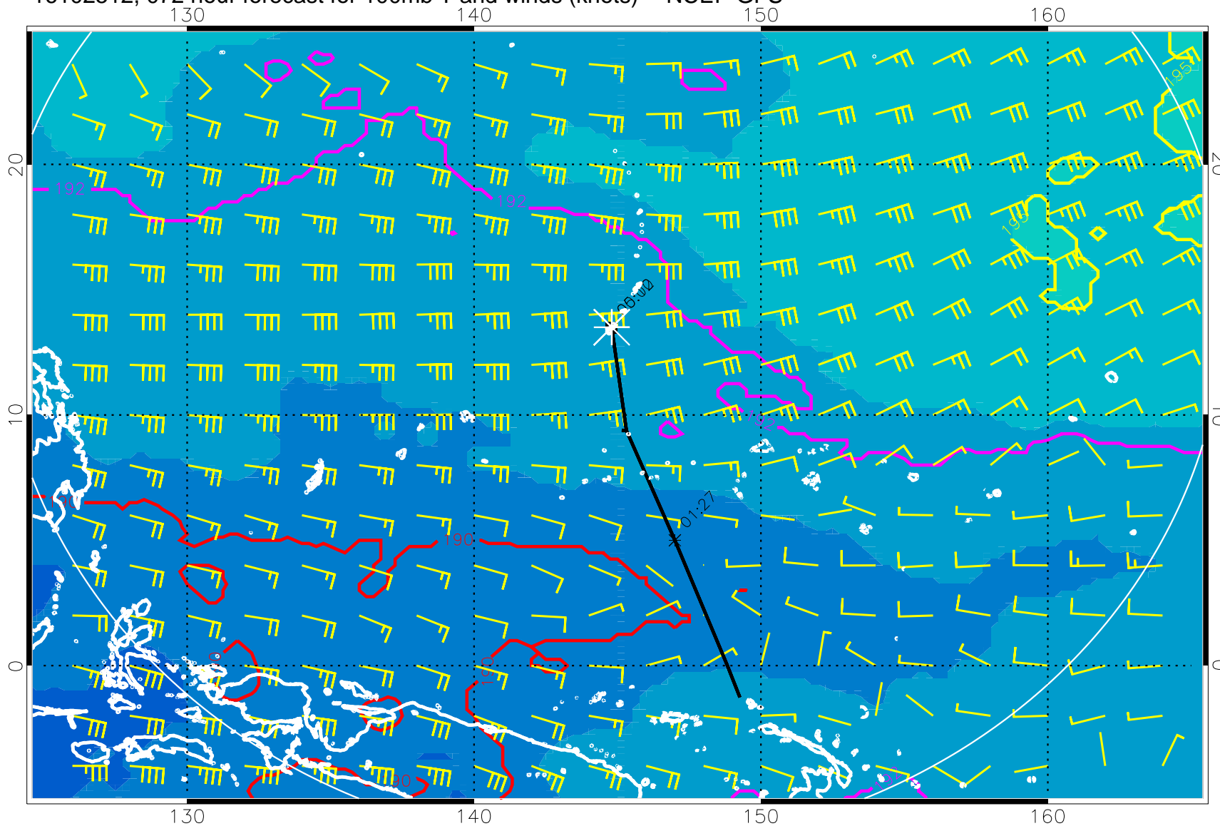
16102512, 072 hour forecast for 100mb T and winds (knots) -- NCEP GFS
