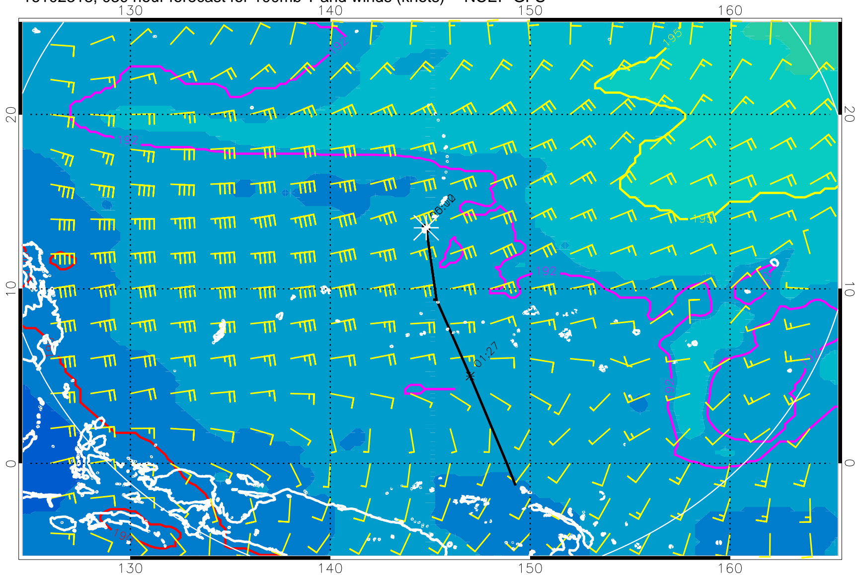
16102318, 030 hour forecast for 100mb T and winds (knots) -- NCEP GFS
