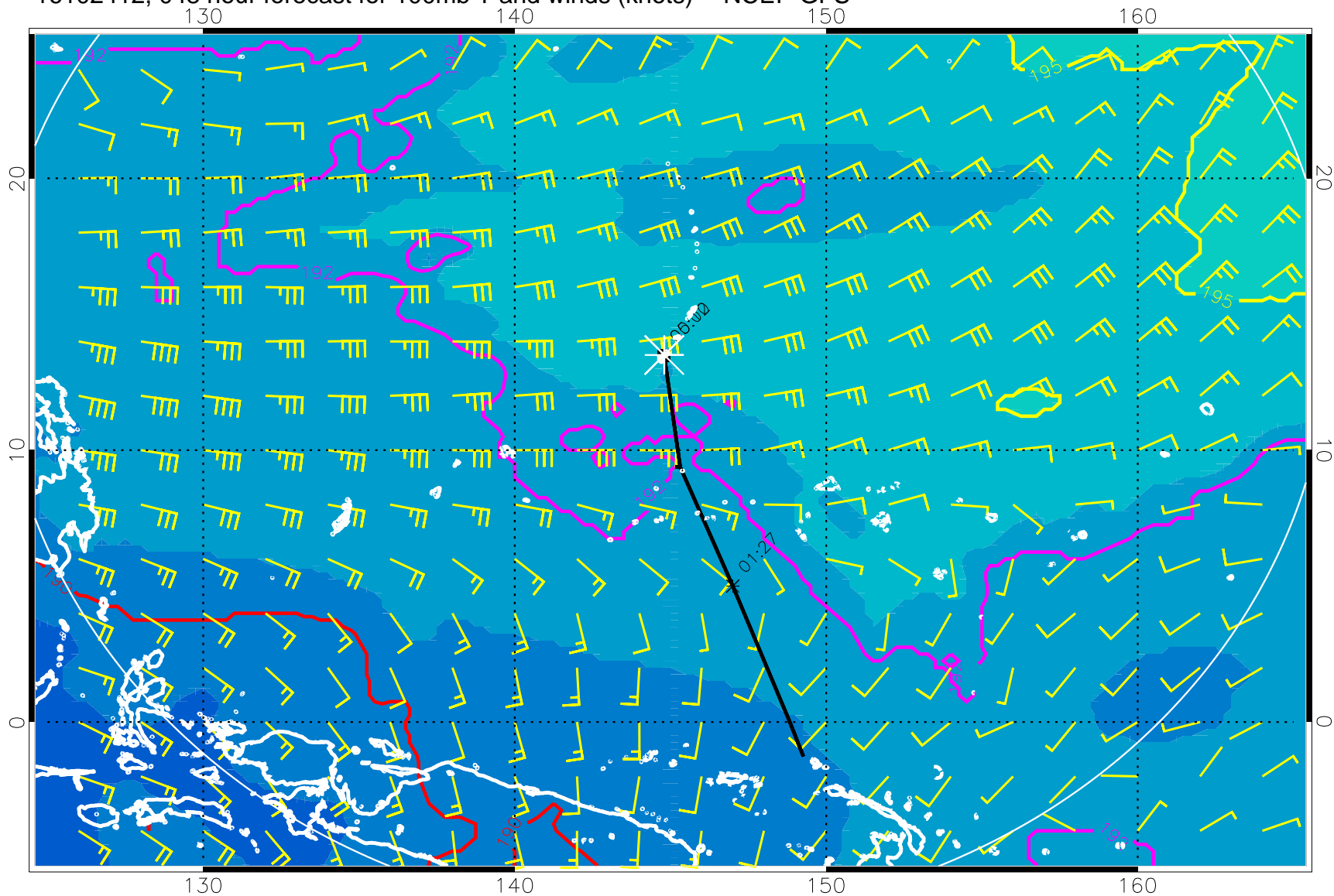
16102412, 048 hour forecast for 100mb T and winds (knots) -- NCEP GFS
