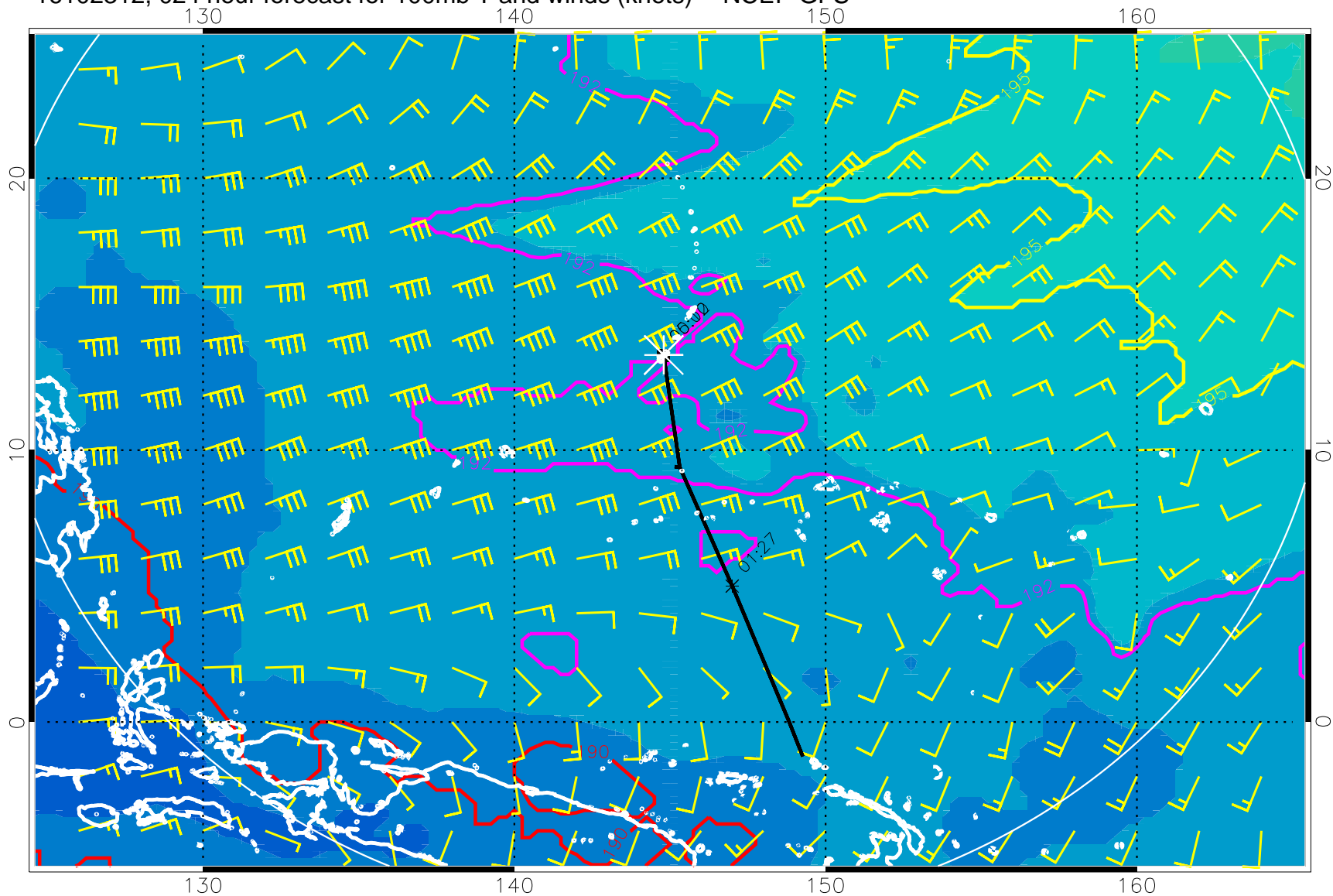
16102312, 024 hour forecast for 100mb T and winds (knots) -- NCEP GFS
