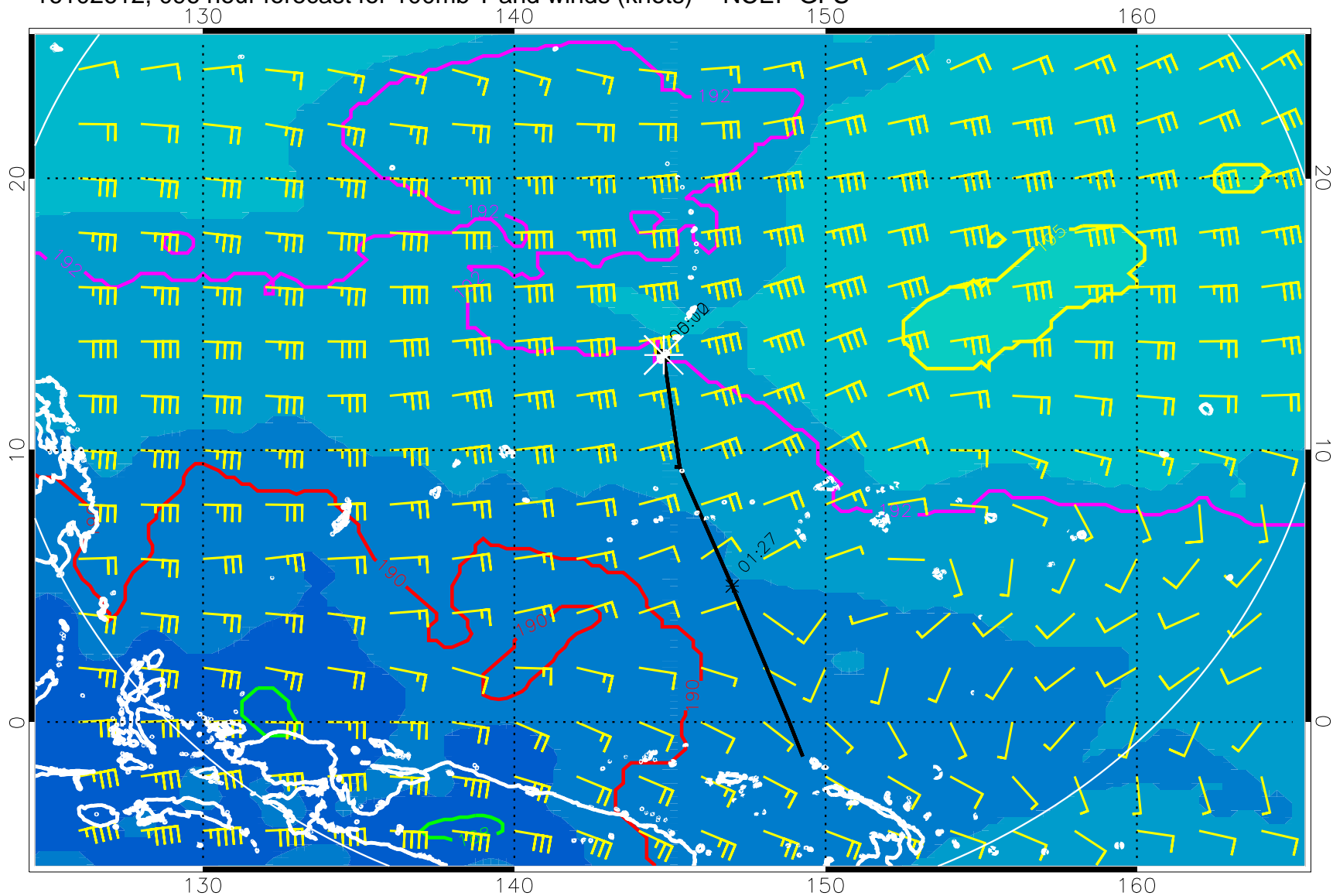
16102612, 096 hour forecast for 100mb T and winds (knots) -- NCEP GFS
