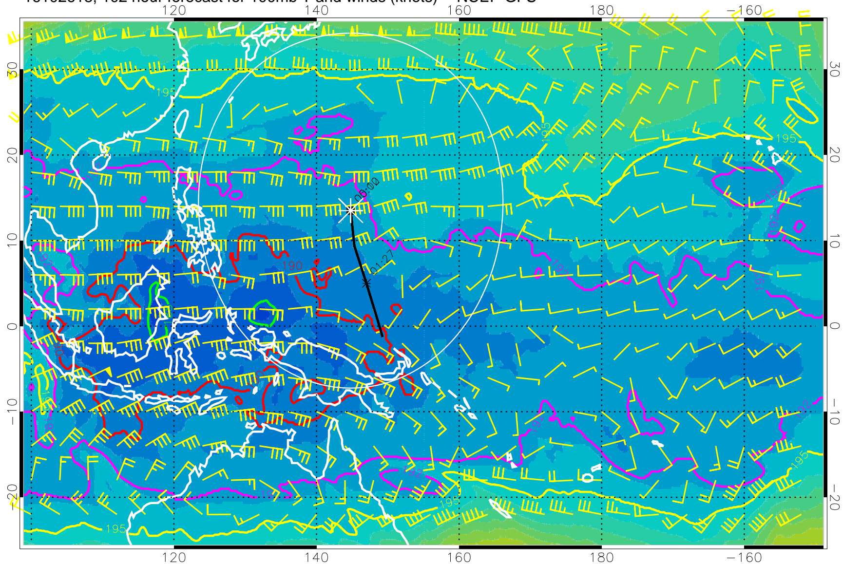
16102618, 102 hour forecast for 100mb T and winds (knots) -- NCEP GFS
