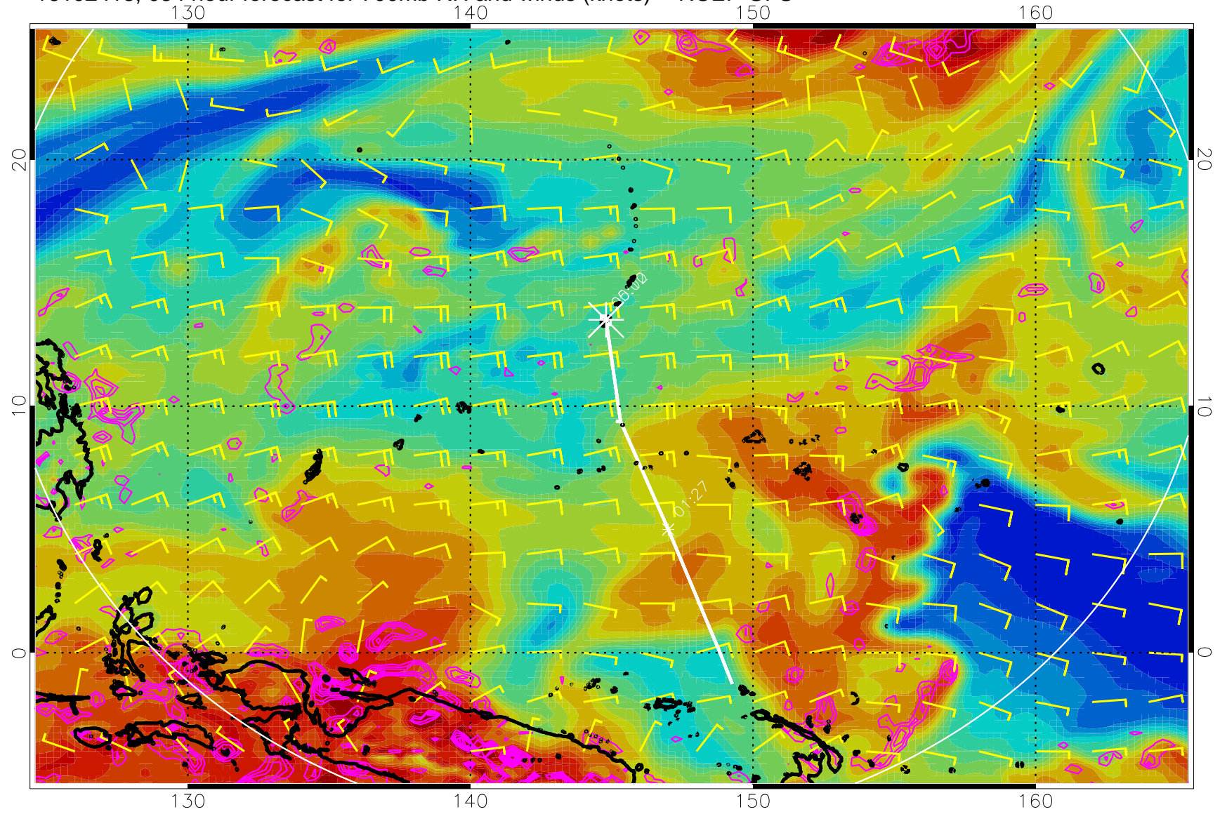
16102418, 054 hour forecast for 700mb RH and winds (knots) -- NCEP GFS
