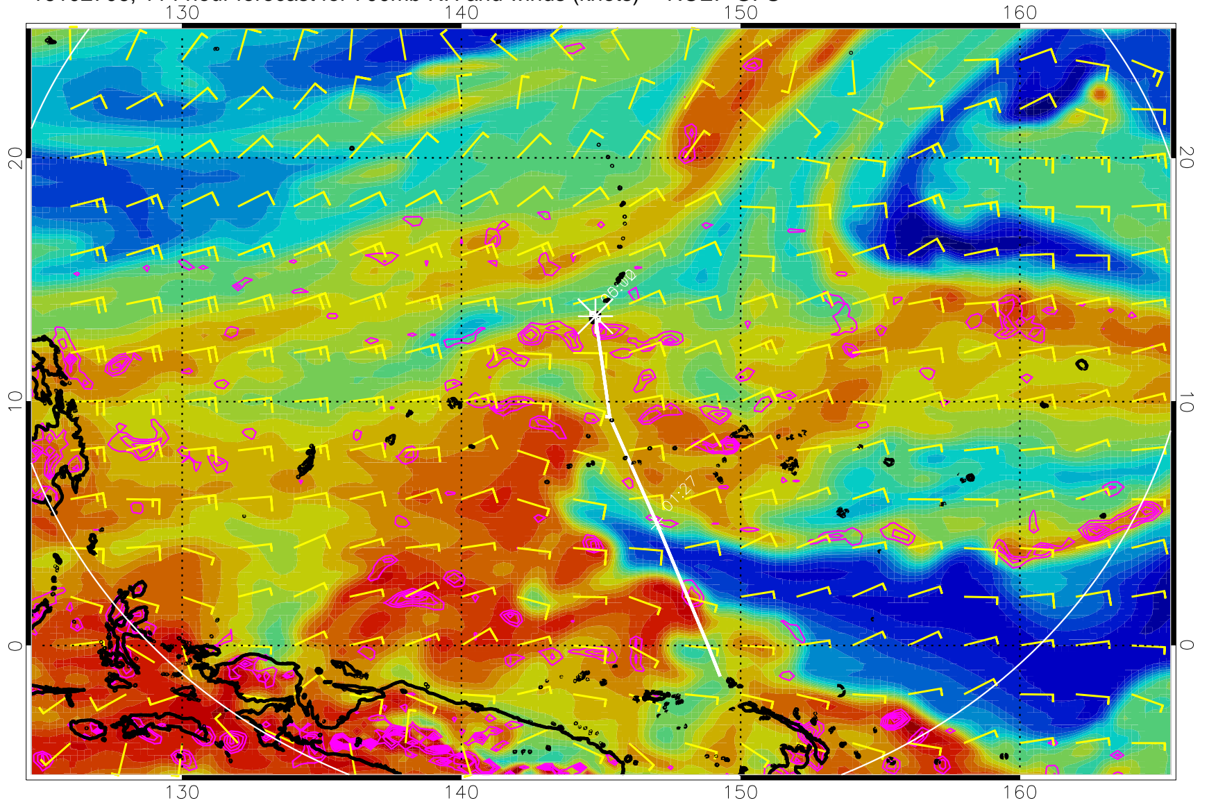
16102706, 114 hour forecast for 700mb RH and winds (knots) -- NCEP GFS
