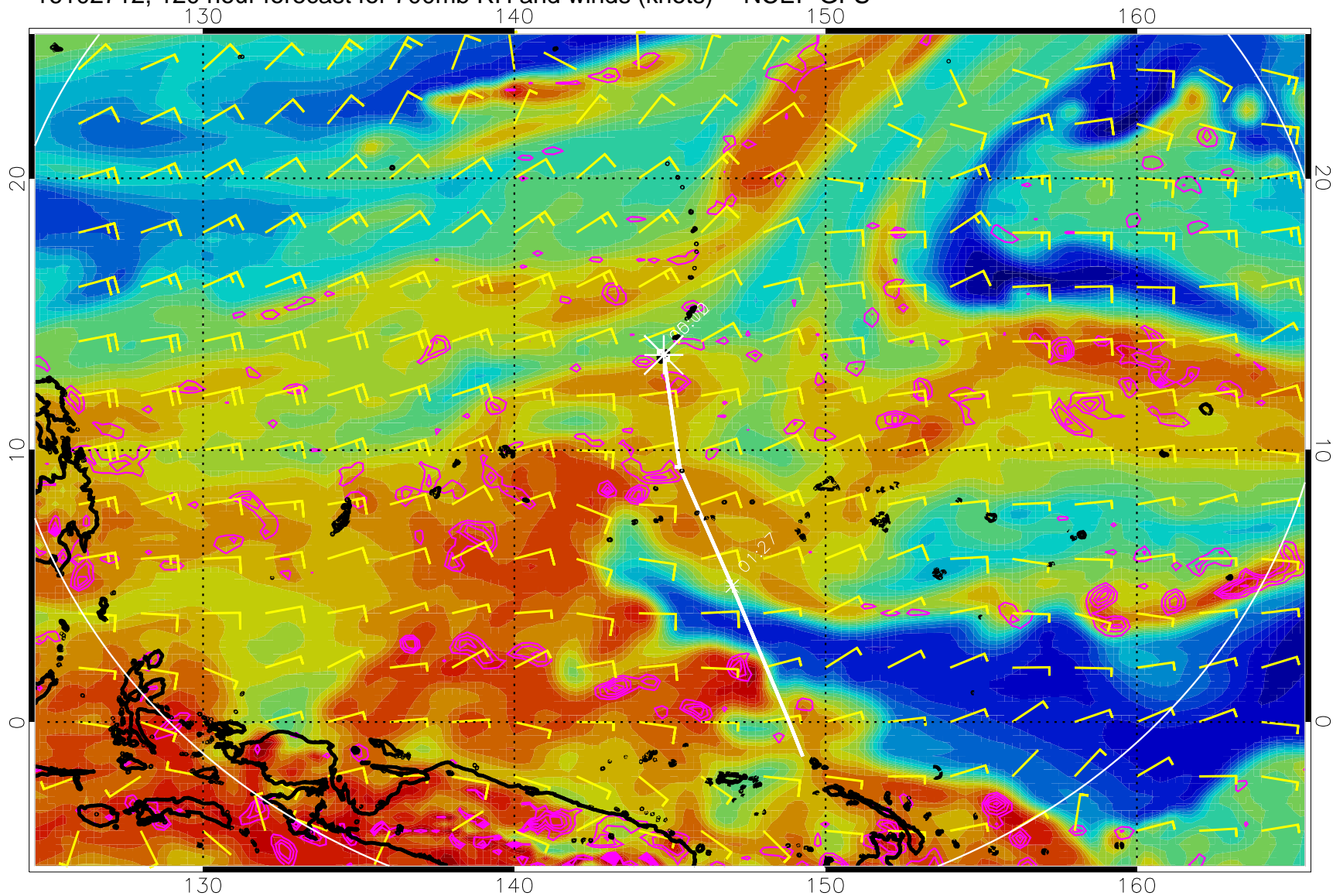
16102712, 120 hour forecast for 700mb RH and winds (knots) -- NCEP GFS
