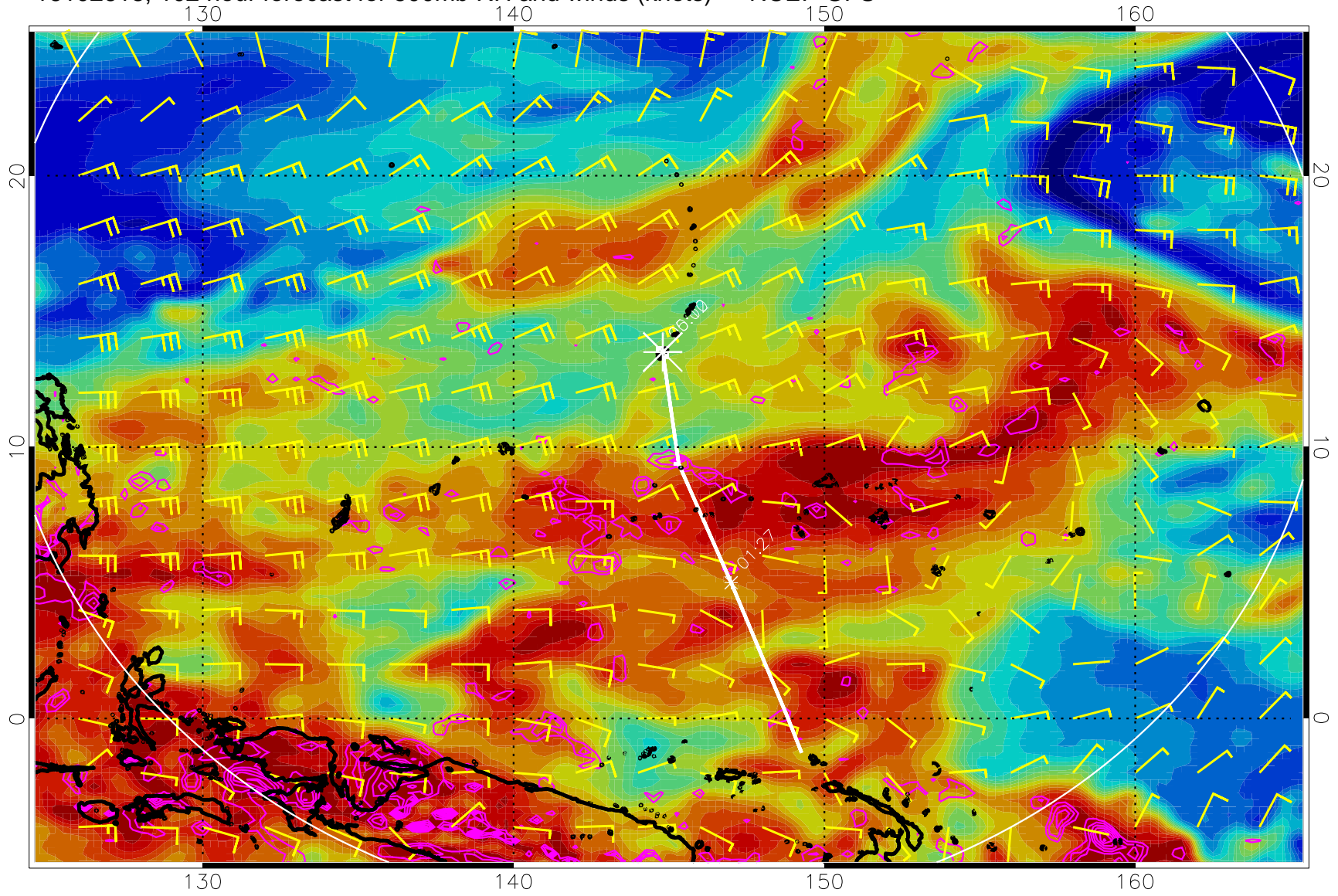
16102618, 102 hour forecast for 500mb RH and winds (knots) -- NCEP GFS
