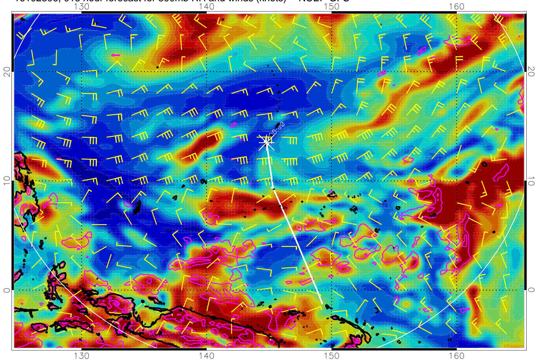
16102306, 018 hour forecast for 300mb RH and winds (knots) -- NCEP GFS
