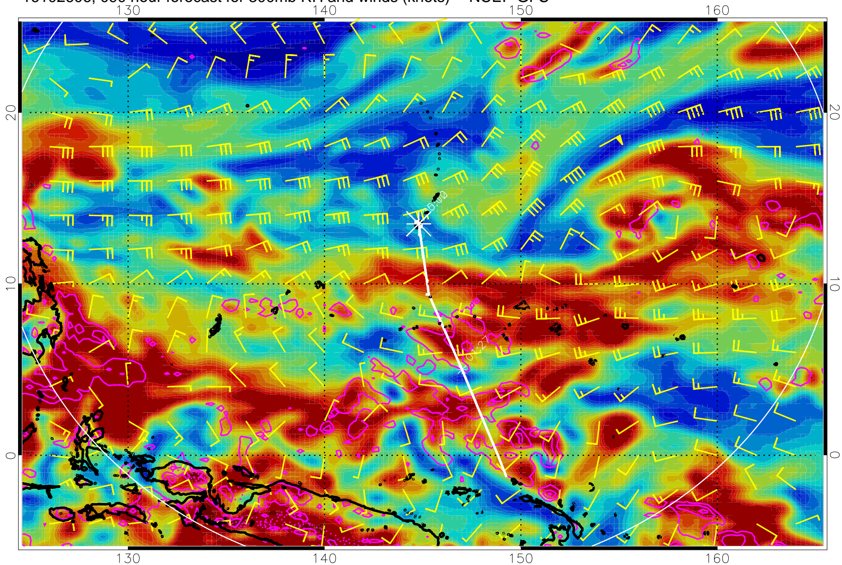
16102606, 090 hour forecast for 300mb RH and winds (knots) -- NCEP GFS
