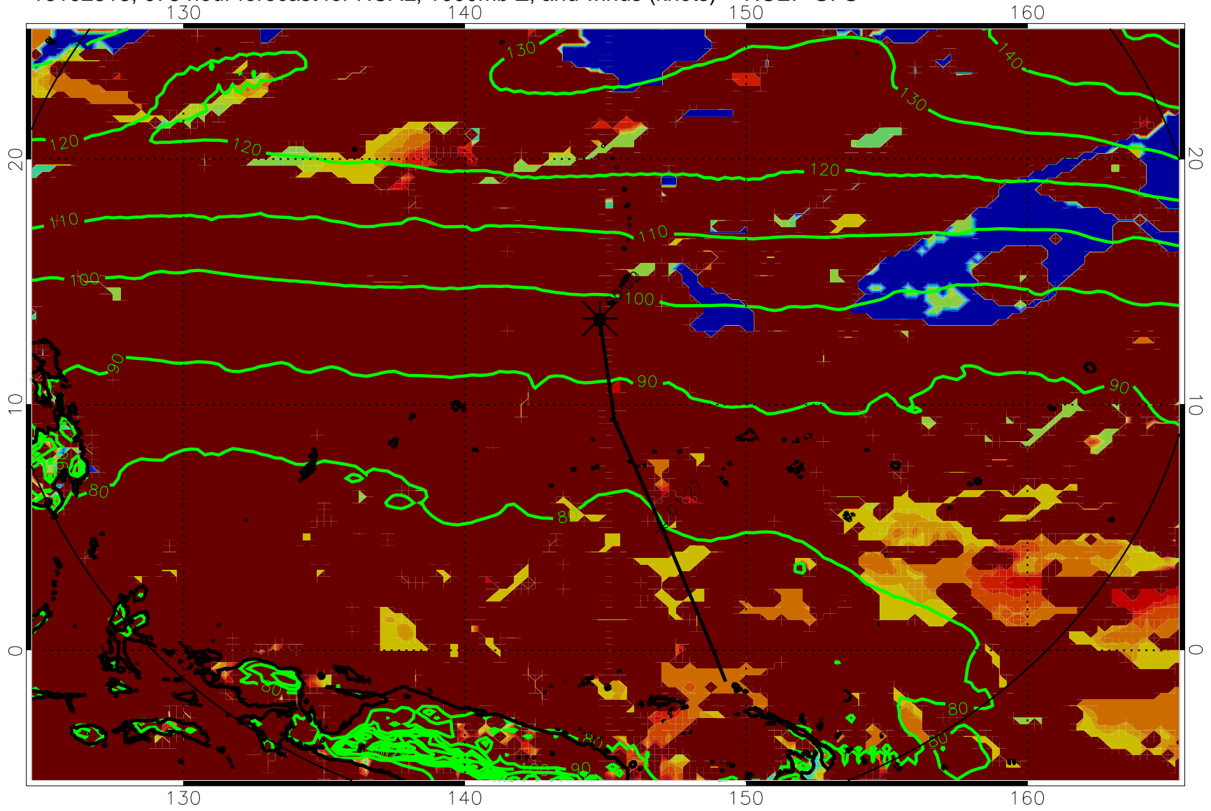
16102518, 078 hour forecast for HCAL, 1000mb Z, and winds (knots) -- NCEP GFS
