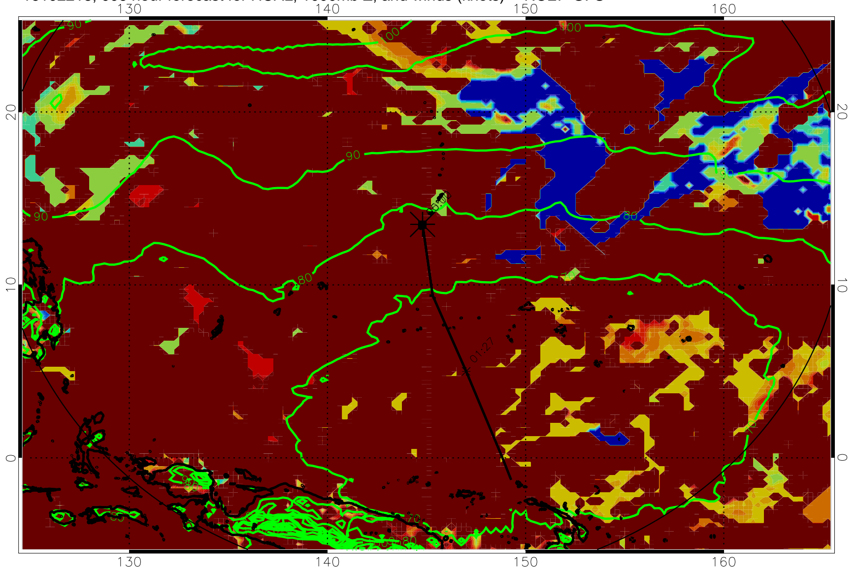
16102218, 006 hour forecast for HCAL, 1000mb Z, and winds (knots) -- NCEP GFS
