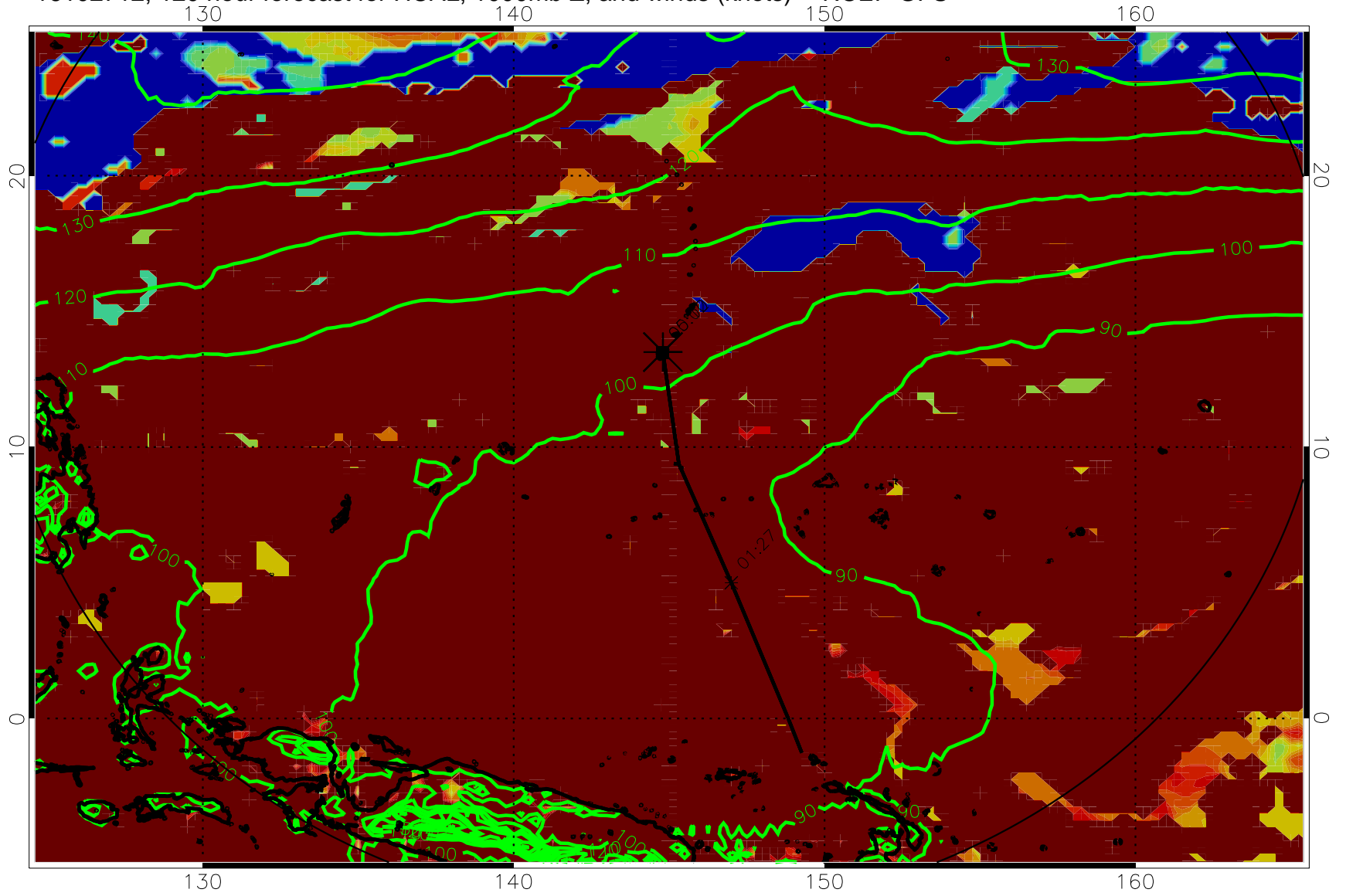
16102712, 120 hour forecast for HCAL, 1000mb Z, and winds (knots) -- NCEP GFS
