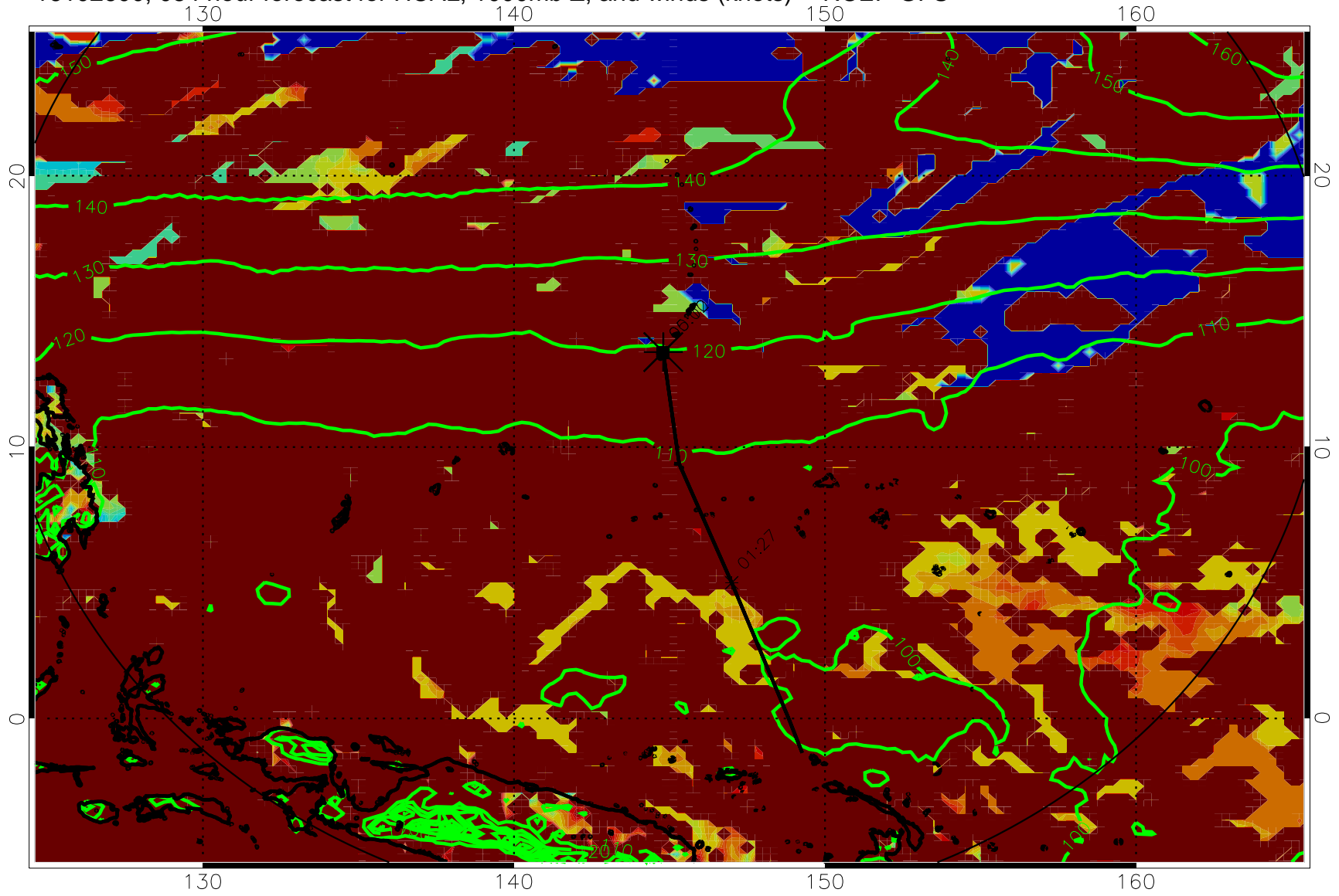
16102600, 084 hour forecast for HCAL, 1000mb Z, and winds (knots) -- NCEP GFS
