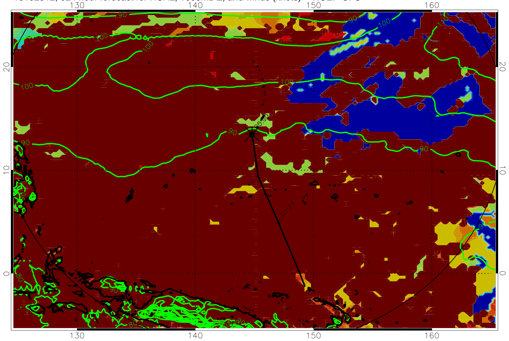
16102312, 024 hour forecast for HCAL, 1000mb Z, and winds (knots) -- NCEP GFS
