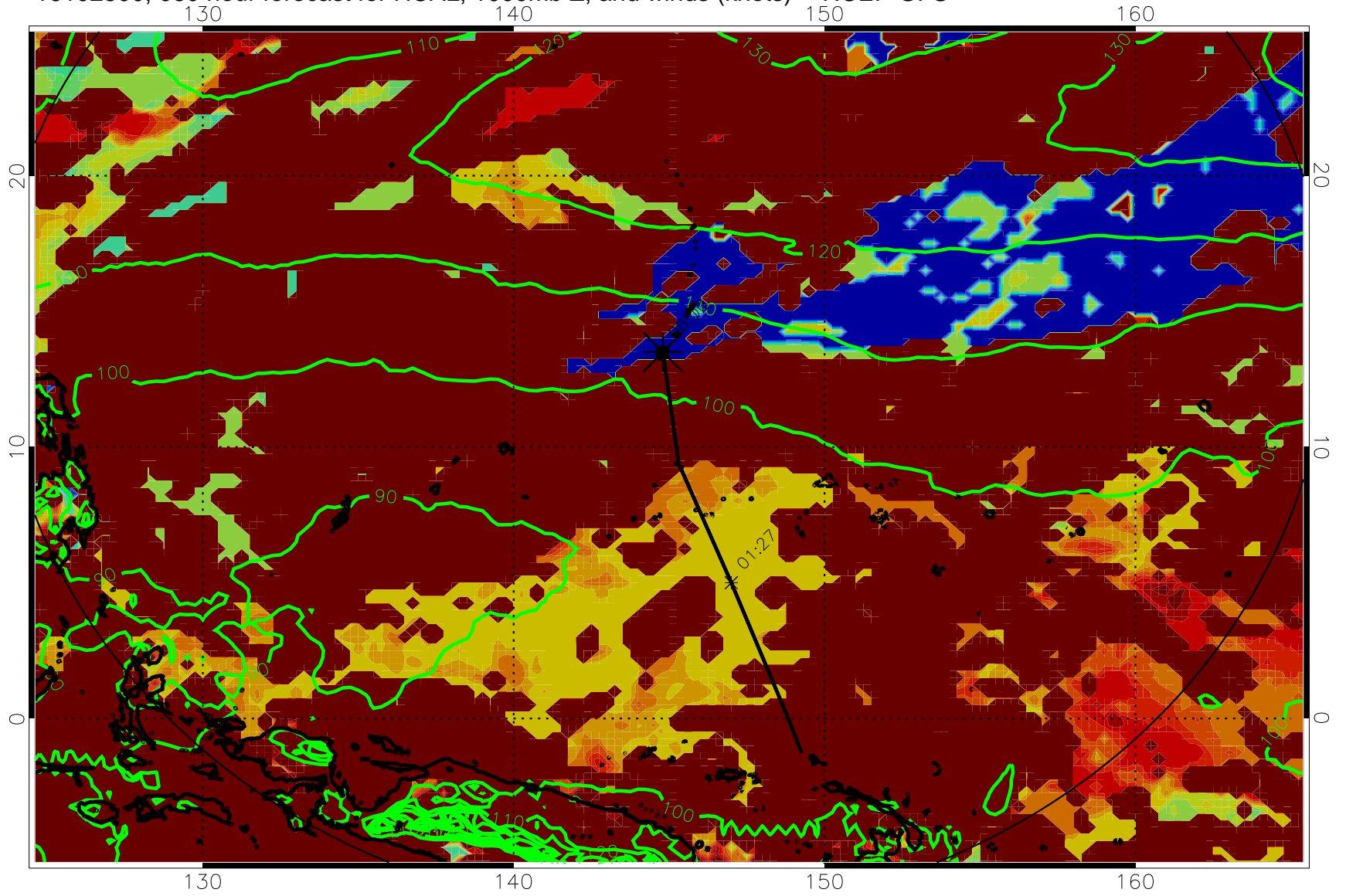
16102500, 060 hour forecast for HCAL, 1000mb Z, and winds (knots) -- NCEP GFS
