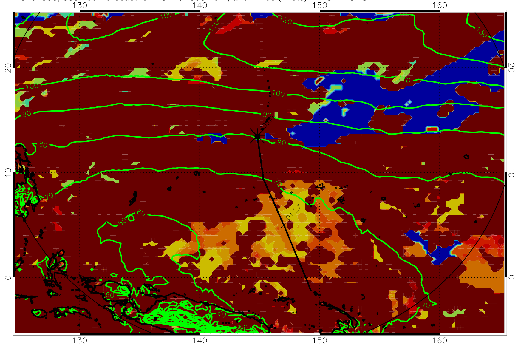
16102506, 066 hour forecast for HCAL, 1000mb Z, and winds (knots) -- NCEP GFS
