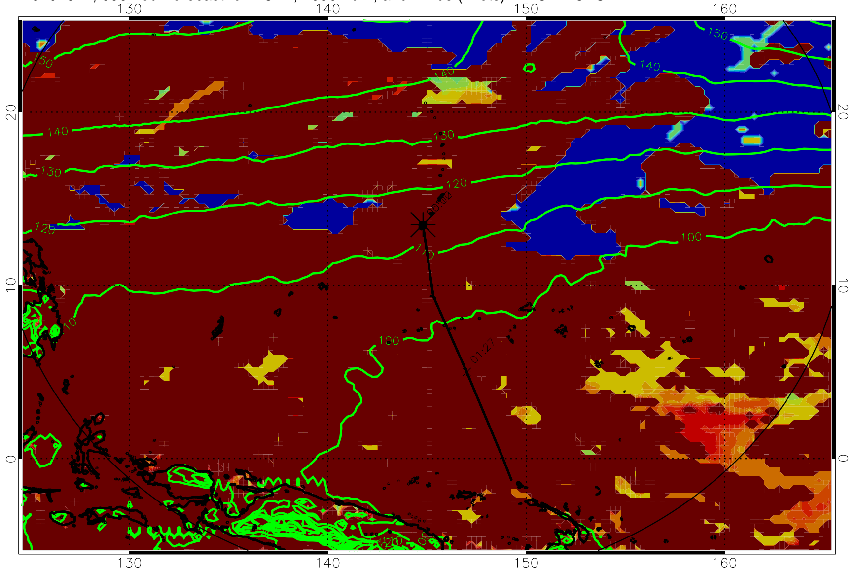
16102612, 096 hour forecast for HCAL, 1000mb Z, and winds (knots) -- NCEP GFS
