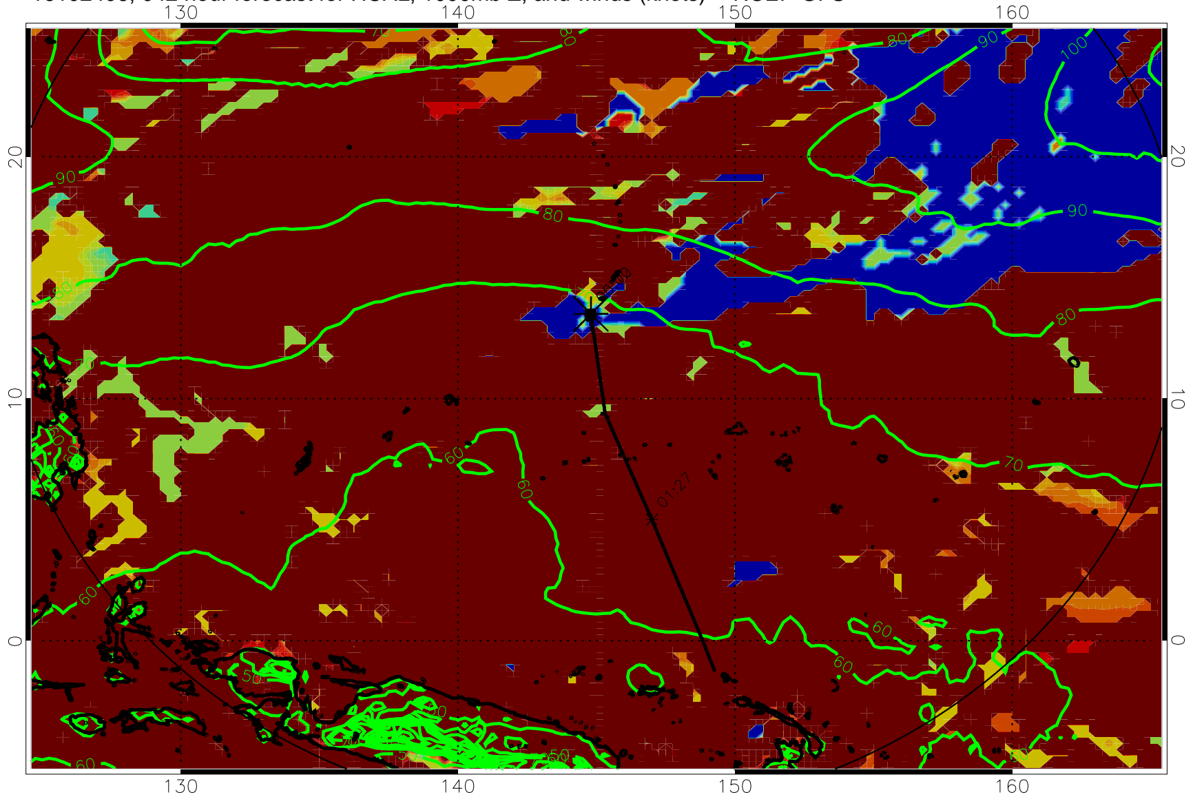
16102406, 042 hour forecast for HCAL, 1000mb Z, and winds (knots) -- NCEP GFS
