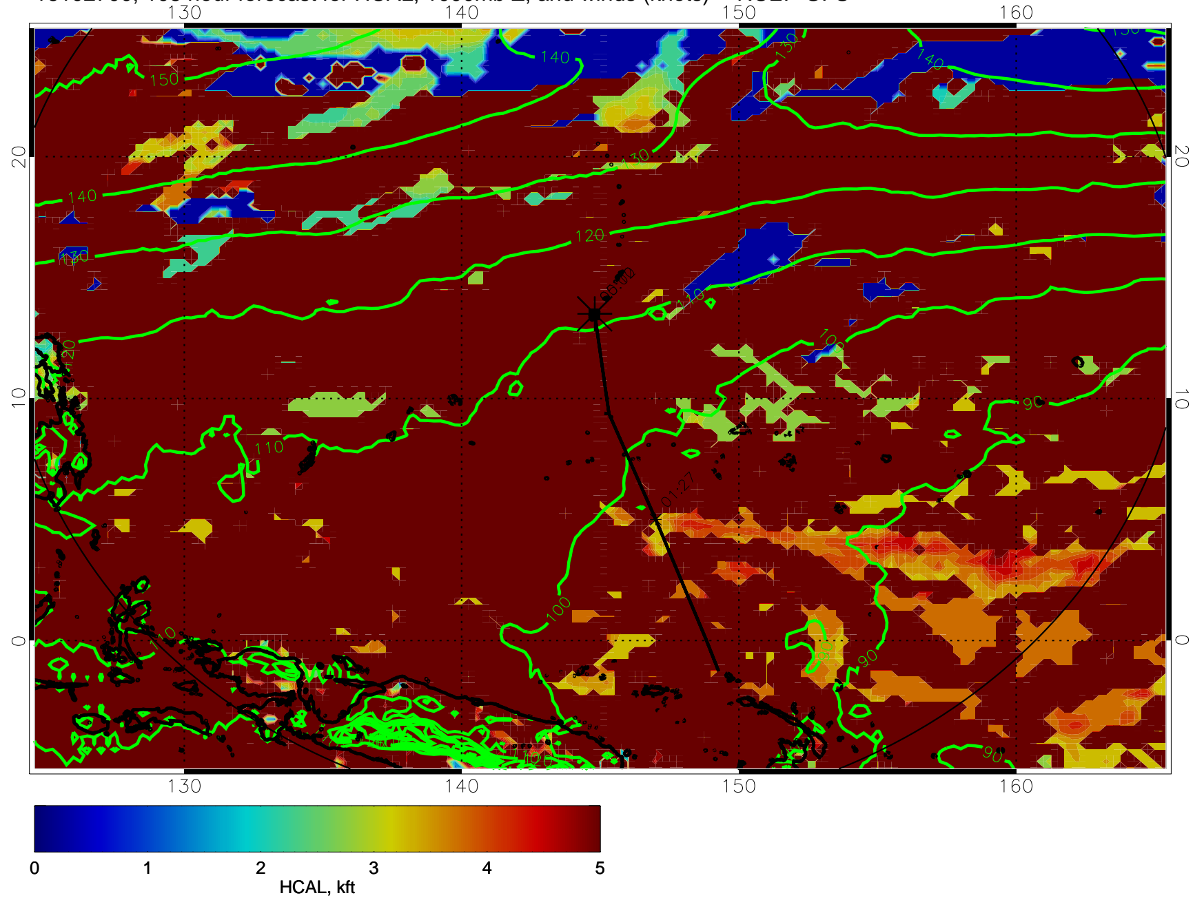
16102700, 108 hour forecast for HCAL, 1000mb Z, and winds (knots) -- NCEP GFS
