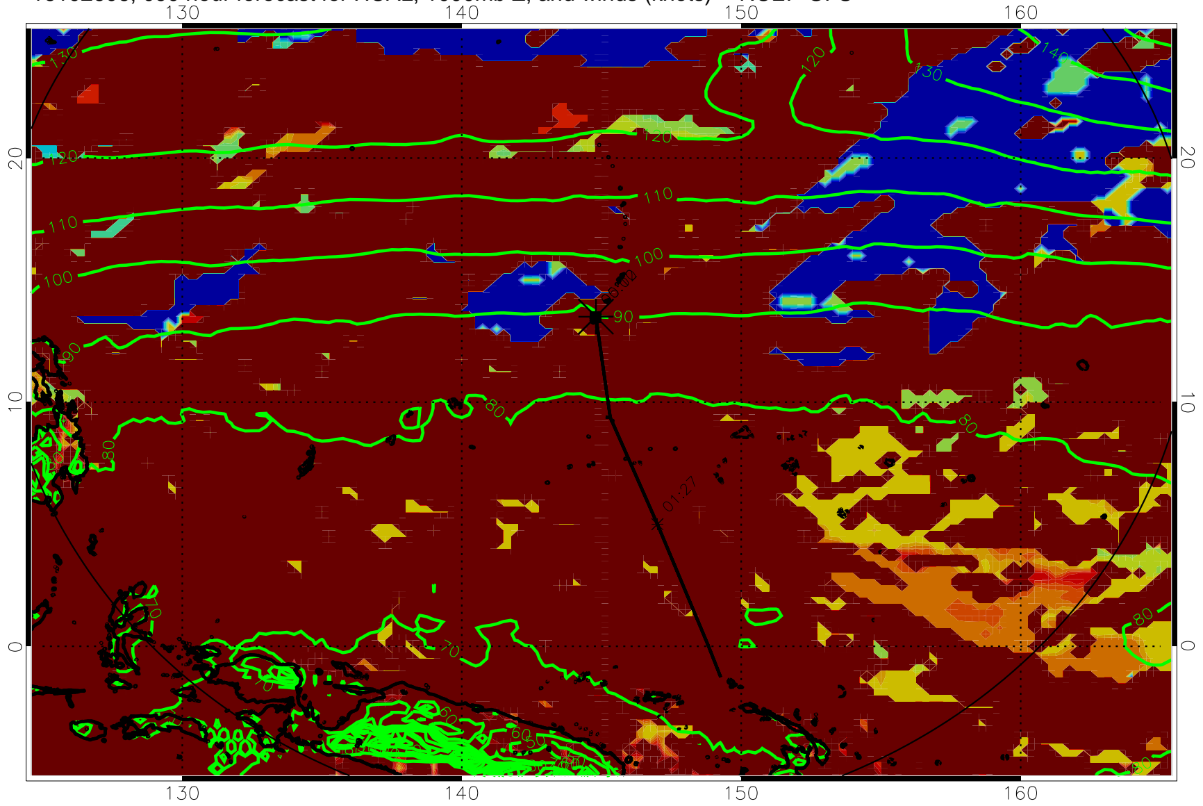
16102606, 090 hour forecast for HCAL, 1000mb Z, and winds (knots) -- NCEP GFS
