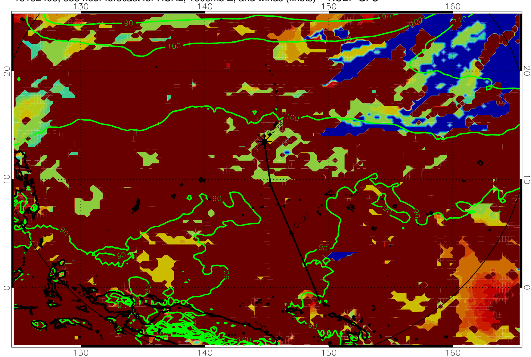
16102400, 036 hour forecast for HCAL, 1000mb Z, and winds (knots) -- NCEP GFS
