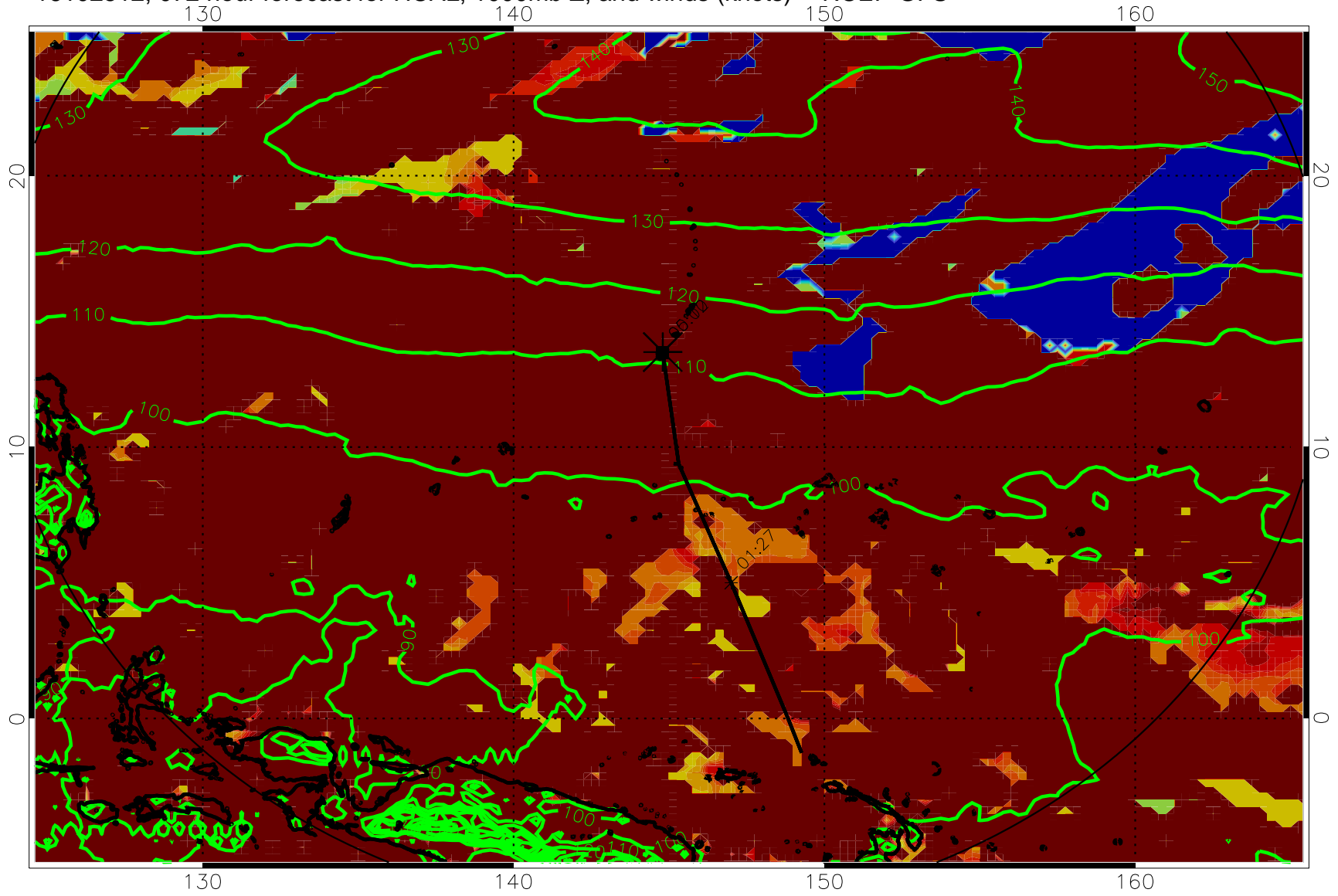
16102512, 072 hour forecast for HCAL, 1000mb Z, and winds (knots) -- NCEP GFS
