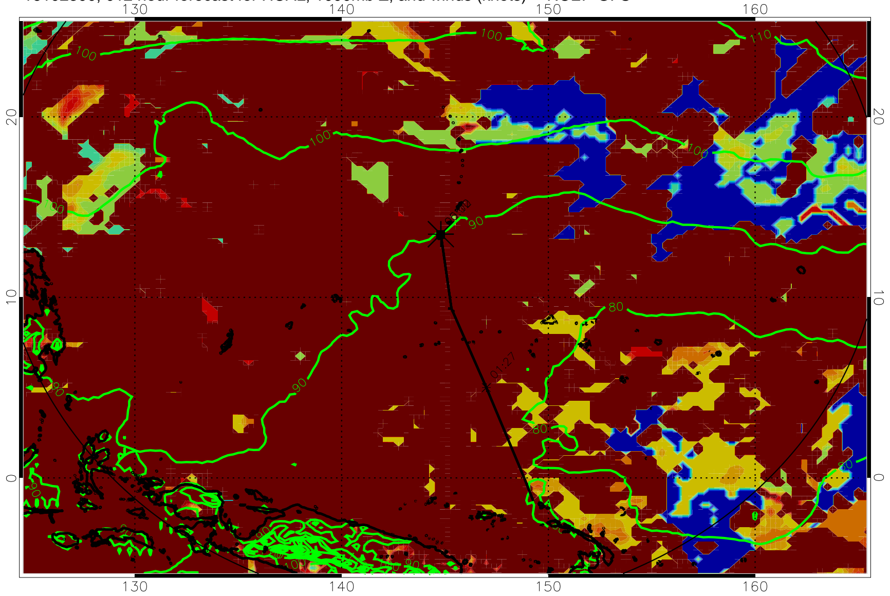
16102300, 012 hour forecast for HCAL, 1000mb Z, and winds (knots) -- NCEP GFS
