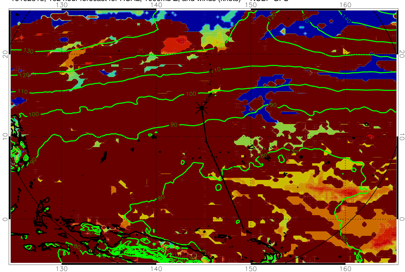
16102618, 102 hour forecast for HCAL, 1000mb Z, and winds (knots) -- NCEP GFS
