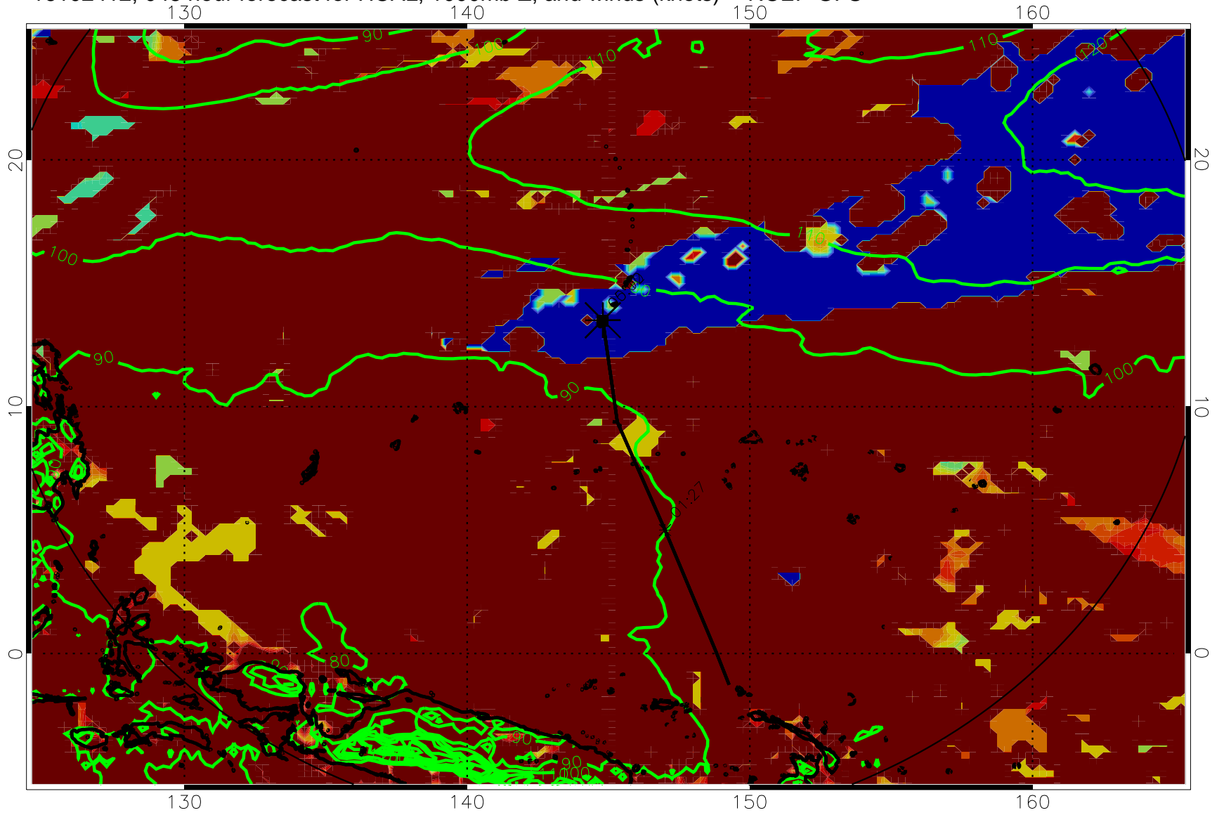
16102412, 048 hour forecast for HCAL, 1000mb Z, and winds (knots) -- NCEP GFS
