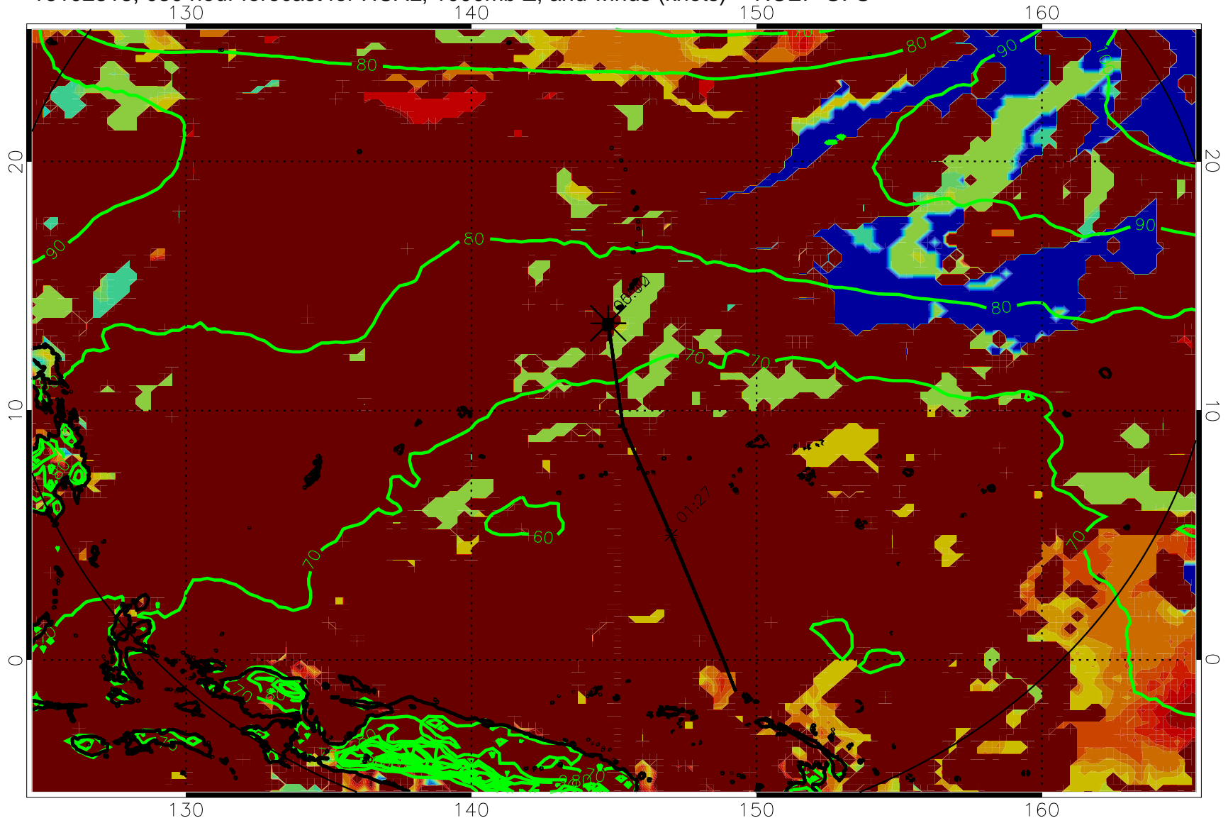
16102318, 030 hour forecast for HCAL, 1000mb Z, and winds (knots) -- NCEP GFS
