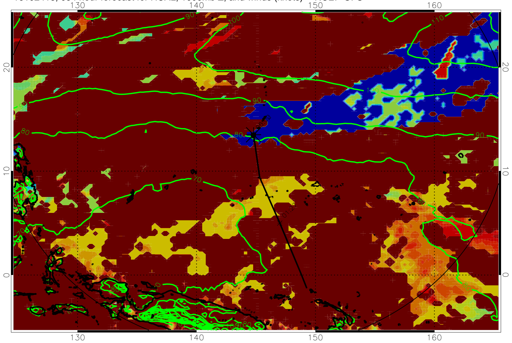
16102418, 054 hour forecast for HCAL, 1000mb Z, and winds (knots) -- NCEP GFS
