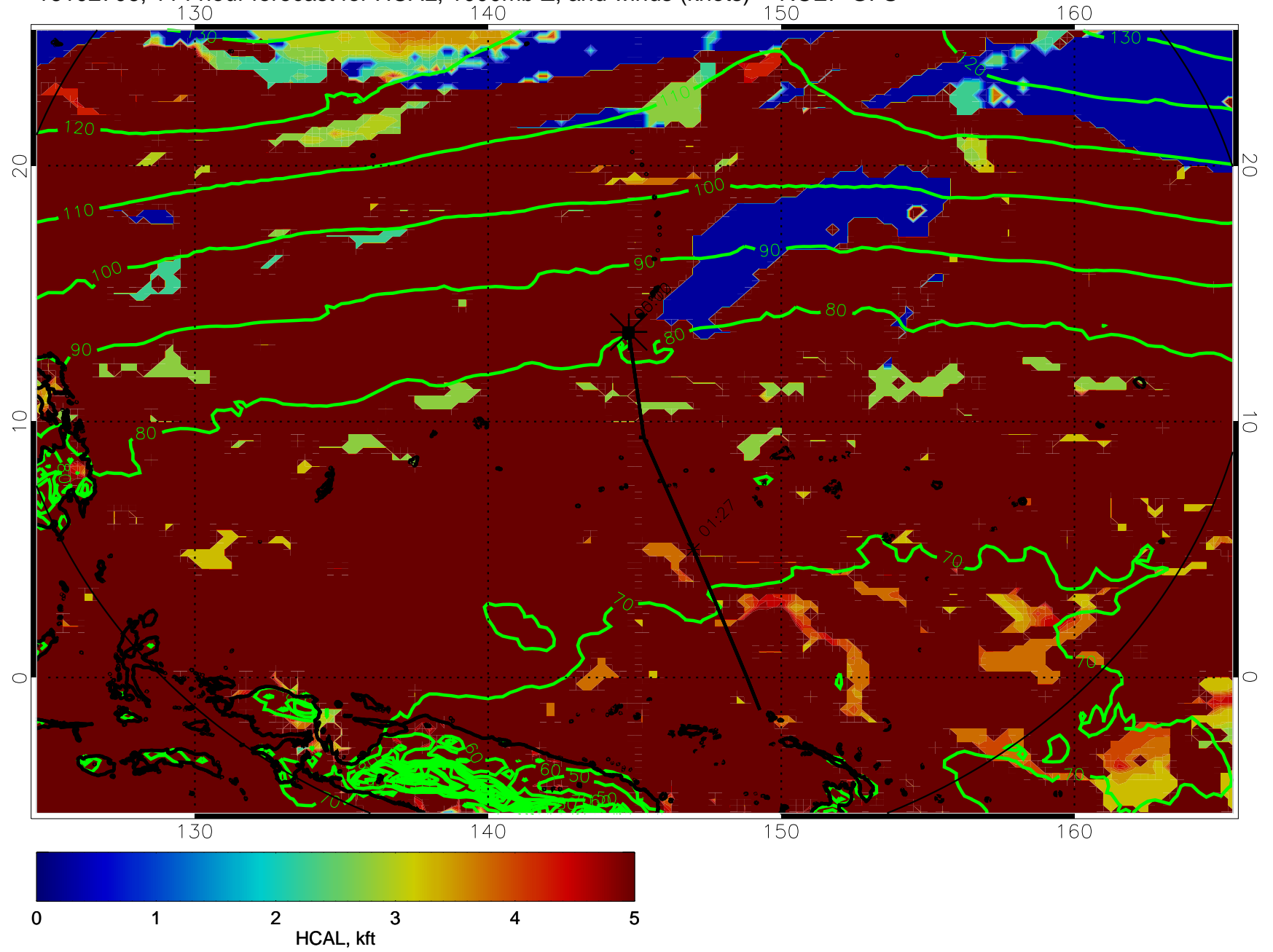
16102706, 114 hour forecast for HCAL, 1000mb Z, and winds (knots) -- NCEP GFS
