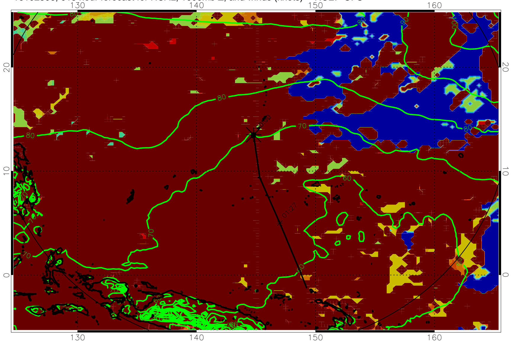
16102306, 018 hour forecast for HCAL, 1000mb Z, and winds (knots) -- NCEP GFS
