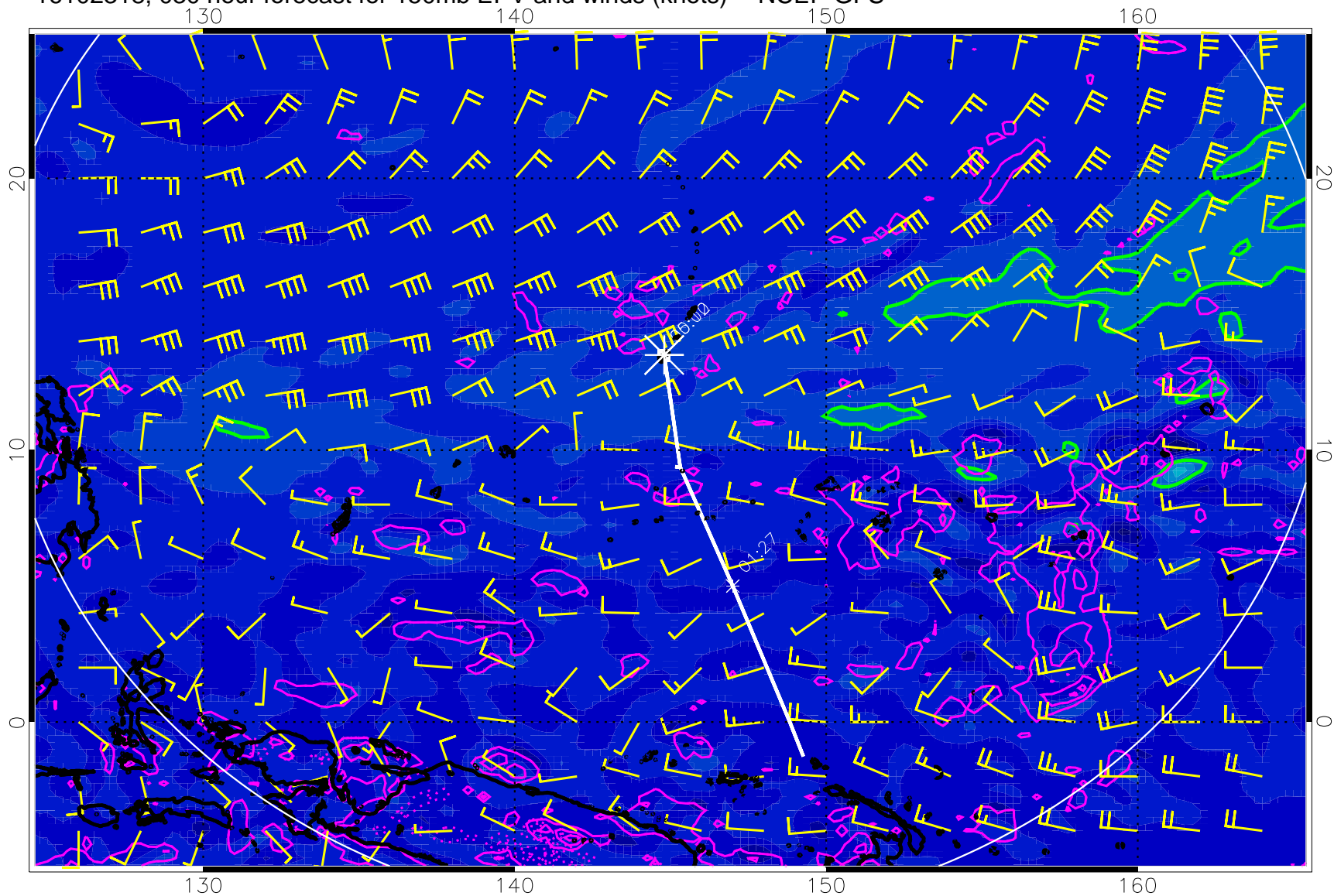
16102318, 030 hour forecast for 150mb EPV and winds (knots) -- NCEP GFS
