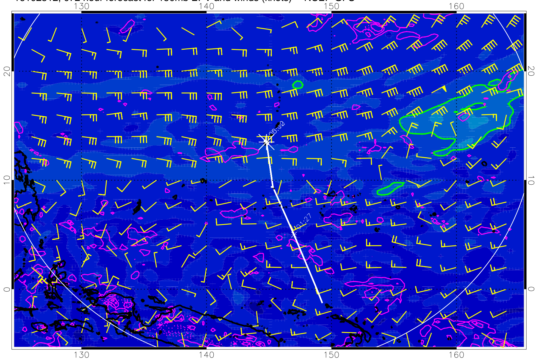
16102512, 072 hour forecast for 150mb EPV and winds (knots) -- NCEP GFS
