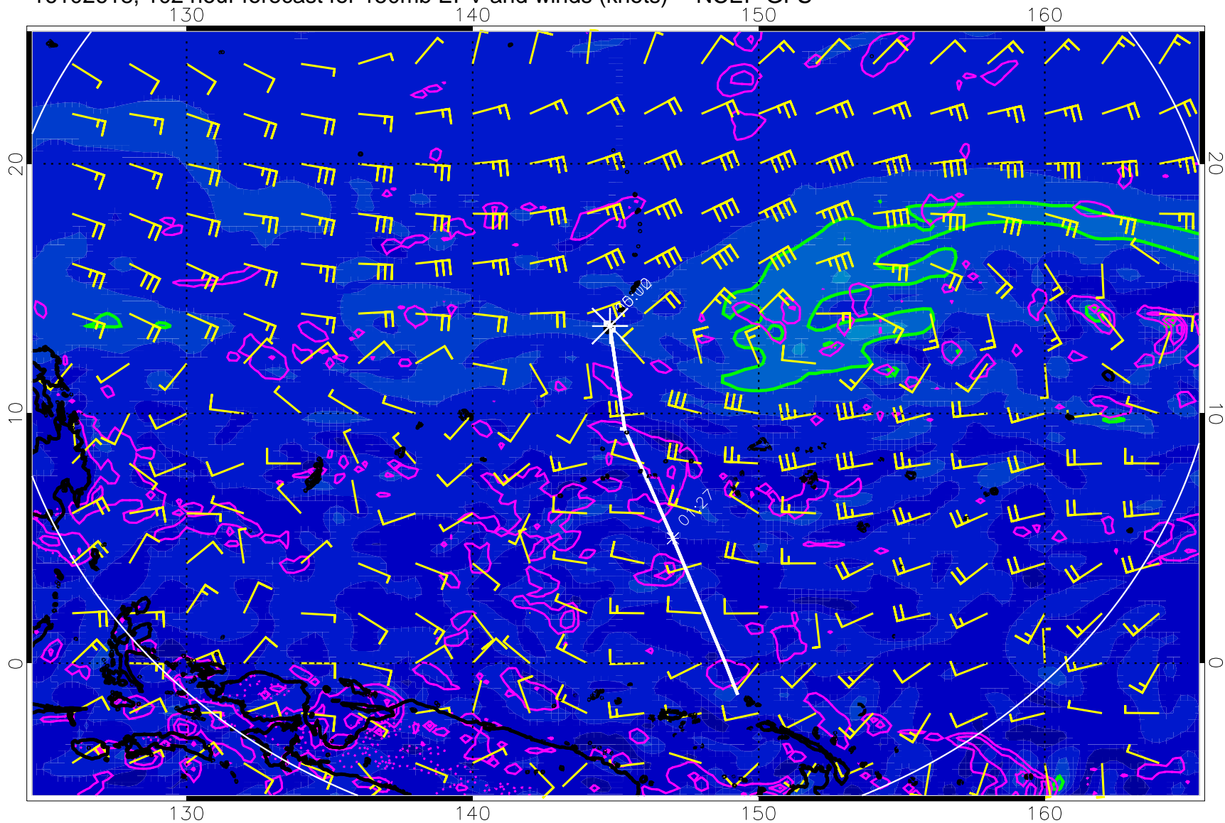
16102618, 102 hour forecast for 150mb EPV and winds (knots) -- NCEP GFS
