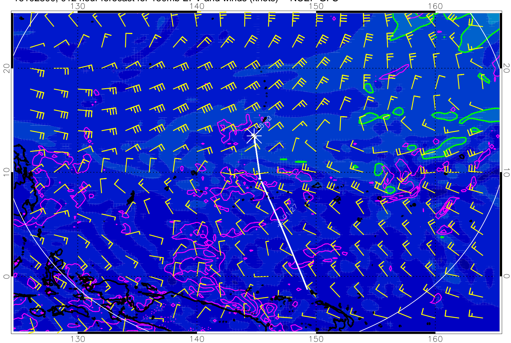
16102300, 012 hour forecast for 150mb EPV and winds (knots) -- NCEP GFS
