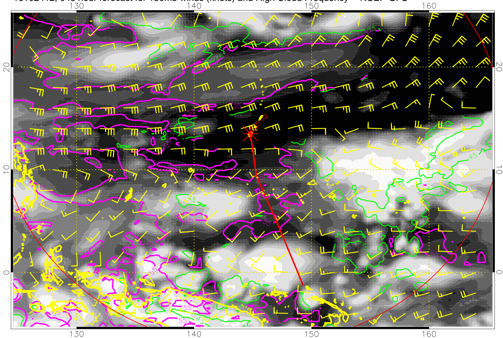
16102412, 048 hour forecast for 150mb winds (knots) and High Cloud Frequency -- NCEP GFS
