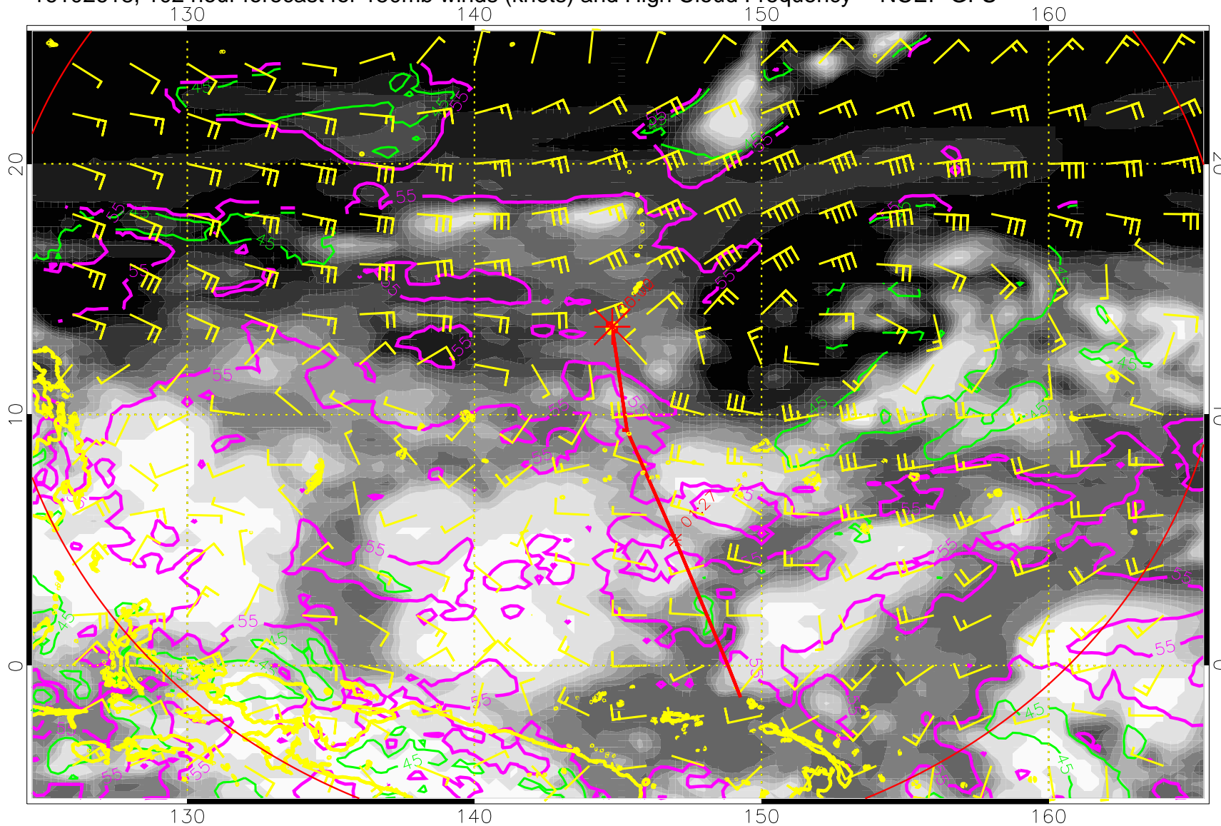
16102618, 102 hour forecast for 150mb winds (knots) and High Cloud Frequency -- NCEP GFS
