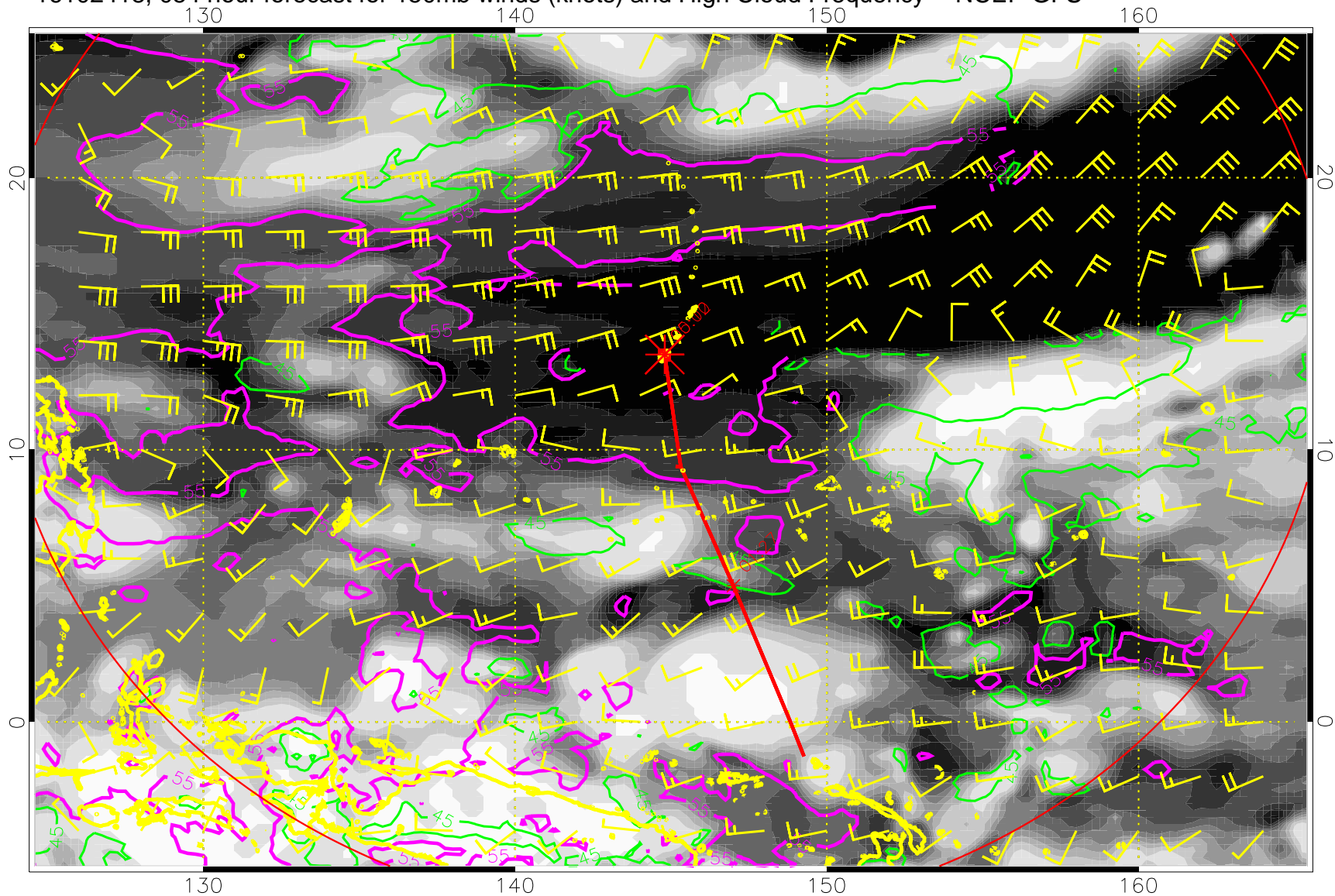
16102418, 054 hour forecast for 150mb winds (knots) and High Cloud Frequency -- NCEP GFS
