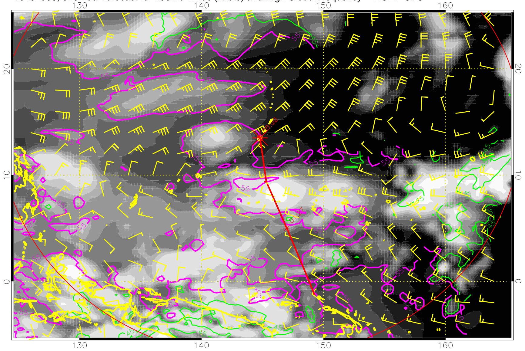
16102306, 018 hour forecast for 150mb winds (knots) and High Cloud Frequency -- NCEP GFS
