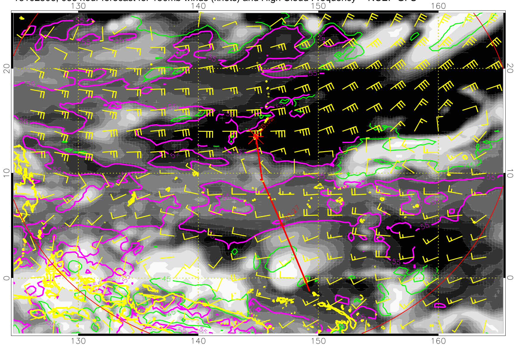
16102506, 066 hour forecast for 150mb winds (knots) and High Cloud Frequency -- NCEP GFS
