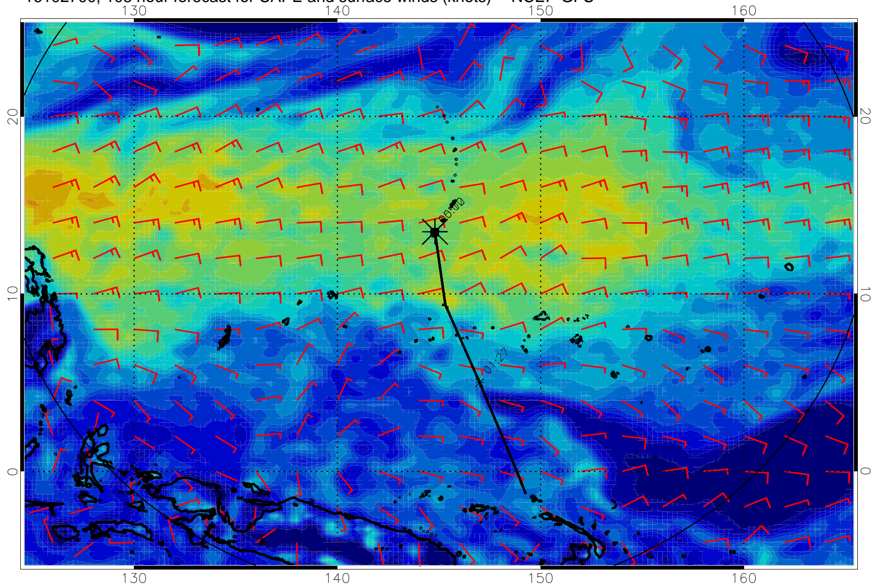
16102700, 108 hour forecast for CAPE and surface winds (knots) -- NCEP GFS
