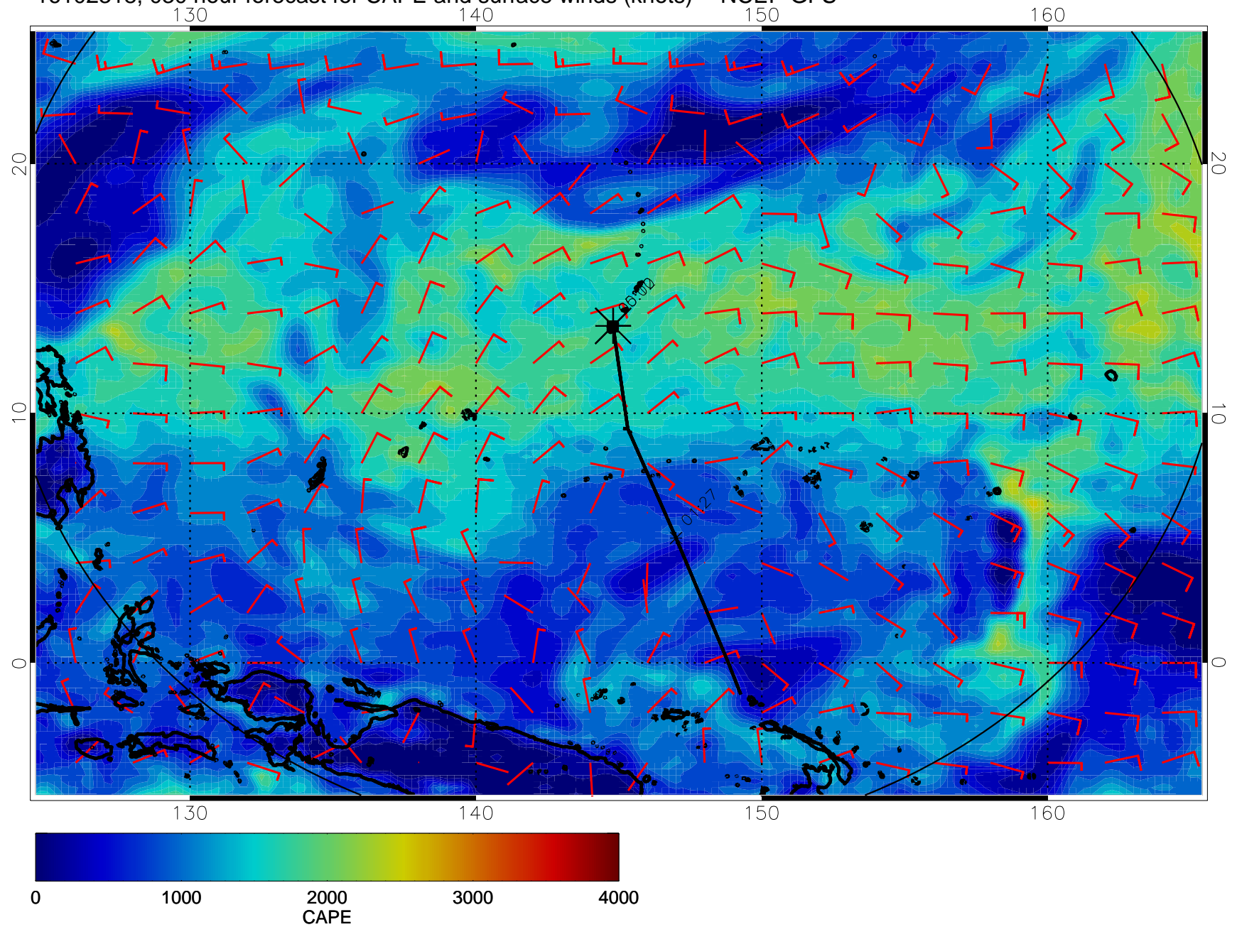
16102318, 030 hour forecast for CAPE and surface winds (knots) -- NCEP GFS
