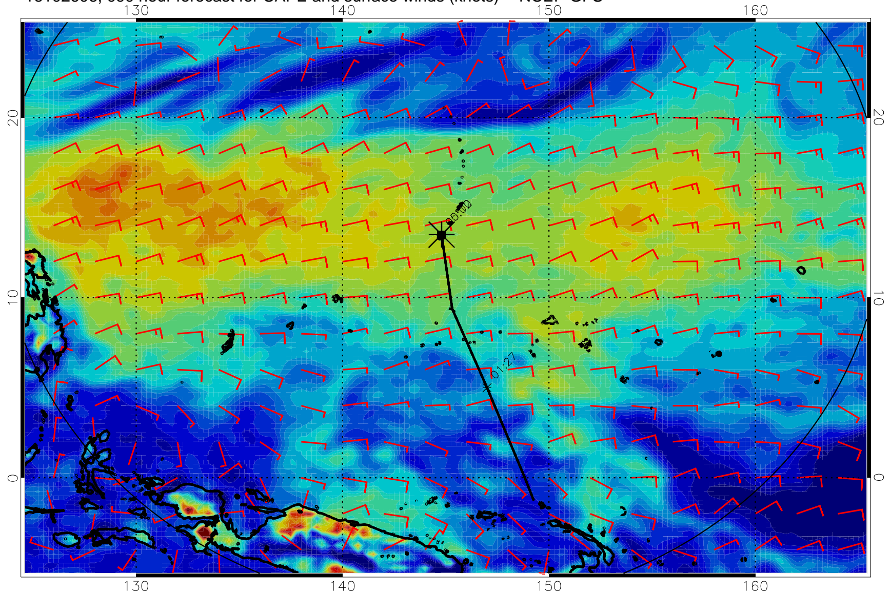
16102606, 090 hour forecast for CAPE and surface winds (knots) -- NCEP GFS
