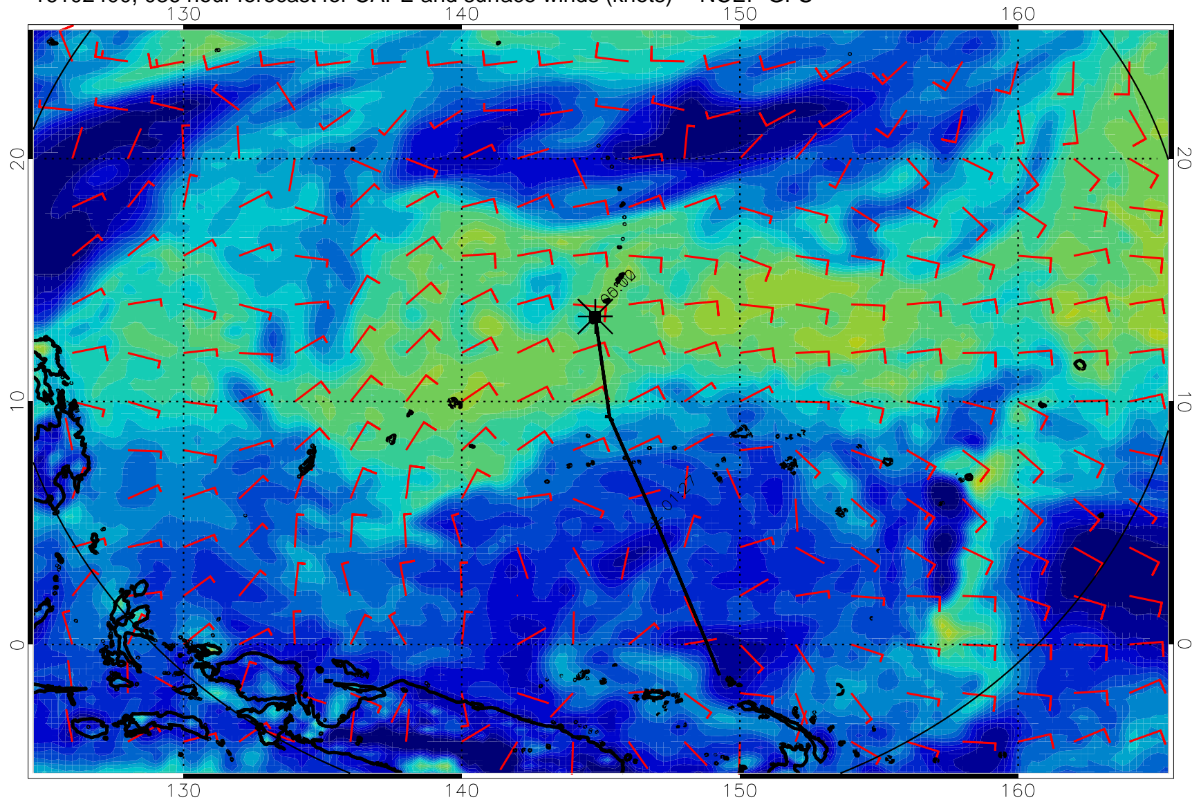
16102400, 036 hour forecast for CAPE and surface winds (knots) -- NCEP GFS
