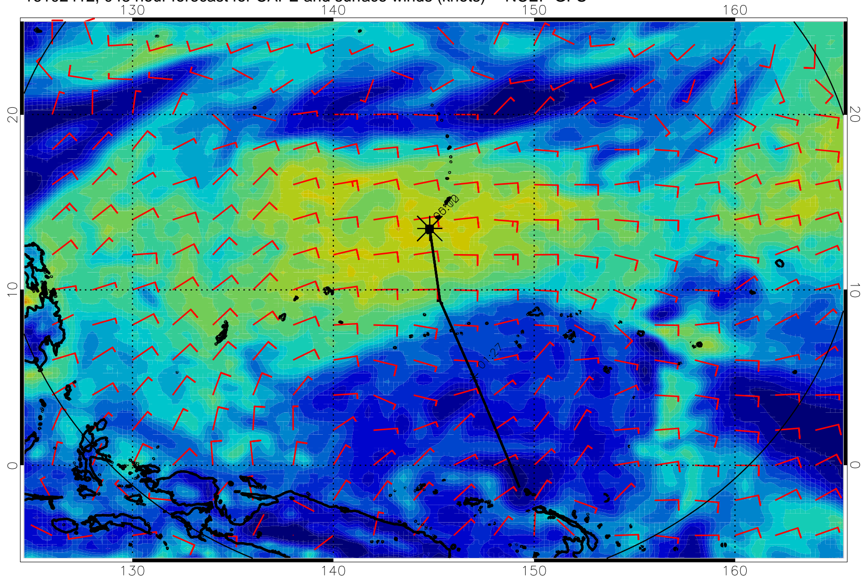
16102412, 048 hour forecast for CAPE and surface winds (knots) -- NCEP GFS
