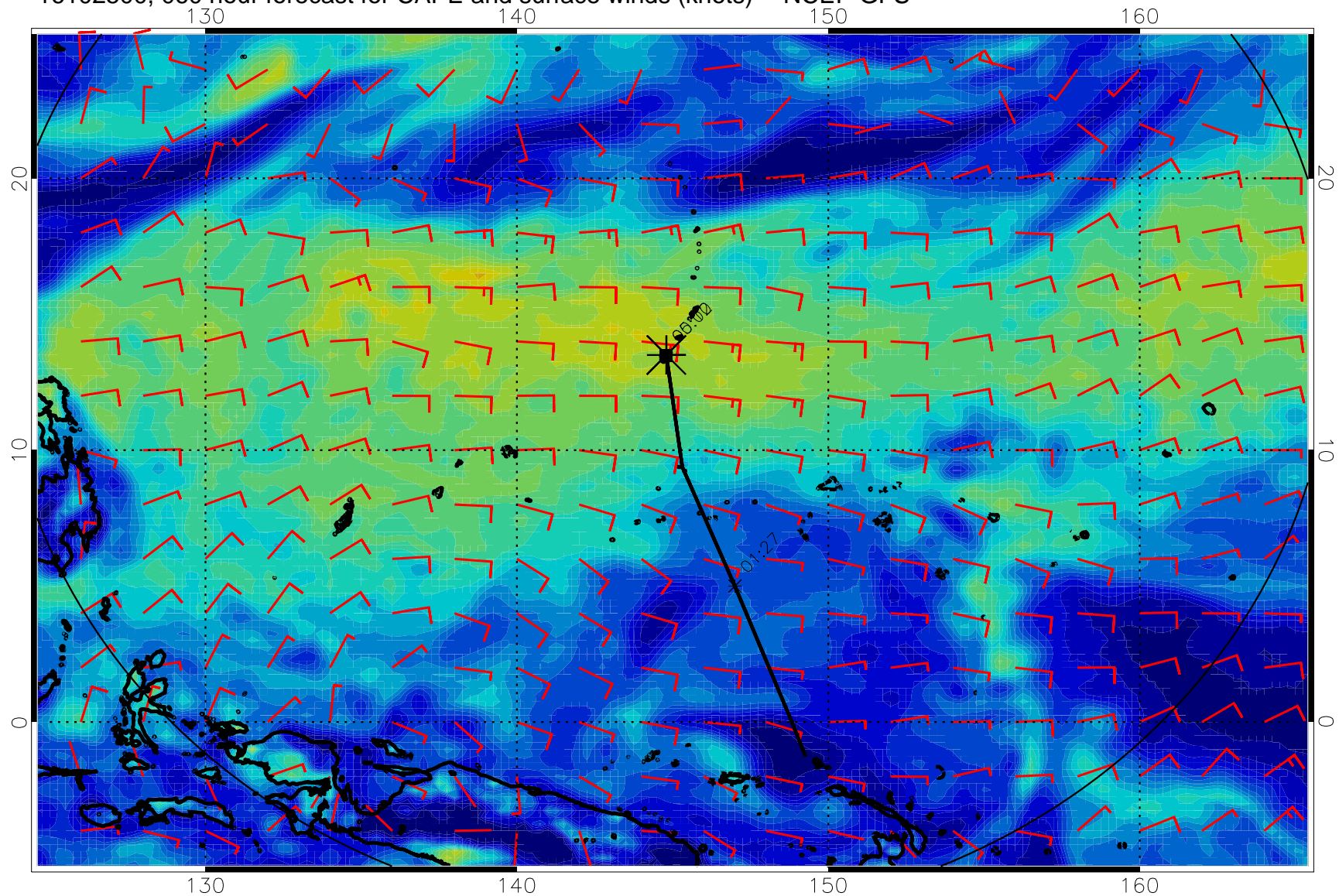
16102500, 060 hour forecast for CAPE and surface winds (knots) -- NCEP GFS
