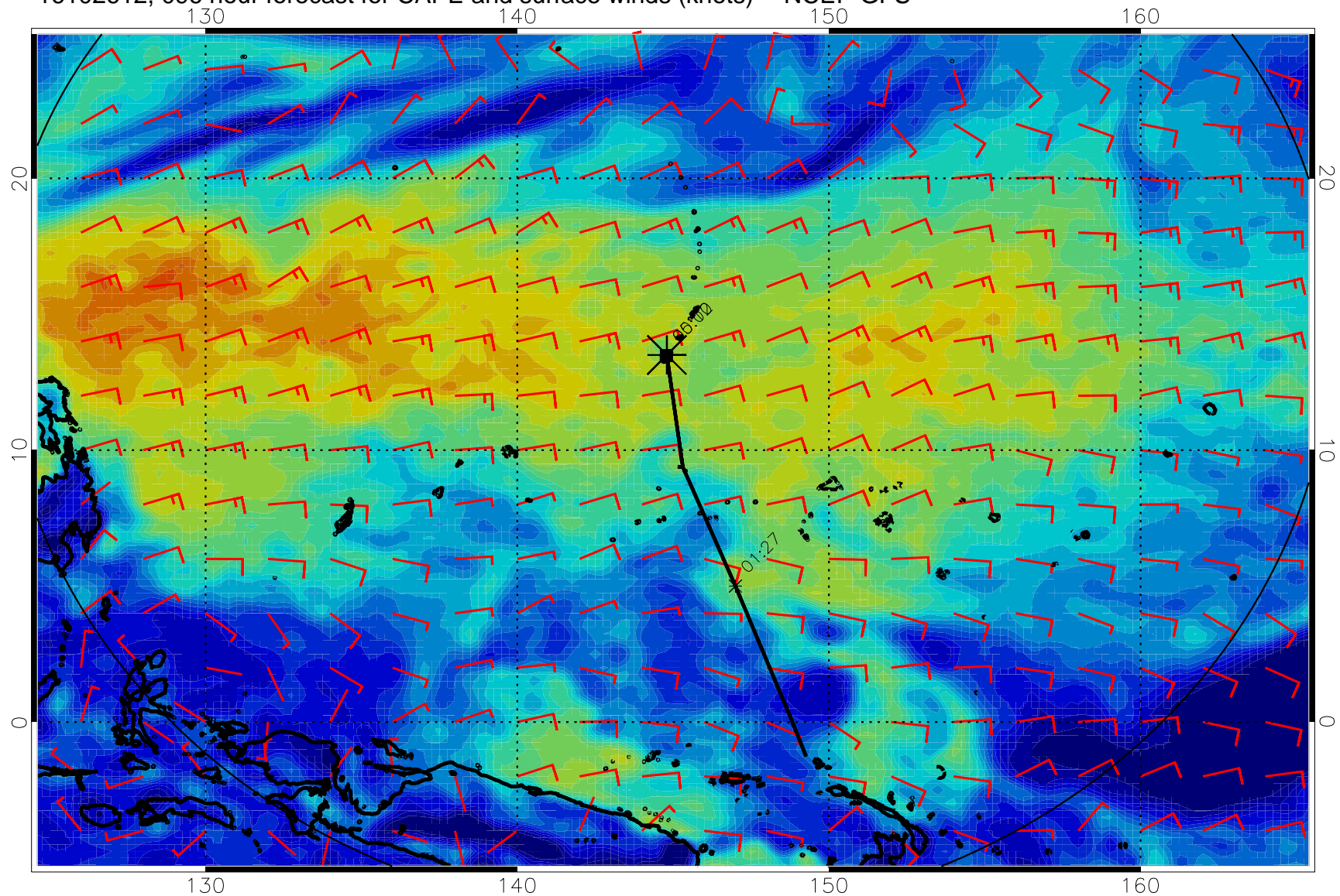
16102612, 096 hour forecast for CAPE and surface winds (knots) -- NCEP GFS
