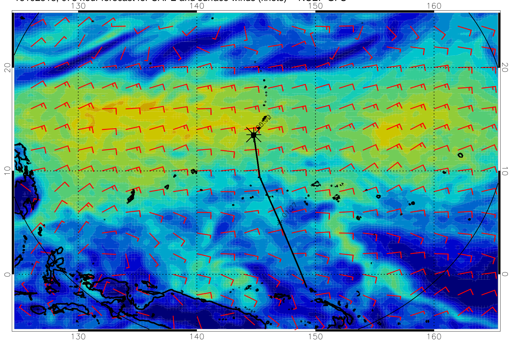
16102518, 078 hour forecast for CAPE and surface winds (knots) -- NCEP GFS
