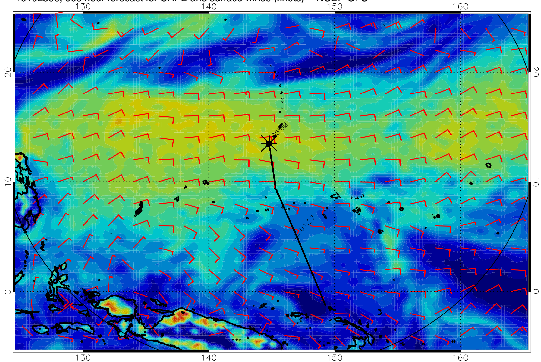
16102506, 066 hour forecast for CAPE and surface winds (knots) -- NCEP GFS
