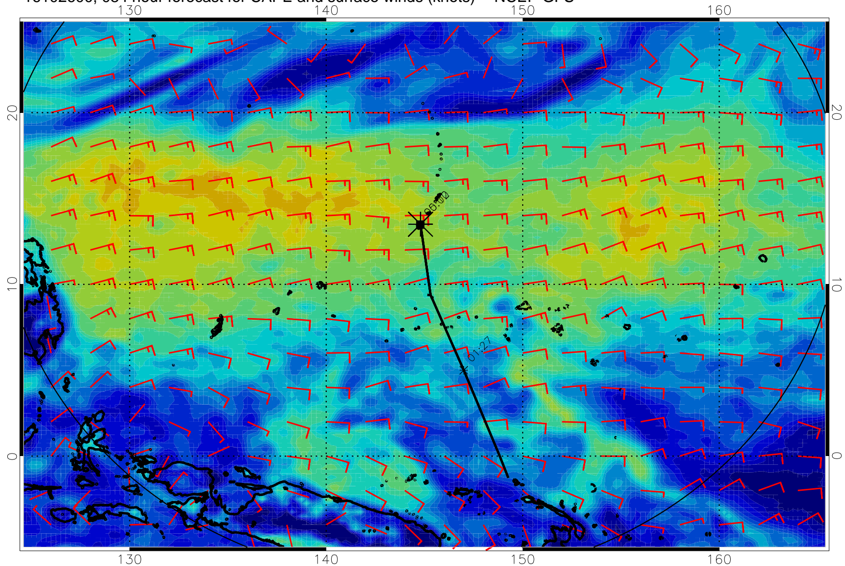
16102600, 084 hour forecast for CAPE and surface winds (knots) -- NCEP GFS
