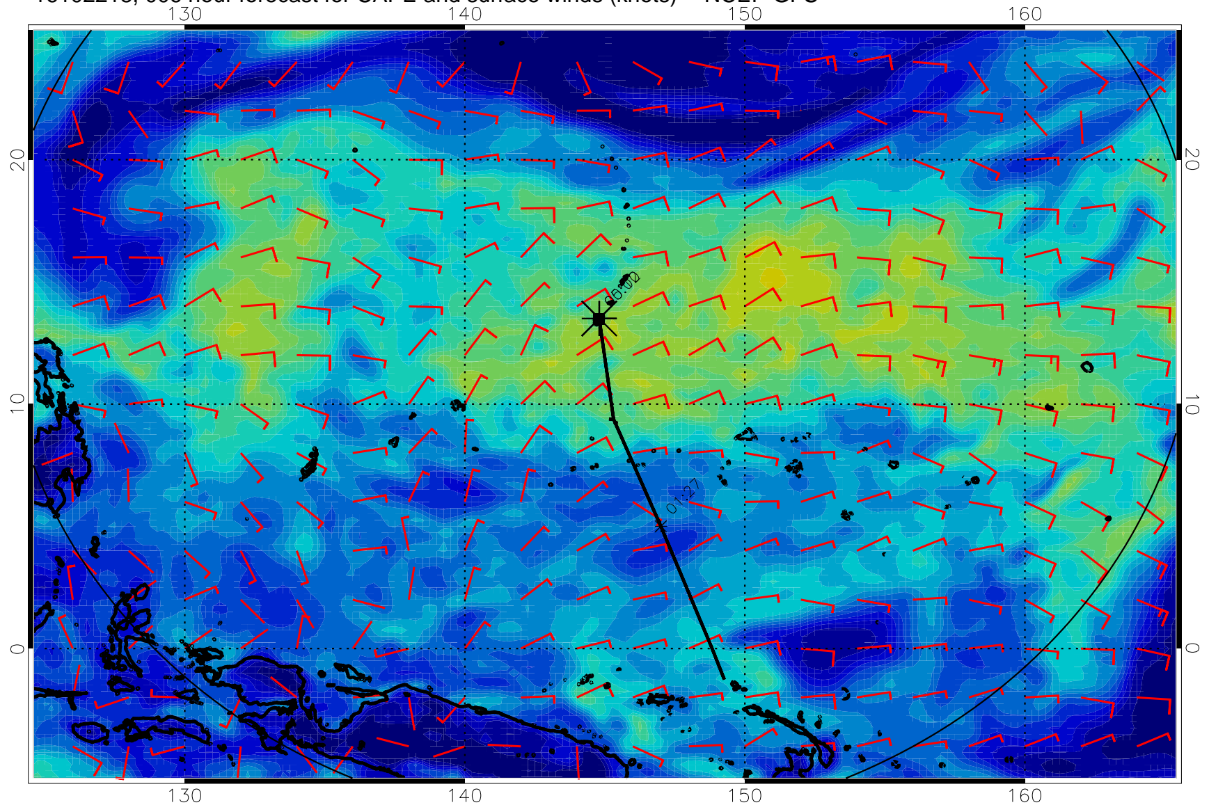
16102218, 006 hour forecast for CAPE and surface winds (knots) -- NCEP GFS
