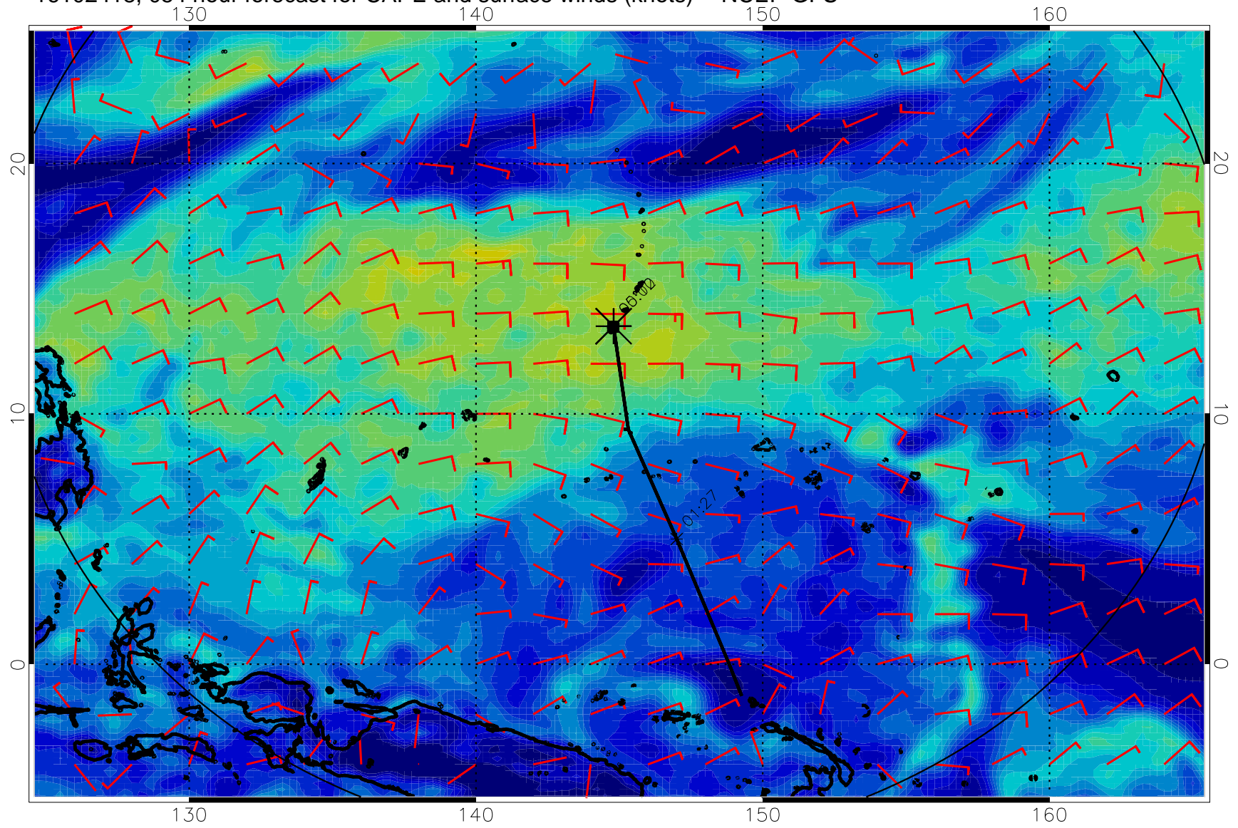
16102418, 054 hour forecast for CAPE and surface winds (knots) -- NCEP GFS
