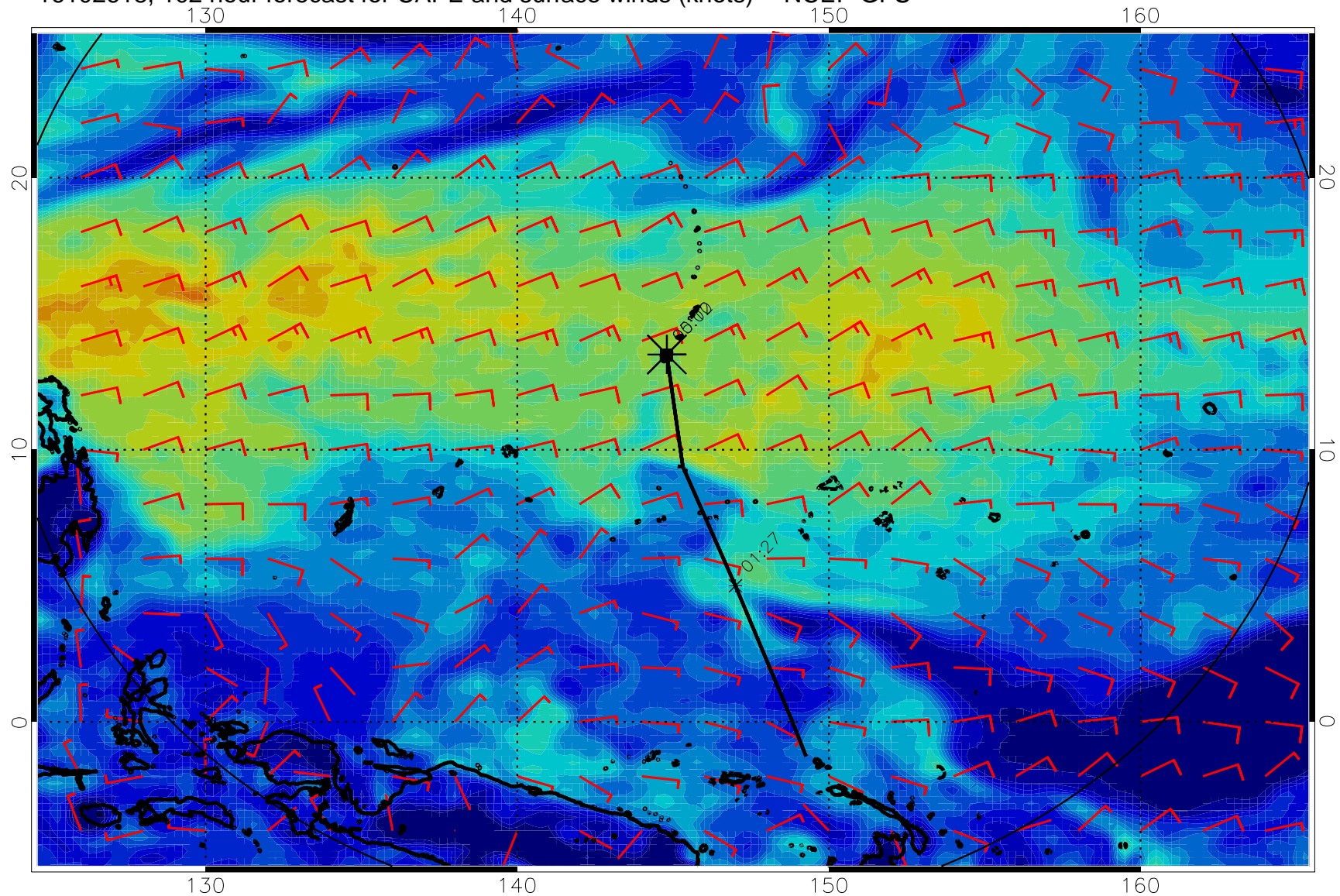
16102618, 102 hour forecast for CAPE and surface winds (knots) -- NCEP GFS
