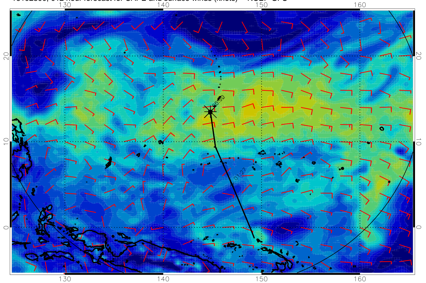
16102300, 012 hour forecast for CAPE and surface winds (knots) -- NCEP GFS
