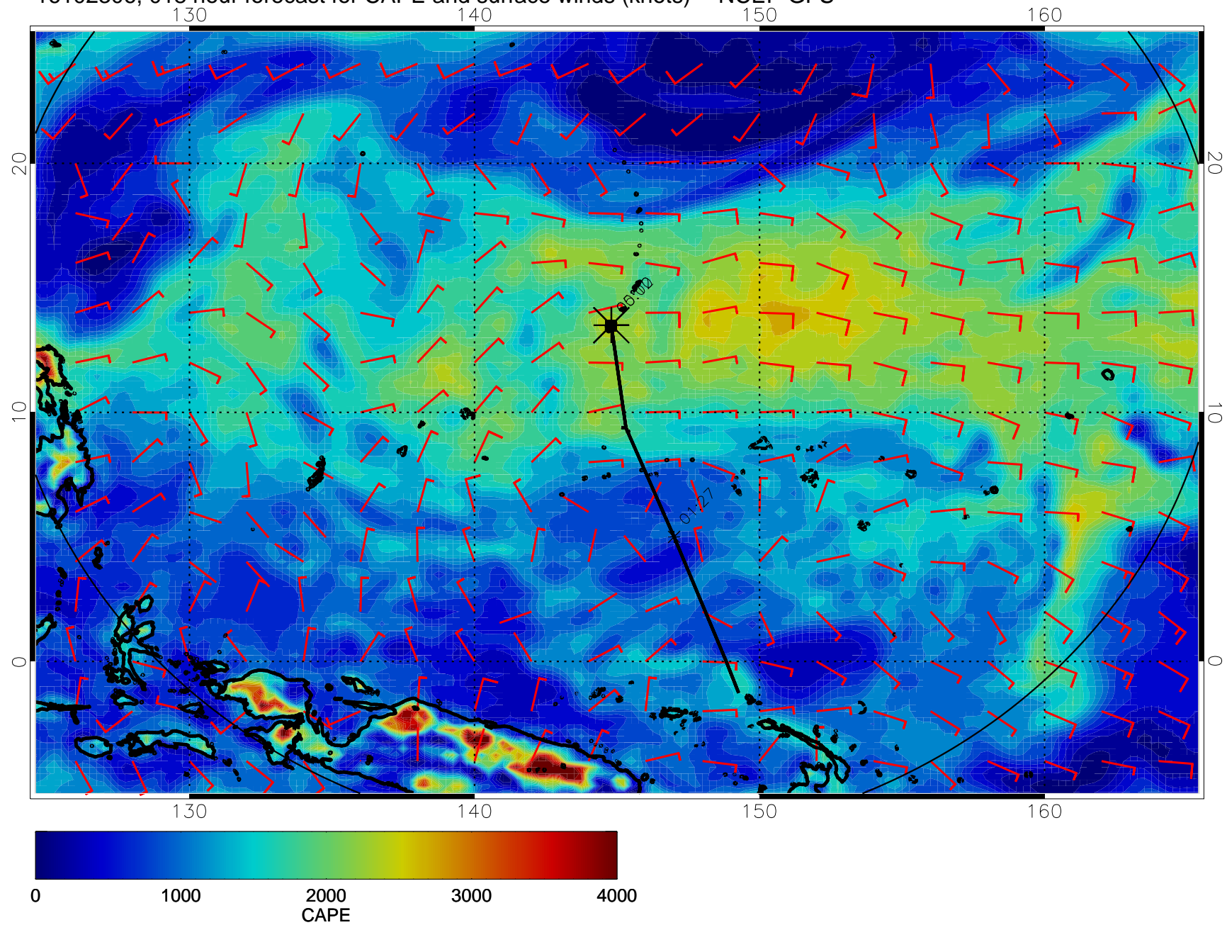
16102306, 018 hour forecast for CAPE and surface winds (knots) -- NCEP GFS
