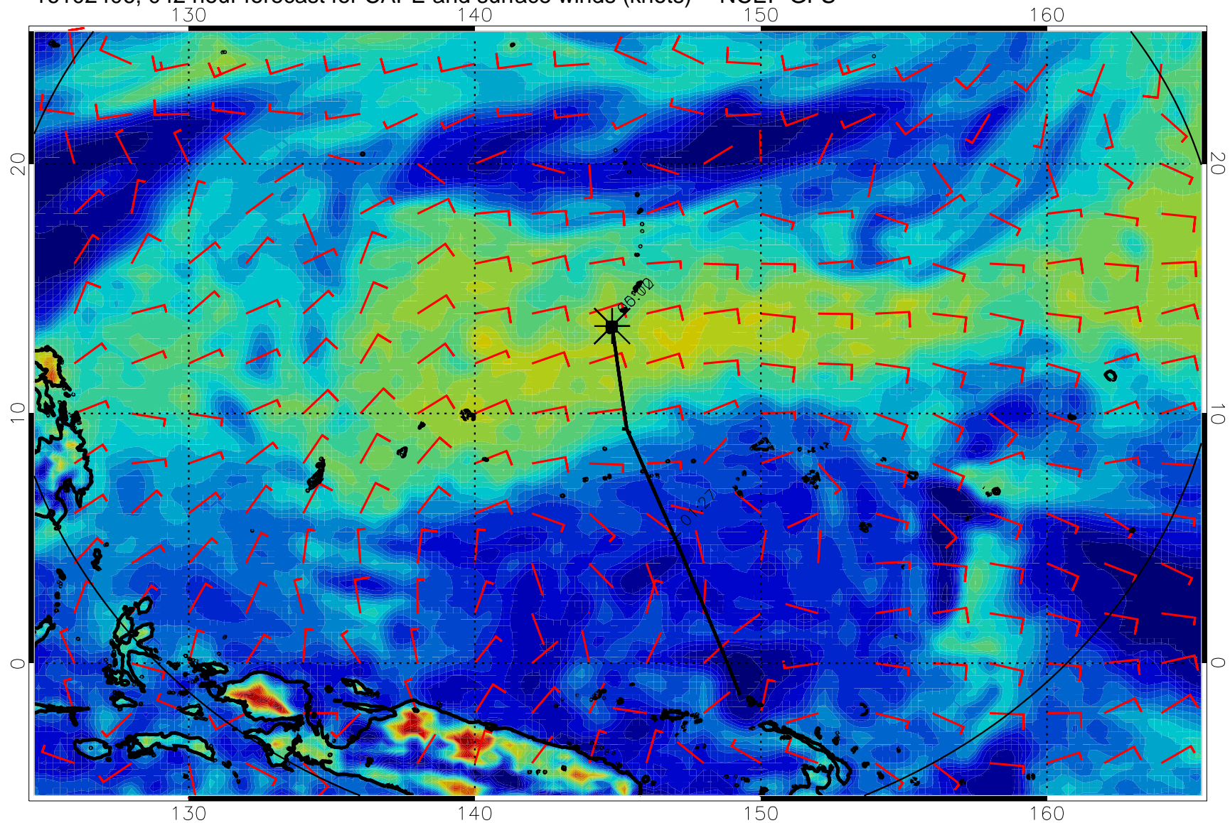
16102406, 042 hour forecast for CAPE and surface winds (knots) -- NCEP GFS
