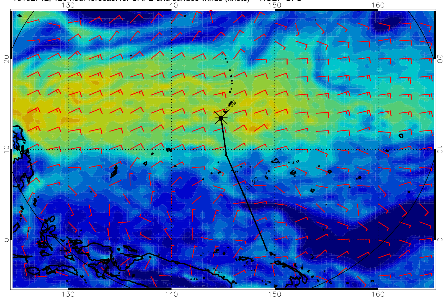
16102712, 120 hour forecast for CAPE and surface winds (knots) -- NCEP GFS
