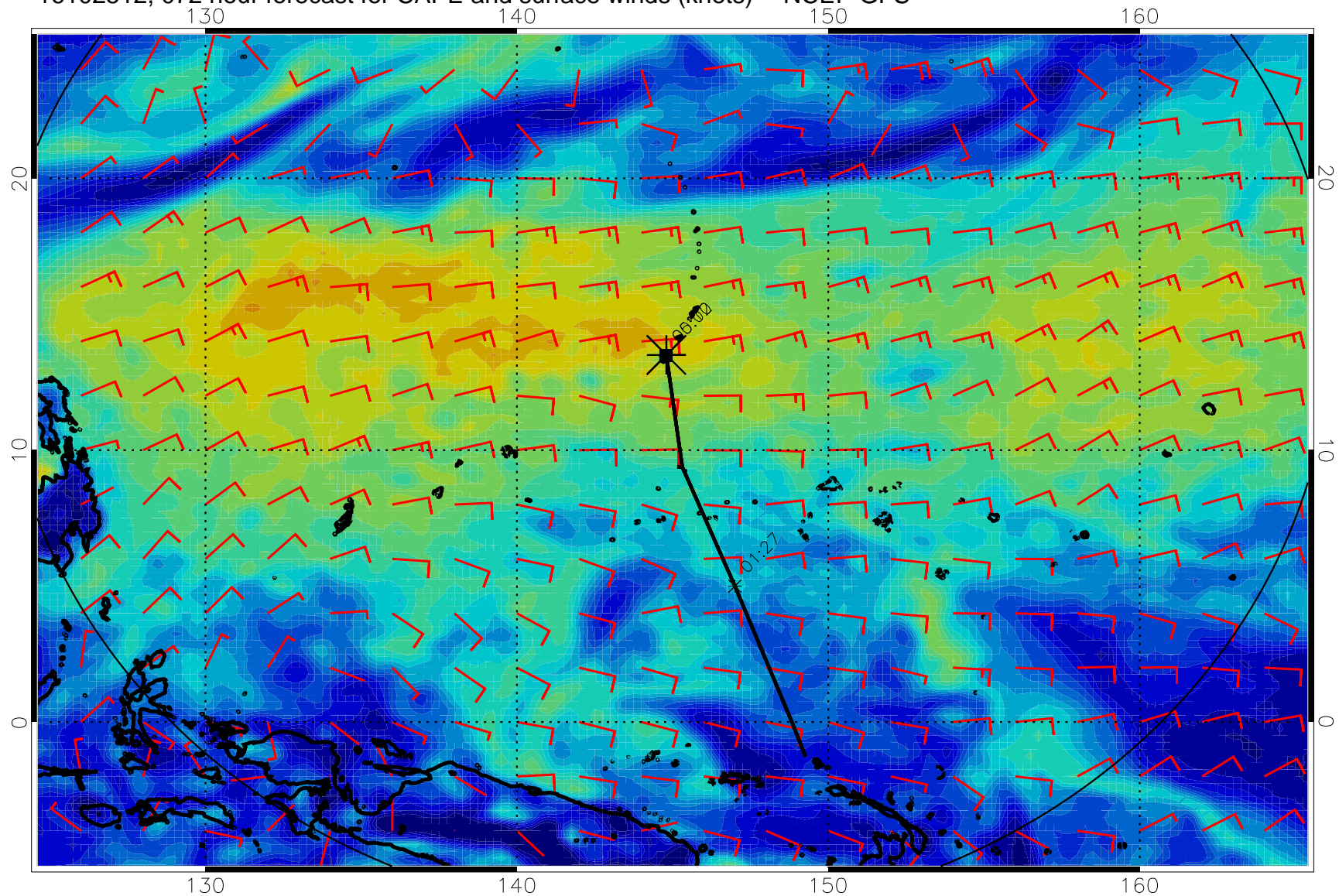
16102512, 072 hour forecast for CAPE and surface winds (knots) -- NCEP GFS
