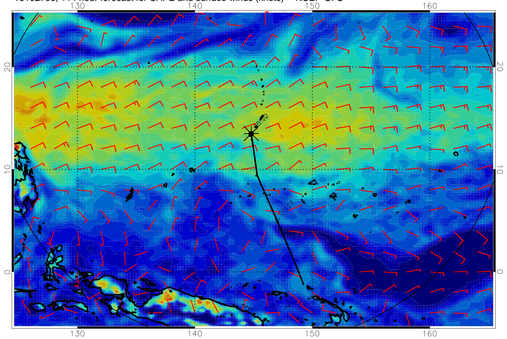
16102706, 114 hour forecast for CAPE and surface winds (knots) -- NCEP GFS
