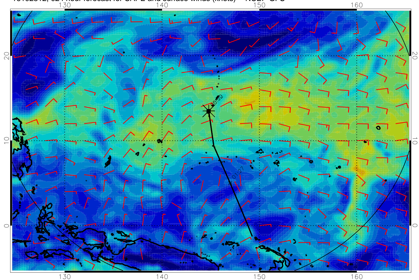
16102312, 024 hour forecast for CAPE and surface winds (knots) -- NCEP GFS
