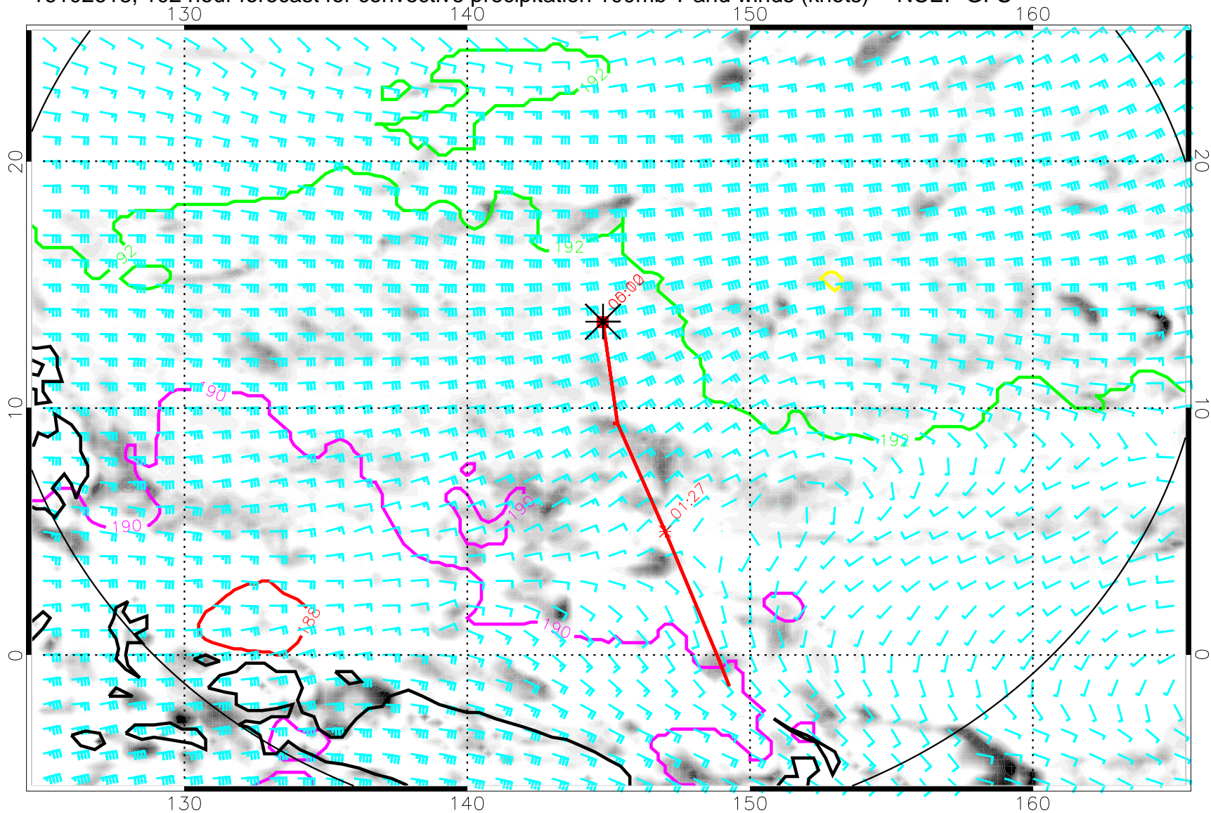
16102618, 102 hour forecast for convective precipitation 100mb T and winds (knots) -- NCEP GFS
