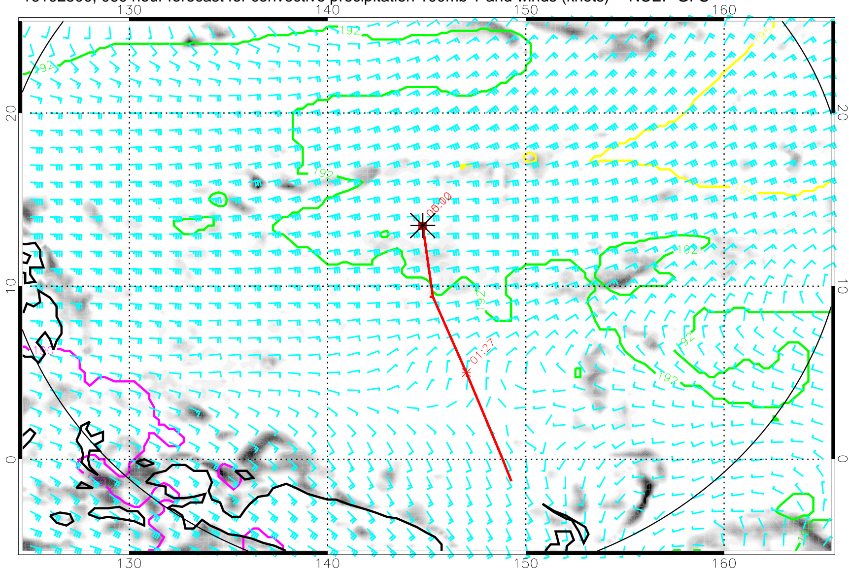
16102500, 060 hour forecast for convective precipitation 100mb T and winds (knots) -- NCEP GFS
