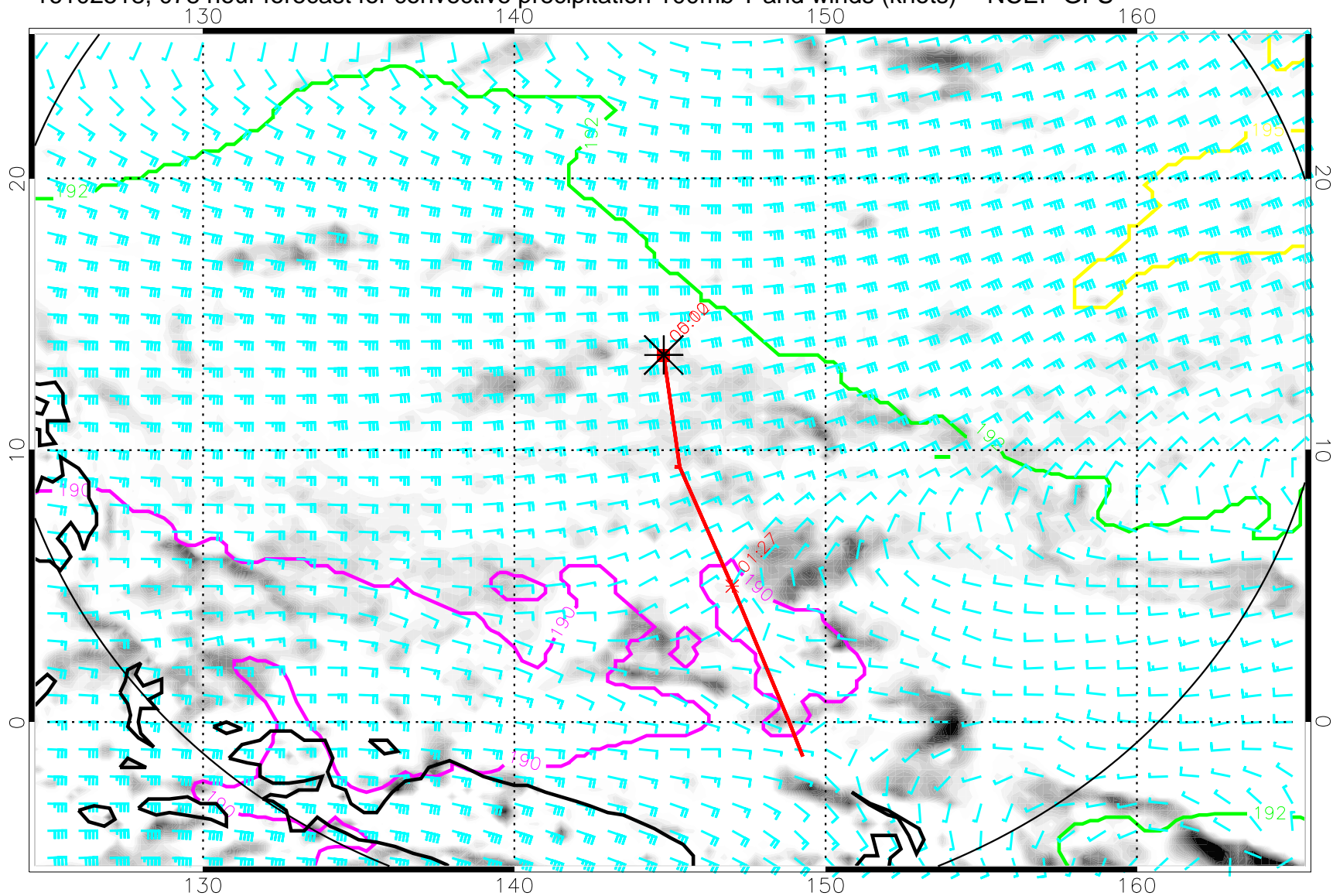
16102518, 078 hour forecast for convective precipitation 100mb T and winds (knots) -- NCEP GFS
