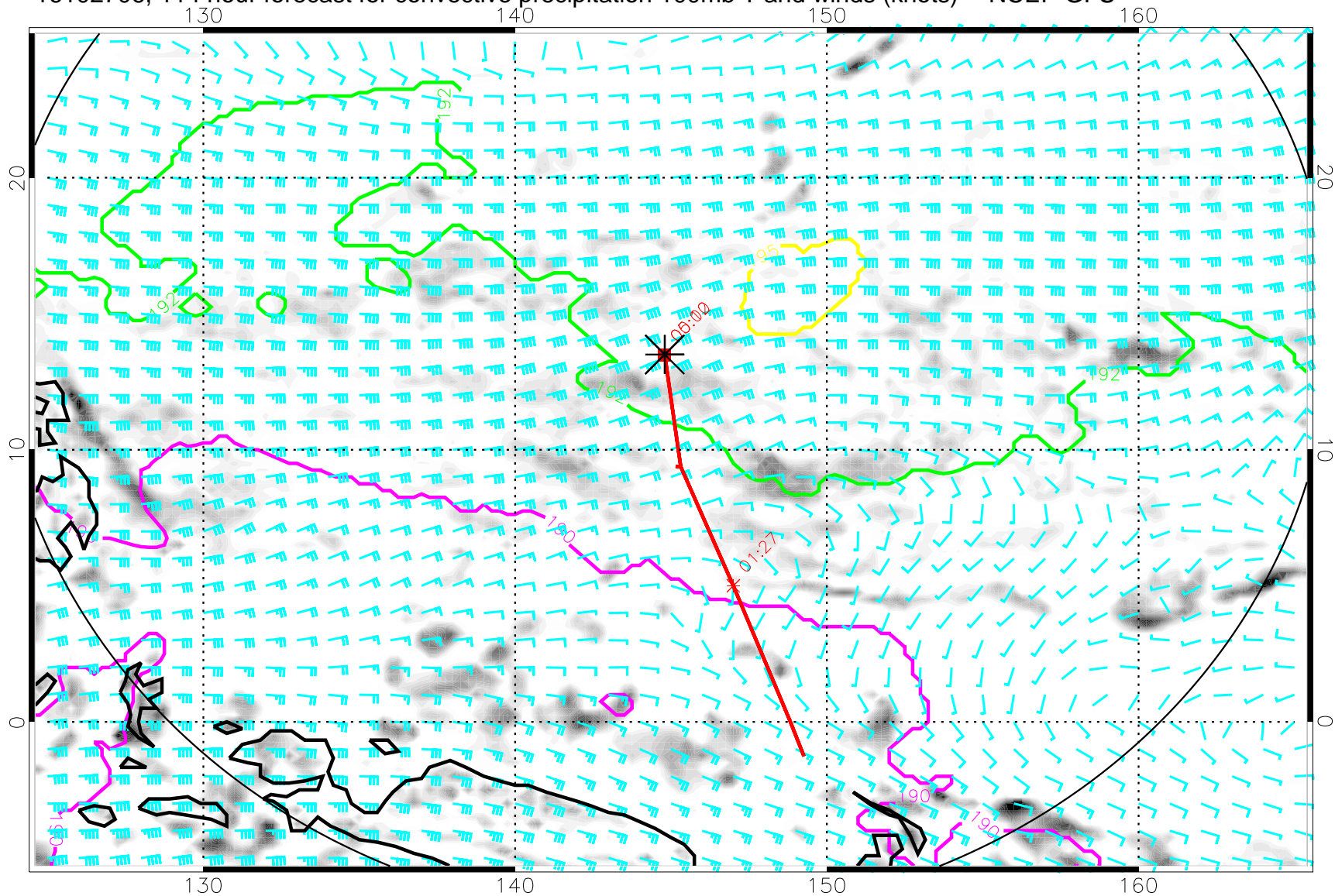
16102706, 114 hour forecast for convective precipitation 100mb T and winds (knots) -- NCEP GFS
