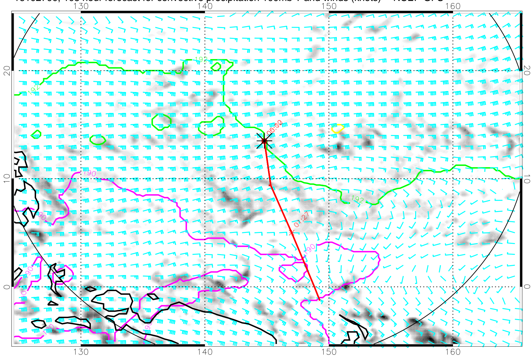
16102700, 108 hour forecast for convective precipitation 100mb T and winds (knots) -- NCEP GFS
