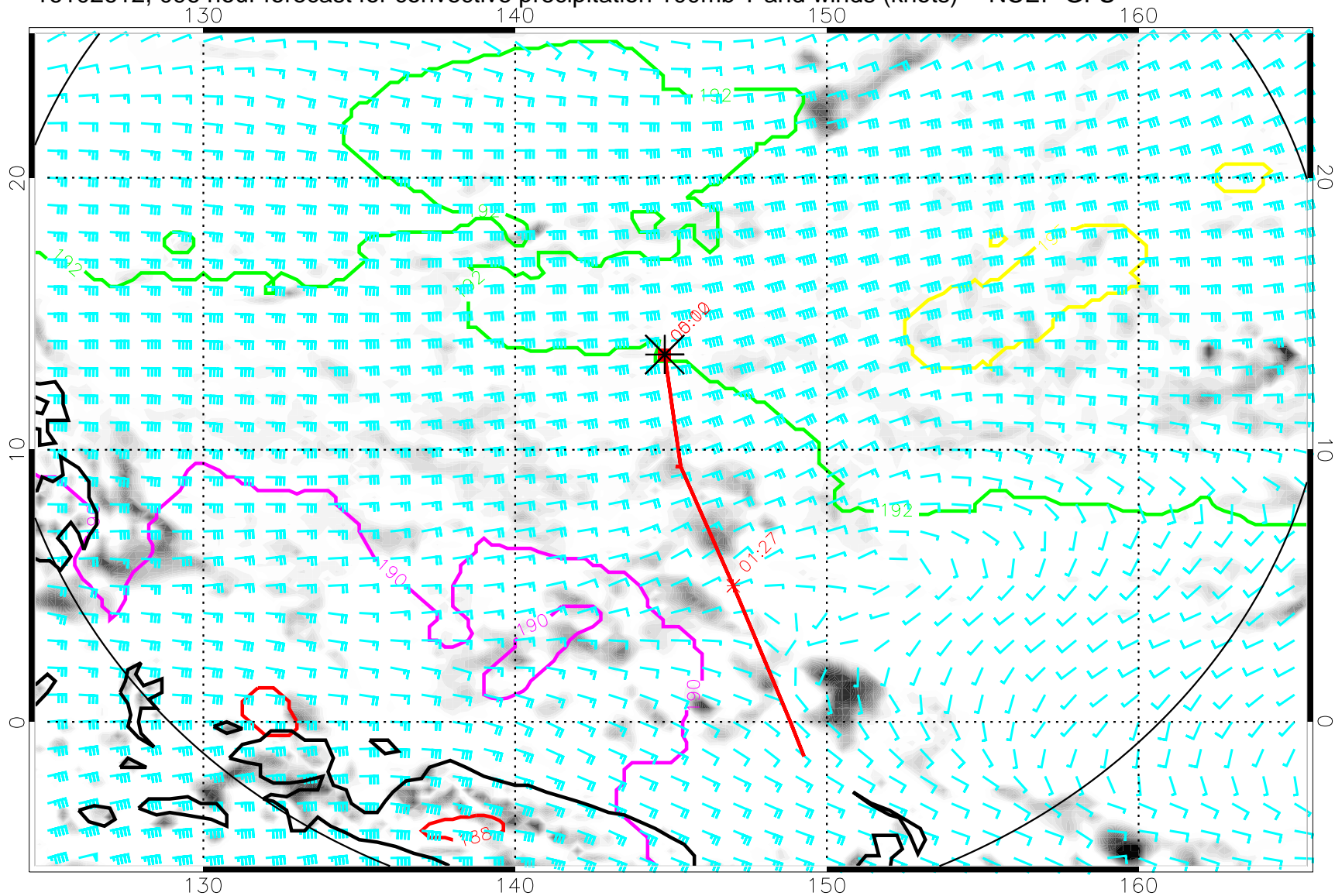
16102612, 096 hour forecast for convective precipitation 100mb T and winds (knots) -- NCEP GFS
