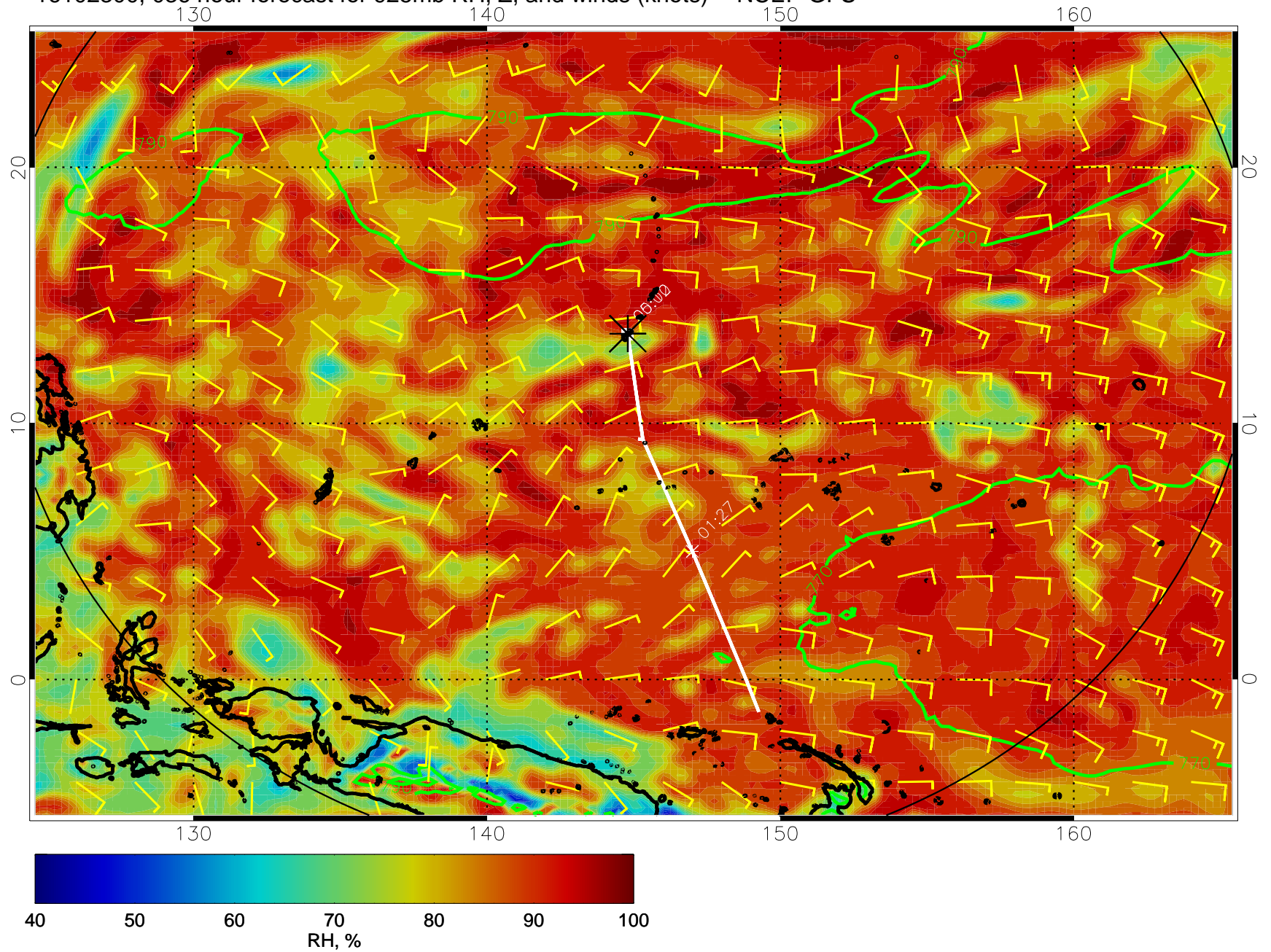
16102300, 036 hour forecast for 925mb RH, Z, and winds (knots) -- NCEP GFS
