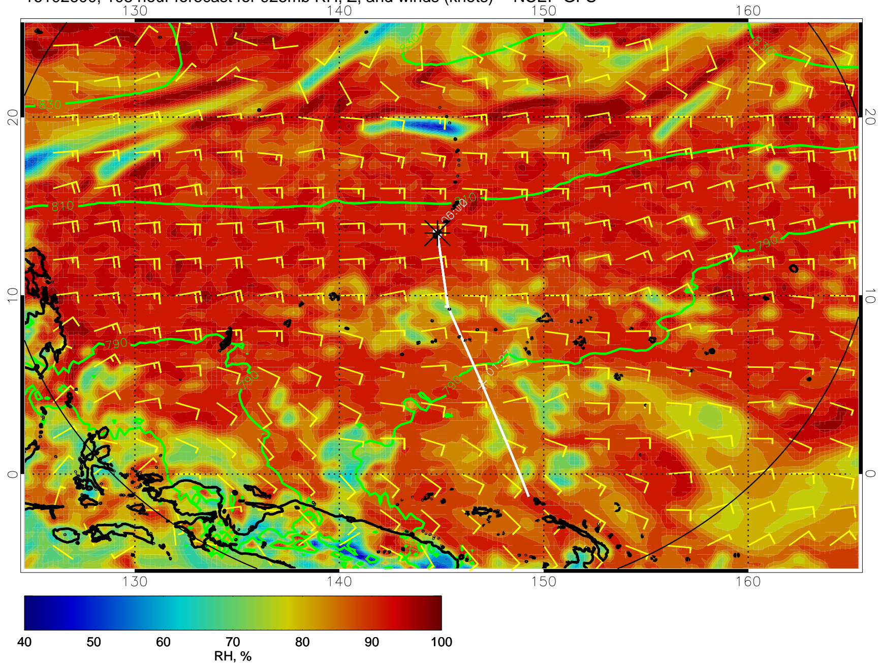
16102600, 108 hour forecast for 925mb RH, Z, and winds (knots) -- NCEP GFS
