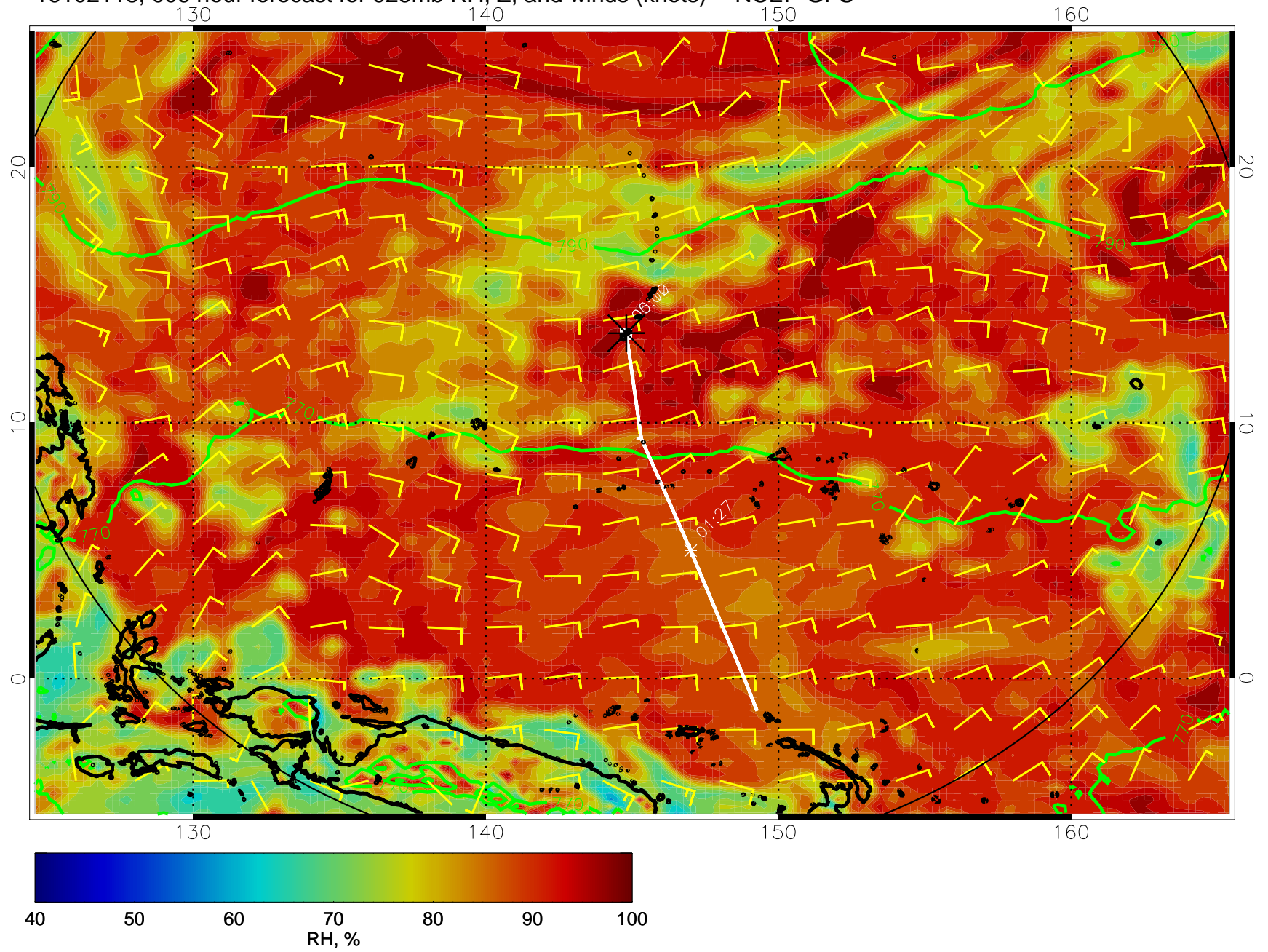
16102118, 006 hour forecast for 925mb RH, Z, and winds (knots) -- NCEP GFS
