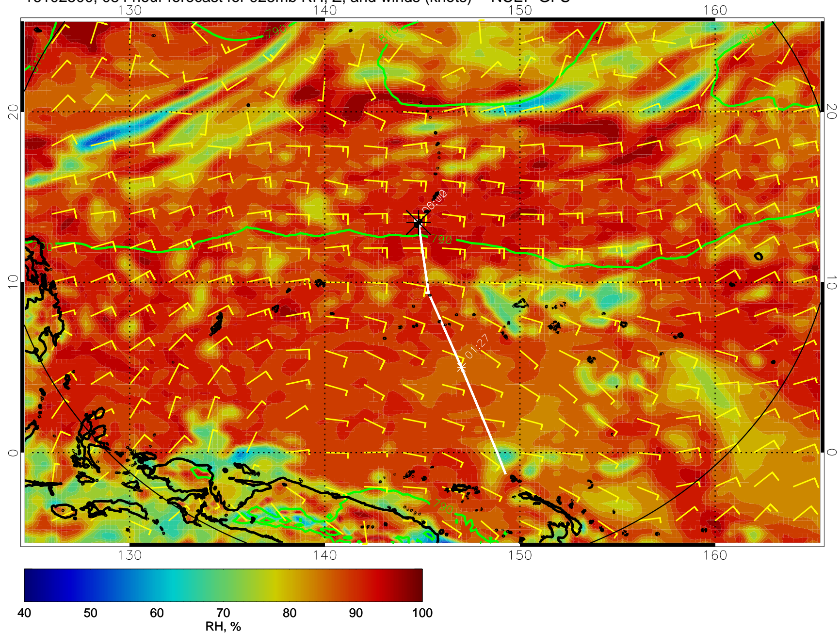
16102500, 084 hour forecast for 925mb RH, Z, and winds (knots) -- NCEP GFS
