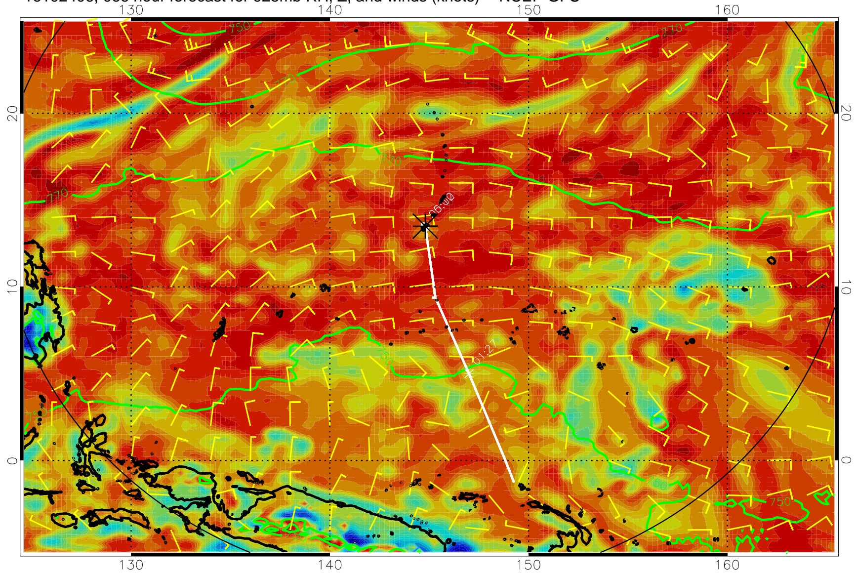
16102406, 066 hour forecast for 925mb RH, Z, and winds (knots) -- NCEP GFS
