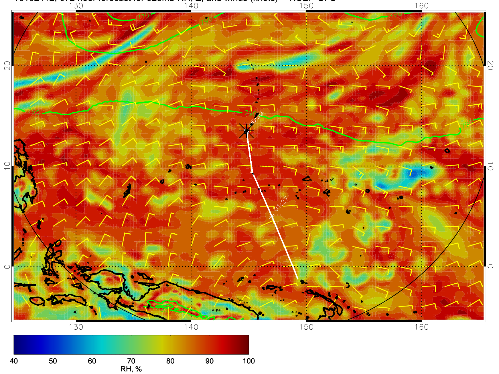
16102412, 072 hour forecast for 925mb RH, Z, and winds (knots) -- NCEP GFS
