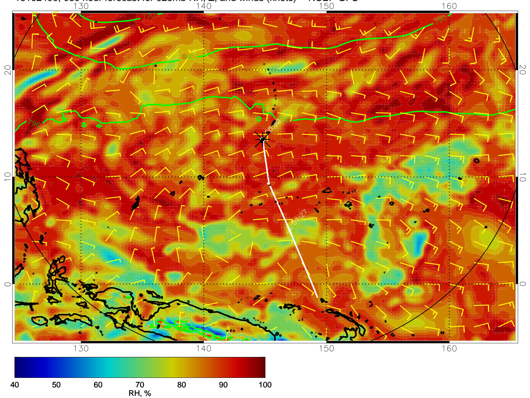
16102400, 060 hour forecast for 925mb RH, Z, and winds (knots) -- NCEP GFS
