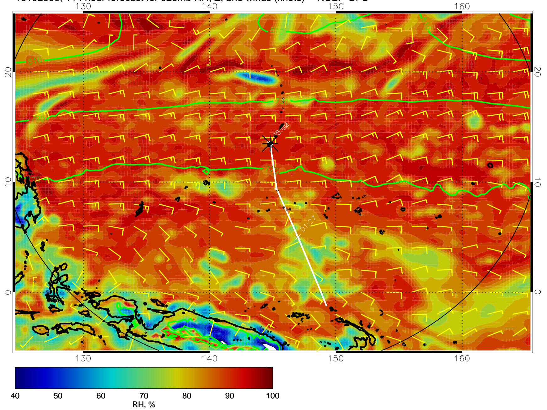
16102606, 114 hour forecast for 925mb RH, Z, and winds (knots) -- NCEP GFS
