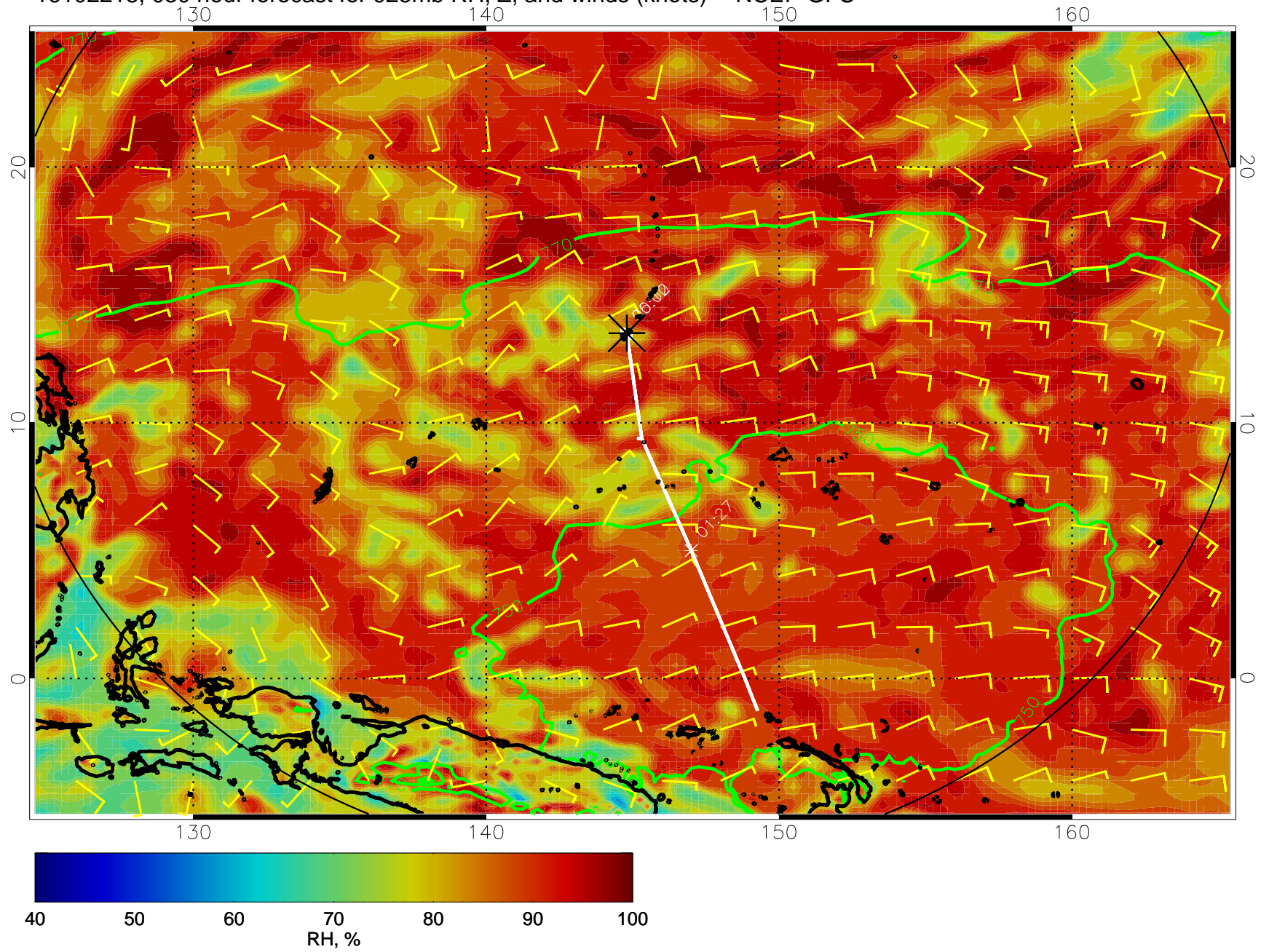
16102218, 030 hour forecast for 925mb RH, Z, and winds (knots) -- NCEP GFS
