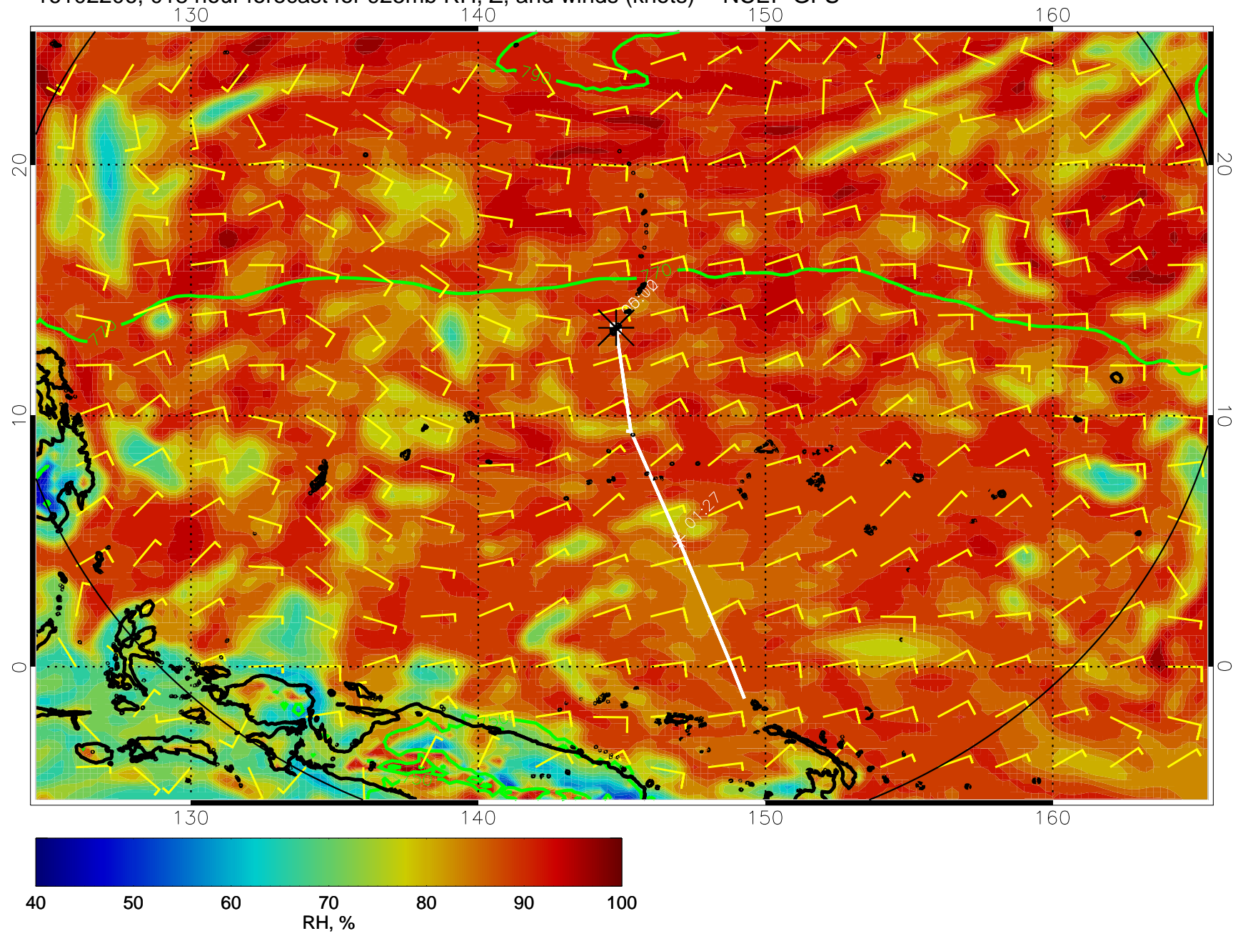
16102206, 018 hour forecast for 925mb RH, Z, and winds (knots) -- NCEP GFS
