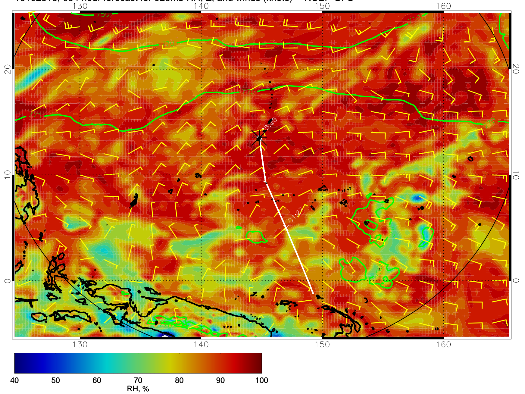
16102318, 054 hour forecast for 925mb RH, Z, and winds (knots) -- NCEP GFS
