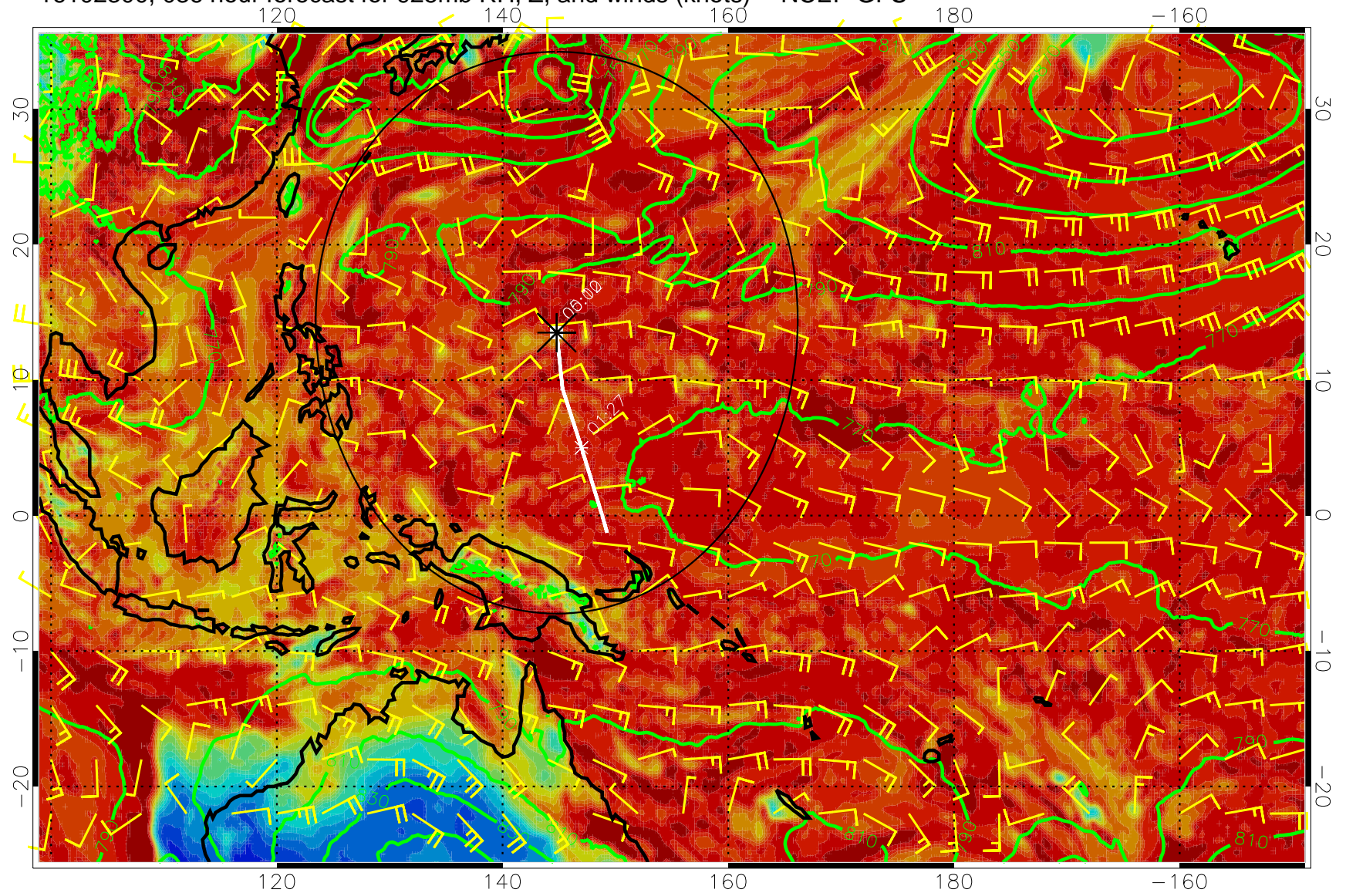
16102300, 036 hour forecast for 925mb RH, Z, and winds (knots) -- NCEP GFS
