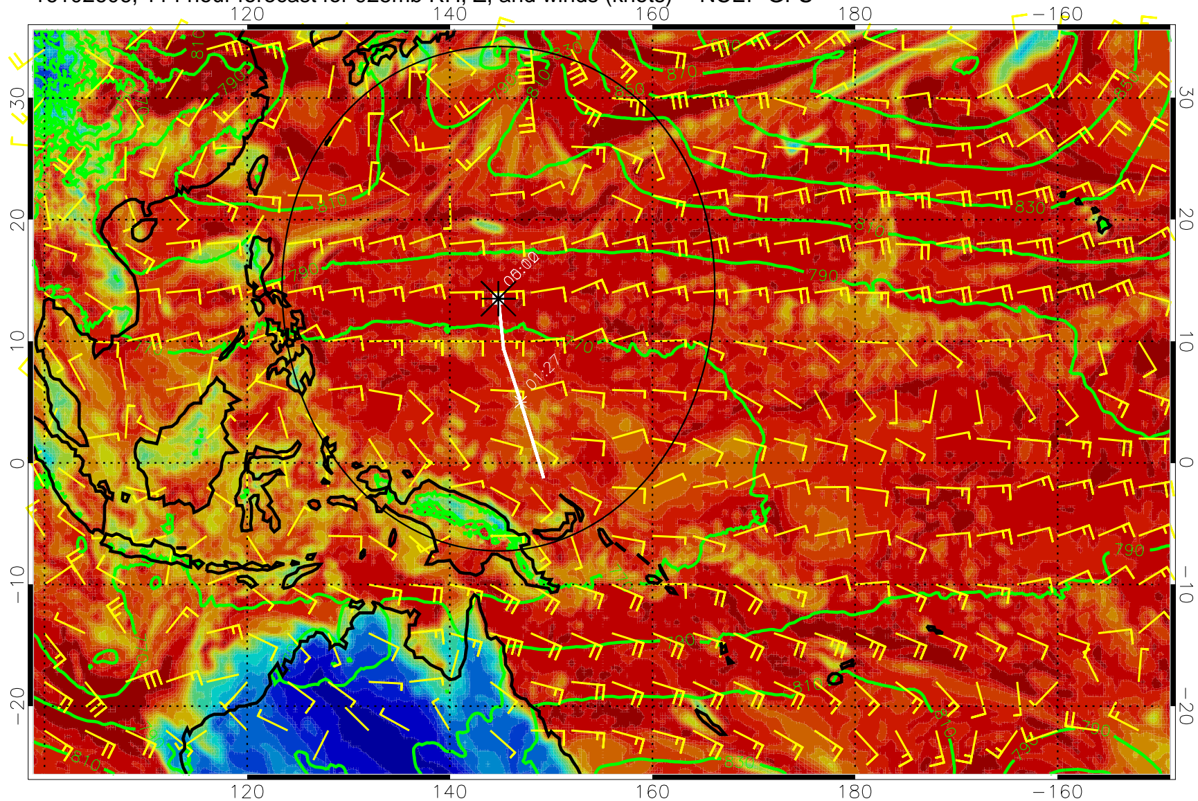
16102606, 114 hour forecast for 925mb RH, Z, and winds (knots) -- NCEP GFS
