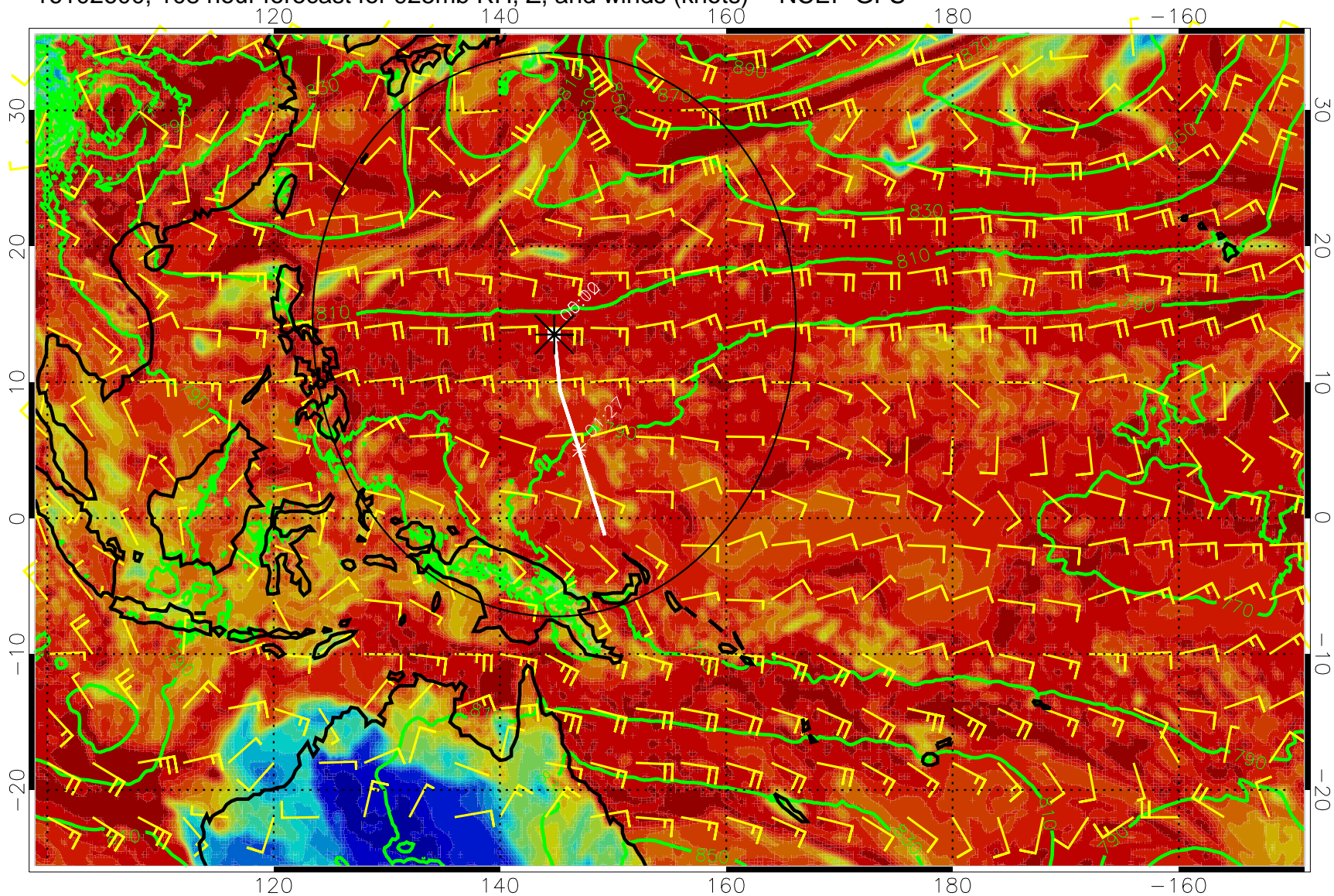
16102600, 108 hour forecast for 925mb RH, Z, and winds (knots) -- NCEP GFS
