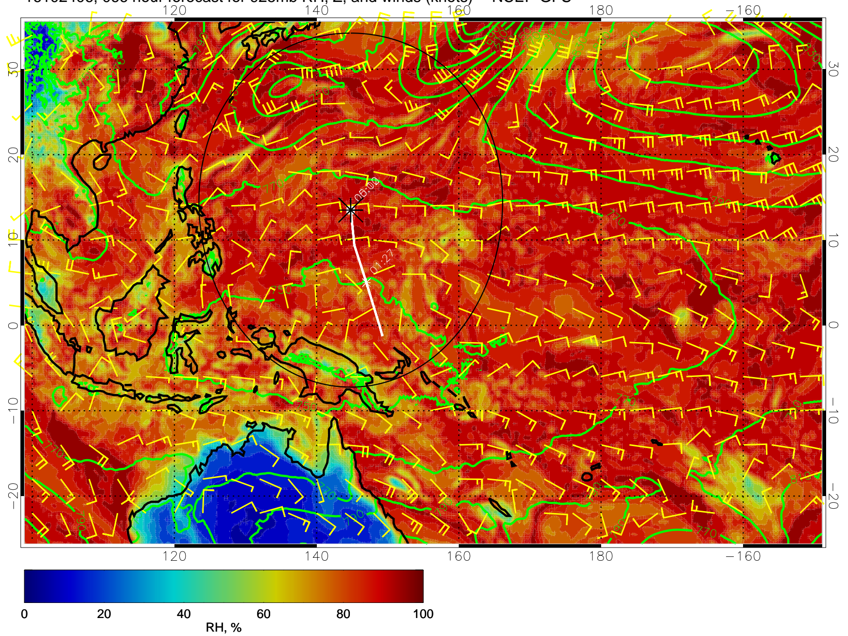
16102406, 066 hour forecast for 925mb RH, Z, and winds (knots) -- NCEP GFS
