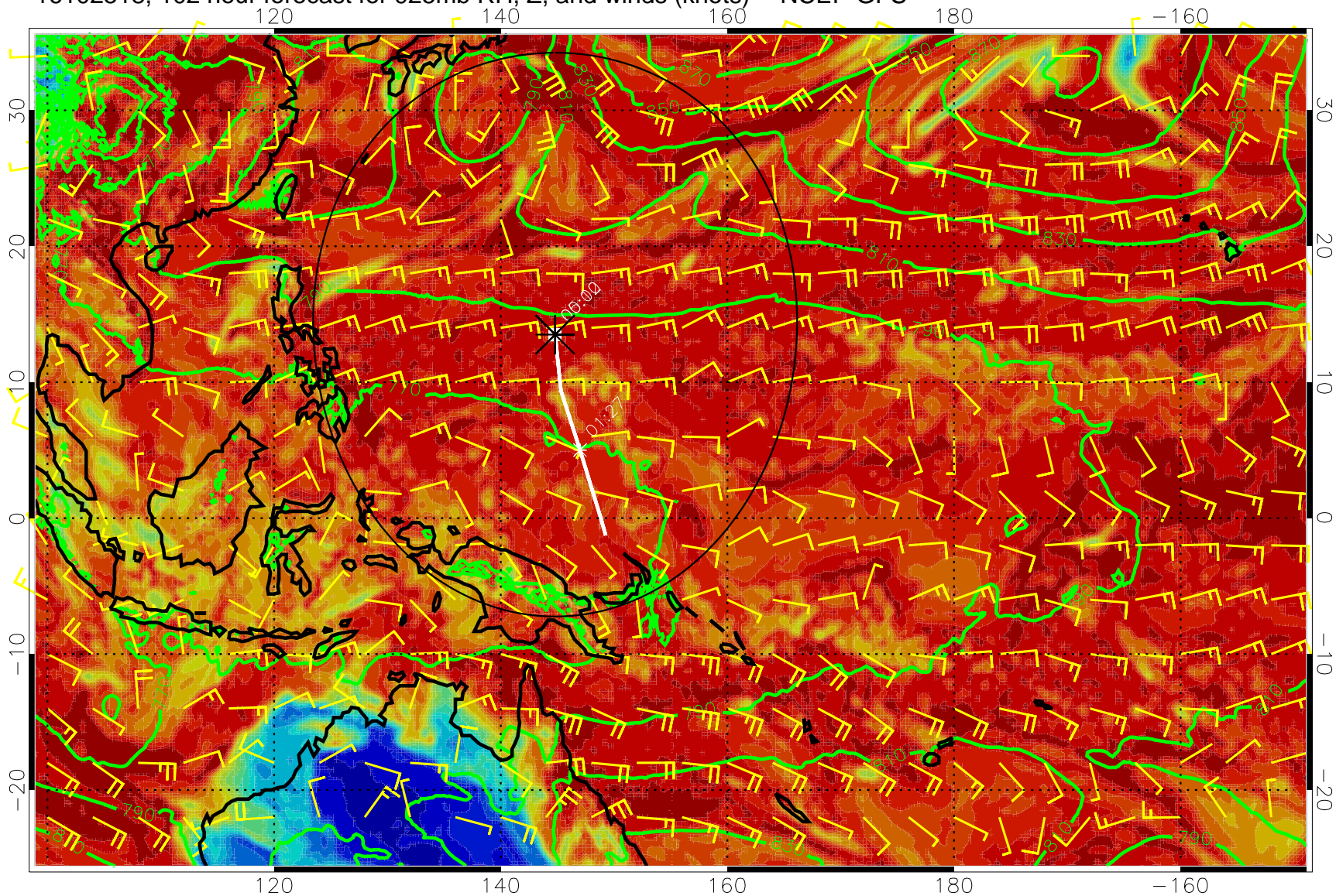
16102518, 102 hour forecast for 925mb RH, Z, and winds (knots) -- NCEP GFS
