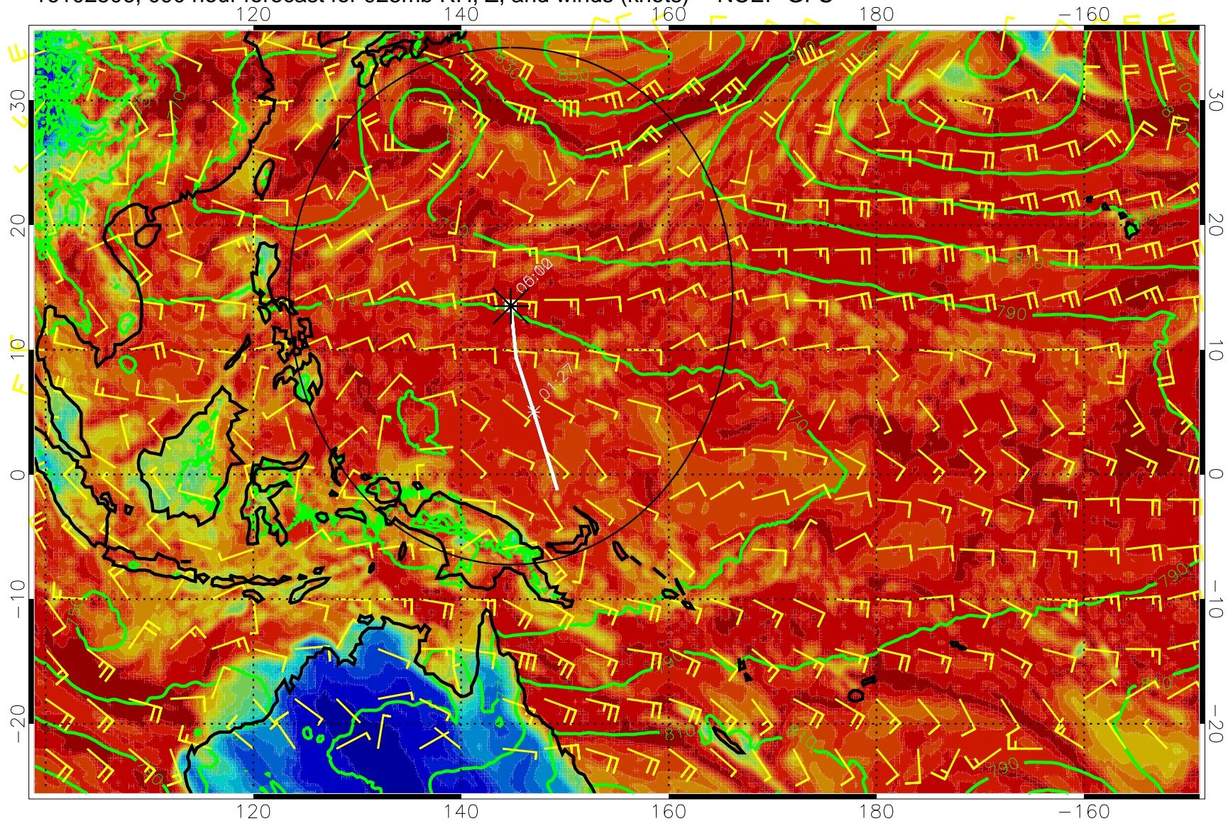
16102506, 090 hour forecast for 925mb RH, Z, and winds (knots) -- NCEP GFS
