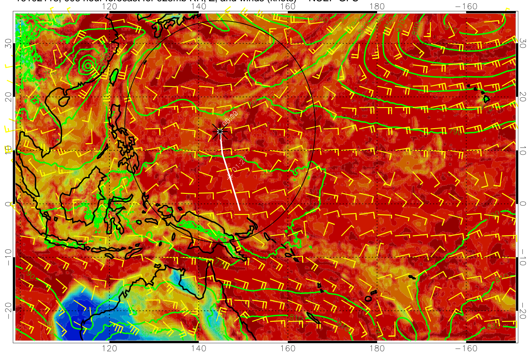
16102118, 006 hour forecast for 925mb RH, Z, and winds (knots) -- NCEP GFS
