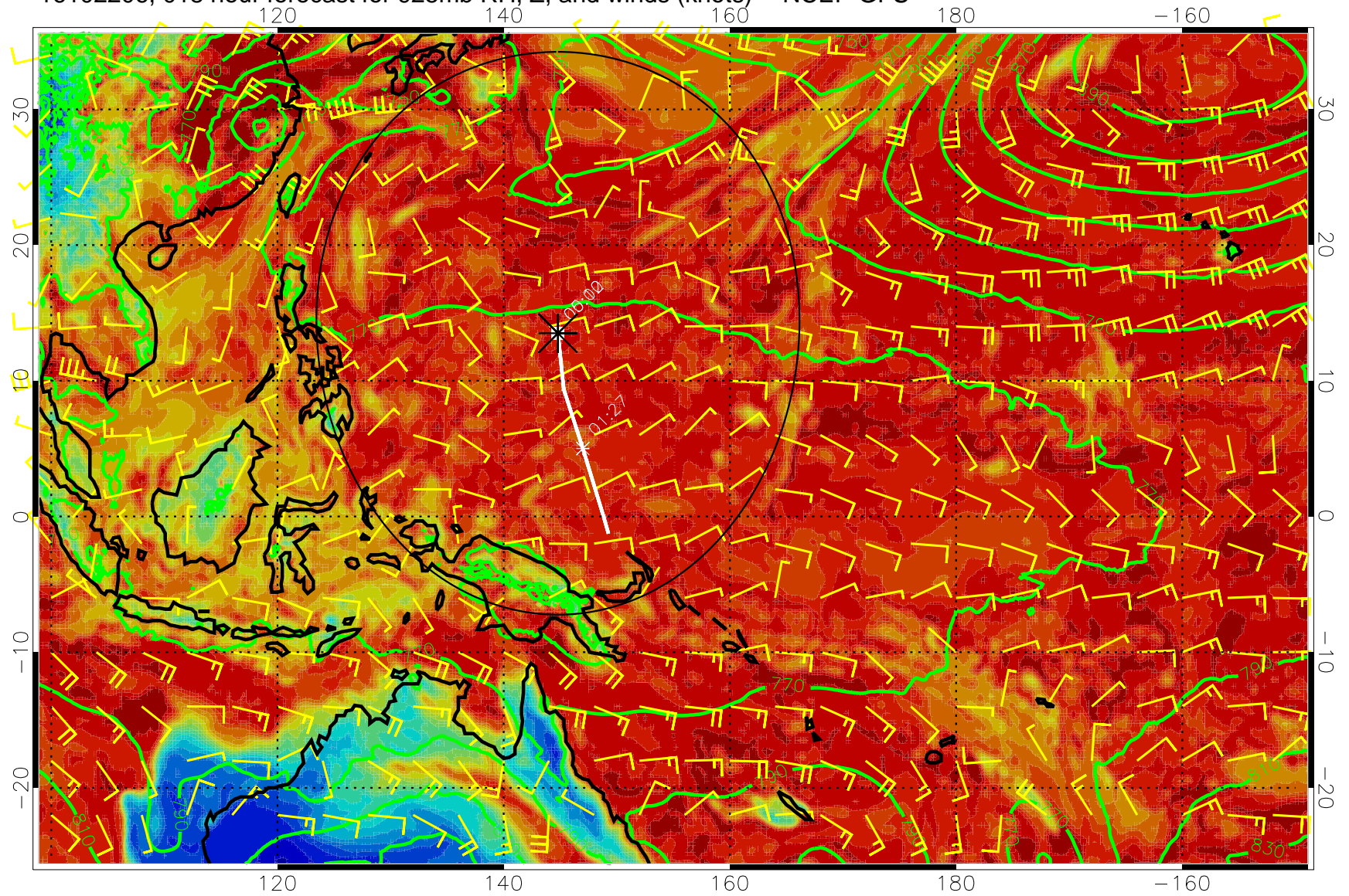
16102206, 018 hour forecast for 925mb RH, Z, and winds (knots) -- NCEP GFS
