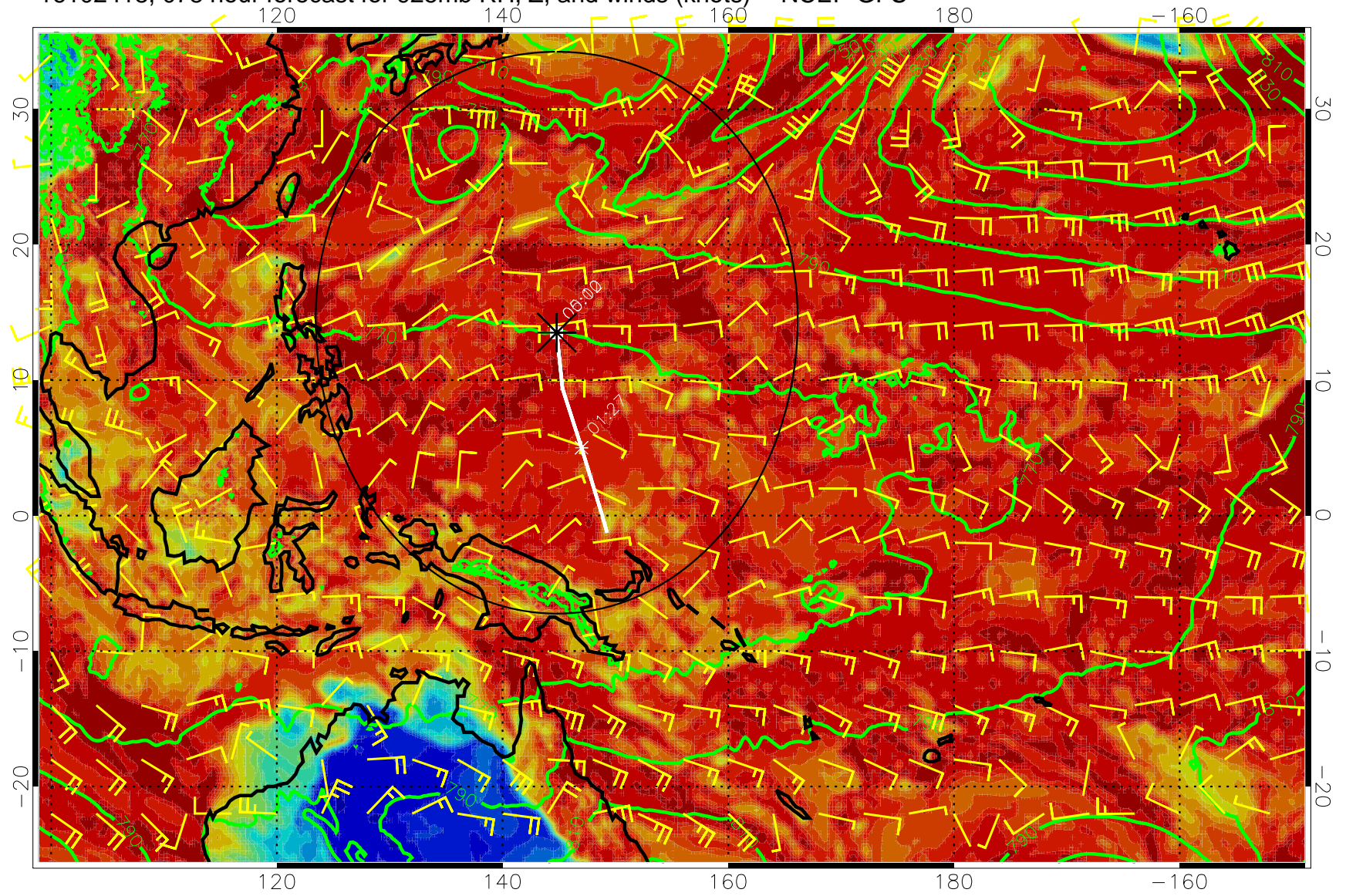
16102418, 078 hour forecast for 925mb RH, Z, and winds (knots) -- NCEP GFS
