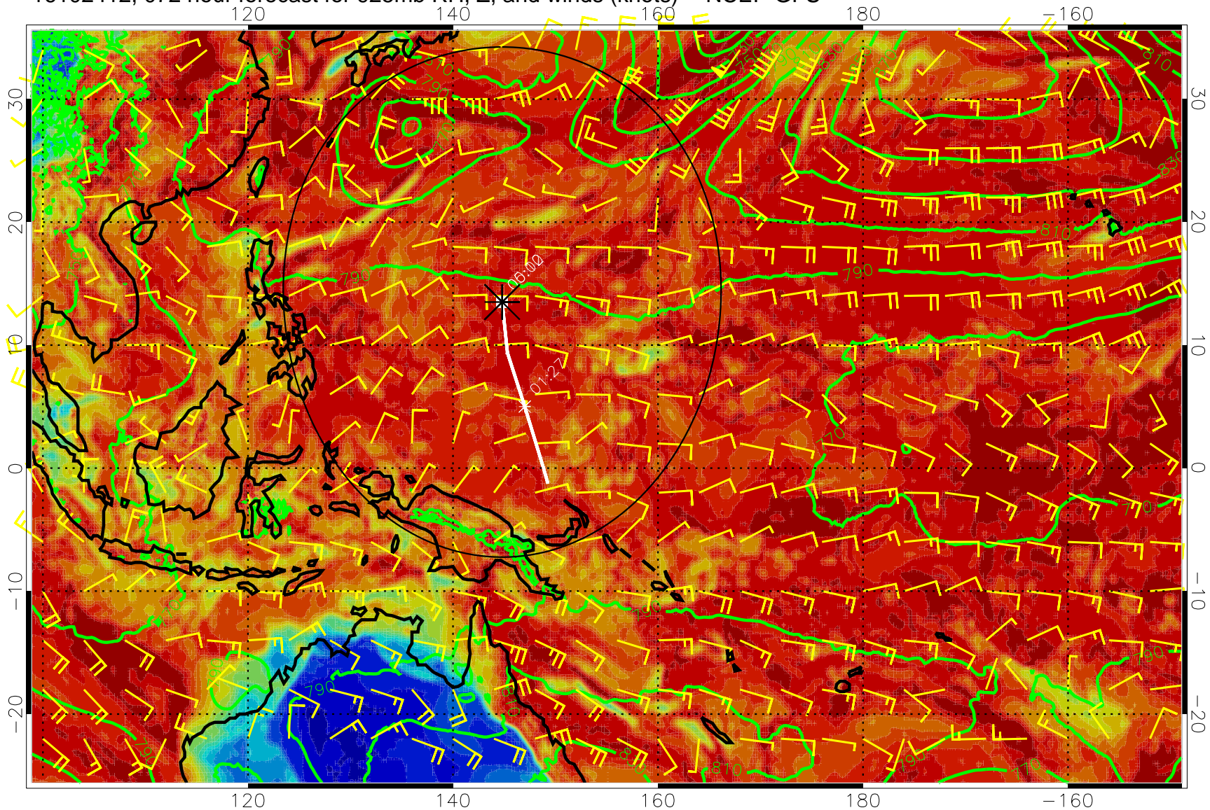
16102412, 072 hour forecast for 925mb RH, Z, and winds (knots) -- NCEP GFS
