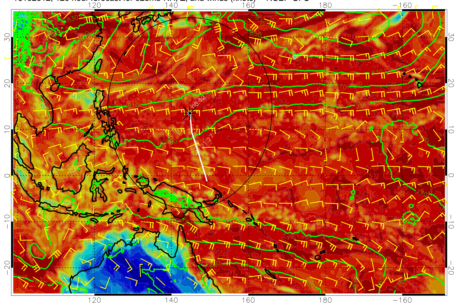
16102612, 120 hour forecast for 925mb RH, Z, and winds (knots) -- NCEP GFS
