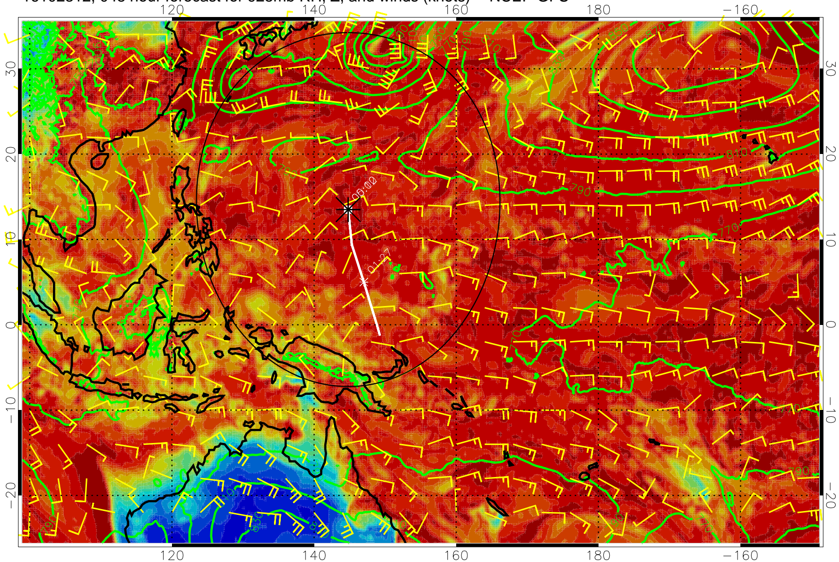
16102312, 048 hour forecast for 925mb RH, Z, and winds (knots) -- NCEP GFS
