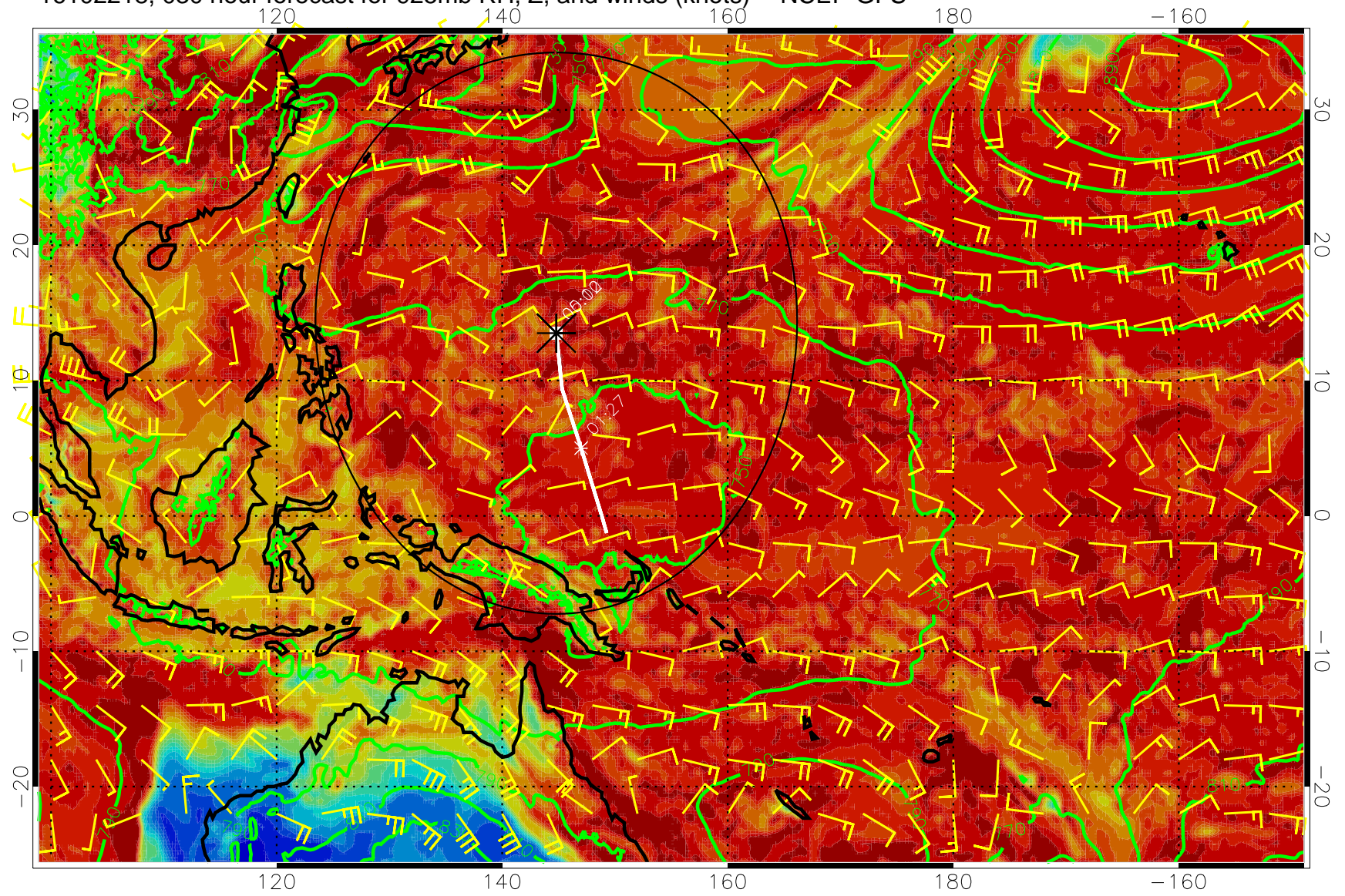
16102218, 030 hour forecast for 925mb RH, Z, and winds (knots) -- NCEP GFS
