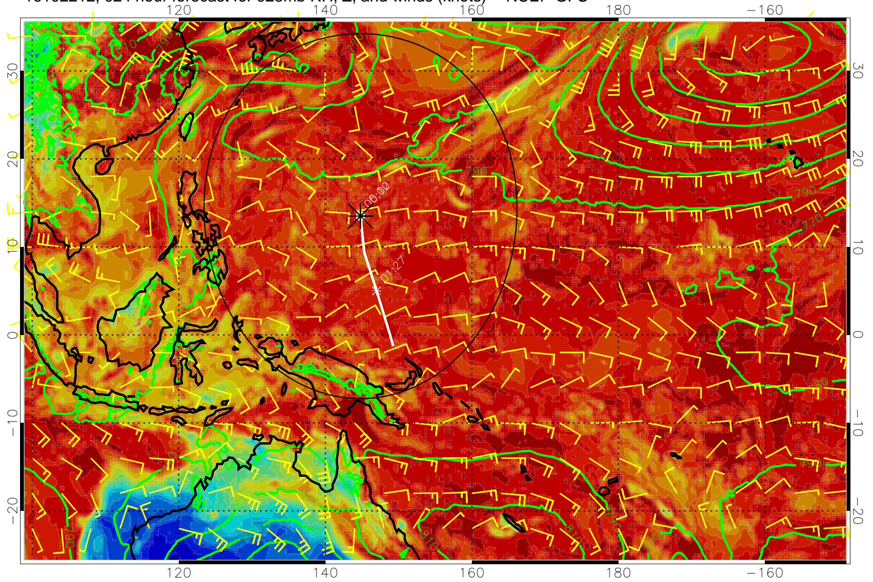
16102212, 024 hour forecast for 925mb RH, Z, and winds (knots) -- NCEP GFS
