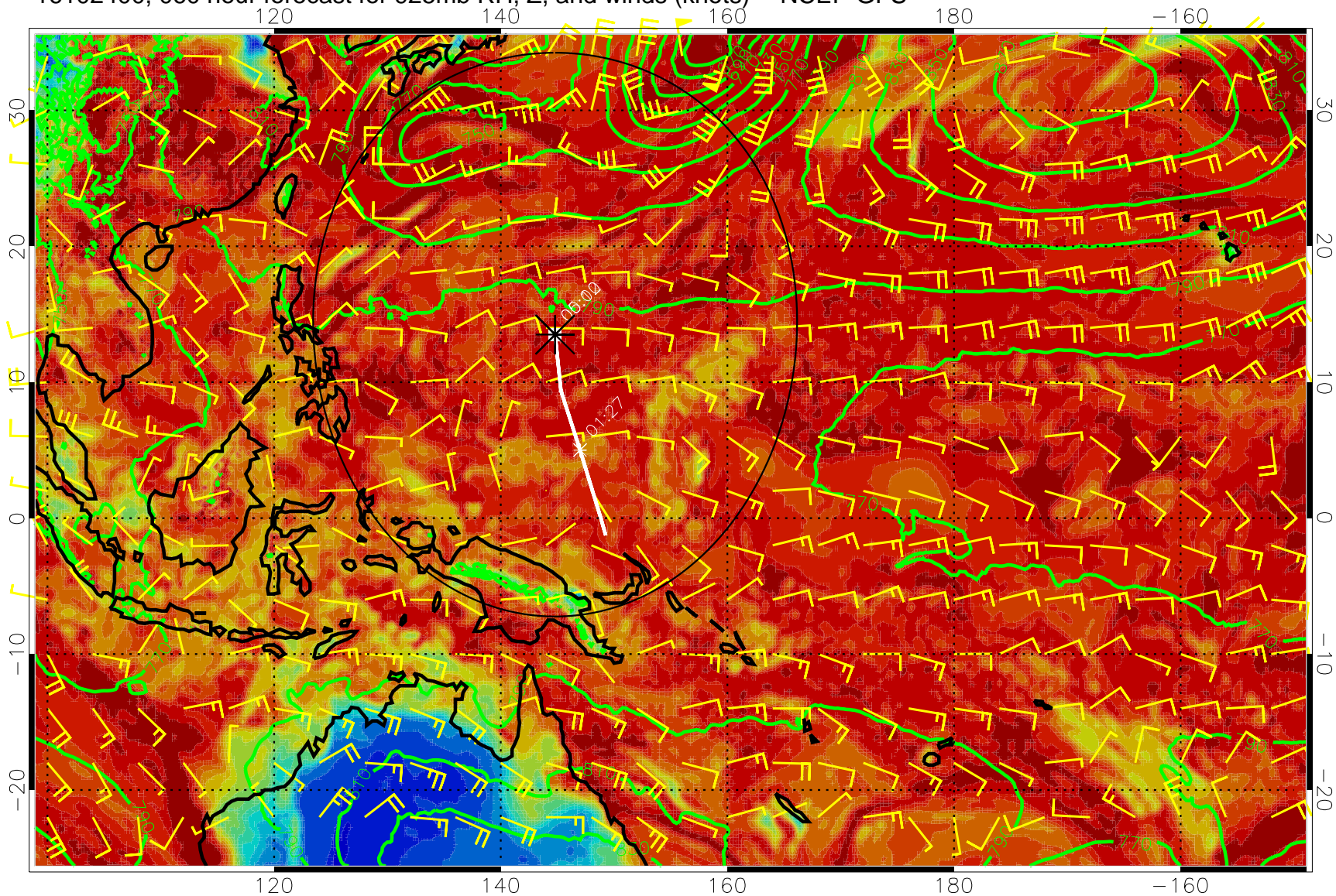
16102400, 060 hour forecast for 925mb RH, Z, and winds (knots) -- NCEP GFS
