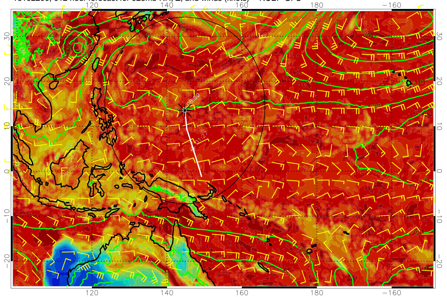
16102200, 012 hour forecast for 925mb RH, Z, and winds (knots) -- NCEP GFS
