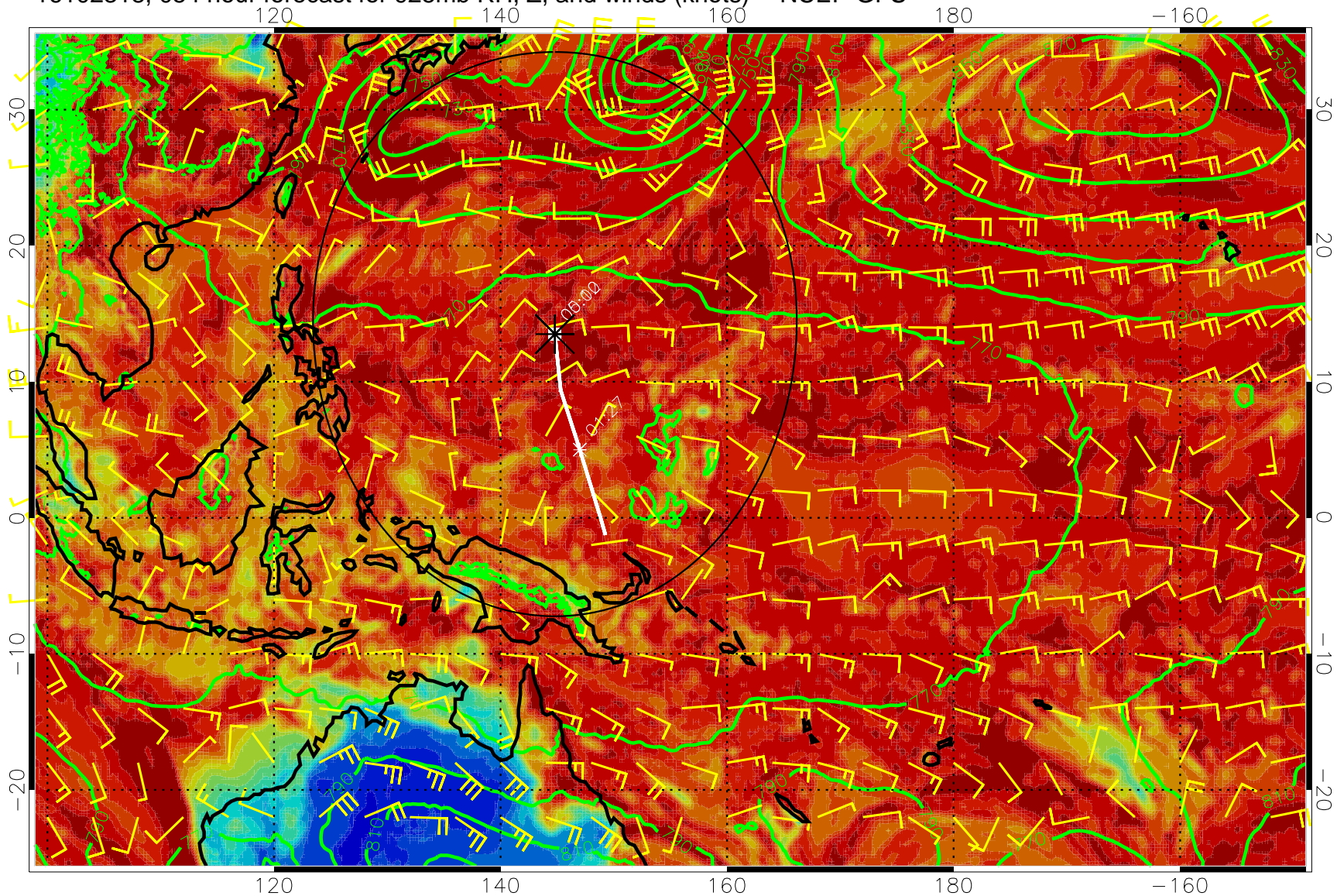
16102318, 054 hour forecast for 925mb RH, Z, and winds (knots) -- NCEP GFS
