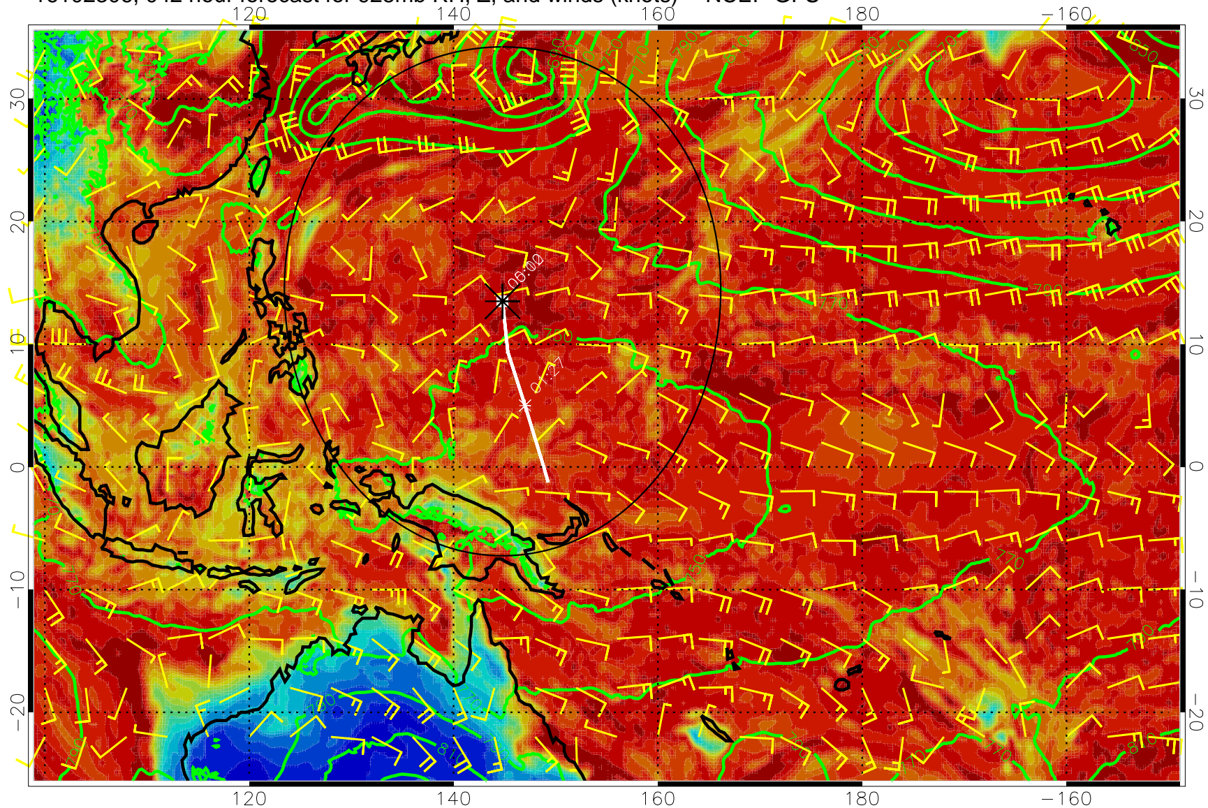
16102306, 042 hour forecast for 925mb RH, Z, and winds (knots) -- NCEP GFS
