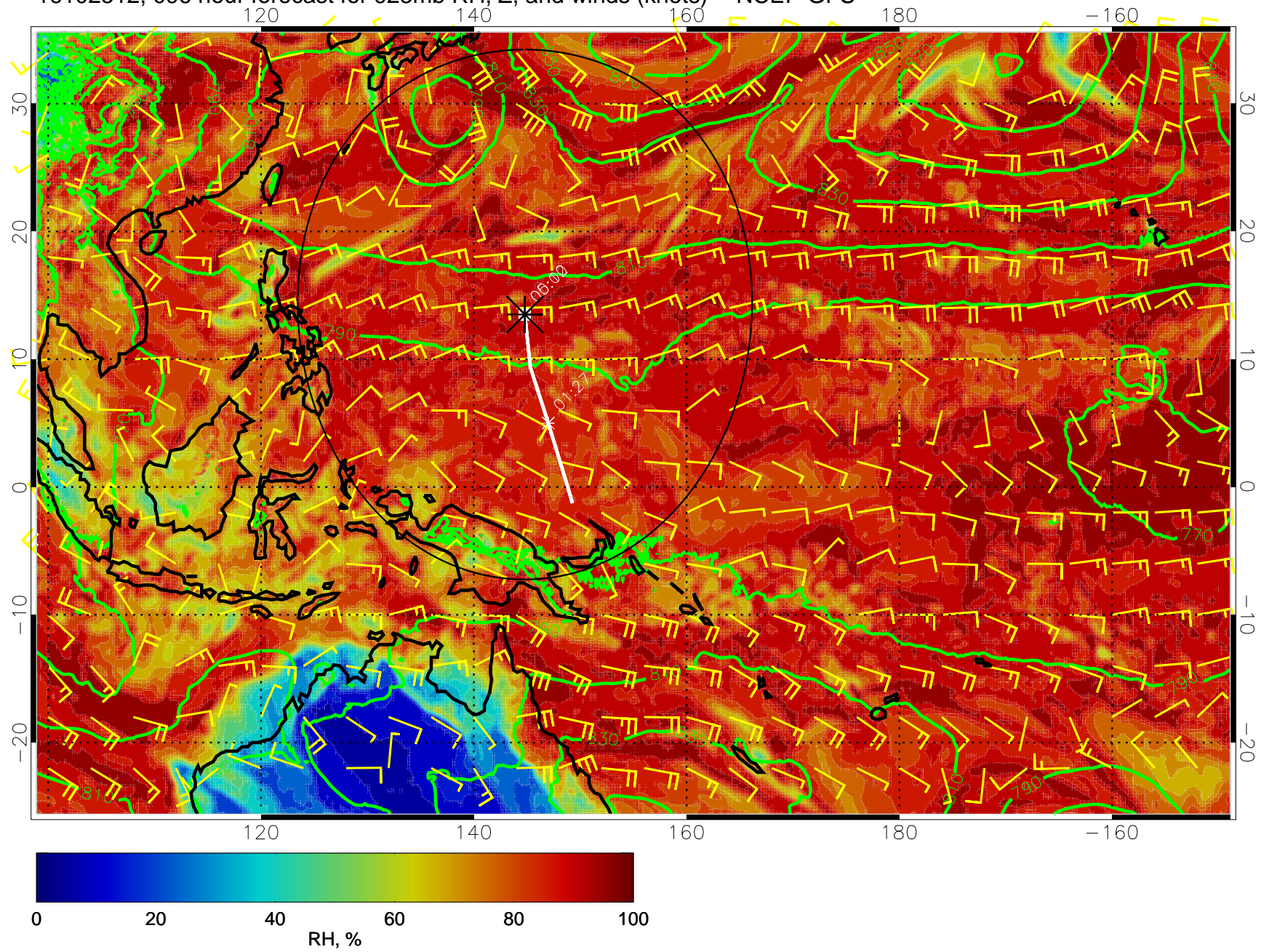
16102512, 096 hour forecast for 925mb RH, Z, and winds (knots) -- NCEP GFS
