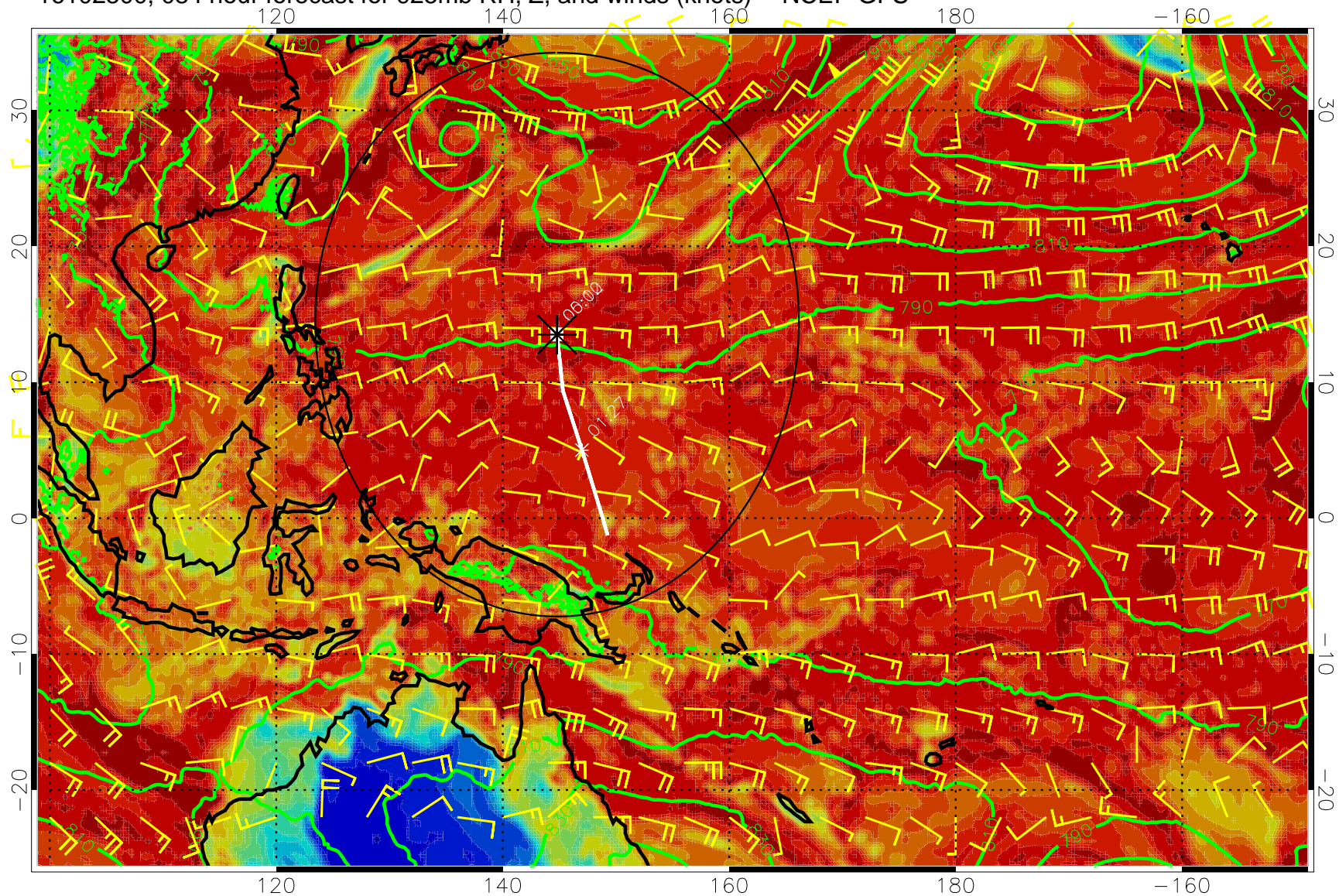
16102500, 084 hour forecast for 925mb RH, Z, and winds (knots) -- NCEP GFS
