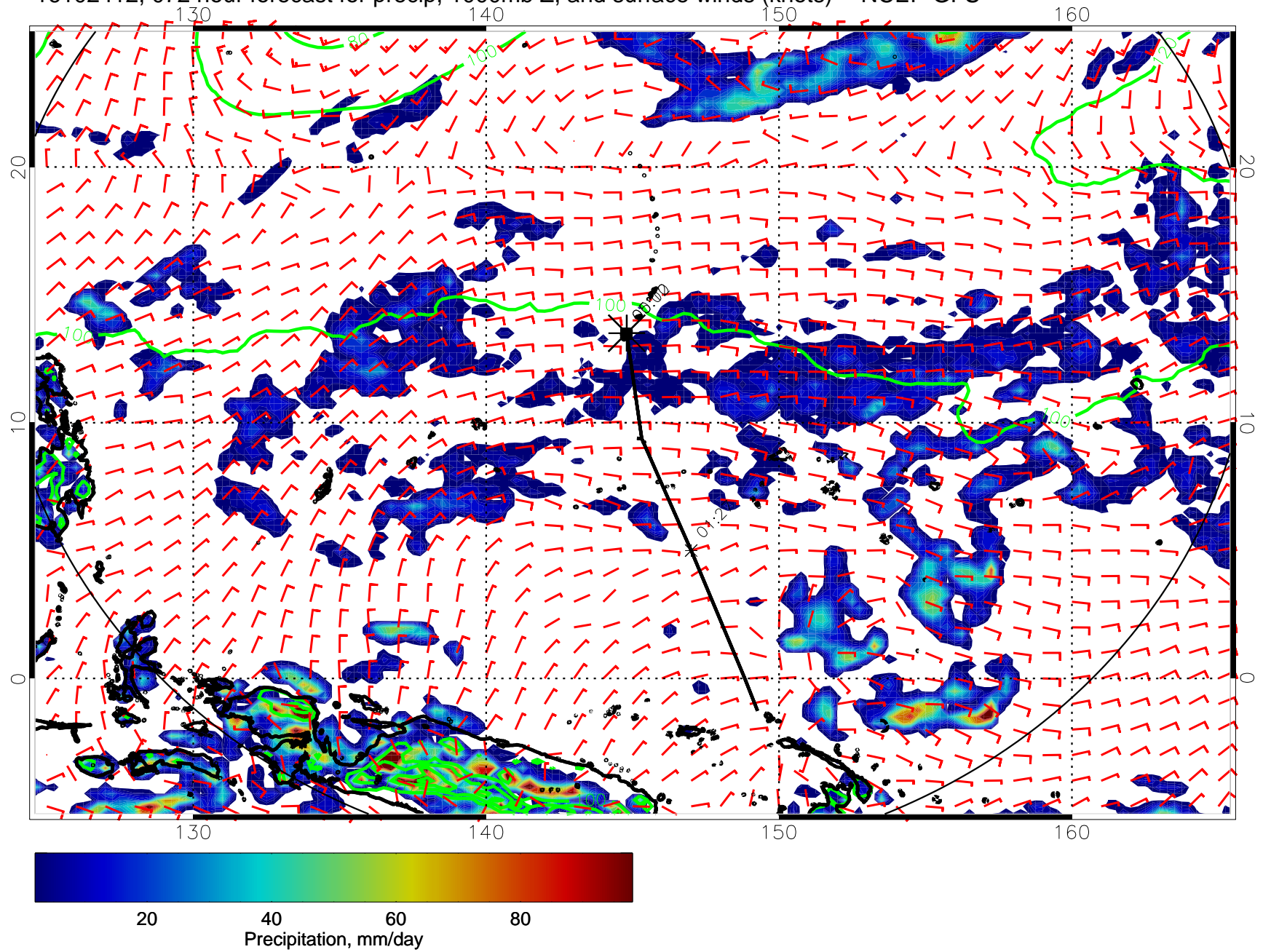
16102412, 072 hour forecast for precip, 1000mb Z, and surface winds (knots) -- NCEP GFS
