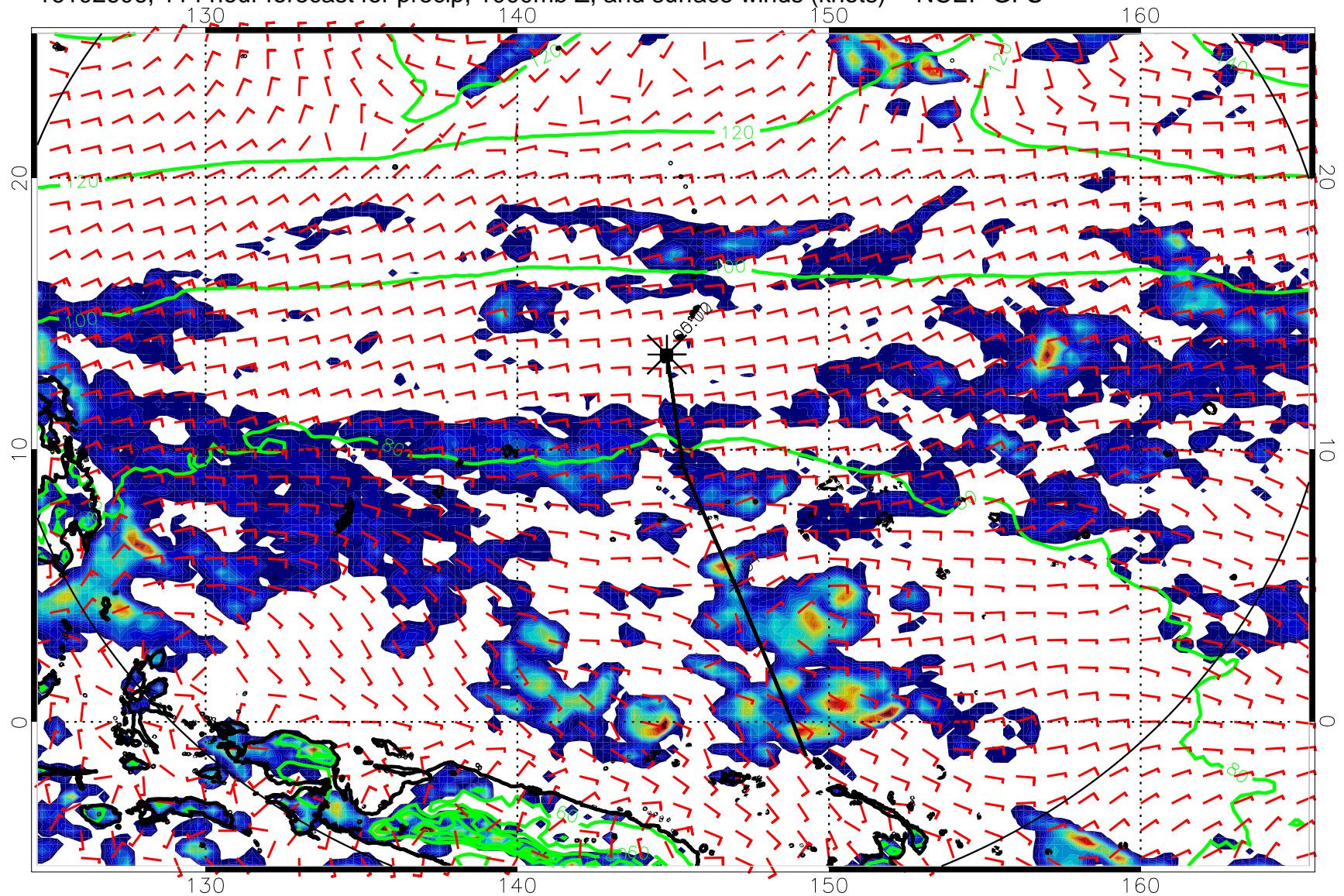
16102606, 114 hour forecast for precip, 1000mb Z, and surface winds (knots) -- NCEP GFS
