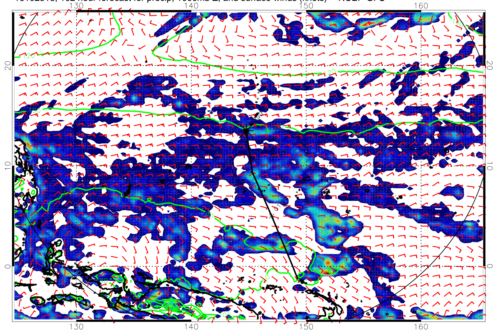
16102518, 102 hour forecast for precip, 1000mb Z, and surface winds (knots) -- NCEP GFS
