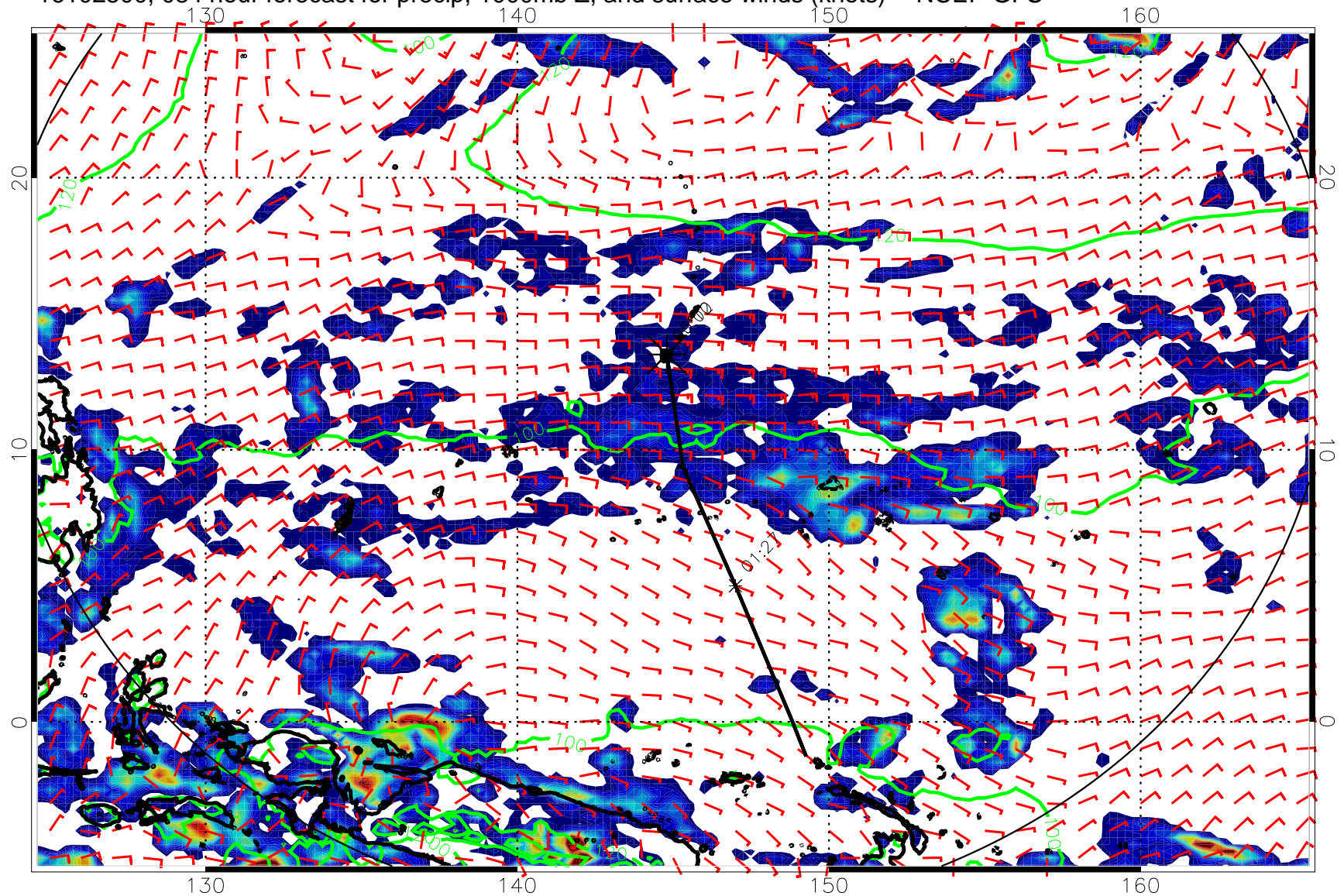
16102500, 084 hour forecast for precip, 1000mb Z, and surface winds (knots) -- NCEP GFS
