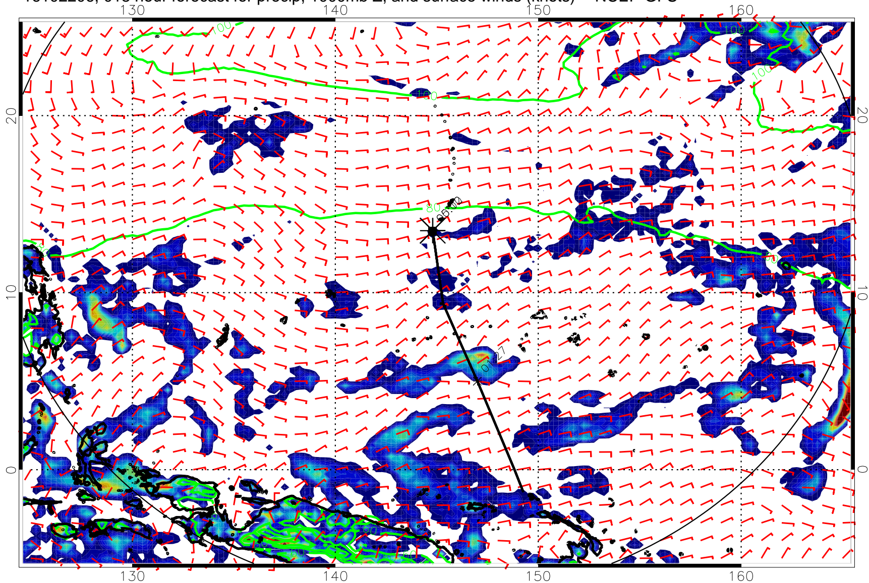
16102206, 018 hour forecast for precip, 1000mb Z, and surface winds (knots) -- NCEP GFS
