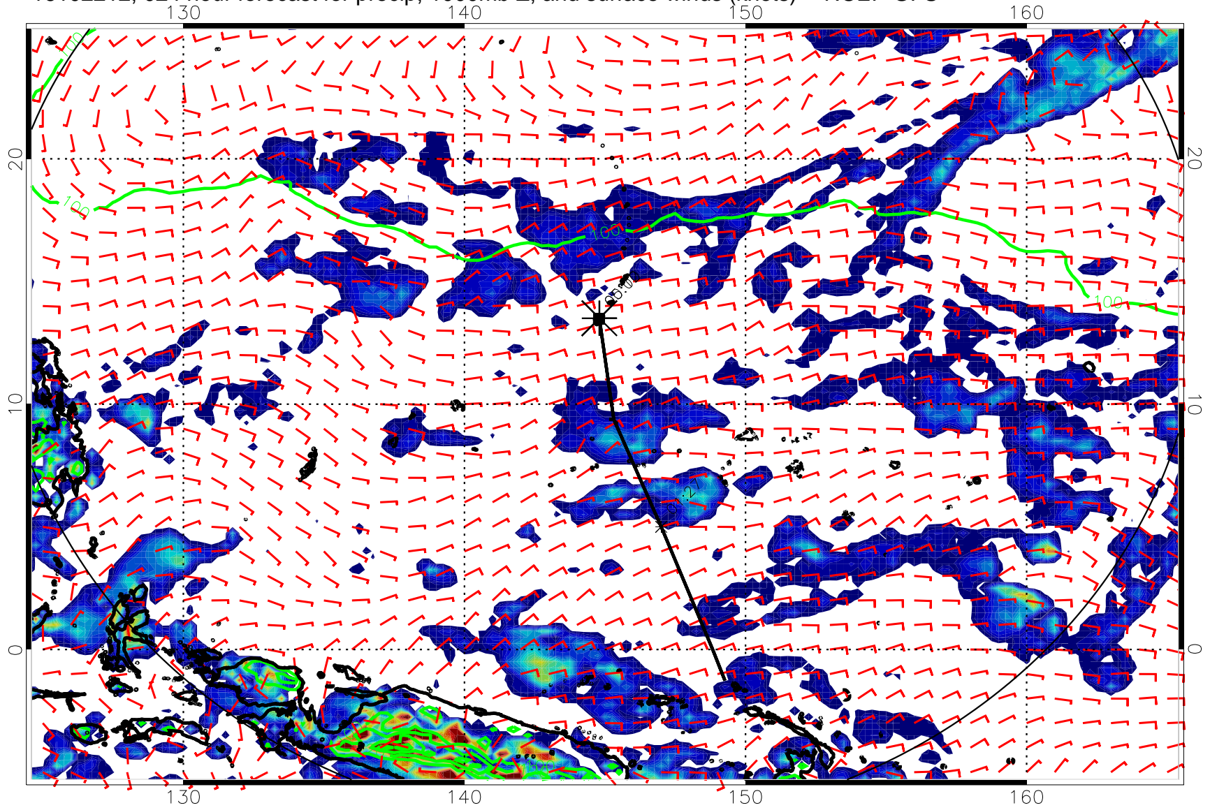
16102212, 024 hour forecast for precip, 1000mb Z, and surface winds (knots) -- NCEP GFS
