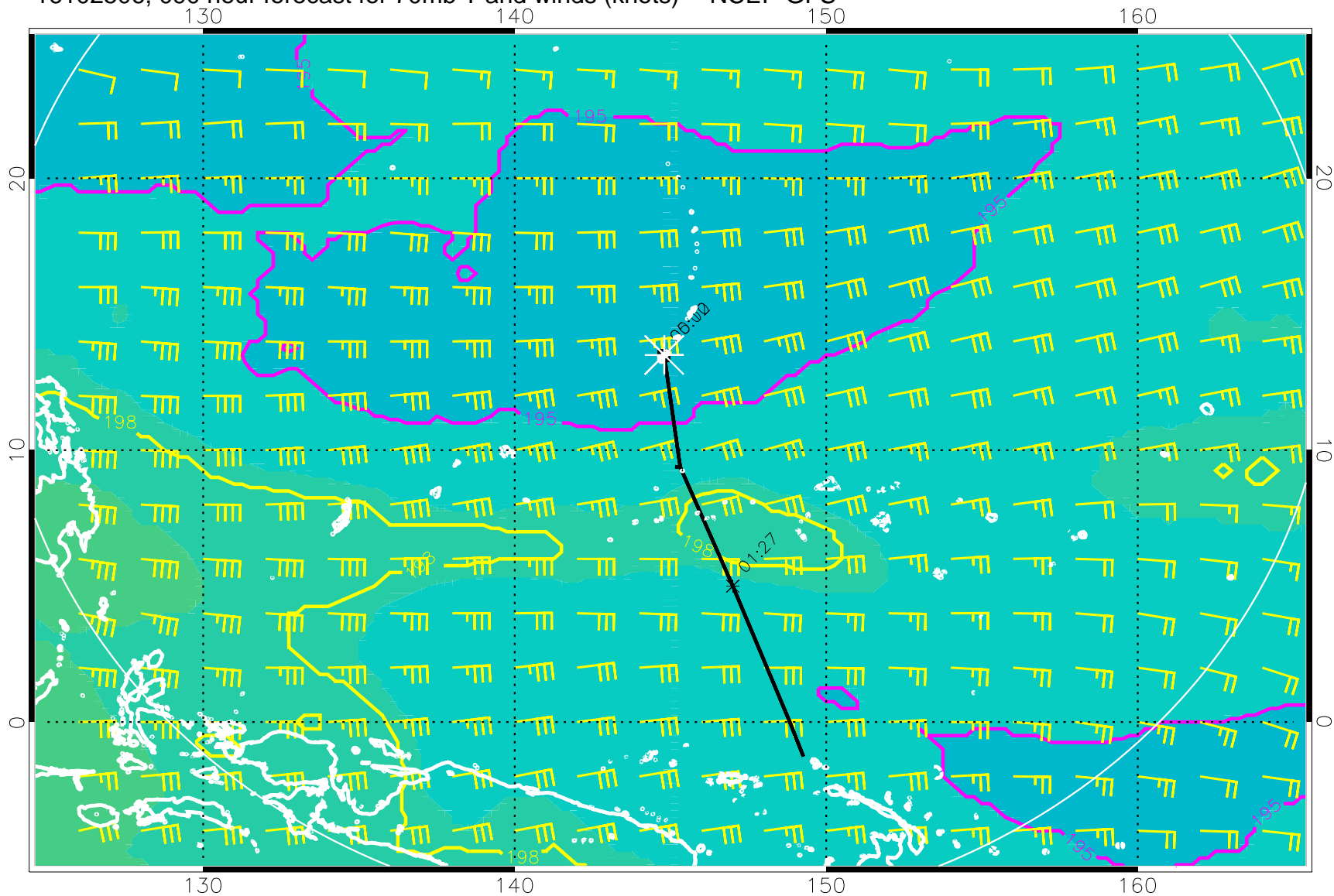
16102506, 090 hour forecast for 70mb T and winds (knots) -- NCEP GFS
