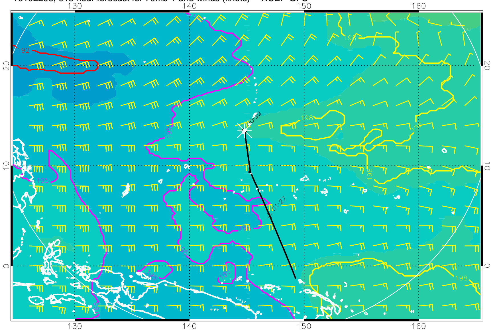
16102206, 018 hour forecast for 70mb T and winds (knots) -- NCEP GFS
