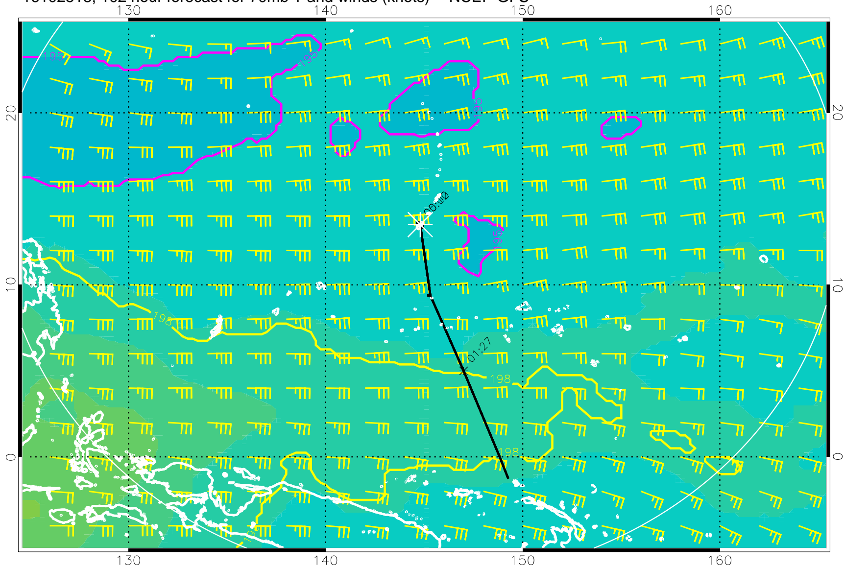
16102518, 102 hour forecast for 70mb T and winds (knots) -- NCEP GFS
