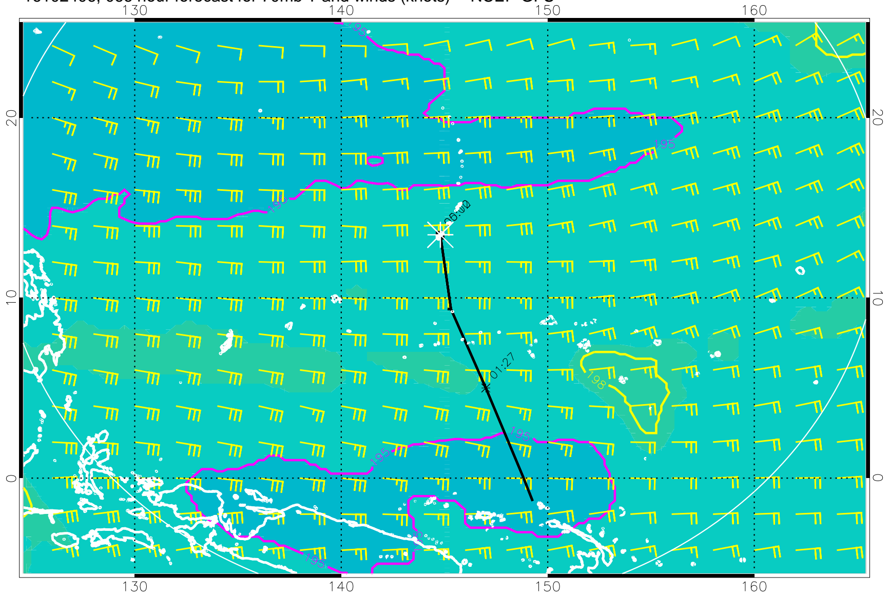
16102406, 066 hour forecast for 70mb T and winds (knots) -- NCEP GFS
