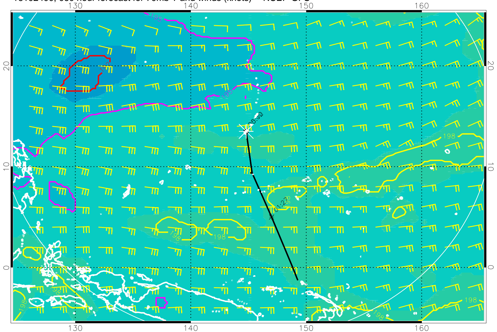
16102400, 060 hour forecast for 70mb T and winds (knots) -- NCEP GFS
