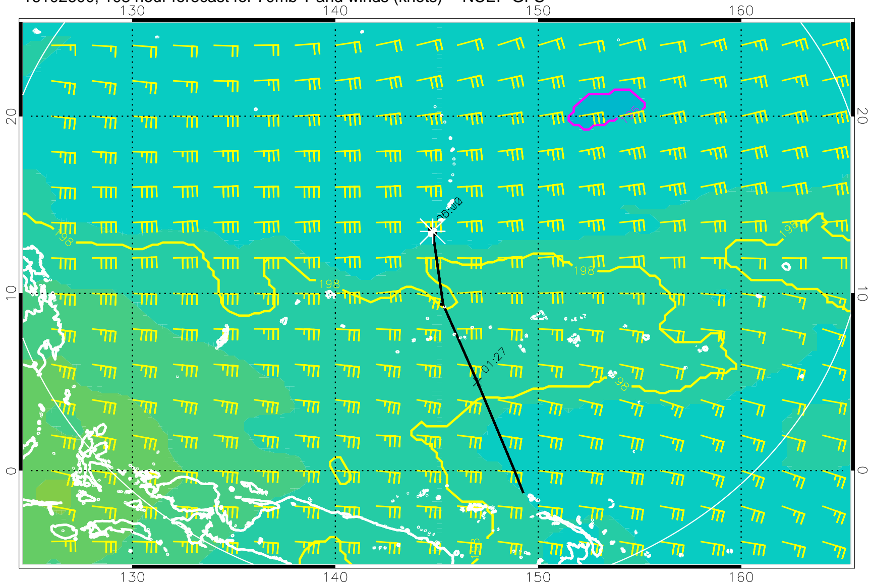
16102600, 108 hour forecast for 70mb T and winds (knots) -- NCEP GFS
