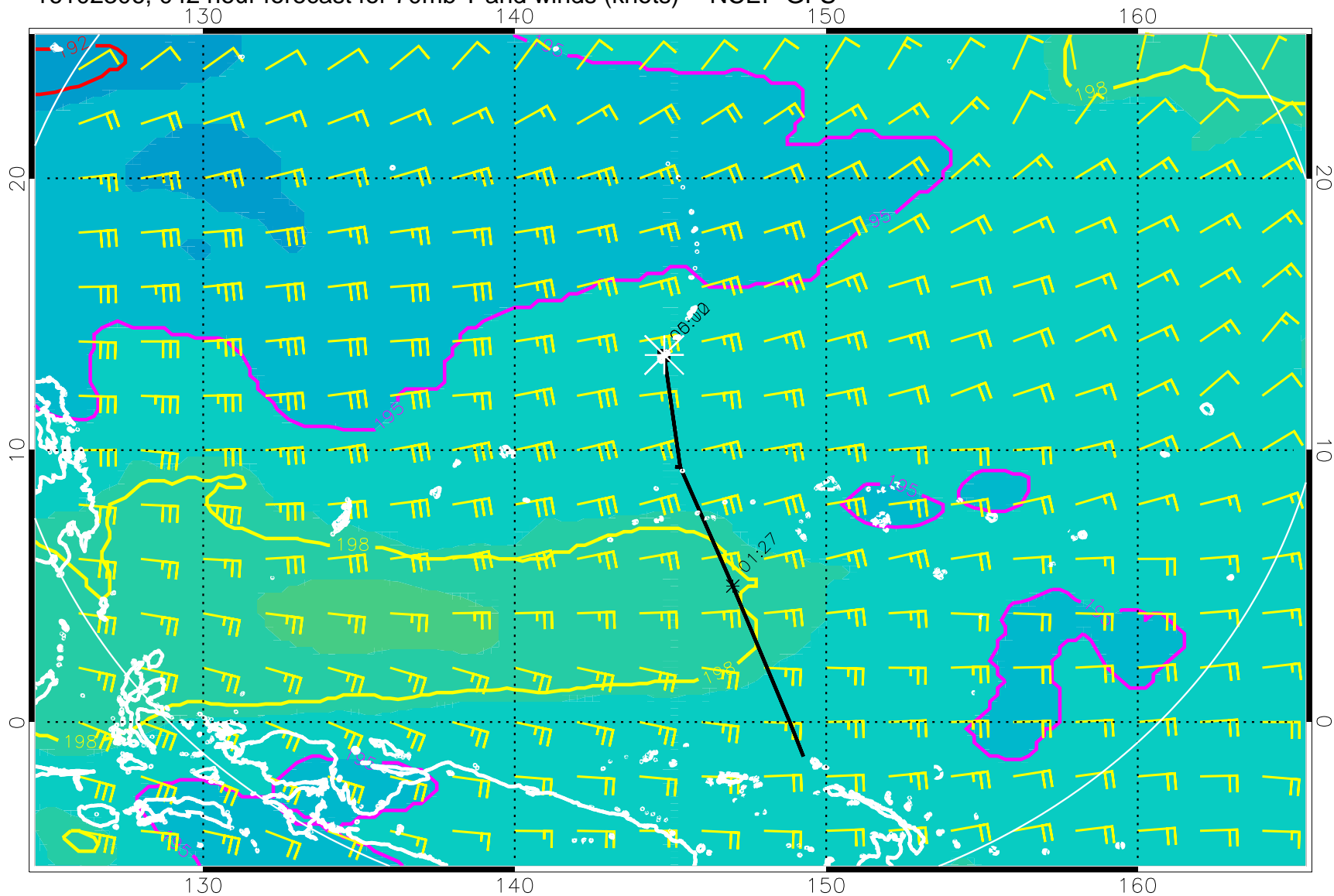
16102306, 042 hour forecast for 70mb T and winds (knots) -- NCEP GFS
