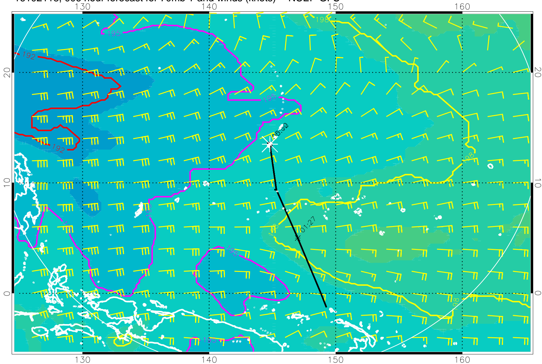
16102118, 006 hour forecast for 70mb T and winds (knots) -- NCEP GFS
