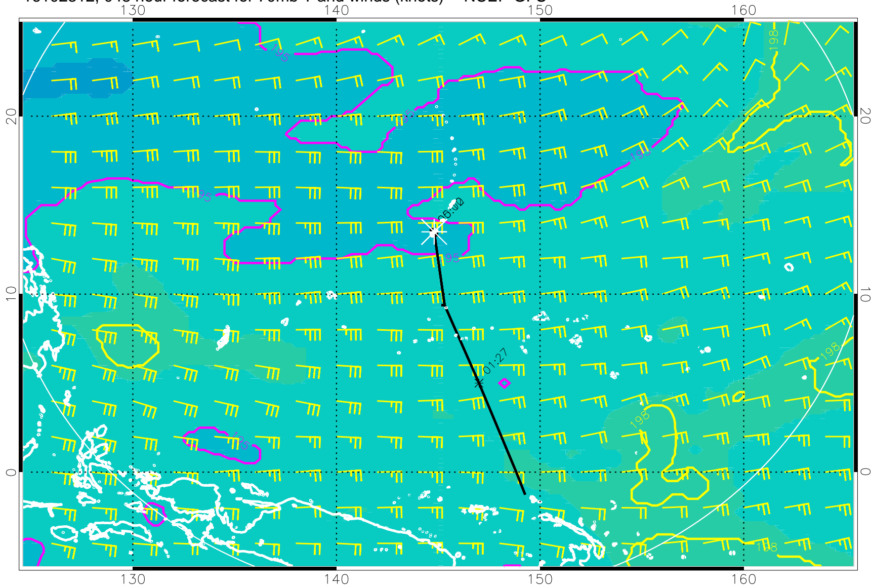
16102312, 048 hour forecast for 70mb T and winds (knots) -- NCEP GFS
