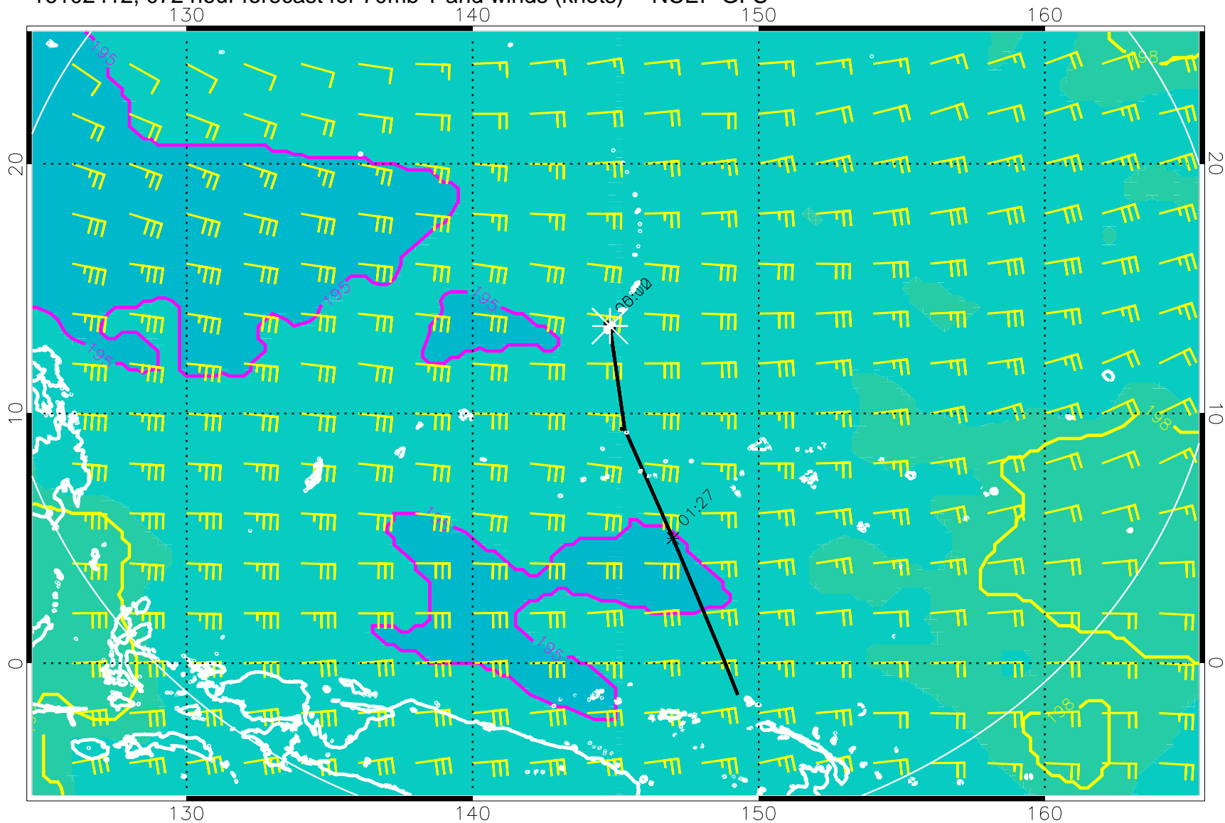
16102412, 072 hour forecast for 70mb T and winds (knots) -- NCEP GFS
