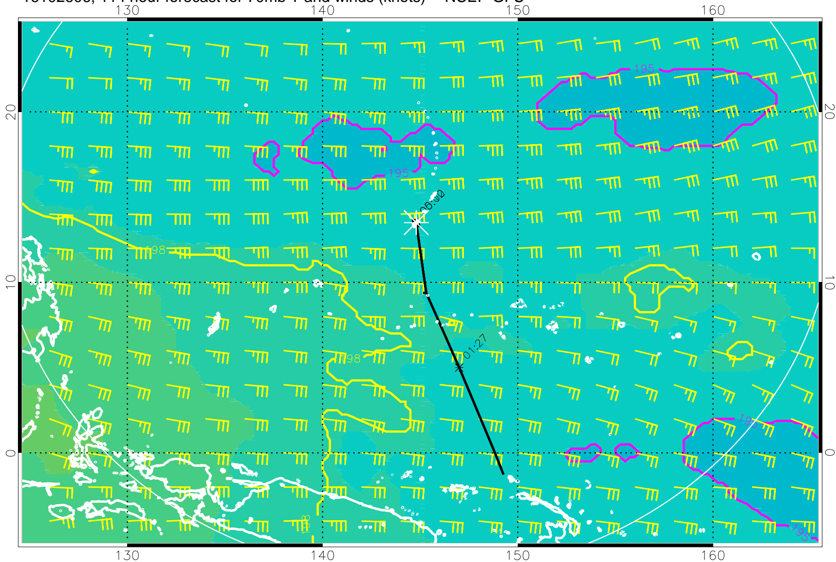
16102606, 114 hour forecast for 70mb T and winds (knots) -- NCEP GFS
