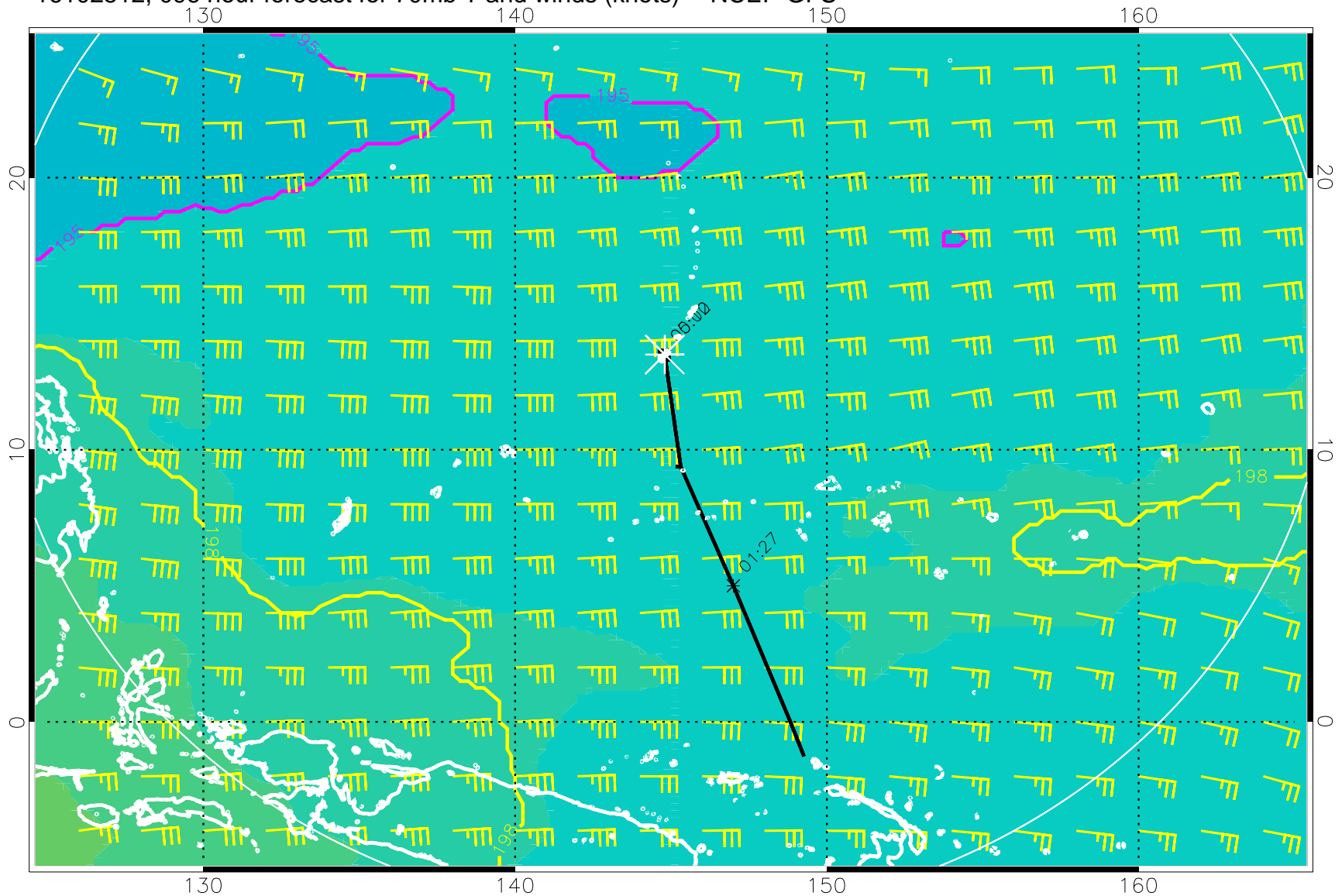
16102512, 096 hour forecast for 70mb T and winds (knots) -- NCEP GFS
