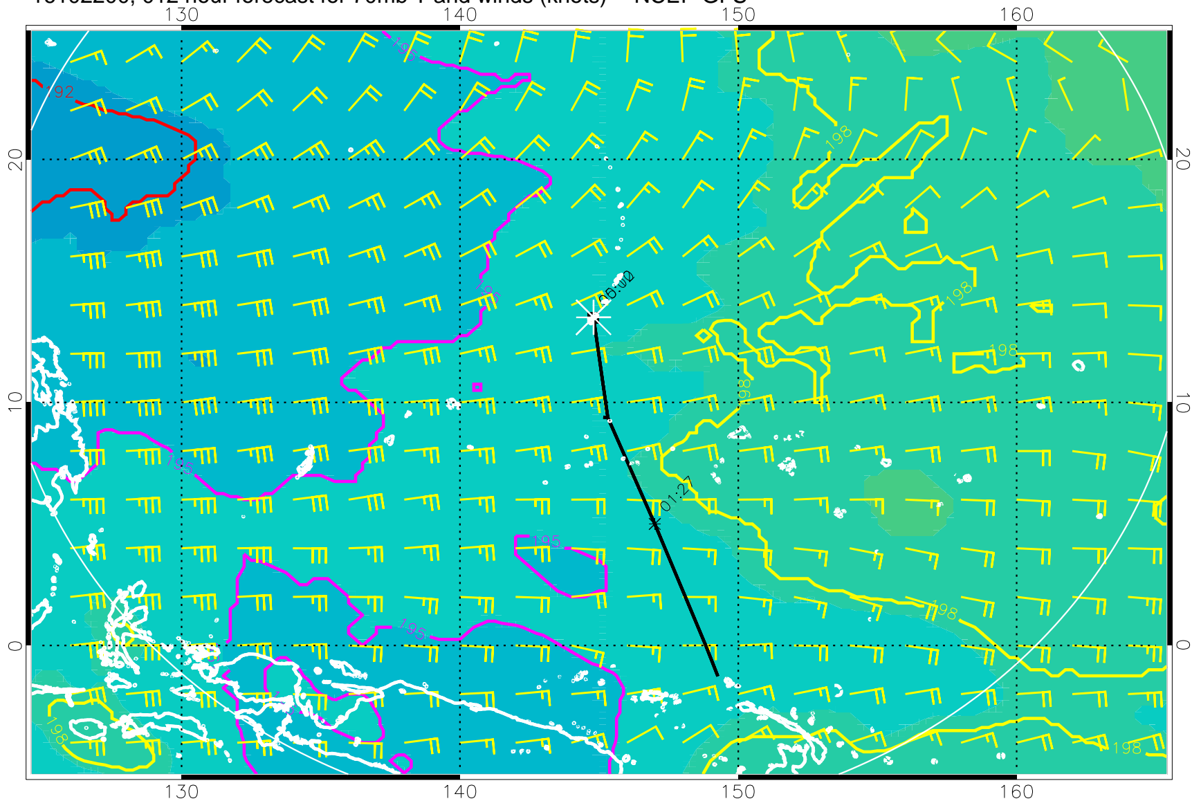
16102200, 012 hour forecast for 70mb T and winds (knots) -- NCEP GFS
