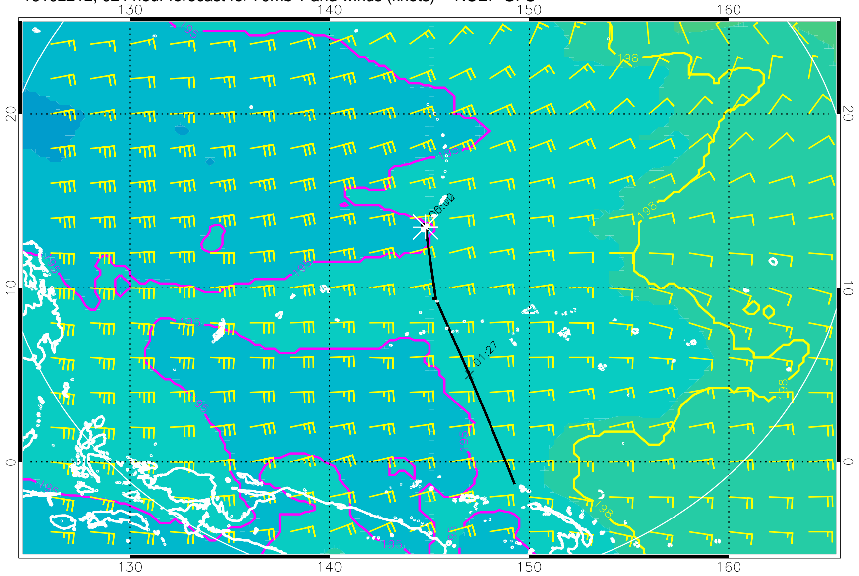
16102212, 024 hour forecast for 70mb T and winds (knots) -- NCEP GFS
