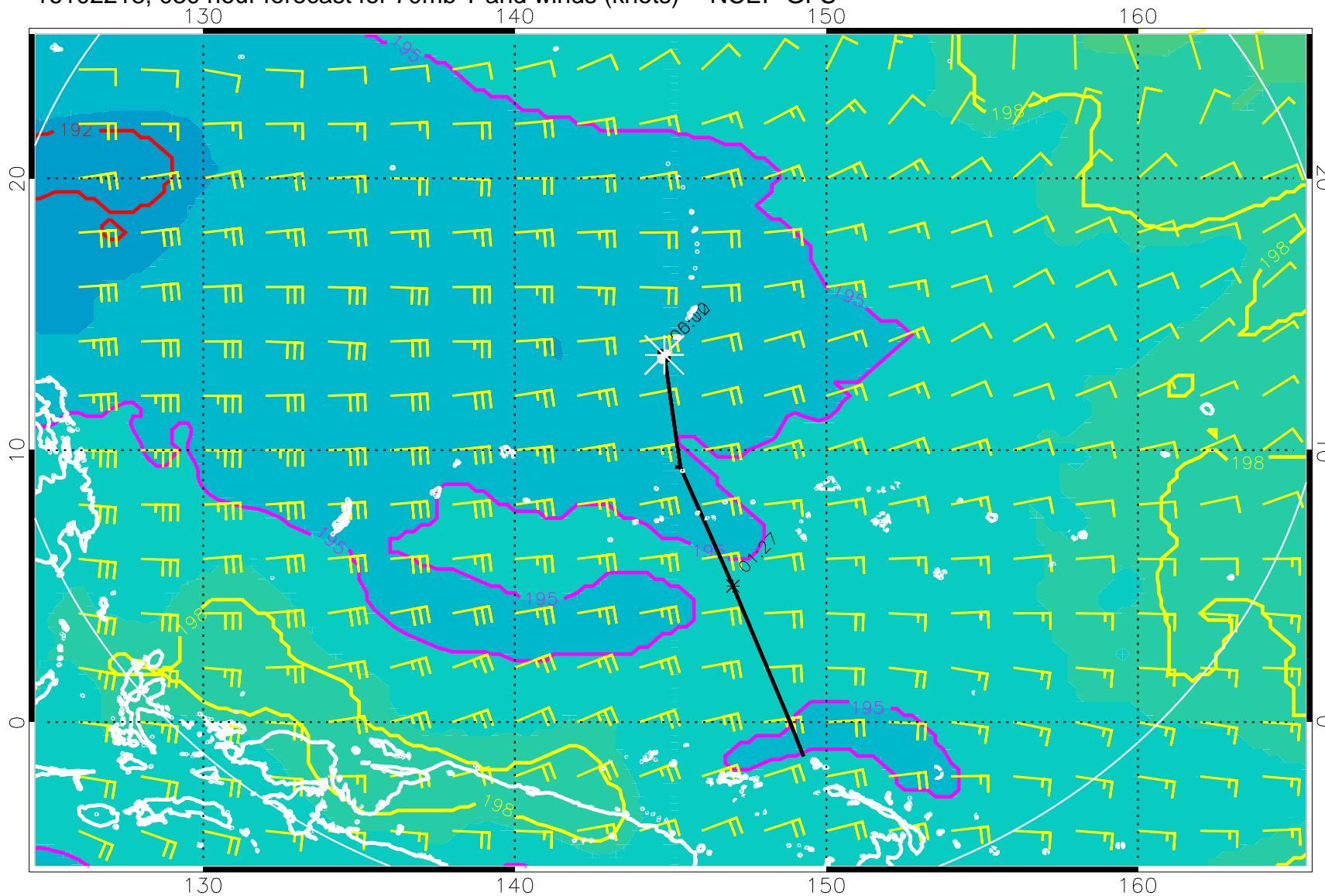
16102218, 030 hour forecast for 70mb T and winds (knots) -- NCEP GFS
