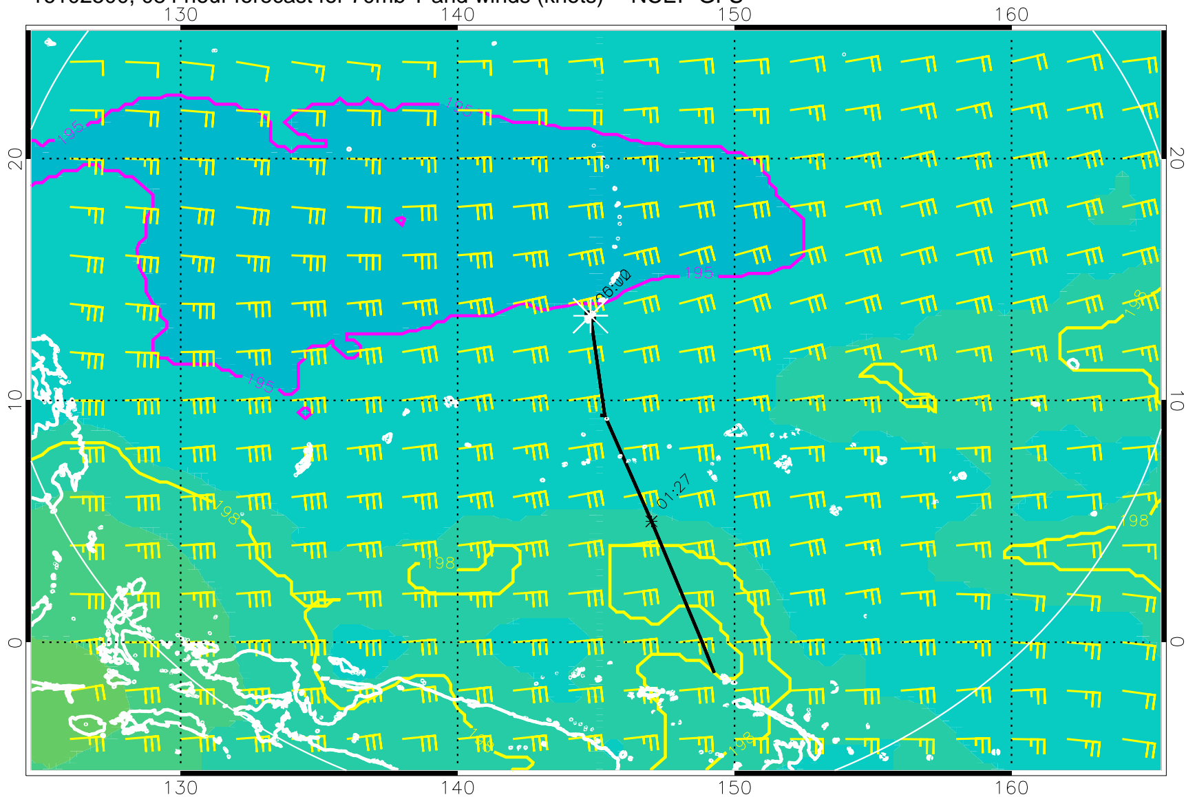
16102500, 084 hour forecast for 70mb T and winds (knots) -- NCEP GFS
