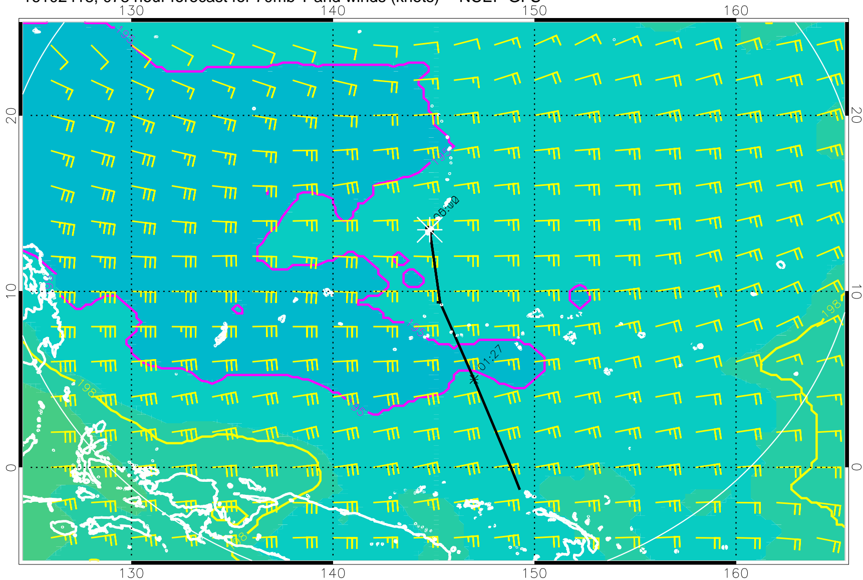
16102418, 078 hour forecast for 70mb T and winds (knots) -- NCEP GFS
