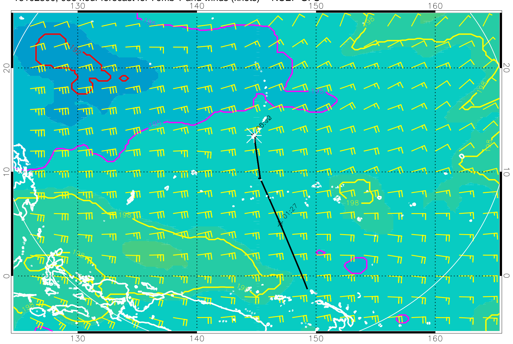
16102300, 036 hour forecast for 70mb T and winds (knots) -- NCEP GFS
