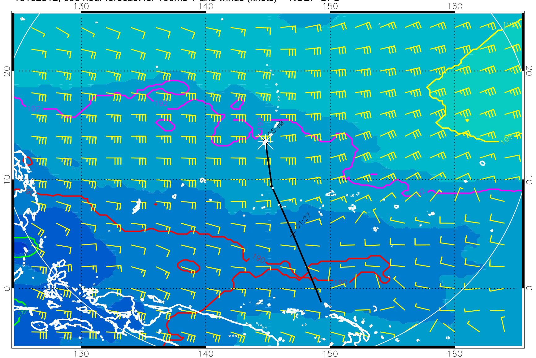
16102512, 096 hour forecast for 100mb T and winds (knots) -- NCEP GFS
