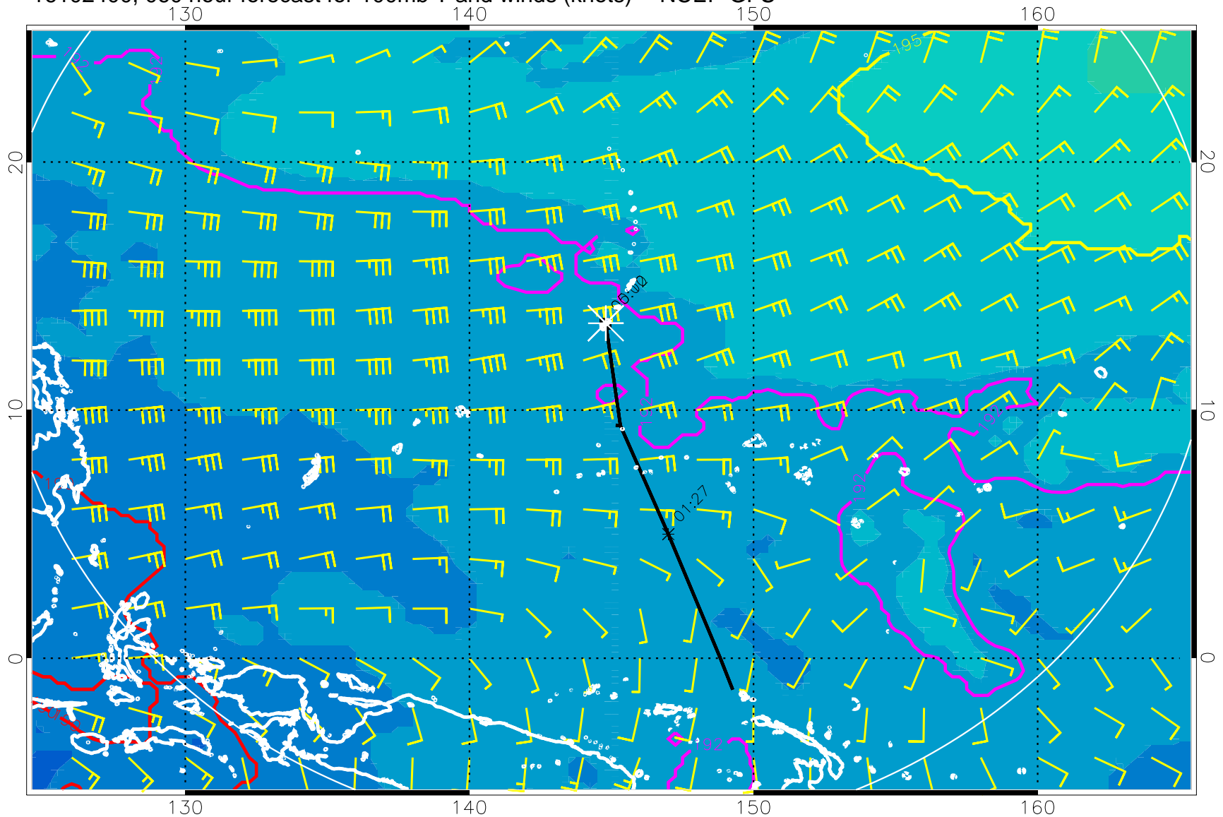
16102400, 060 hour forecast for 100mb T and winds (knots) -- NCEP GFS
