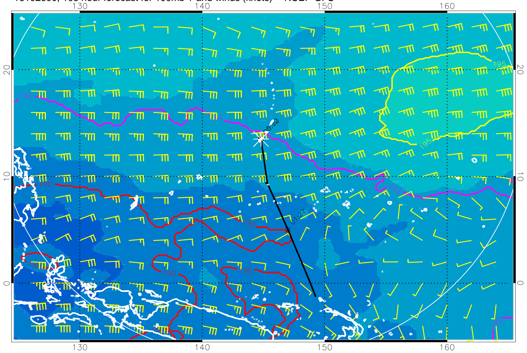
16102600, 108 hour forecast for 100mb T and winds (knots) -- NCEP GFS
