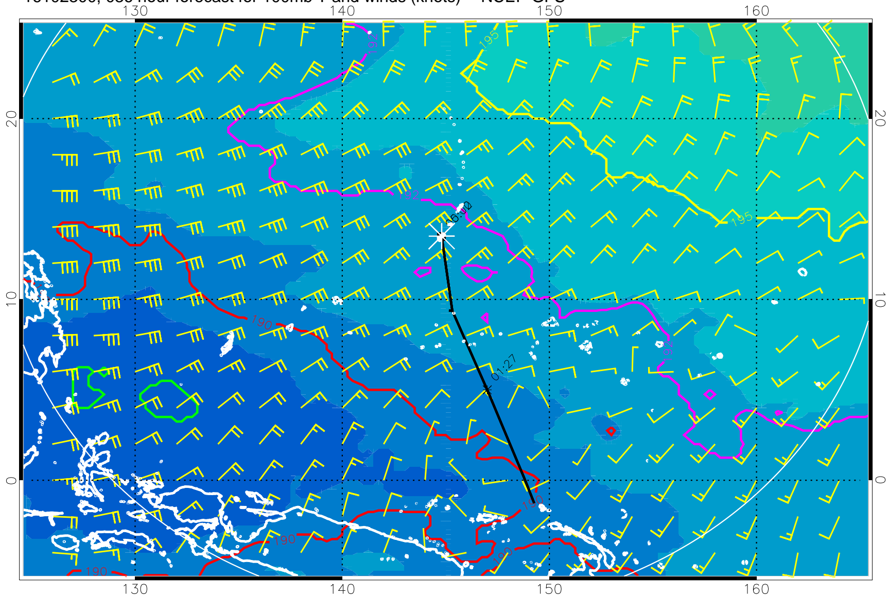
16102300, 036 hour forecast for 100mb T and winds (knots) -- NCEP GFS
