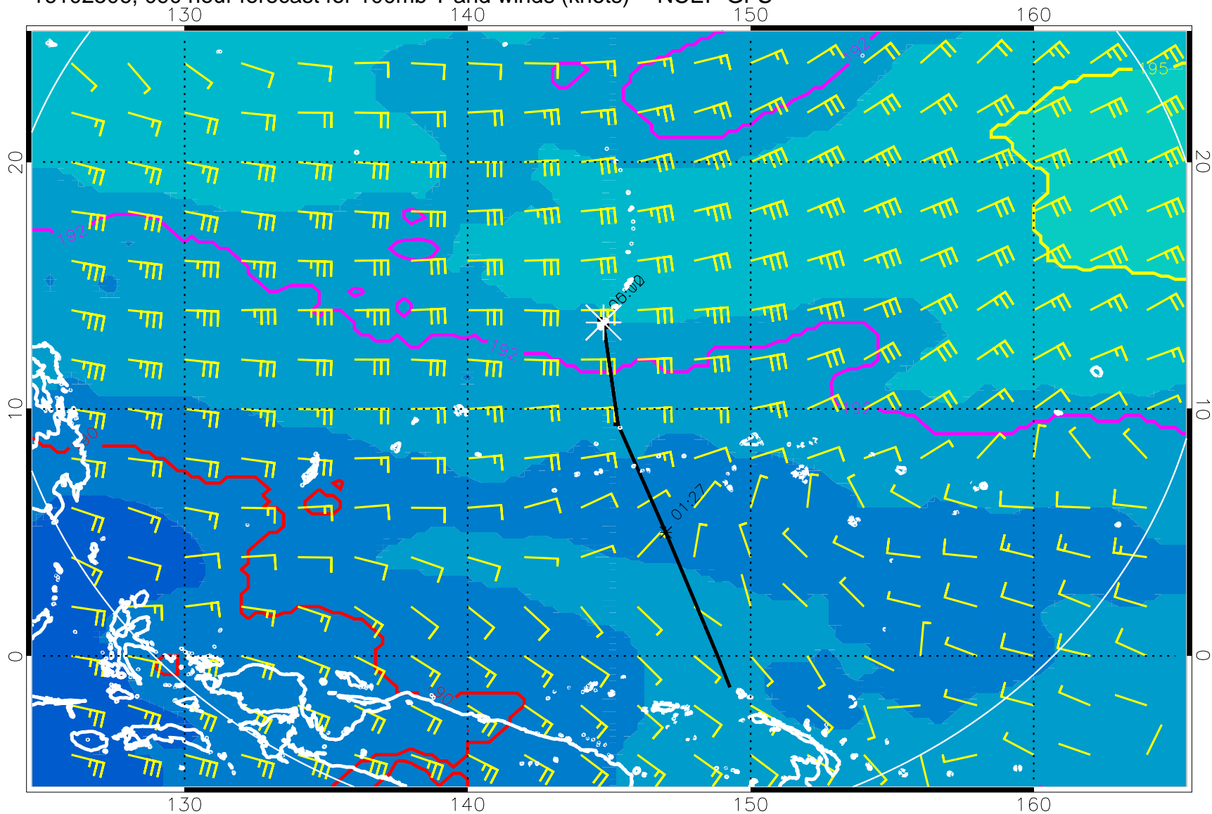
16102506, 090 hour forecast for 100mb T and winds (knots) -- NCEP GFS
