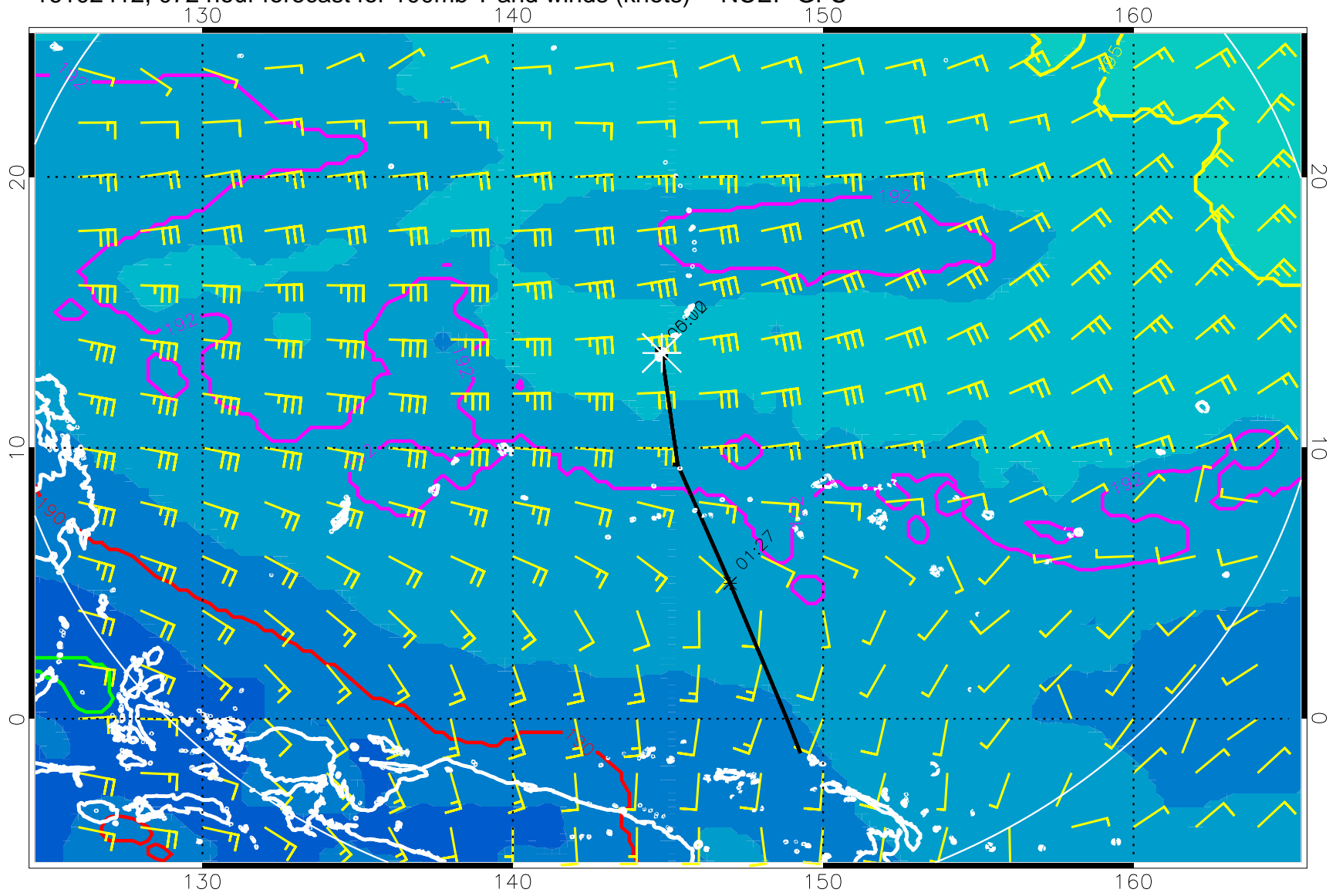
16102412, 072 hour forecast for 100mb T and winds (knots) -- NCEP GFS
