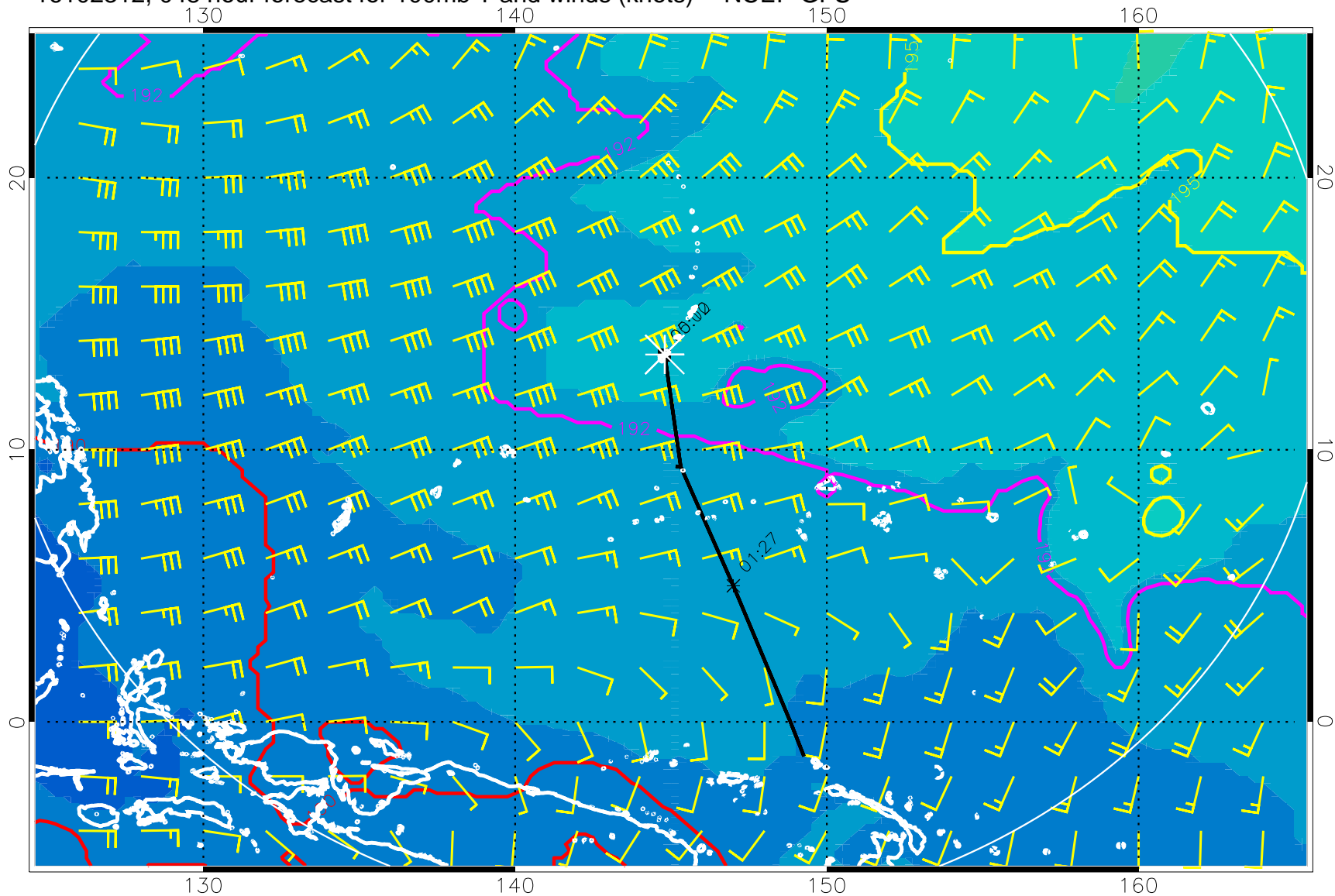
16102312, 048 hour forecast for 100mb T and winds (knots) -- NCEP GFS
