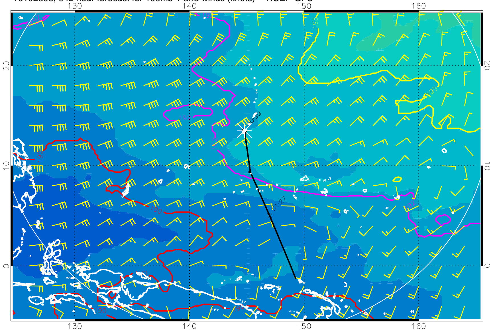
16102306, 042 hour forecast for 100mb T and winds (knots) -- NCEP GFS
