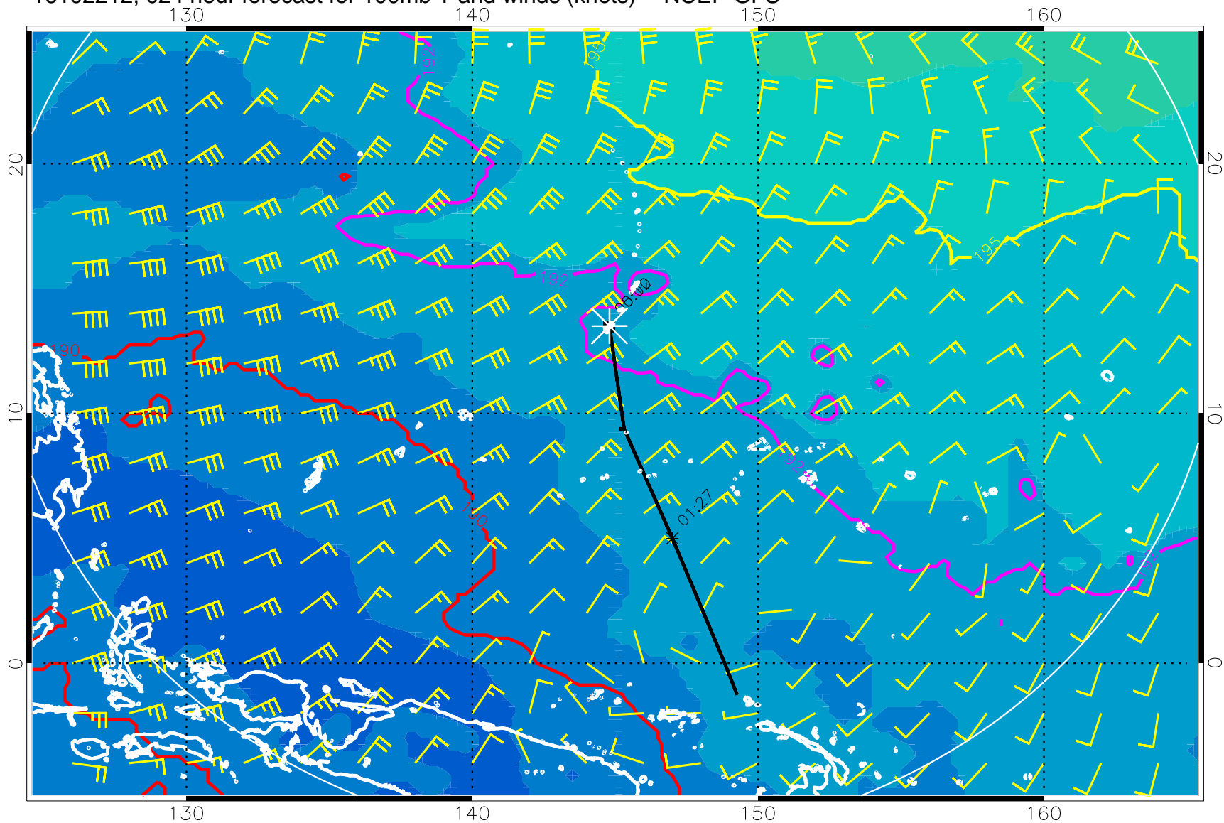
16102212, 024 hour forecast for 100mb T and winds (knots) -- NCEP GFS
