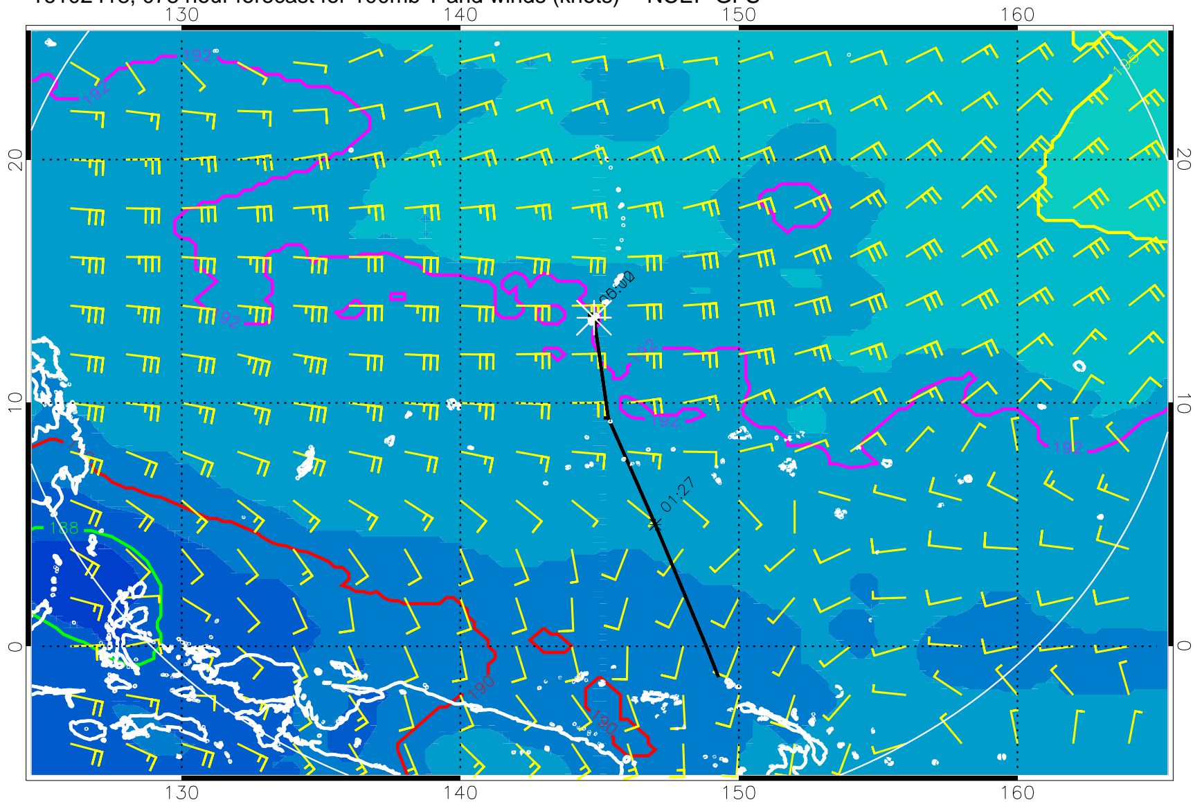
16102418, 078 hour forecast for 100mb T and winds (knots) -- NCEP GFS
