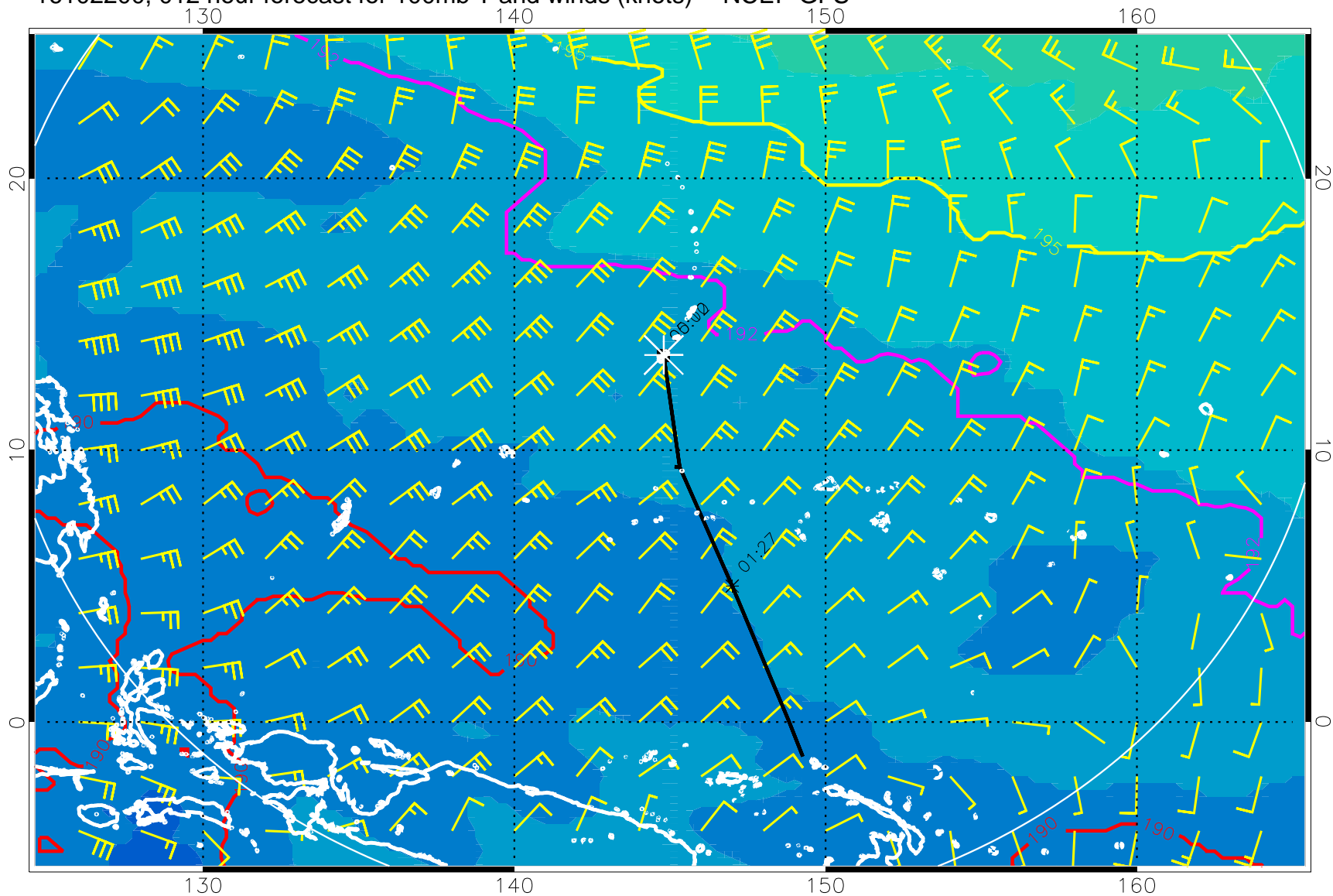
16102200, 012 hour forecast for 100mb T and winds (knots) -- NCEP GFS
