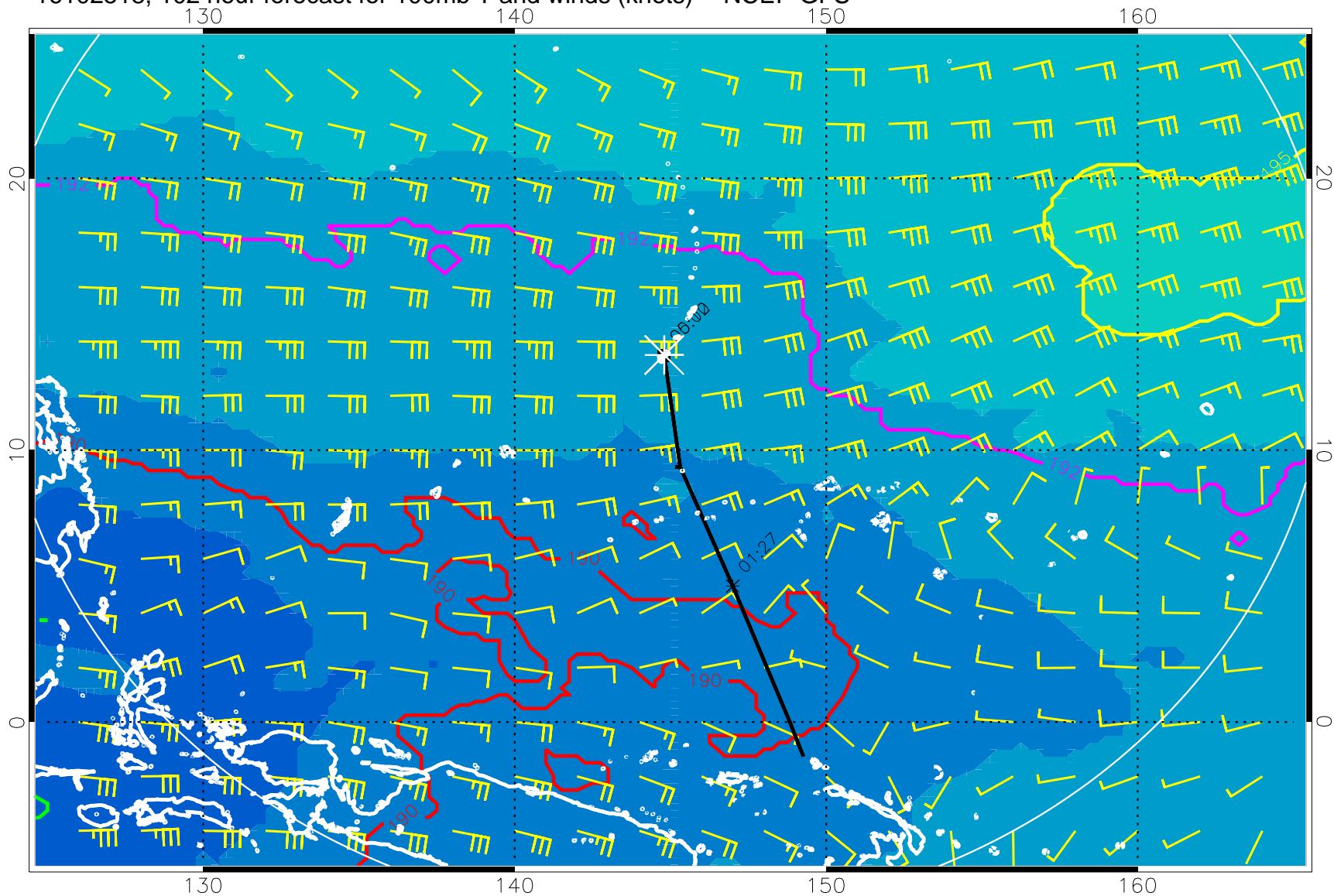
16102518, 102 hour forecast for 100mb T and winds (knots) -- NCEP GFS
