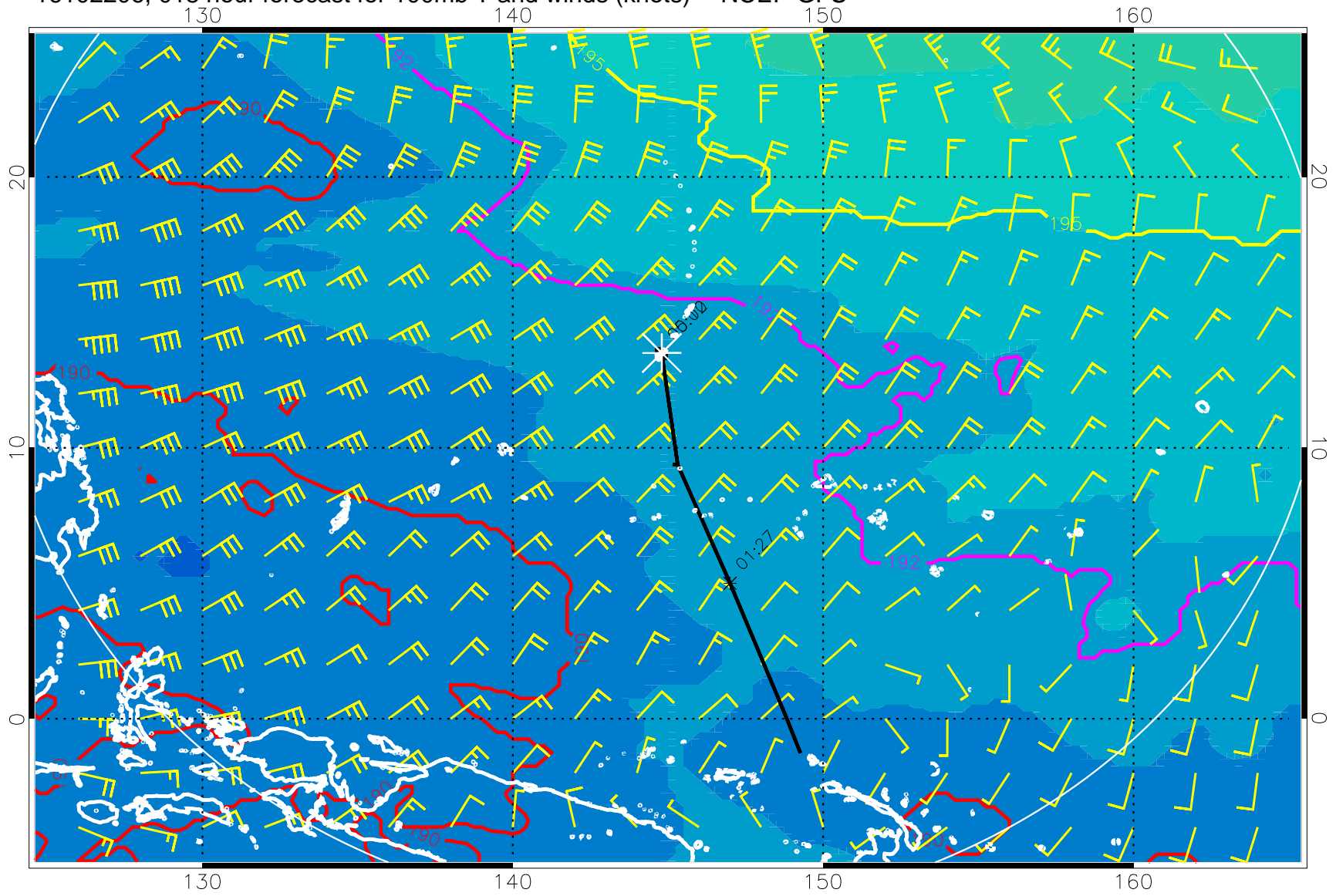
16102206, 018 hour forecast for 100mb T and winds (knots) -- NCEP GFS
