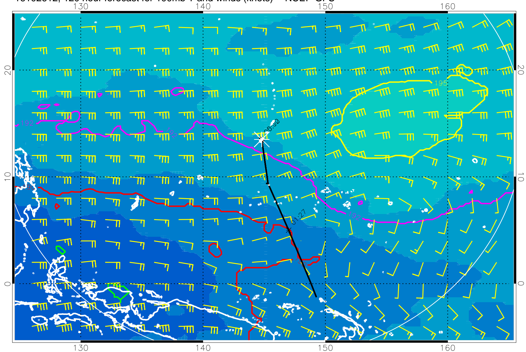
16102612, 120 hour forecast for 100mb T and winds (knots) -- NCEP GFS
