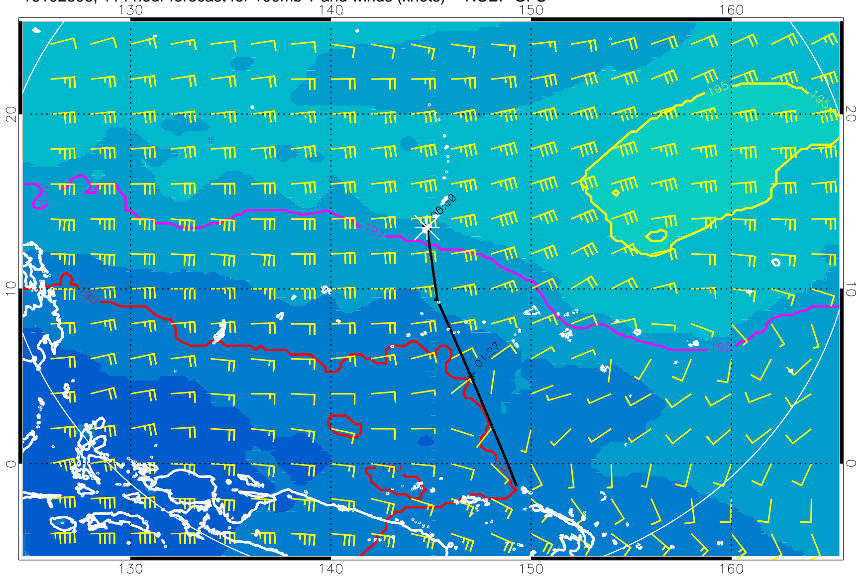
16102606, 114 hour forecast for 100mb T and winds (knots) -- NCEP GFS
